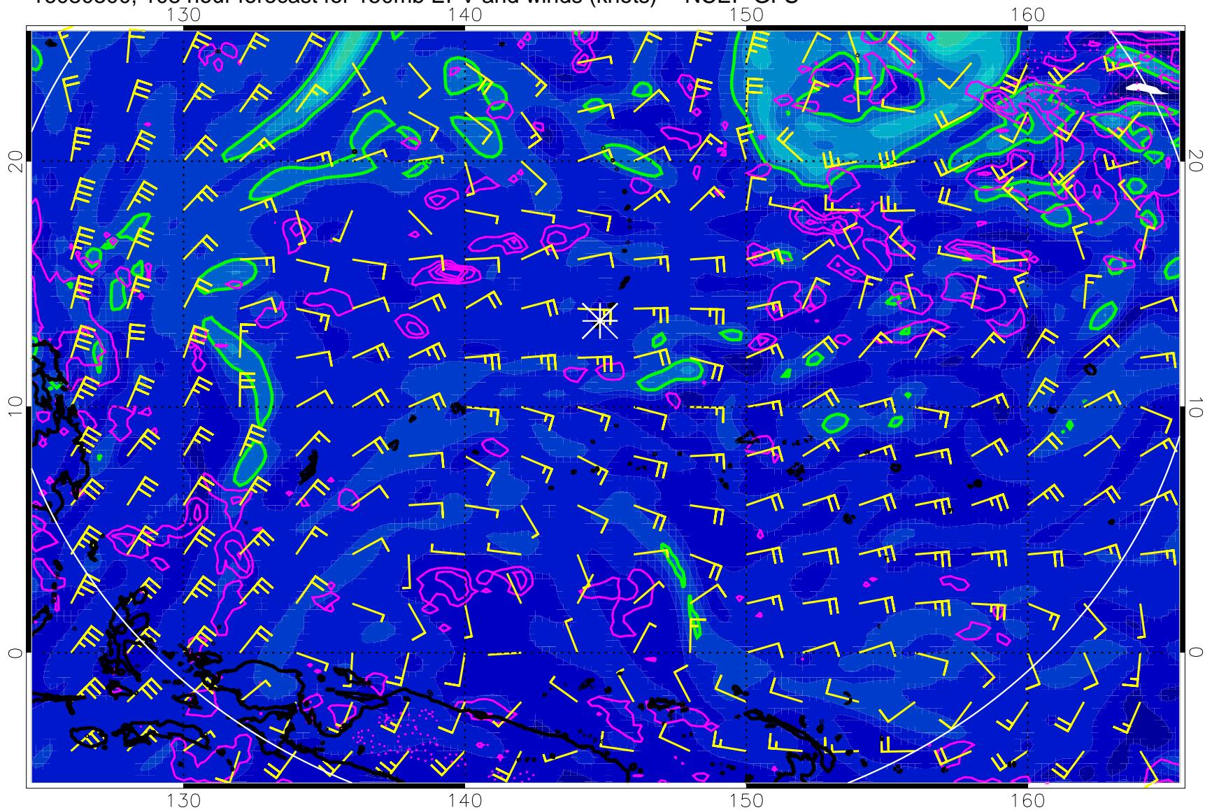
16080300, 108 hour forecast for 150mb EPV and winds (knots) -- NCEP GFS
