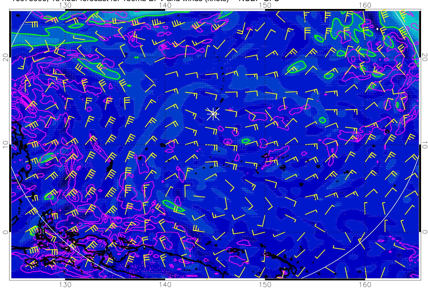
16073006, 18 hour forecast for 150mb EPV and winds (knots) -- NCEP GFS
