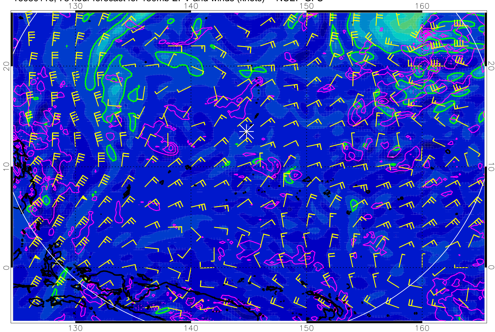
16080118, 78 hour forecast for 150mb EPV and winds (knots) -- NCEP GFS
