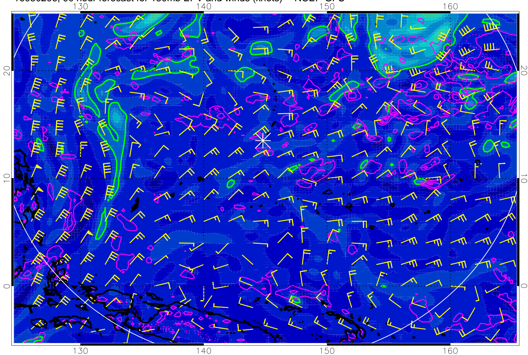
16080206, 90 hour forecast for 150mb EPV and winds (knots) -- NCEP GFS
