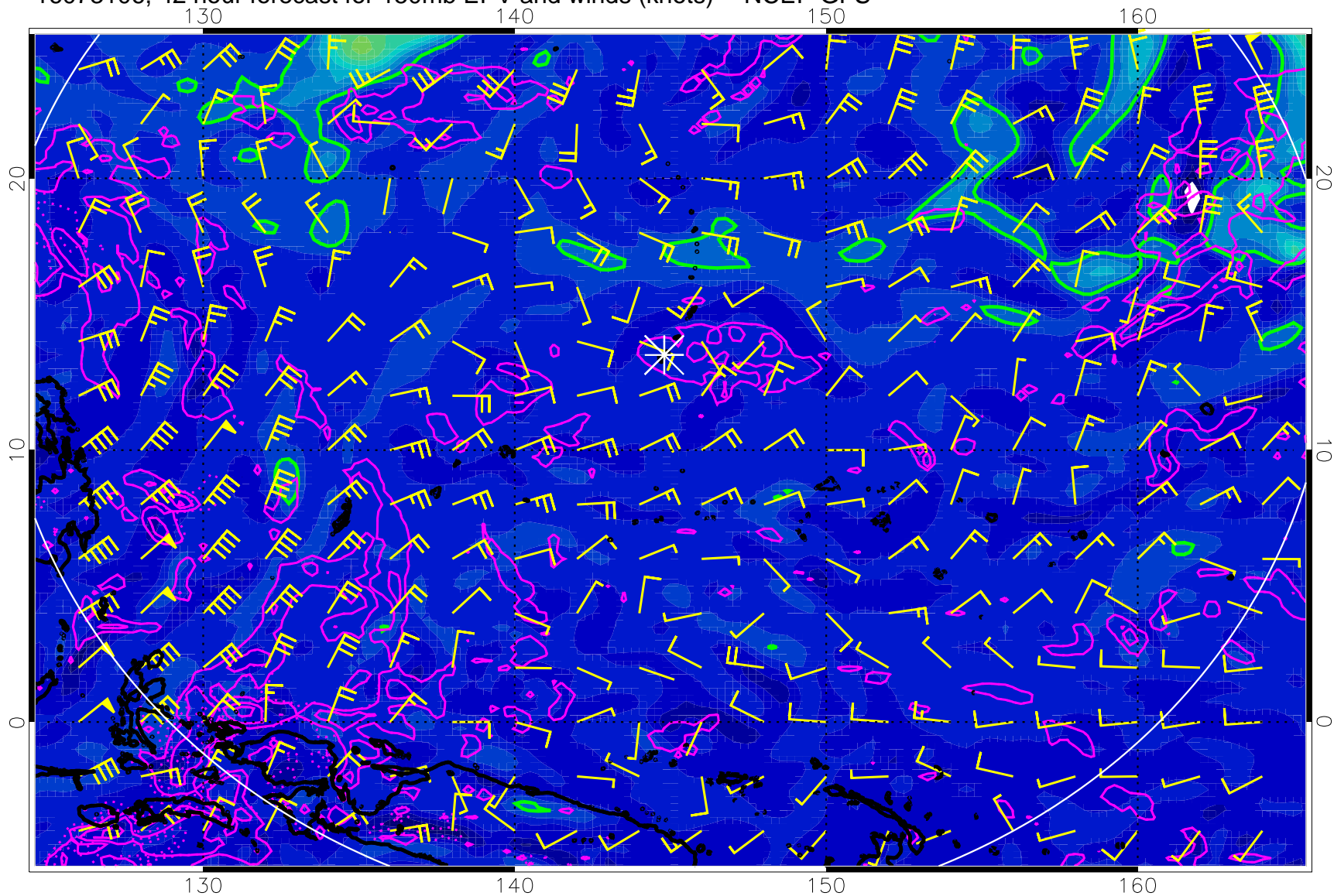
16073106, 42 hour forecast for 150mb EPV and winds (knots) -- NCEP GFS
