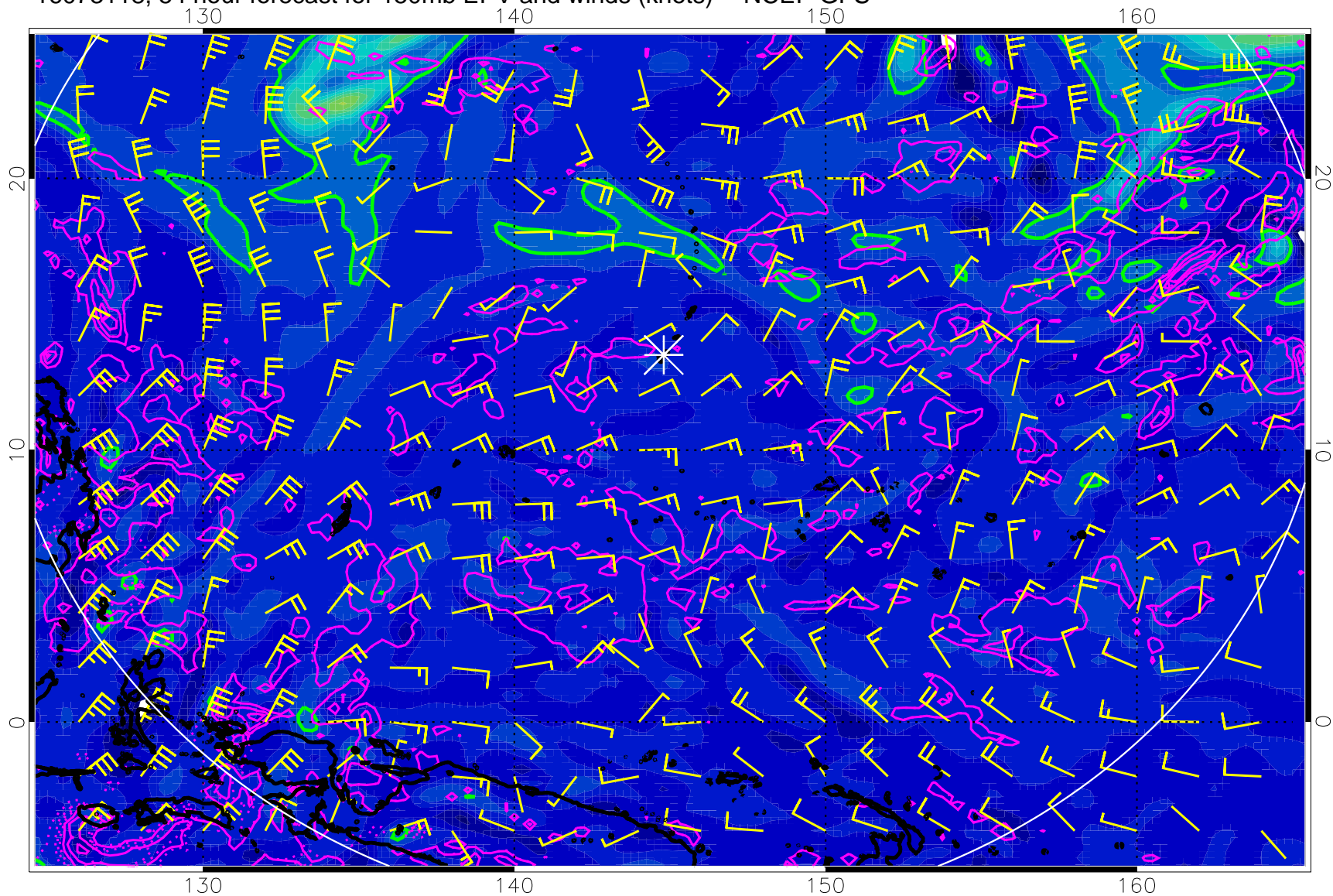
16073118, 54 hour forecast for 150mb EPV and winds (knots) -- NCEP GFS
