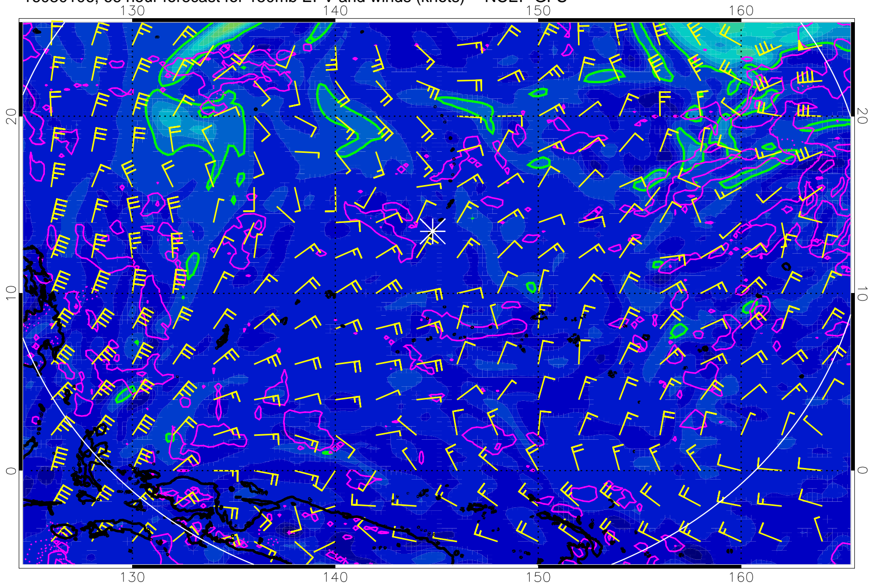
16080106, 66 hour forecast for 150mb EPV and winds (knots) -- NCEP GFS
