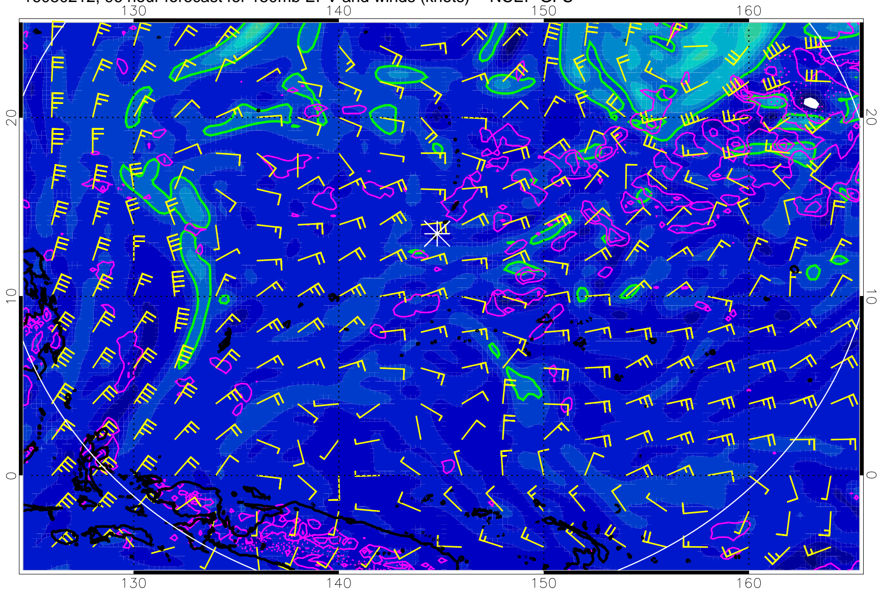
16080212, 96 hour forecast for 150mb EPV and winds (knots) -- NCEP GFS
