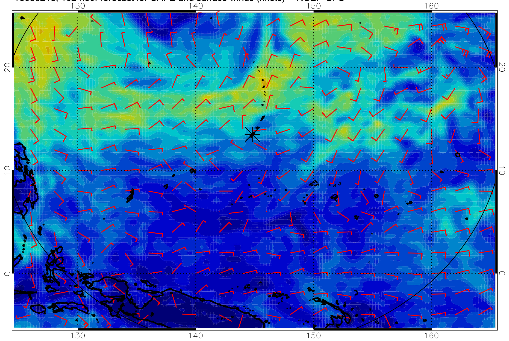
16080218, 102 hour forecast for CAPE and surface winds (knots) -- NCEP GFS
