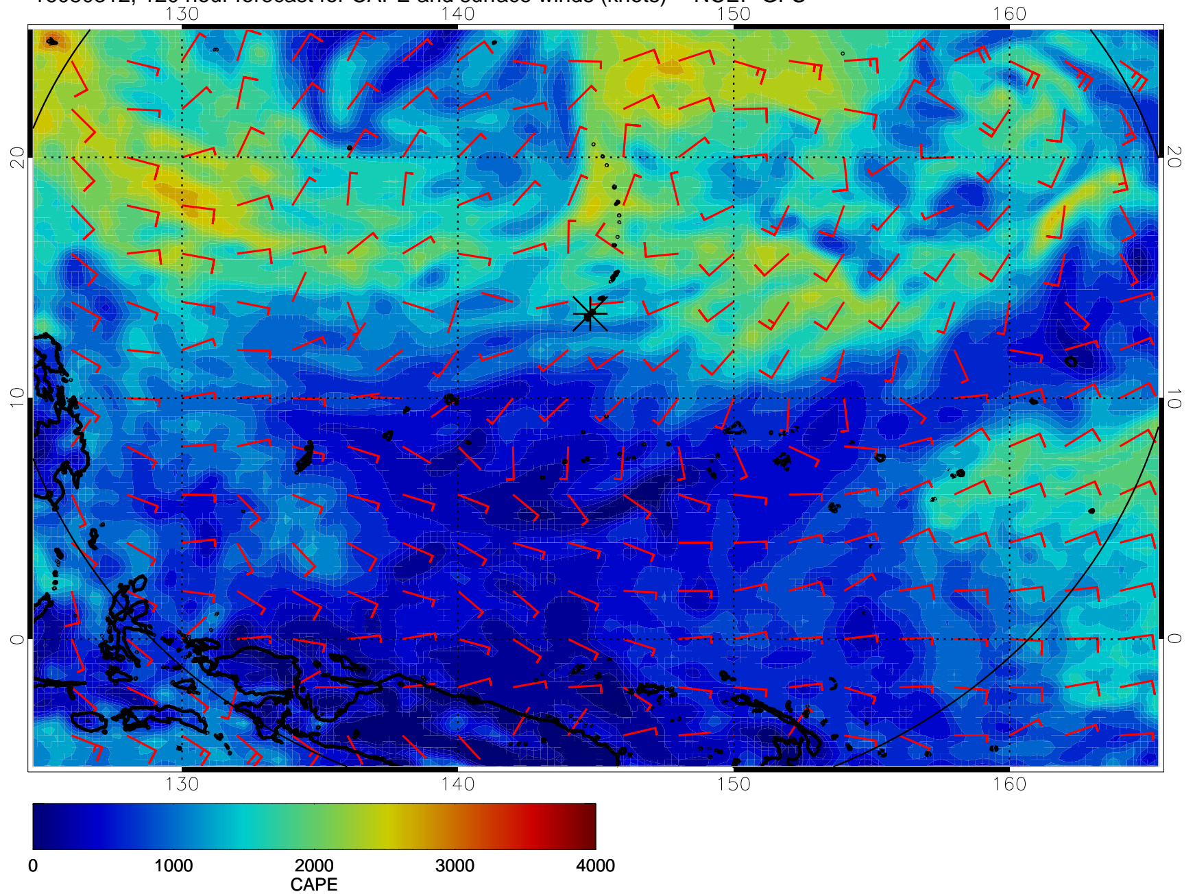
16080312, 120 hour forecast for CAPE and surface winds (knots) -- NCEP GFS
