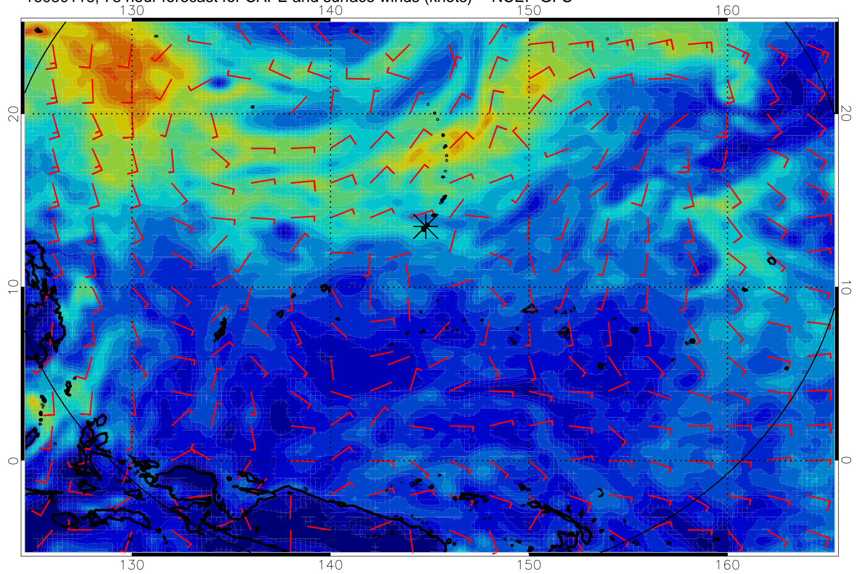
16080118, 78 hour forecast for CAPE and surface winds (knots) -- NCEP GFS
