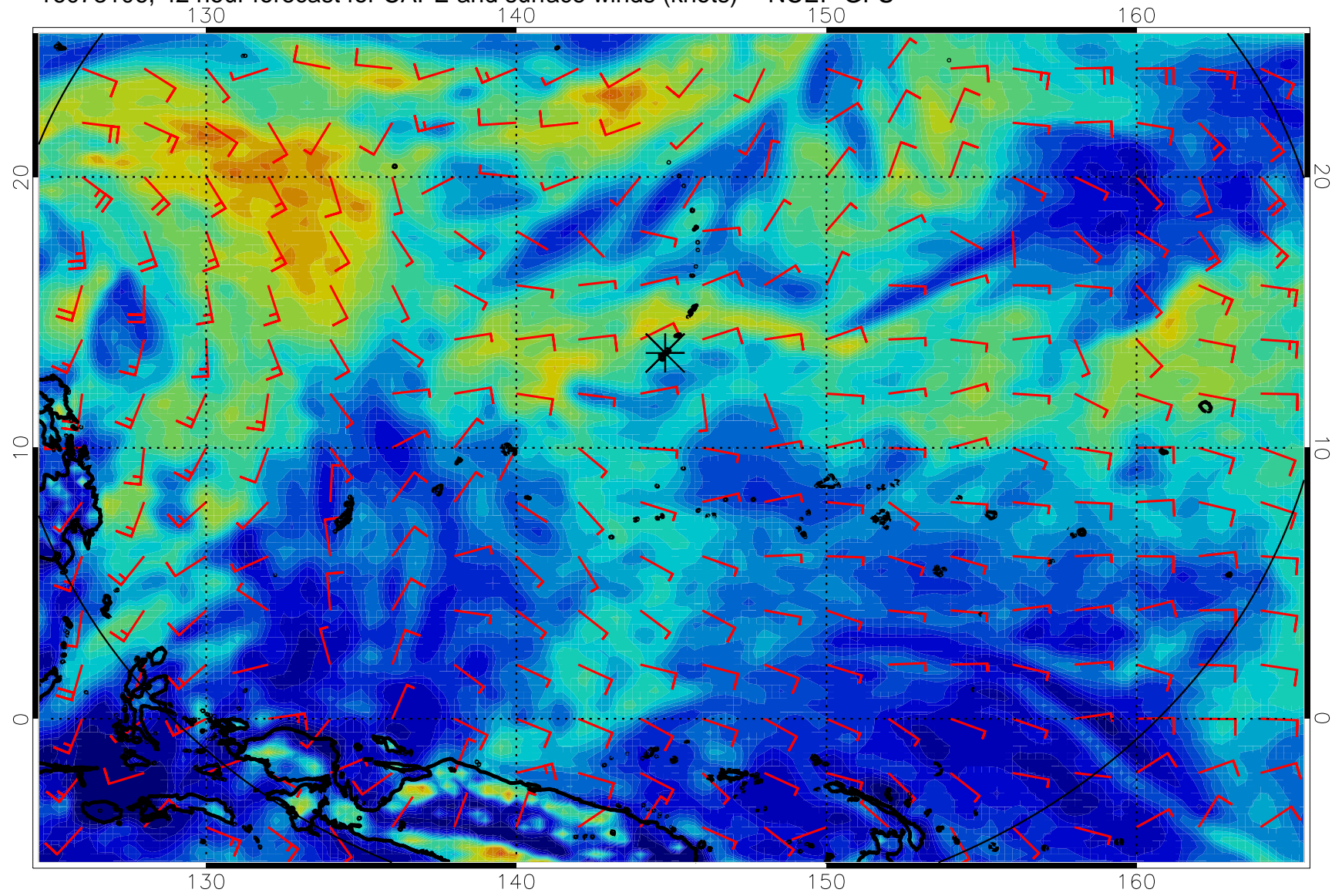
16073106, 42 hour forecast for CAPE and surface winds (knots) -- NCEP GFS
