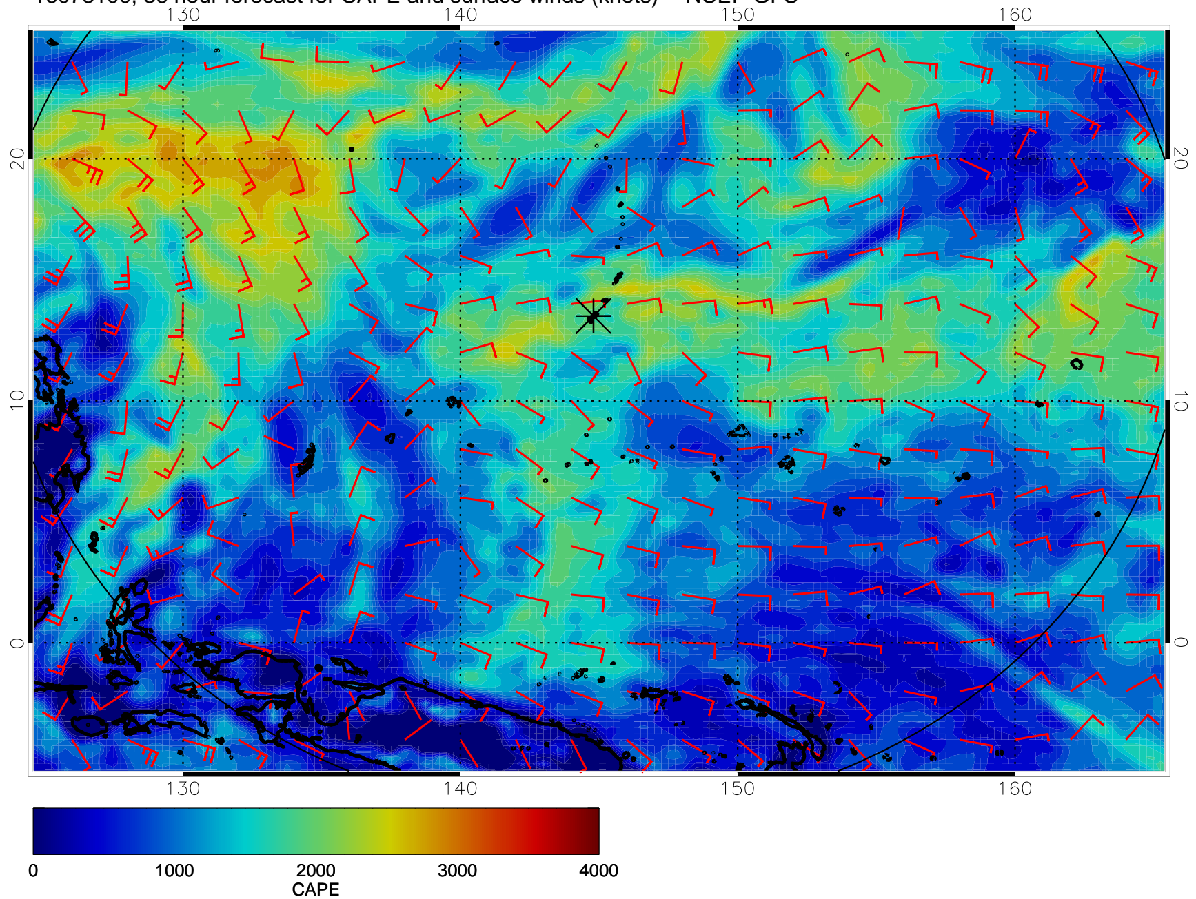
16073100, 36 hour forecast for CAPE and surface winds (knots) -- NCEP GFS
