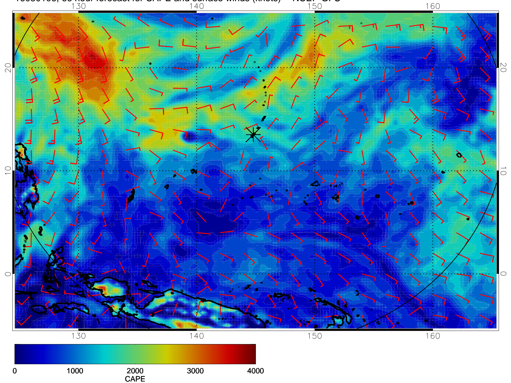
16080106, 66 hour forecast for CAPE and surface winds (knots) -- NCEP GFS
