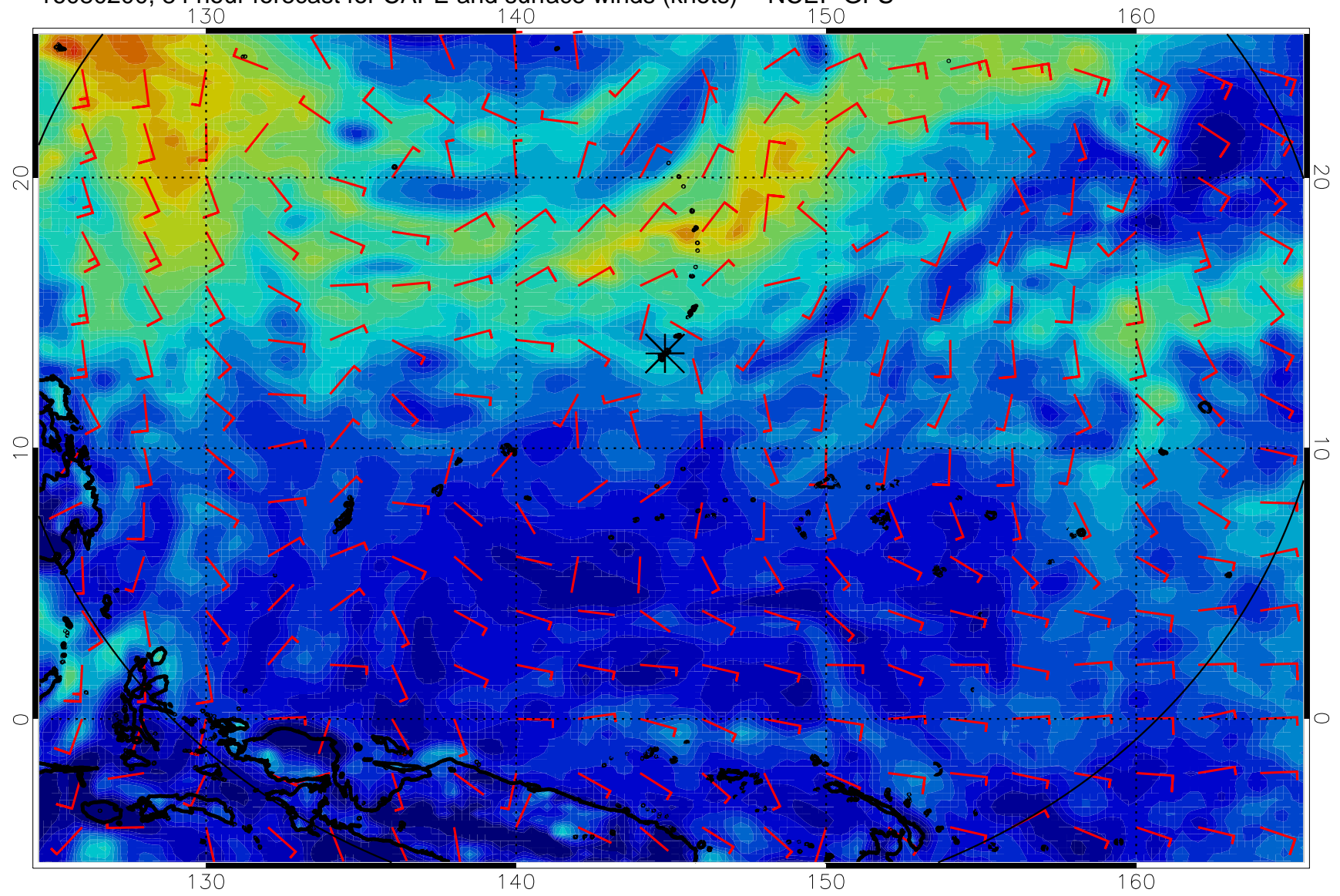
16080200, 84 hour forecast for CAPE and surface winds (knots) -- NCEP GFS
