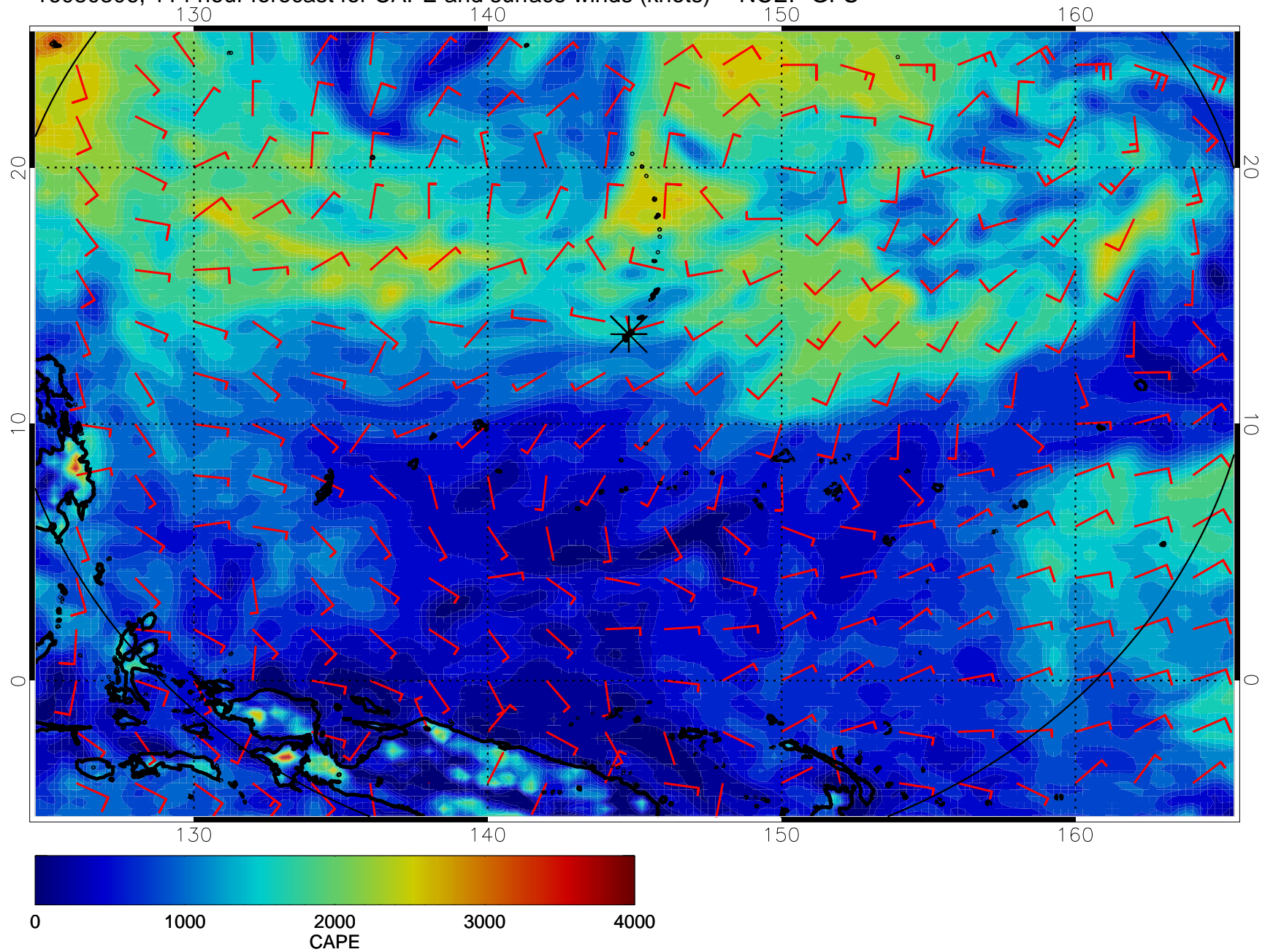
16080306, 114 hour forecast for CAPE and surface winds (knots) -- NCEP GFS
