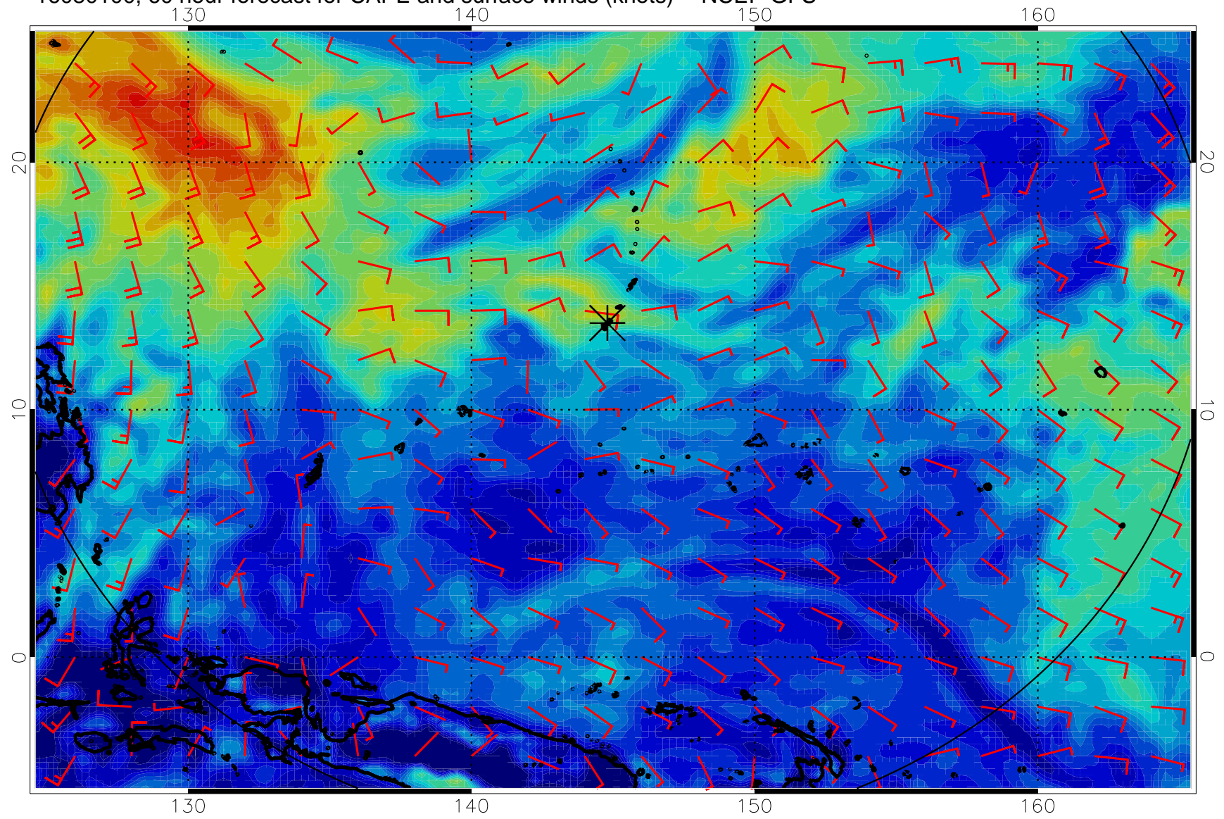
16080100, 60 hour forecast for CAPE and surface winds (knots) -- NCEP GFS
