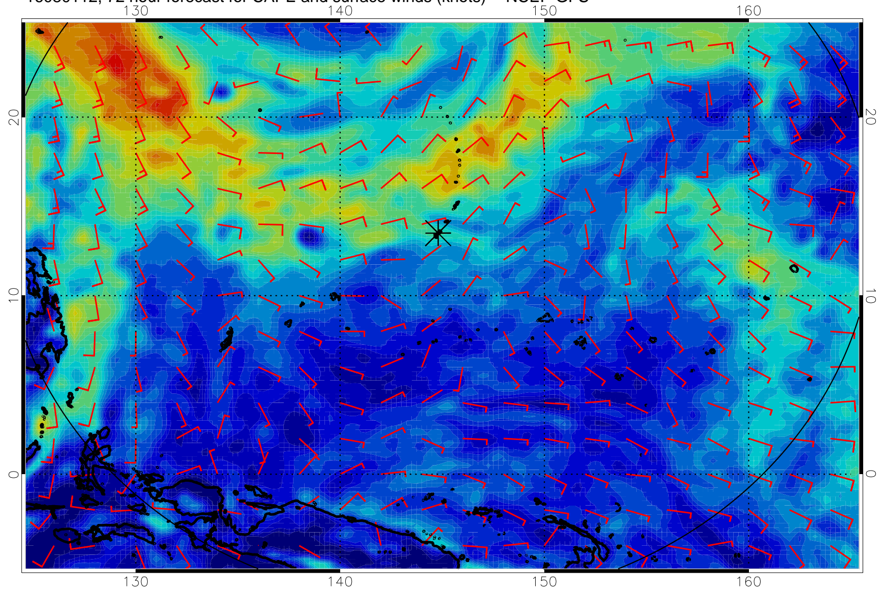
16080112, 72 hour forecast for CAPE and surface winds (knots) -- NCEP GFS
