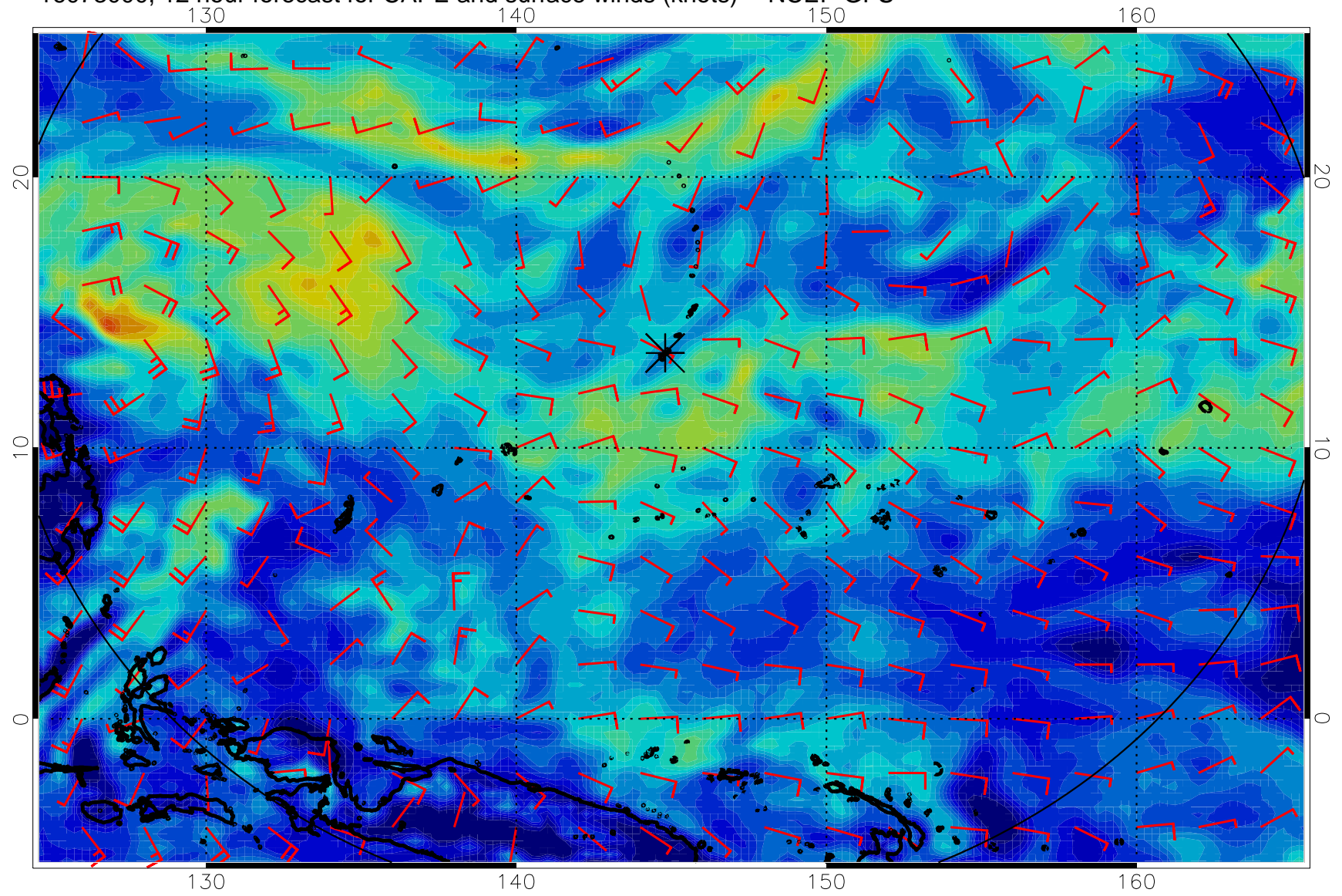
16073000, 12 hour forecast for CAPE and surface winds (knots) -- NCEP GFS
