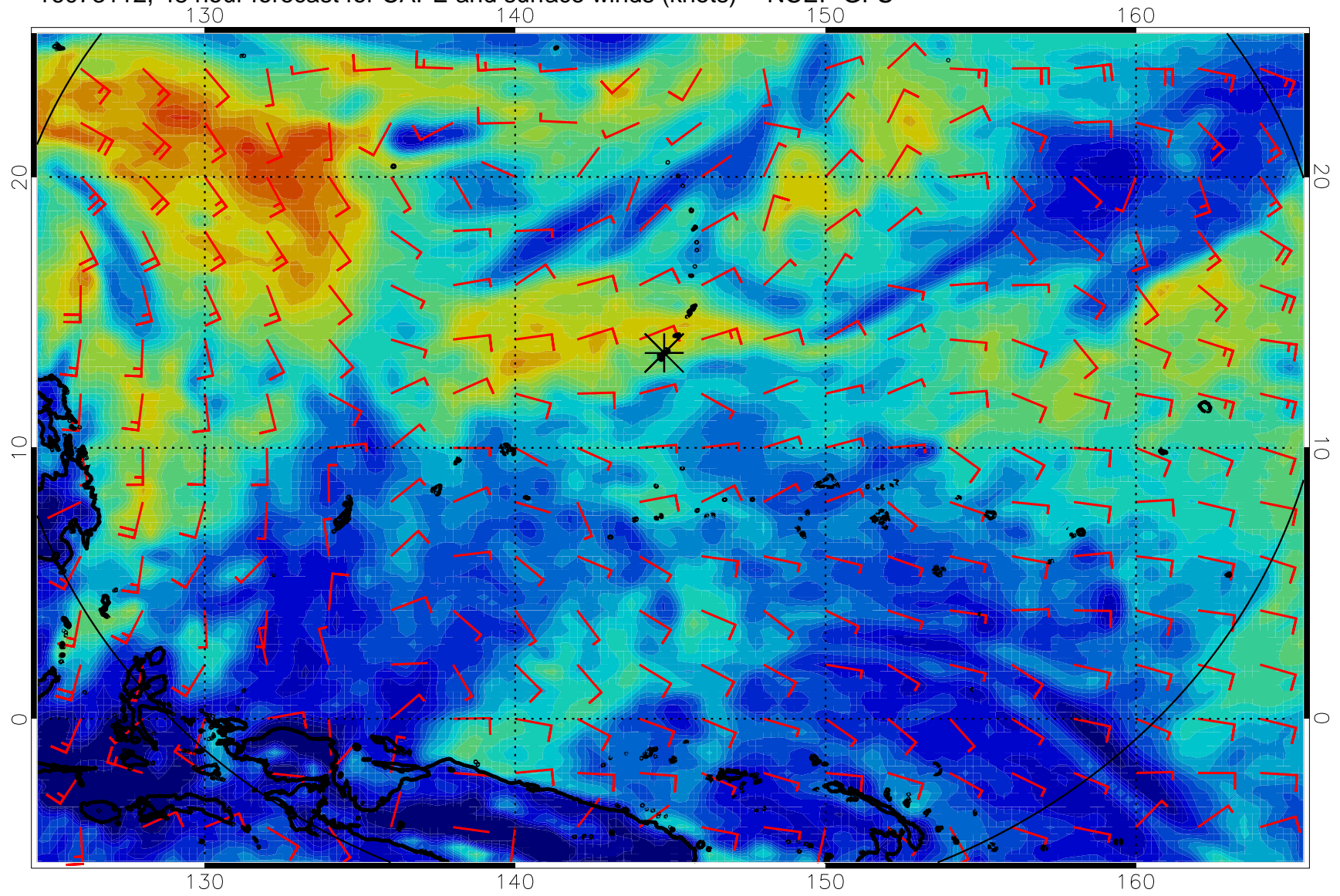
16073112, 48 hour forecast for CAPE and surface winds (knots) -- NCEP GFS
