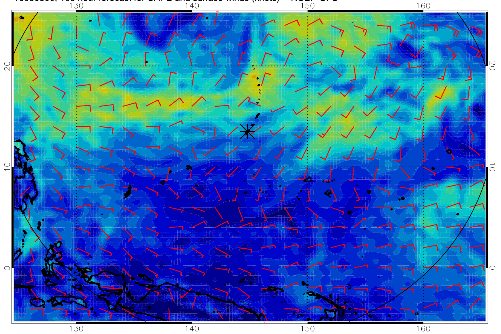
16080300, 108 hour forecast for CAPE and surface winds (knots) -- NCEP GFS
