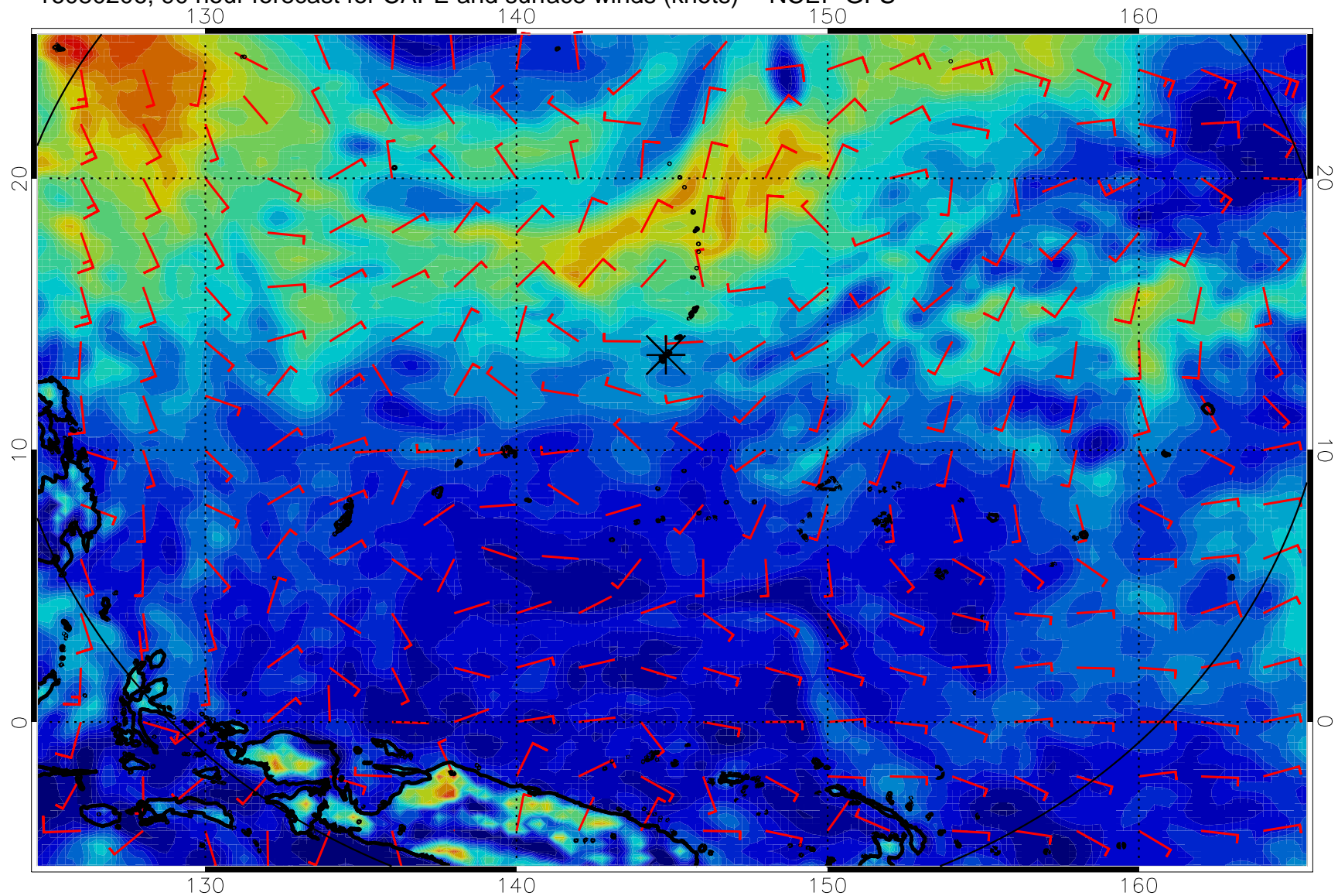
16080206, 90 hour forecast for CAPE and surface winds (knots) -- NCEP GFS
