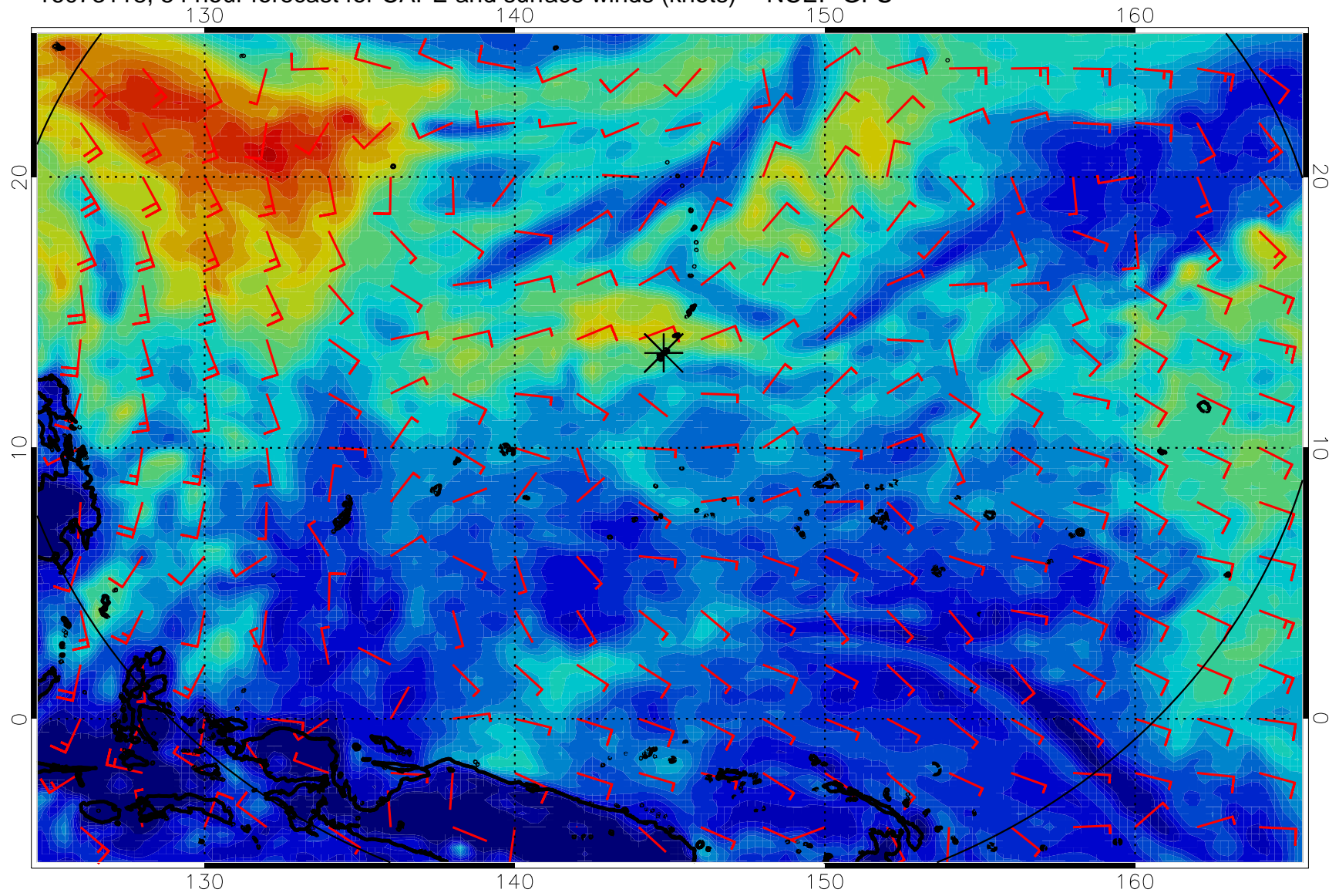
16073118, 54 hour forecast for CAPE and surface winds (knots) -- NCEP GFS
