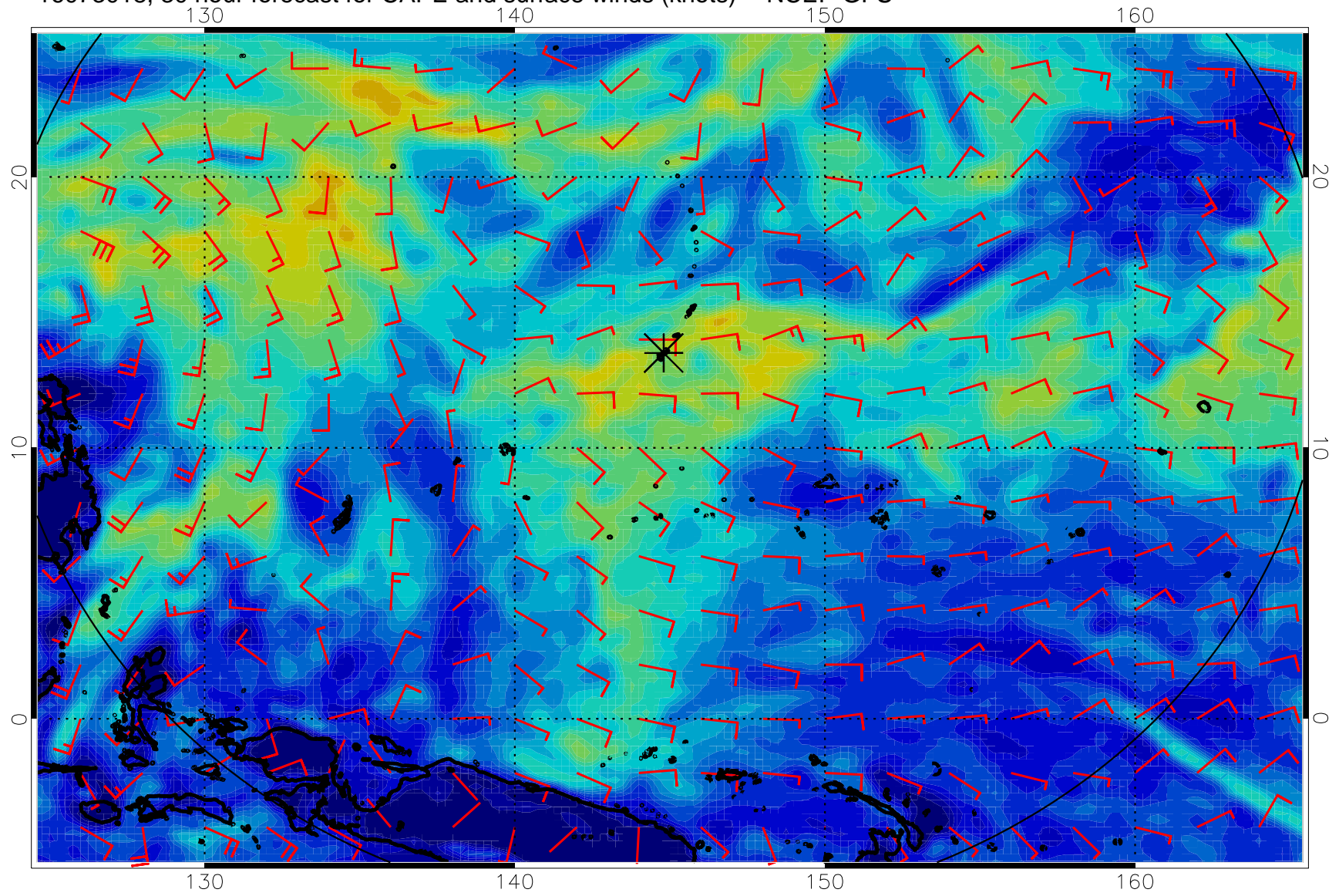
16073018, 30 hour forecast for CAPE and surface winds (knots) -- NCEP GFS
