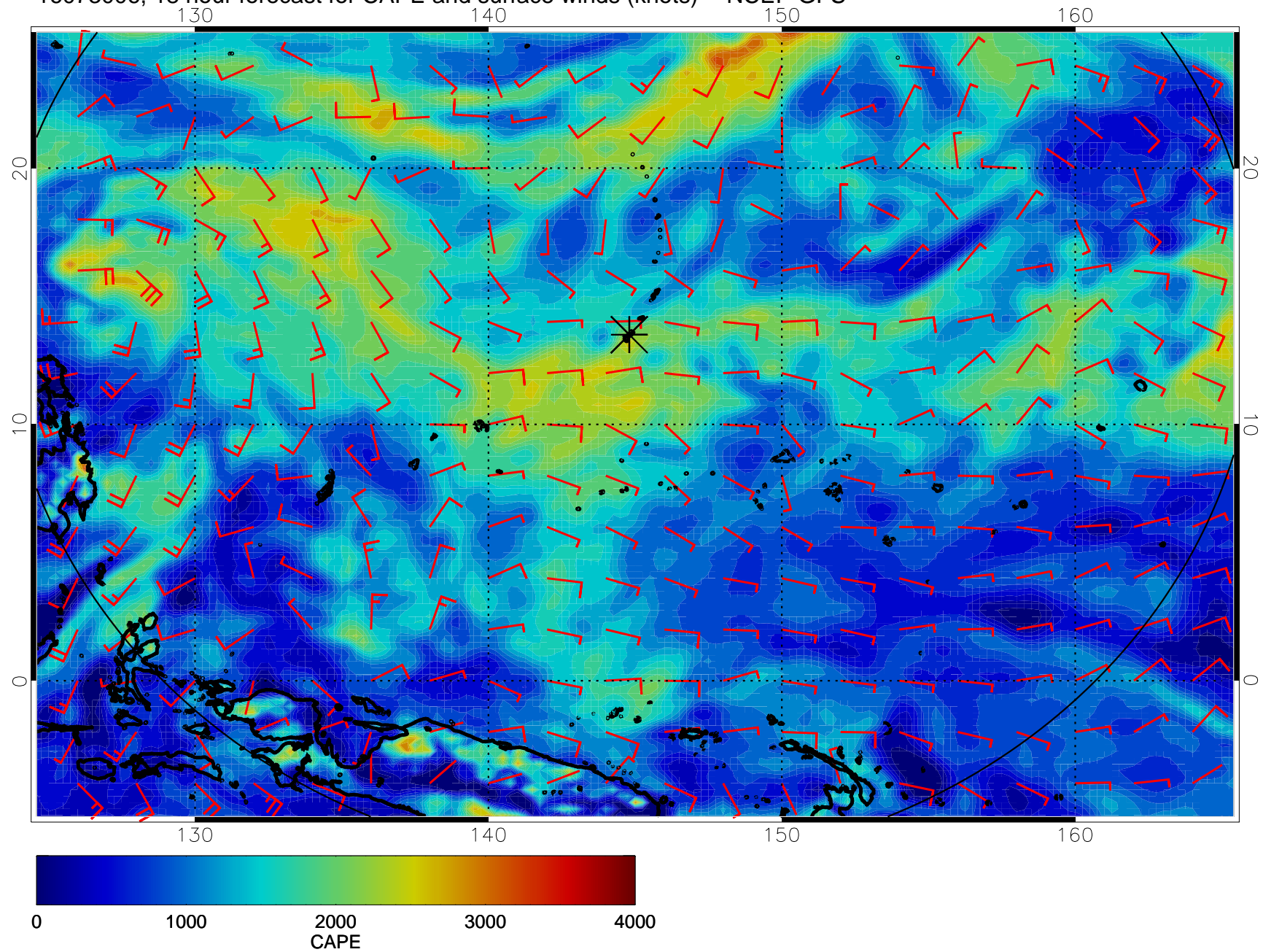
16073006, 18 hour forecast for CAPE and surface winds (knots) -- NCEP GFS
