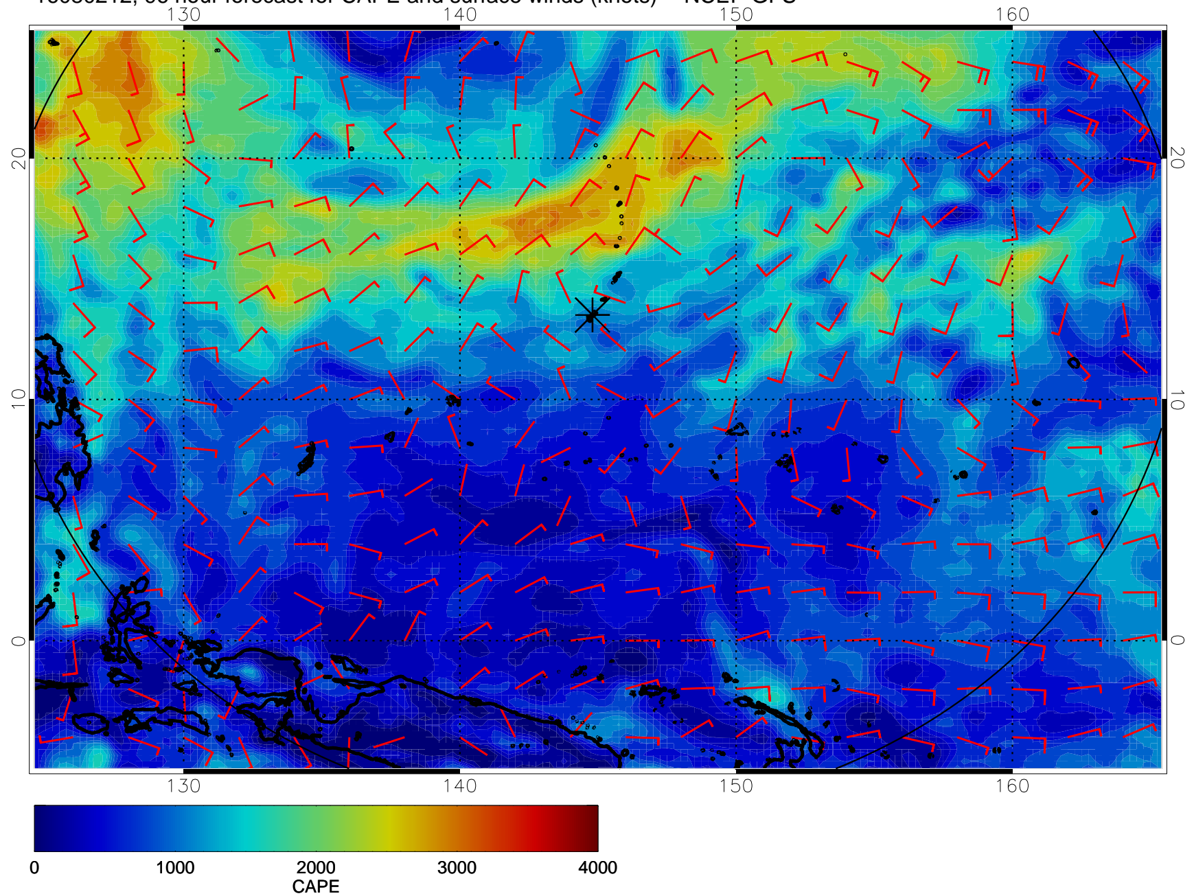
16080212, 96 hour forecast for CAPE and surface winds (knots) -- NCEP GFS
