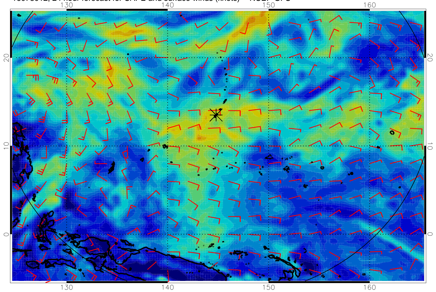
16073012, 24 hour forecast for CAPE and surface winds (knots) -- NCEP GFS
