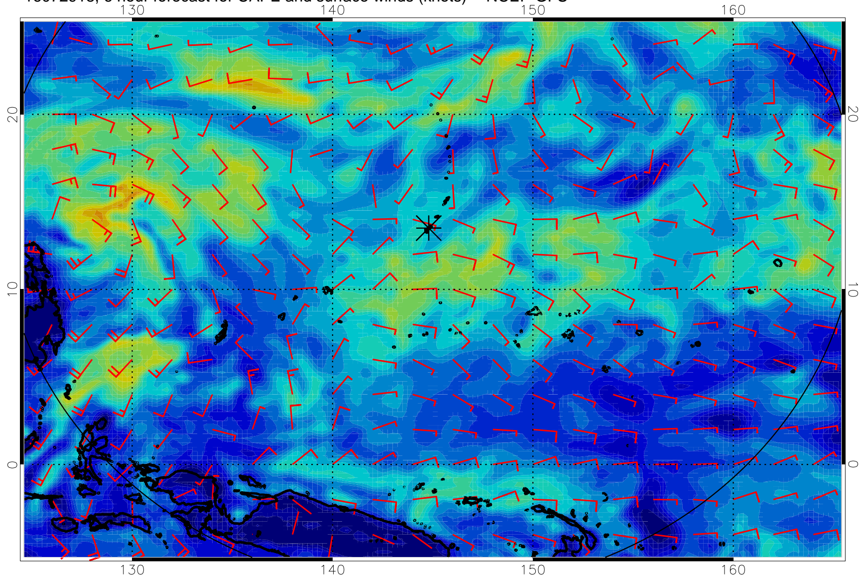
16072918, 6 hour forecast for CAPE and surface winds (knots) -- NCEP GFS
