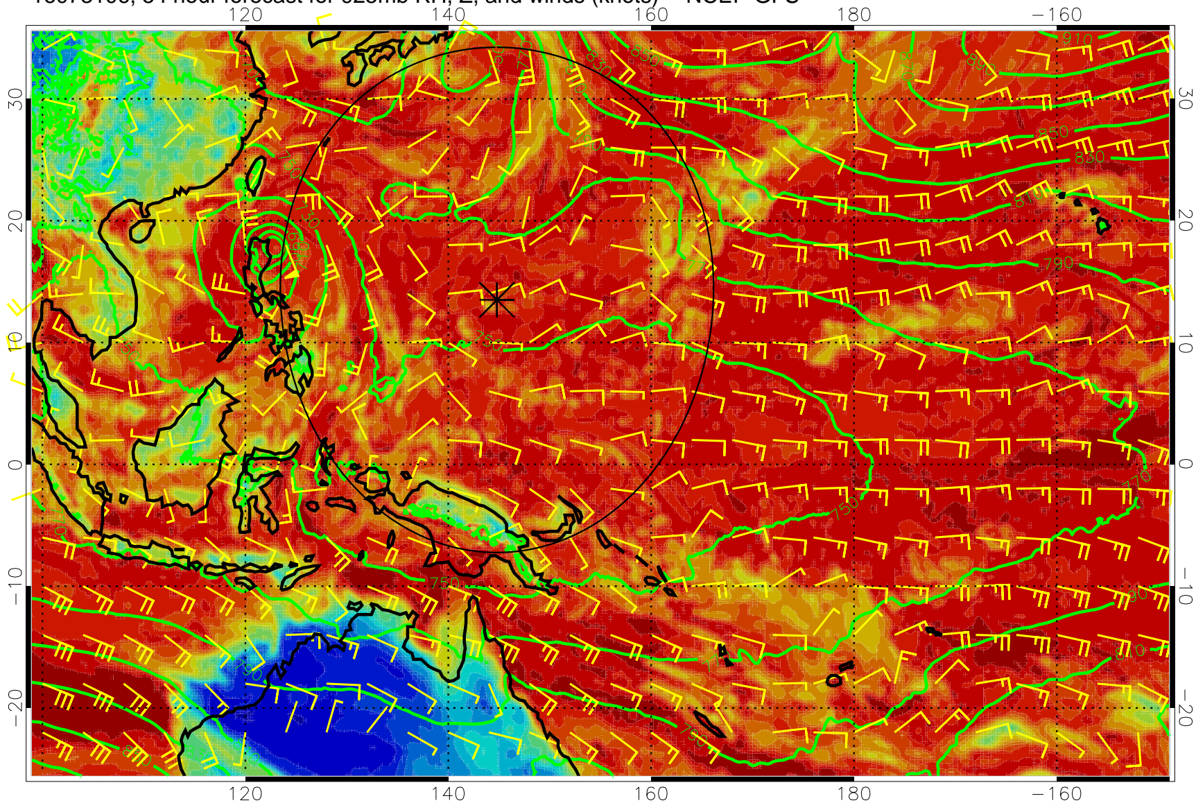
16073106, 54 hour forecast for 925mb RH, Z, and winds (knots) -- NCEP GFS
