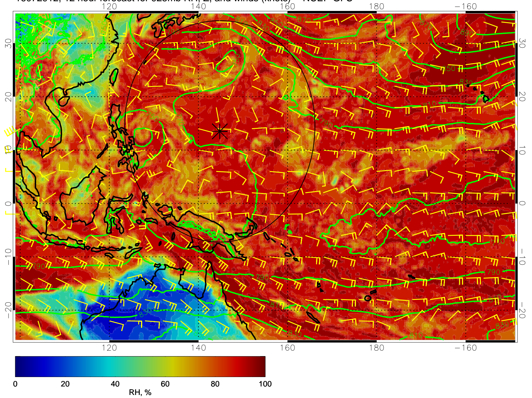
16072912, 12 hour forecast for 925mb RH, Z, and winds (knots) -- NCEP GFS
