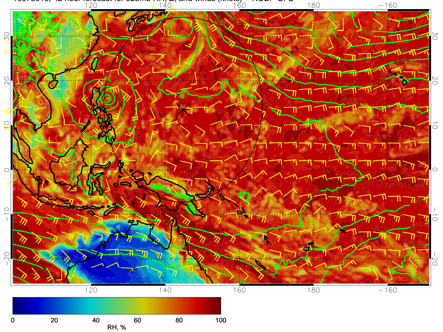
16073018, 42 hour forecast for 925mb RH, Z, and winds (knots) -- NCEP GFS
