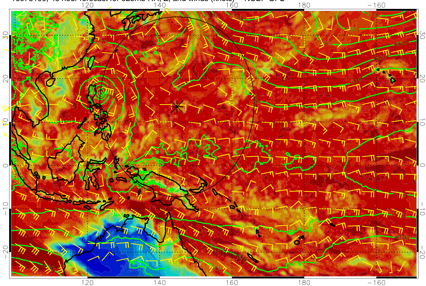
16073100, 48 hour forecast for 925mb RH, Z, and winds (knots) -- NCEP GFS
