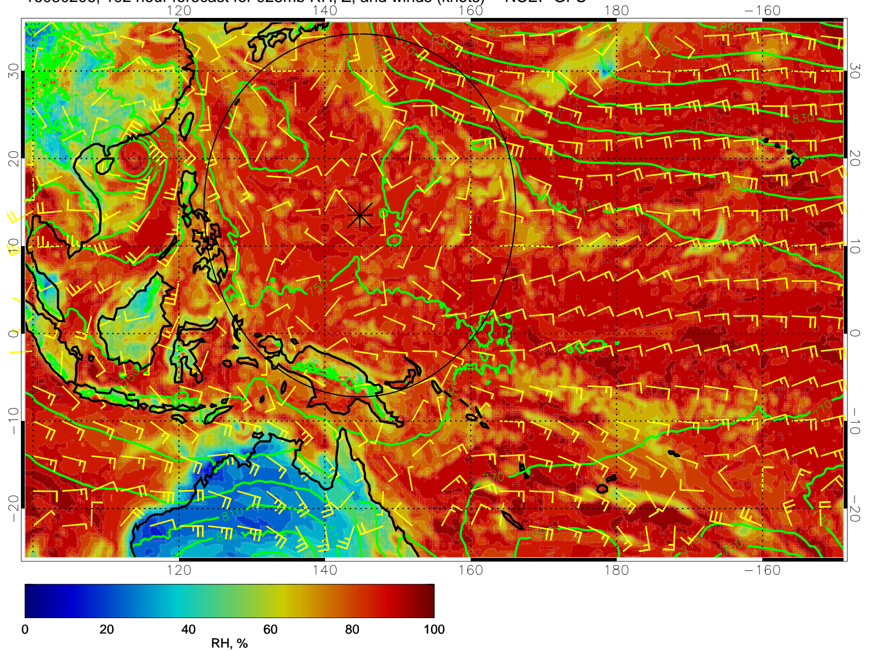
16080206, 102 hour forecast for 925mb RH, Z, and winds (knots) -- NCEP GFS
