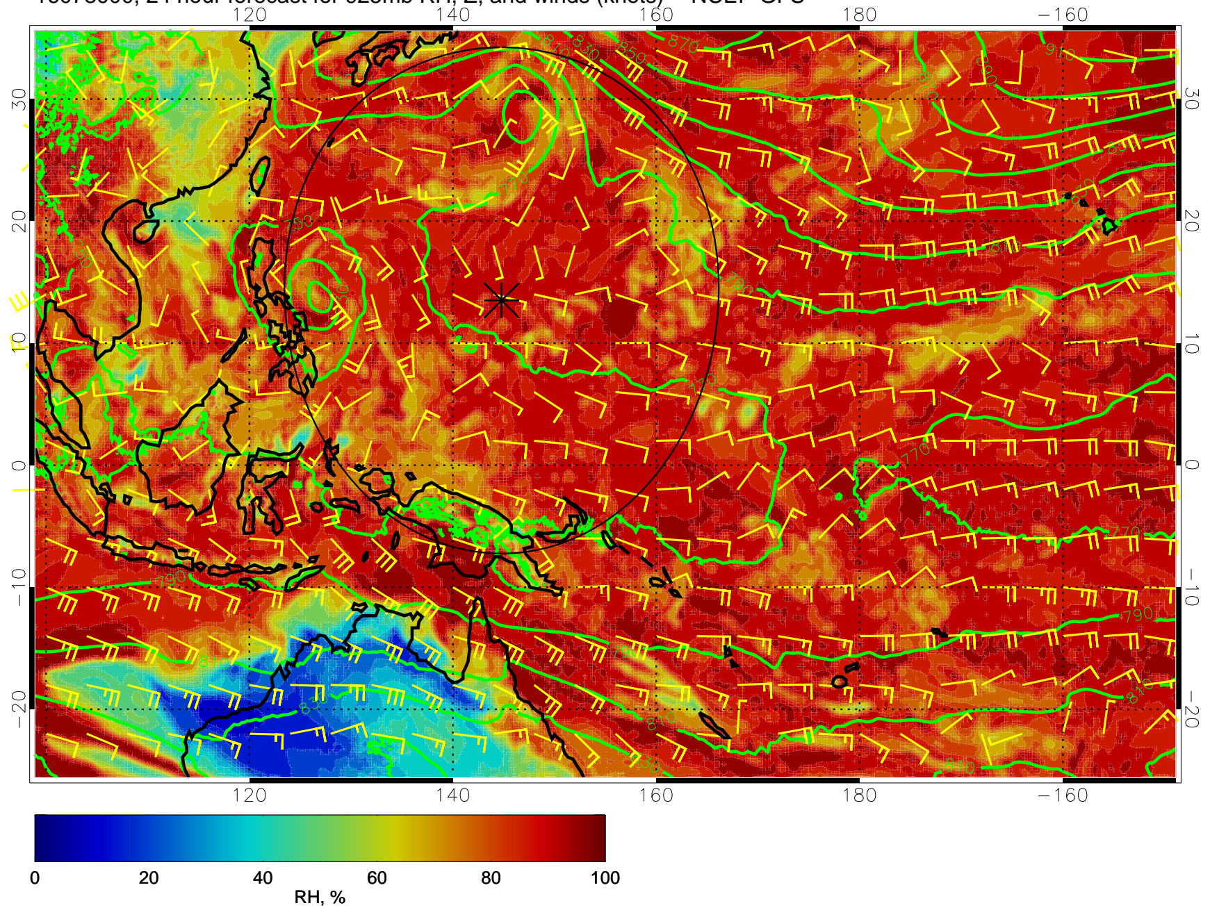
16073000, 24 hour forecast for 925mb RH, Z, and winds (knots) -- NCEP GFS
