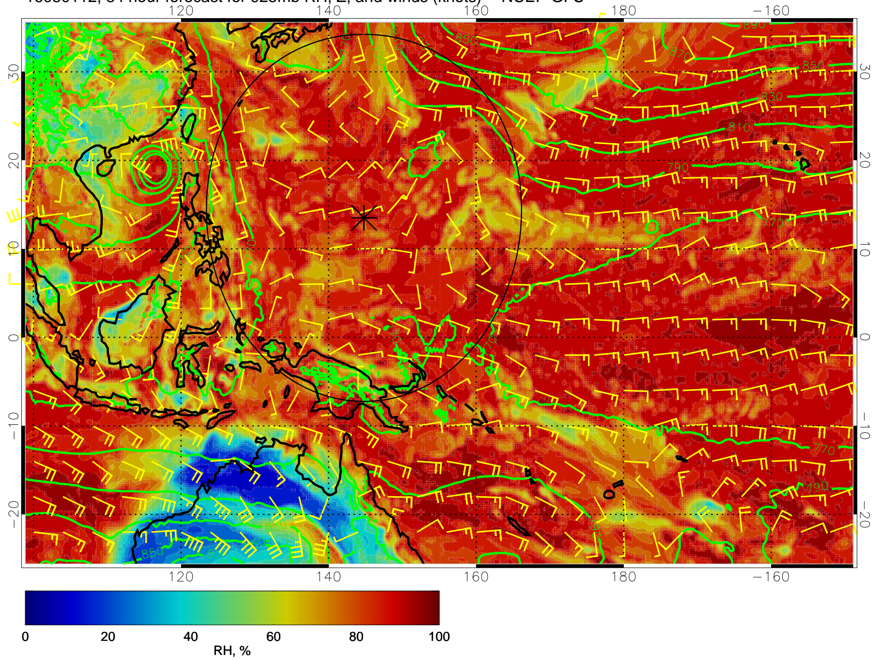
16080112, 84 hour forecast for 925mb RH, Z, and winds (knots) -- NCEP GFS
