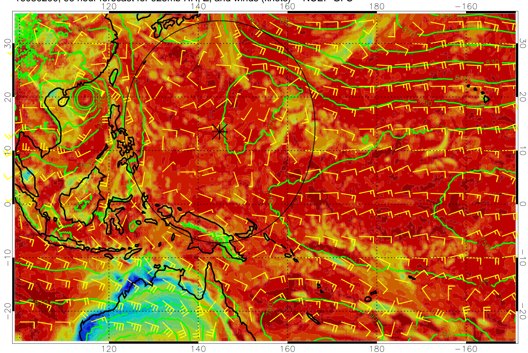
16080200, 96 hour forecast for 925mb RH, Z, and winds (knots) -- NCEP GFS
