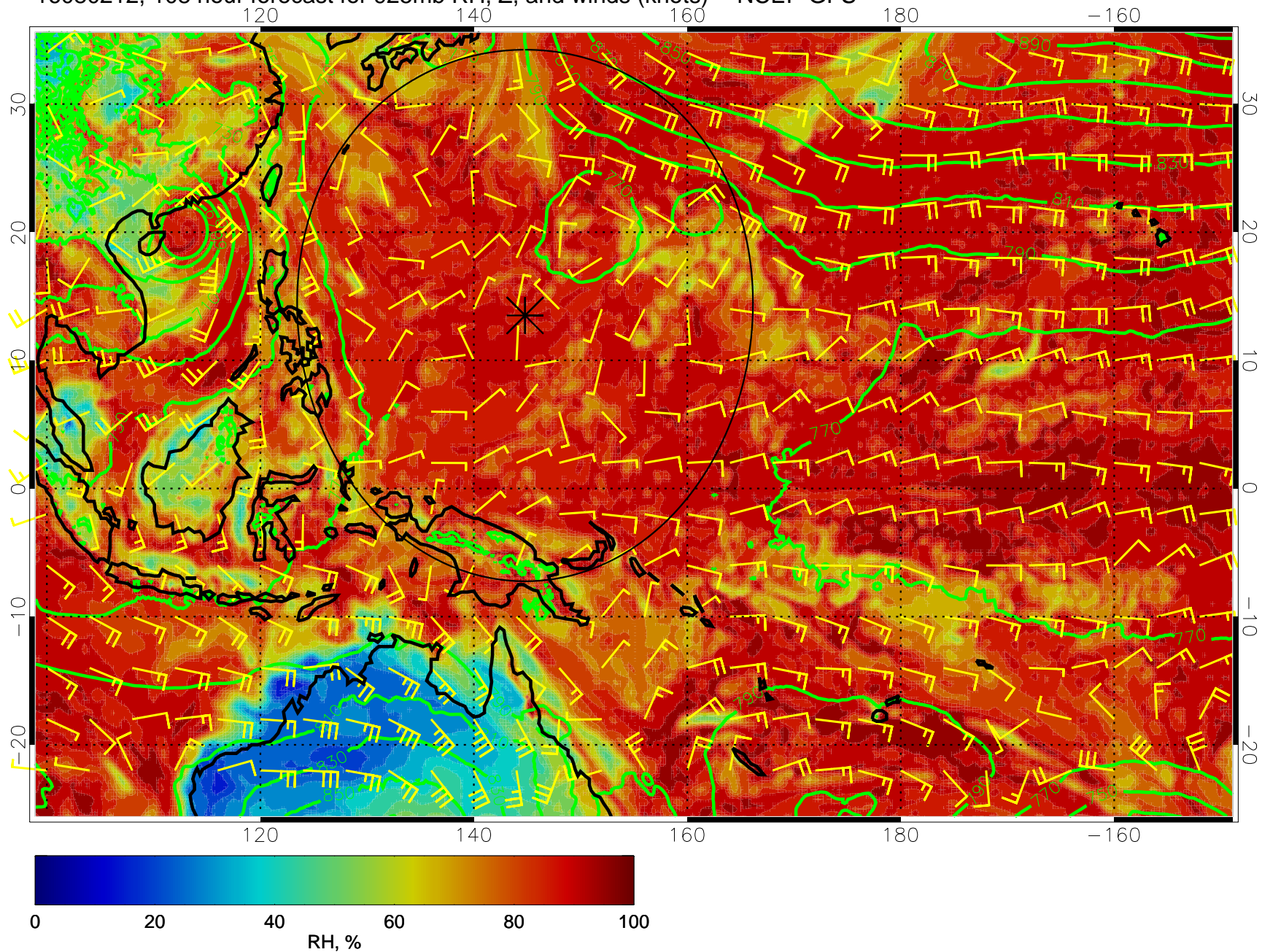
16080212, 108 hour forecast for 925mb RH, Z, and winds (knots) -- NCEP GFS
