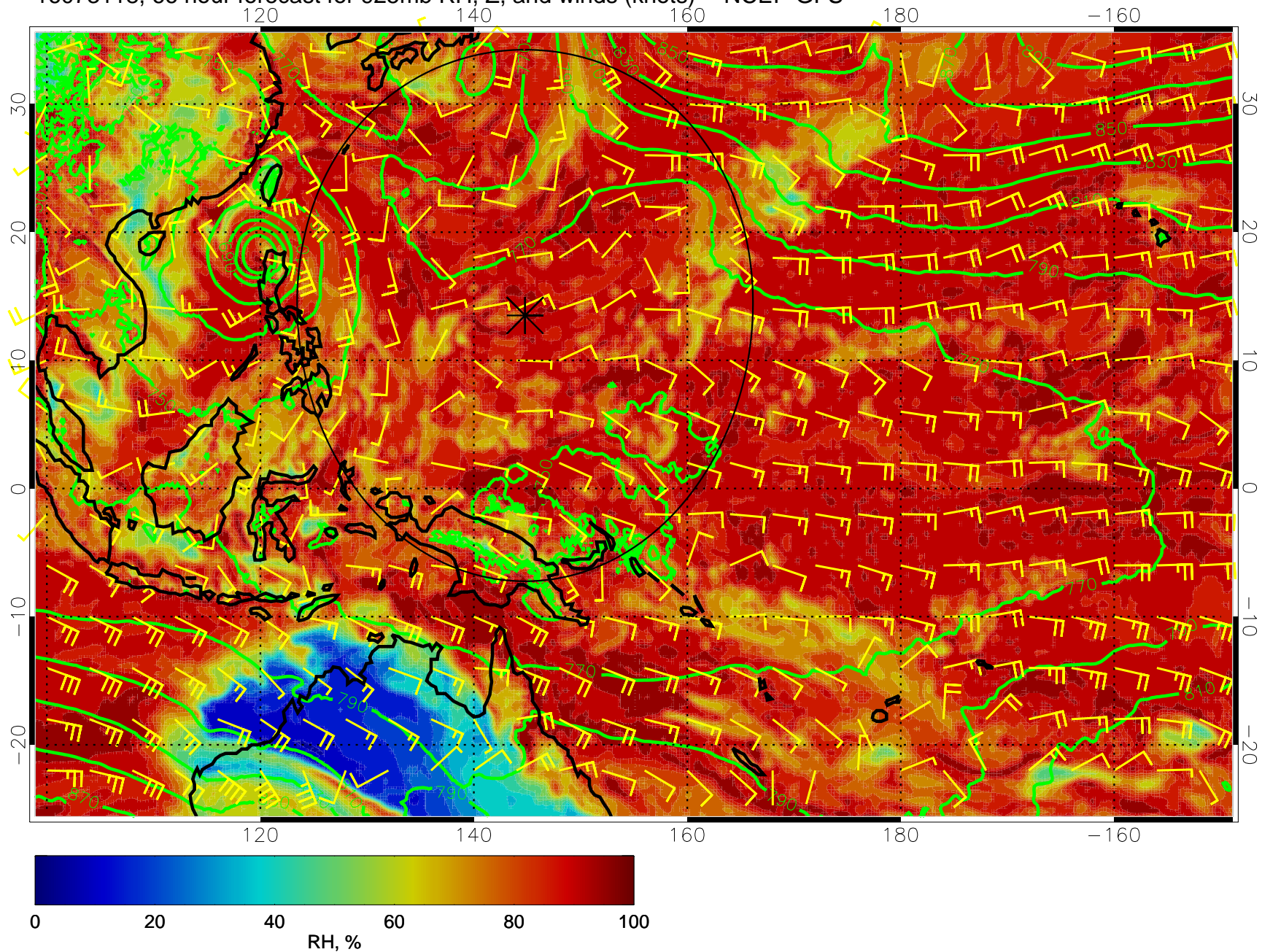
16073118, 66 hour forecast for 925mb RH, Z, and winds (knots) -- NCEP GFS
