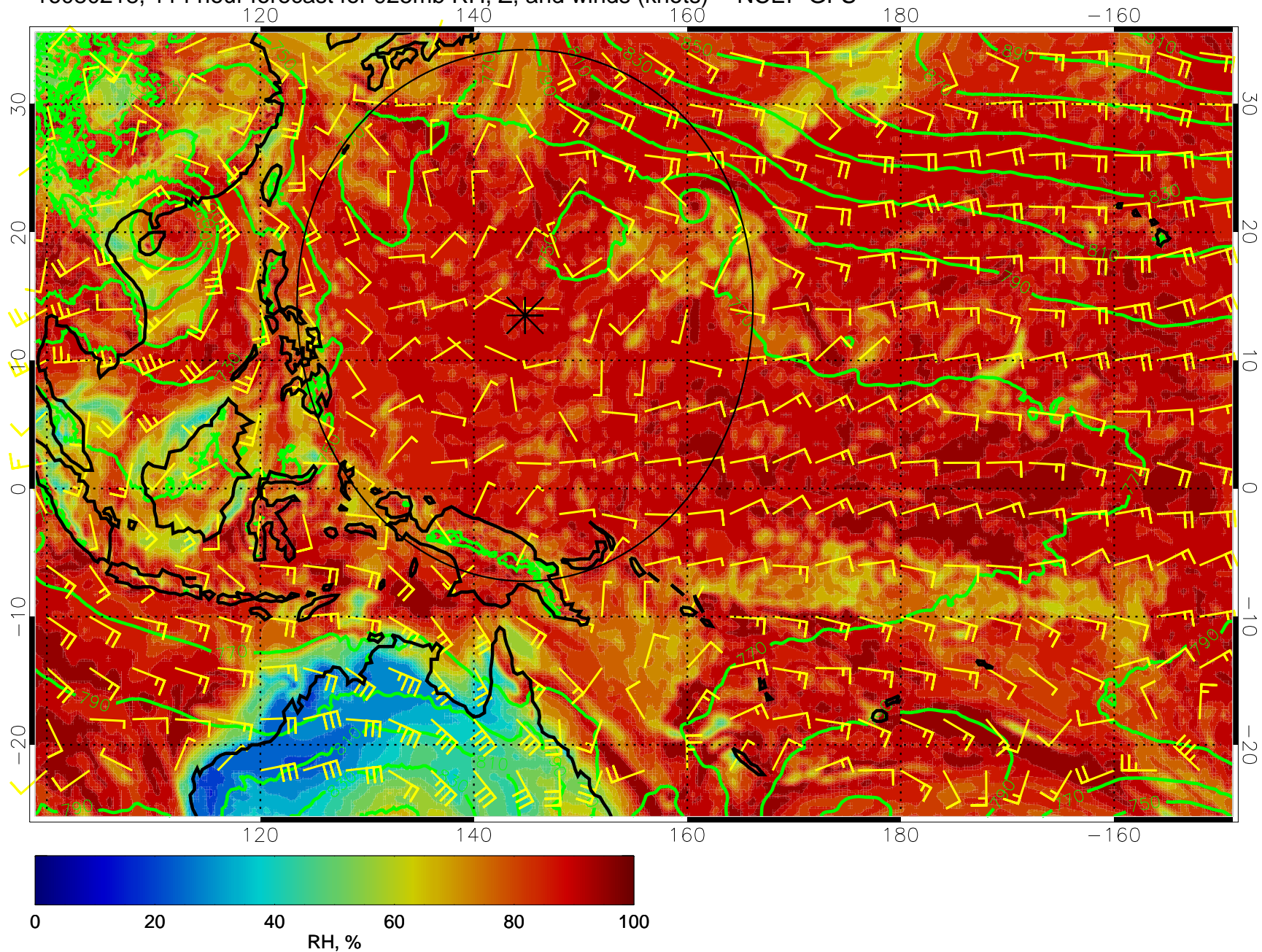
16080218, 114 hour forecast for 925mb RH, Z, and winds (knots) -- NCEP GFS
