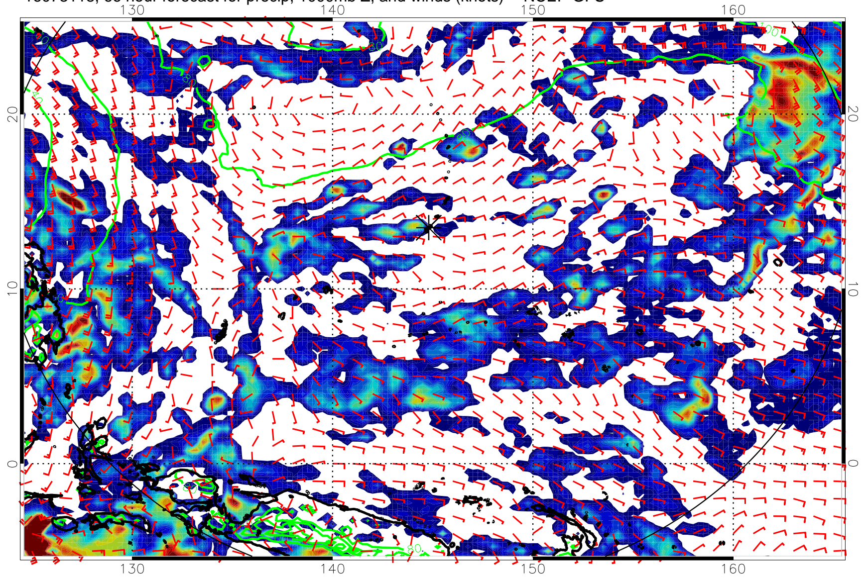
16073118, 66 hour forecast for precip, 1000mb Z, and winds (knots) -- NCEP GFS
