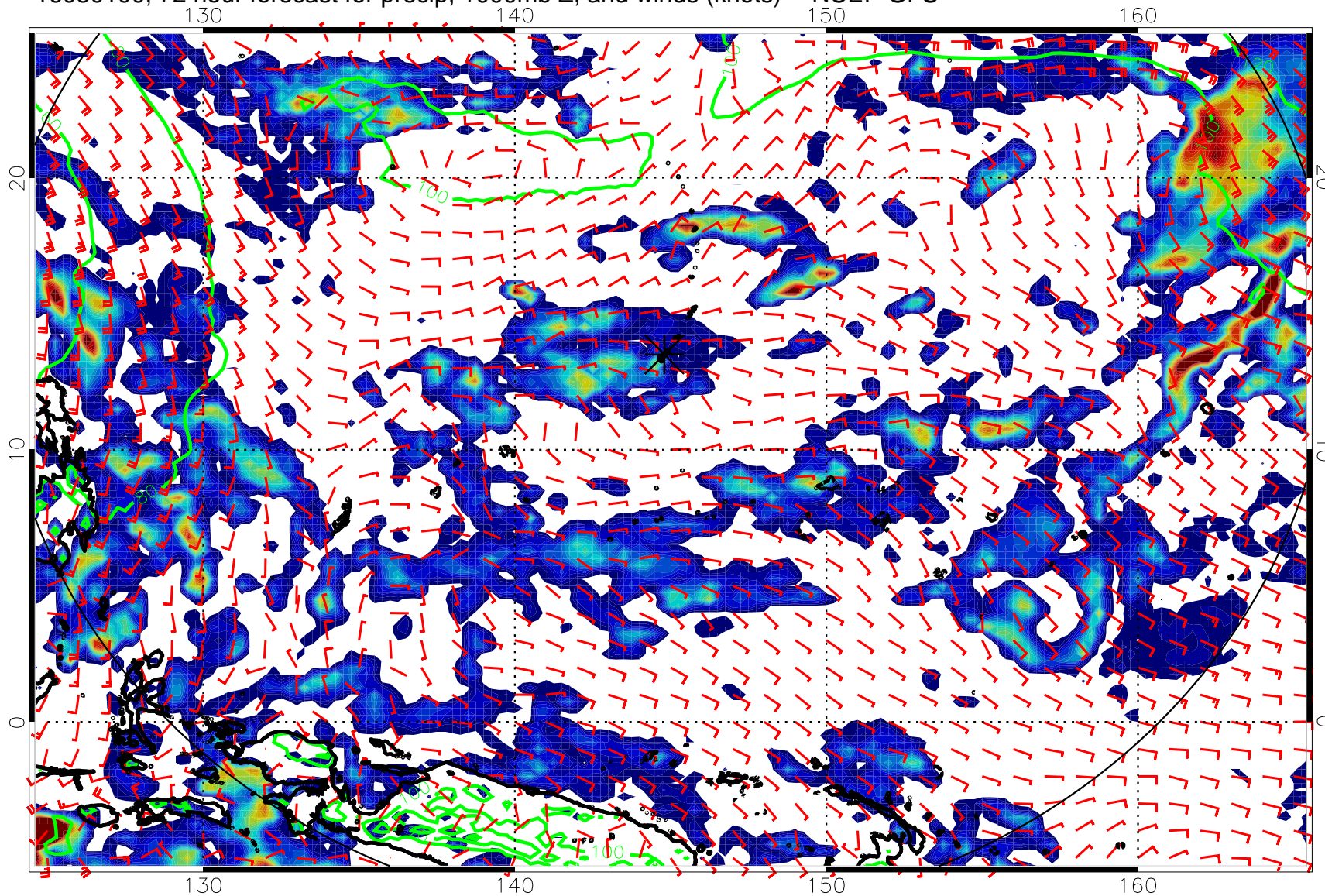
16080100, 72 hour forecast for precip, 1000mb Z, and winds (knots) -- NCEP GFS
