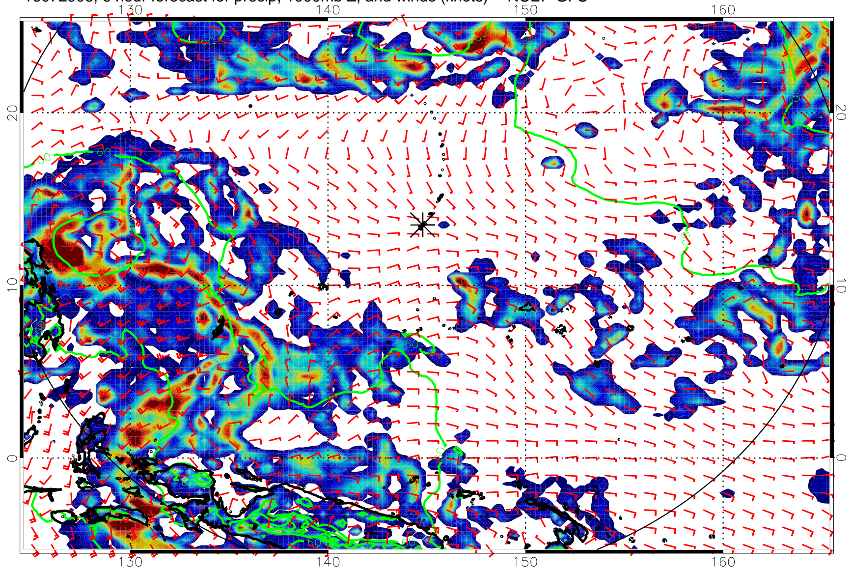
16072906, 6 hour forecast for precip, 1000mb Z, and winds (knots) -- NCEP GFS
