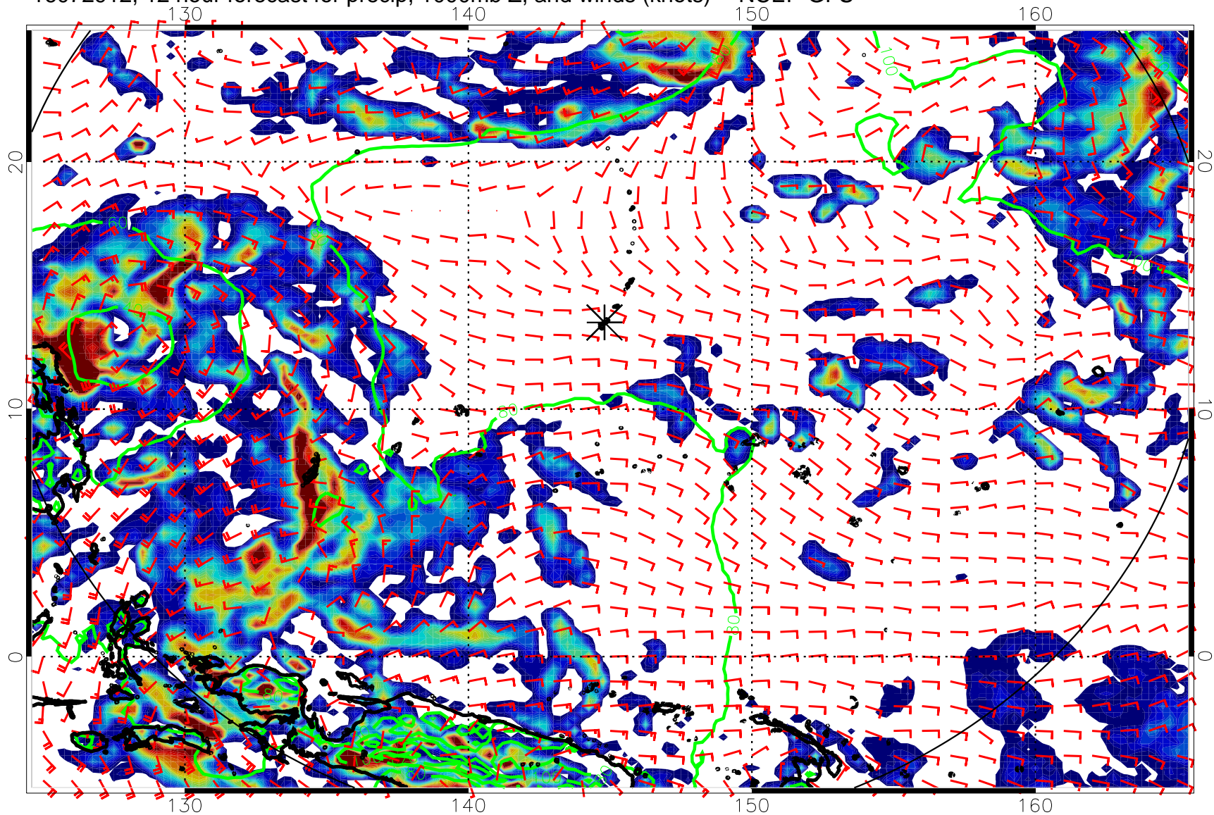
16072912, 12 hour forecast for precip, 1000mb Z, and winds (knots) -- NCEP GFS
