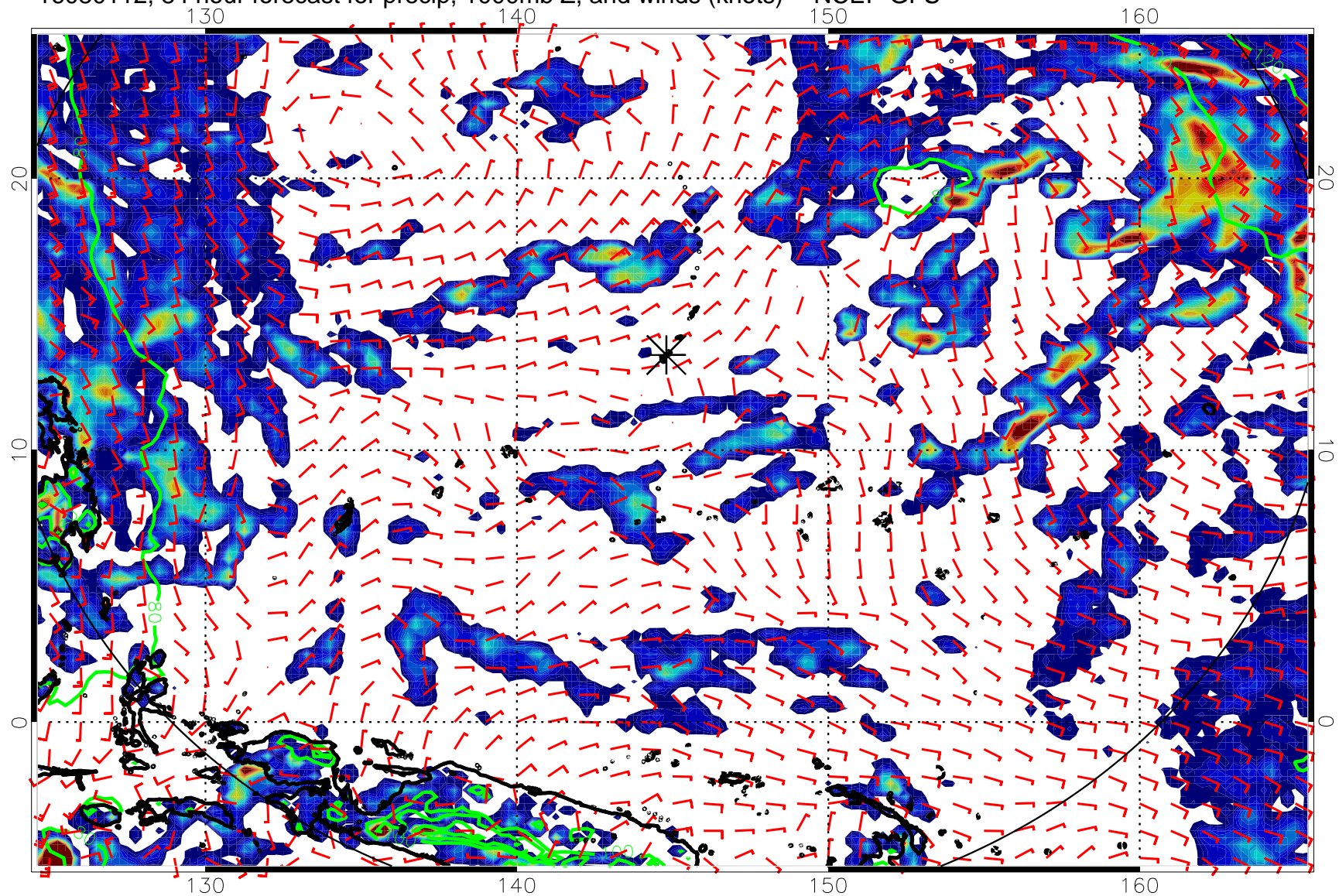
16080112, 84 hour forecast for precip, 1000mb Z, and winds (knots) -- NCEP GFS
