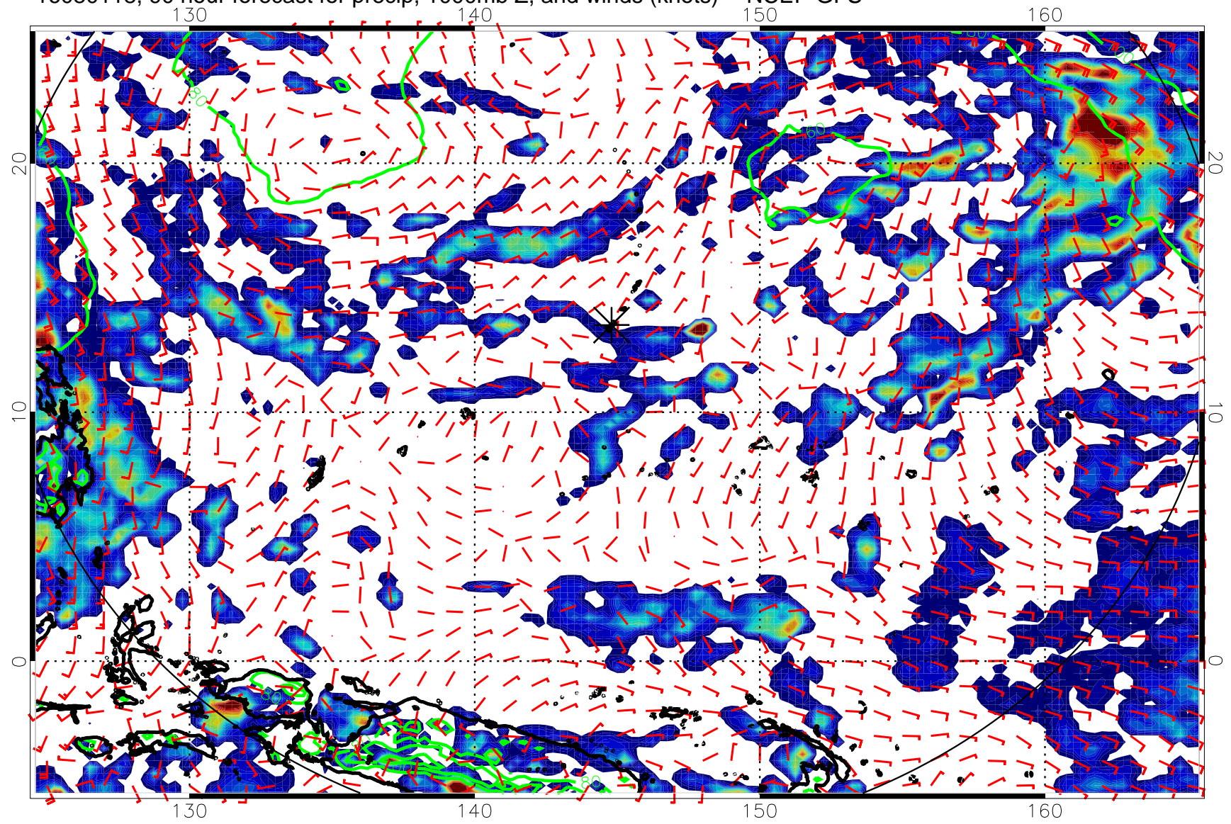
16080118, 90 hour forecast for precip, 1000mb Z, and winds (knots) -- NCEP GFS
