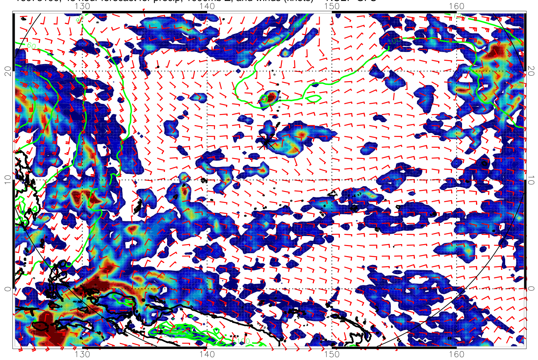
16073100, 48 hour forecast for precip, 1000mb Z, and winds (knots) -- NCEP GFS
