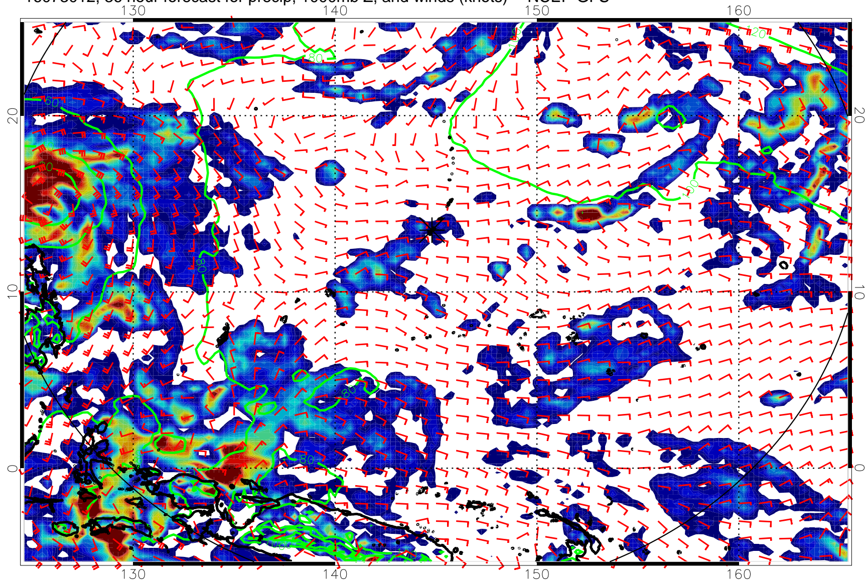
16073012, 36 hour forecast for precip, 1000mb Z, and winds (knots) -- NCEP GFS
