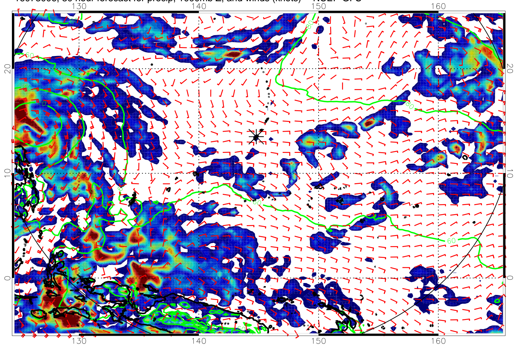
16073006, 30 hour forecast for precip, 1000mb Z, and winds (knots) -- NCEP GFS
