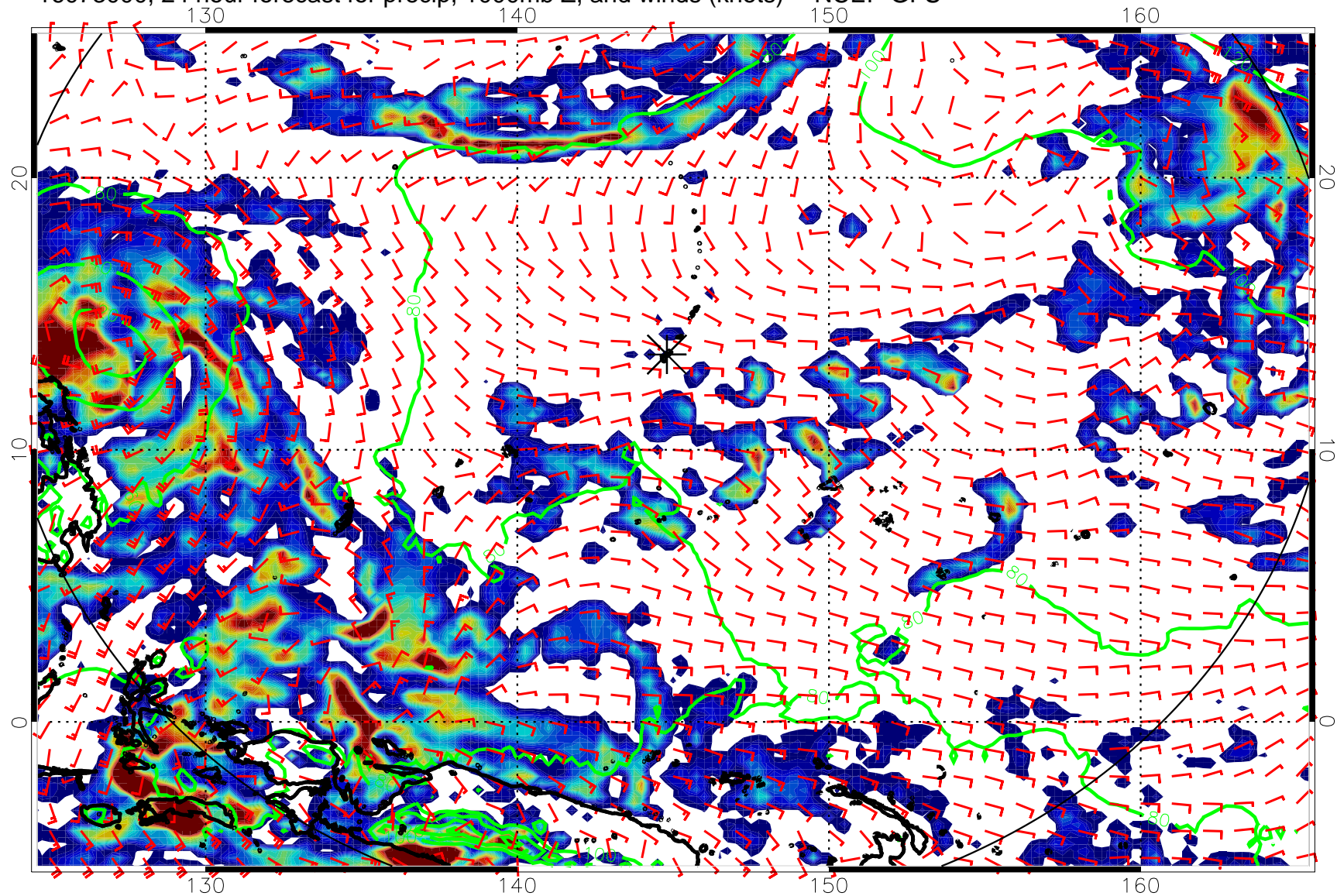
16073000, 24 hour forecast for precip, 1000mb Z, and winds (knots) -- NCEP GFS
