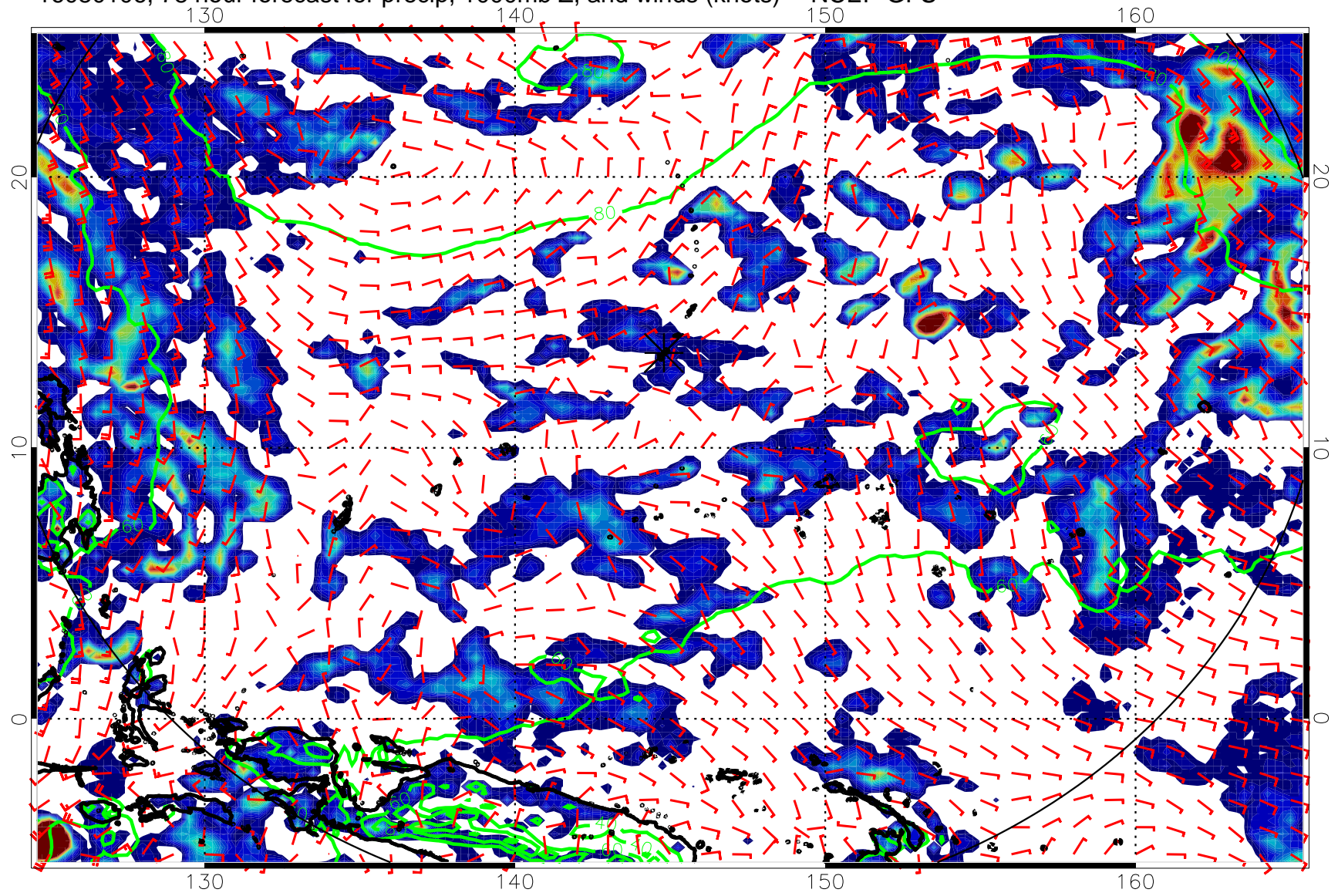
16080106, 78 hour forecast for precip, 1000mb Z, and winds (knots) -- NCEP GFS
