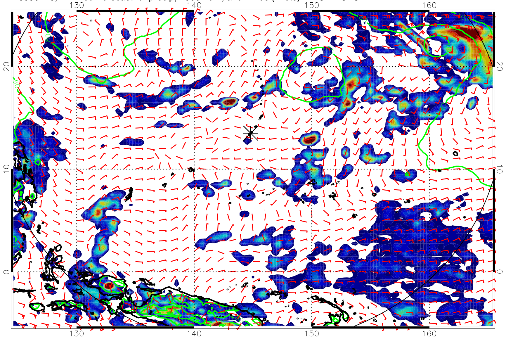
16080218, 114 hour forecast for precip, 1000mb Z, and winds (knots) -- NCEP GFS
