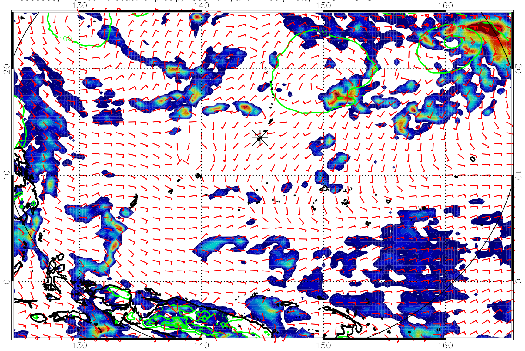
16080300, 120 hour forecast for precip, 1000mb Z, and winds (knots) -- NCEP GFS
