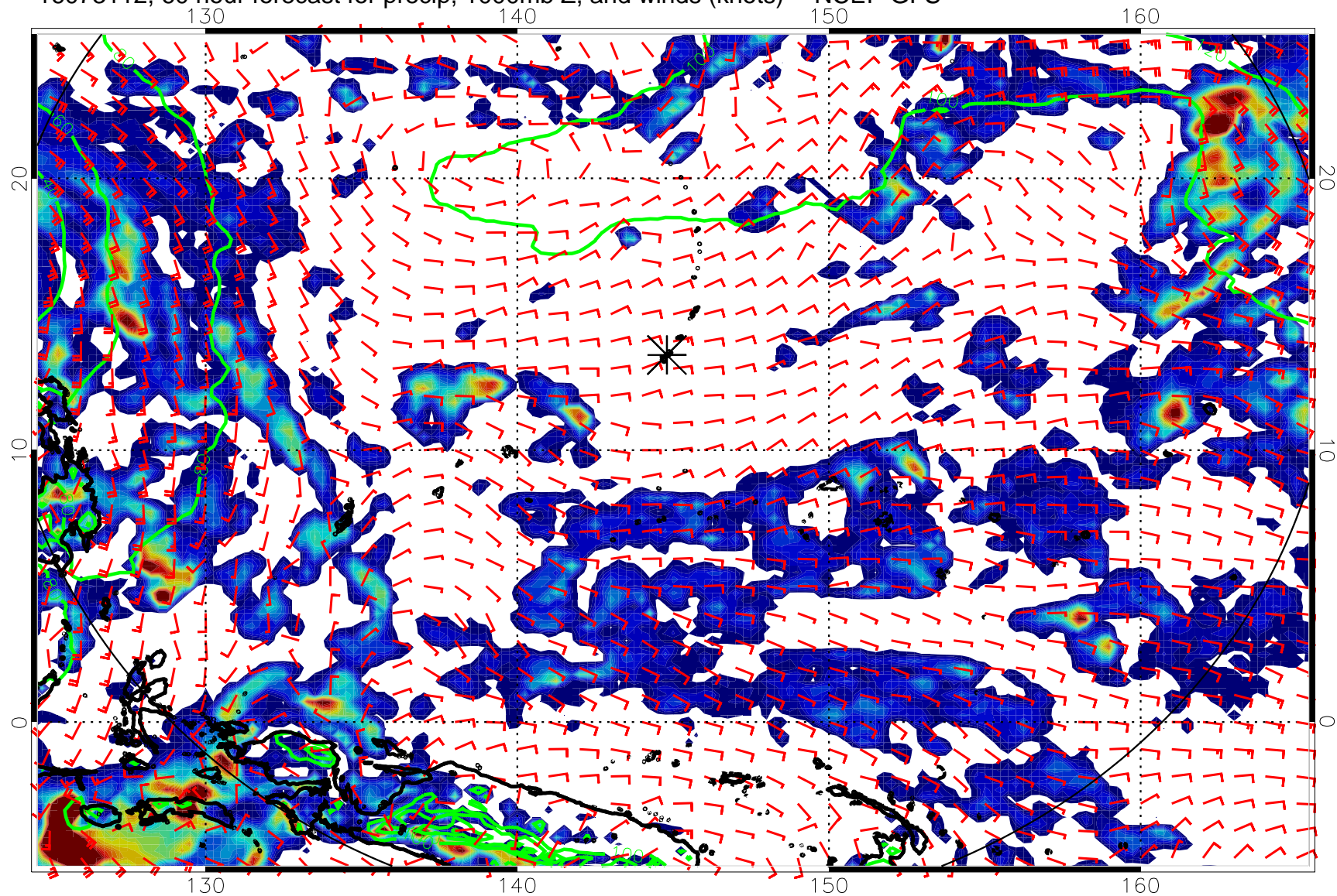
16073112, 60 hour forecast for precip, 1000mb Z, and winds (knots) -- NCEP GFS
