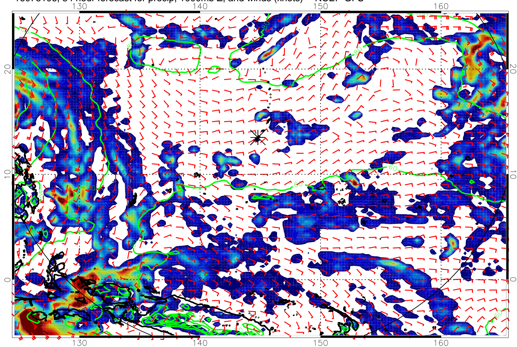
16073106, 54 hour forecast for precip, 1000mb Z, and winds (knots) -- NCEP GFS
