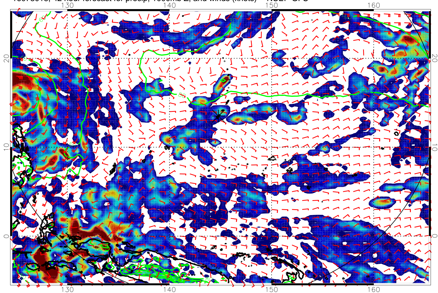
16073018, 42 hour forecast for precip, 1000mb Z, and winds (knots) -- NCEP GFS
