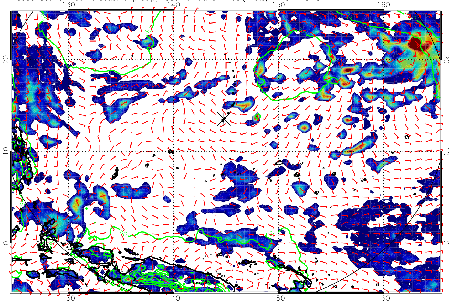
16080206, 102 hour forecast for precip, 1000mb Z, and winds (knots) -- NCEP GFS
