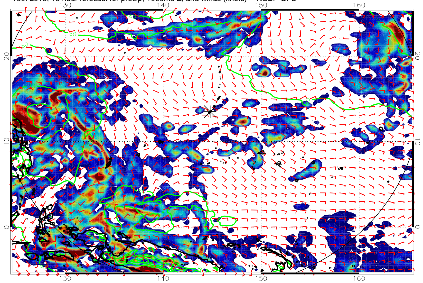
16072918, 18 hour forecast for precip, 1000mb Z, and winds (knots) -- NCEP GFS
