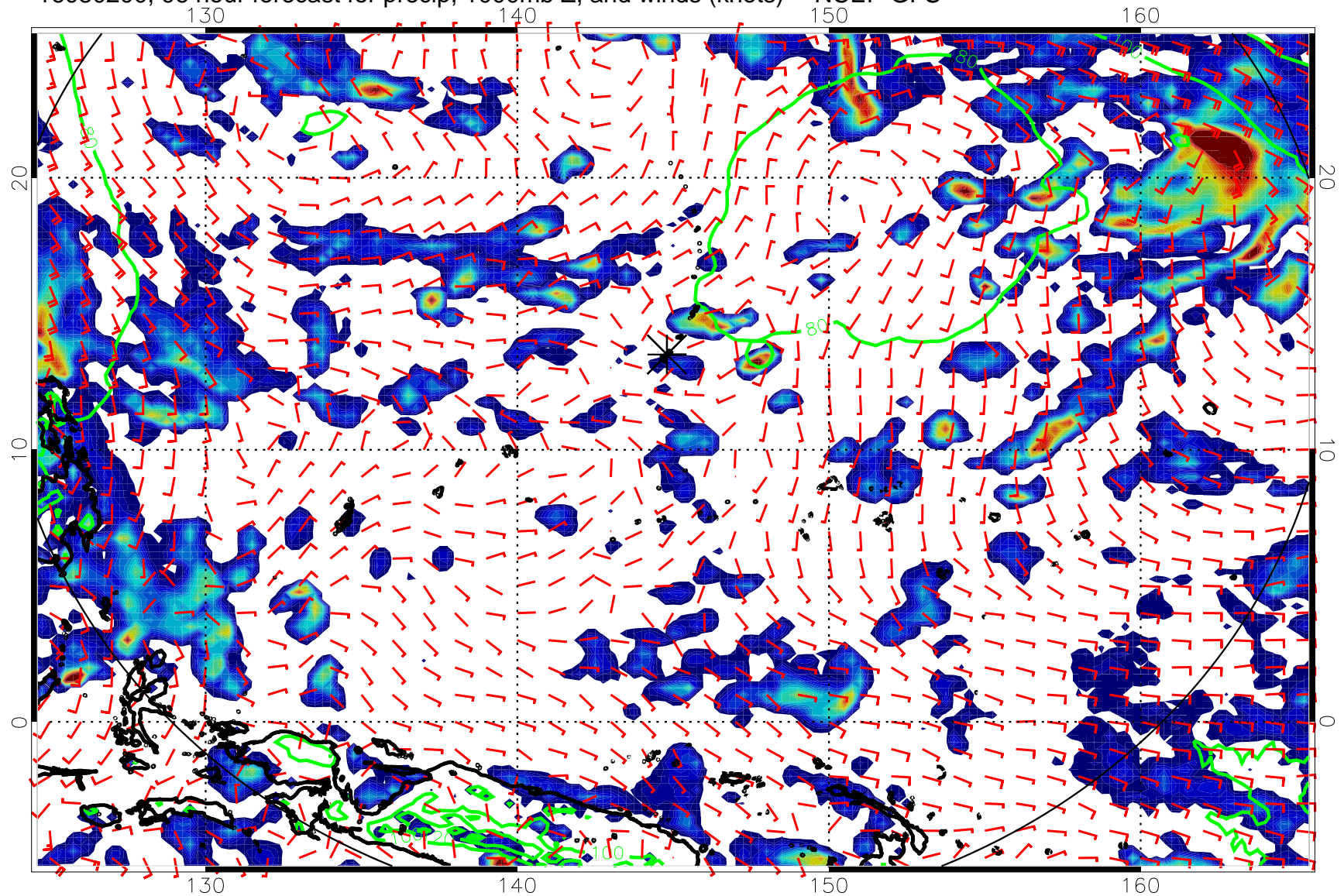
16080200, 96 hour forecast for precip, 1000mb Z, and winds (knots) -- NCEP GFS
