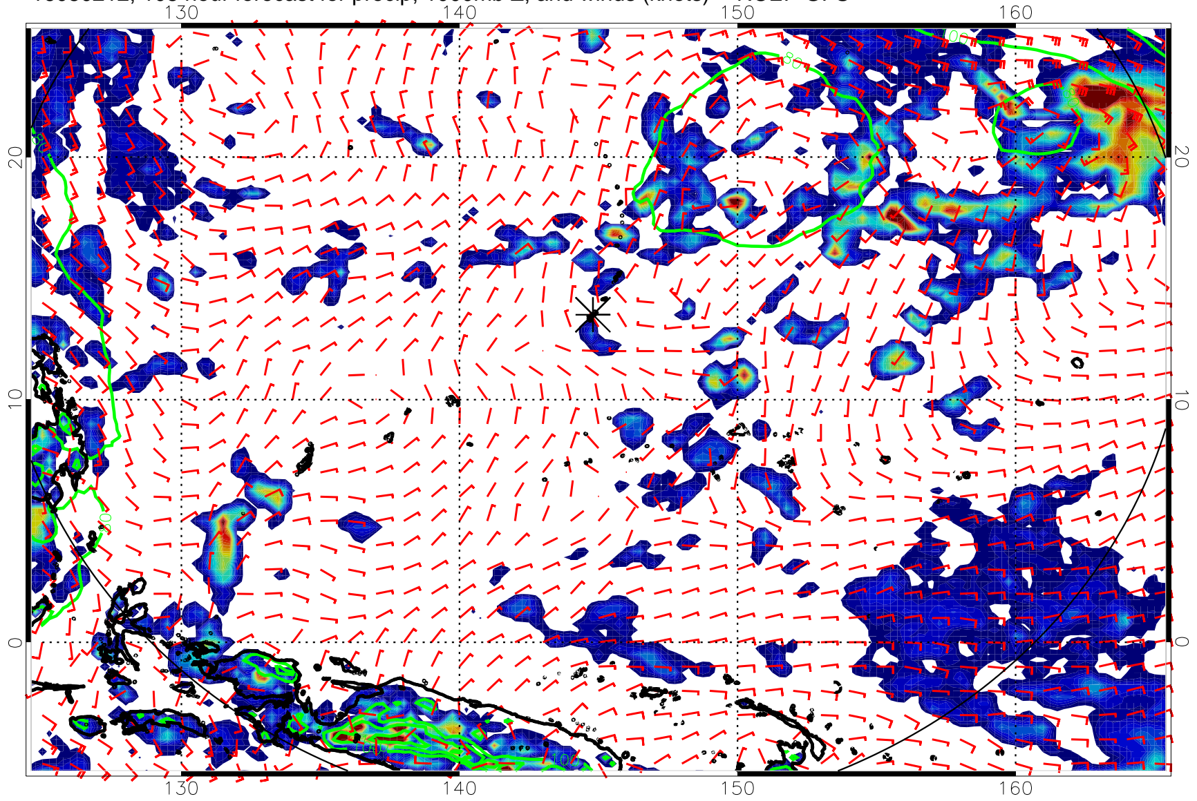
16080212, 108 hour forecast for precip, 1000mb Z, and winds (knots) -- NCEP GFS
