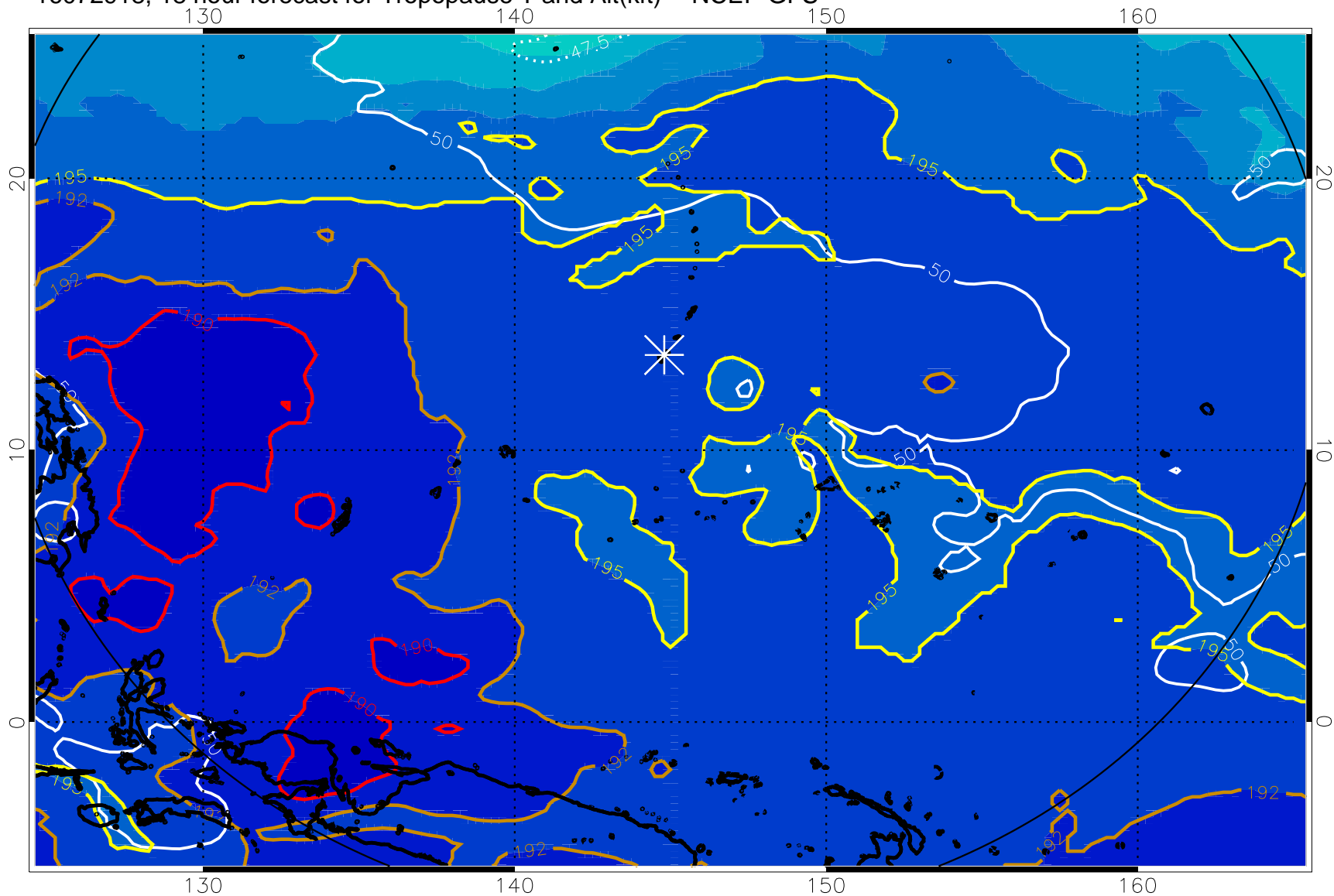
16072918, 18 hour forecast for Tropopause T and Alt(kft) -- NCEP GFS
