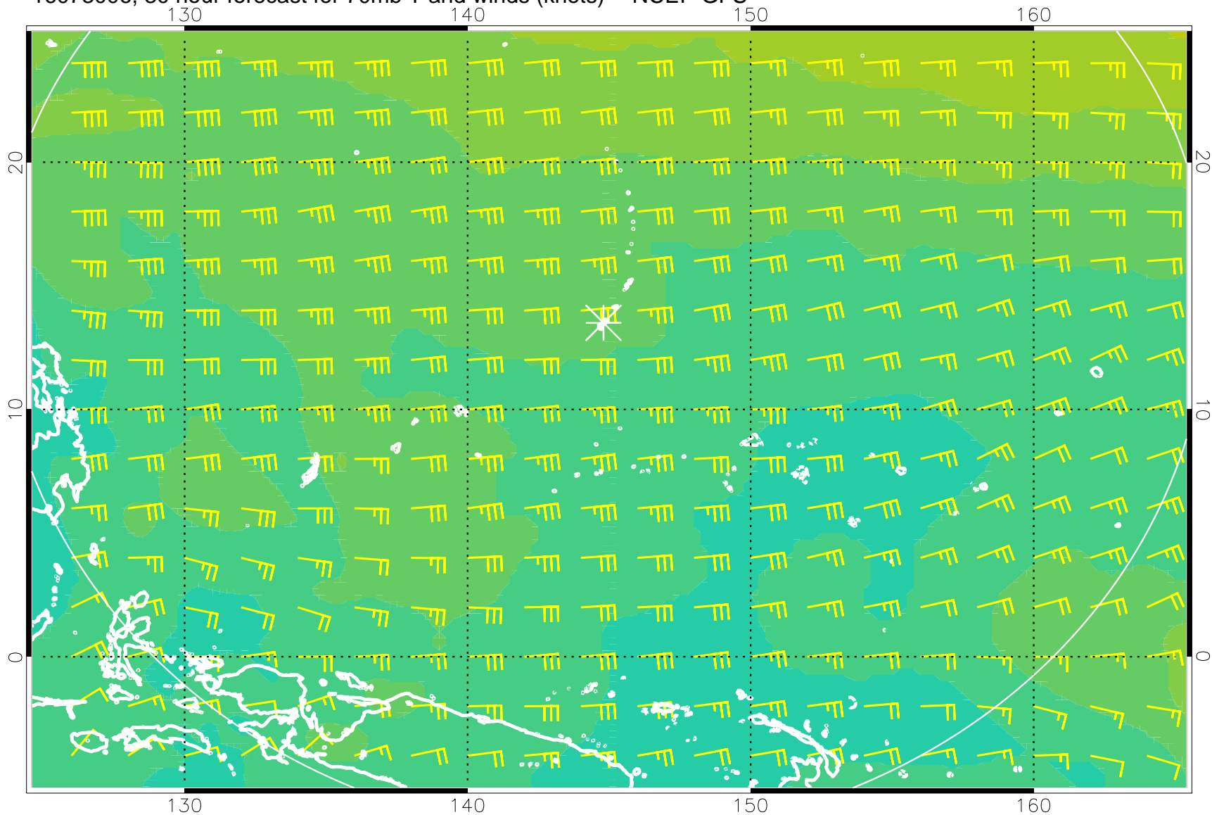
16073006, 30 hour forecast for 70mb T and winds (knots) -- NCEP GFS
