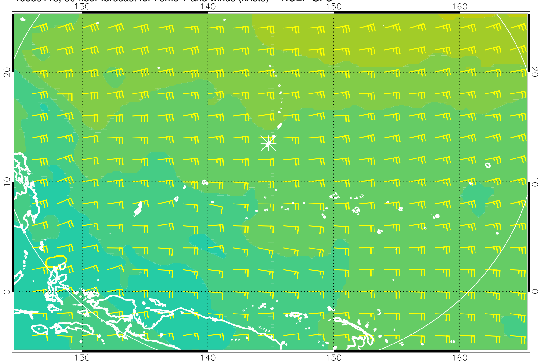
16080118, 90 hour forecast for 70mb T and winds (knots) -- NCEP GFS
