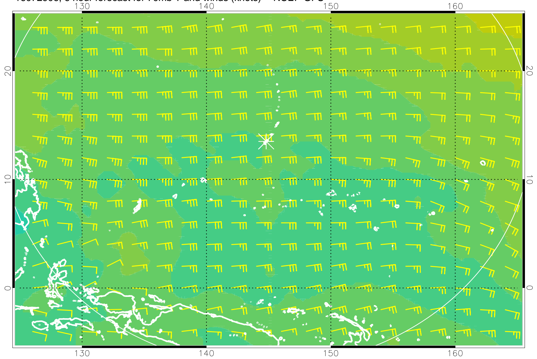
16072906, 6 hour forecast for 70mb T and winds (knots) -- NCEP GFS
