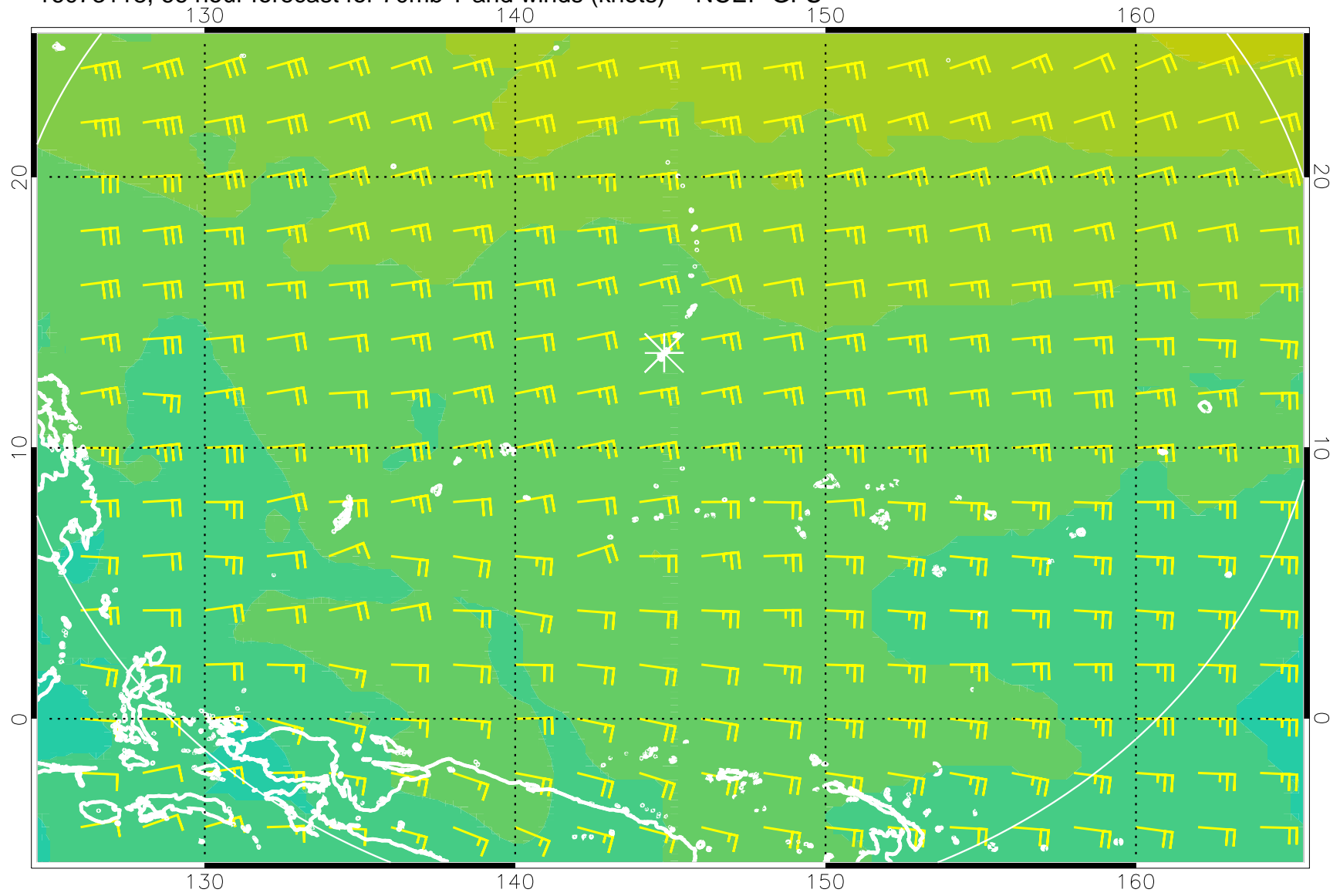
16073118, 66 hour forecast for 70mb T and winds (knots) -- NCEP GFS
