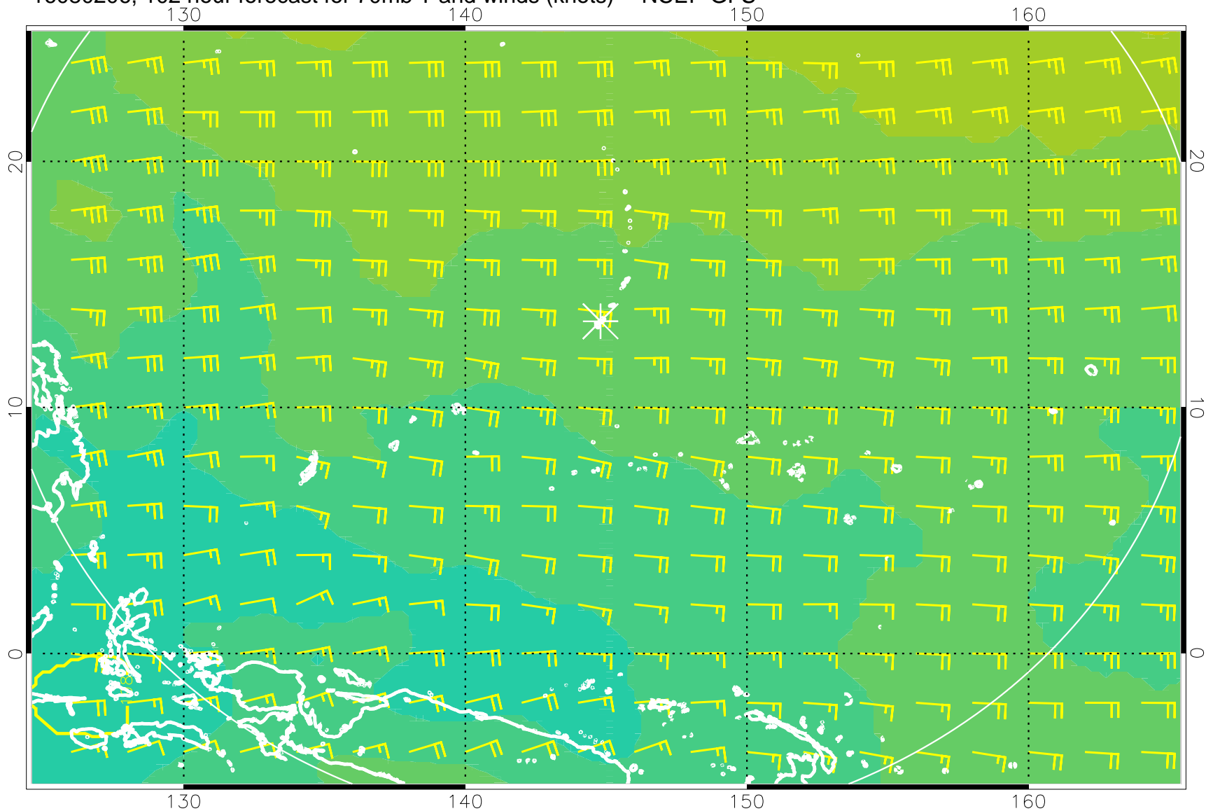
16080206, 102 hour forecast for 70mb T and winds (knots) -- NCEP GFS
