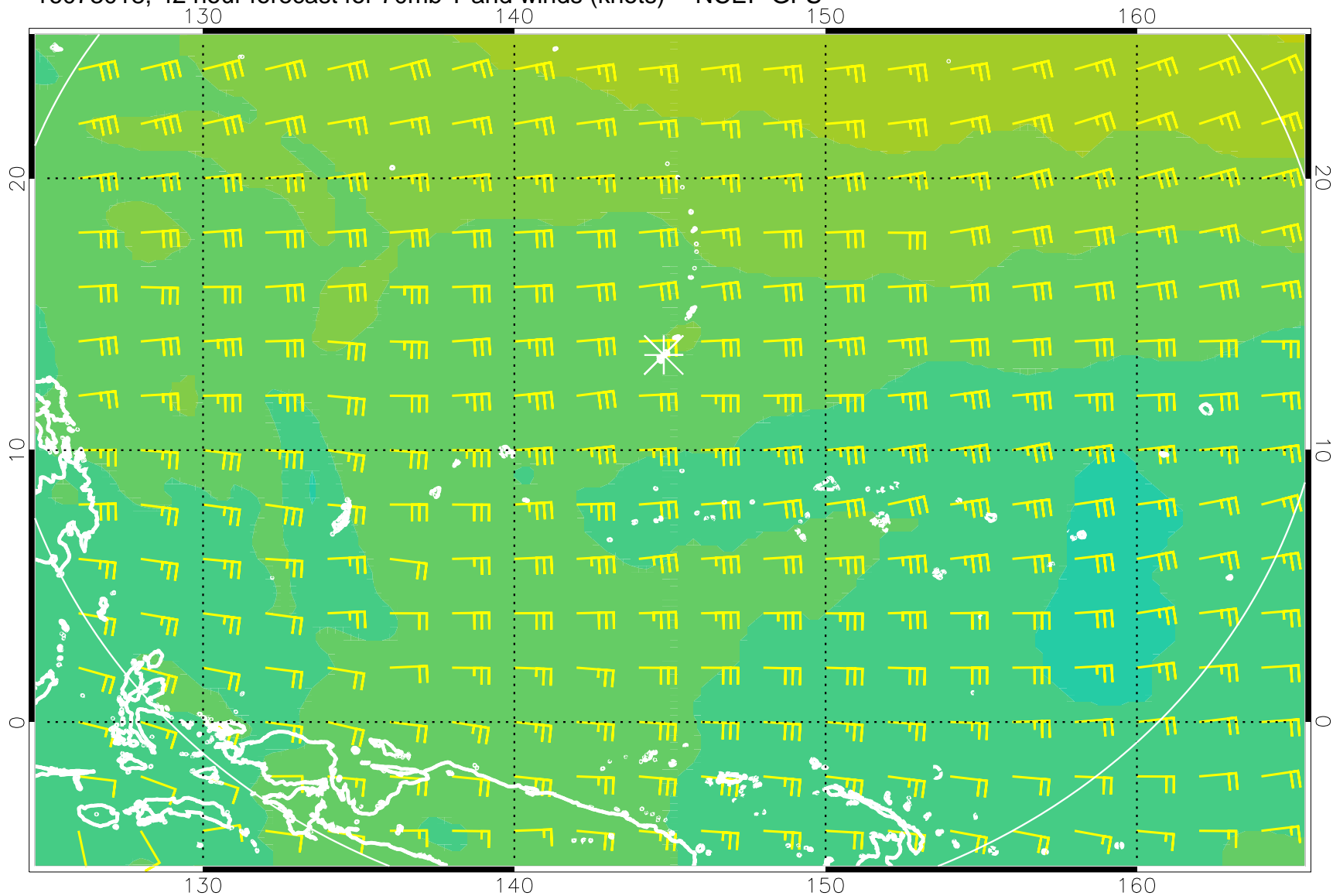
16073018, 42 hour forecast for 70mb T and winds (knots) -- NCEP GFS
