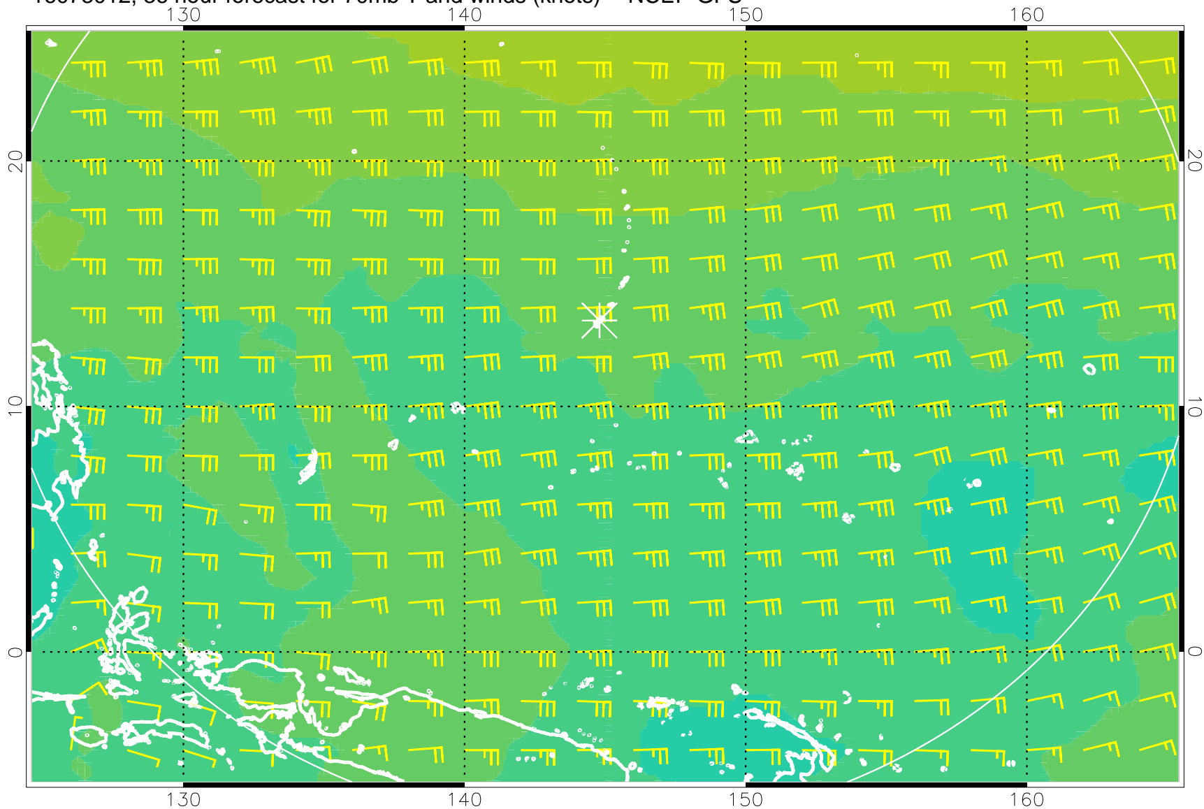
16073012, 36 hour forecast for 70mb T and winds (knots) -- NCEP GFS
