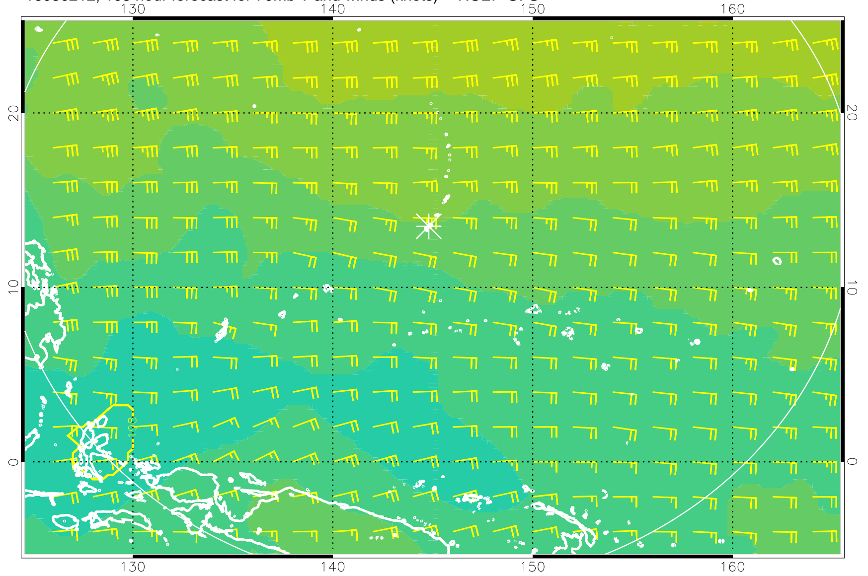
16080212, 108 hour forecast for 70mb T and winds (knots) -- NCEP GFS
