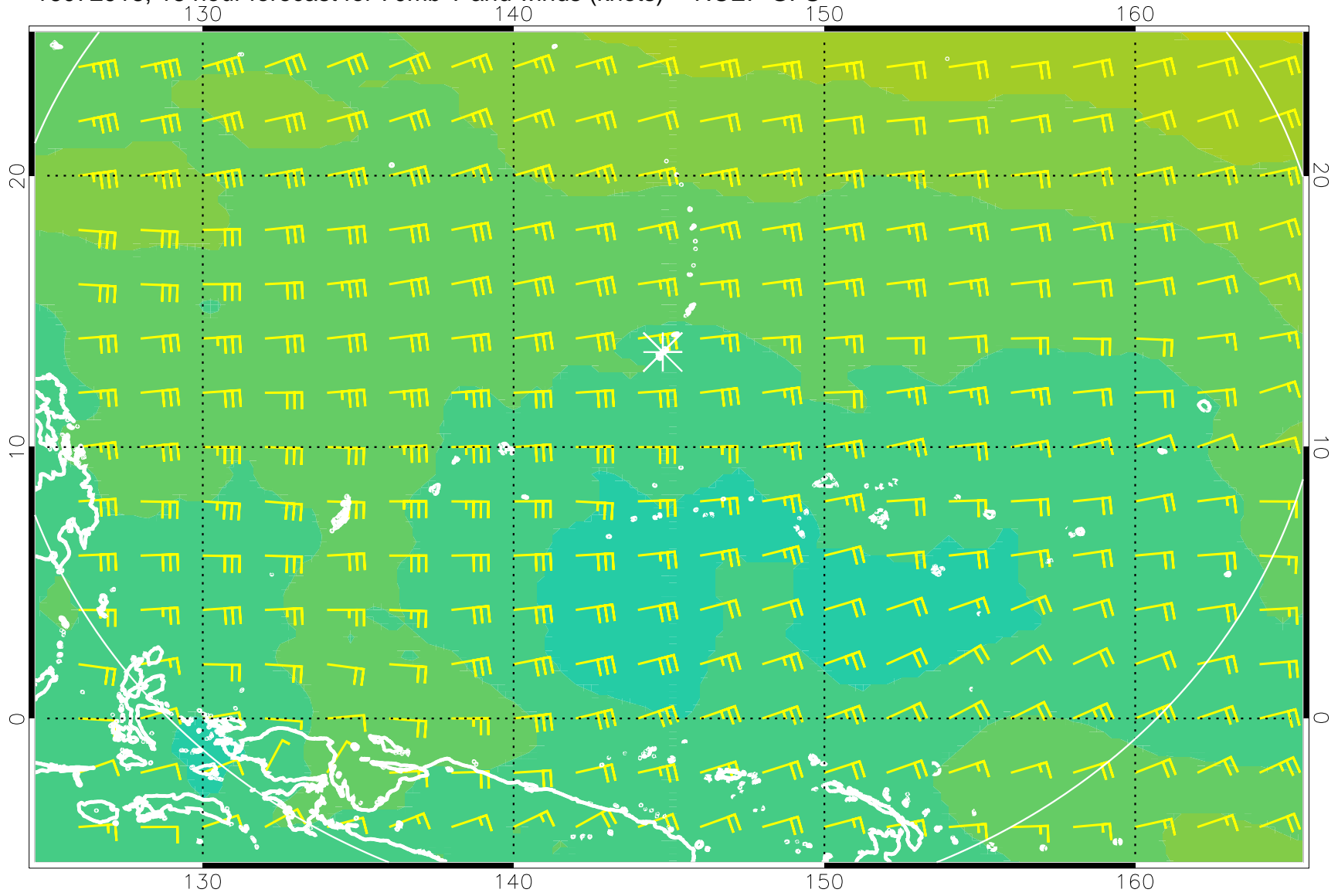
16072918, 18 hour forecast for 70mb T and winds (knots) -- NCEP GFS
