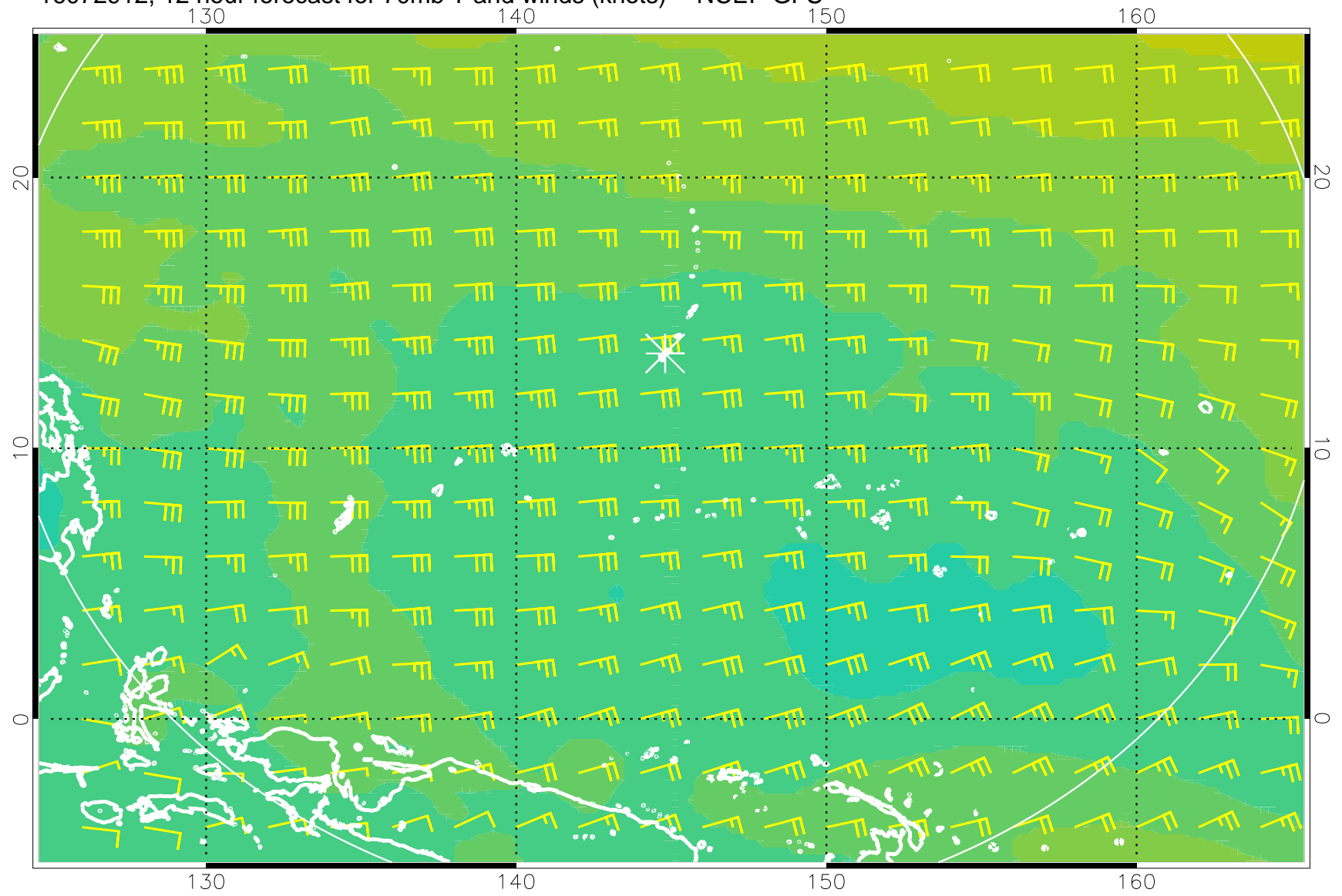
16072912, 12 hour forecast for 70mb T and winds (knots) -- NCEP GFS
