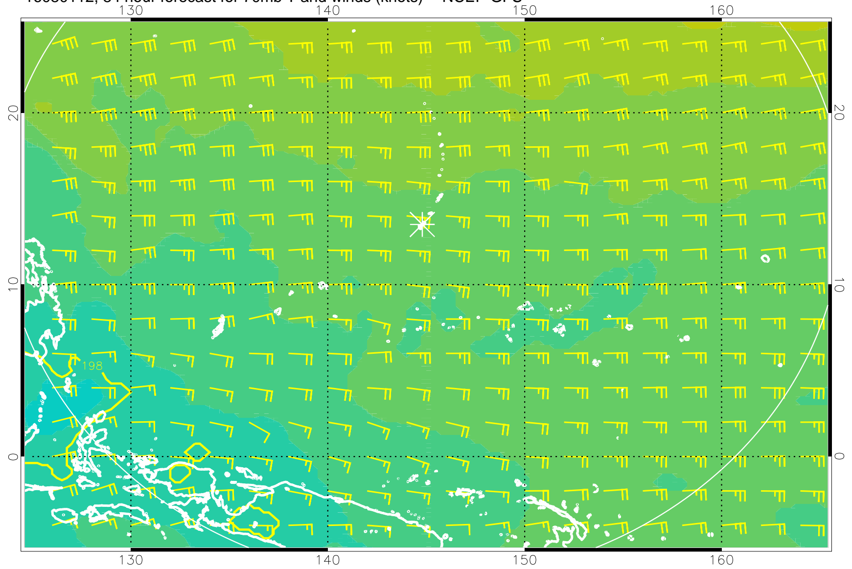
16080112, 84 hour forecast for 70mb T and winds (knots) -- NCEP GFS
