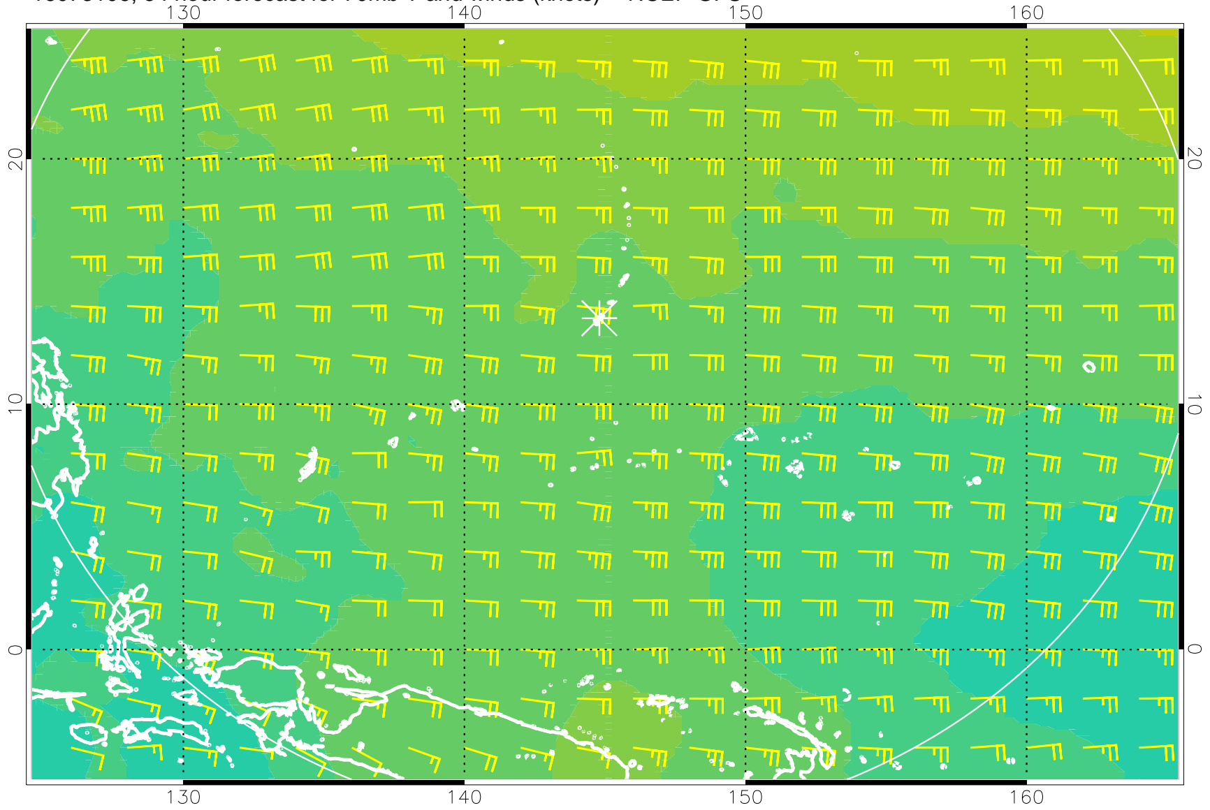
16073106, 54 hour forecast for 70mb T and winds (knots) -- NCEP GFS
