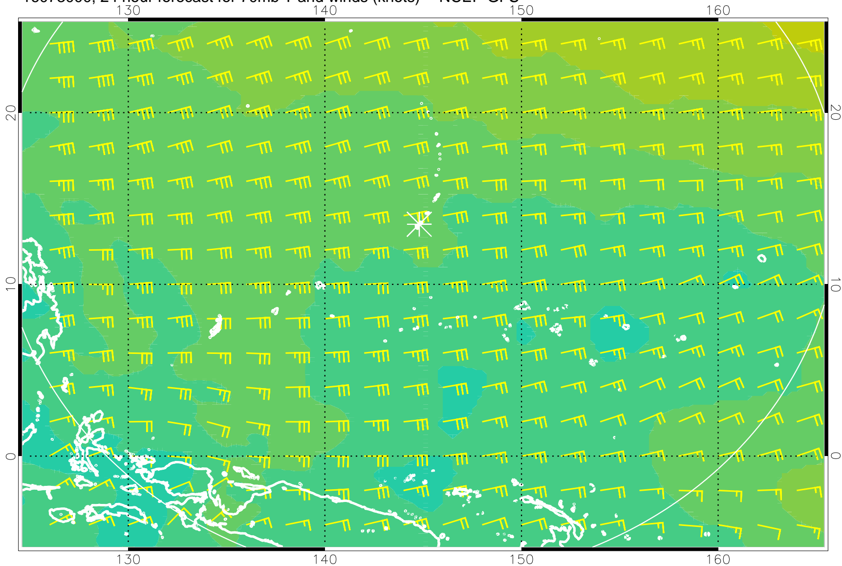
16073000, 24 hour forecast for 70mb T and winds (knots) -- NCEP GFS
