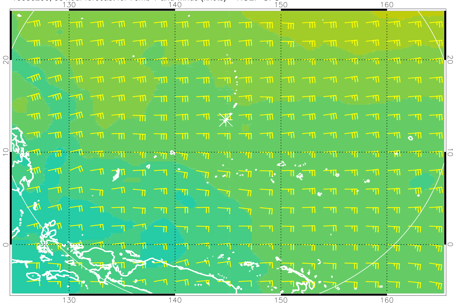
16080200, 96 hour forecast for 70mb T and winds (knots) -- NCEP GFS
