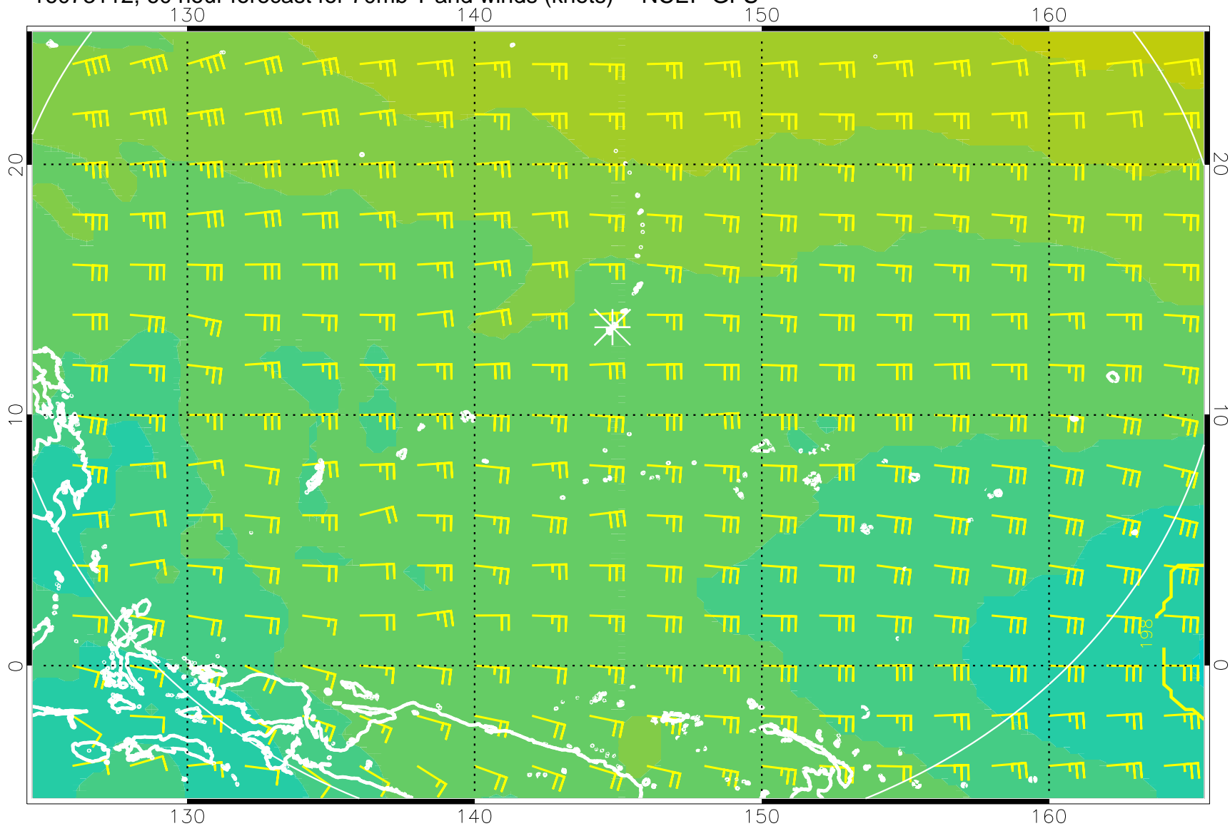
16073112, 60 hour forecast for 70mb T and winds (knots) -- NCEP GFS
