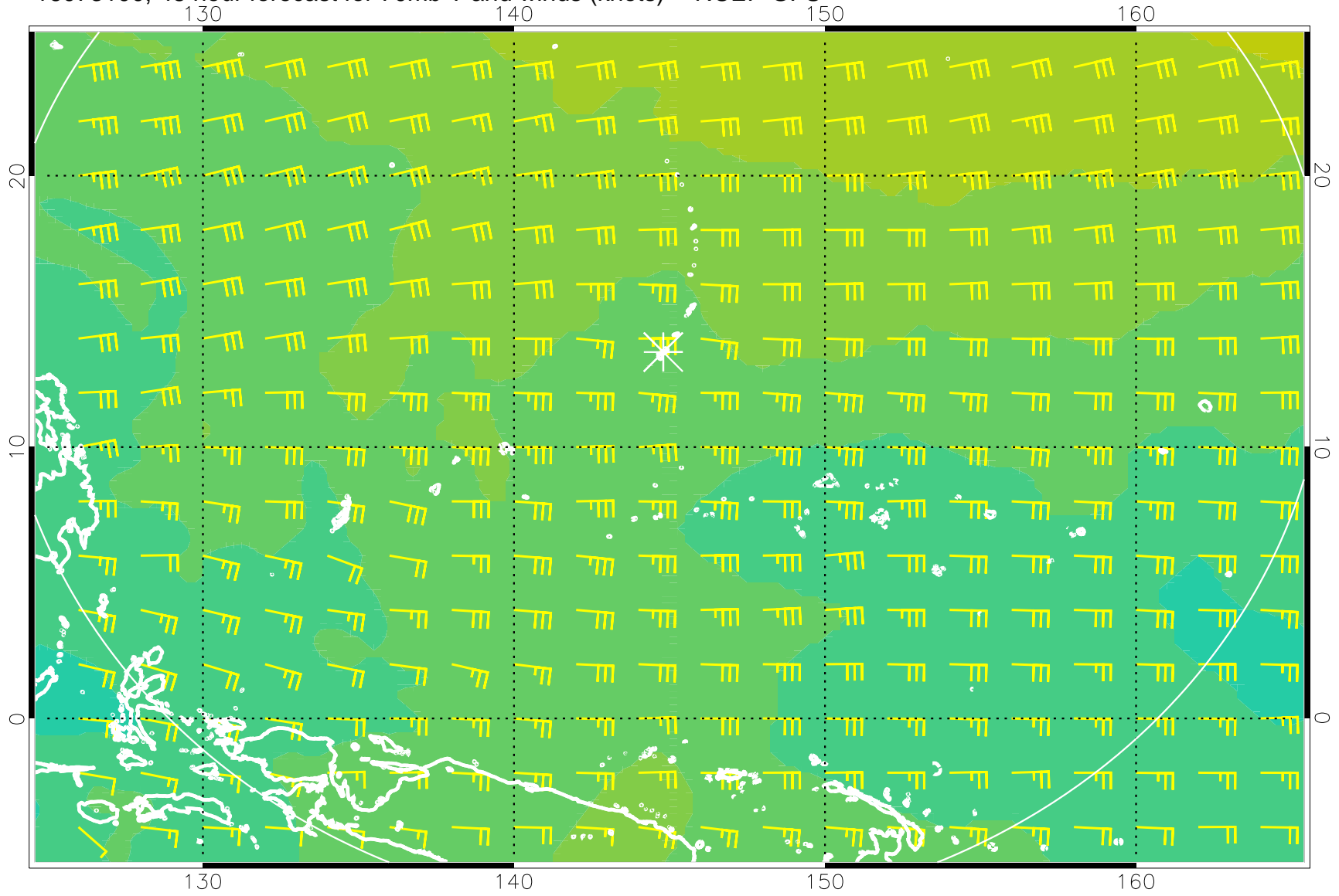
16073100, 48 hour forecast for 70mb T and winds (knots) -- NCEP GFS
