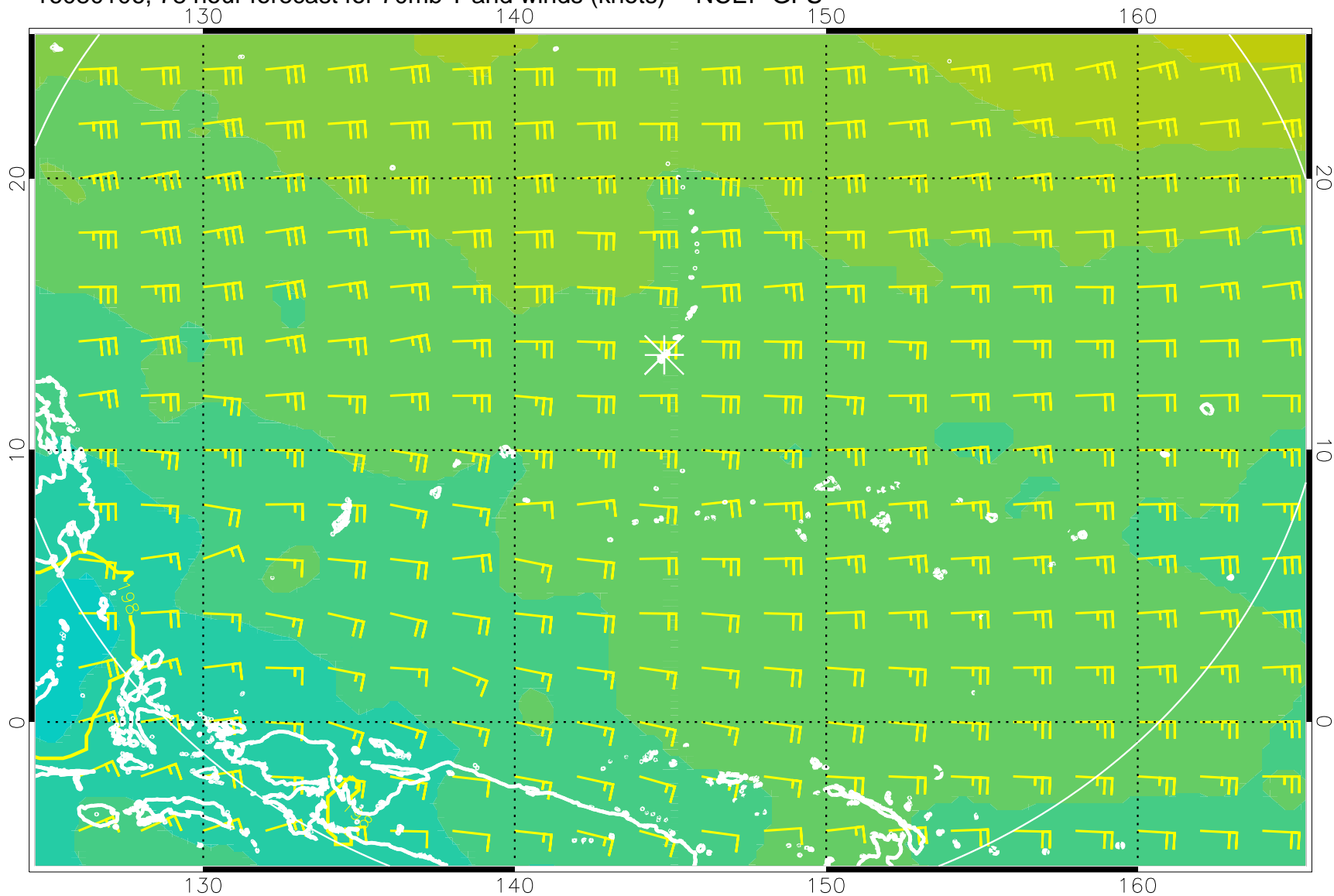
16080106, 78 hour forecast for 70mb T and winds (knots) -- NCEP GFS
