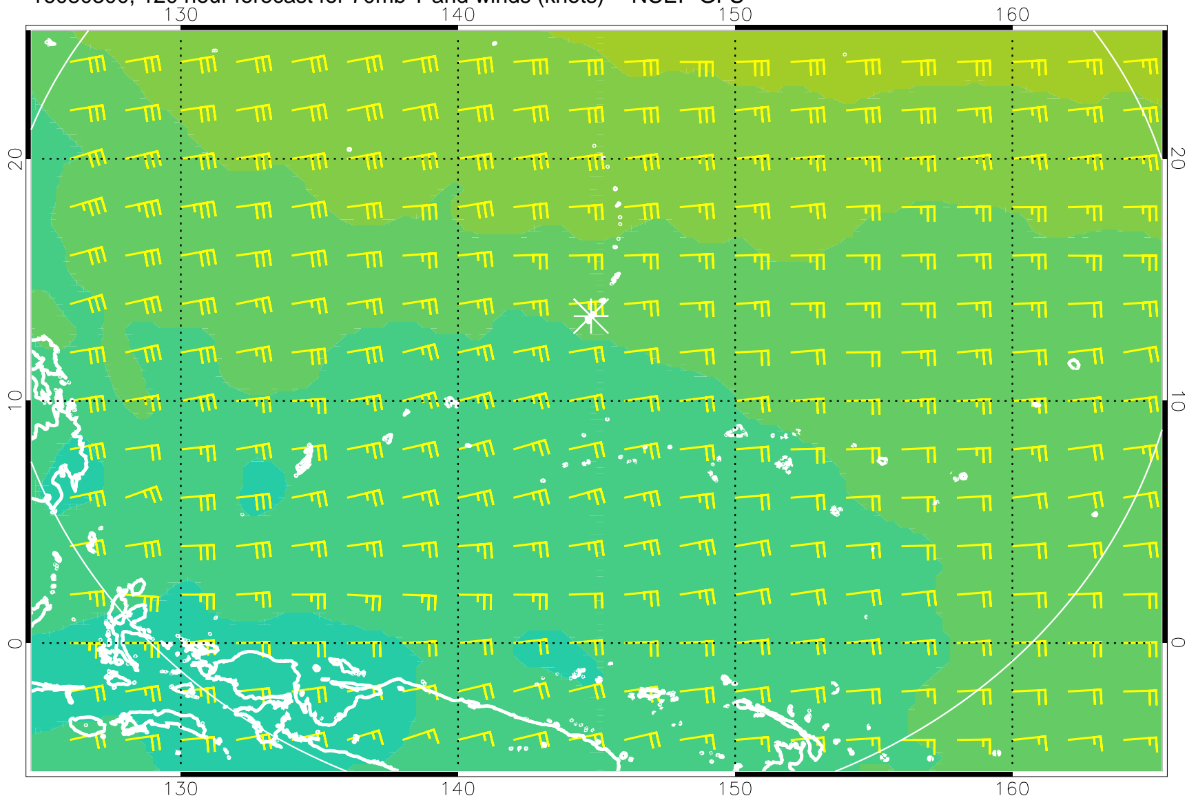
16080300, 120 hour forecast for 70mb T and winds (knots) -- NCEP GFS
