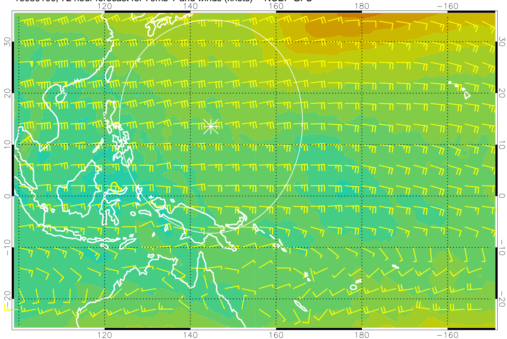
16080100, 72 hour forecast for 70mb T and winds (knots) -- NCEP GFS
