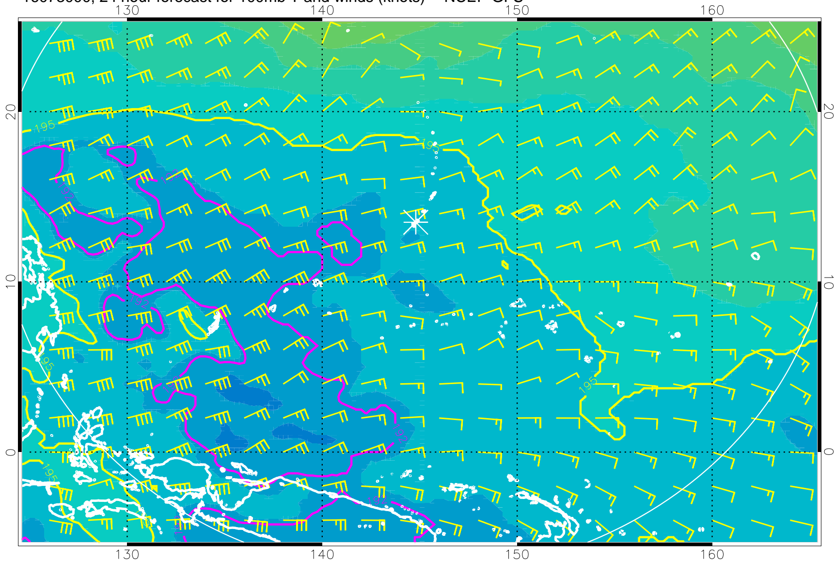
16073000, 24 hour forecast for 100mb T and winds (knots) -- NCEP GFS
