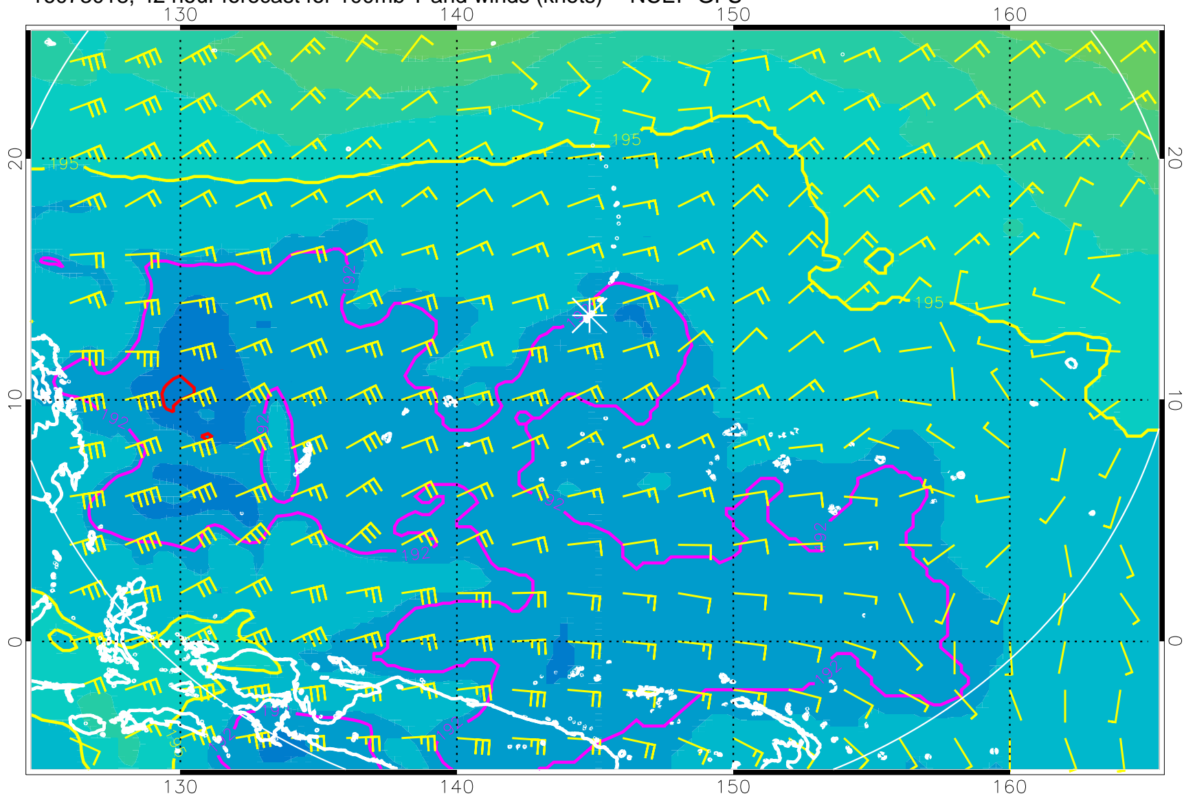
16073018, 42 hour forecast for 100mb T and winds (knots) -- NCEP GFS
