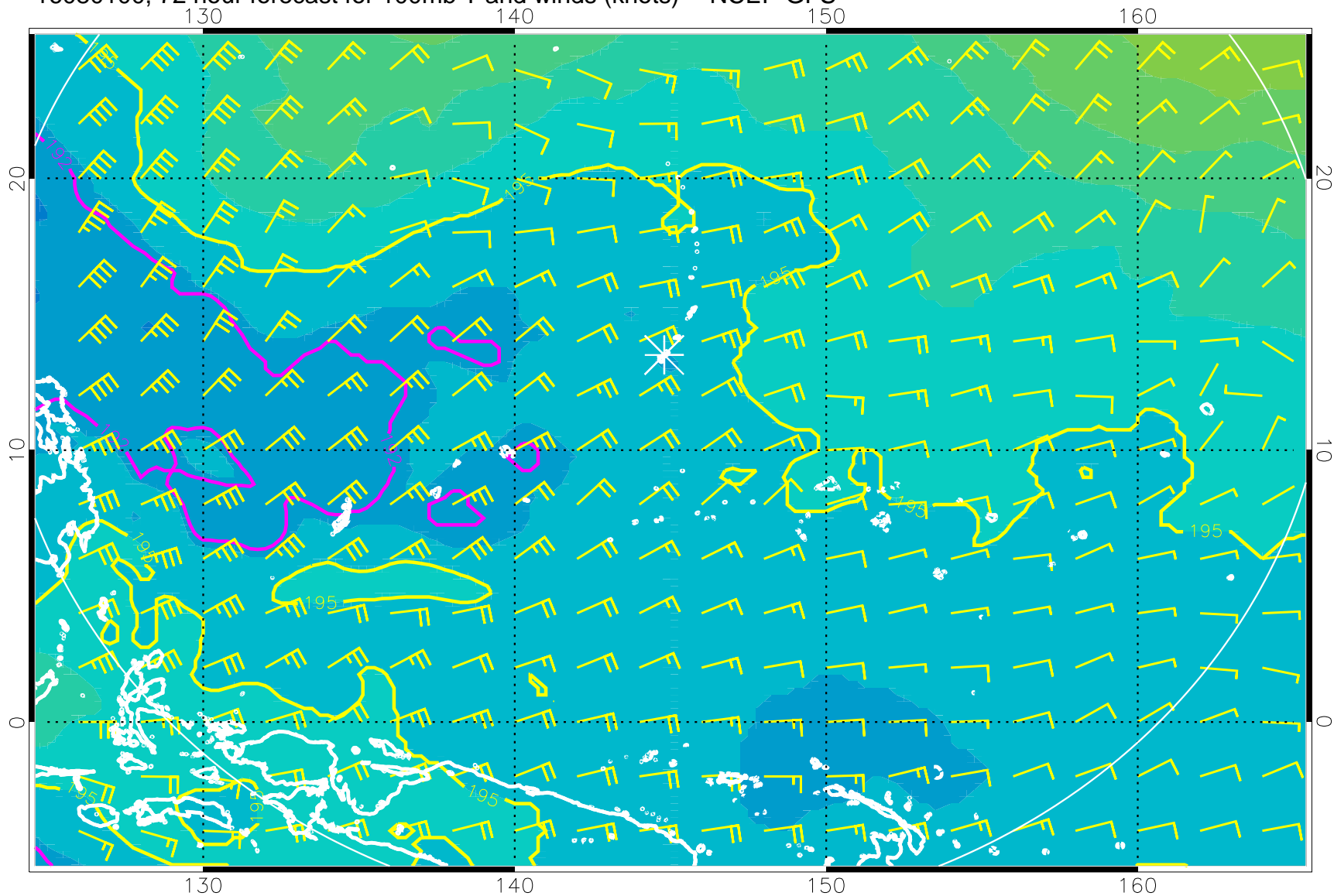
16080100, 72 hour forecast for 100mb T and winds (knots) -- NCEP GFS
