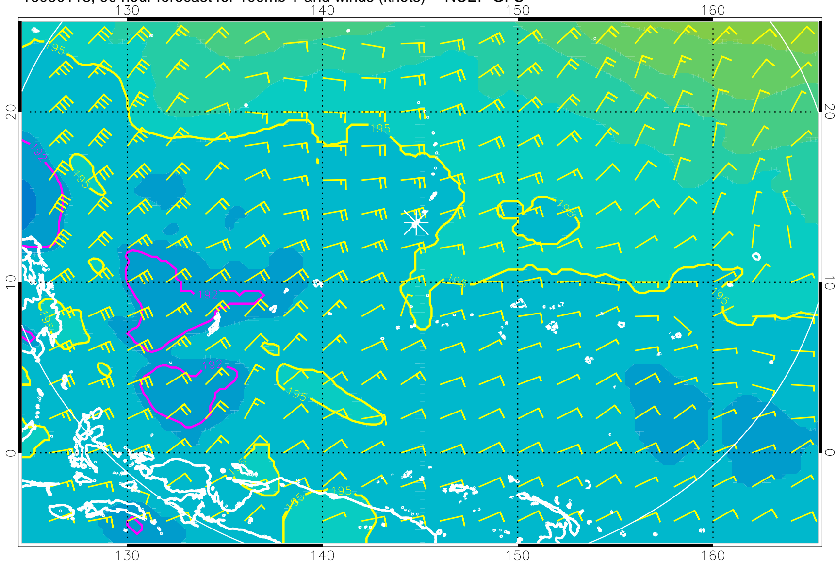
16080118, 90 hour forecast for 100mb T and winds (knots) -- NCEP GFS
