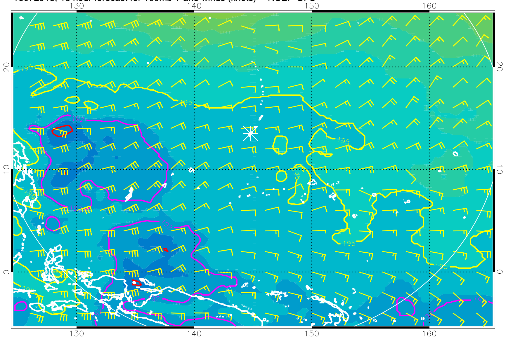
16072918, 18 hour forecast for 100mb T and winds (knots) -- NCEP GFS
