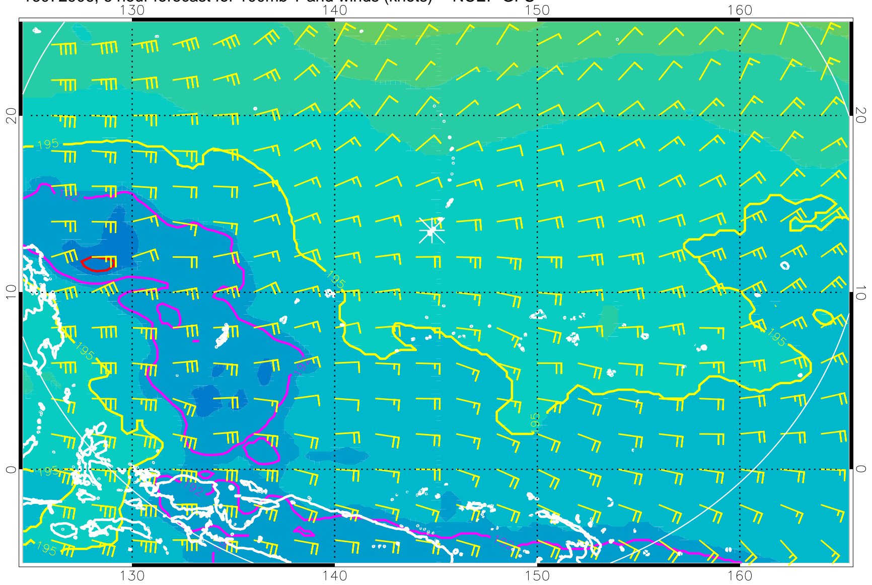
16072906, 6 hour forecast for 100mb T and winds (knots) -- NCEP GFS
