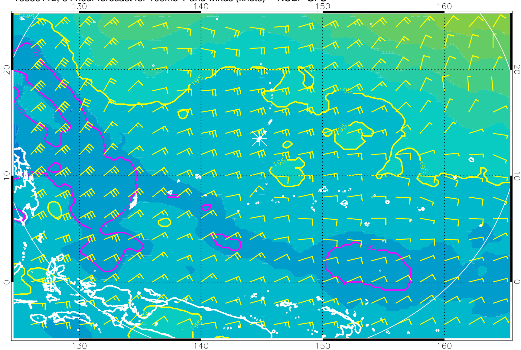
16080112, 84 hour forecast for 100mb T and winds (knots) -- NCEP GFS
