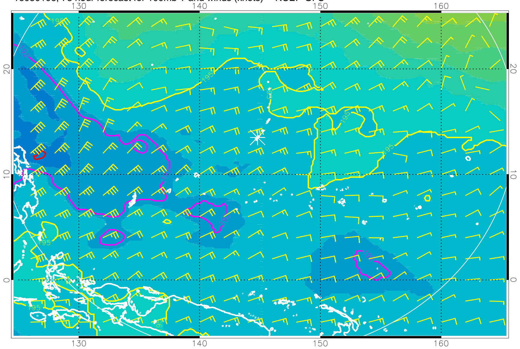
16080106, 78 hour forecast for 100mb T and winds (knots) -- NCEP GFS
