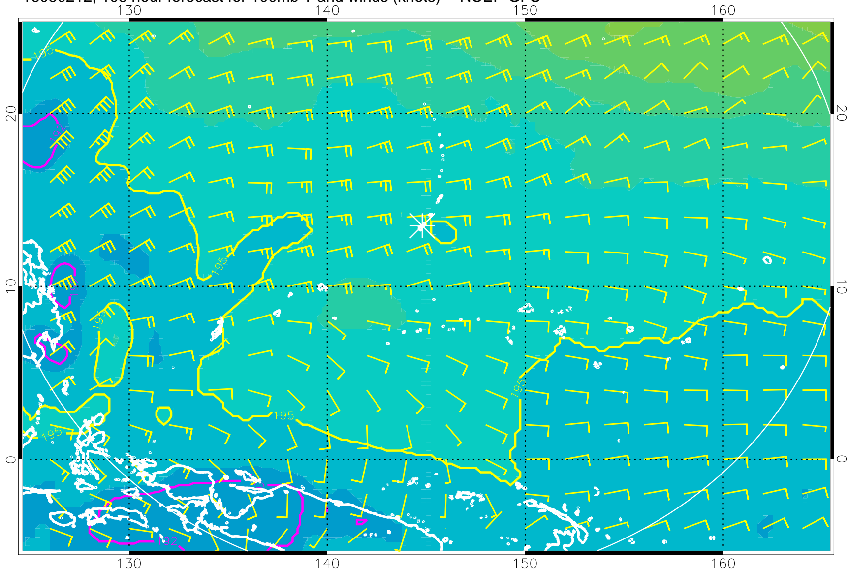
16080212, 108 hour forecast for 100mb T and winds (knots) -- NCEP GFS
