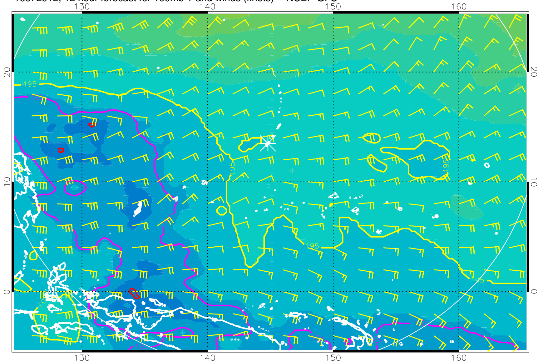
16072912, 12 hour forecast for 100mb T and winds (knots) -- NCEP GFS
