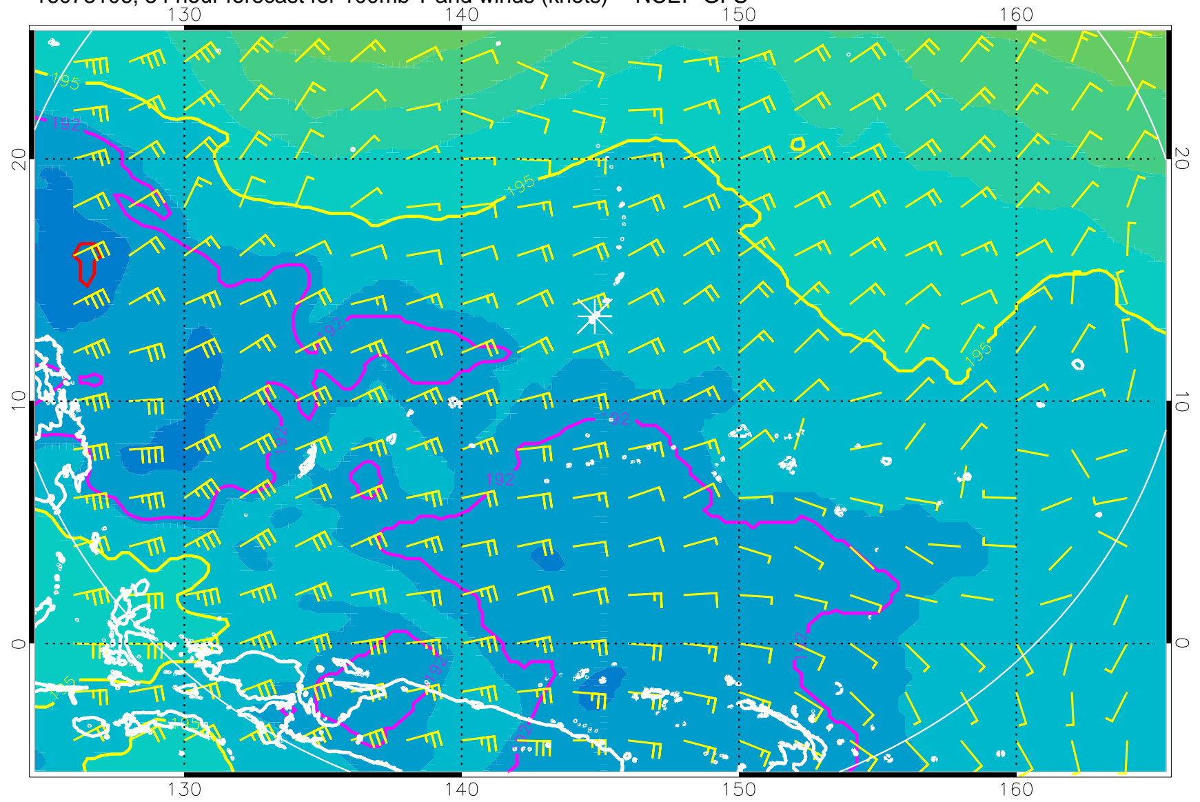
16073106, 54 hour forecast for 100mb T and winds (knots) -- NCEP GFS
