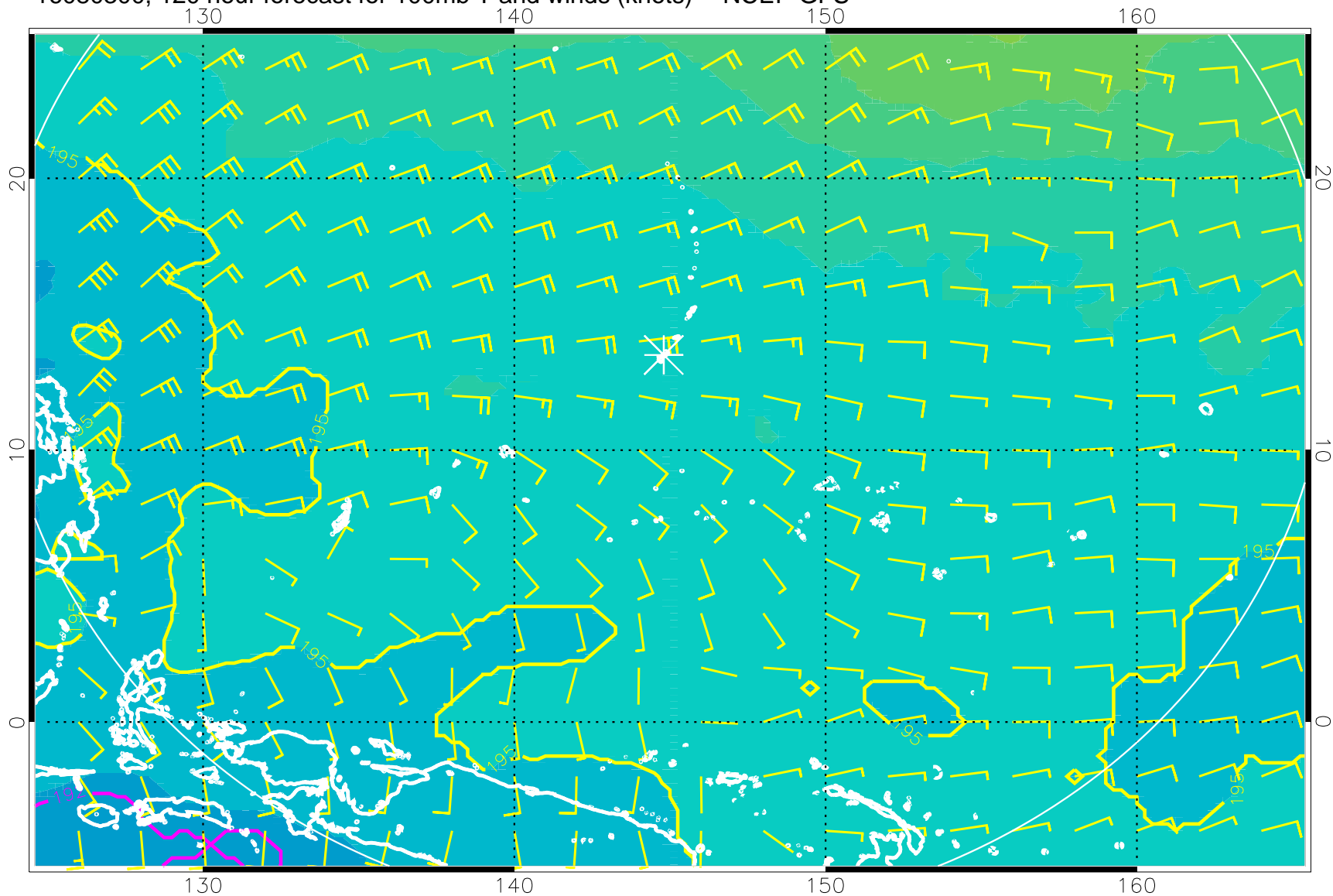
16080300, 120 hour forecast for 100mb T and winds (knots) -- NCEP GFS
