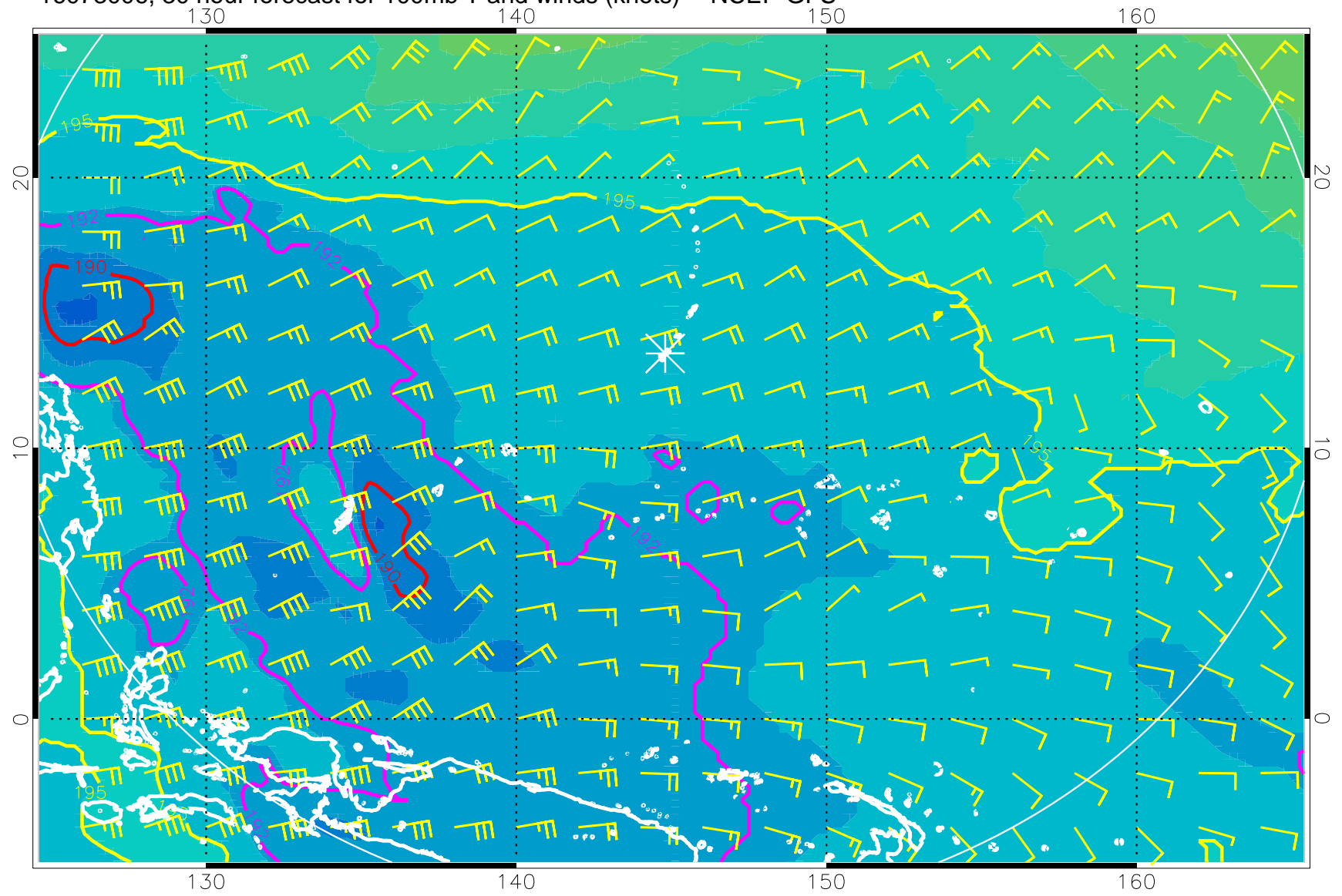
16073006, 30 hour forecast for 100mb T and winds (knots) -- NCEP GFS
