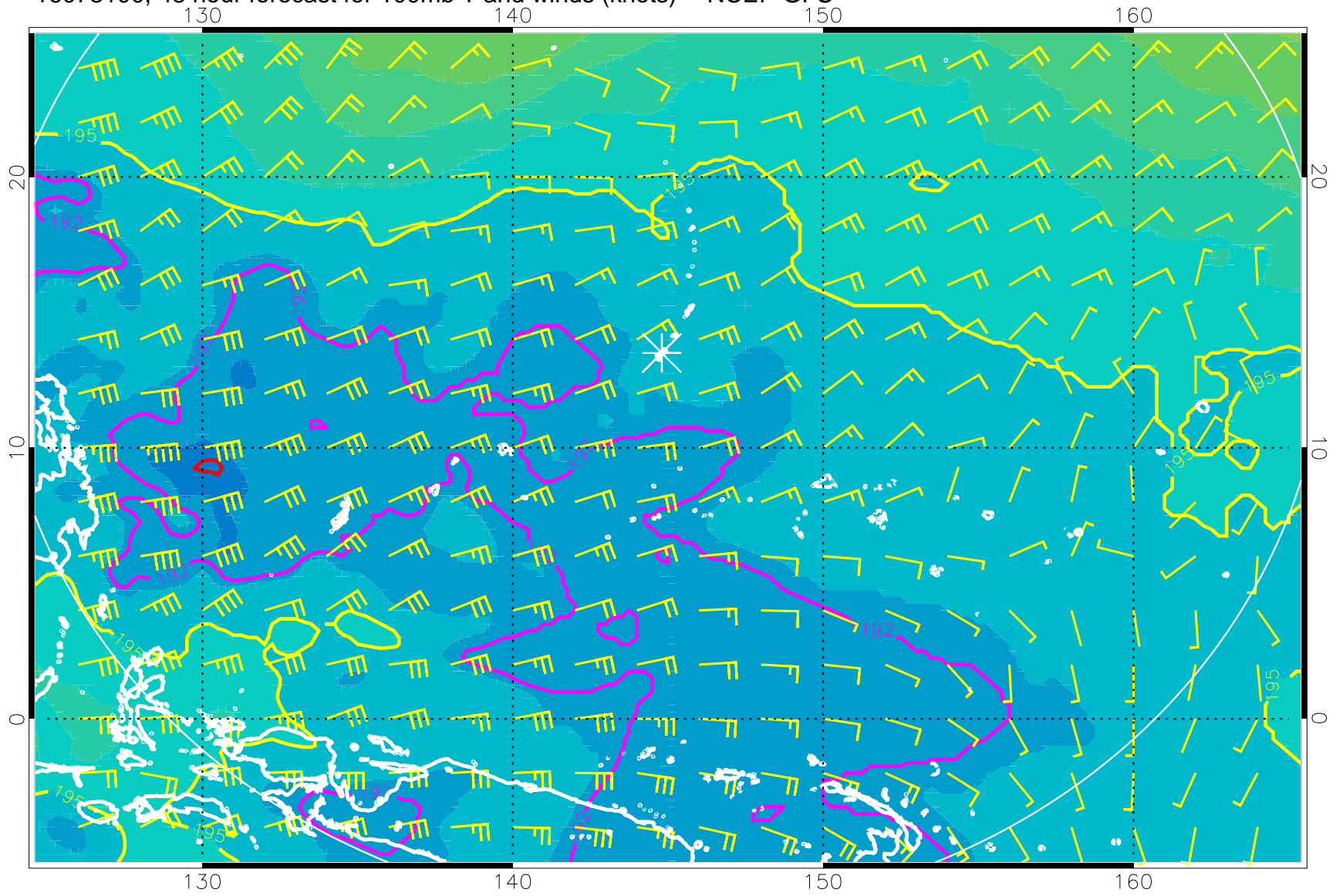
16073100, 48 hour forecast for 100mb T and winds (knots) -- NCEP GFS
