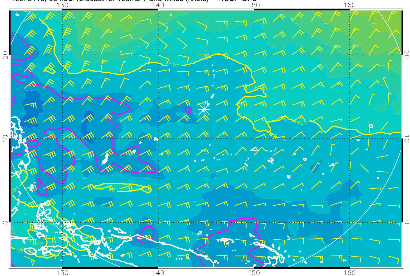
16073118, 66 hour forecast for 100mb T and winds (knots) -- NCEP GFS
