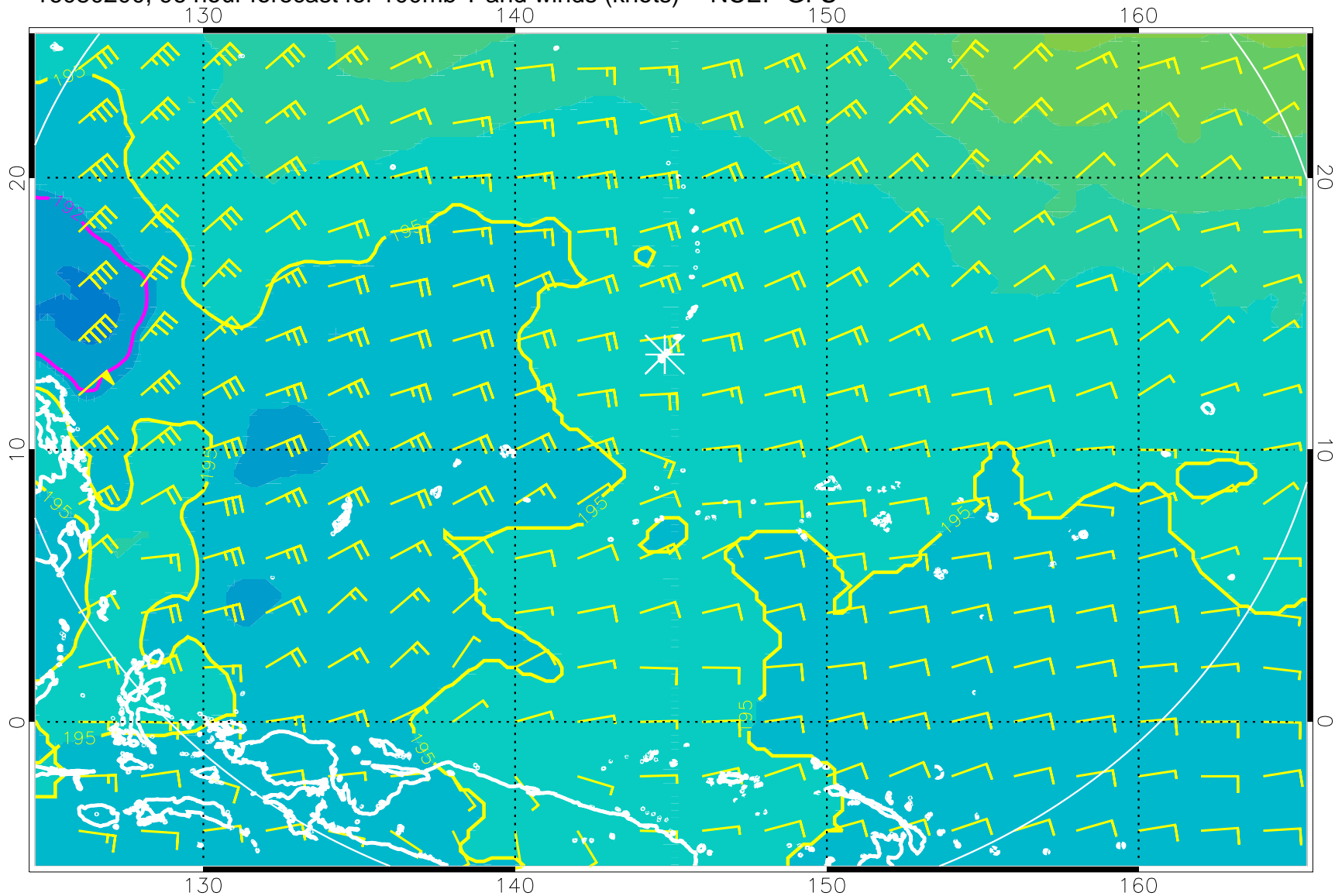
16080200, 96 hour forecast for 100mb T and winds (knots) -- NCEP GFS
