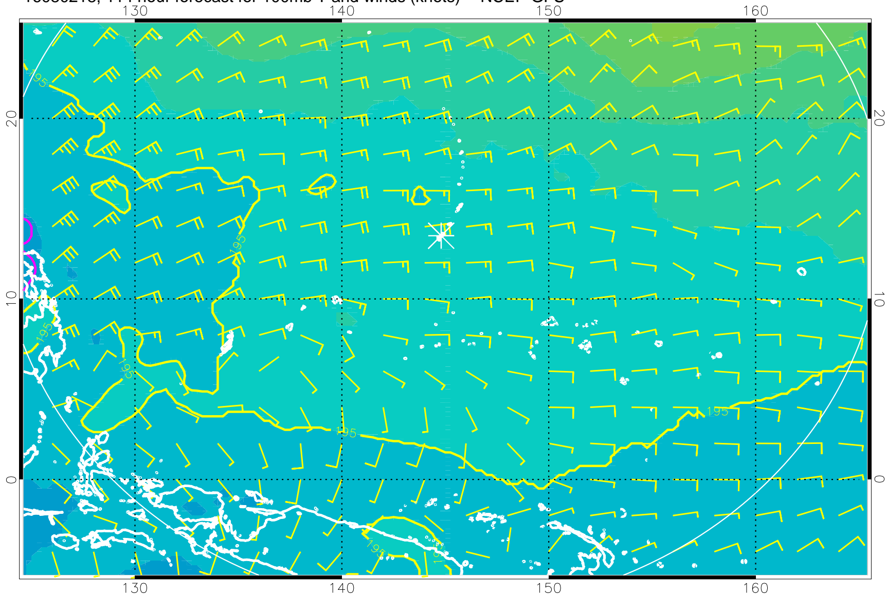
16080218, 114 hour forecast for 100mb T and winds (knots) -- NCEP GFS
