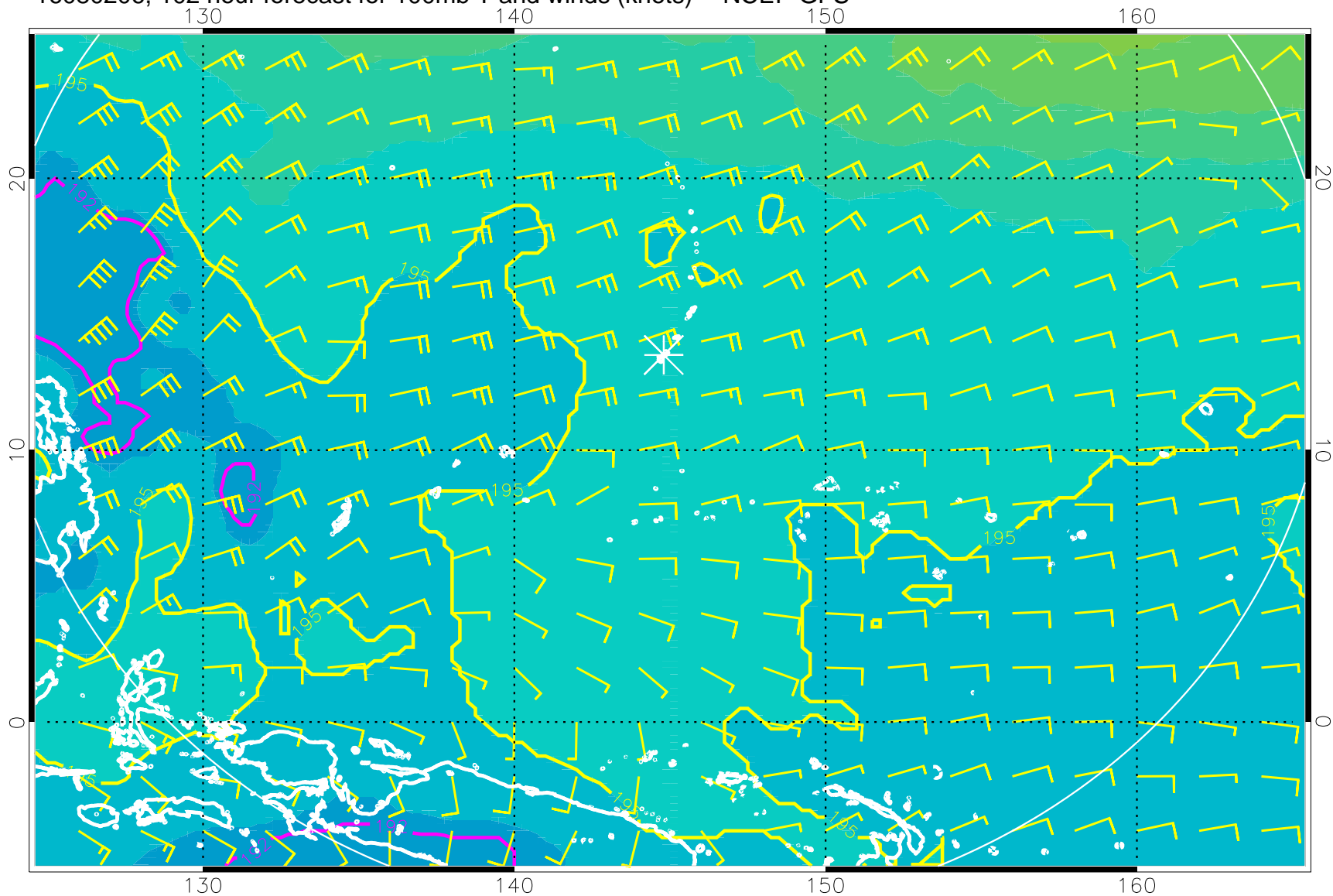
16080206, 102 hour forecast for 100mb T and winds (knots) -- NCEP GFS
