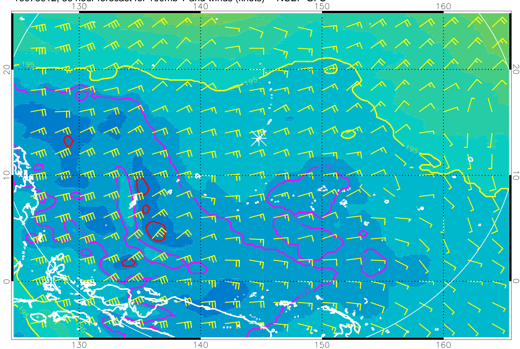
16073012, 36 hour forecast for 100mb T and winds (knots) -- NCEP GFS
