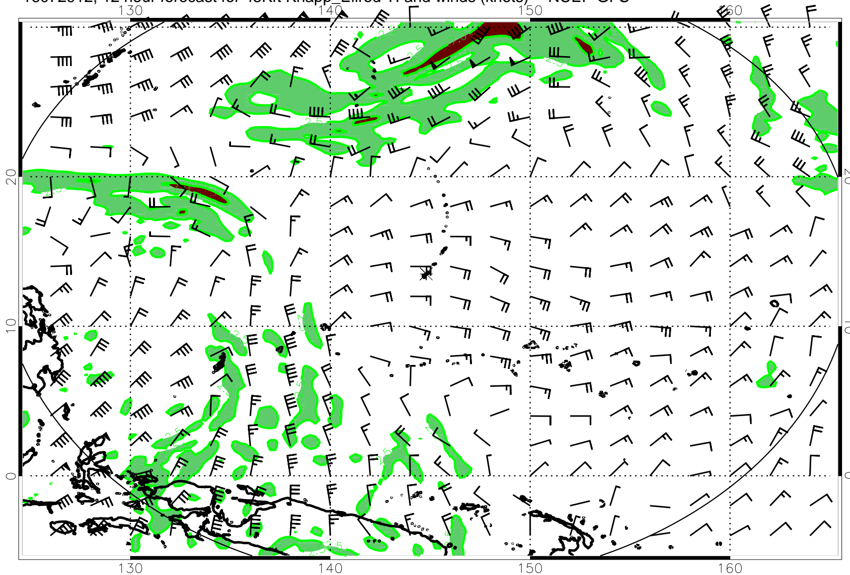
16072912, 12 hour forecast for 45Kft Knapp_Ellrod TI and winds (knots) -- NCEP GFS
