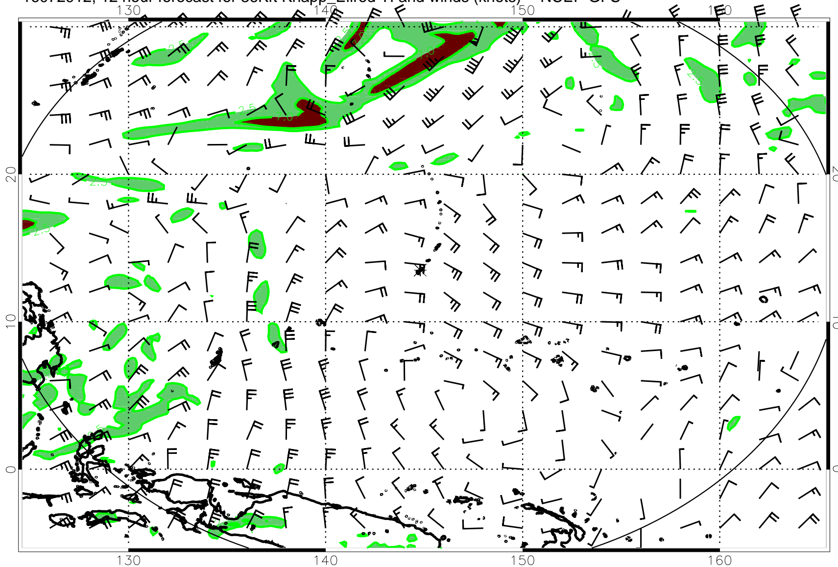
16072912, 12 hour forecast for 36Kft Knapp_Ellrod TI and winds (knots) -- NCEP GFS
