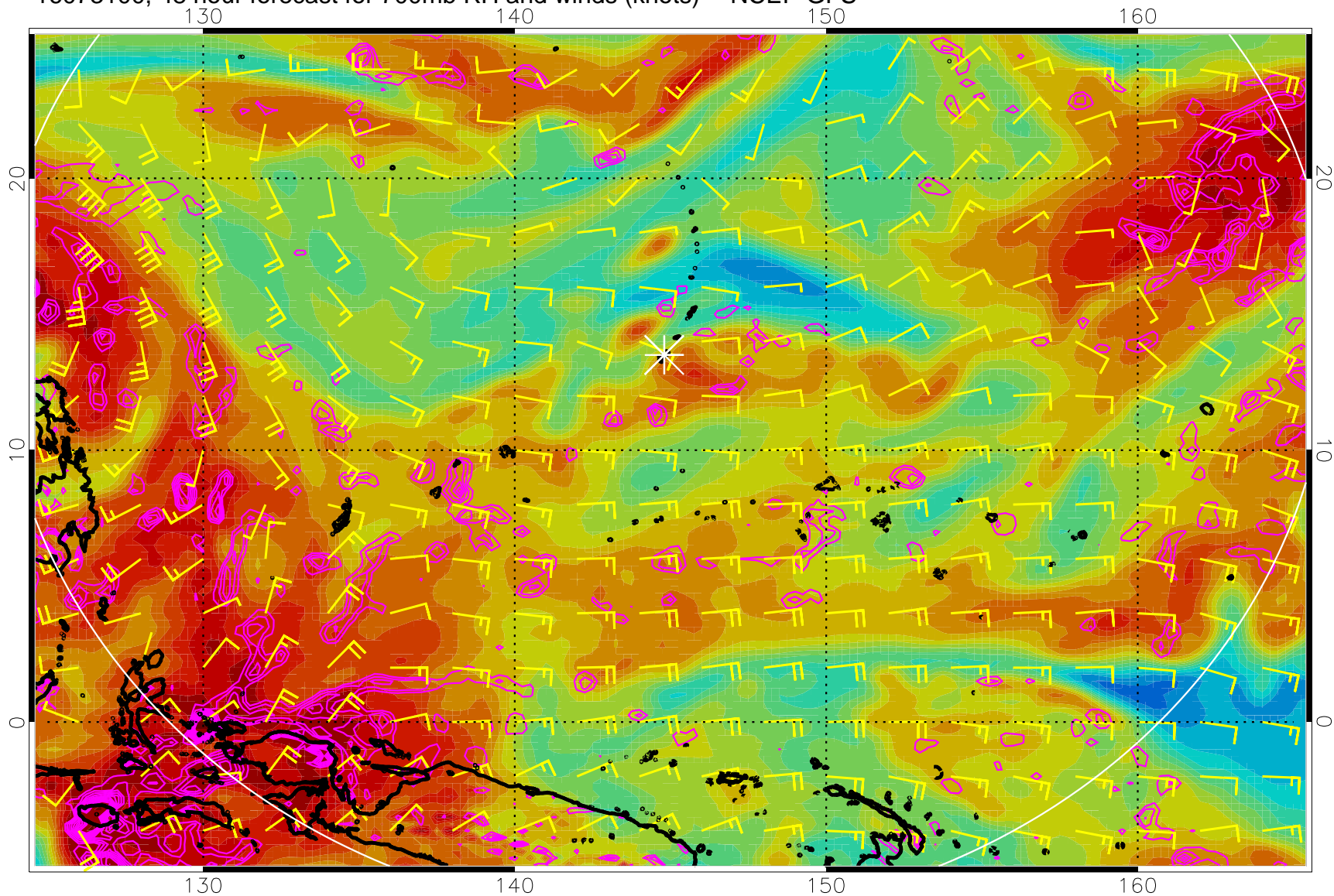
16073100, 48 hour forecast for 700mb RH and winds (knots) -- NCEP GFS
