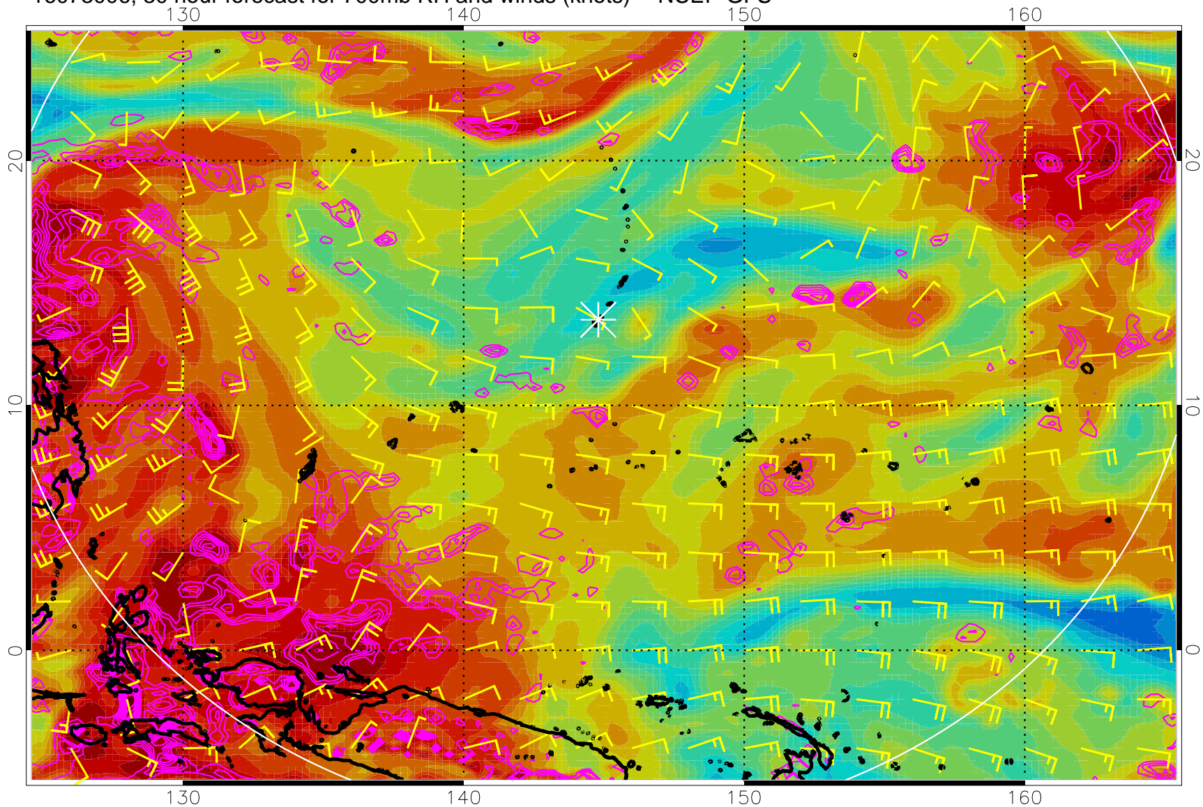
16073006, 30 hour forecast for 700mb RH and winds (knots) -- NCEP GFS
