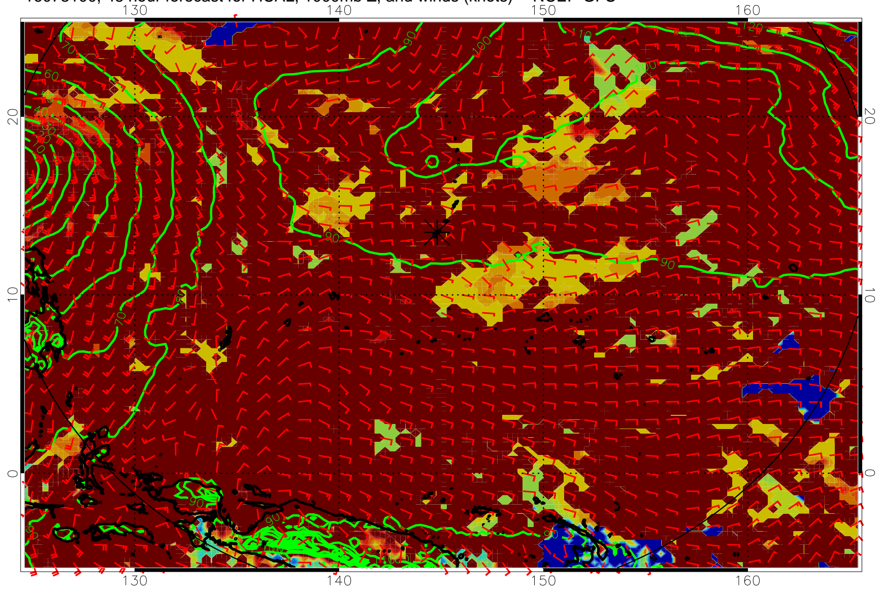
16073100, 48 hour forecast for HCAL, 1000mb Z, and winds (knots) -- NCEP GFS
