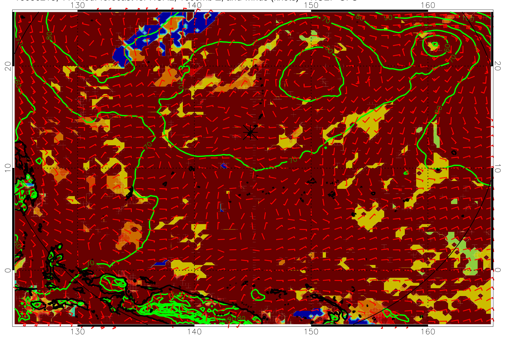
16080218, 114 hour forecast for HCAL, 1000mb Z, and winds (knots) -- NCEP GFS
