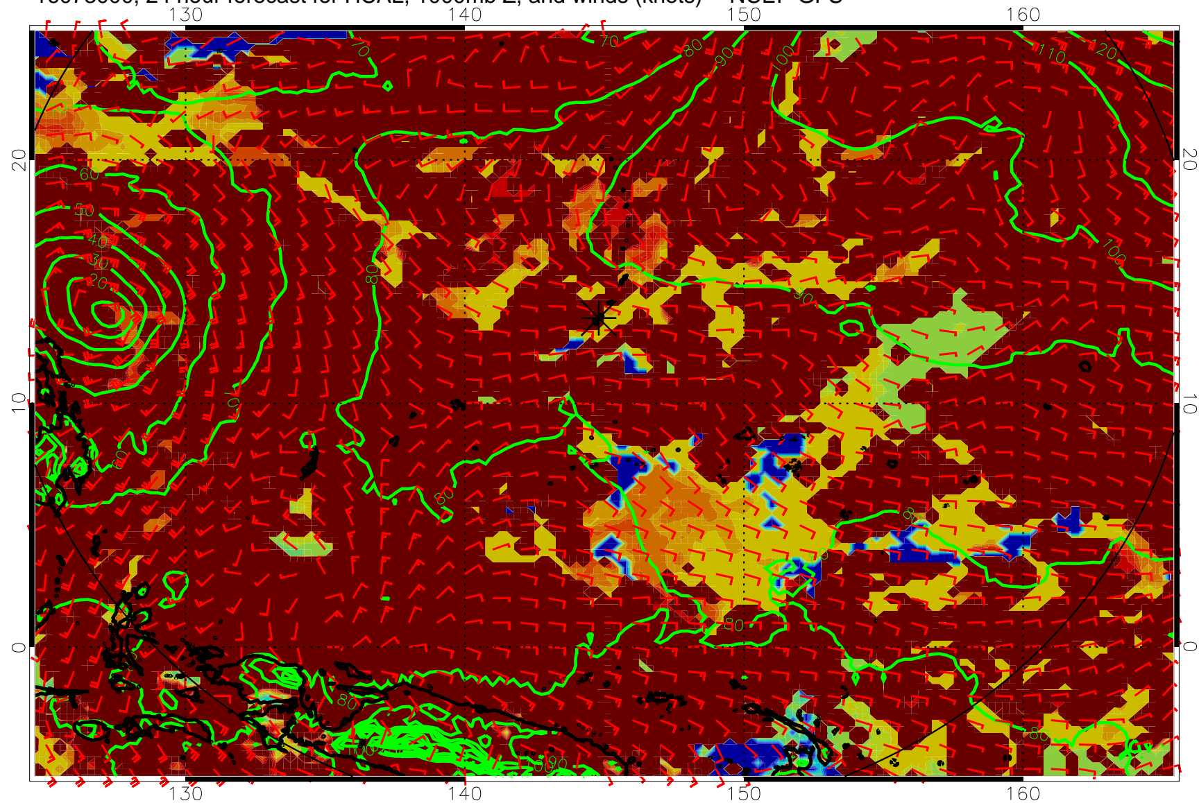
16073000, 24 hour forecast for HCAL, 1000mb Z, and winds (knots) -- NCEP GFS
