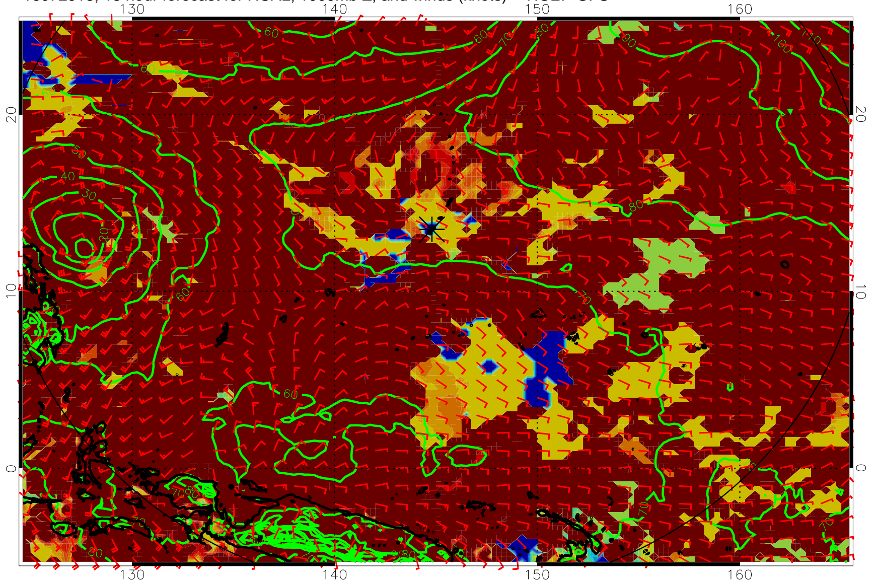
16072918, 18 hour forecast for HCAL, 1000mb Z, and winds (knots) -- NCEP GFS
