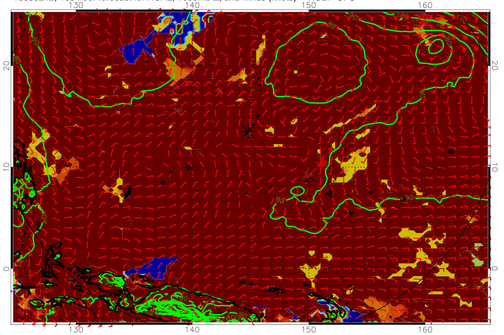
16080212, 108 hour forecast for HCAL, 1000mb Z, and winds (knots) -- NCEP GFS
