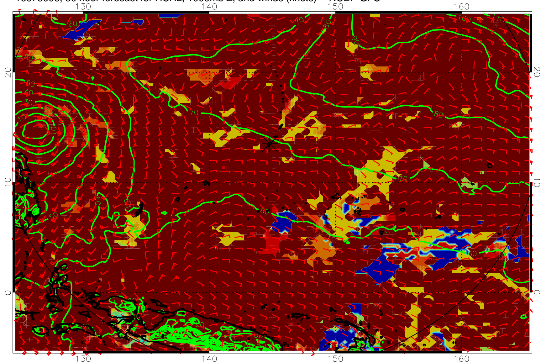
16073006, 30 hour forecast for HCAL, 1000mb Z, and winds (knots) -- NCEP GFS
