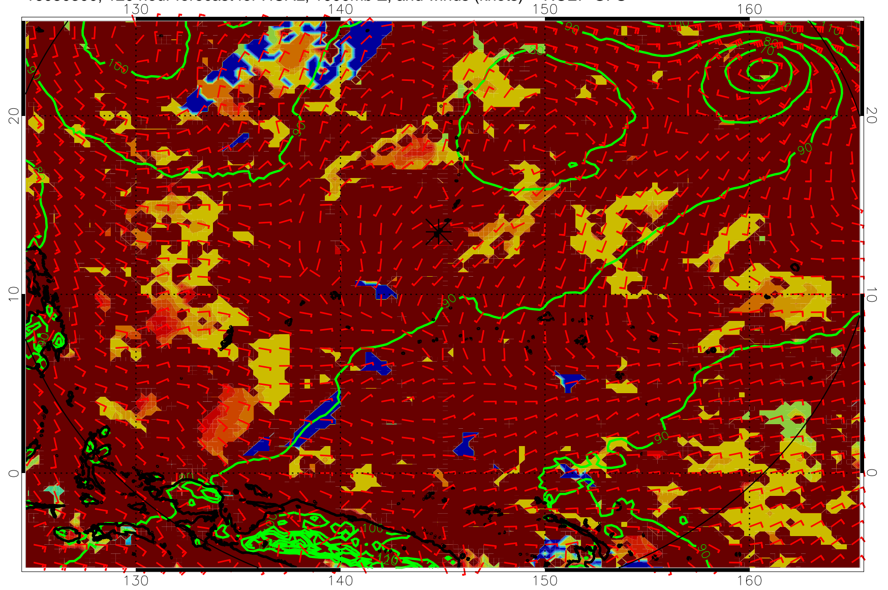
16080300, 120 hour forecast for HCAL, 1000mb Z, and winds (knots) -- NCEP GFS
