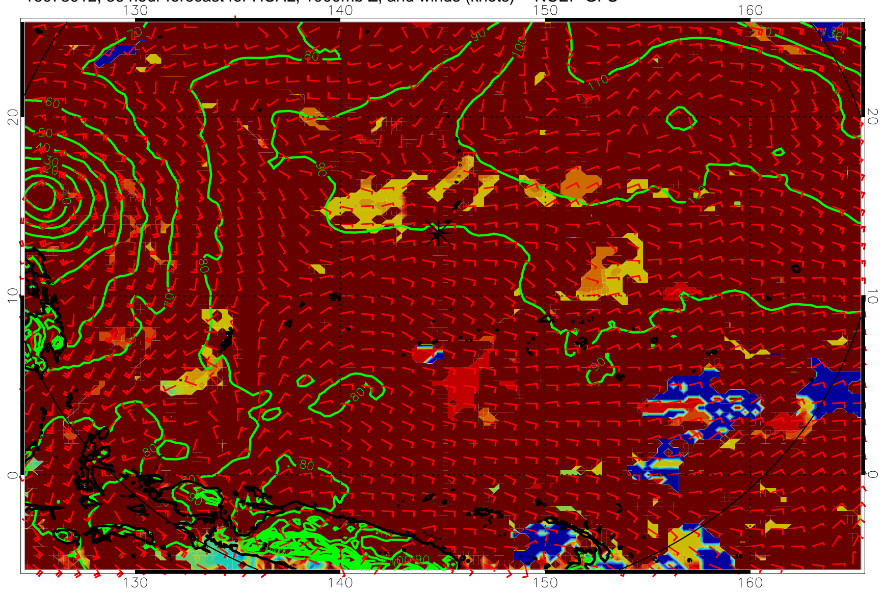
16073012, 36 hour forecast for HCAL, 1000mb Z, and winds (knots) -- NCEP GFS
