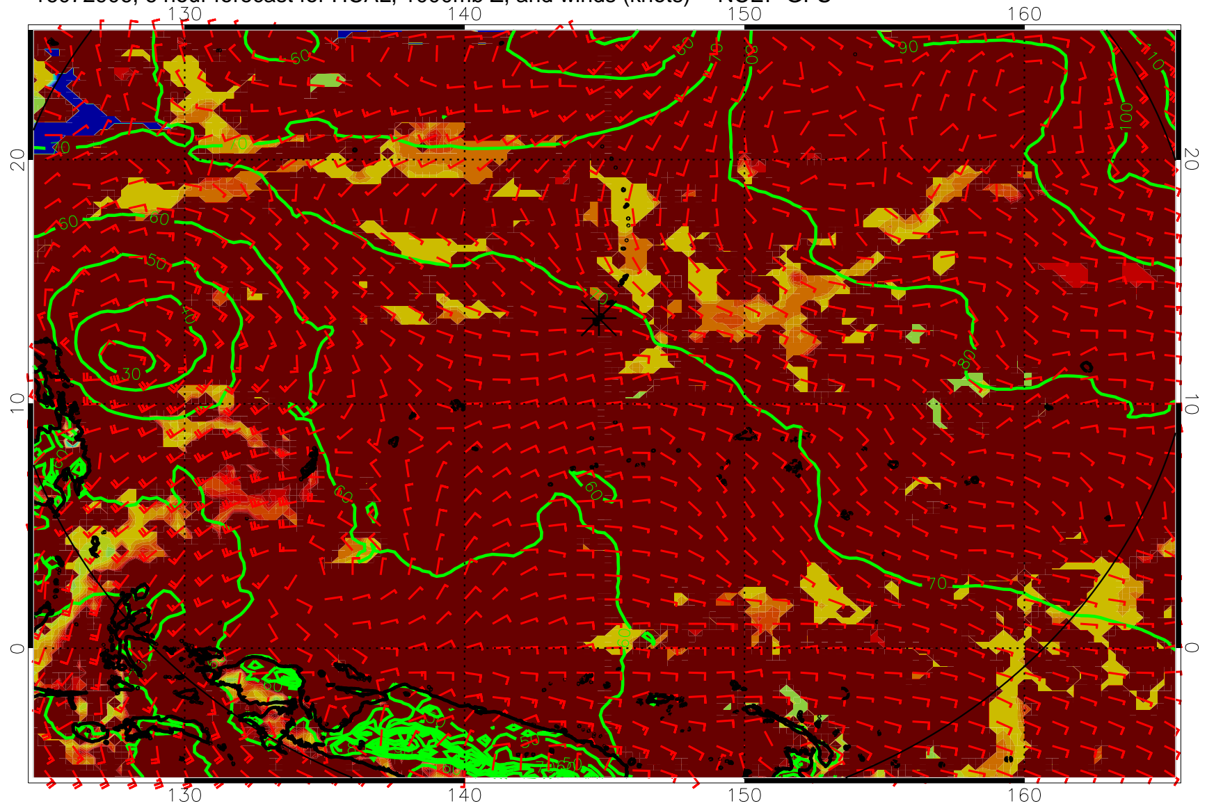
16072906, 6 hour forecast for HCAL, 1000mb Z, and winds (knots) -- NCEP GFS
