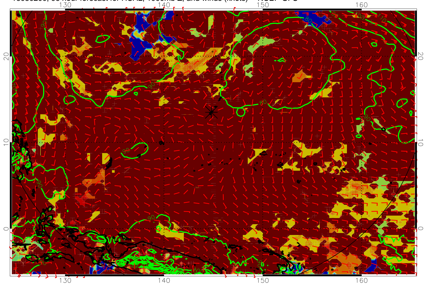
16080200, 96 hour forecast for HCAL, 1000mb Z, and winds (knots) -- NCEP GFS
