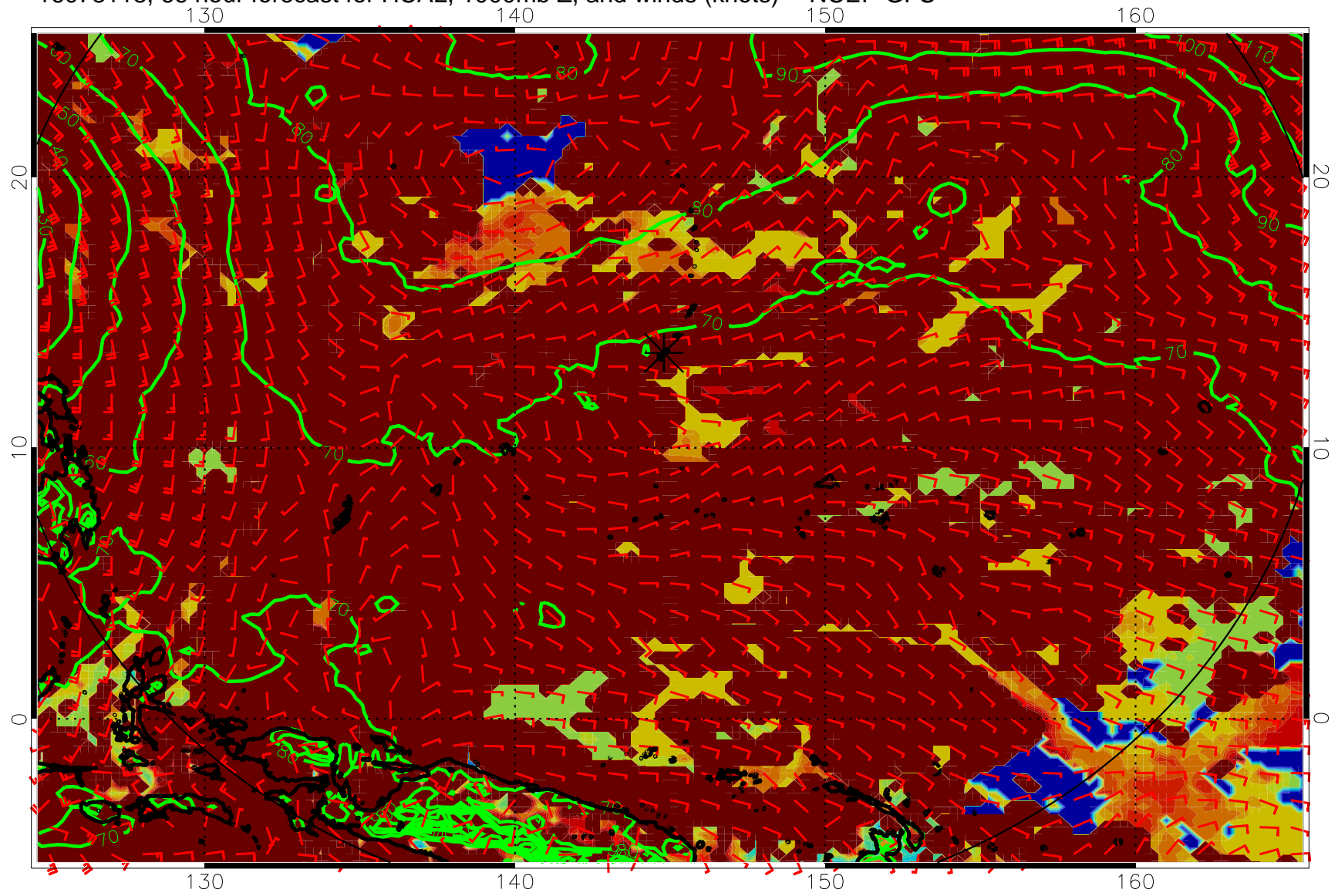
16073118, 66 hour forecast for HCAL, 1000mb Z, and winds (knots) -- NCEP GFS
