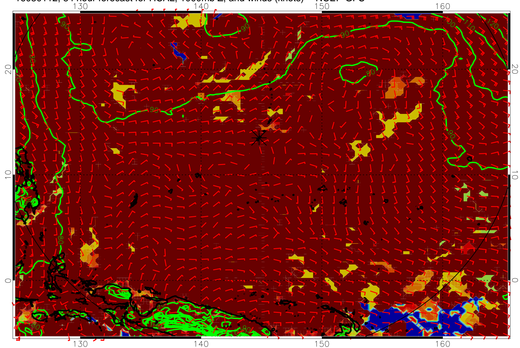
16080112, 84 hour forecast for HCAL, 1000mb Z, and winds (knots) -- NCEP GFS
