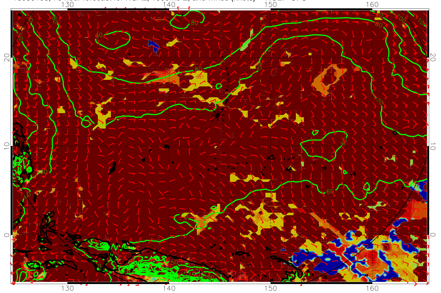
16080106, 78 hour forecast for HCAL, 1000mb Z, and winds (knots) -- NCEP GFS
