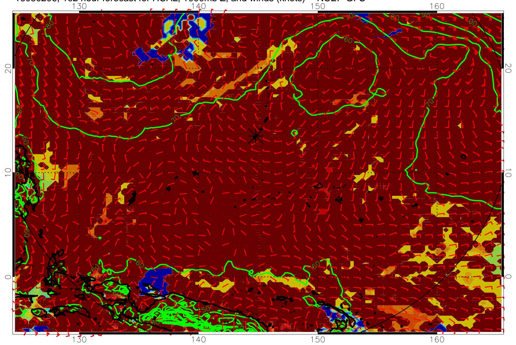
16080206, 102 hour forecast for HCAL, 1000mb Z, and winds (knots) -- NCEP GFS
