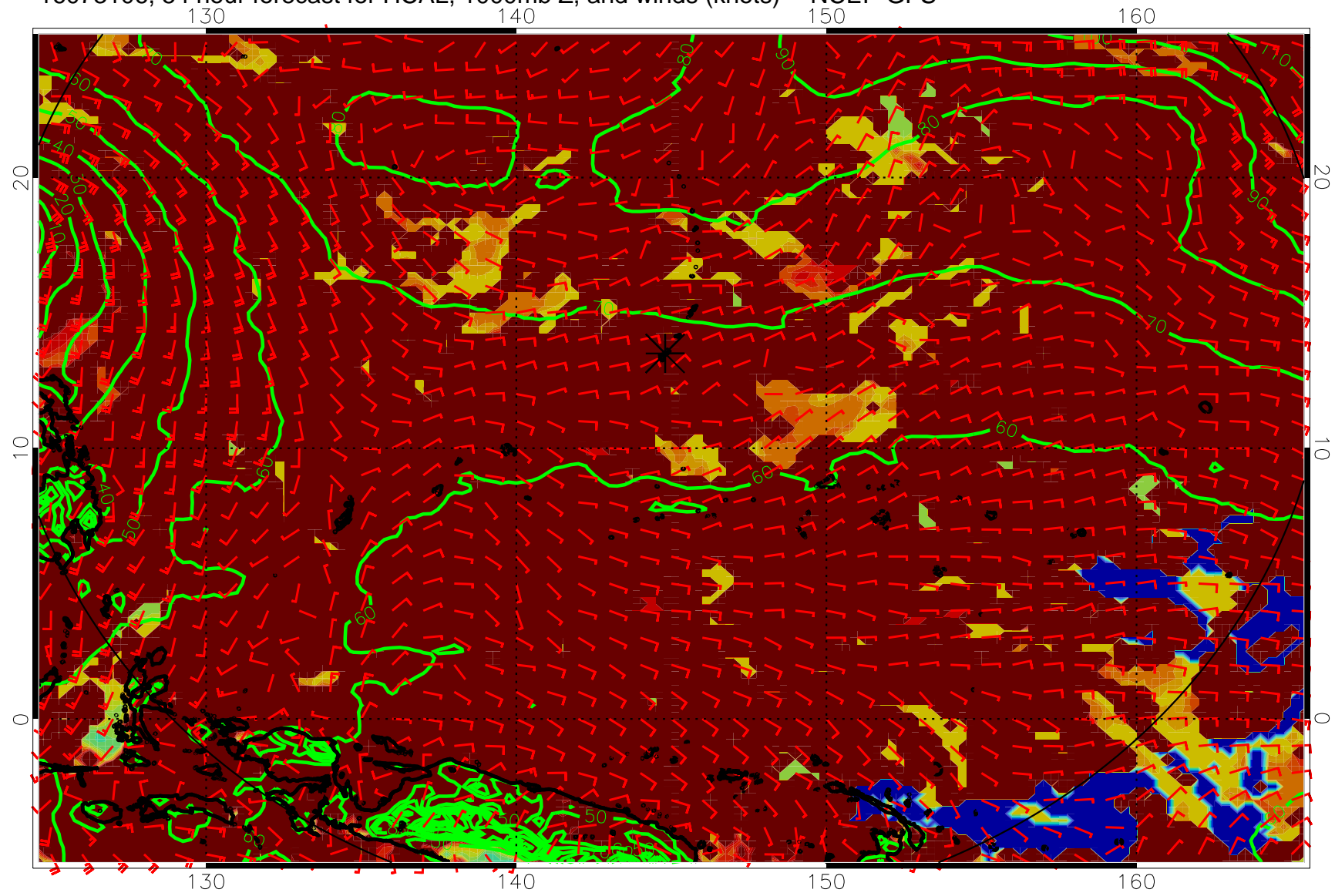
16073106, 54 hour forecast for HCAL, 1000mb Z, and winds (knots) -- NCEP GFS
