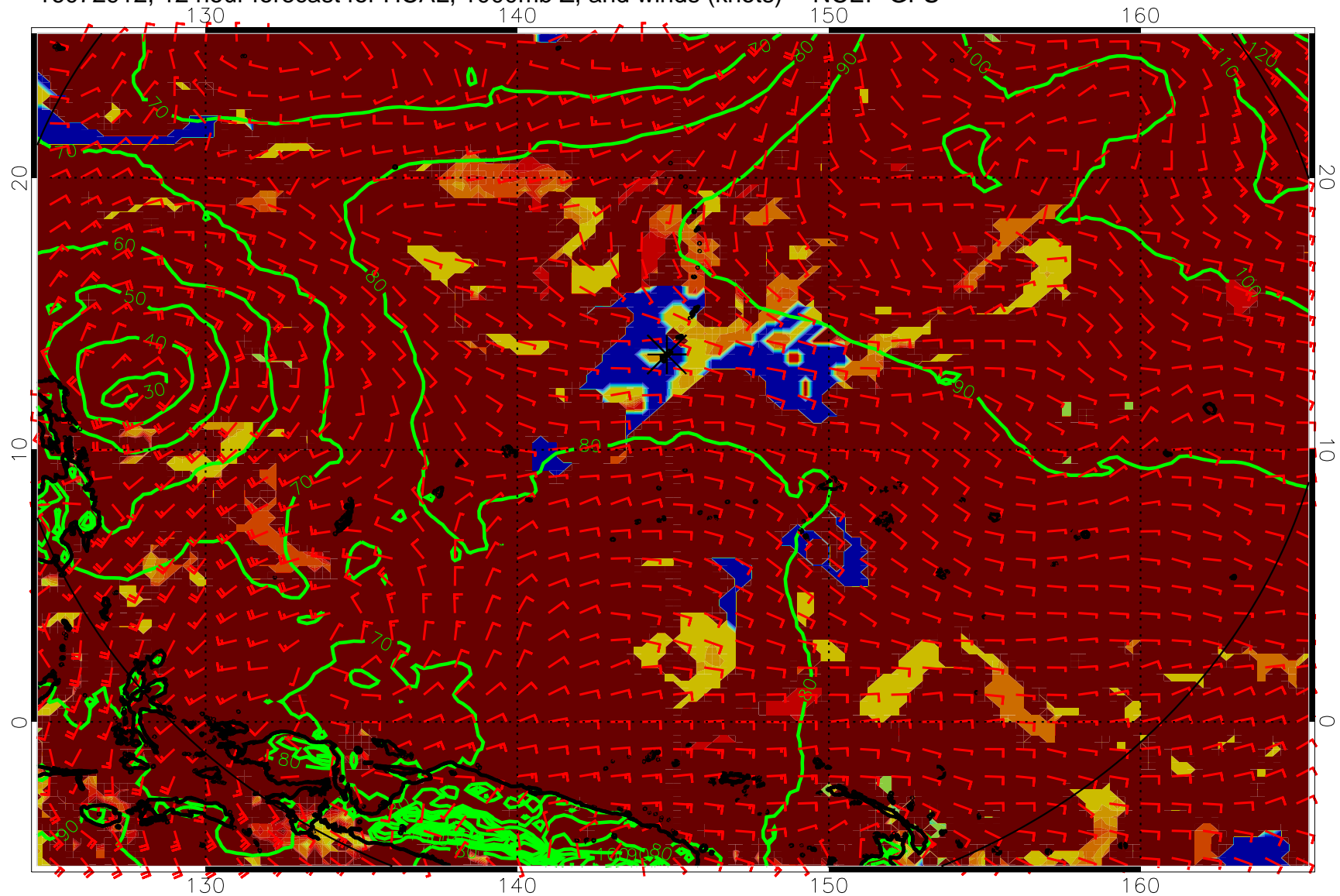
16072912, 12 hour forecast for HCAL, 1000mb Z, and winds (knots) -- NCEP GFS
