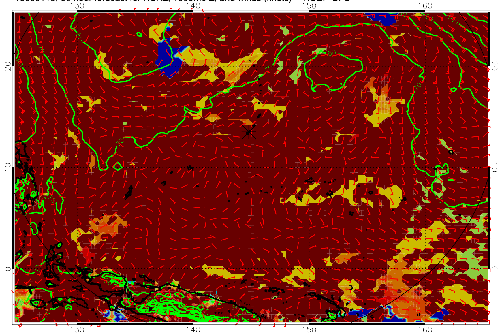
16080118, 90 hour forecast for HCAL, 1000mb Z, and winds (knots) -- NCEP GFS
