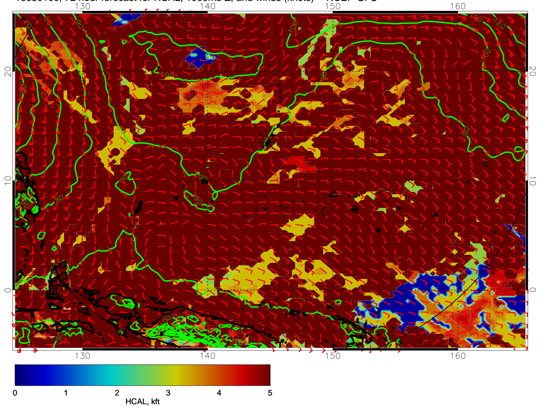
16080100, 72 hour forecast for HCAL, 1000mb Z, and winds (knots) -- NCEP GFS
