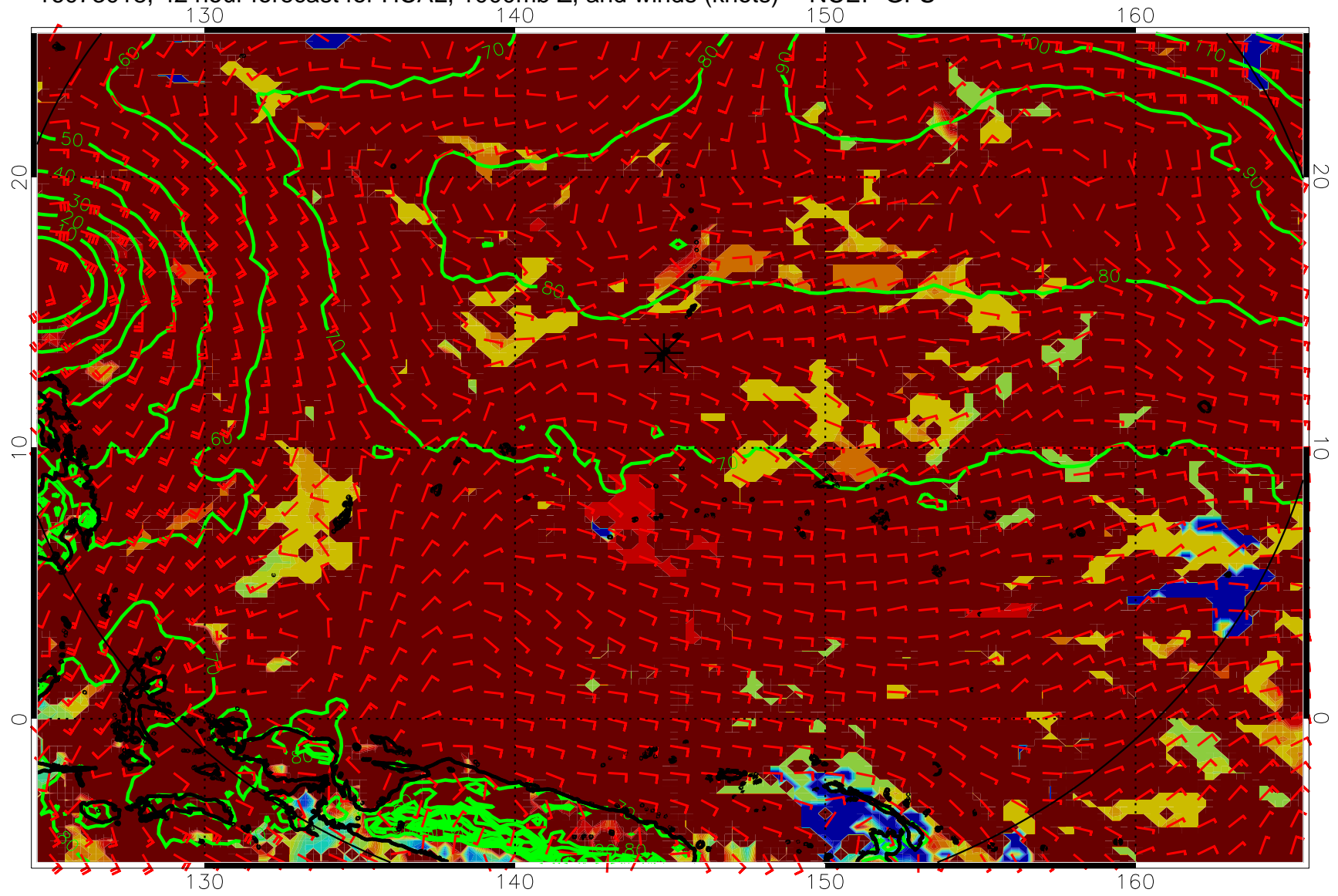
16073018, 42 hour forecast for HCAL, 1000mb Z, and winds (knots) -- NCEP GFS
