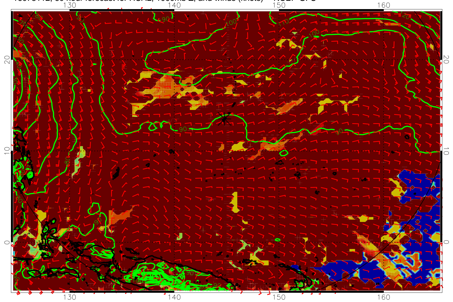
16073112, 60 hour forecast for HCAL, 1000mb Z, and winds (knots) -- NCEP GFS
