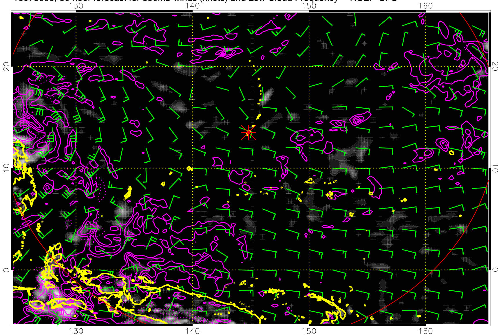
16073006, 30 hour forecast for 850mb winds (knots) and Low Cloud Frequency -- NCEP GFS
