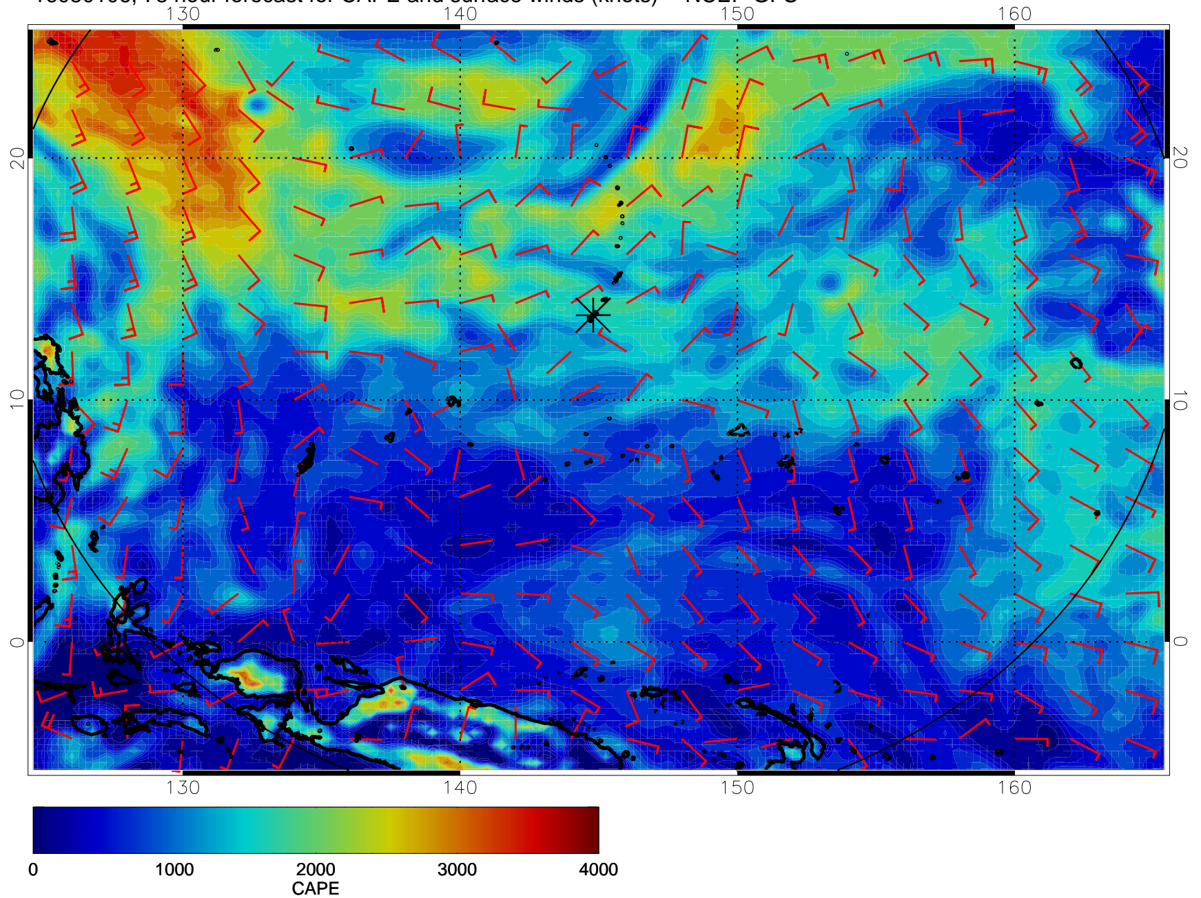
16080106, 78 hour forecast for CAPE and surface winds (knots) -- NCEP GFS
