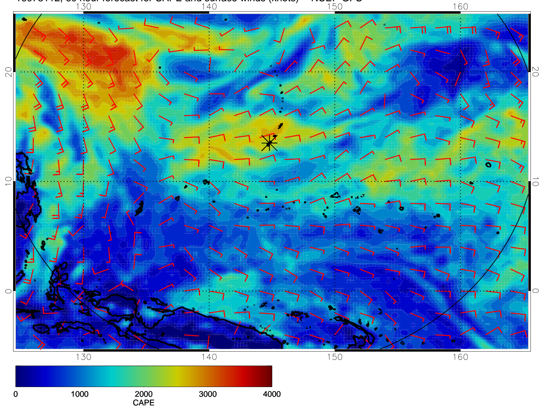
16073112, 60 hour forecast for CAPE and surface winds (knots) -- NCEP GFS
