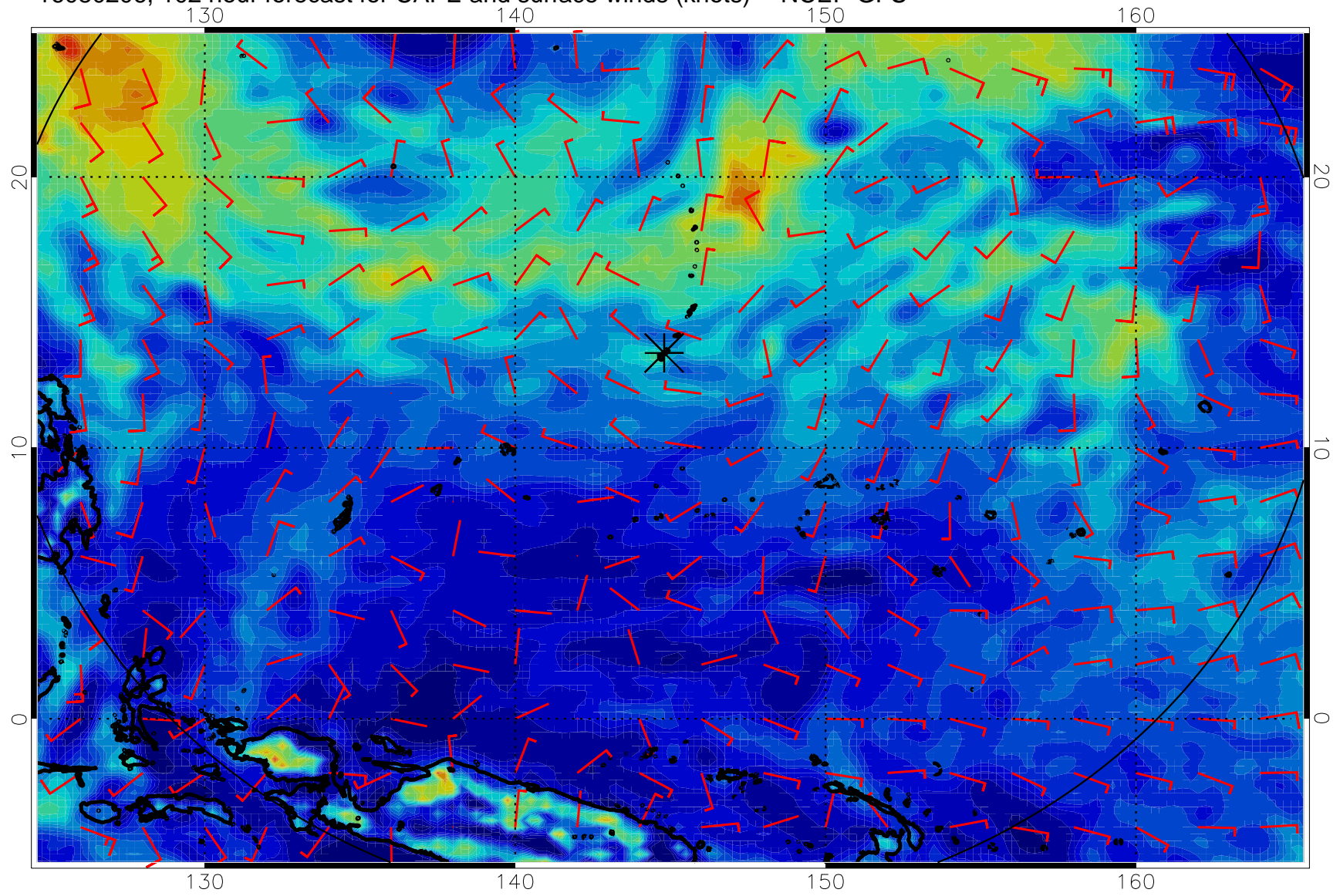
16080206, 102 hour forecast for CAPE and surface winds (knots) -- NCEP GFS
