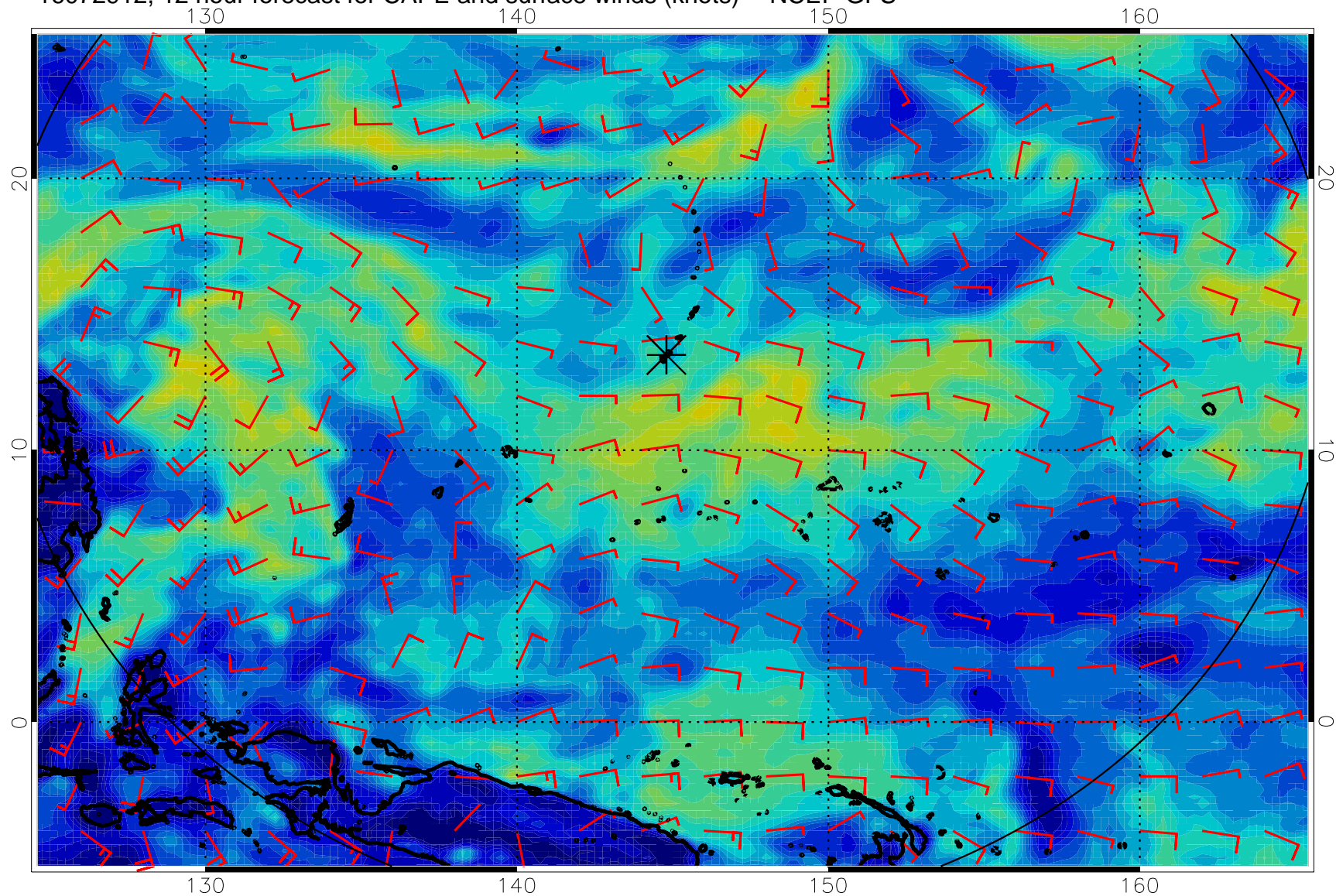
16072912, 12 hour forecast for CAPE and surface winds (knots) -- NCEP GFS
