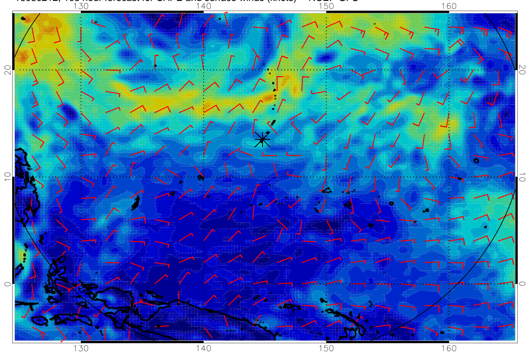
16080212, 108 hour forecast for CAPE and surface winds (knots) -- NCEP GFS
