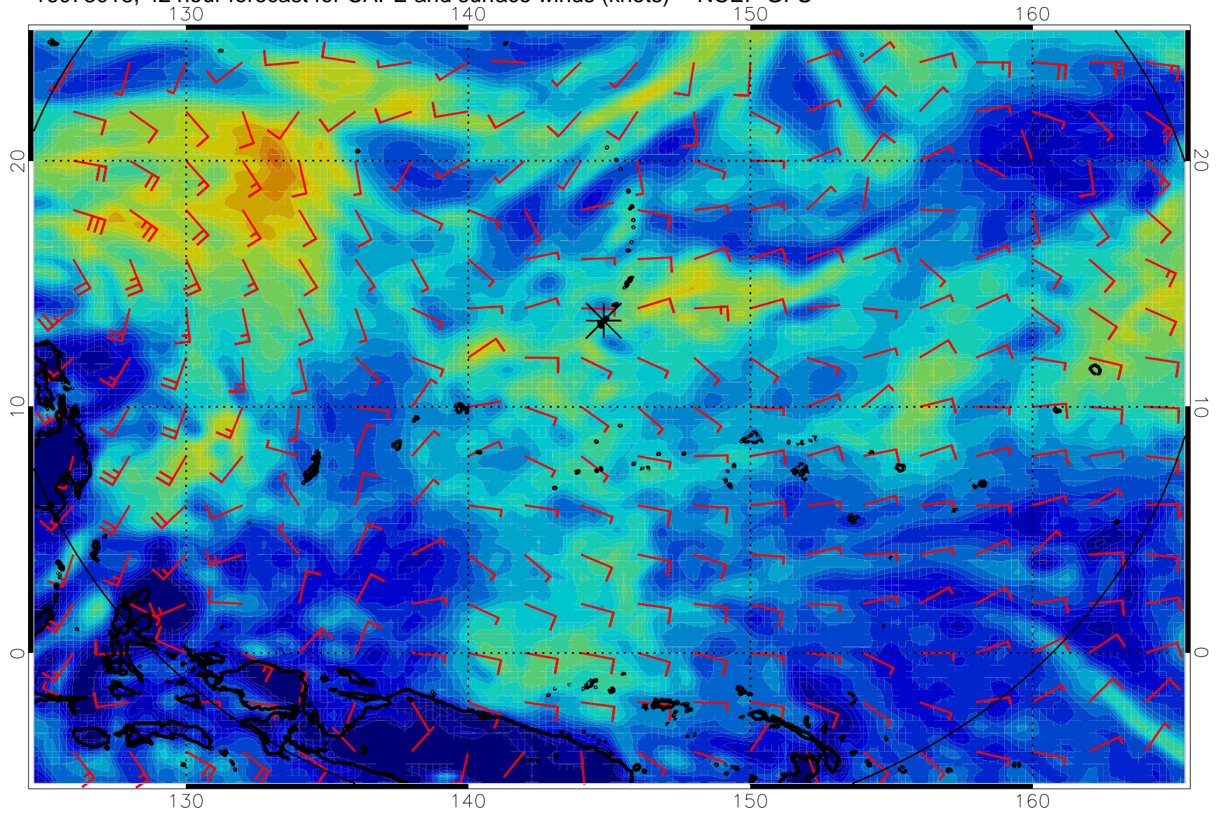
16073018, 42 hour forecast for CAPE and surface winds (knots) -- NCEP GFS
