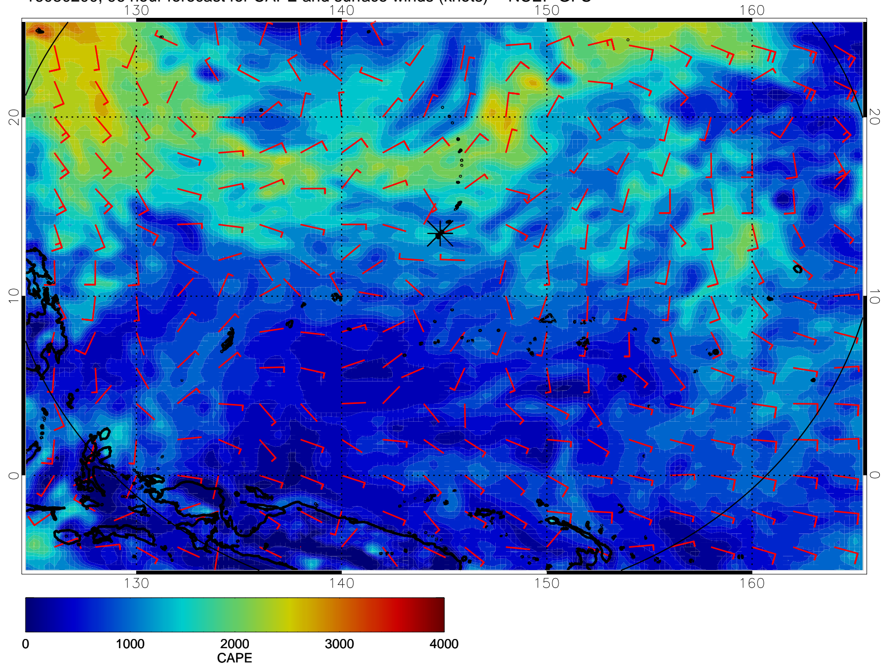
16080200, 96 hour forecast for CAPE and surface winds (knots) -- NCEP GFS
