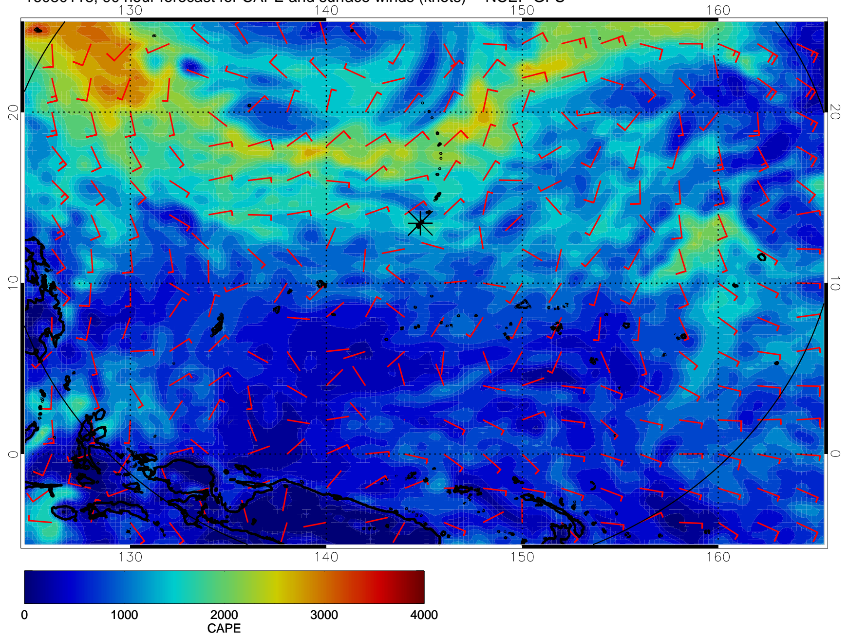
16080118, 90 hour forecast for CAPE and surface winds (knots) -- NCEP GFS
