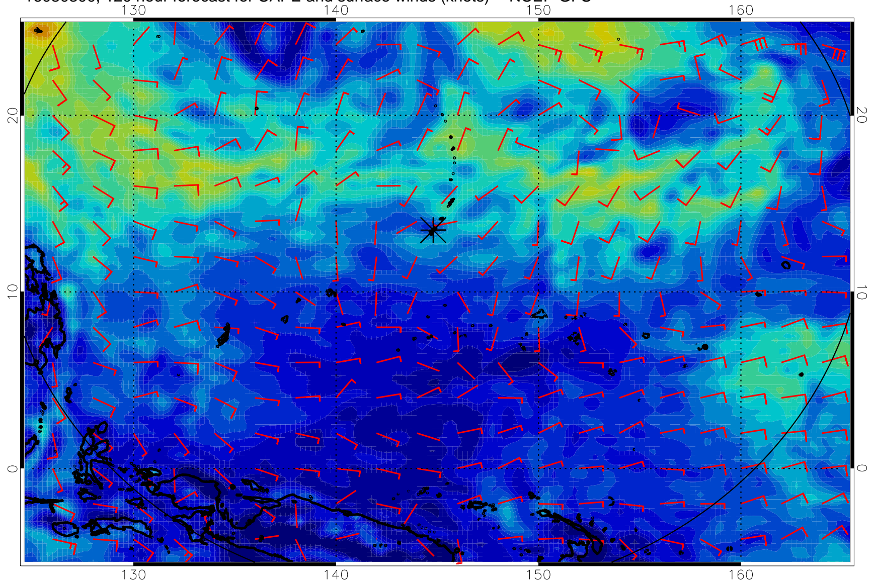
16080300, 120 hour forecast for CAPE and surface winds (knots) -- NCEP GFS
