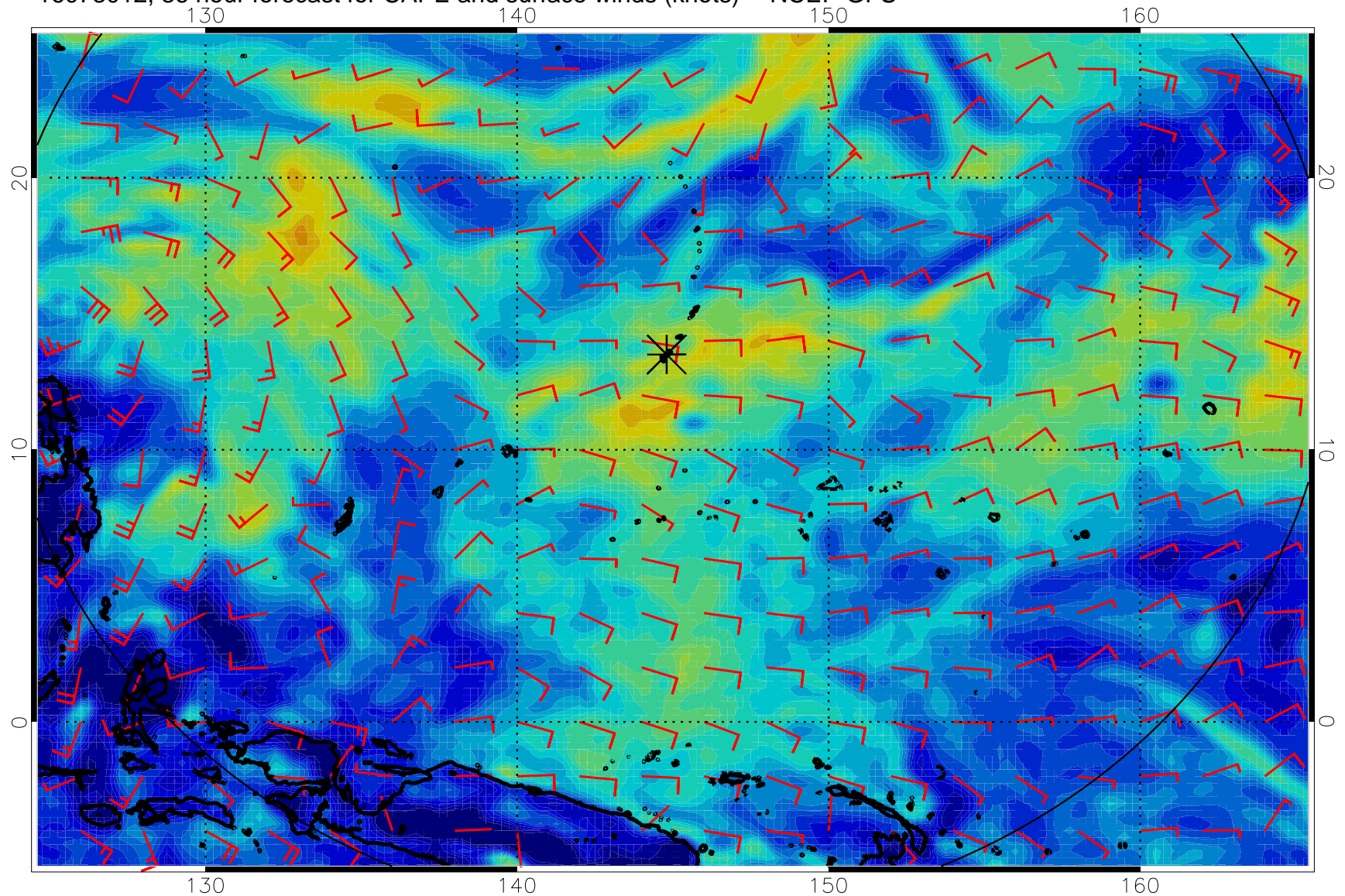
16073012, 36 hour forecast for CAPE and surface winds (knots) -- NCEP GFS
