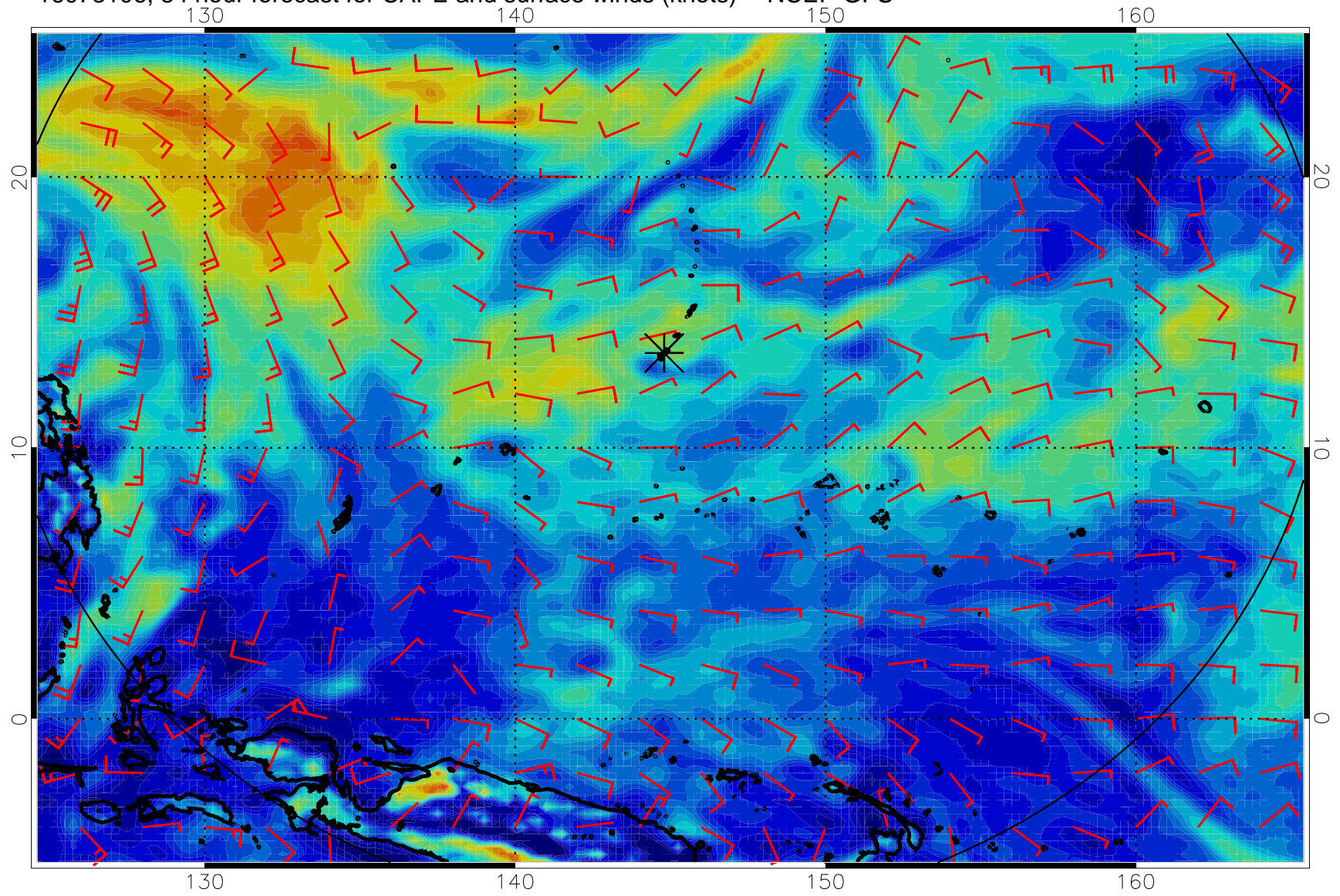
16073106, 54 hour forecast for CAPE and surface winds (knots) -- NCEP GFS
