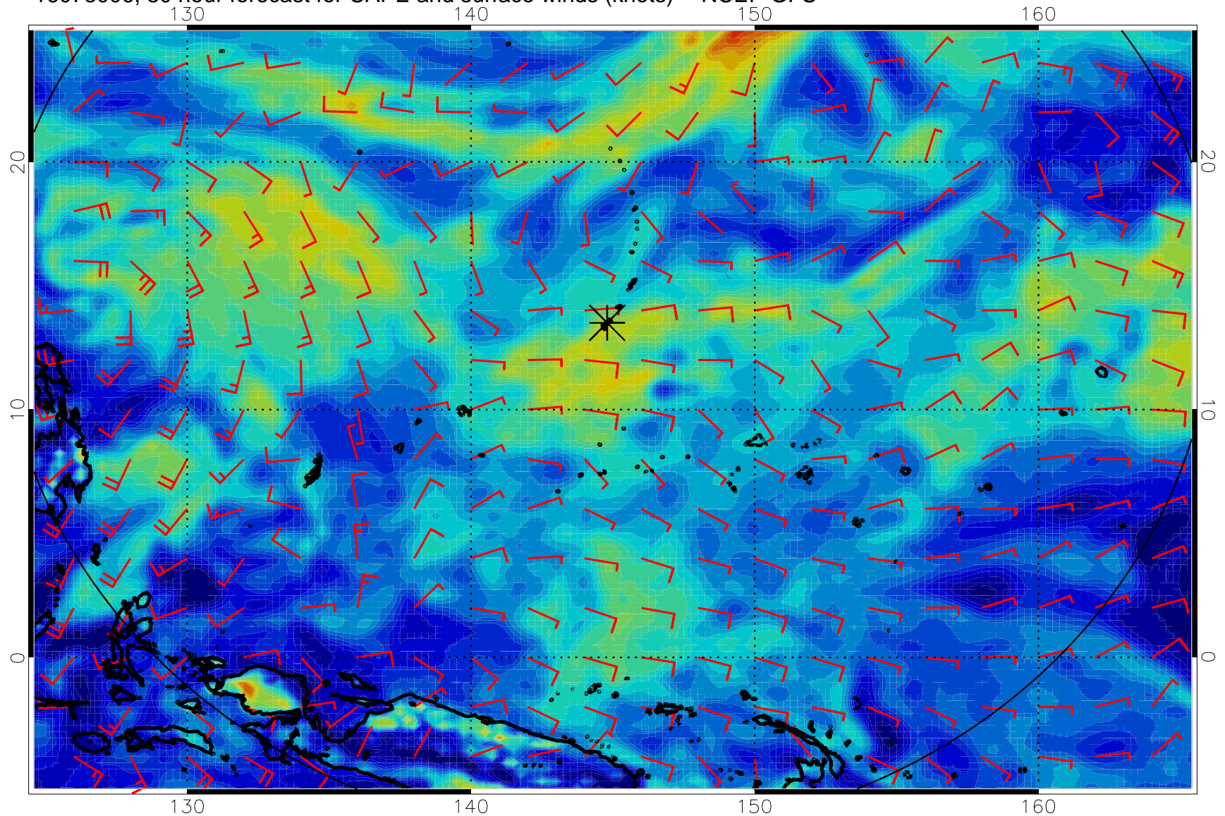
16073006, 30 hour forecast for CAPE and surface winds (knots) -- NCEP GFS
