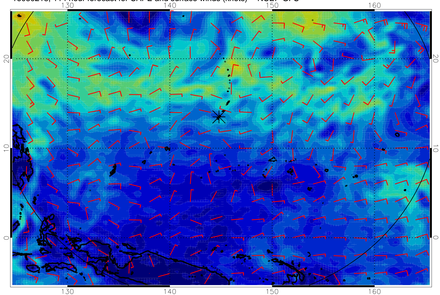
16080218, 114 hour forecast for CAPE and surface winds (knots) -- NCEP GFS
