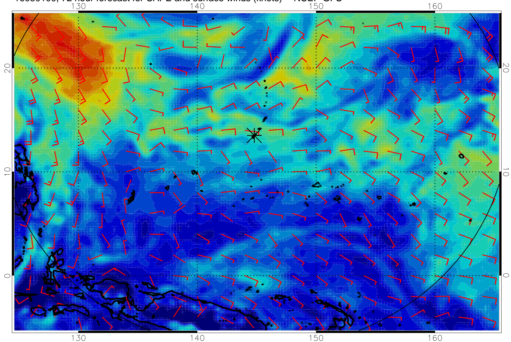
16080100, 72 hour forecast for CAPE and surface winds (knots) -- NCEP GFS
