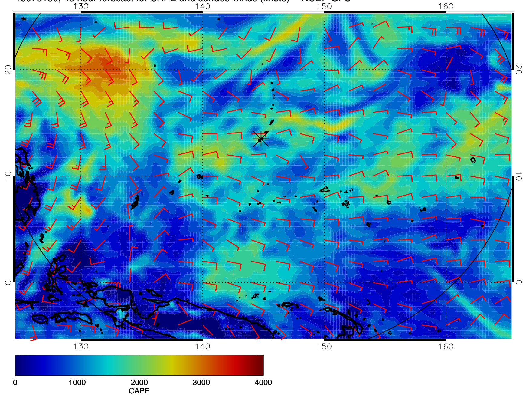
16073100, 48 hour forecast for CAPE and surface winds (knots) -- NCEP GFS
