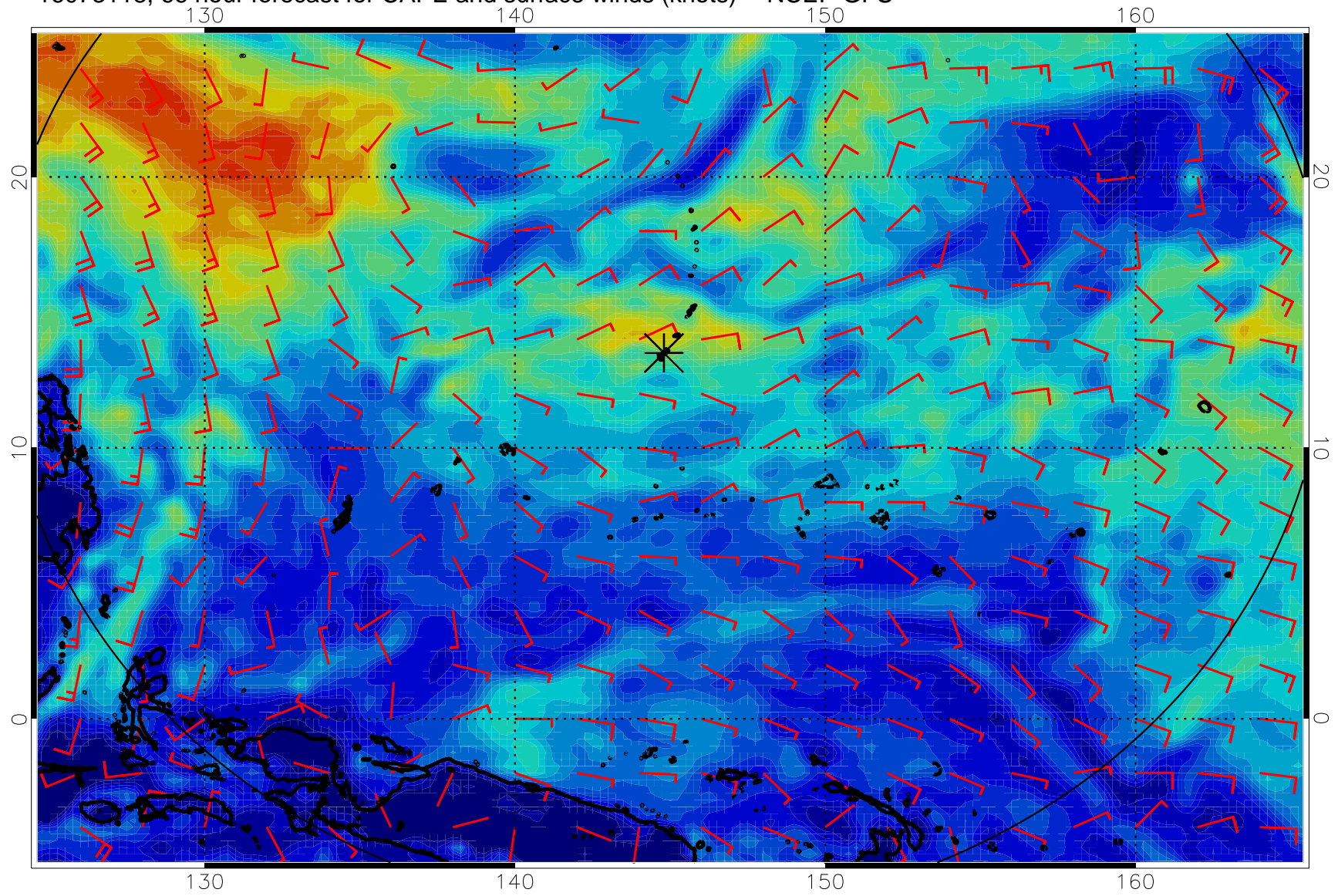
16073118, 66 hour forecast for CAPE and surface winds (knots) -- NCEP GFS
