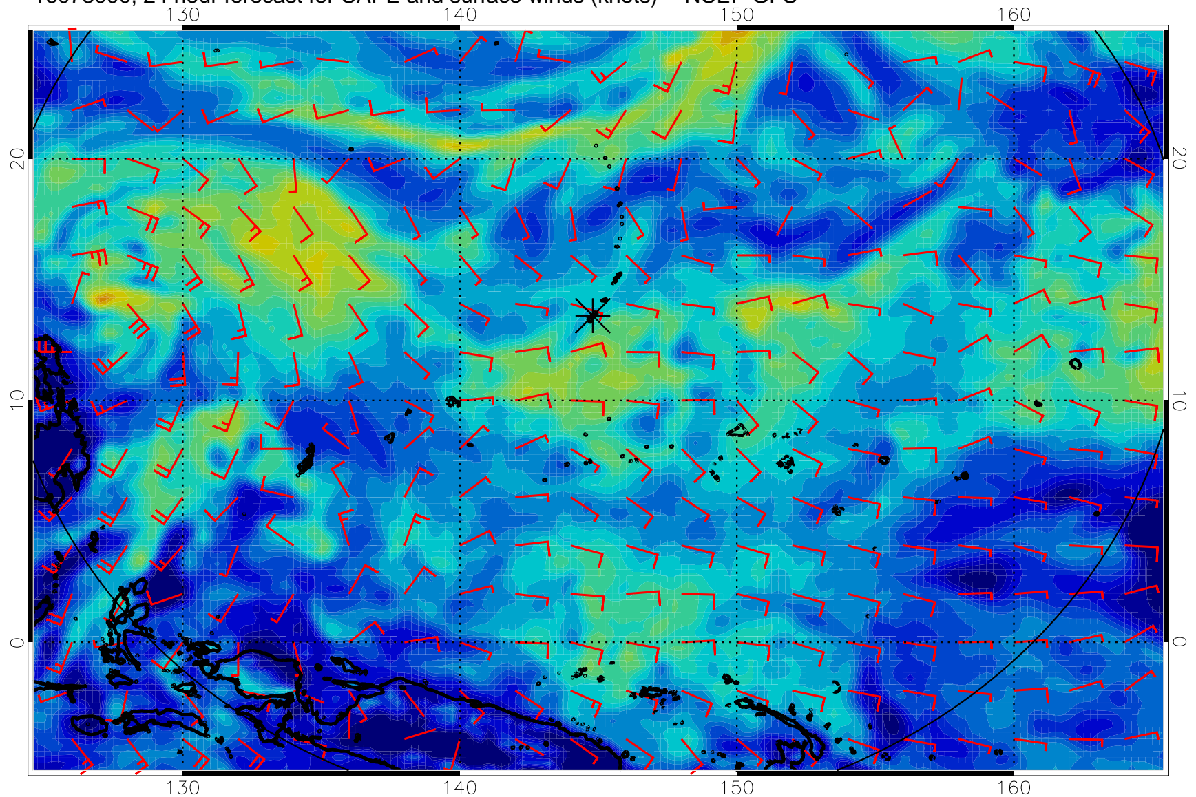
16073000, 24 hour forecast for CAPE and surface winds (knots) -- NCEP GFS
