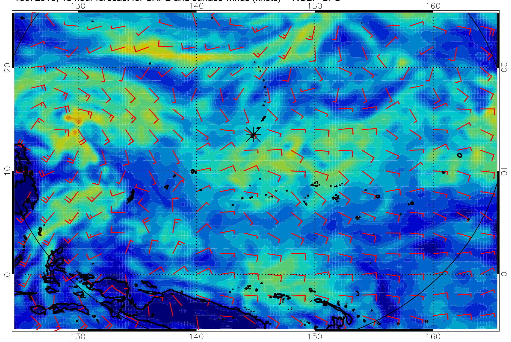
16072918, 18 hour forecast for CAPE and surface winds (knots) -- NCEP GFS
