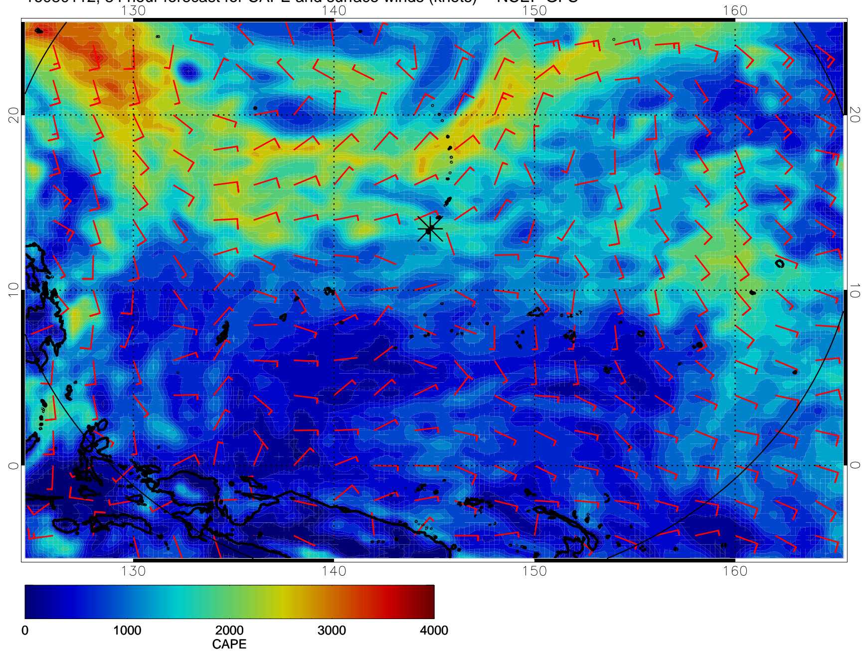
16080112, 84 hour forecast for CAPE and surface winds (knots) -- NCEP GFS
