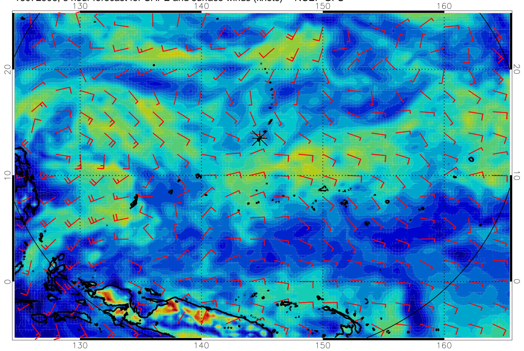
16072906, 6 hour forecast for CAPE and surface winds (knots) -- NCEP GFS
