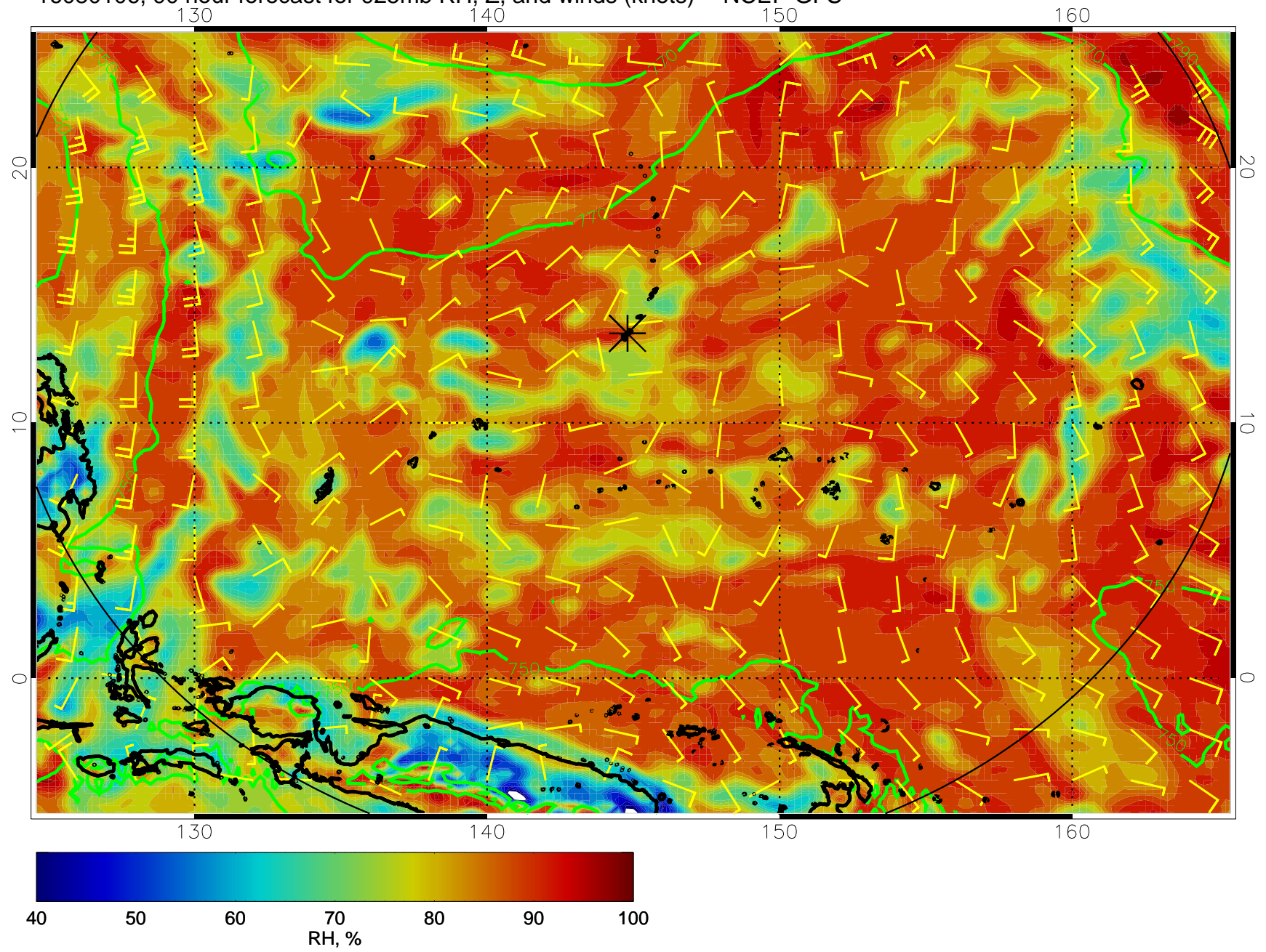
16080106, 90 hour forecast for 925mb RH, Z, and winds (knots) -- NCEP GFS
