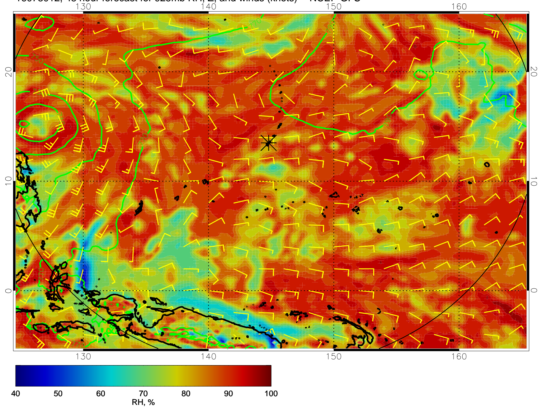
16073012, 48 hour forecast for 925mb RH, Z, and winds (knots) -- NCEP GFS
