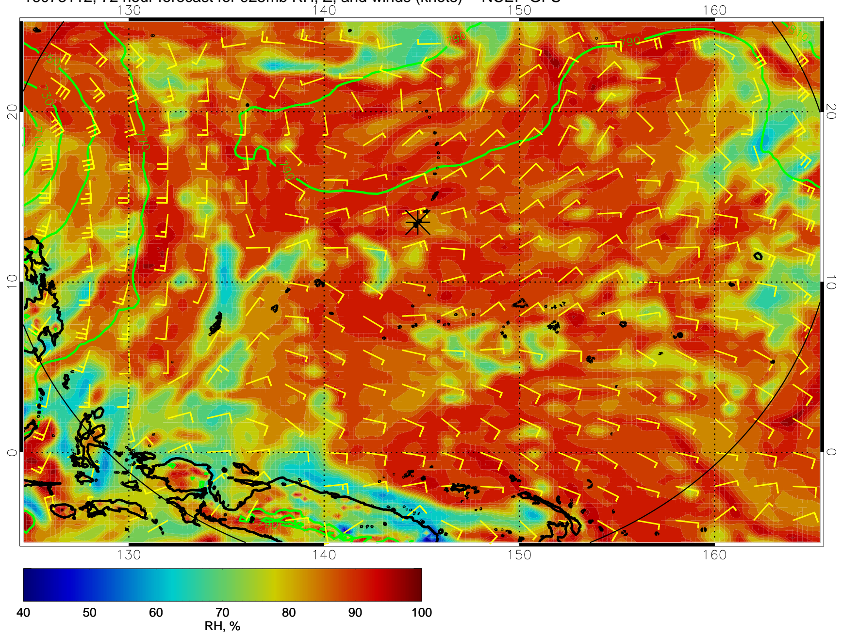
16073112, 72 hour forecast for 925mb RH, Z, and winds (knots) -- NCEP GFS
