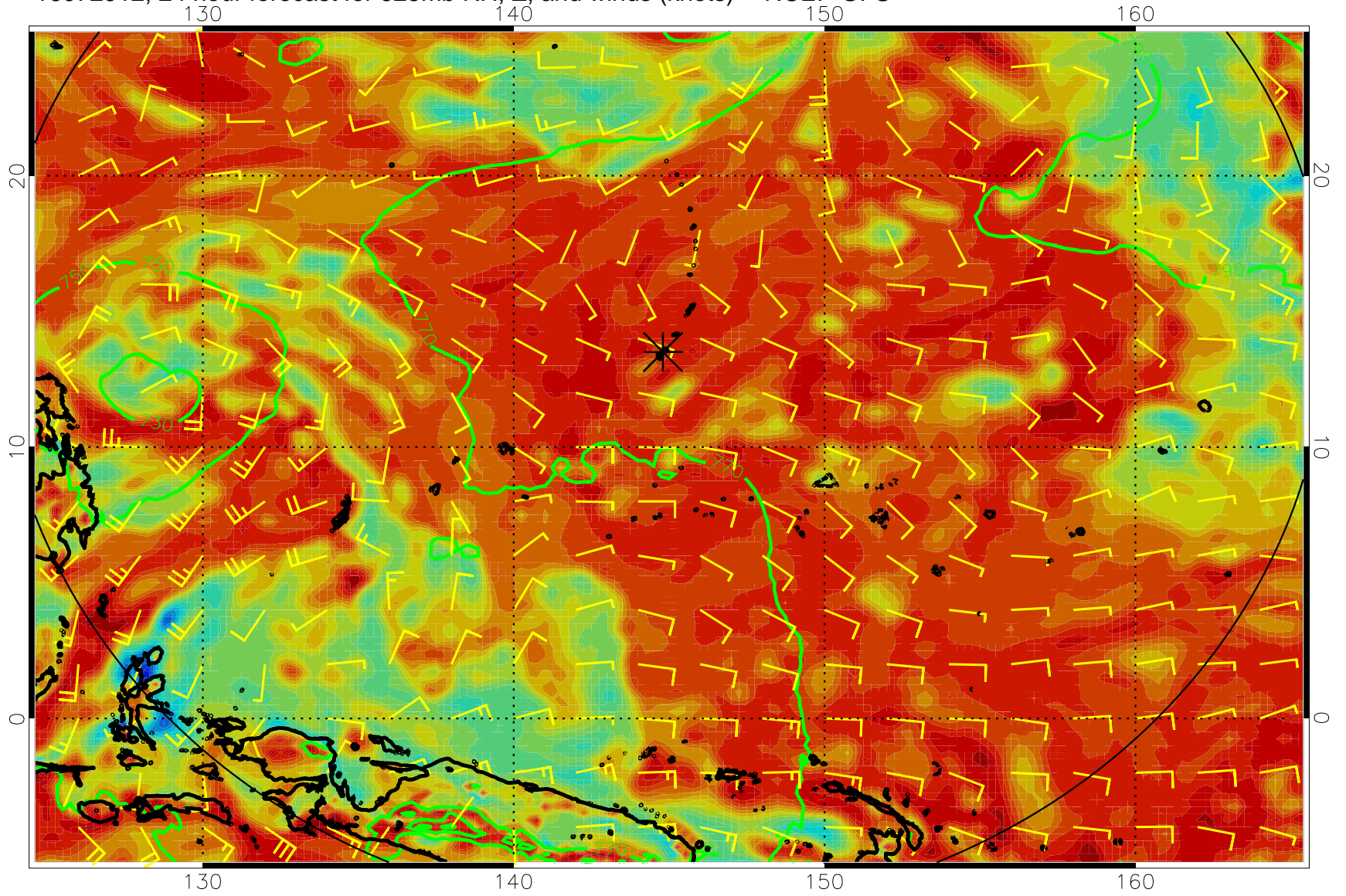
16072912, 24 hour forecast for 925mb RH, Z, and winds (knots) -- NCEP GFS
