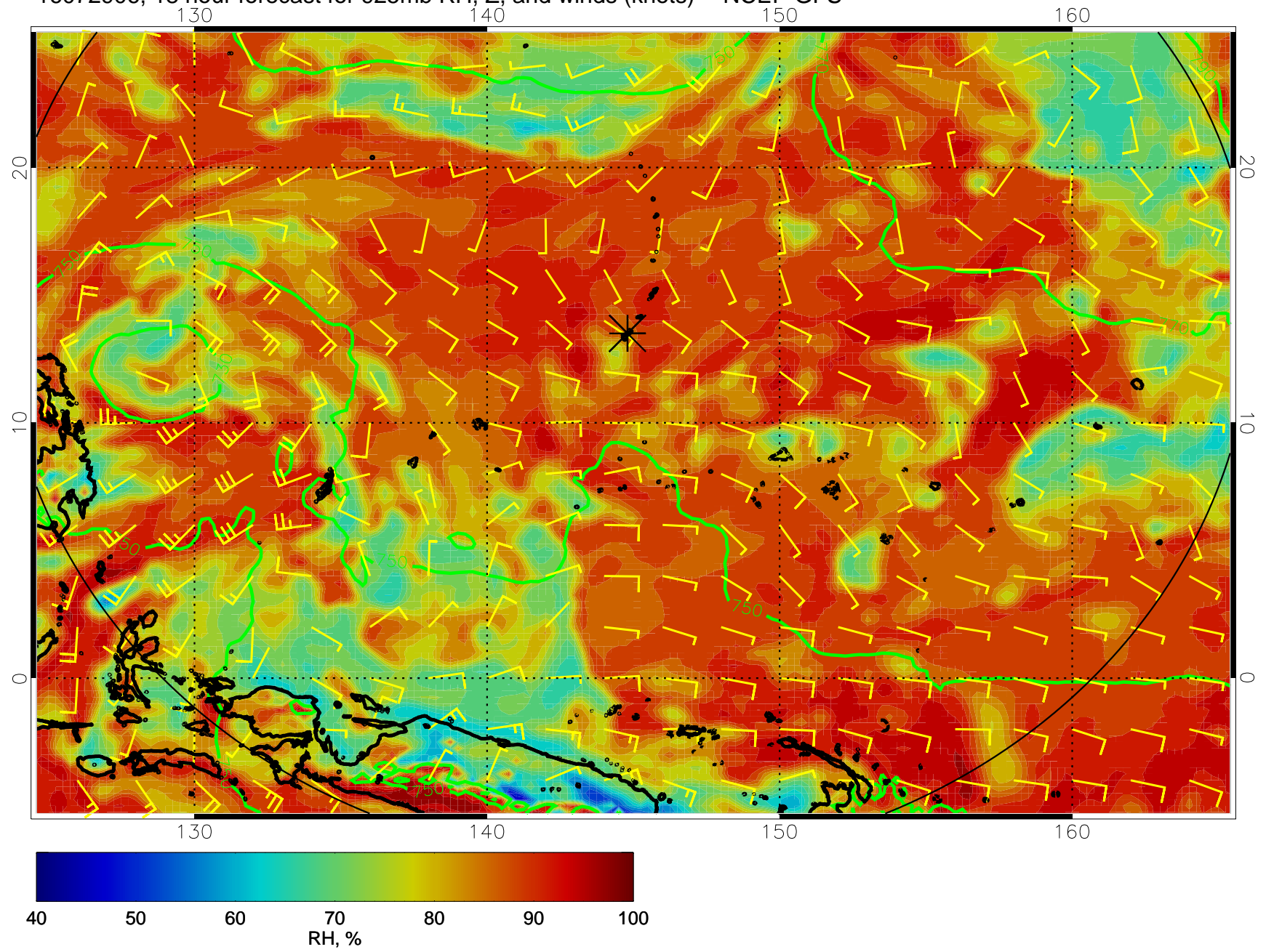
16072906, 18 hour forecast for 925mb RH, Z, and winds (knots) -- NCEP GFS
