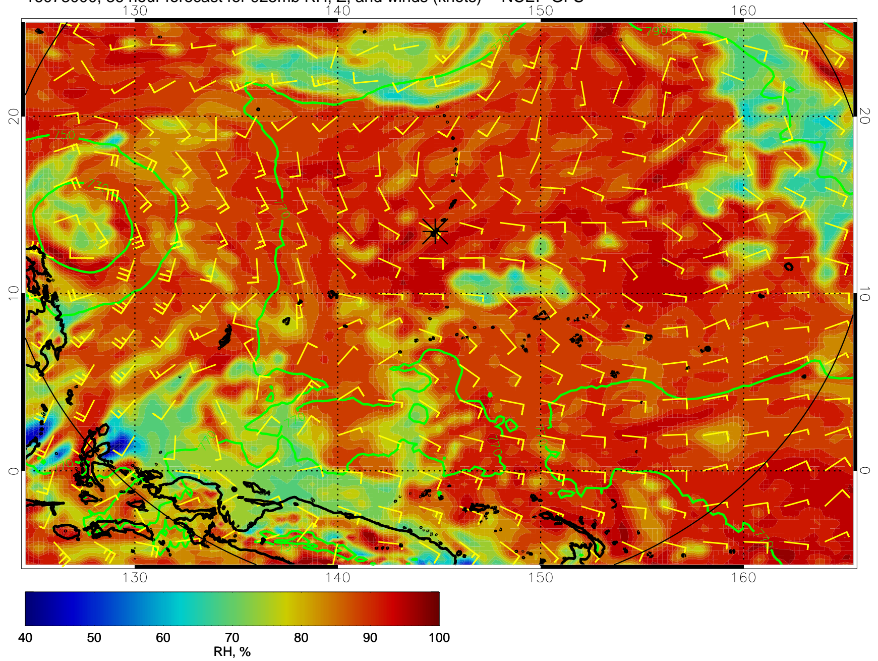
16073000, 36 hour forecast for 925mb RH, Z, and winds (knots) -- NCEP GFS
