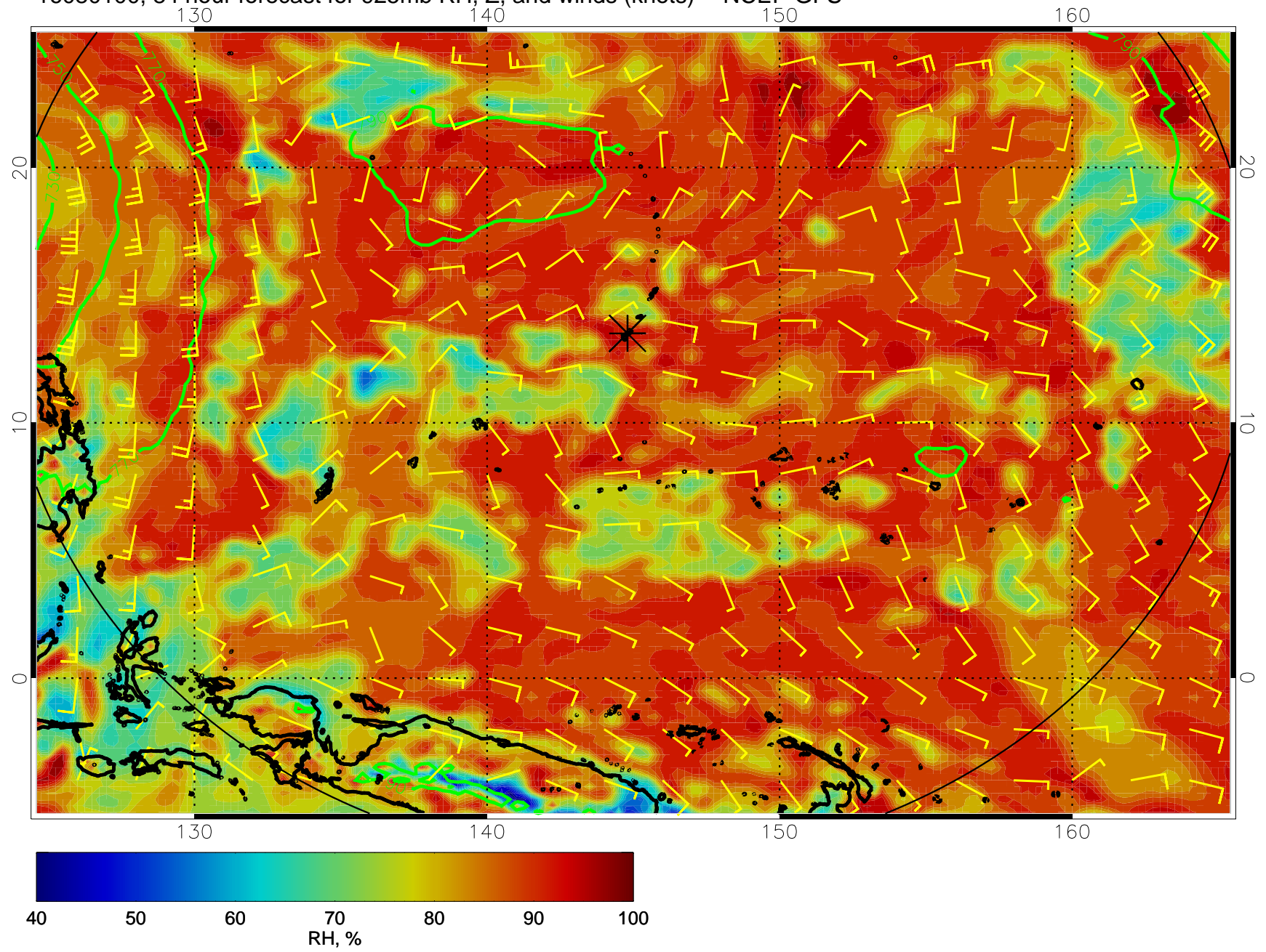
16080100, 84 hour forecast for 925mb RH, Z, and winds (knots) -- NCEP GFS
