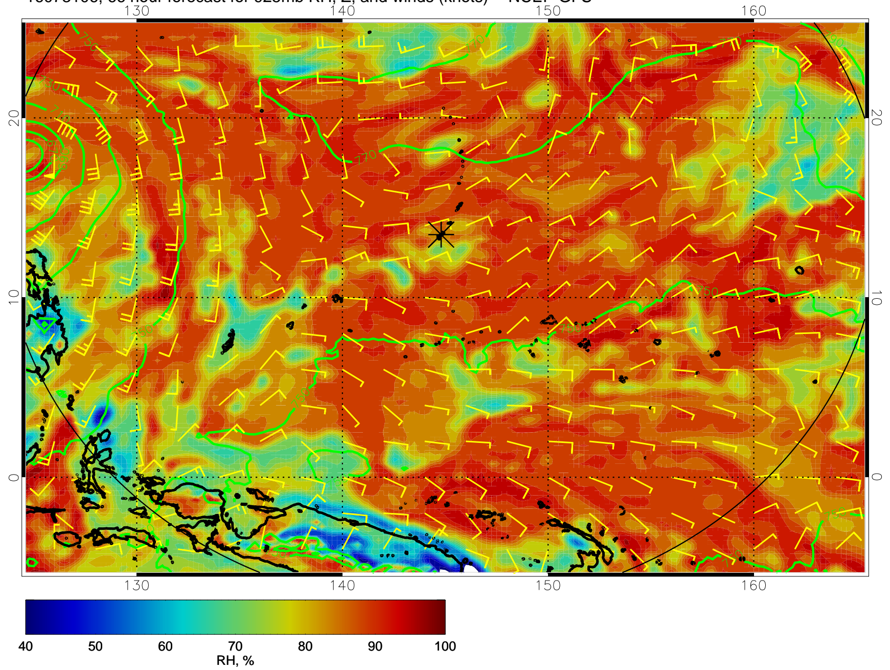
16073106, 66 hour forecast for 925mb RH, Z, and winds (knots) -- NCEP GFS
