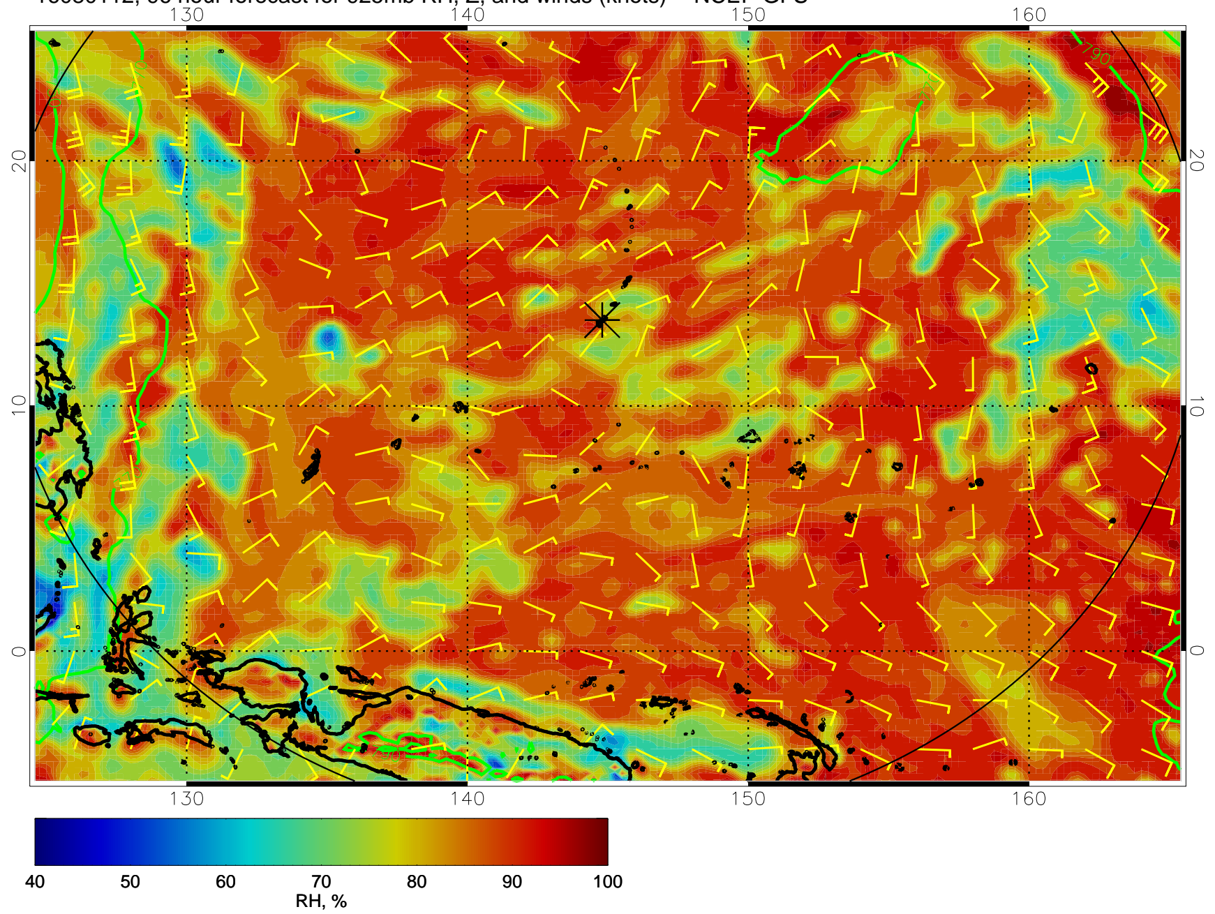
16080112, 96 hour forecast for 925mb RH, Z, and winds (knots) -- NCEP GFS
