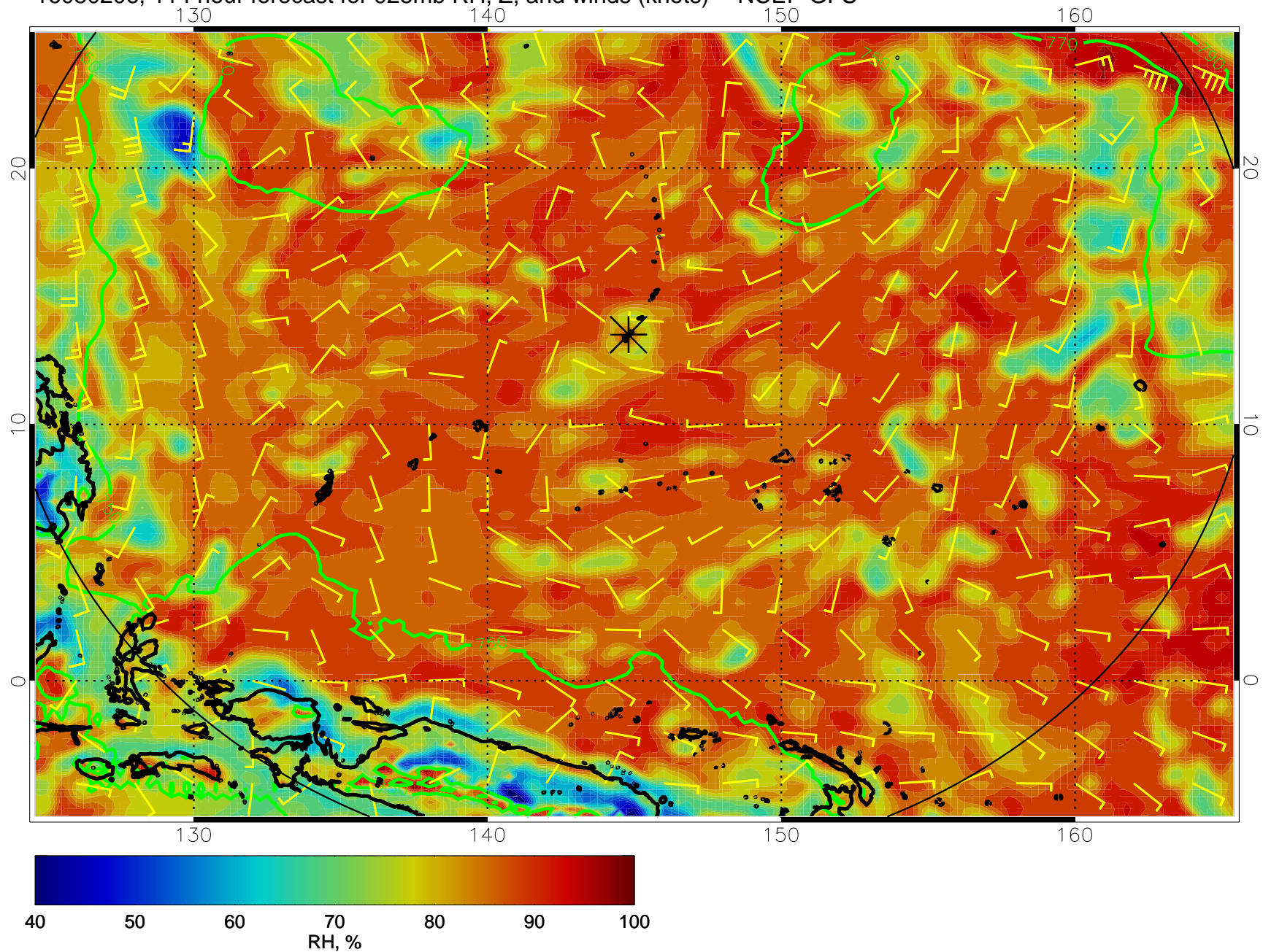
16080206, 114 hour forecast for 925mb RH, Z, and winds (knots) -- NCEP GFS
