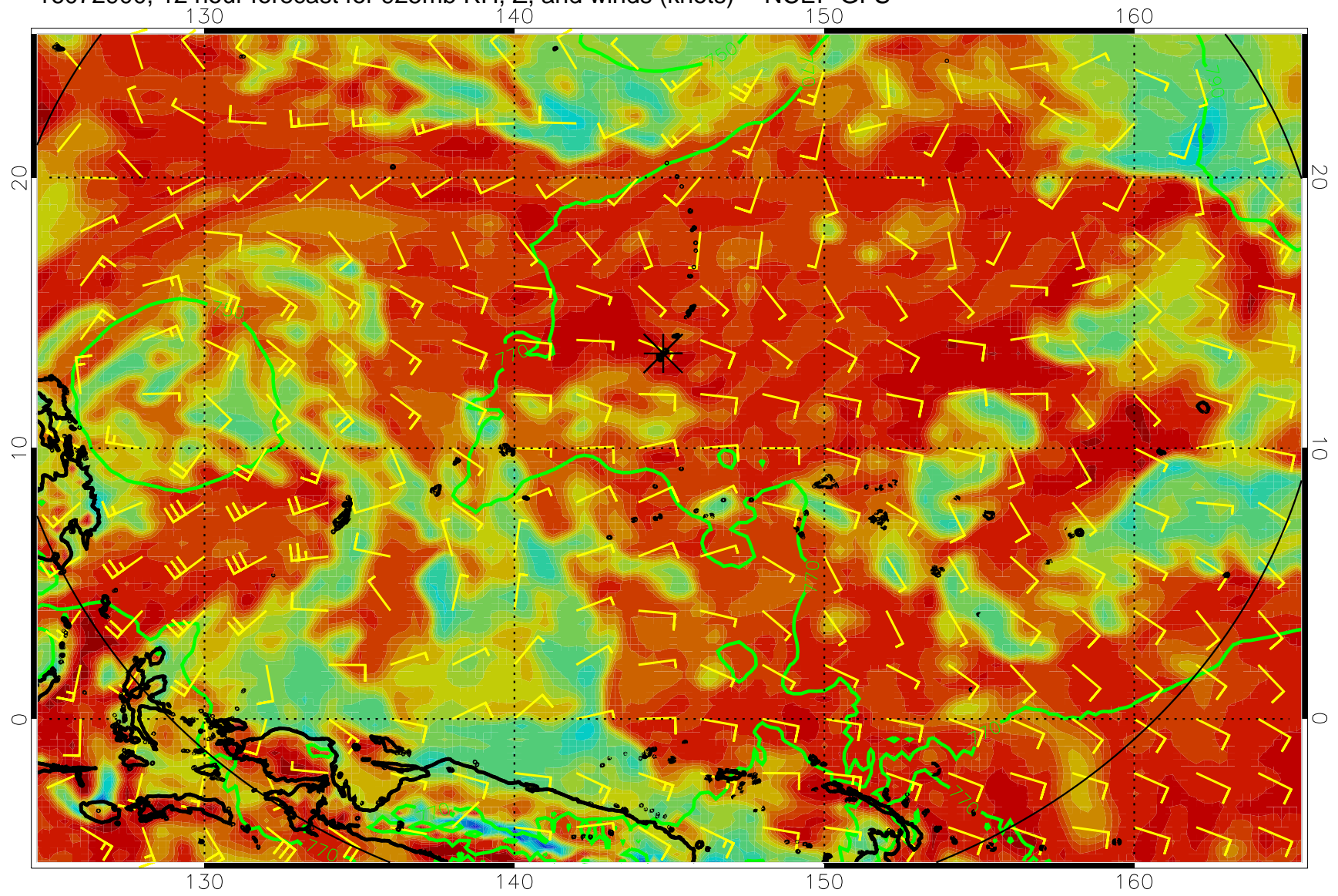
16072900, 12 hour forecast for 925mb RH, Z, and winds (knots) -- NCEP GFS
