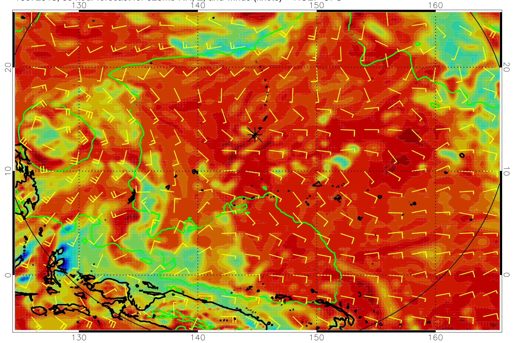
16072918, 30 hour forecast for 925mb RH, Z, and winds (knots) -- NCEP GFS
