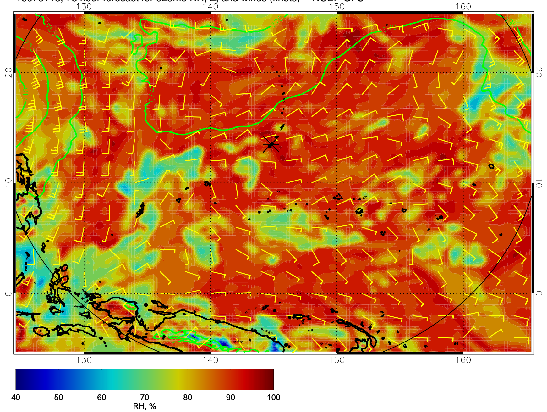
16073118, 78 hour forecast for 925mb RH, Z, and winds (knots) -- NCEP GFS
