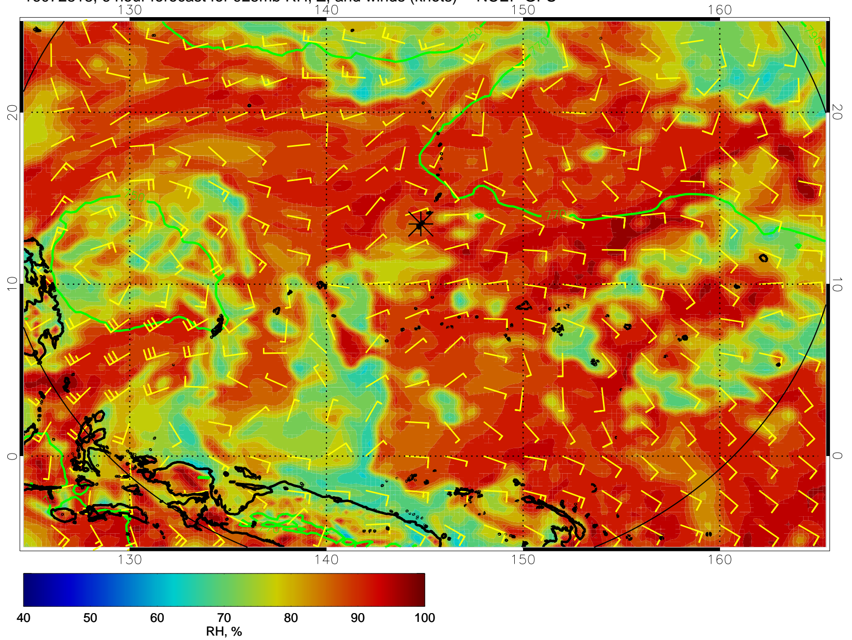
16072818, 6 hour forecast for 925mb RH, Z, and winds (knots) -- NCEP GFS
