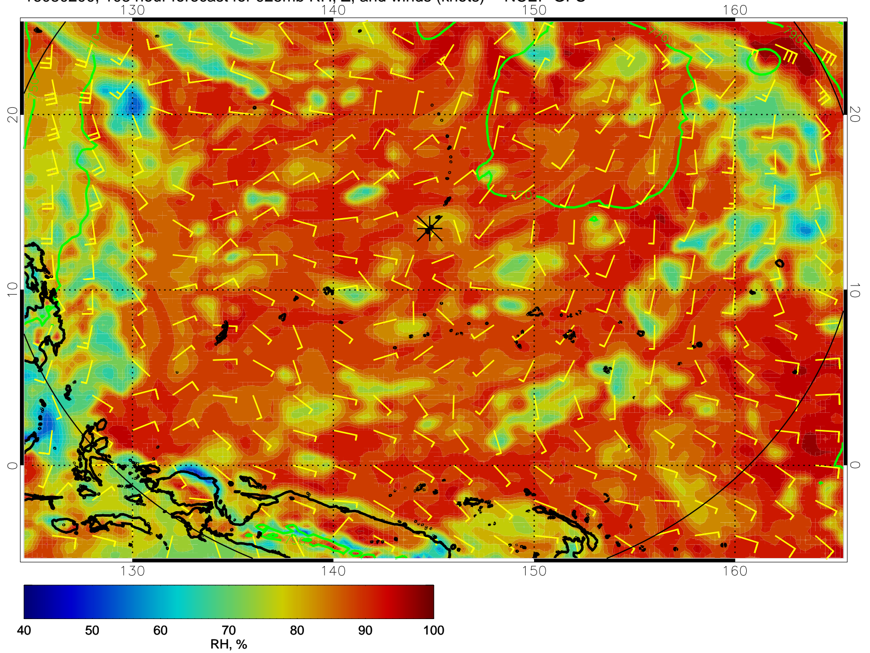
16080200, 108 hour forecast for 925mb RH, Z, and winds (knots) -- NCEP GFS
