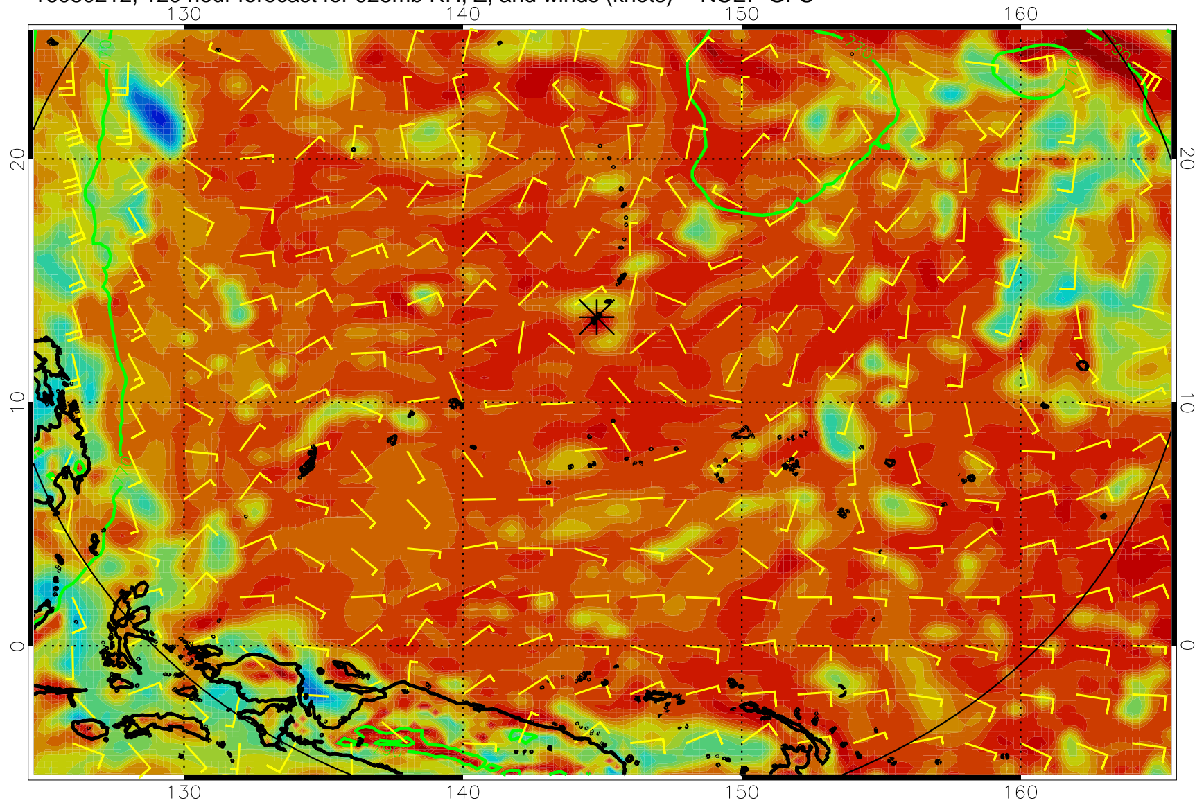
16080212, 120 hour forecast for 925mb RH, Z, and winds (knots) -- NCEP GFS
