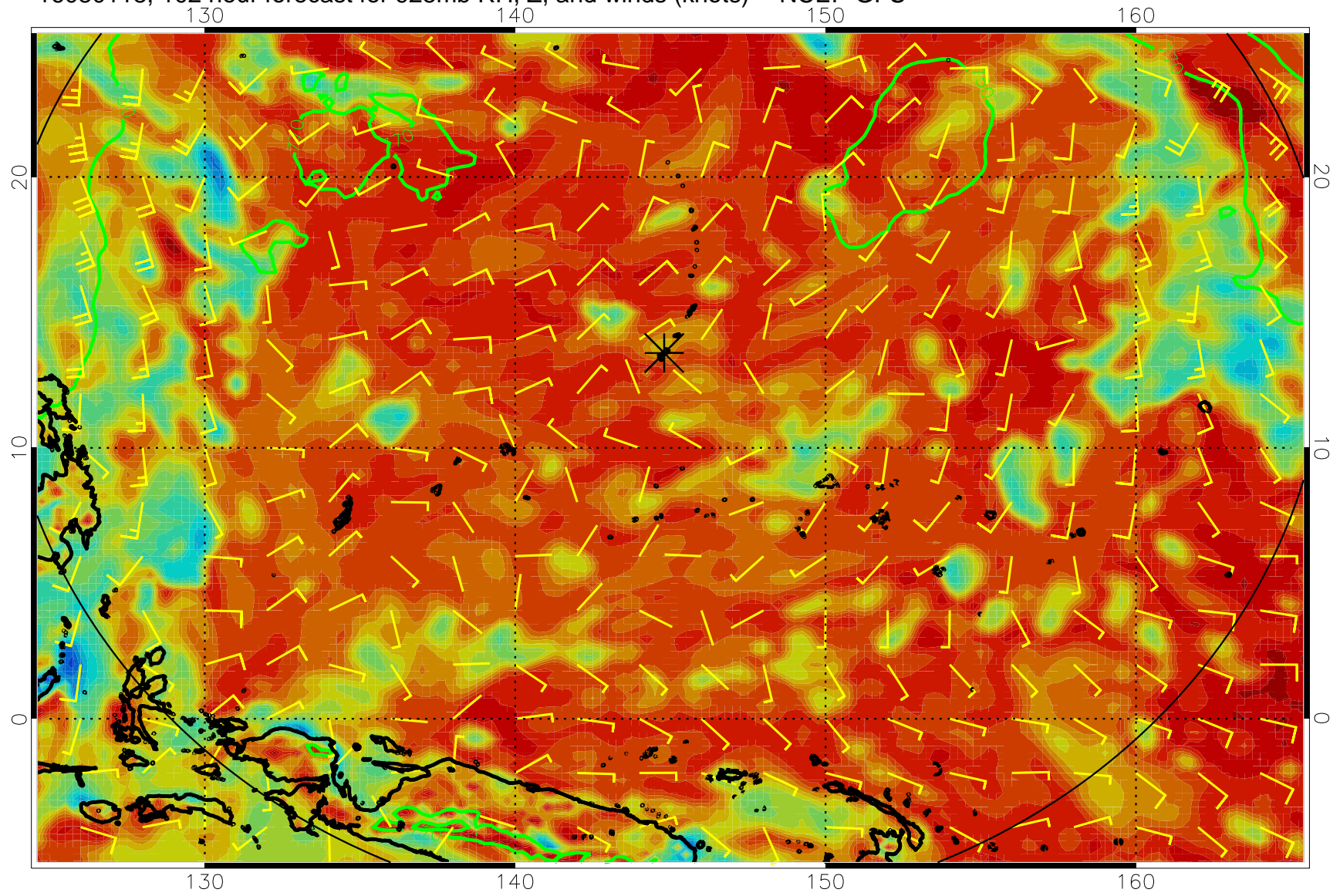
16080118, 102 hour forecast for 925mb RH, Z, and winds (knots) -- NCEP GFS
