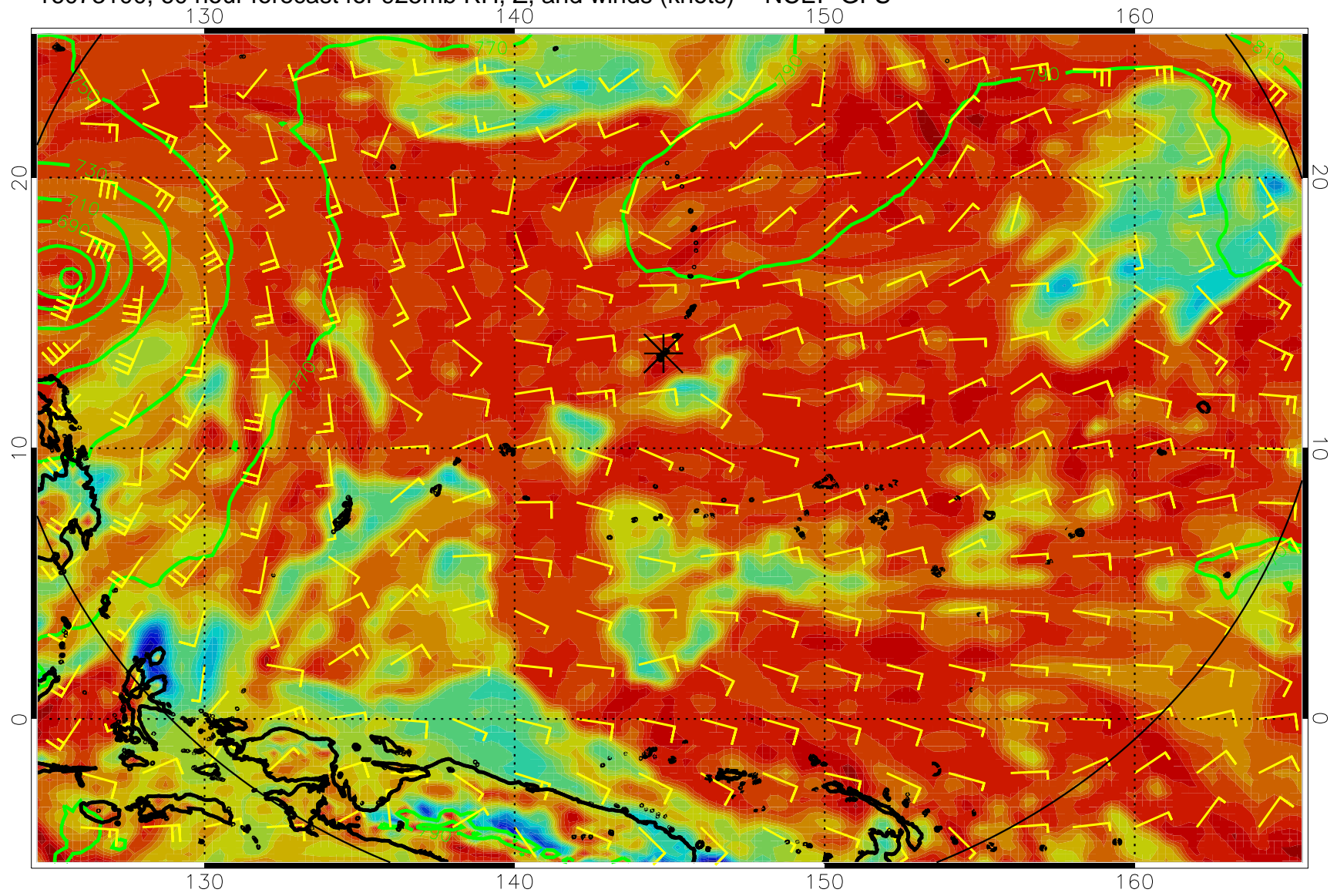
16073100, 60 hour forecast for 925mb RH, Z, and winds (knots) -- NCEP GFS
