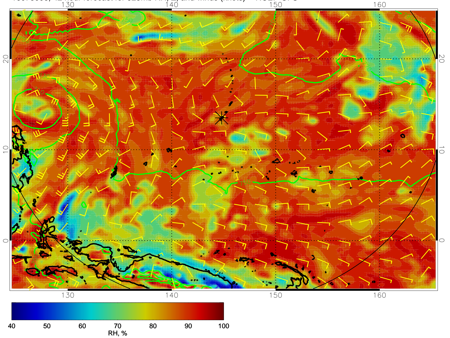
16073006, 42 hour forecast for 925mb RH, Z, and winds (knots) -- NCEP GFS
