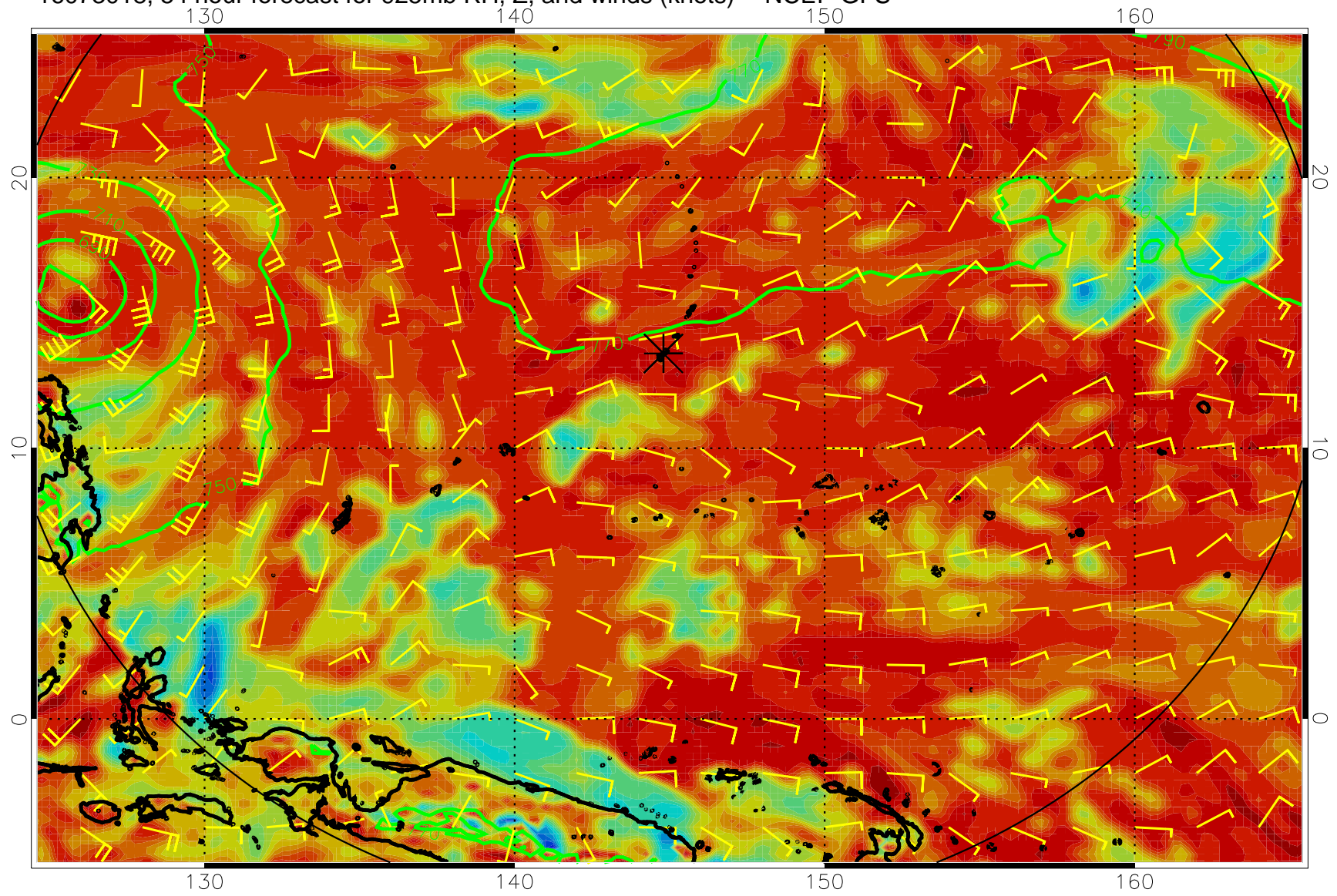
16073018, 54 hour forecast for 925mb RH, Z, and winds (knots) -- NCEP GFS
