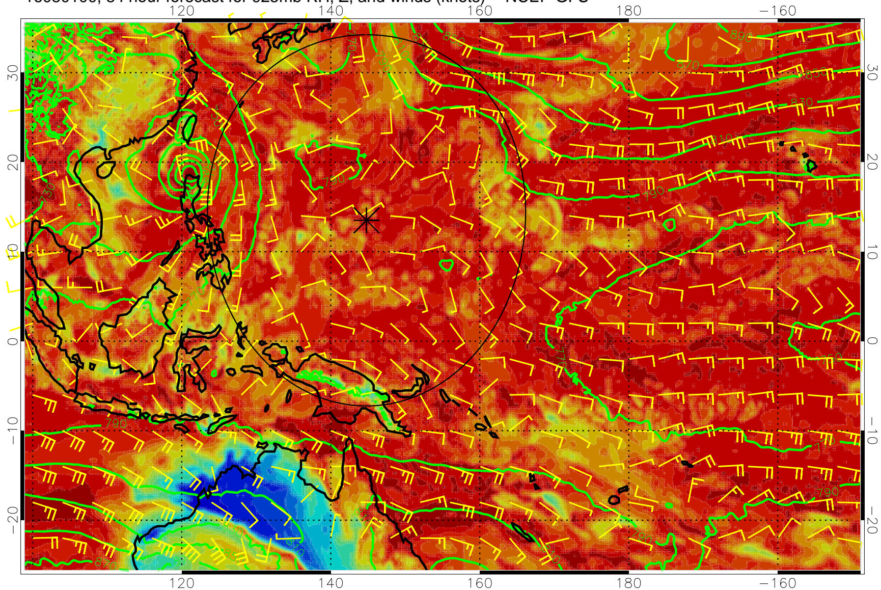
16080100, 84 hour forecast for 925mb RH, Z, and winds (knots) -- NCEP GFS
