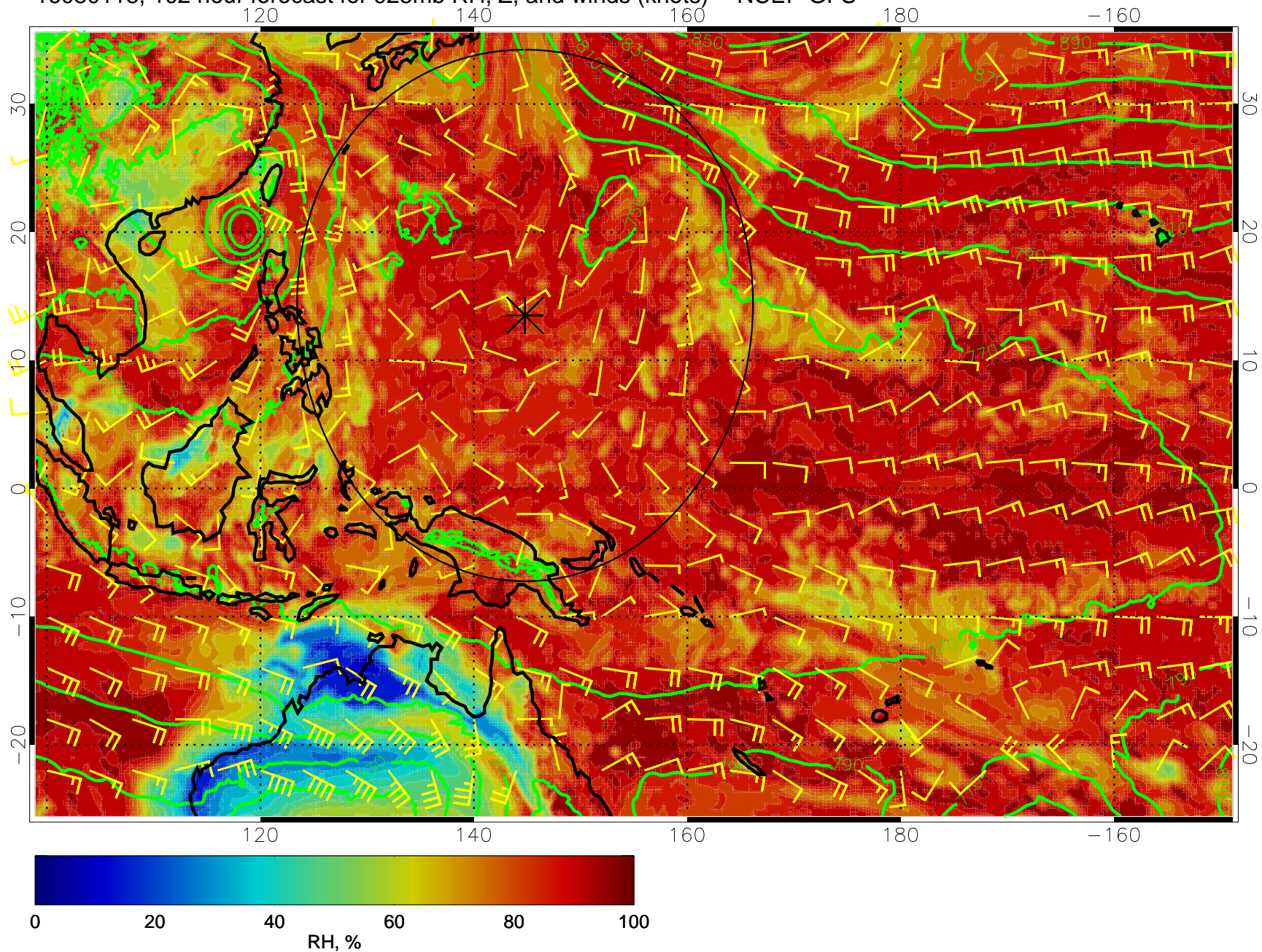
16080118, 102 hour forecast for 925mb RH, Z, and winds (knots) -- NCEP GFS
