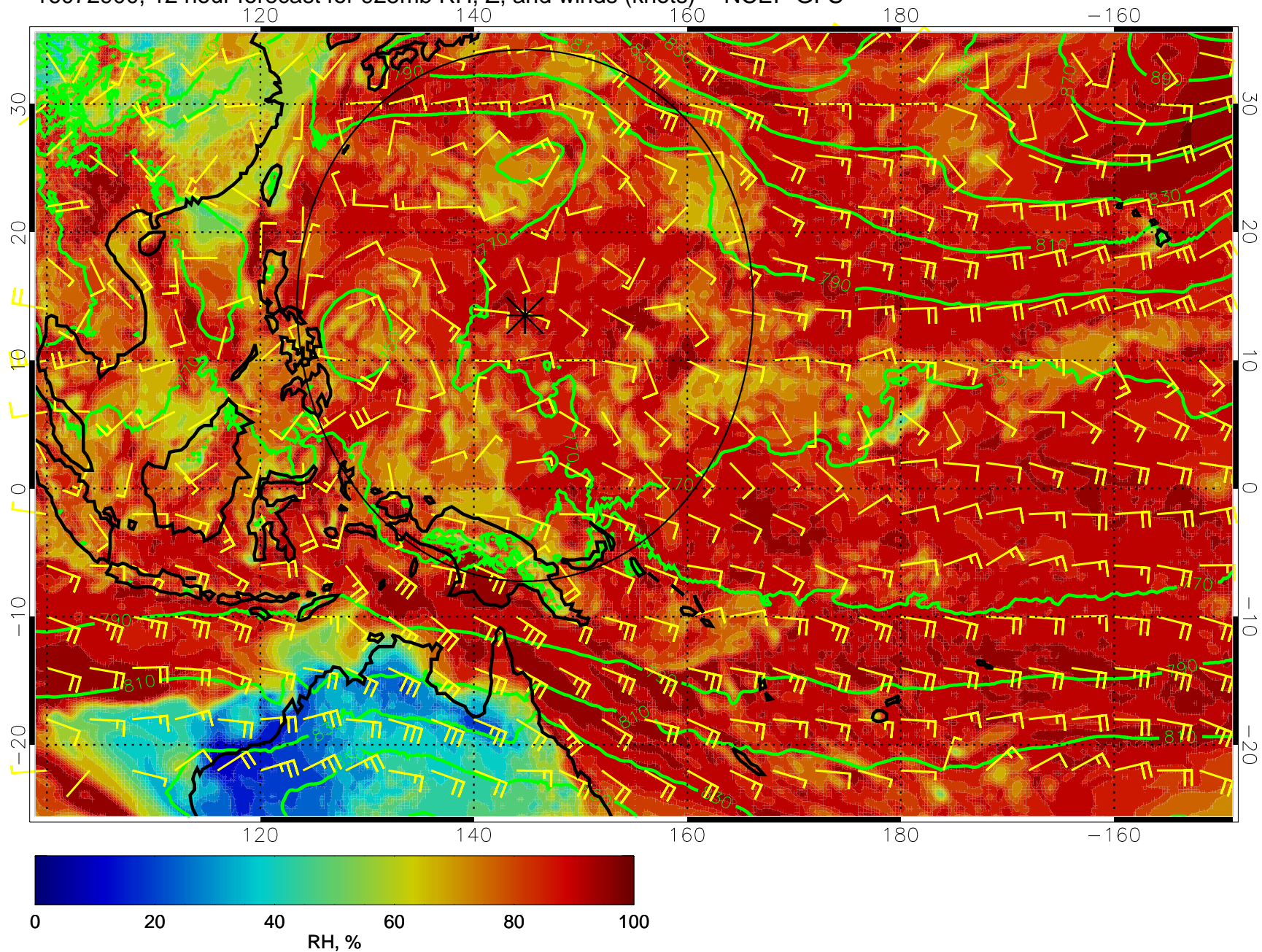
16072900, 12 hour forecast for 925mb RH, Z, and winds (knots) -- NCEP GFS
