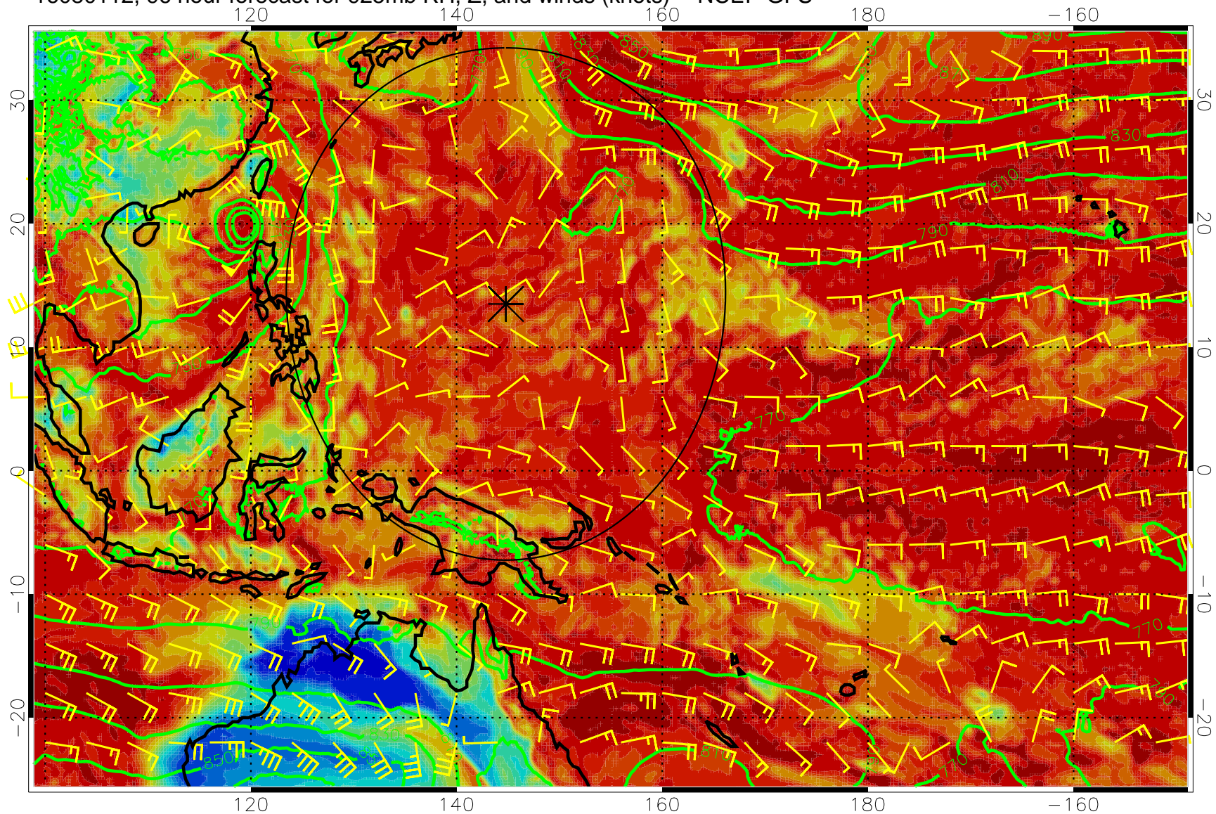
16080112, 96 hour forecast for 925mb RH, Z, and winds (knots) -- NCEP GFS
