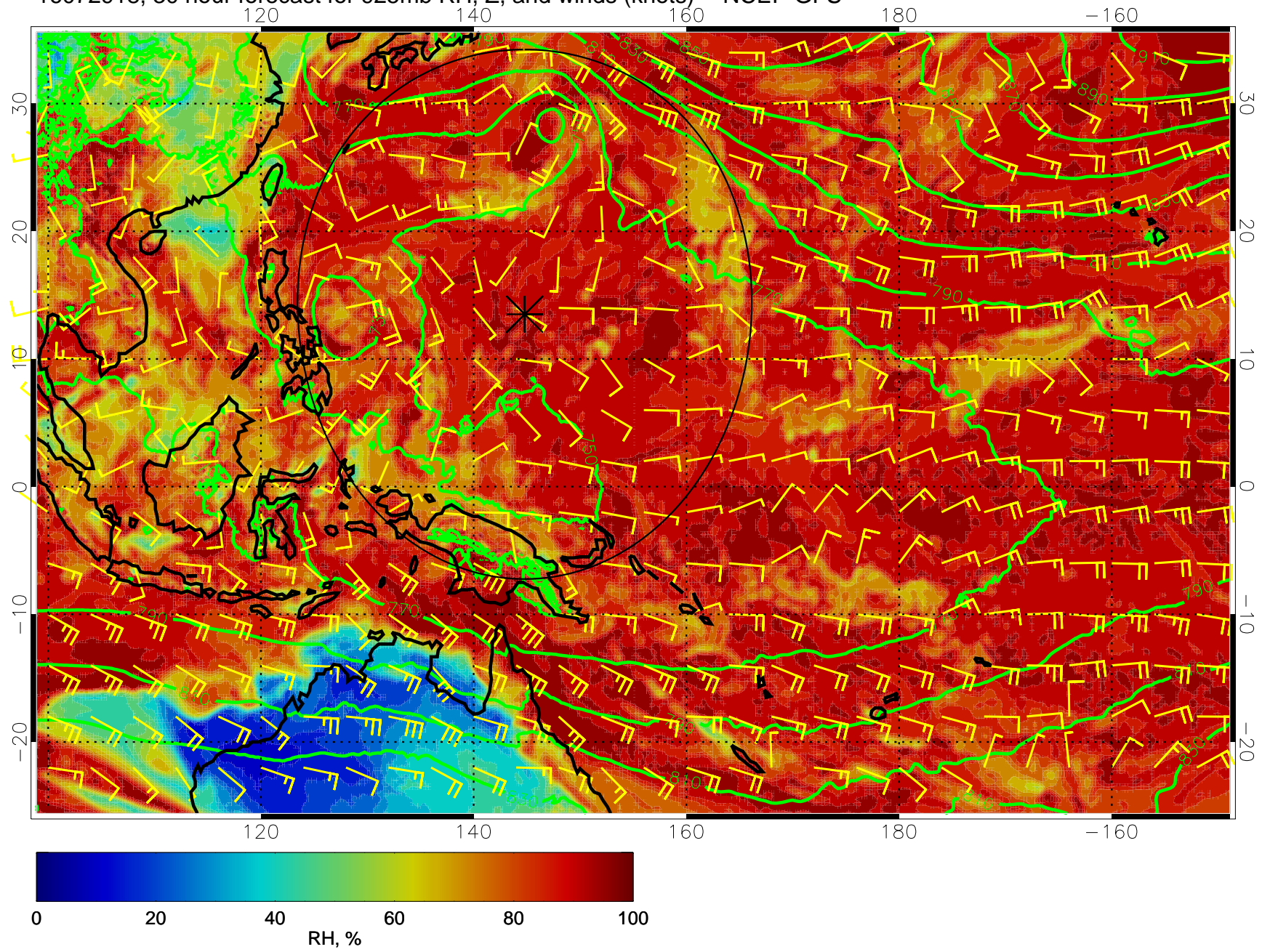
16072918, 30 hour forecast for 925mb RH, Z, and winds (knots) -- NCEP GFS
