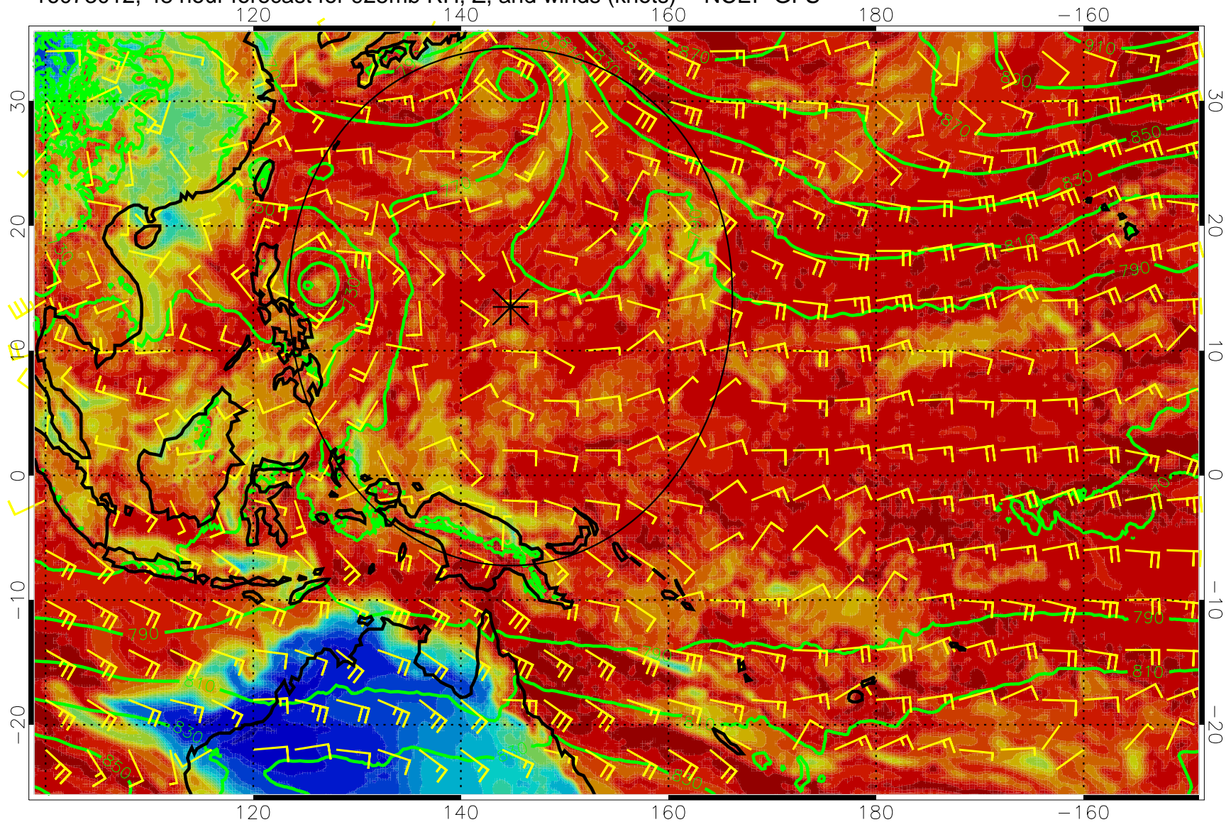
16073012, 48 hour forecast for 925mb RH, Z, and winds (knots) -- NCEP GFS
