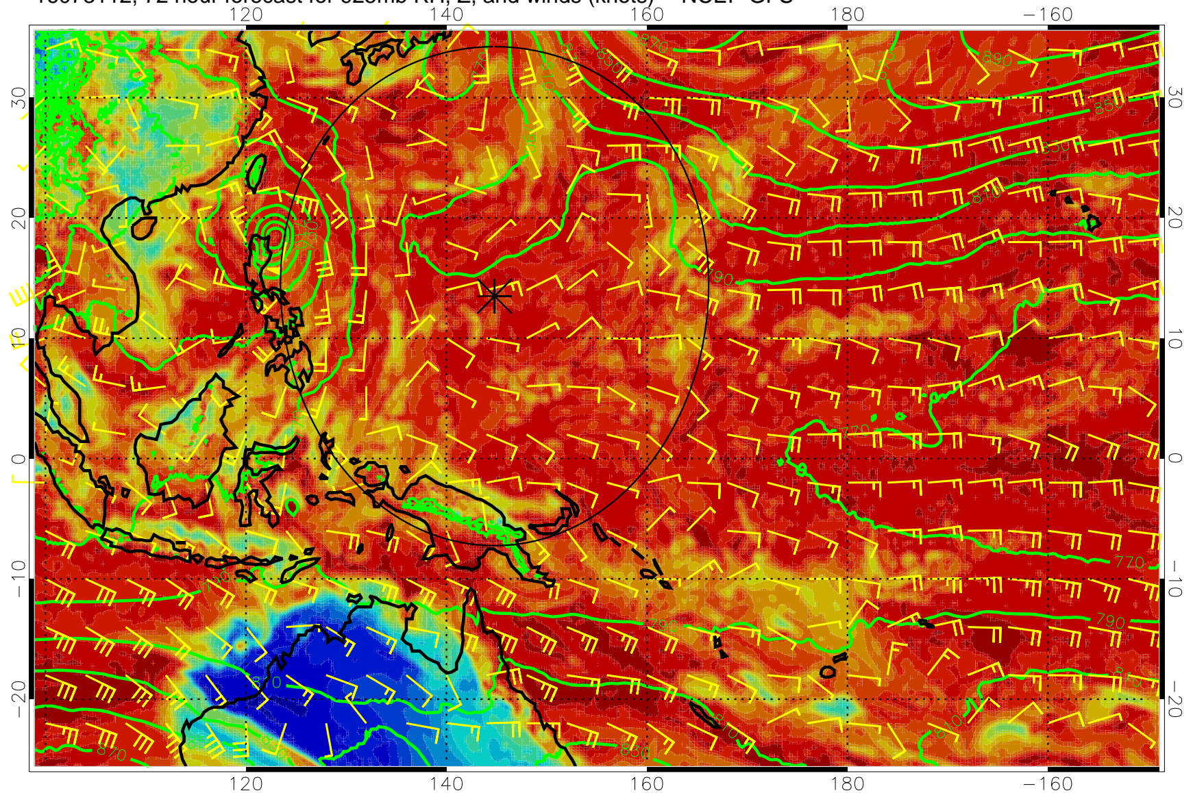
16073112, 72 hour forecast for 925mb RH, Z, and winds (knots) -- NCEP GFS
