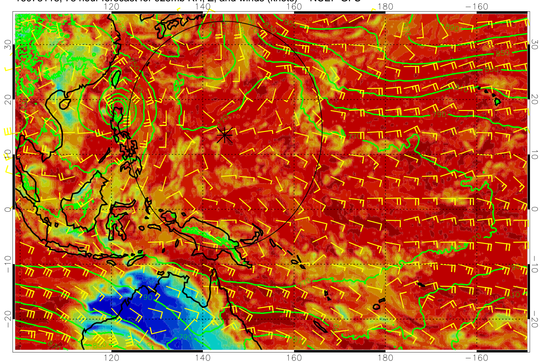
16073118, 78 hour forecast for 925mb RH, Z, and winds (knots) -- NCEP GFS
