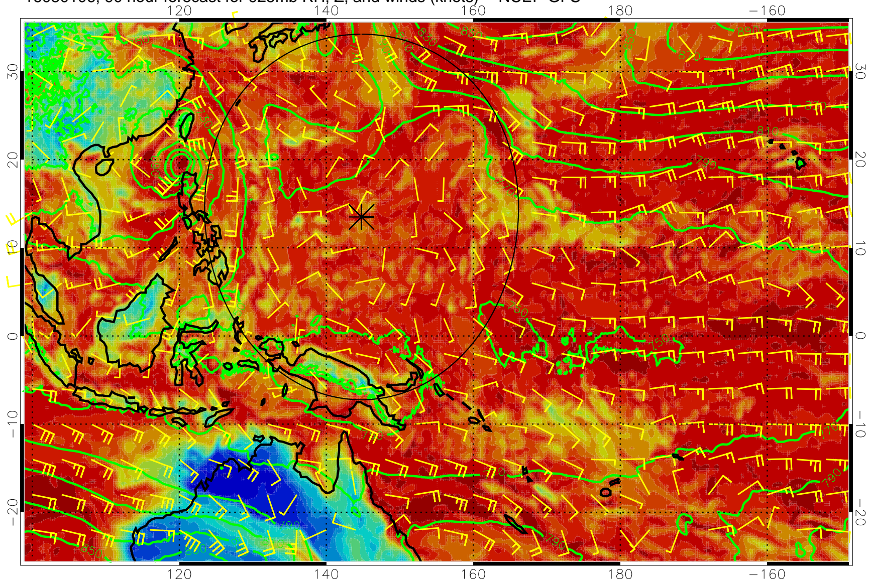
16080106, 90 hour forecast for 925mb RH, Z, and winds (knots) -- NCEP GFS
