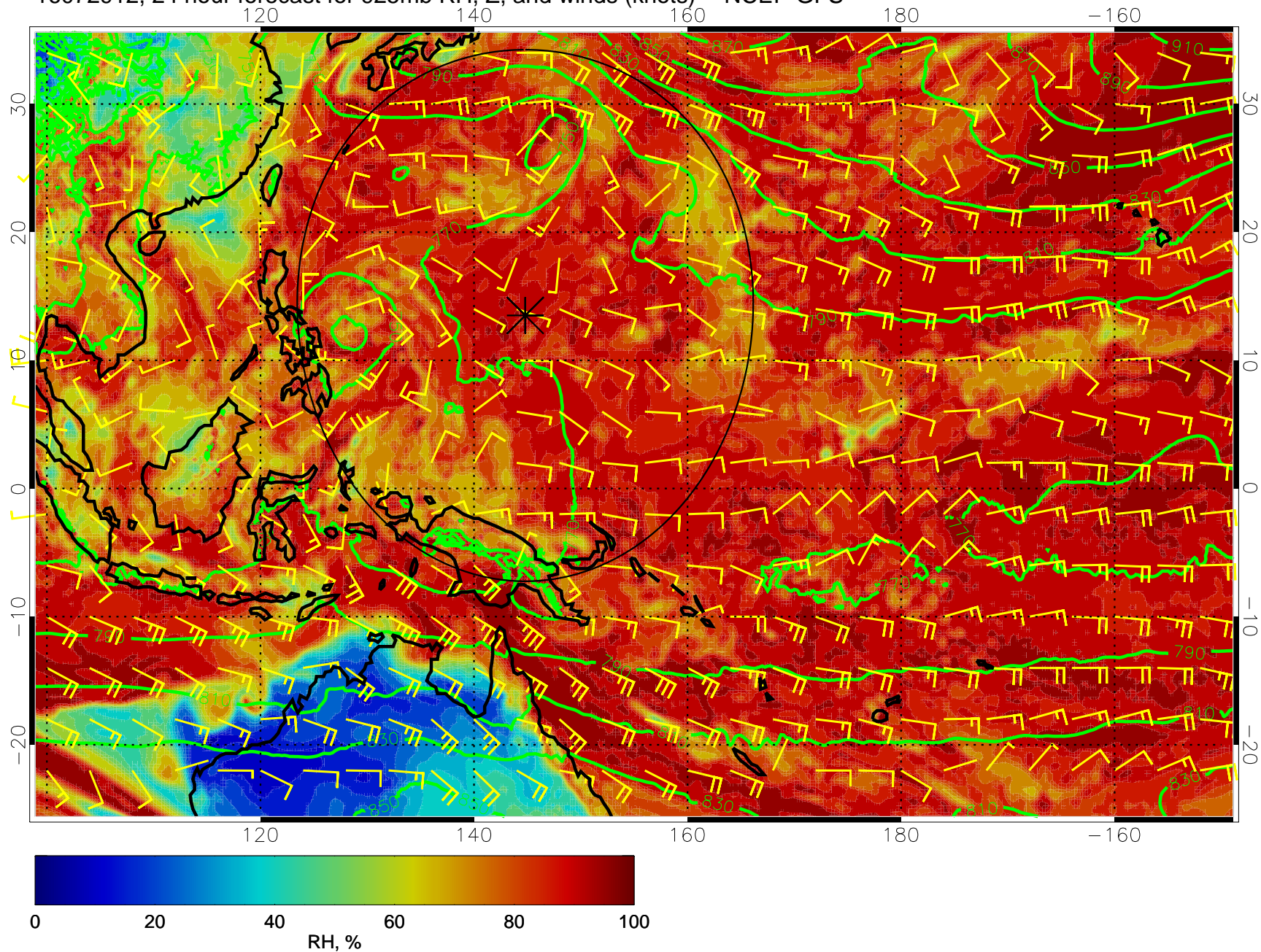
16072912, 24 hour forecast for 925mb RH, Z, and winds (knots) -- NCEP GFS
