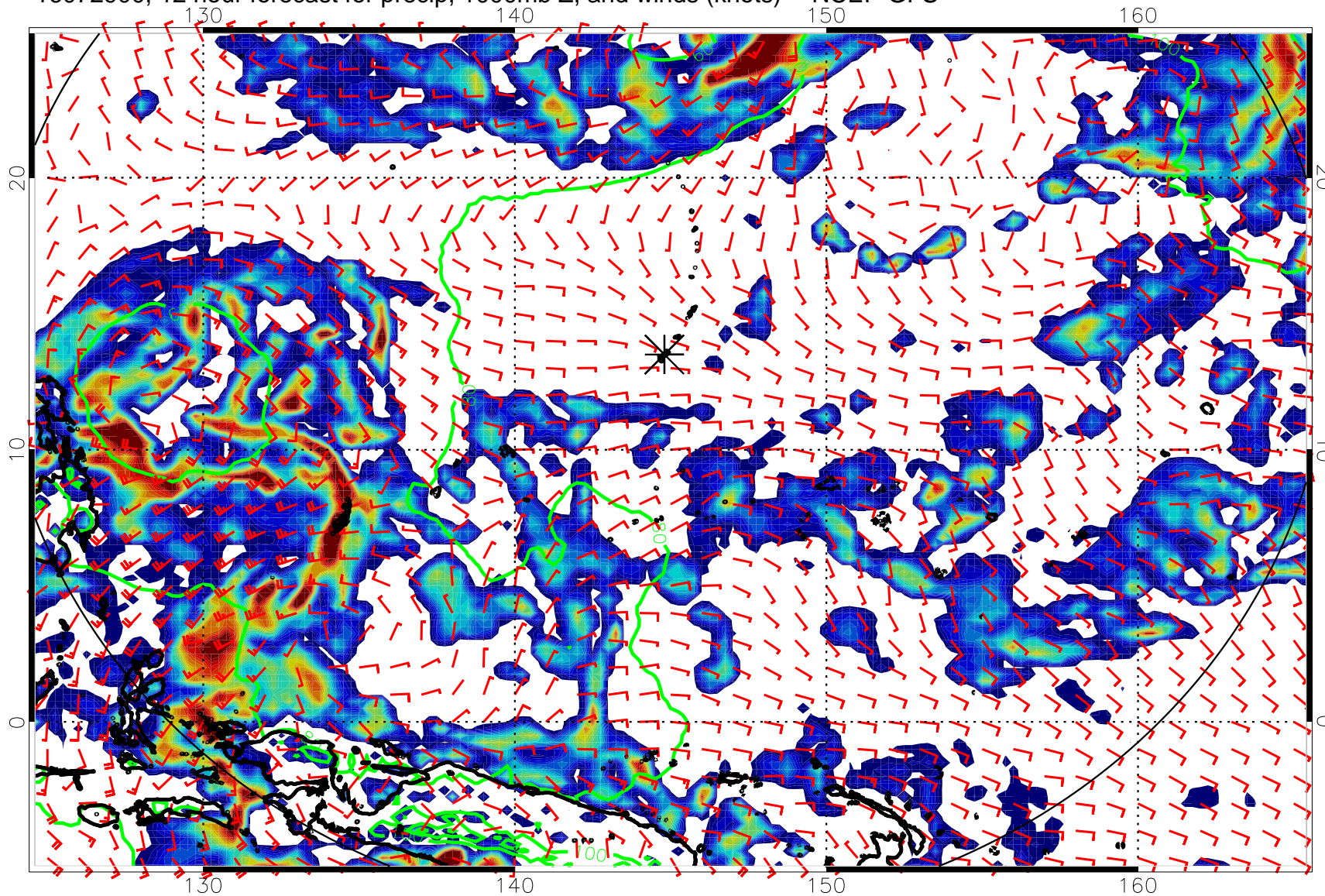
16072900, 12 hour forecast for precip, 1000mb Z, and winds (knots) -- NCEP GFS
