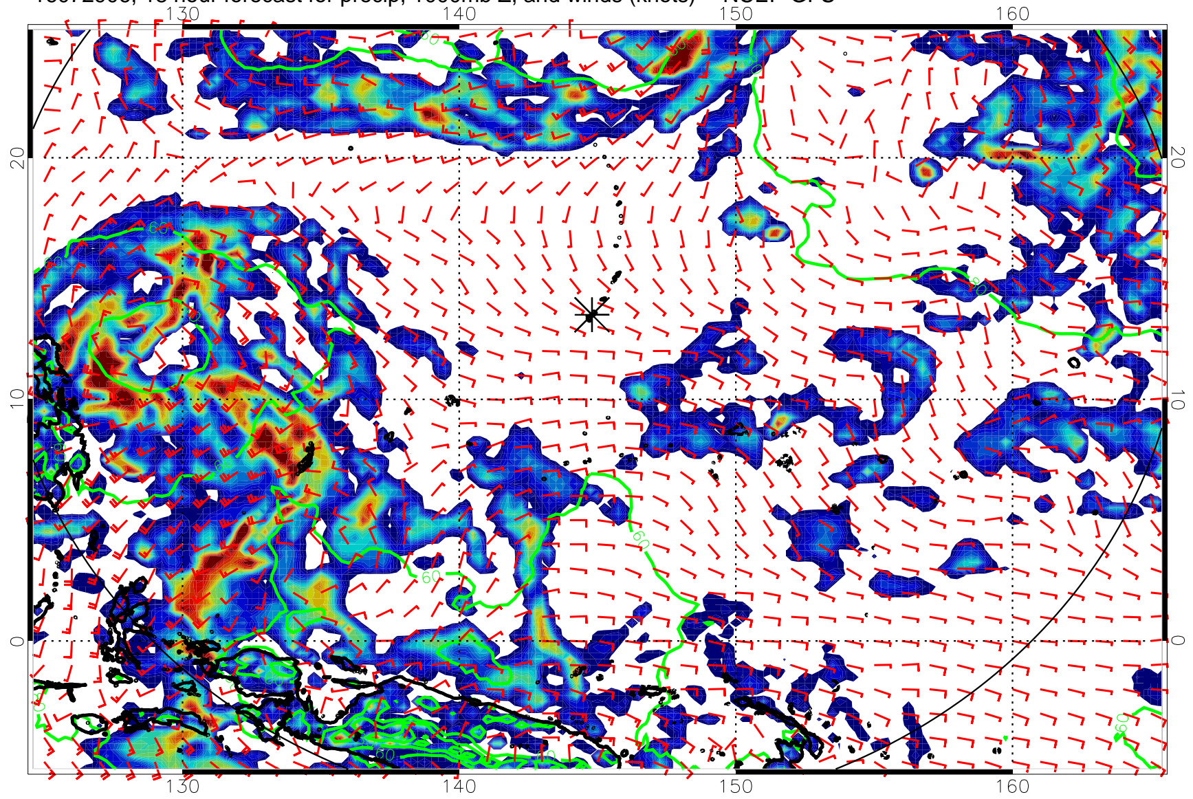
16072906, 18 hour forecast for precip, 1000mb Z, and winds (knots) -- NCEP GFS
