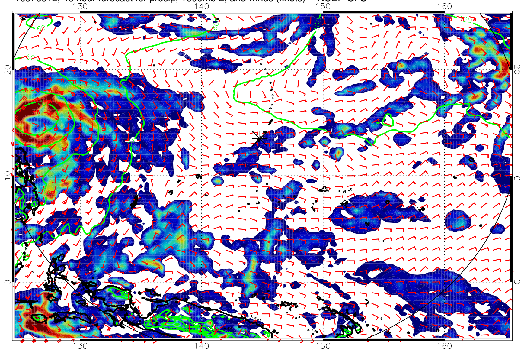
16073012, 48 hour forecast for precip, 1000mb Z, and winds (knots) -- NCEP GFS
