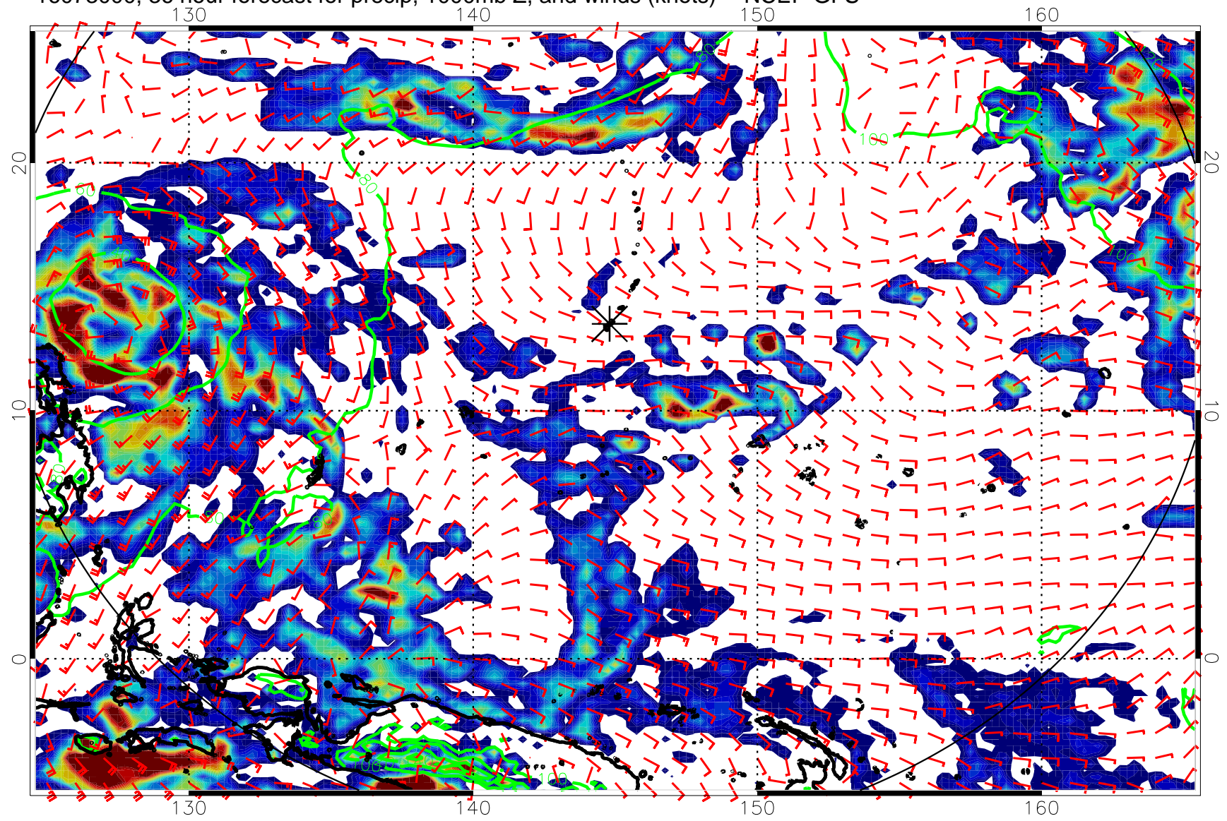
16073000, 36 hour forecast for precip, 1000mb Z, and winds (knots) -- NCEP GFS
