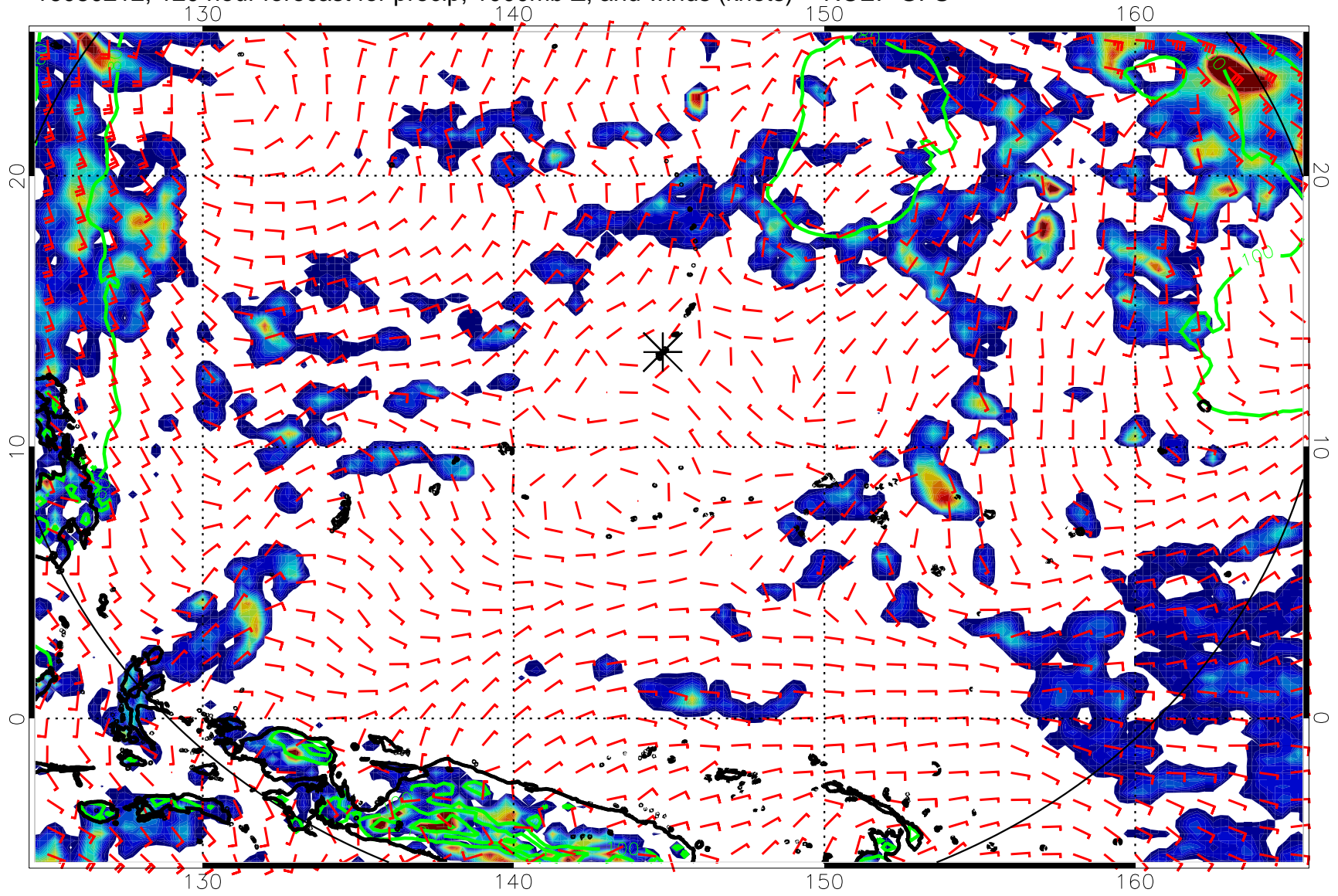
16080212, 120 hour forecast for precip, 1000mb Z, and winds (knots) -- NCEP GFS
