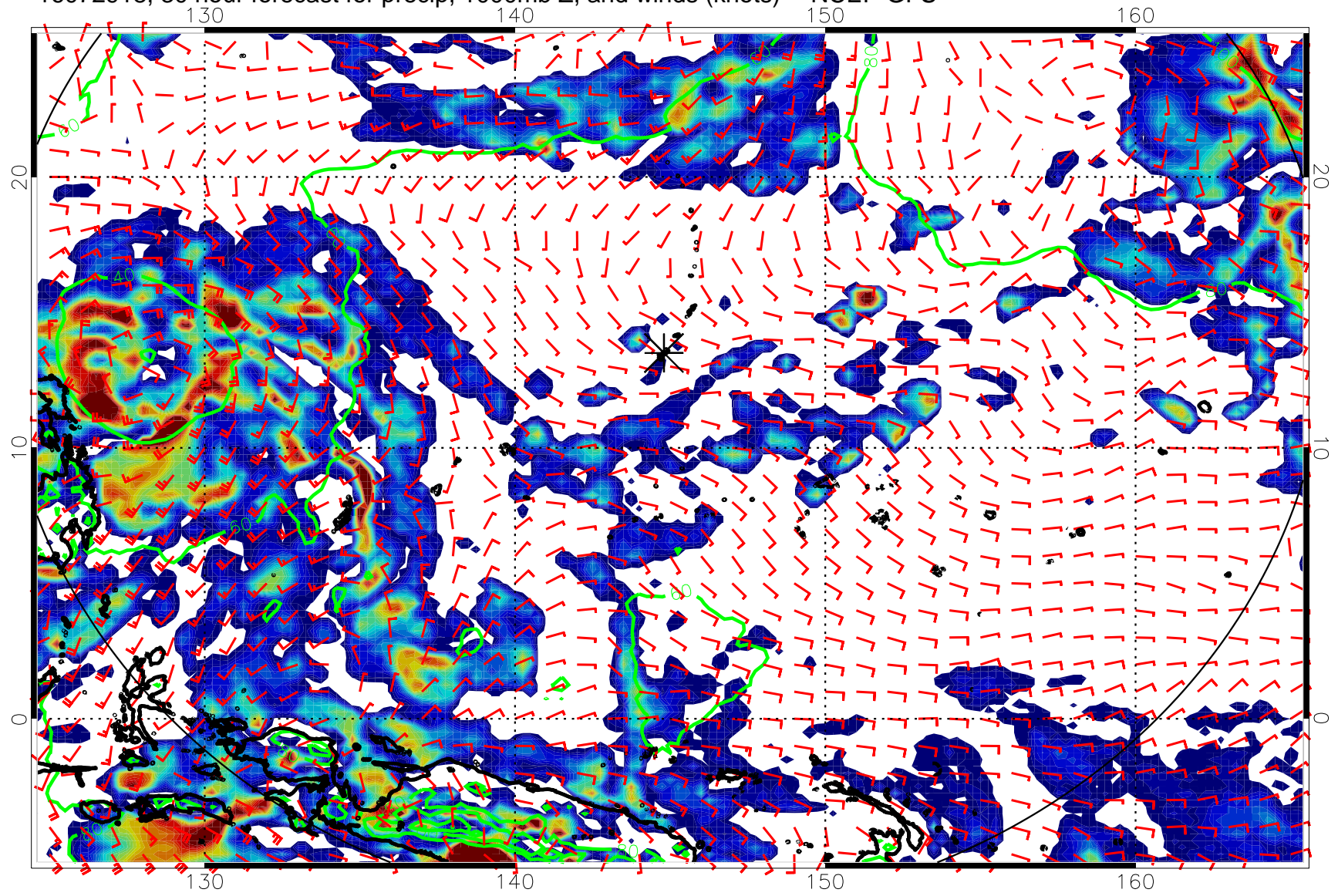
16072918, 30 hour forecast for precip, 1000mb Z, and winds (knots) -- NCEP GFS
