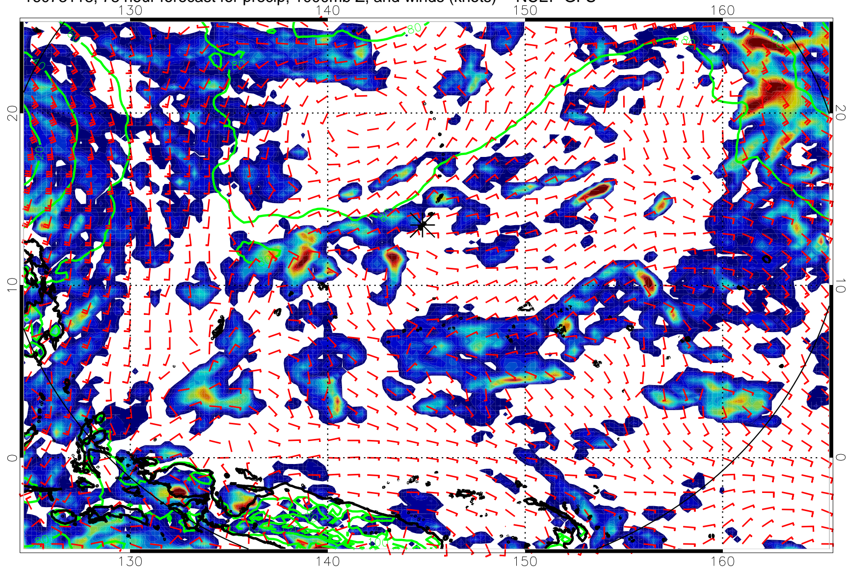
16073118, 78 hour forecast for precip, 1000mb Z, and winds (knots) -- NCEP GFS
