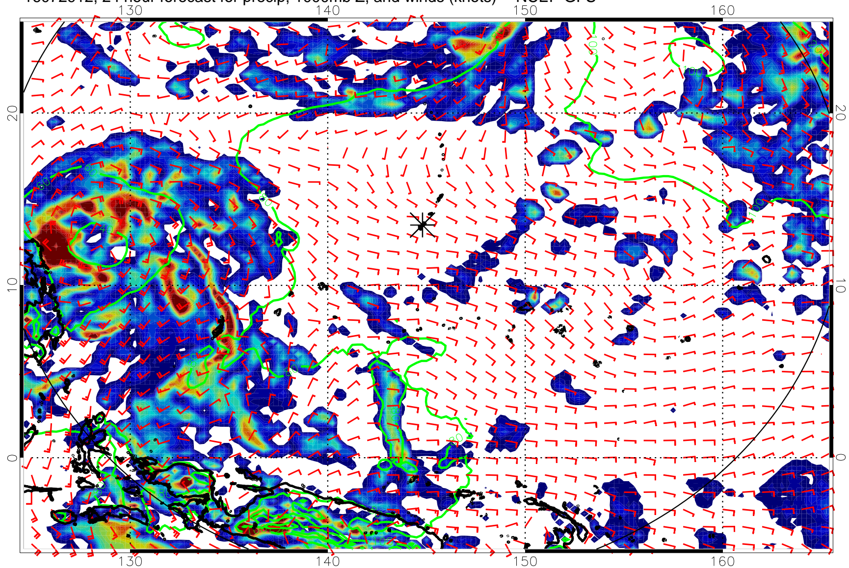
16072912, 24 hour forecast for precip, 1000mb Z, and winds (knots) -- NCEP GFS
