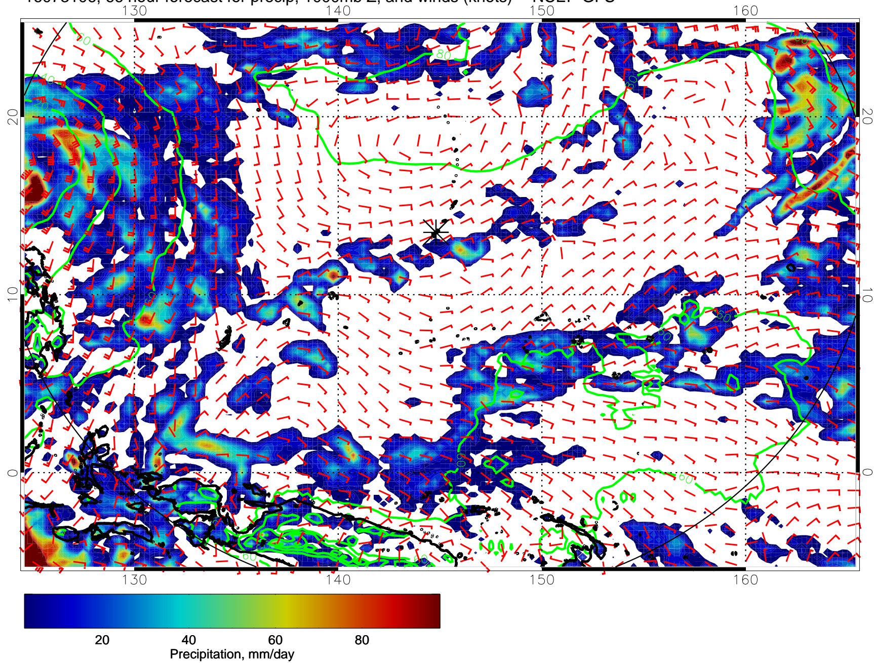
16073106, 66 hour forecast for precip, 1000mb Z, and winds (knots) -- NCEP GFS
