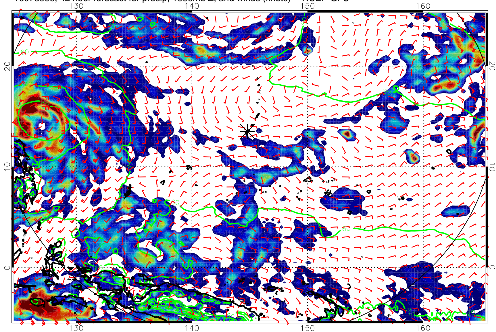
16073006, 42 hour forecast for precip, 1000mb Z, and winds (knots) -- NCEP GFS
