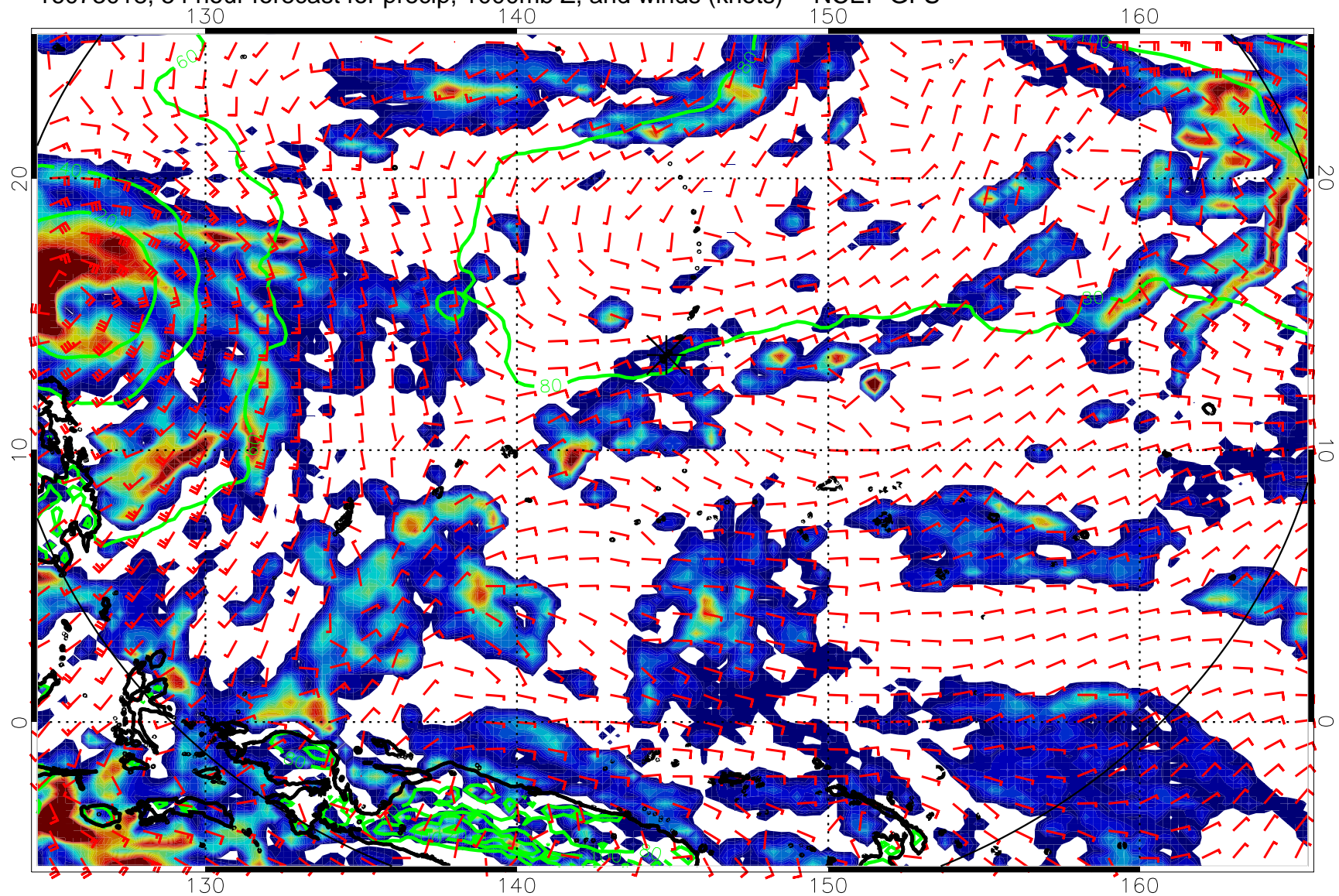
16073018, 54 hour forecast for precip, 1000mb Z, and winds (knots) -- NCEP GFS
