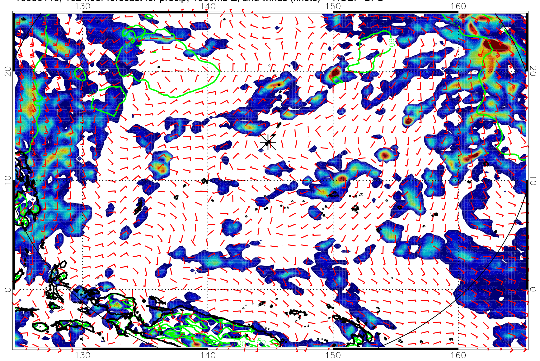
16080118, 102 hour forecast for precip, 1000mb Z, and winds (knots) -- NCEP GFS
