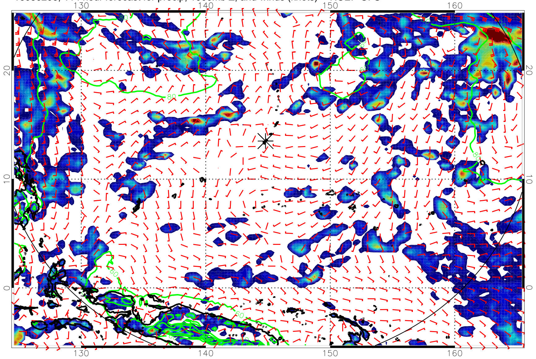
16080206, 114 hour forecast for precip, 1000mb Z, and winds (knots) -- NCEP GFS
