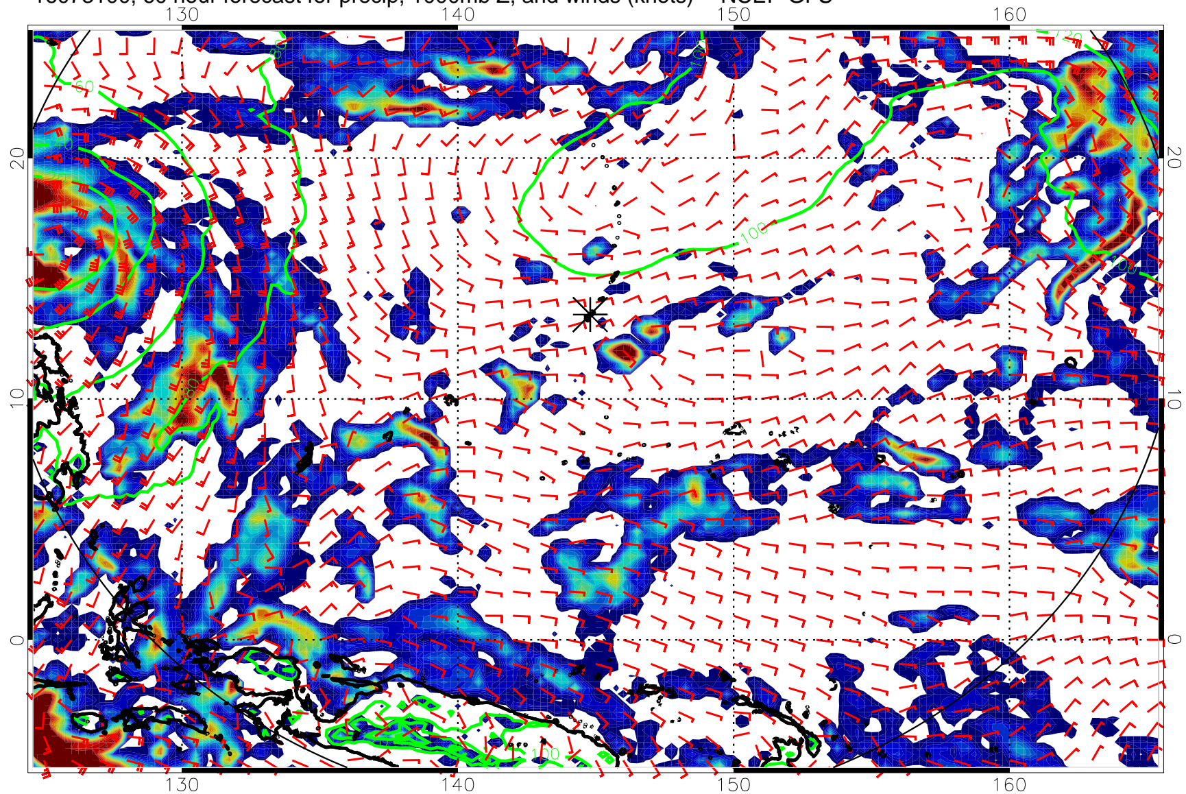
16073100, 60 hour forecast for precip, 1000mb Z, and winds (knots) -- NCEP GFS
