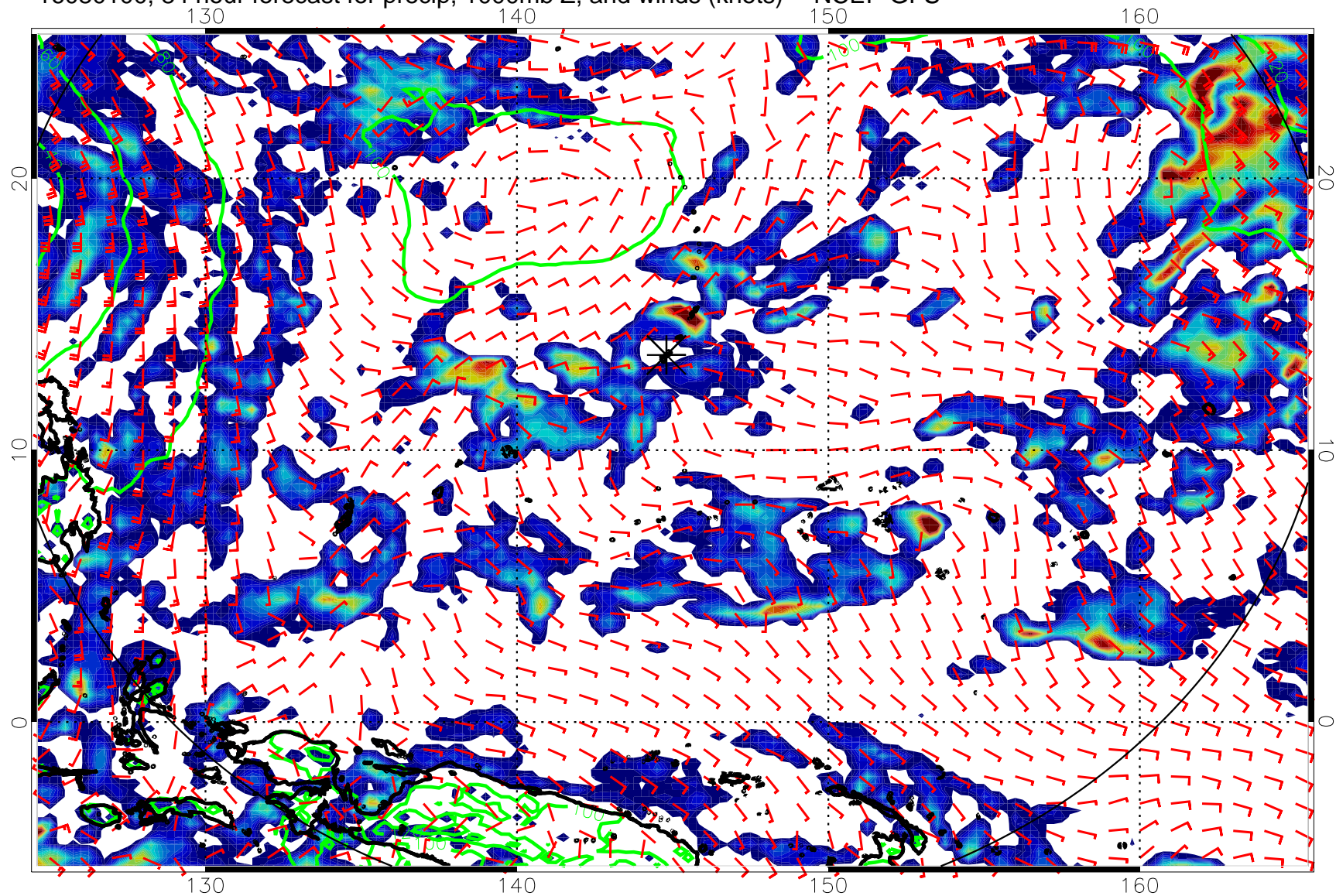
16080100, 84 hour forecast for precip, 1000mb Z, and winds (knots) -- NCEP GFS
