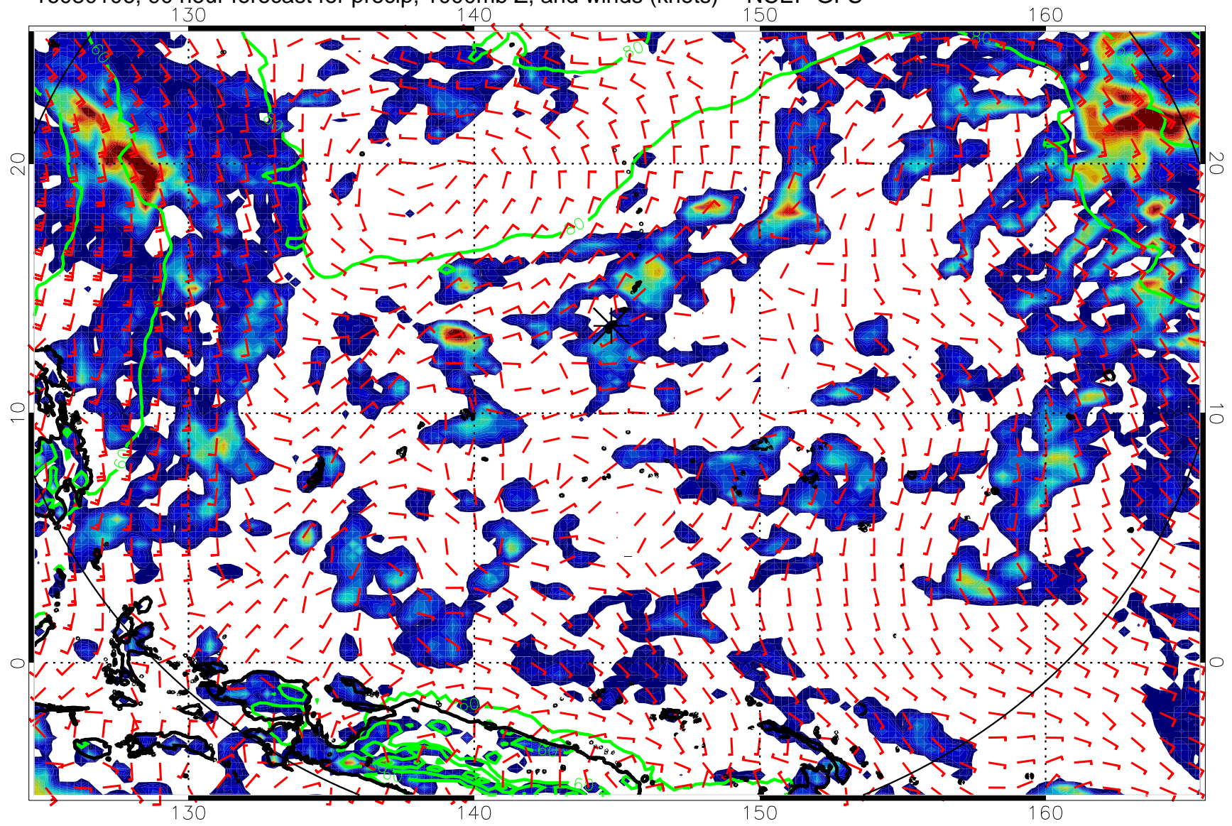
16080106, 90 hour forecast for precip, 1000mb Z, and winds (knots) -- NCEP GFS
