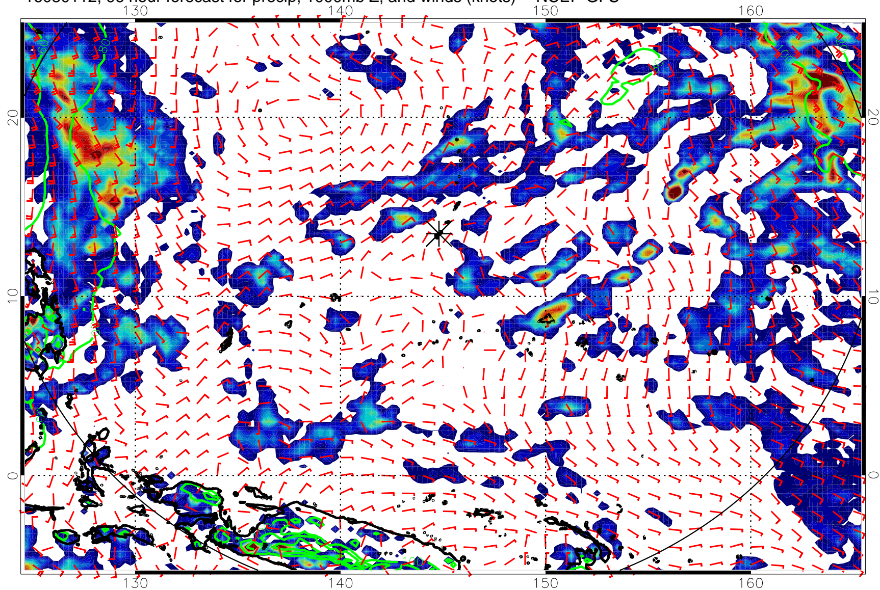
16080112, 96 hour forecast for precip, 1000mb Z, and winds (knots) -- NCEP GFS
