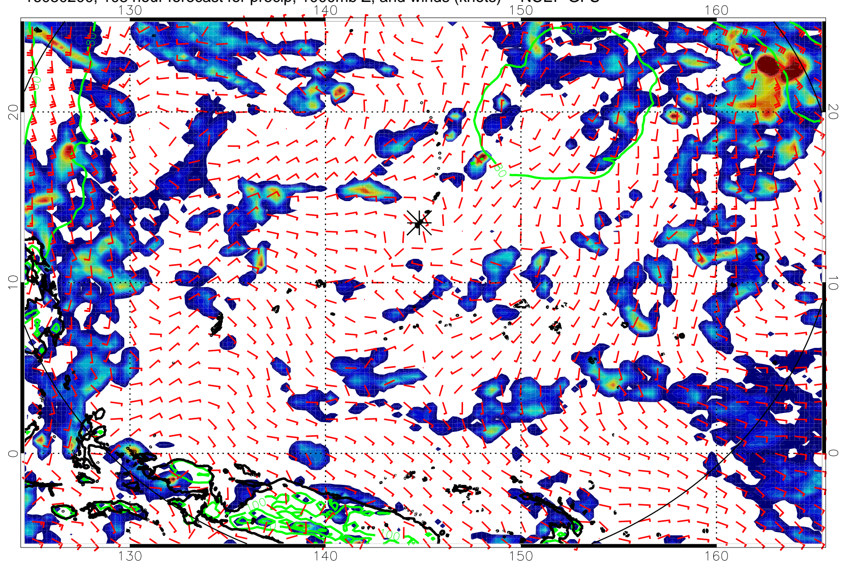
16080200, 108 hour forecast for precip, 1000mb Z, and winds (knots) -- NCEP GFS
