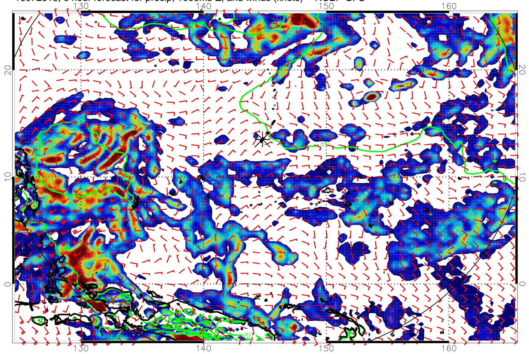
16072818, 6 hour forecast for precip, 1000mb Z, and winds (knots) -- NCEP GFS
