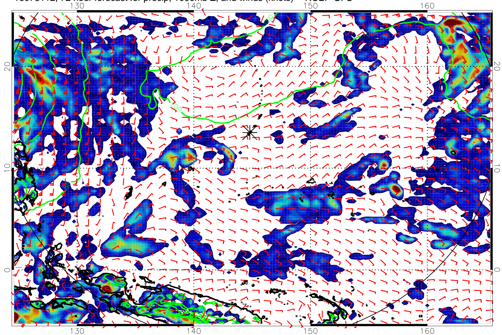
16073112, 72 hour forecast for precip, 1000mb Z, and winds (knots) -- NCEP GFS
