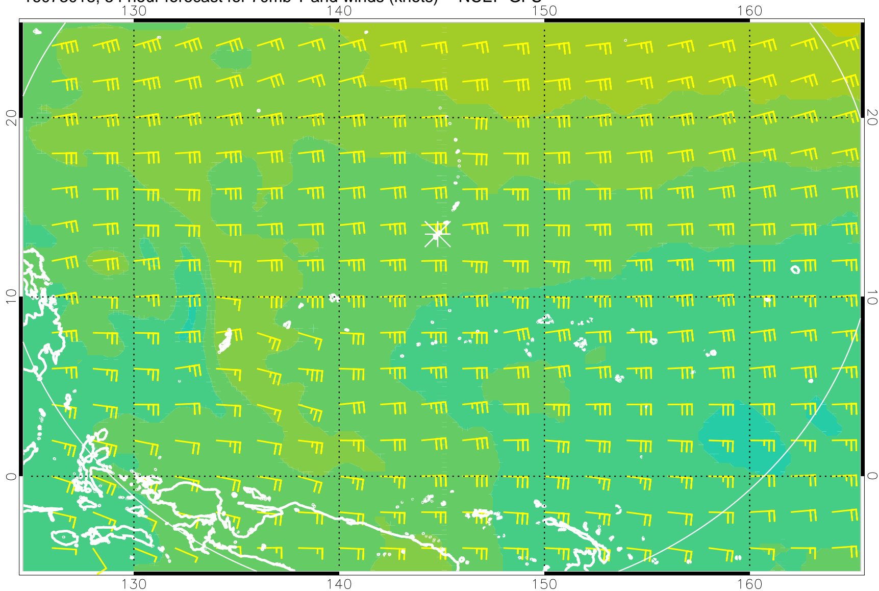
16073018, 54 hour forecast for 70mb T and winds (knots) -- NCEP GFS
