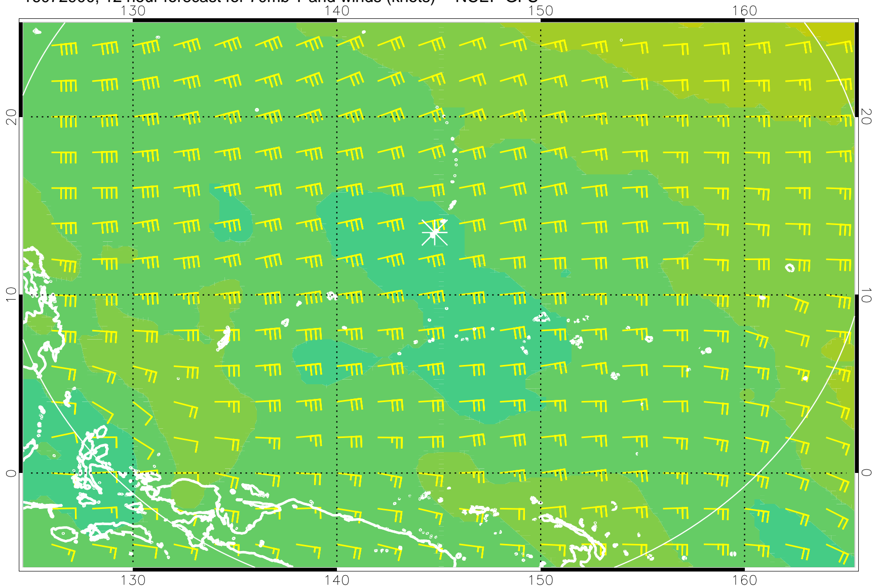
16072900, 12 hour forecast for 70mb T and winds (knots) -- NCEP GFS
