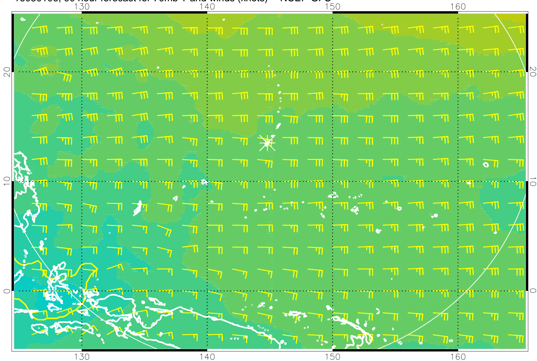
16080106, 90 hour forecast for 70mb T and winds (knots) -- NCEP GFS
