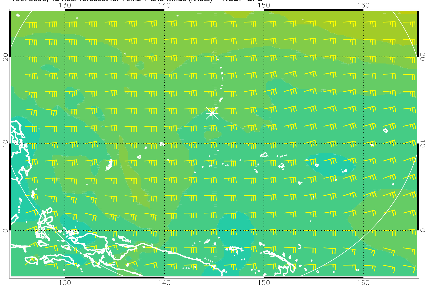
16073006, 42 hour forecast for 70mb T and winds (knots) -- NCEP GFS
