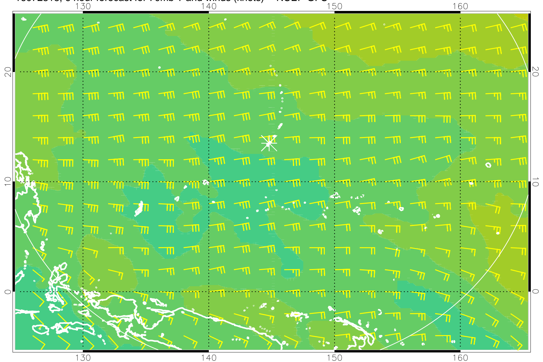
16072818, 6 hour forecast for 70mb T and winds (knots) -- NCEP GFS
