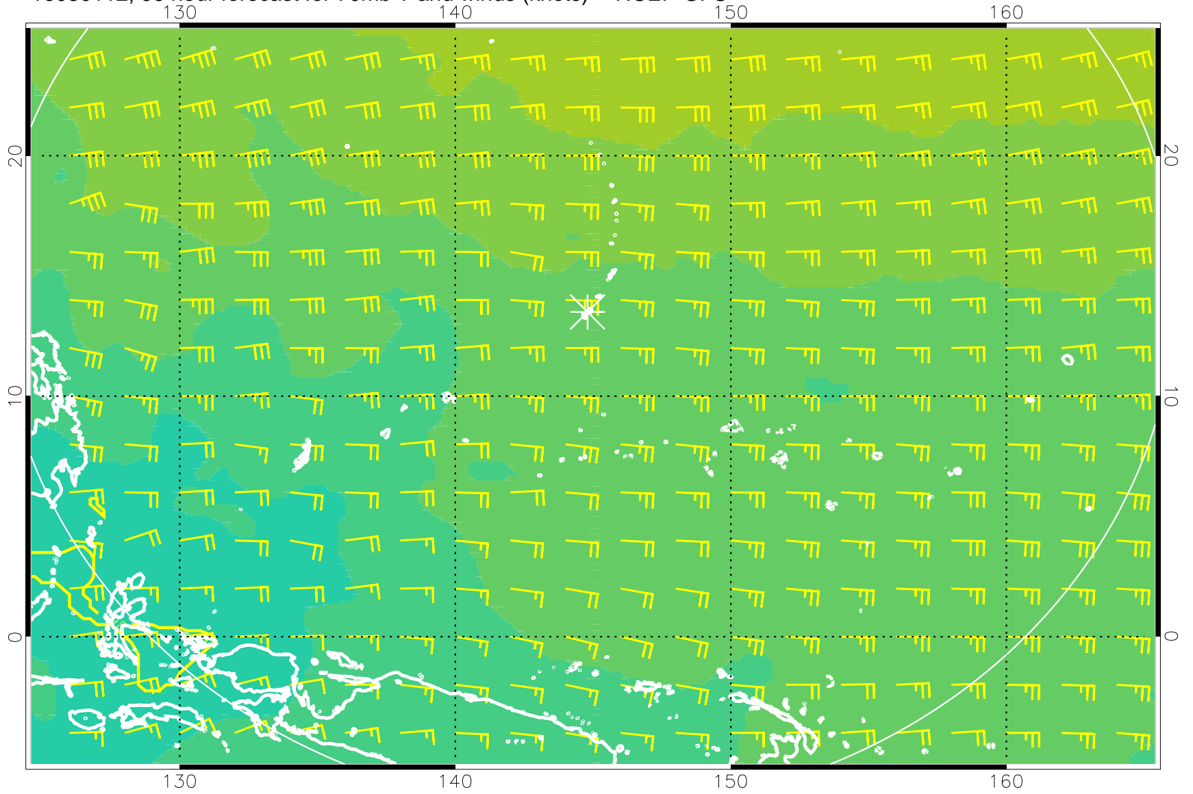
16080112, 96 hour forecast for 70mb T and winds (knots) -- NCEP GFS
