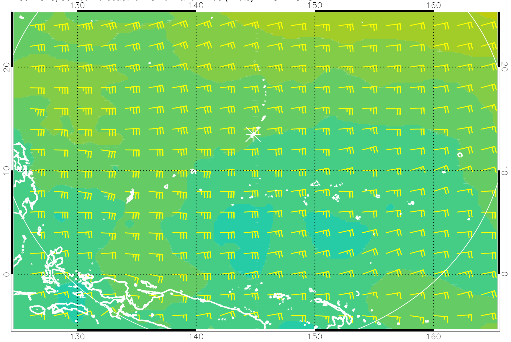
16072918, 30 hour forecast for 70mb T and winds (knots) -- NCEP GFS
