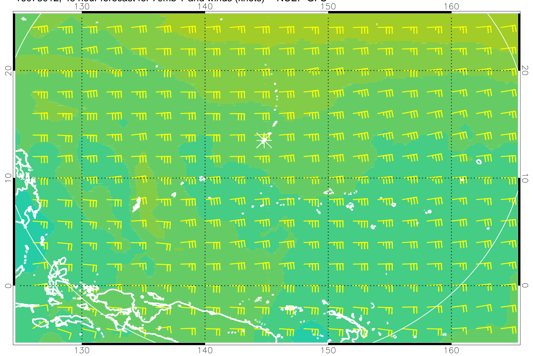
16073012, 48 hour forecast for 70mb T and winds (knots) -- NCEP GFS
