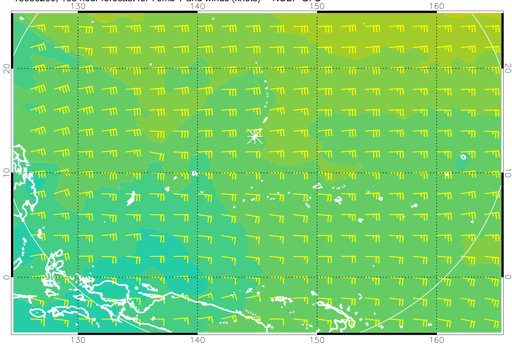
16080200, 108 hour forecast for 70mb T and winds (knots) -- NCEP GFS
