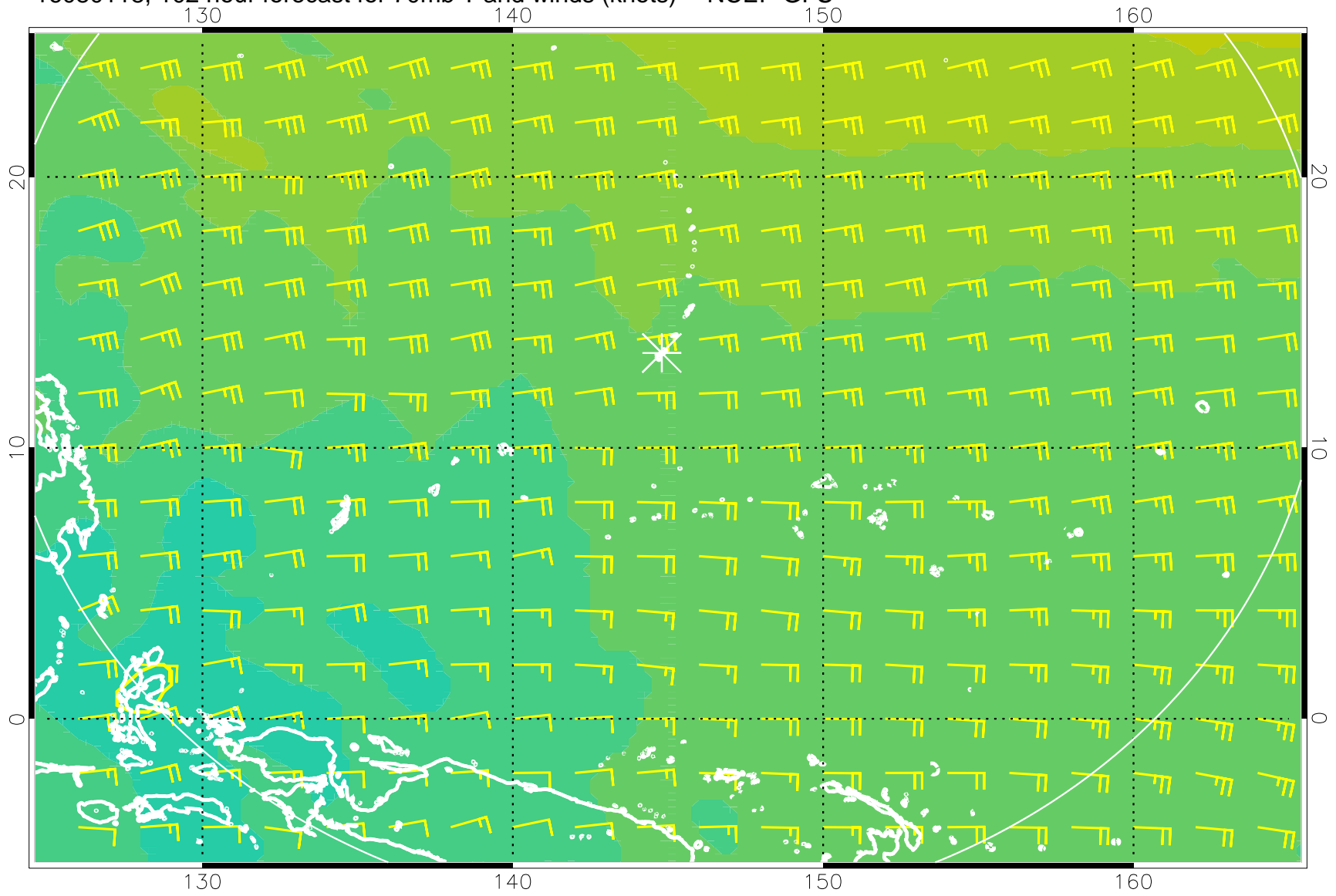
16080118, 102 hour forecast for 70mb T and winds (knots) -- NCEP GFS
