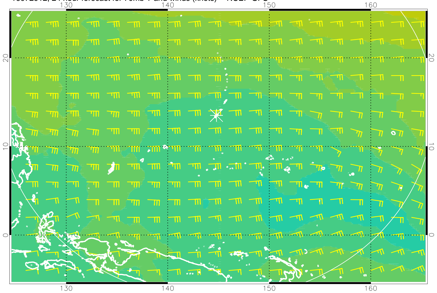
16072912, 24 hour forecast for 70mb T and winds (knots) -- NCEP GFS
