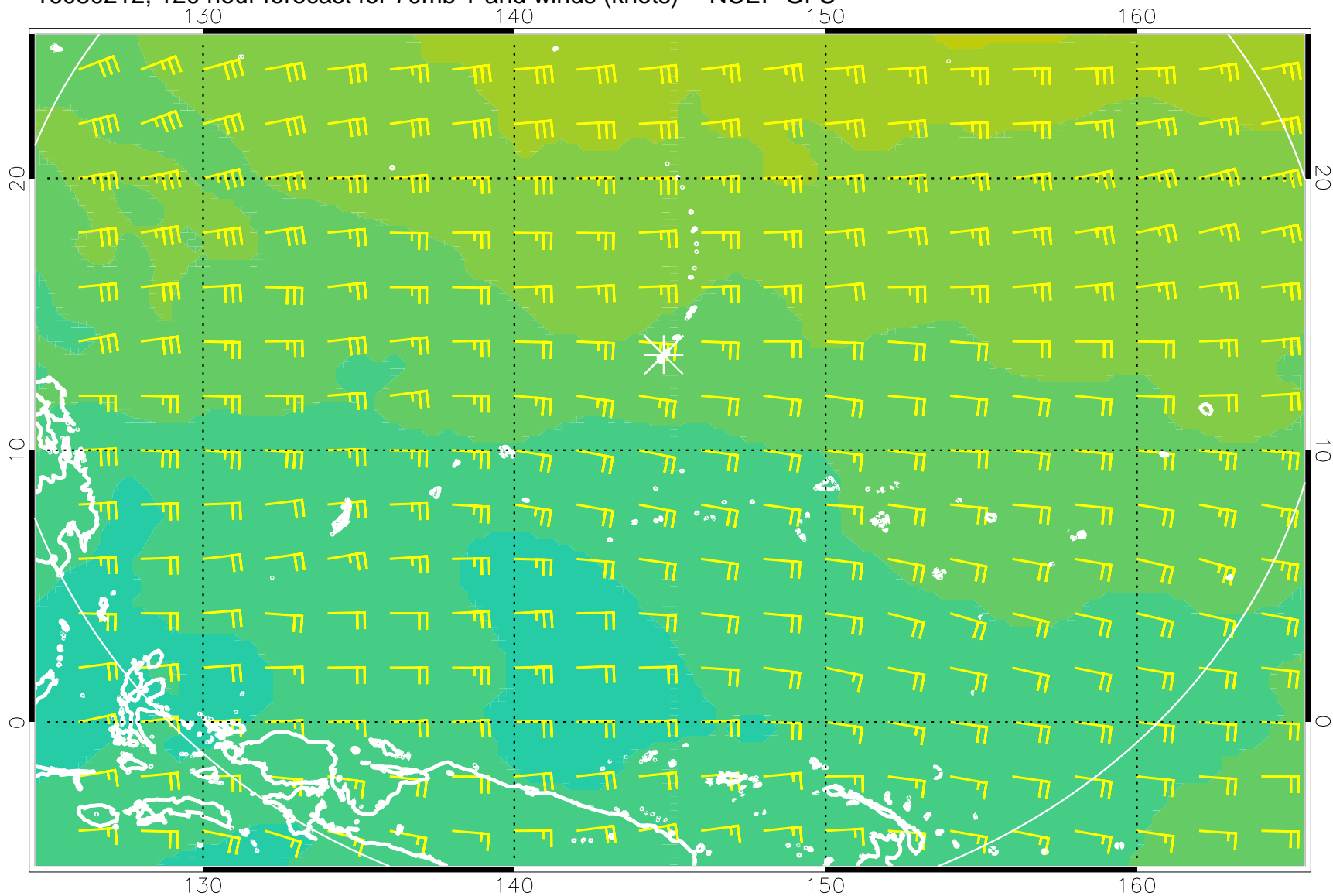
16080212, 120 hour forecast for 70mb T and winds (knots) -- NCEP GFS
