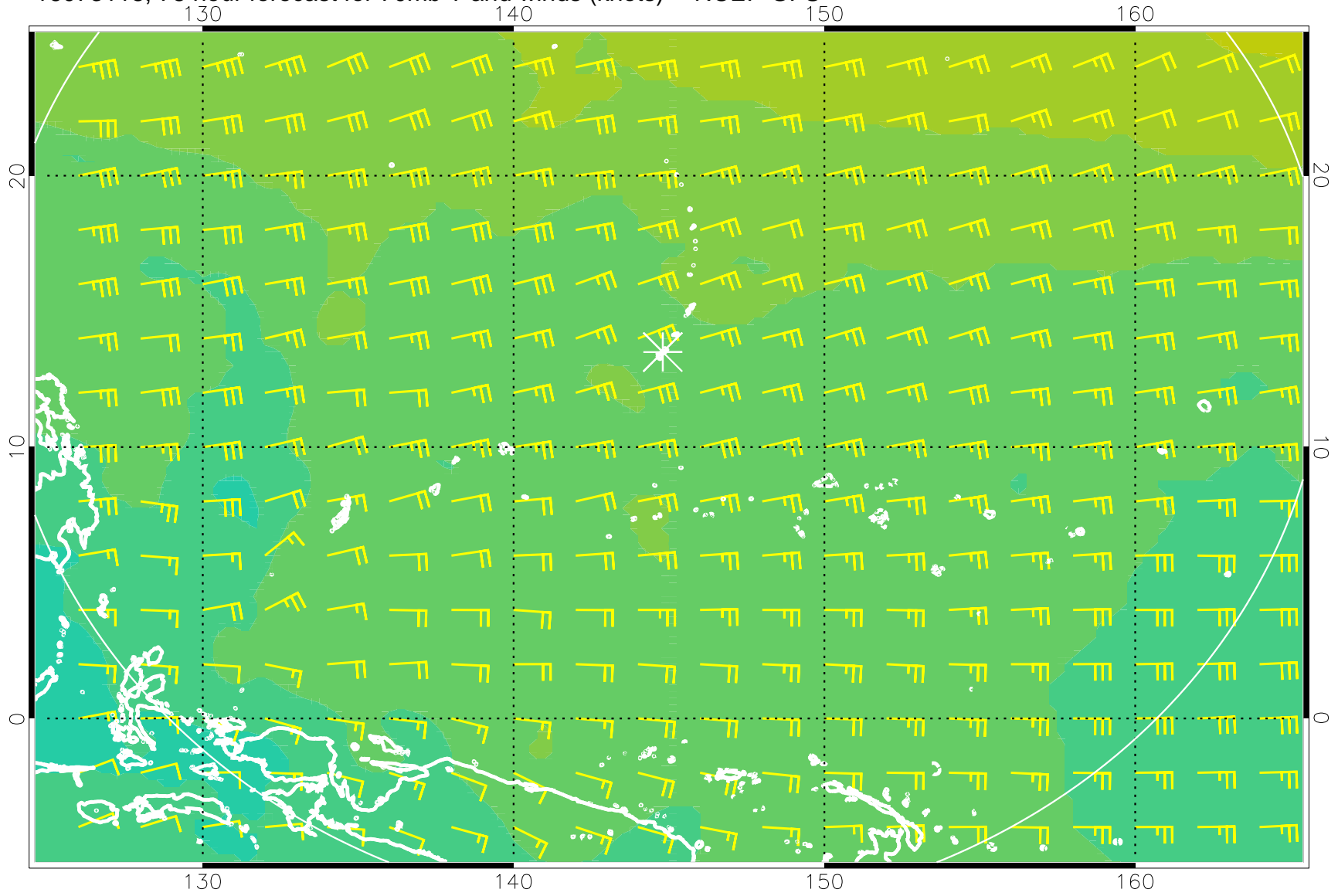
16073118, 78 hour forecast for 70mb T and winds (knots) -- NCEP GFS
