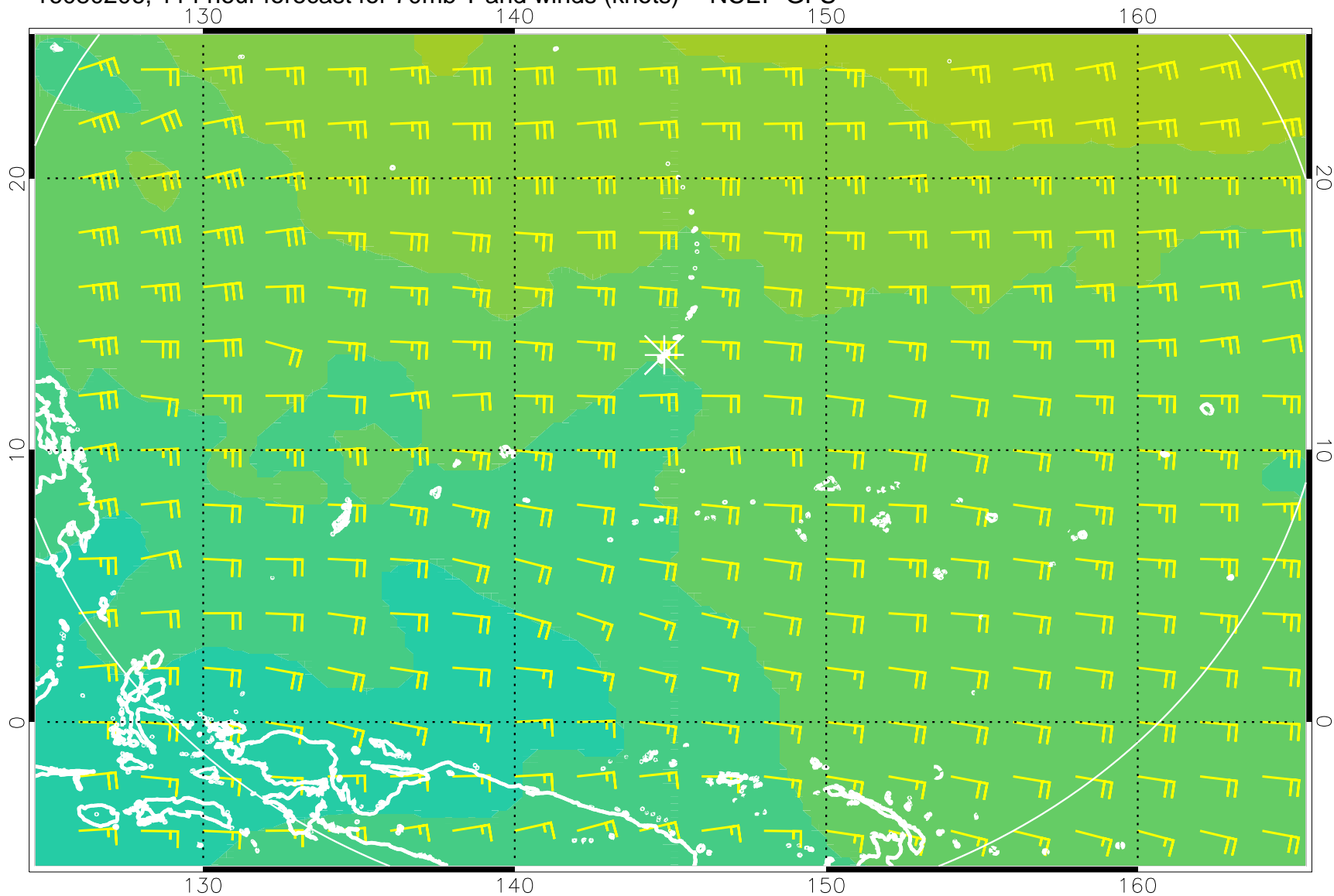
16080206, 114 hour forecast for 70mb T and winds (knots) -- NCEP GFS
