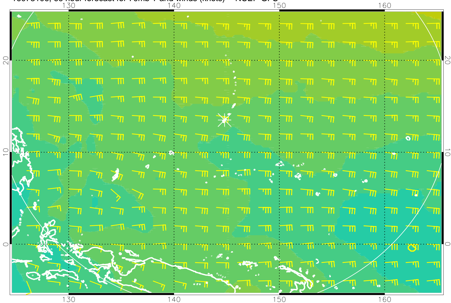
16073106, 66 hour forecast for 70mb T and winds (knots) -- NCEP GFS
