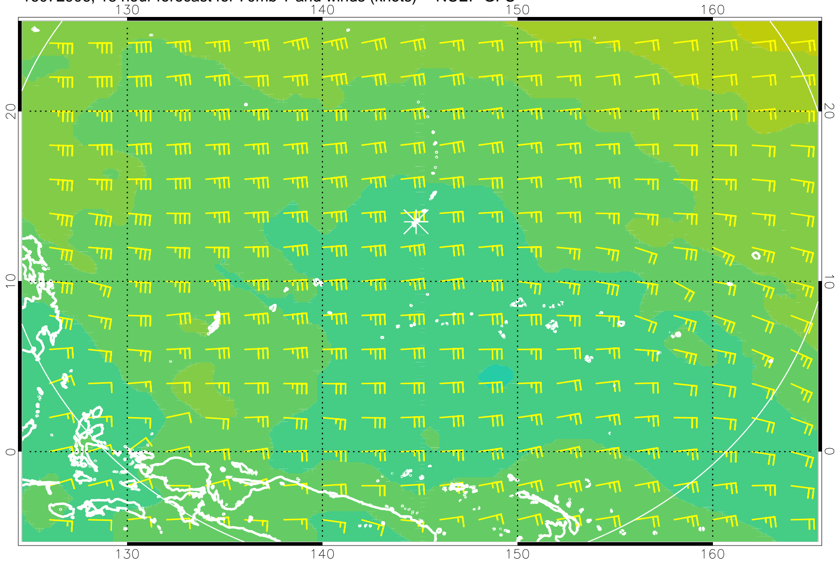
16072906, 18 hour forecast for 70mb T and winds (knots) -- NCEP GFS
