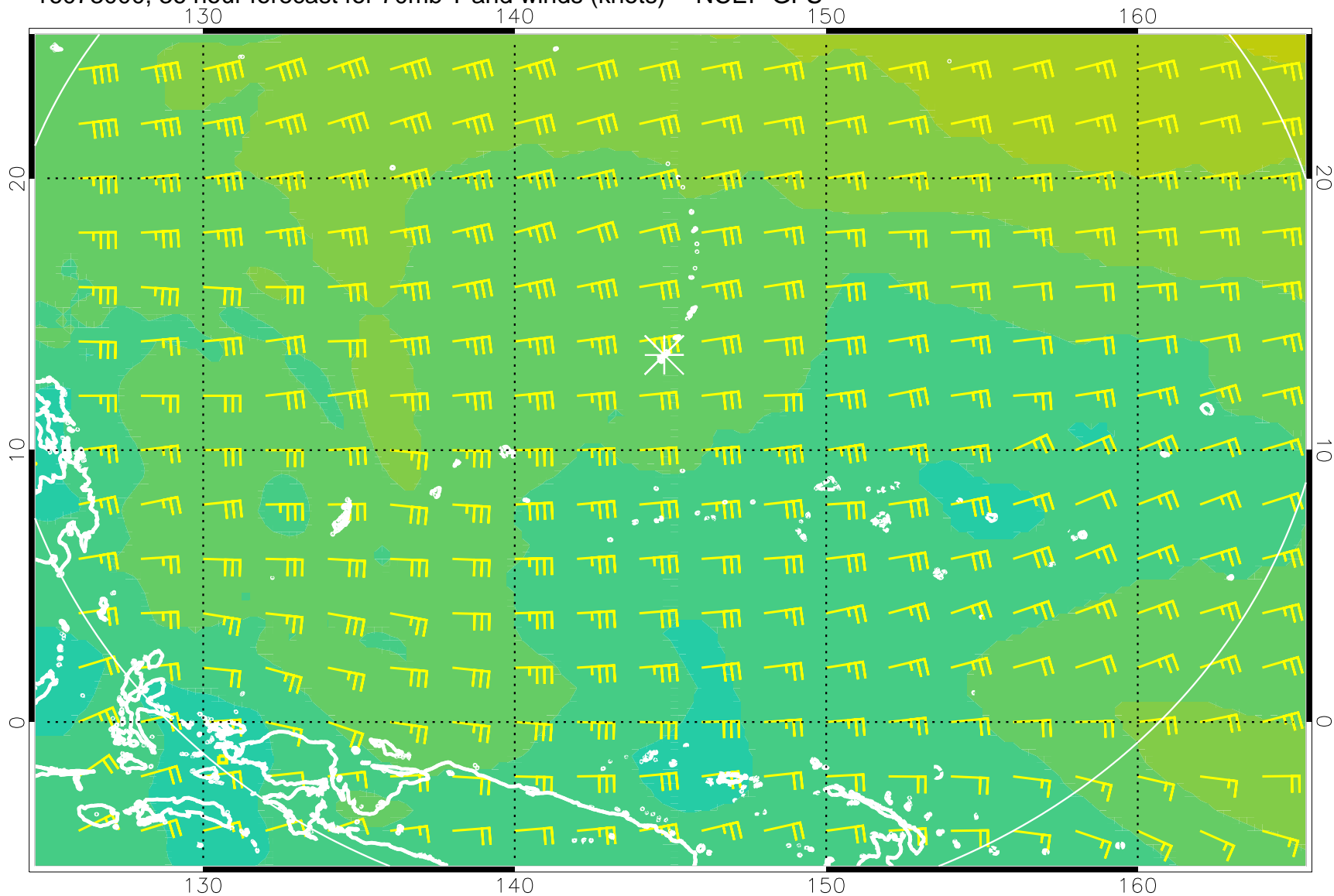
16073000, 36 hour forecast for 70mb T and winds (knots) -- NCEP GFS
