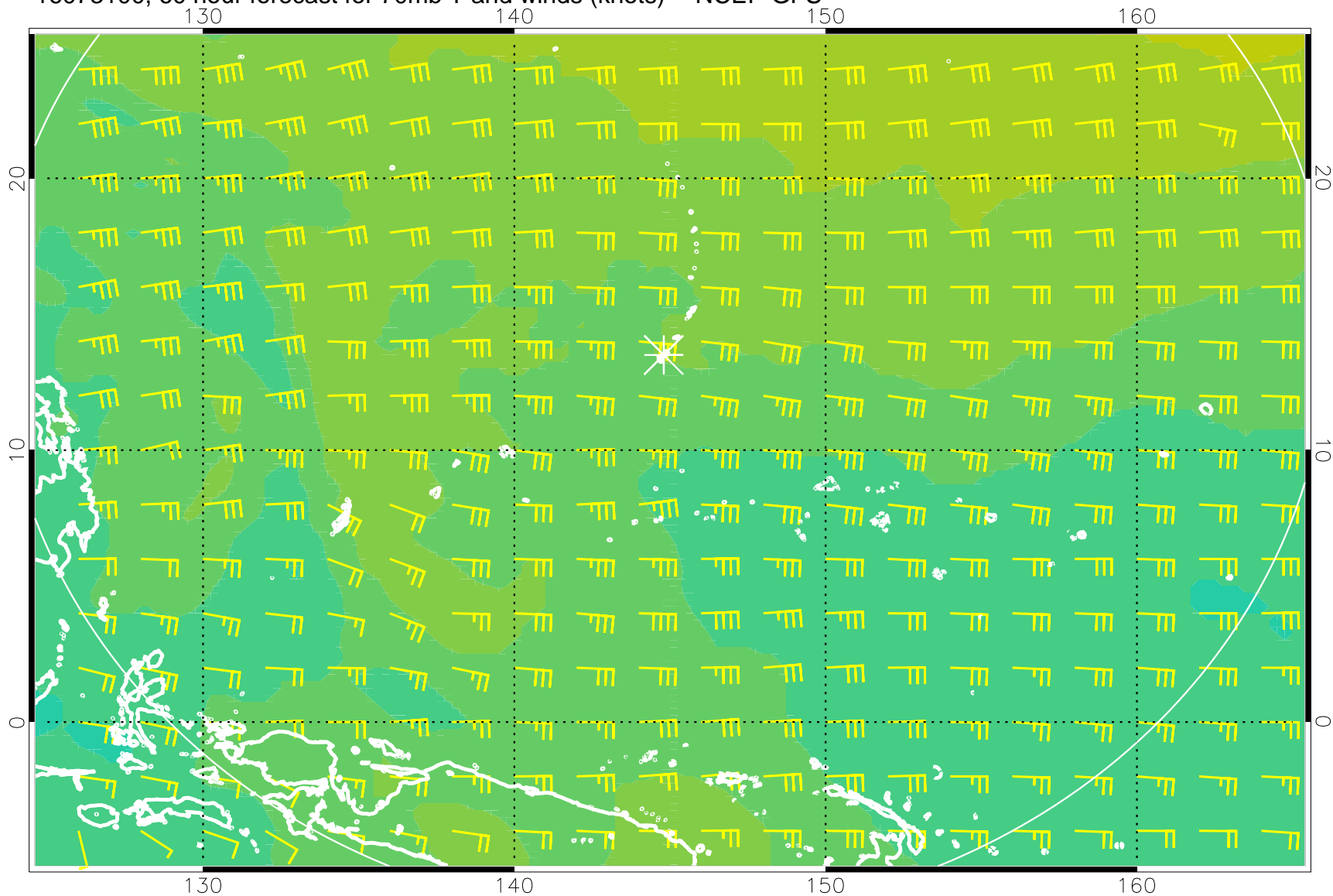
16073100, 60 hour forecast for 70mb T and winds (knots) -- NCEP GFS
