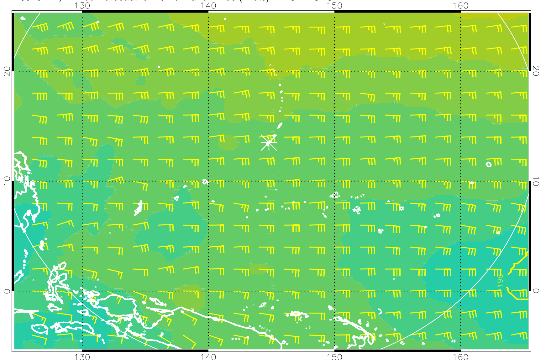
16073112, 72 hour forecast for 70mb T and winds (knots) -- NCEP GFS
