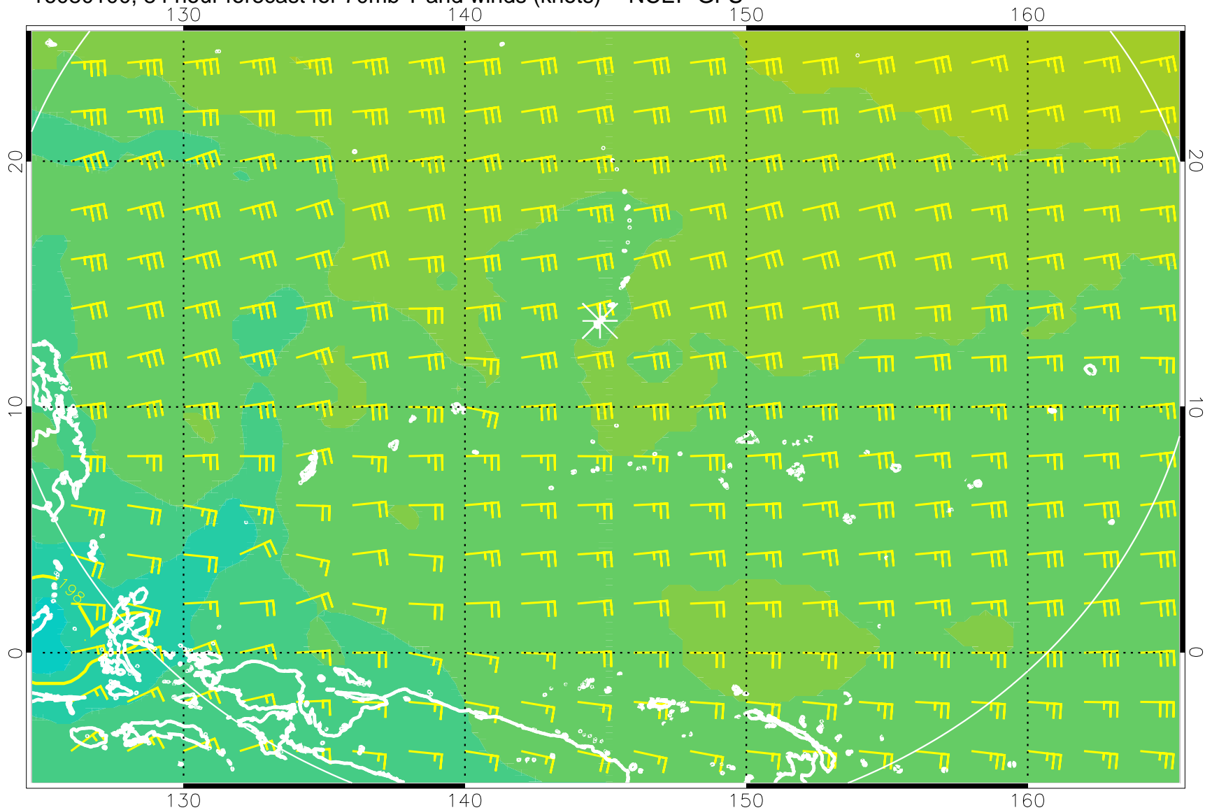
16080100, 84 hour forecast for 70mb T and winds (knots) -- NCEP GFS
