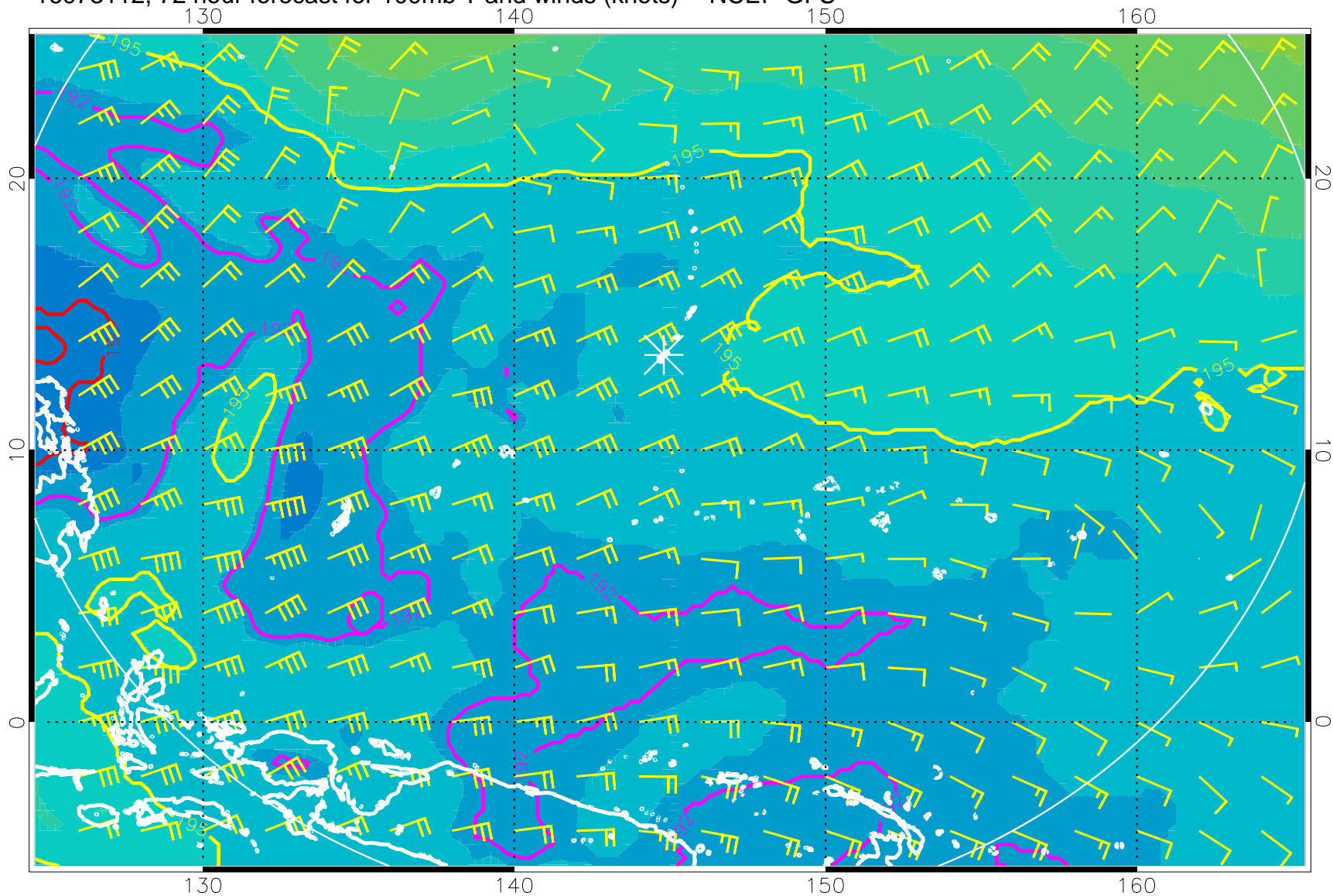
16073112, 72 hour forecast for 100mb T and winds (knots) -- NCEP GFS
