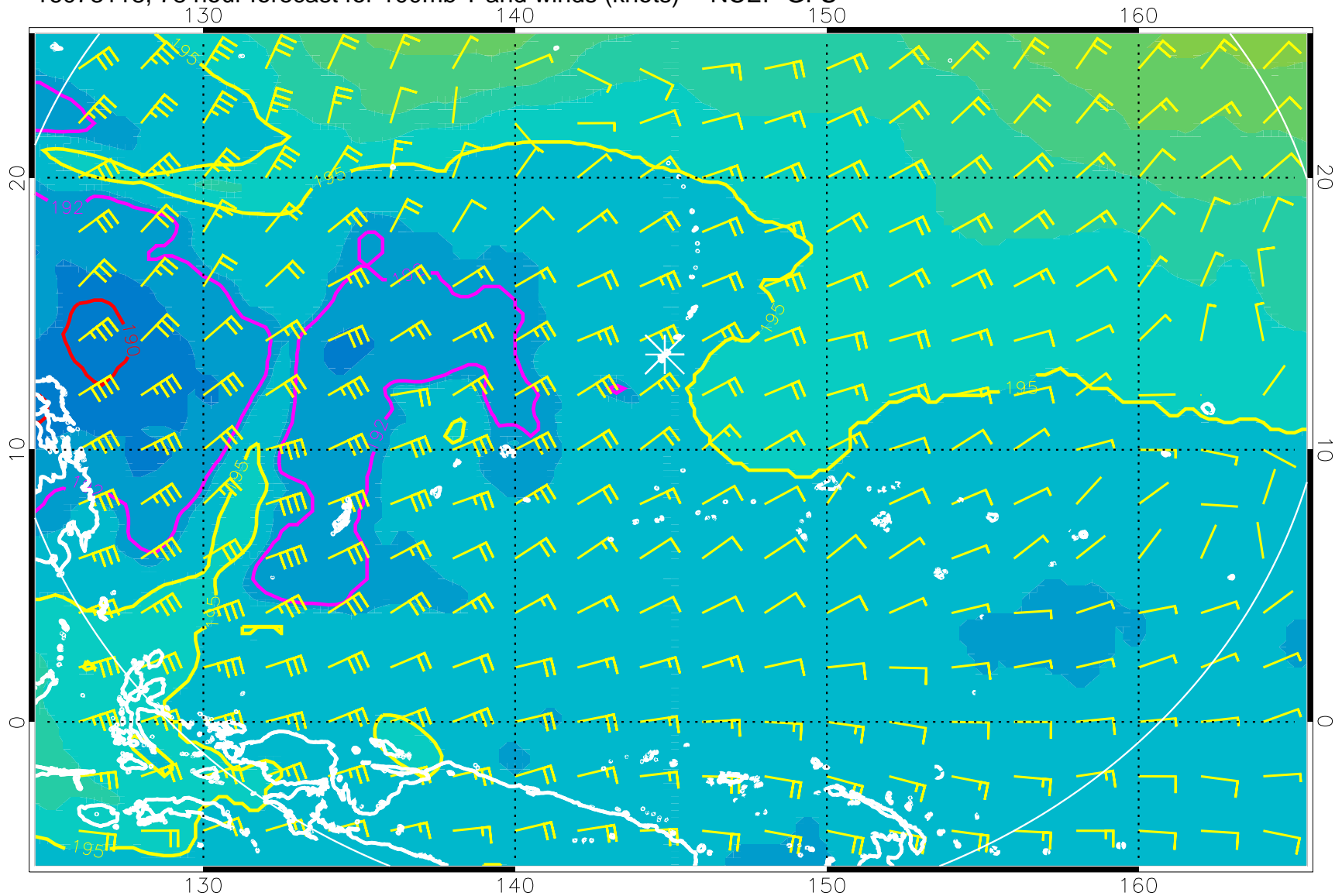
16073118, 78 hour forecast for 100mb T and winds (knots) -- NCEP GFS
