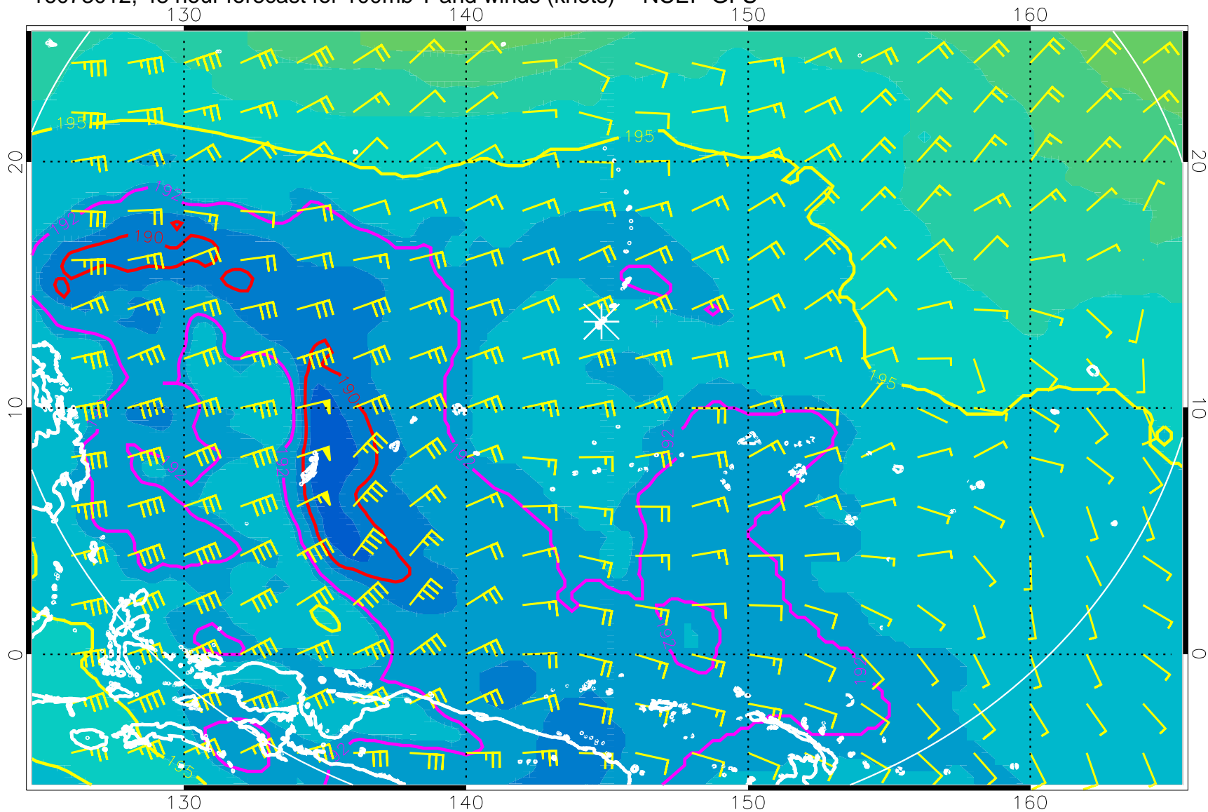
16073012, 48 hour forecast for 100mb T and winds (knots) -- NCEP GFS
