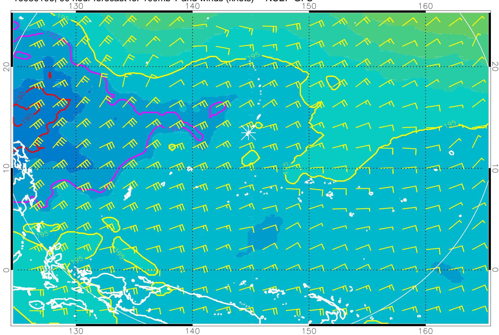
16080106, 90 hour forecast for 100mb T and winds (knots) -- NCEP GFS
