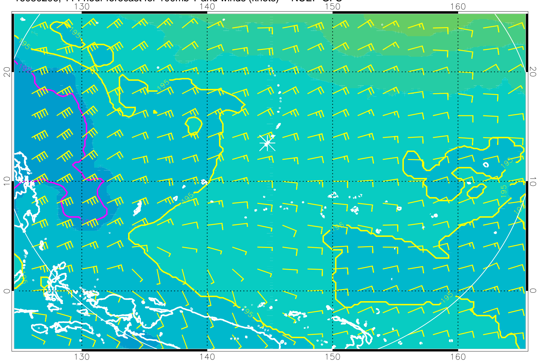
16080206, 114 hour forecast for 100mb T and winds (knots) -- NCEP GFS
