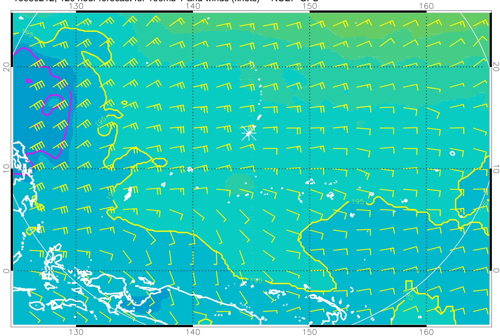
16080212, 120 hour forecast for 100mb T and winds (knots) -- NCEP GFS
