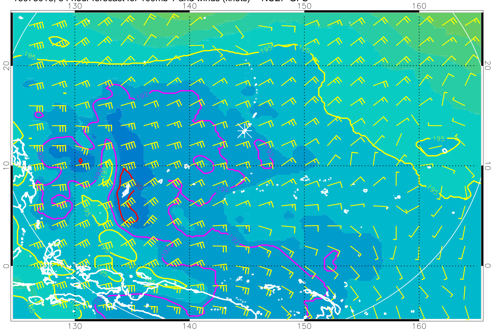
16073018, 54 hour forecast for 100mb T and winds (knots) -- NCEP GFS
