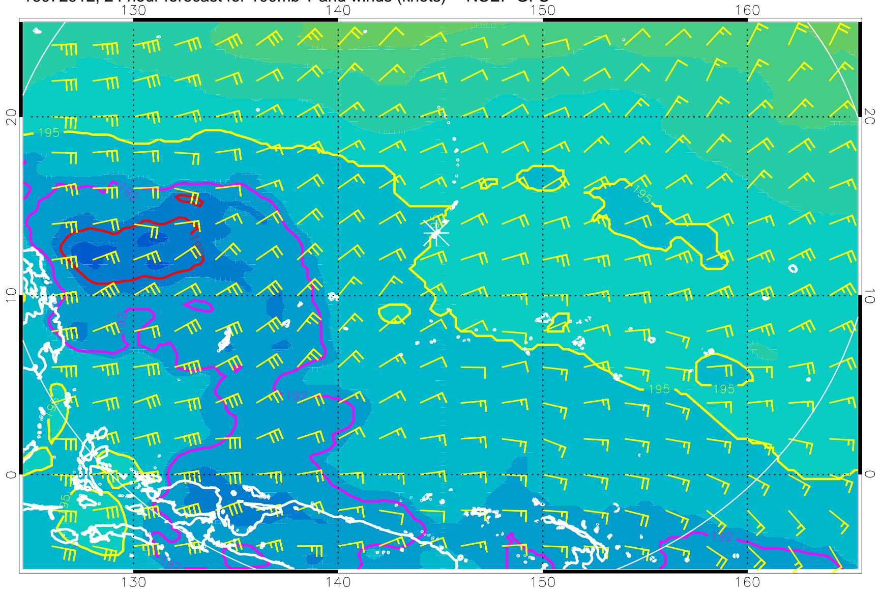
16072912, 24 hour forecast for 100mb T and winds (knots) -- NCEP GFS
