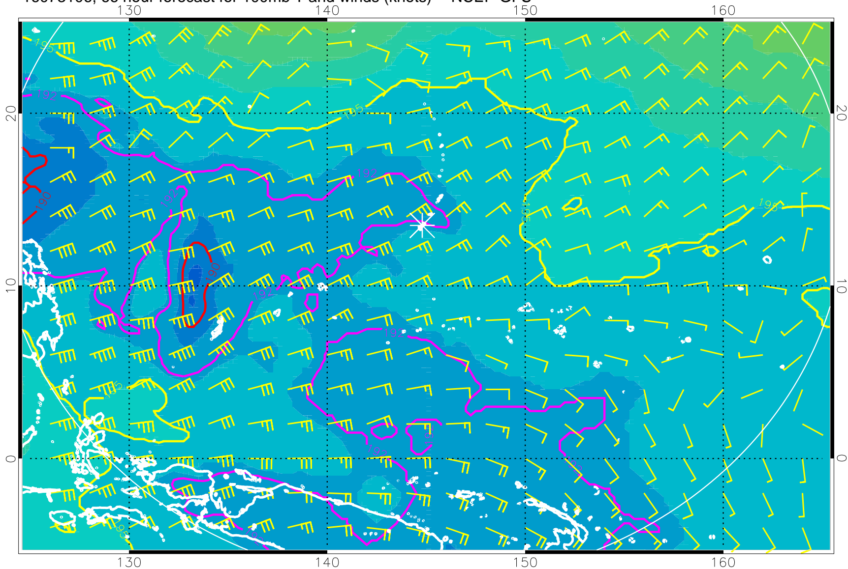
16073106, 66 hour forecast for 100mb T and winds (knots) -- NCEP GFS
