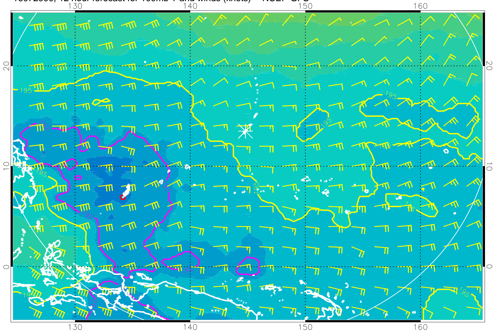
16072900, 12 hour forecast for 100mb T and winds (knots) -- NCEP GFS
