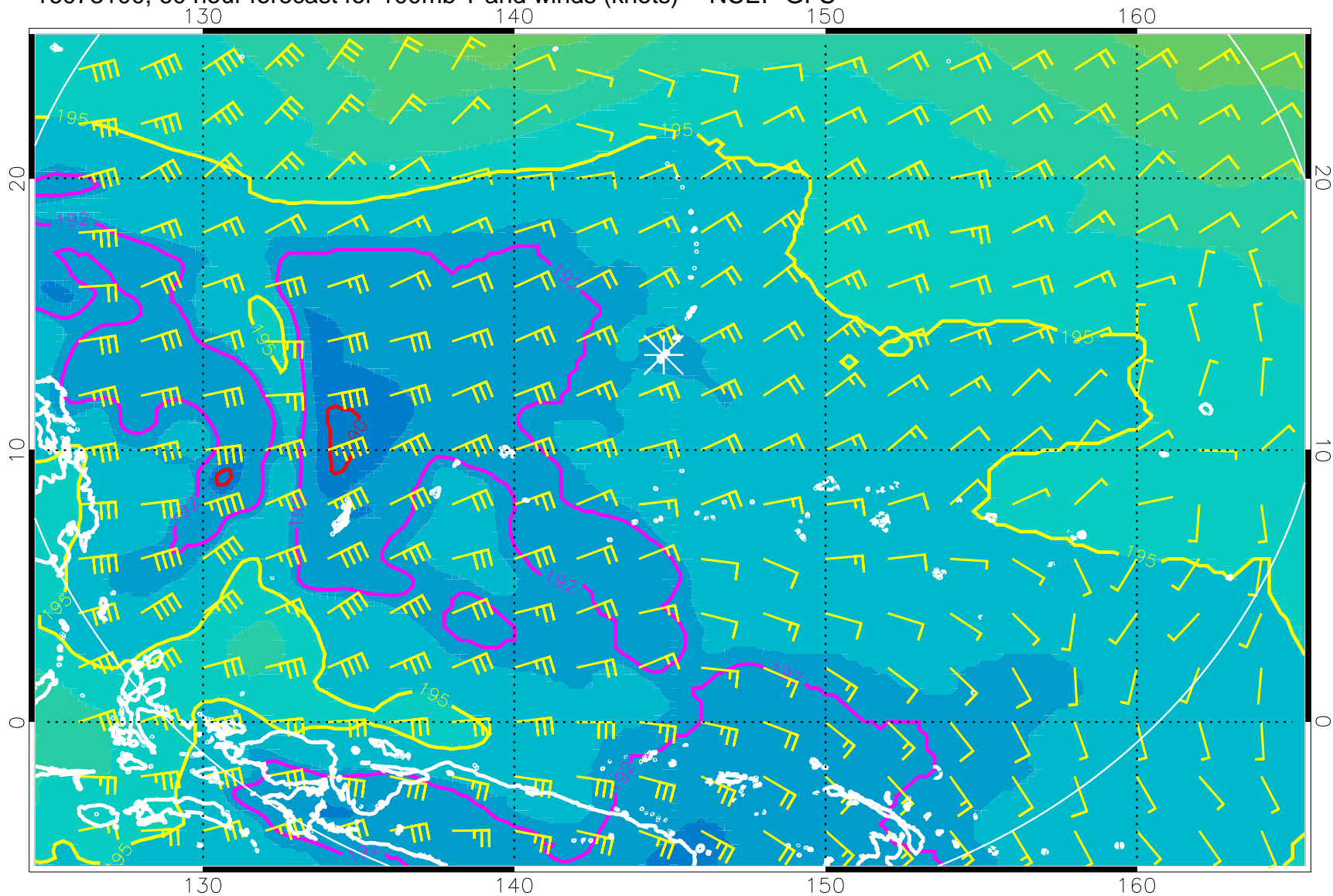
16073100, 60 hour forecast for 100mb T and winds (knots) -- NCEP GFS
