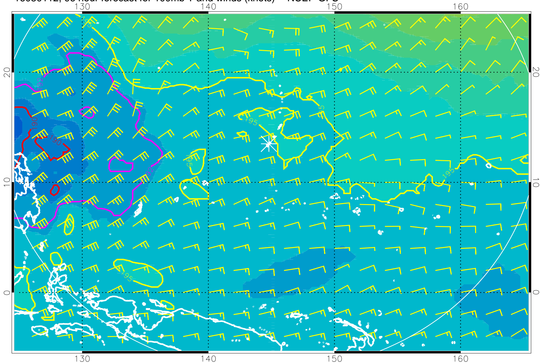
16080112, 96 hour forecast for 100mb T and winds (knots) -- NCEP GFS
