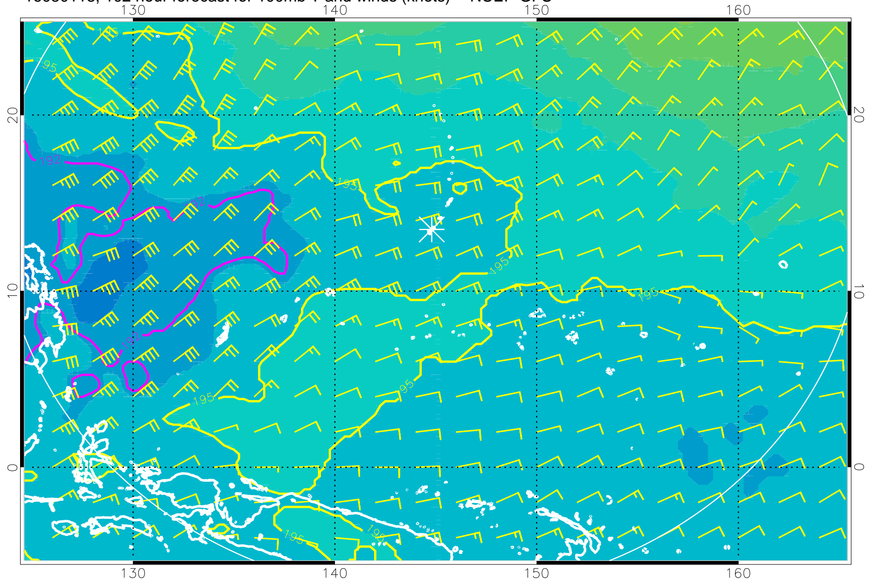
16080118, 102 hour forecast for 100mb T and winds (knots) -- NCEP GFS
