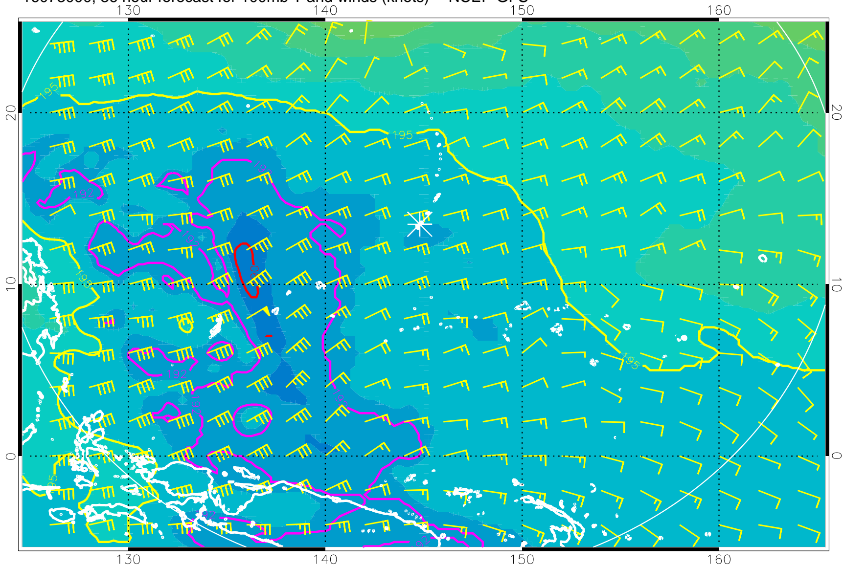
16073000, 36 hour forecast for 100mb T and winds (knots) -- NCEP GFS
