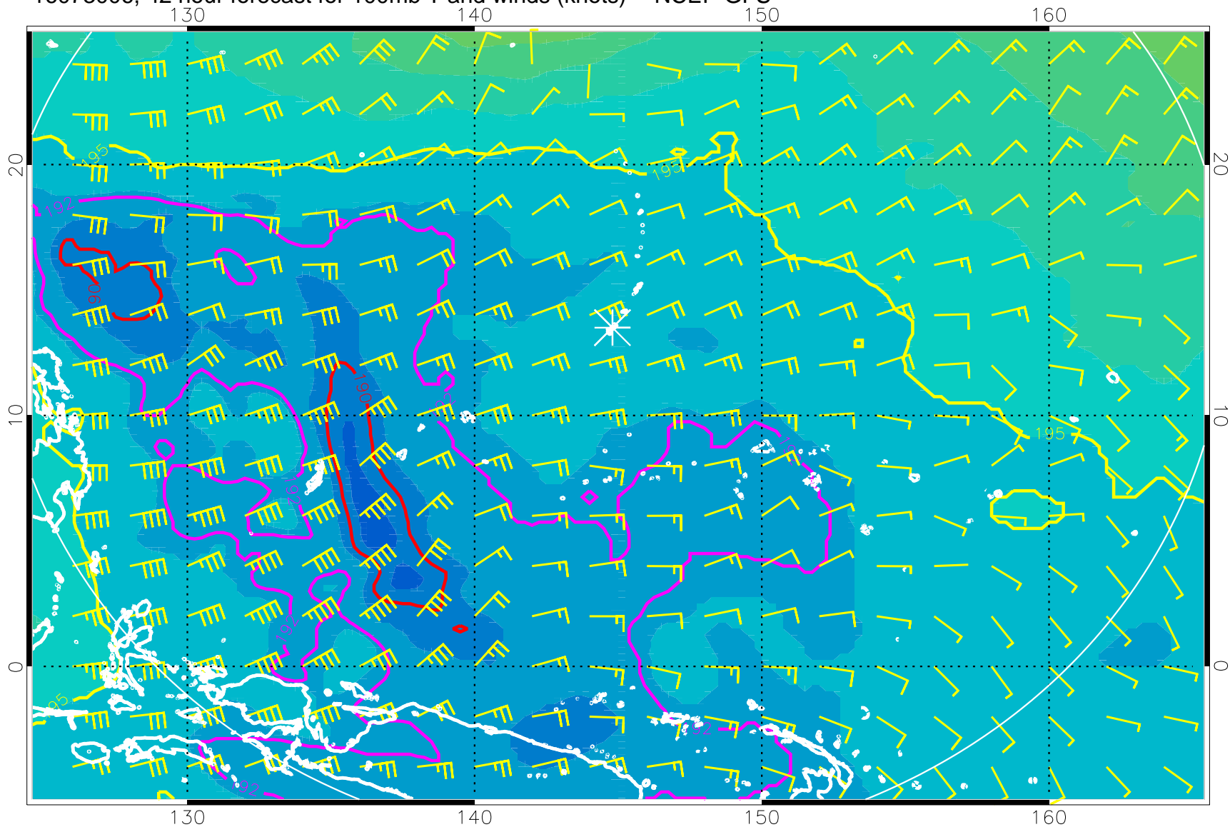
16073006, 42 hour forecast for 100mb T and winds (knots) -- NCEP GFS
