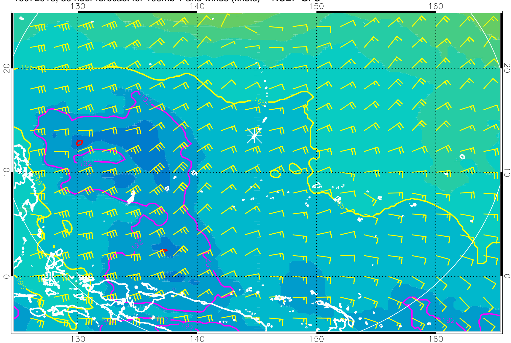
16072918, 30 hour forecast for 100mb T and winds (knots) -- NCEP GFS
