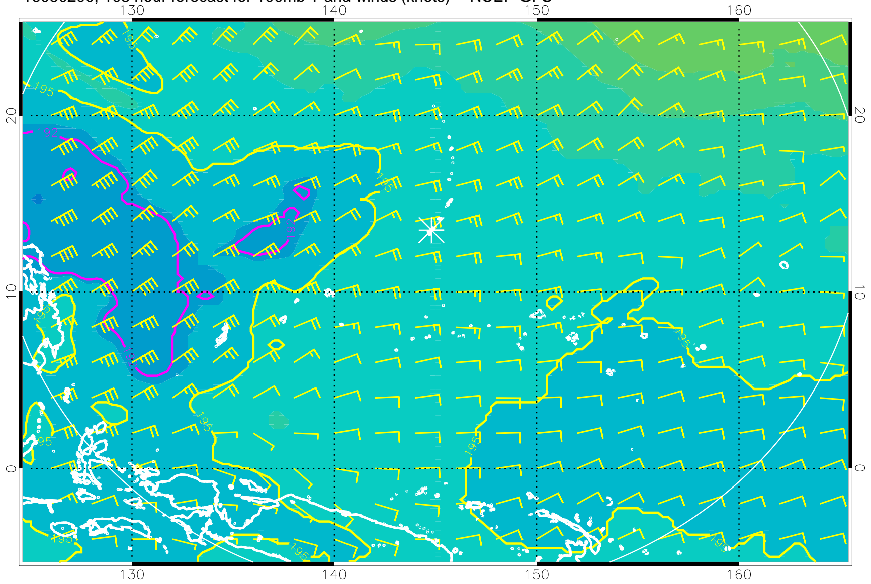
16080200, 108 hour forecast for 100mb T and winds (knots) -- NCEP GFS
