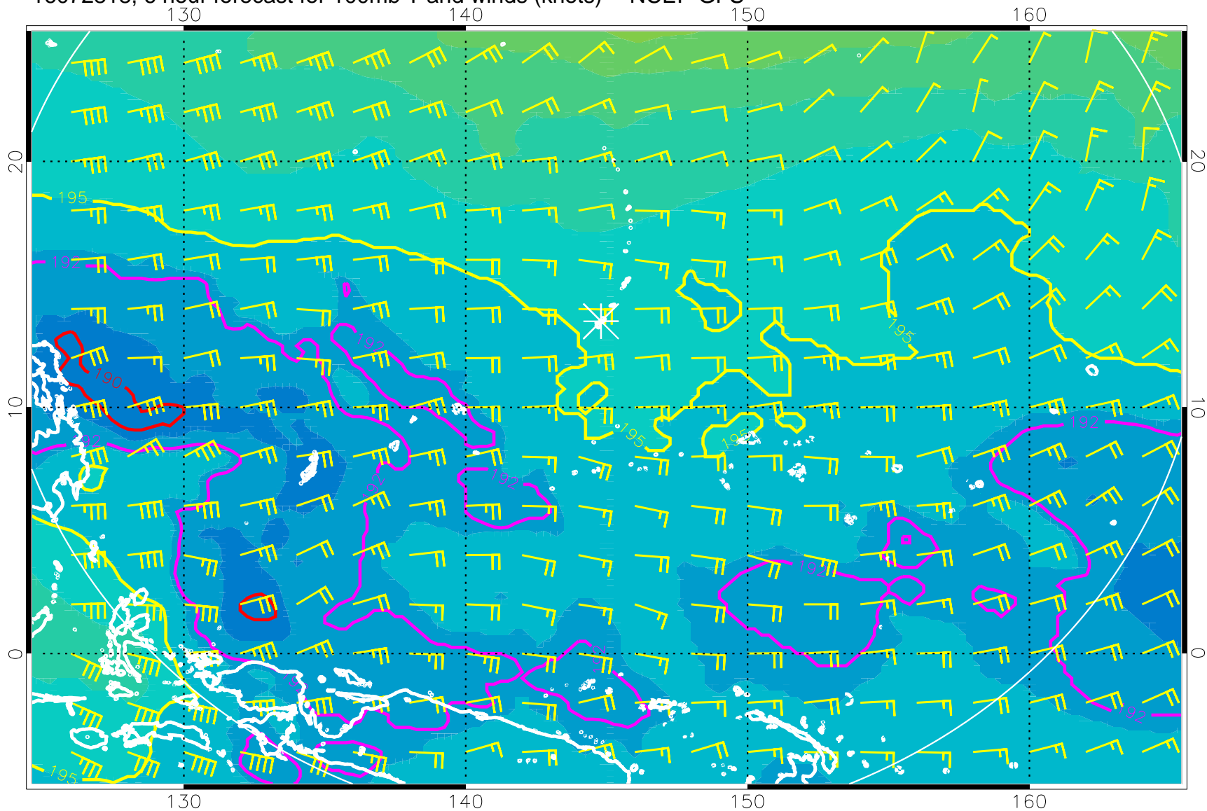
16072818, 6 hour forecast for 100mb T and winds (knots) -- NCEP GFS
