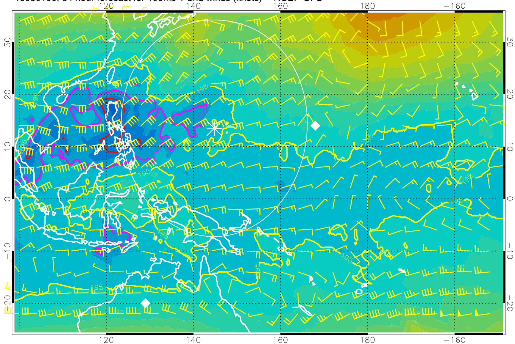
16080100, 84 hour forecast for 100mb T and winds (knots) -- NCEP GFS
