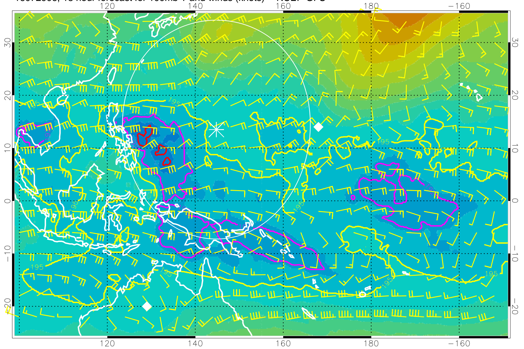
16072906, 18 hour forecast for 100mb T and winds (knots) -- NCEP GFS
