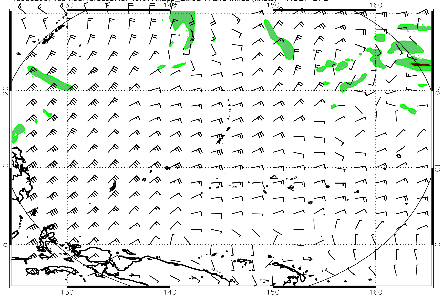
16080200, 108 hour forecast for 49Kft Knapp_Ellrod TI and winds (knots) -- NCEP GFS
