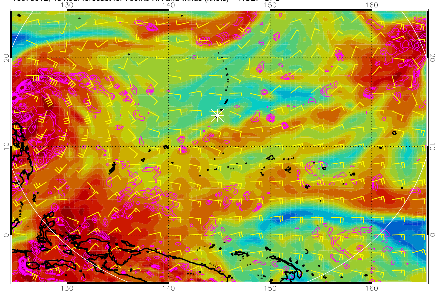
16073012, 48 hour forecast for 700mb RH and winds (knots) -- NCEP GFS
