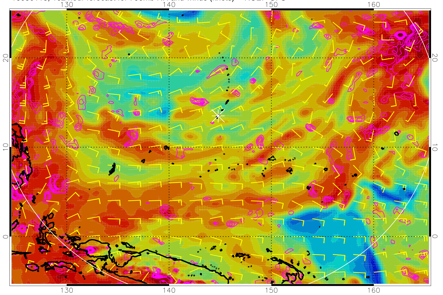
16080118, 102 hour forecast for 700mb RH and winds (knots) -- NCEP GFS
