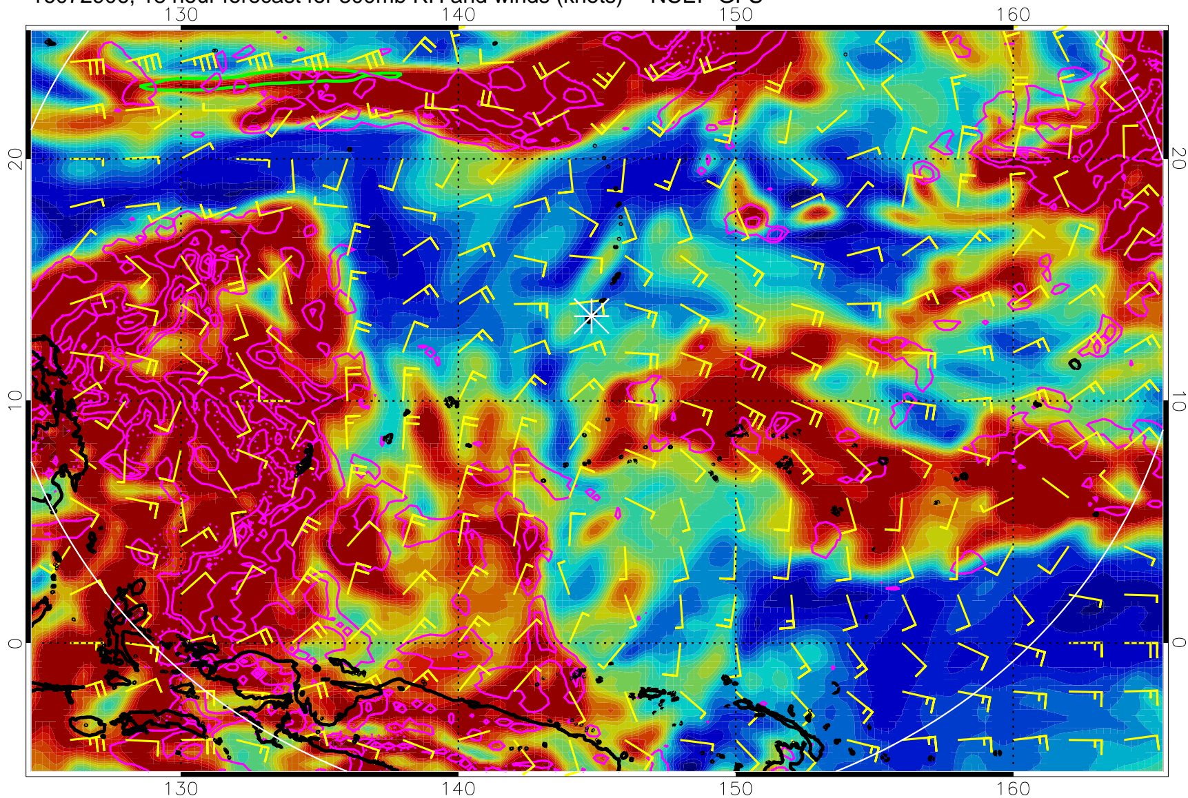
16072906, 18 hour forecast for 300mb RH and winds (knots) -- NCEP GFS
