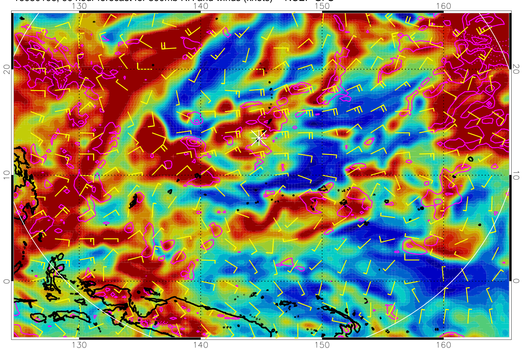
16080106, 90 hour forecast for 300mb RH and winds (knots) -- NCEP GFS
