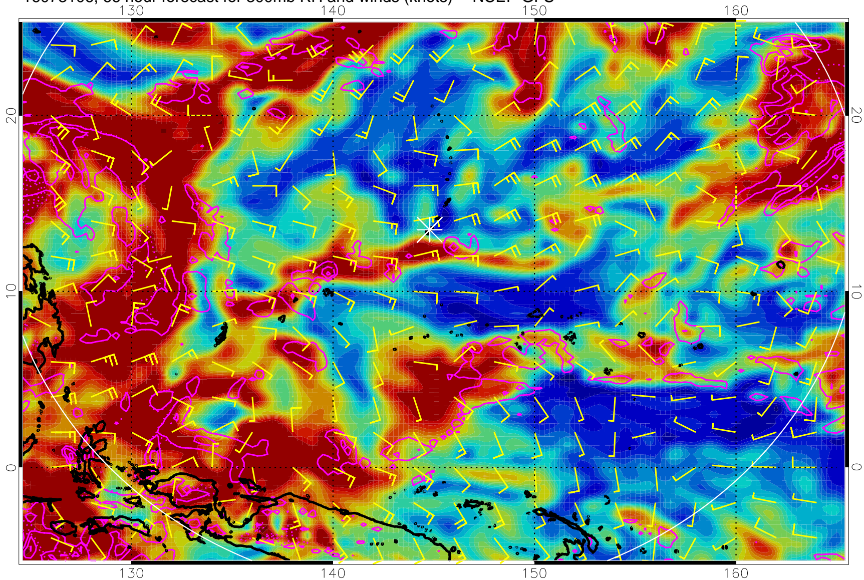
16073106, 66 hour forecast for 300mb RH and winds (knots) -- NCEP GFS
