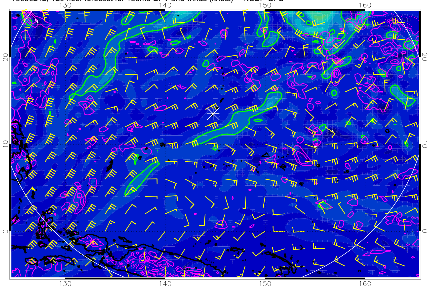
16080212, 120 hour forecast for 150mb EPV and winds (knots) -- NCEP GFS
