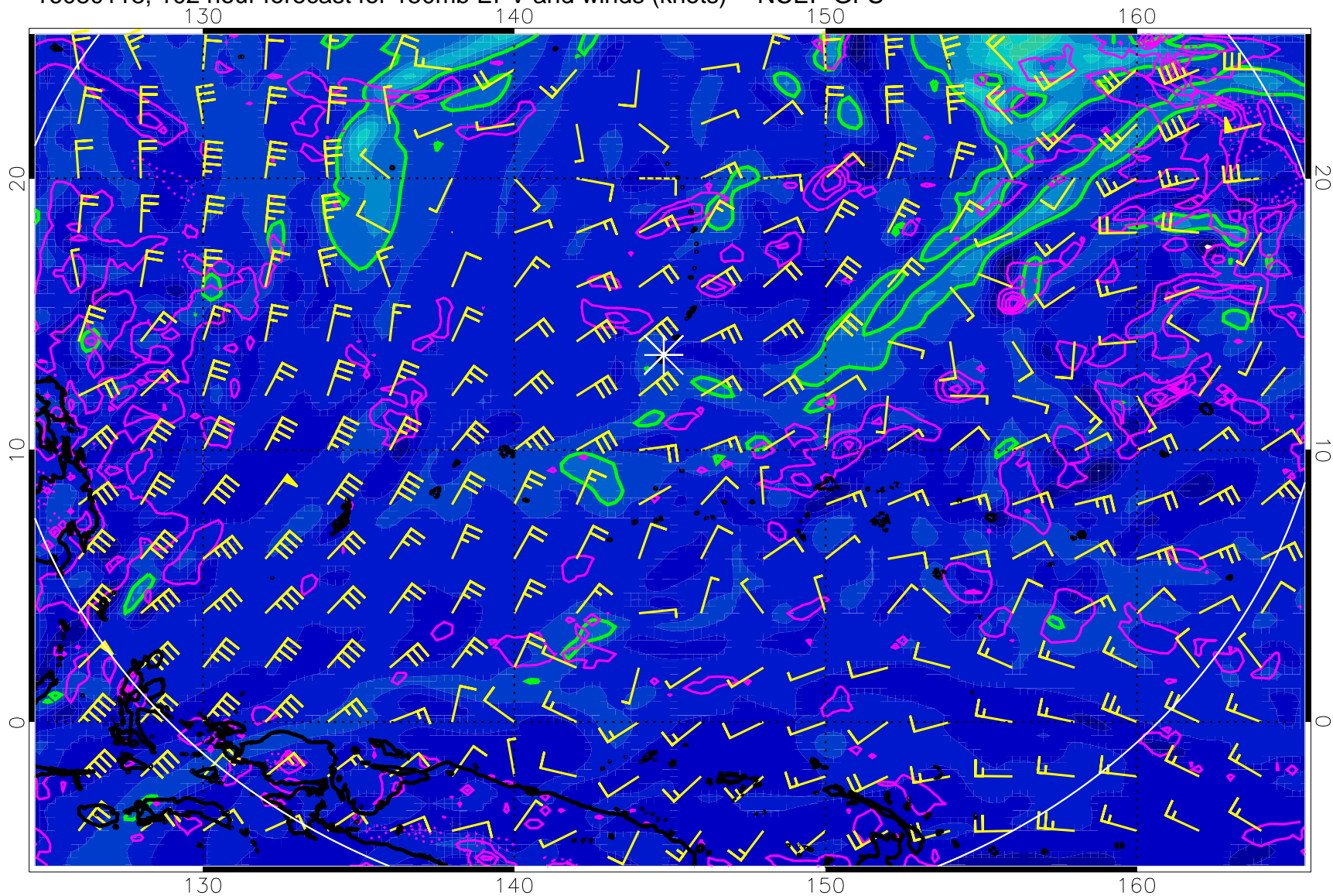
16080118, 102 hour forecast for 150mb EPV and winds (knots) -- NCEP GFS
