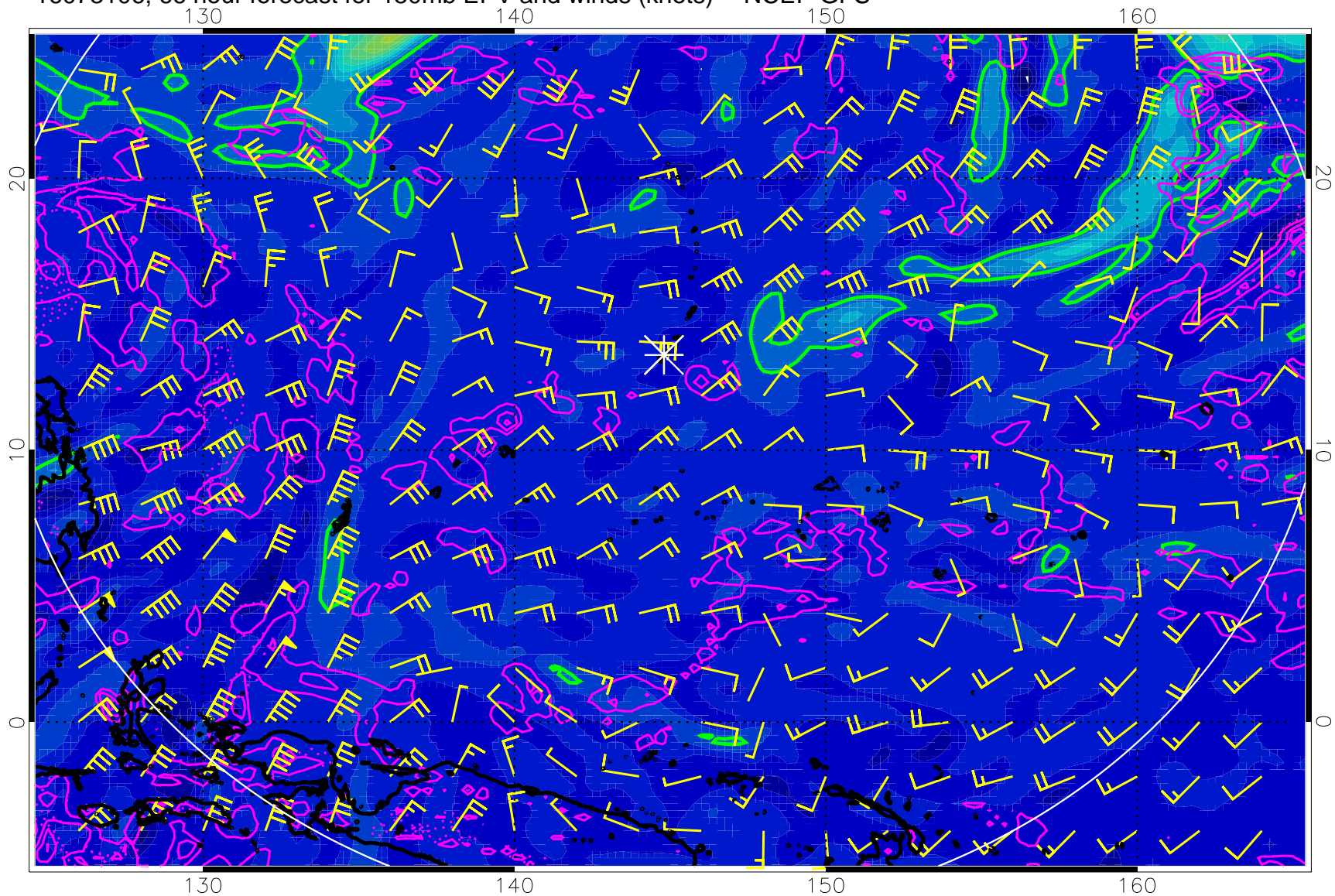
16073106, 66 hour forecast for 150mb EPV and winds (knots) -- NCEP GFS
