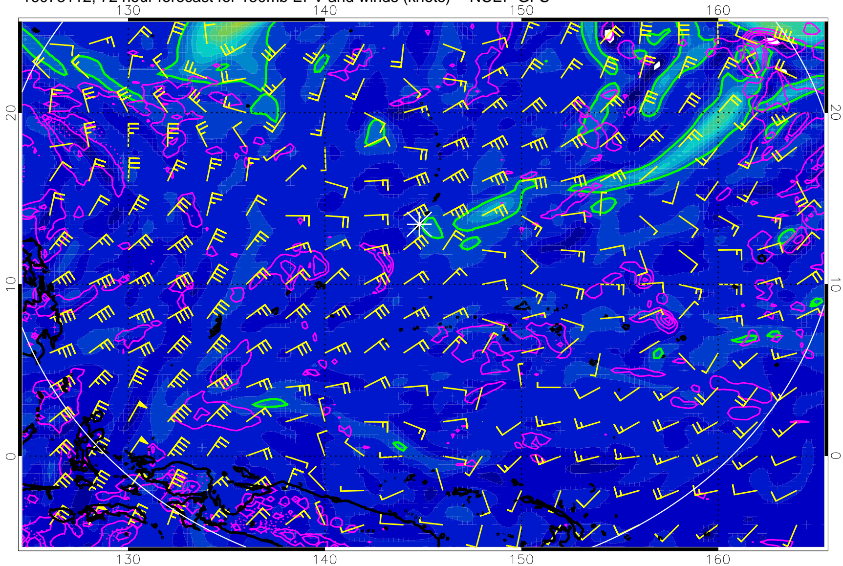
16073112, 72 hour forecast for 150mb EPV and winds (knots) -- NCEP GFS
