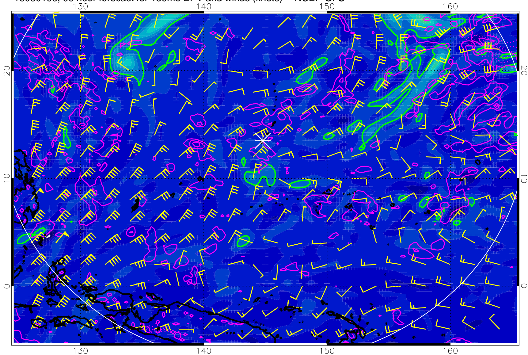
16080106, 90 hour forecast for 150mb EPV and winds (knots) -- NCEP GFS
