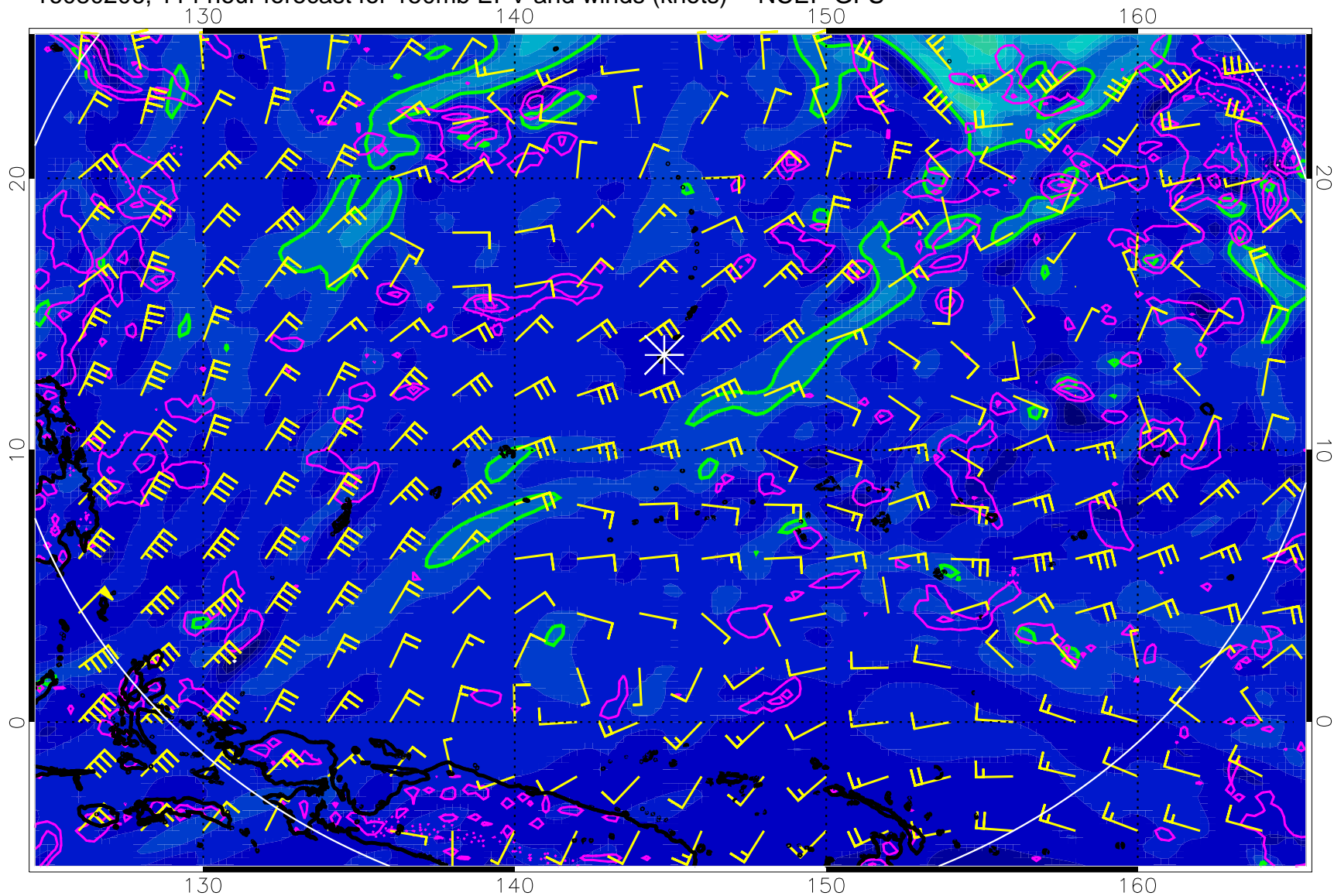
16080206, 114 hour forecast for 150mb EPV and winds (knots) -- NCEP GFS
