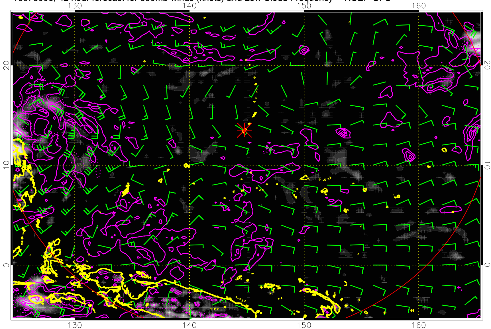
16073006, 42 hour forecast for 850mb winds (knots) and Low Cloud Frequency -- NCEP GFS
