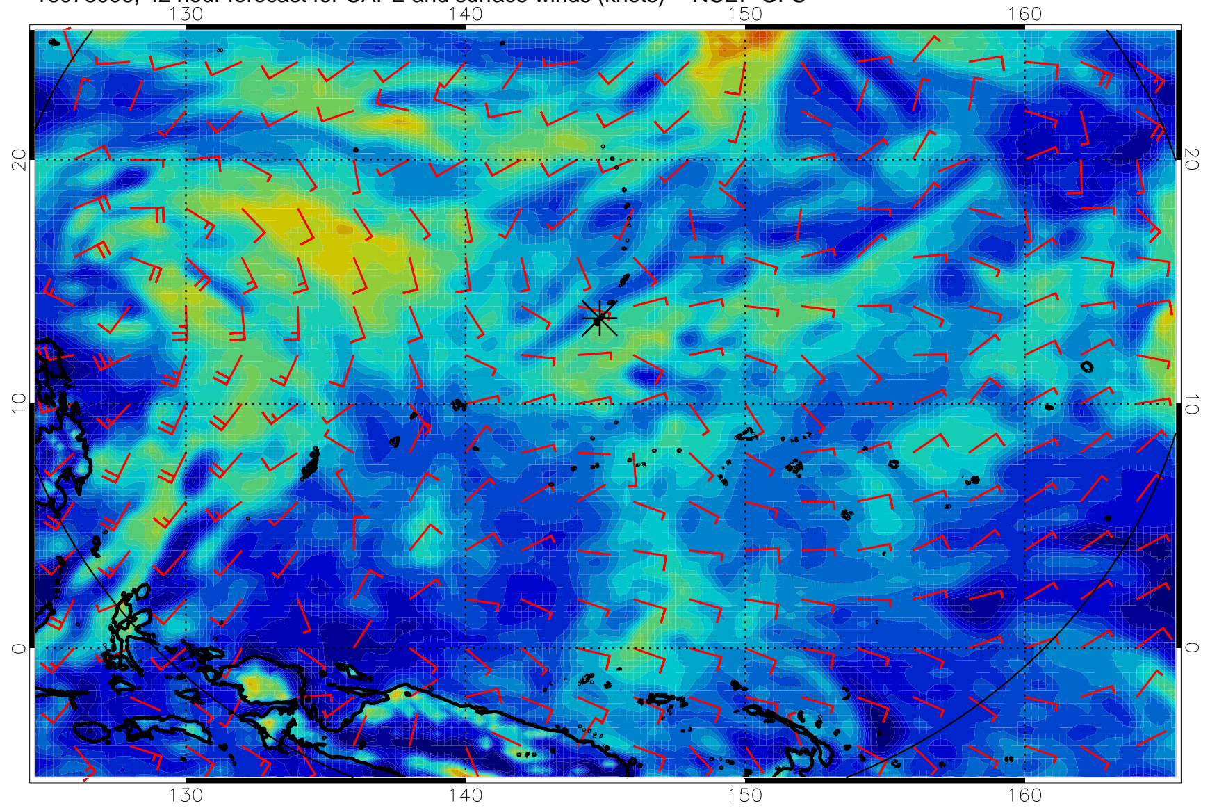
16073006, 42 hour forecast for CAPE and surface winds (knots) -- NCEP GFS
