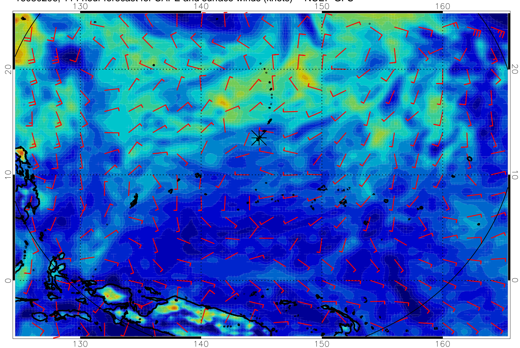
16080206, 114 hour forecast for CAPE and surface winds (knots) -- NCEP GFS
