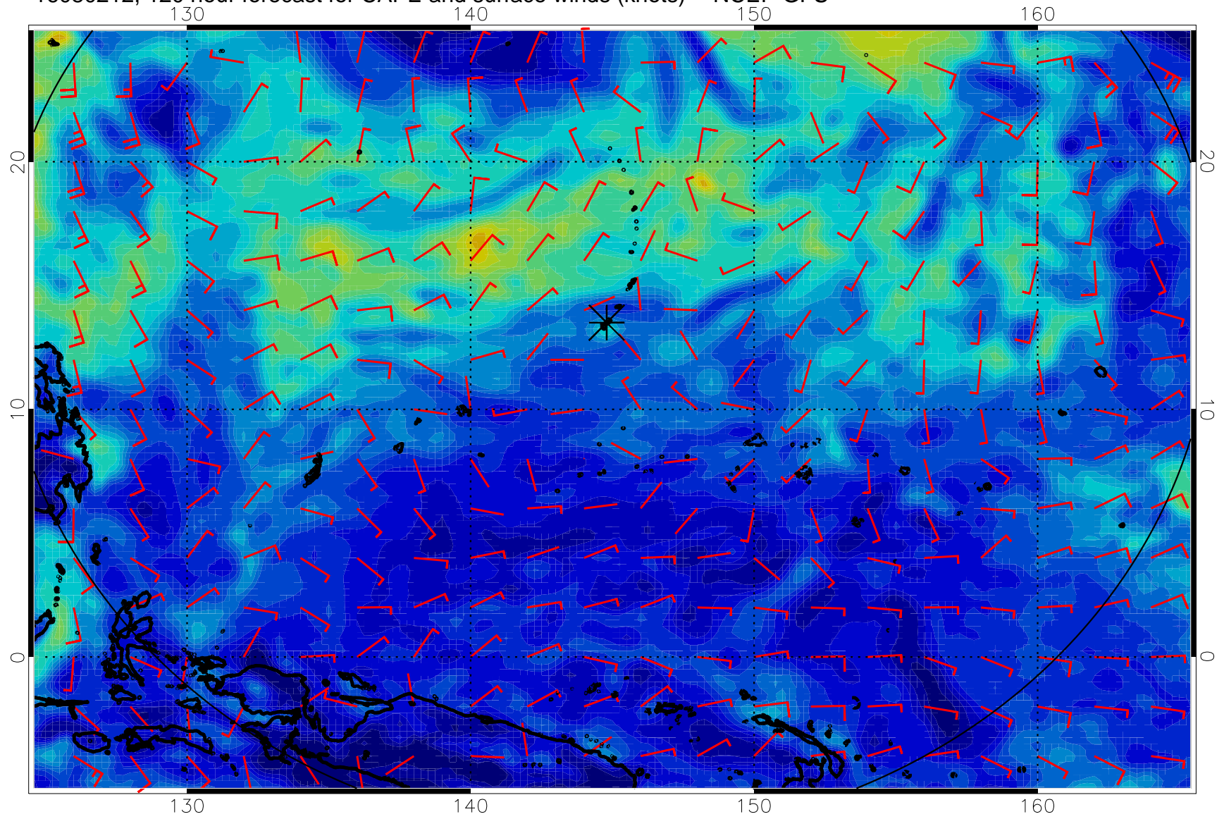
16080212, 120 hour forecast for CAPE and surface winds (knots) -- NCEP GFS
