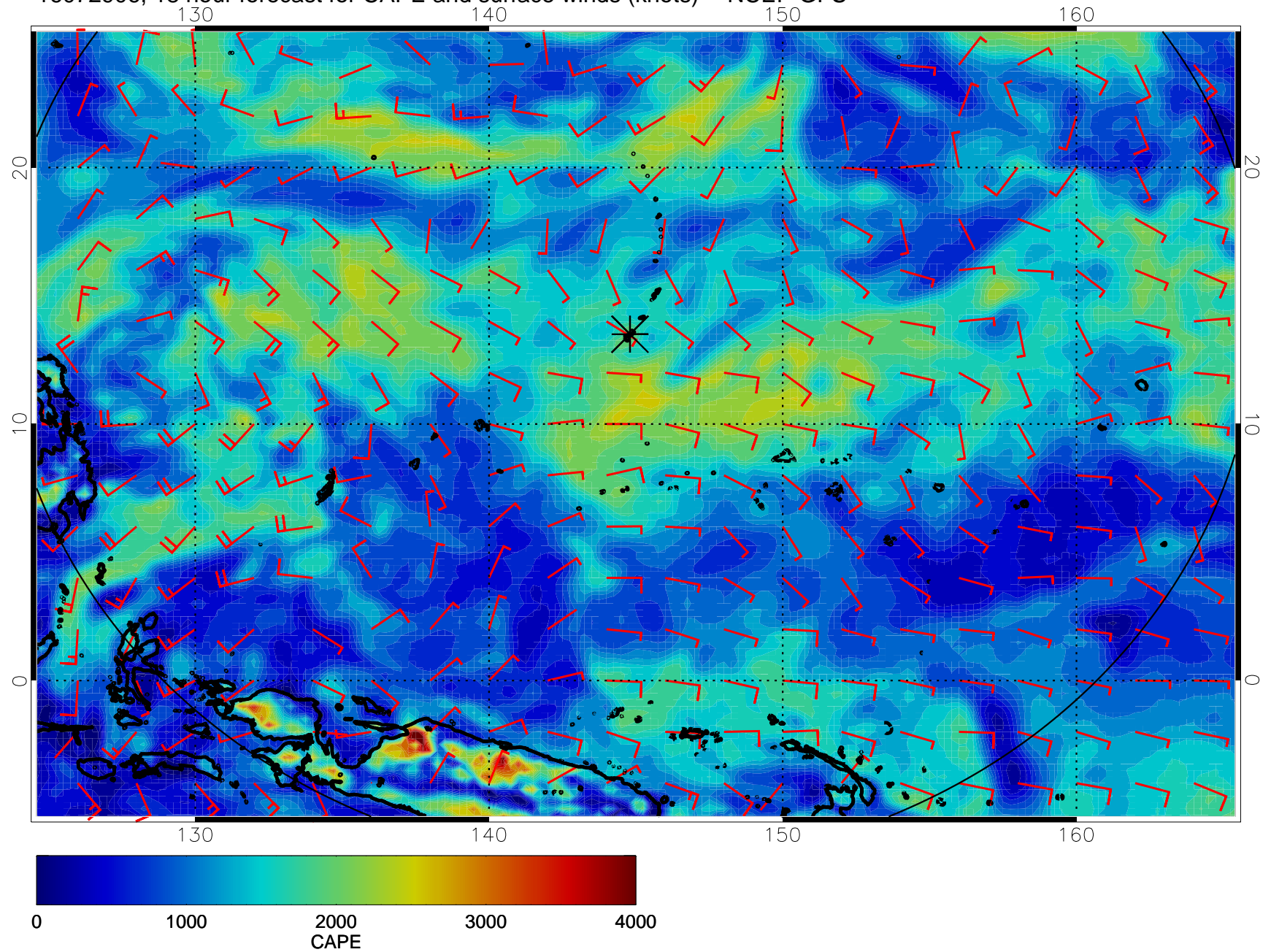
16072906, 18 hour forecast for CAPE and surface winds (knots) -- NCEP GFS
