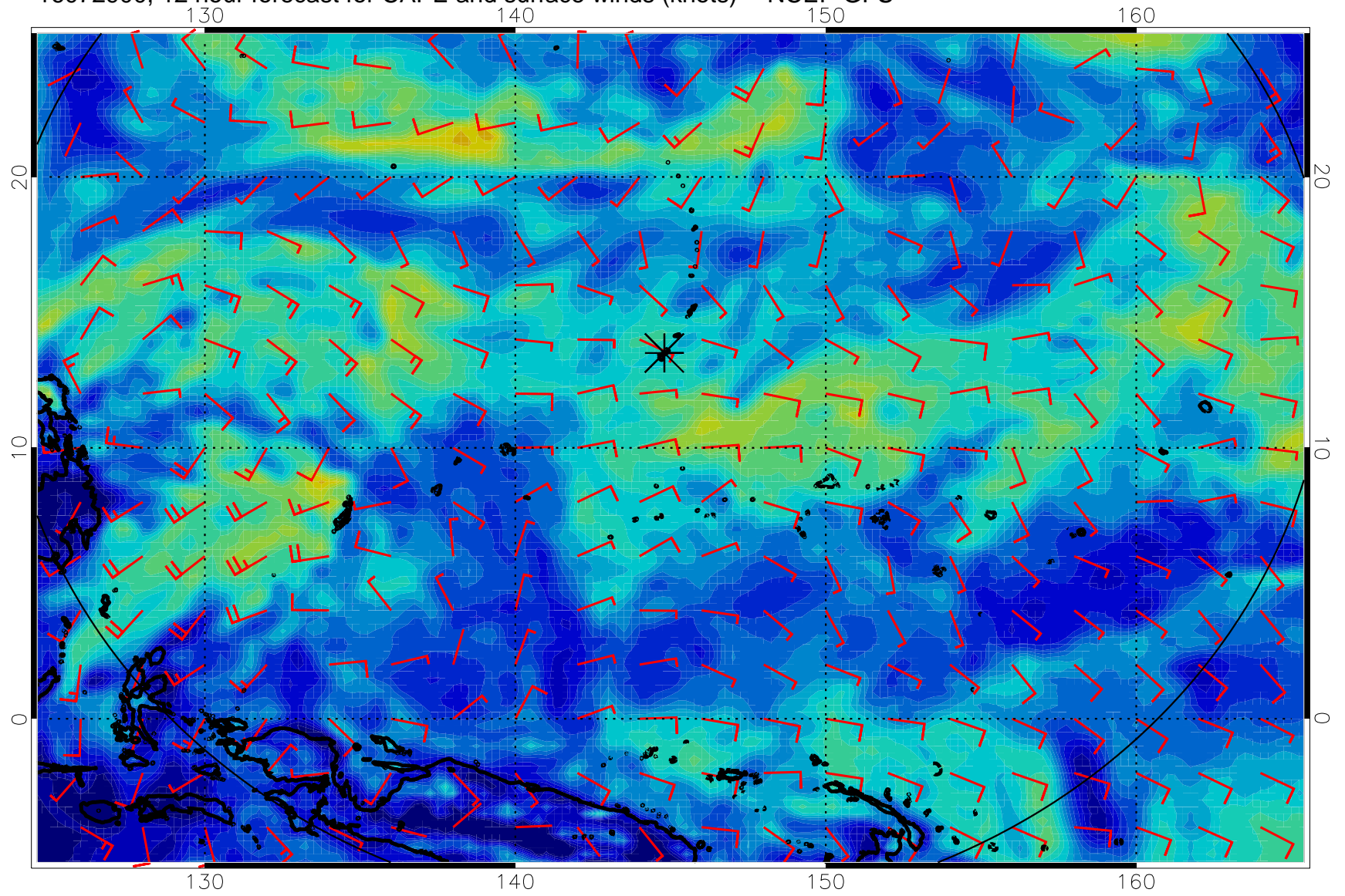
16072900, 12 hour forecast for CAPE and surface winds (knots) -- NCEP GFS
