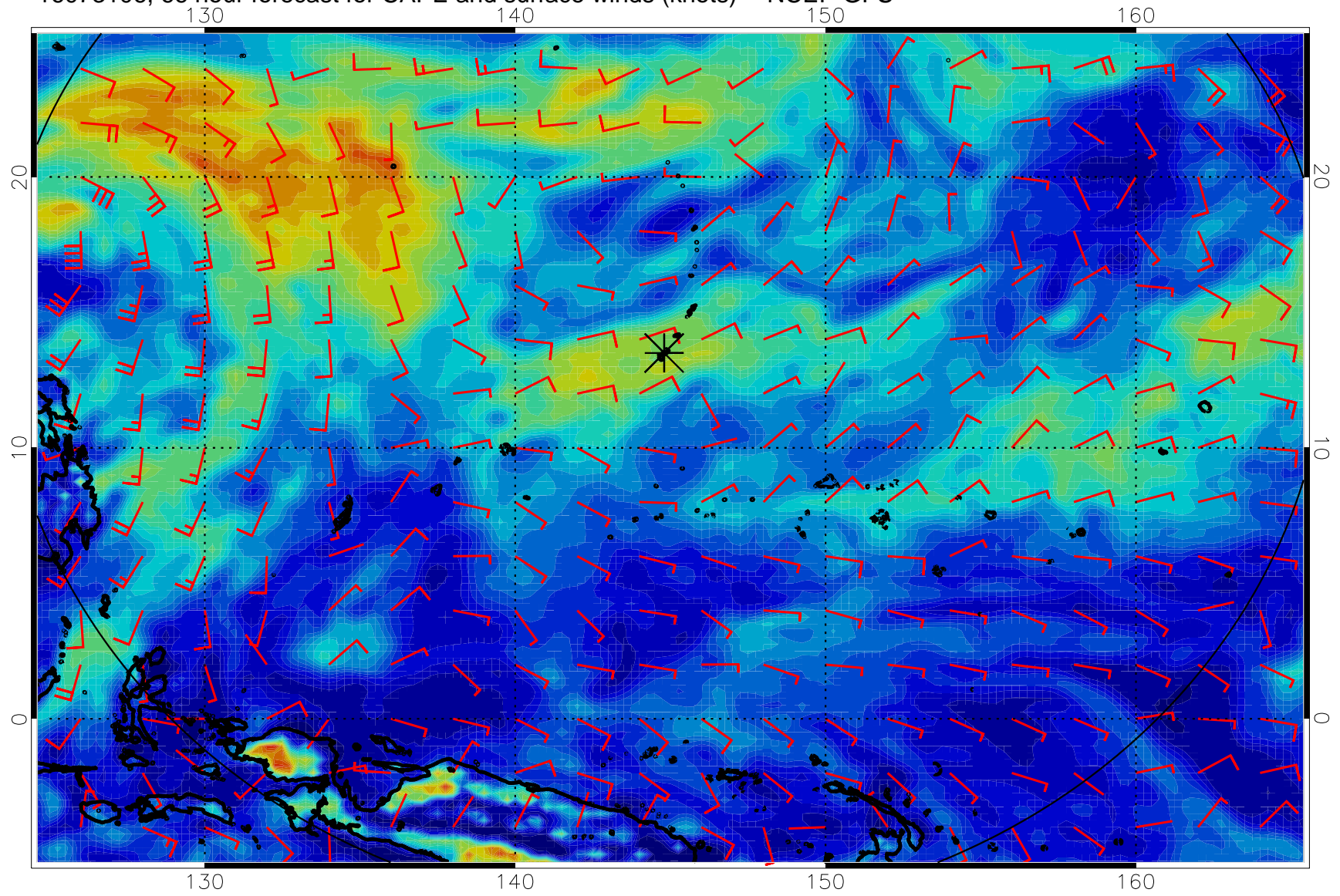
16073106, 66 hour forecast for CAPE and surface winds (knots) -- NCEP GFS
