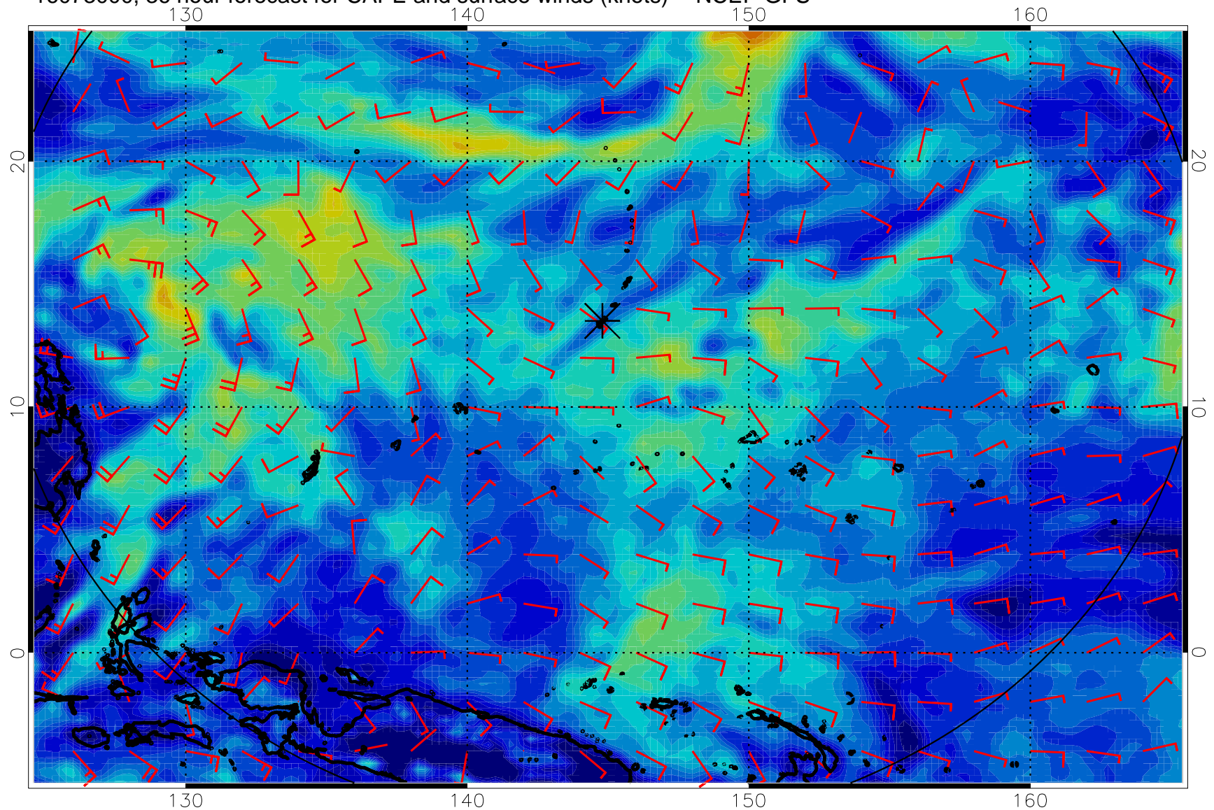
16073000, 36 hour forecast for CAPE and surface winds (knots) -- NCEP GFS
