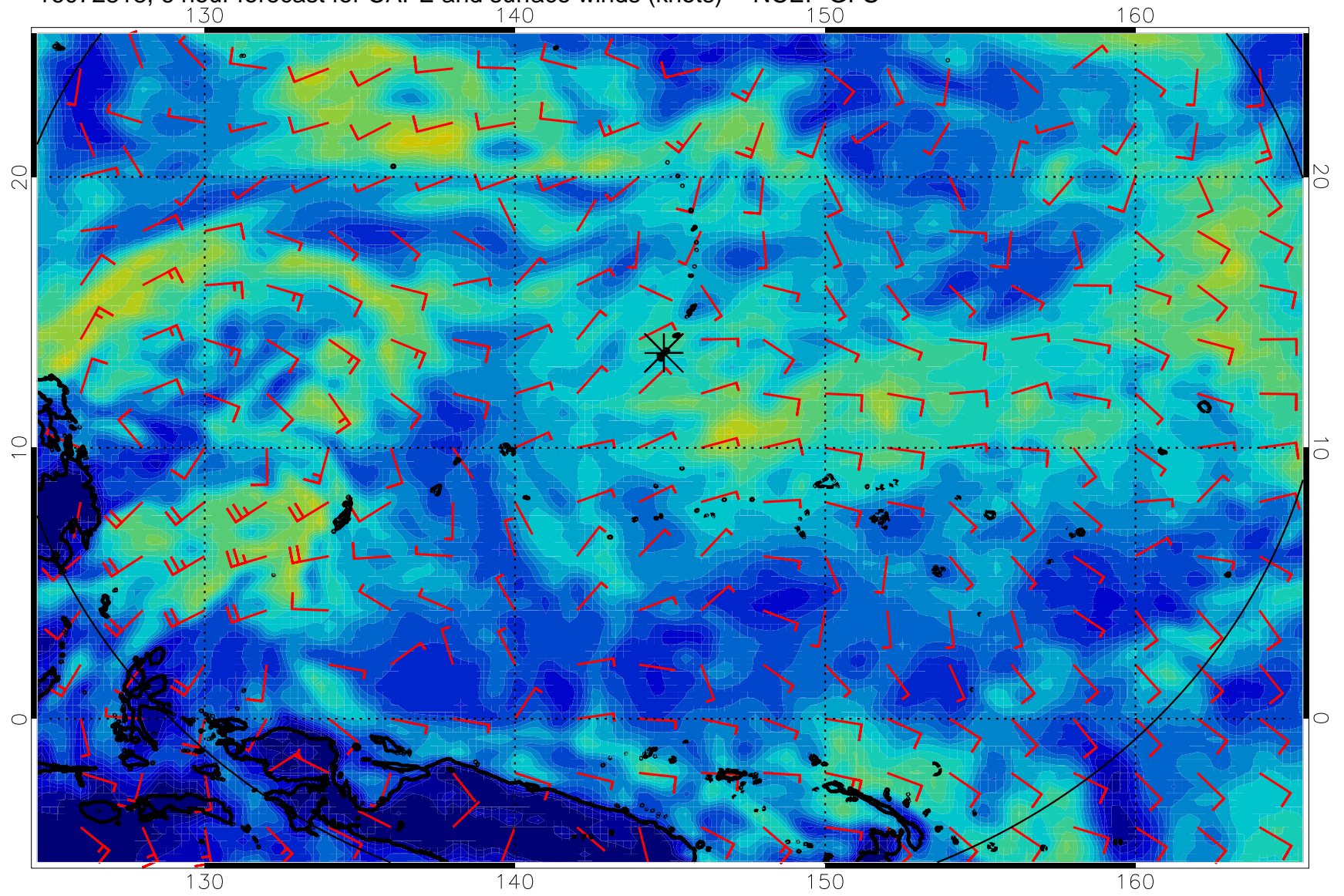
16072818, 6 hour forecast for CAPE and surface winds (knots) -- NCEP GFS
