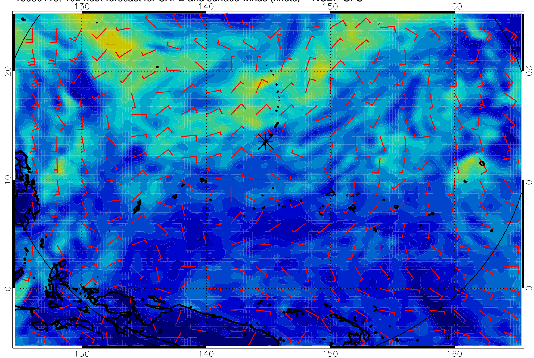
16080118, 102 hour forecast for CAPE and surface winds (knots) -- NCEP GFS
