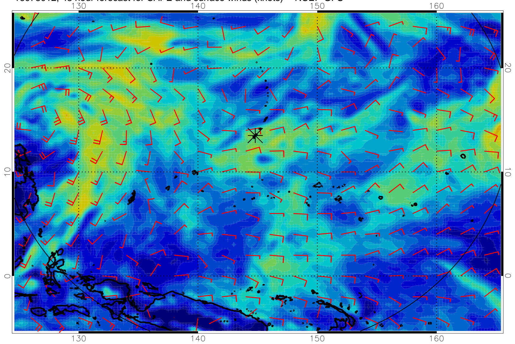
16073012, 48 hour forecast for CAPE and surface winds (knots) -- NCEP GFS
