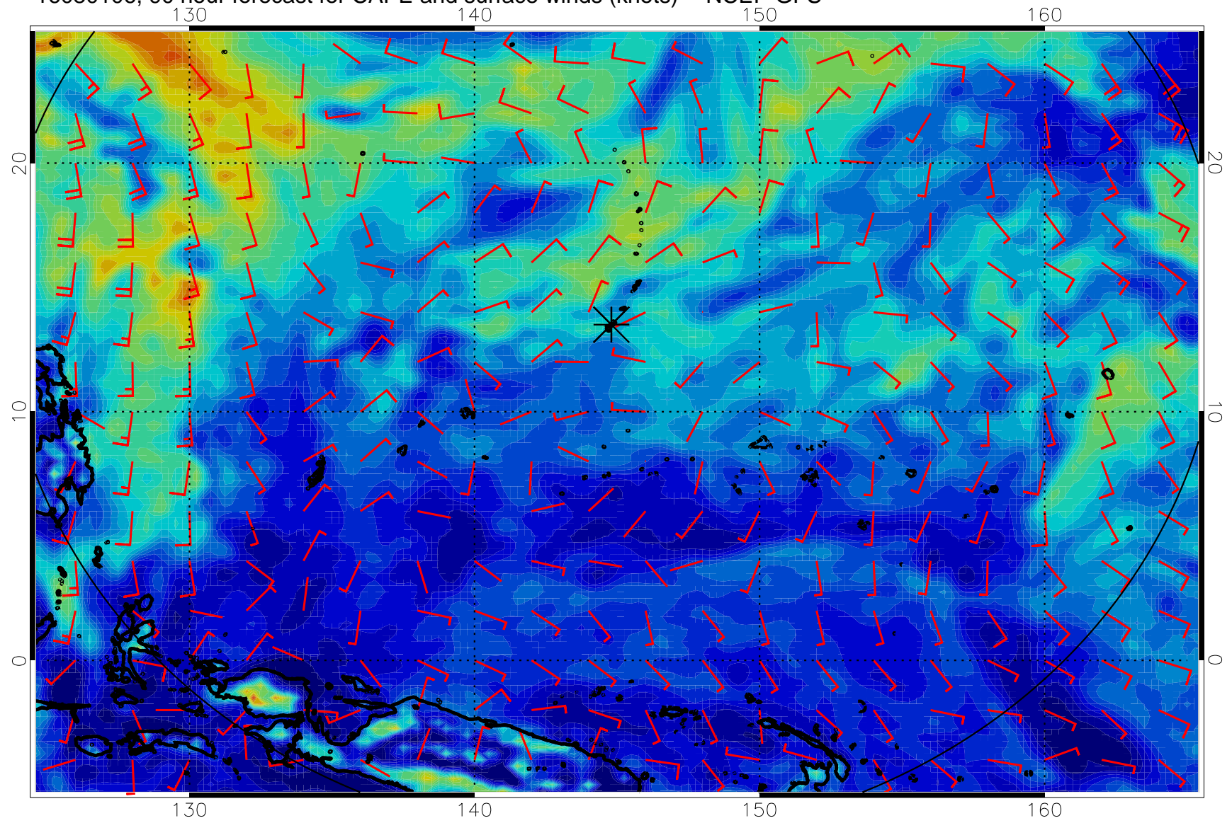
16080106, 90 hour forecast for CAPE and surface winds (knots) -- NCEP GFS
