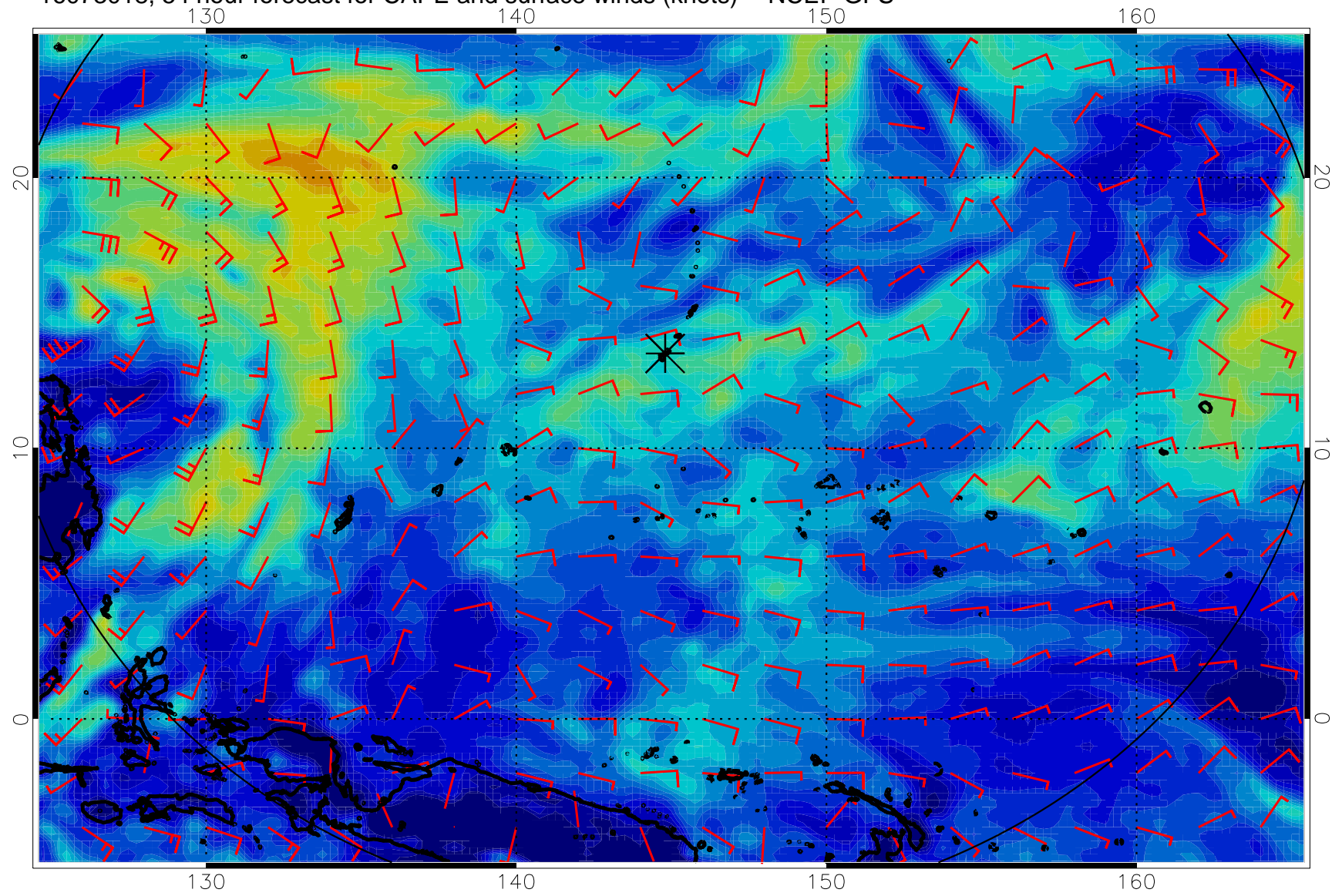
16073018, 54 hour forecast for CAPE and surface winds (knots) -- NCEP GFS
