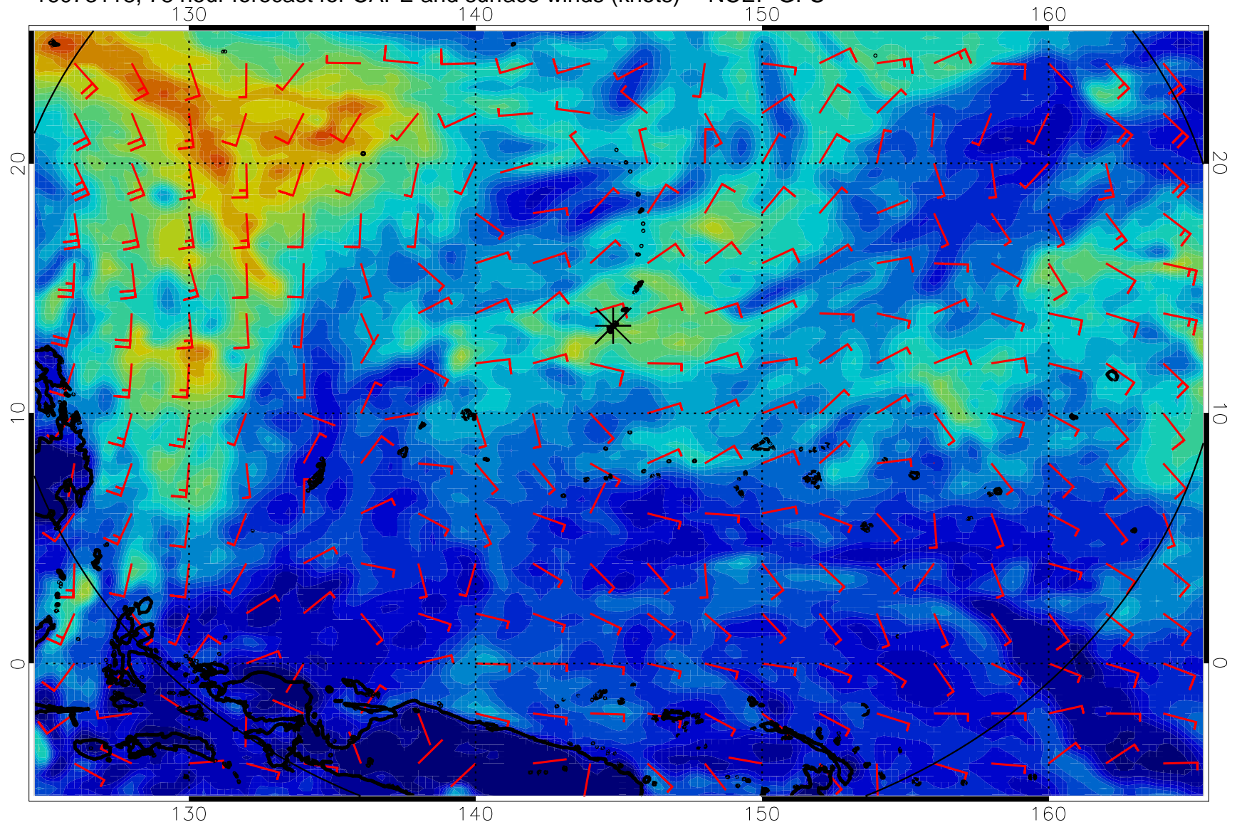
16073118, 78 hour forecast for CAPE and surface winds (knots) -- NCEP GFS
