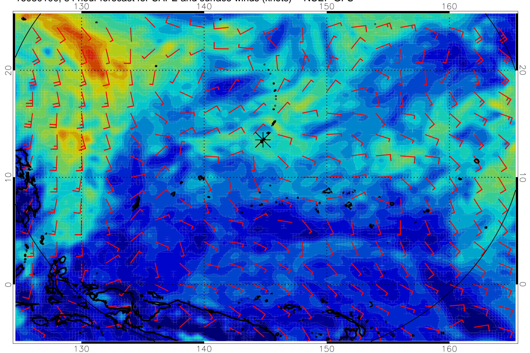
16080100, 84 hour forecast for CAPE and surface winds (knots) -- NCEP GFS
