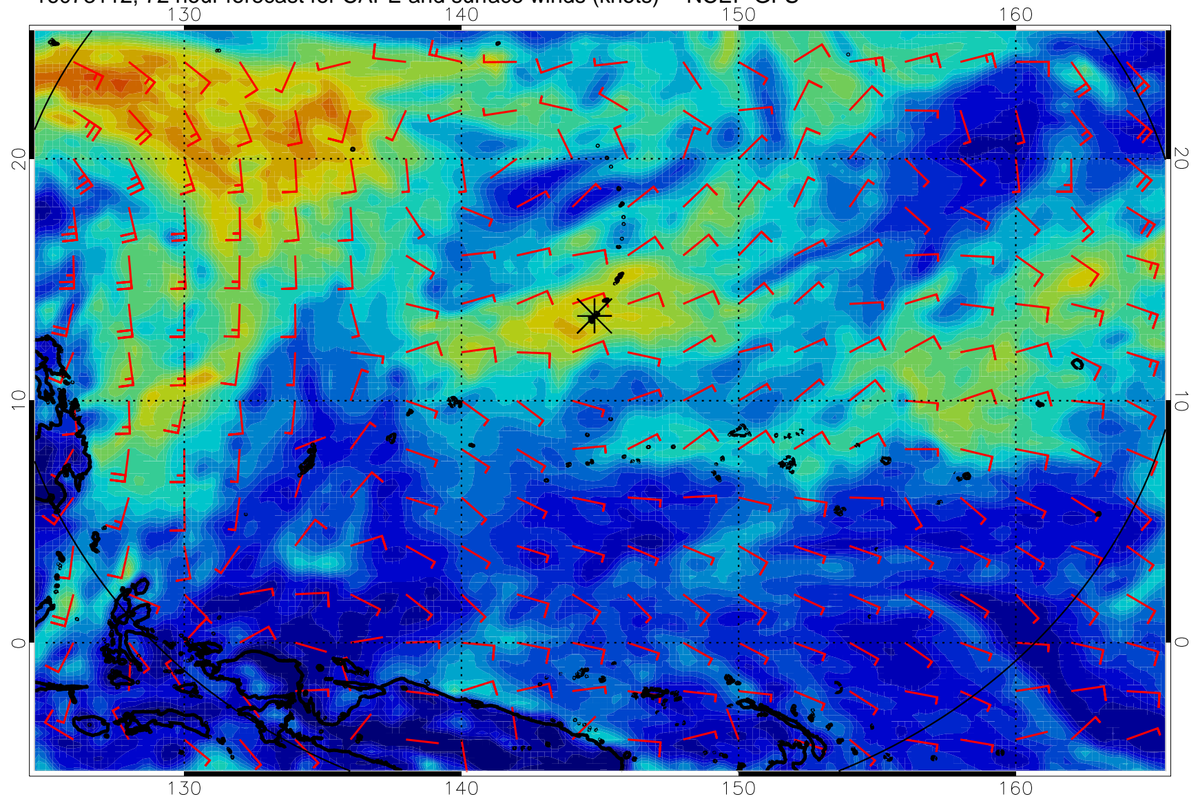
16073112, 72 hour forecast for CAPE and surface winds (knots) -- NCEP GFS
