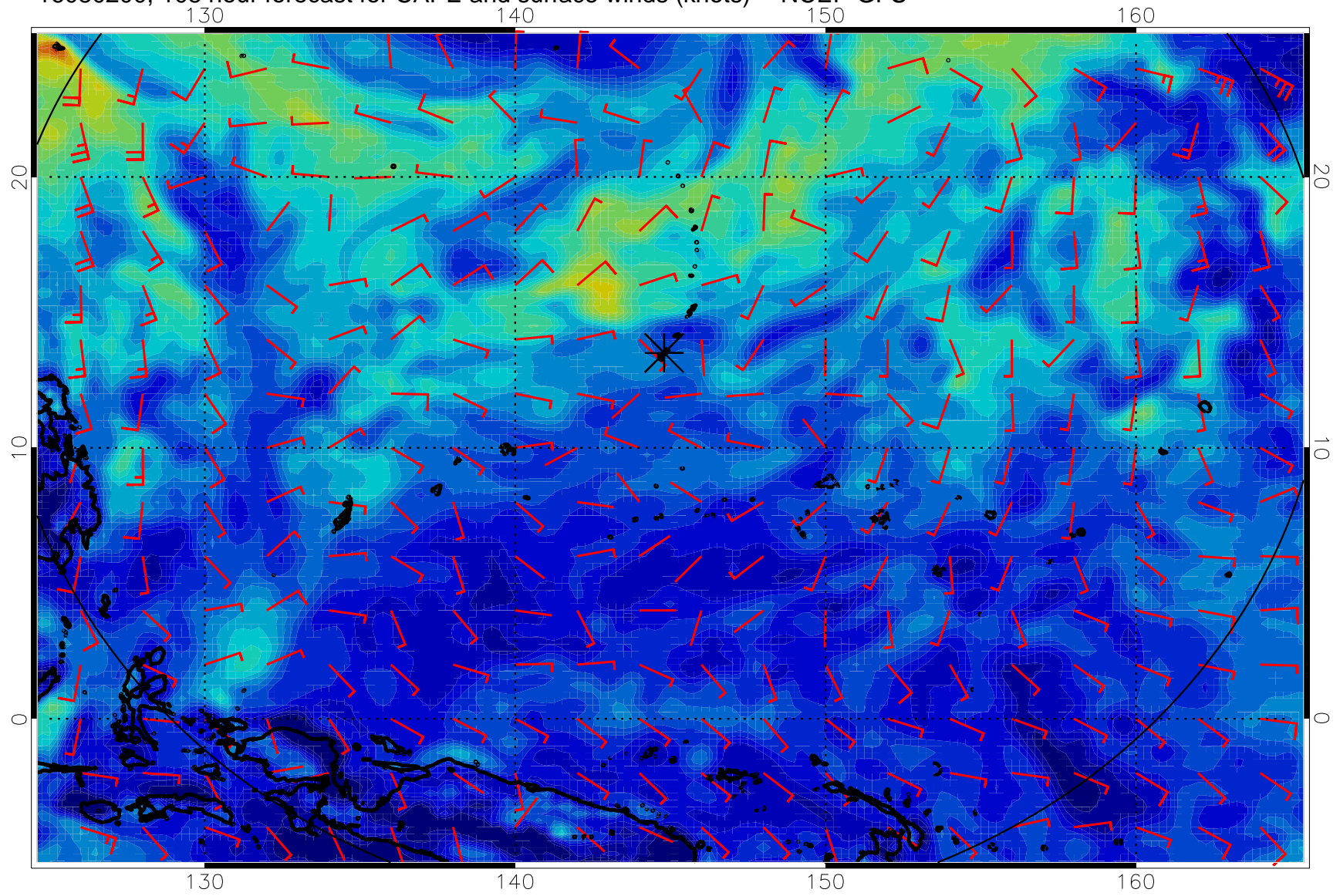
16080200, 108 hour forecast for CAPE and surface winds (knots) -- NCEP GFS
