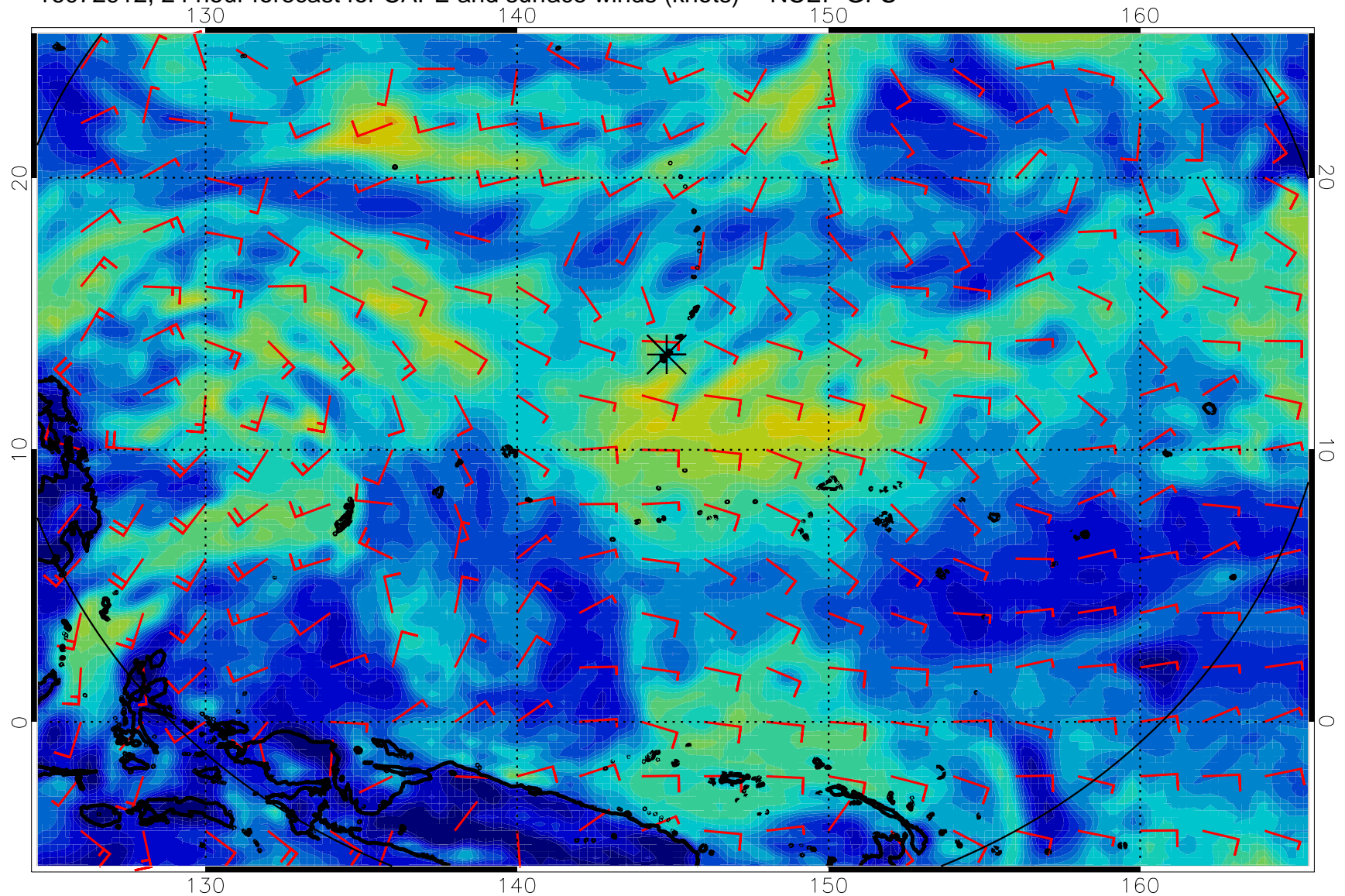
16072912, 24 hour forecast for CAPE and surface winds (knots) -- NCEP GFS
