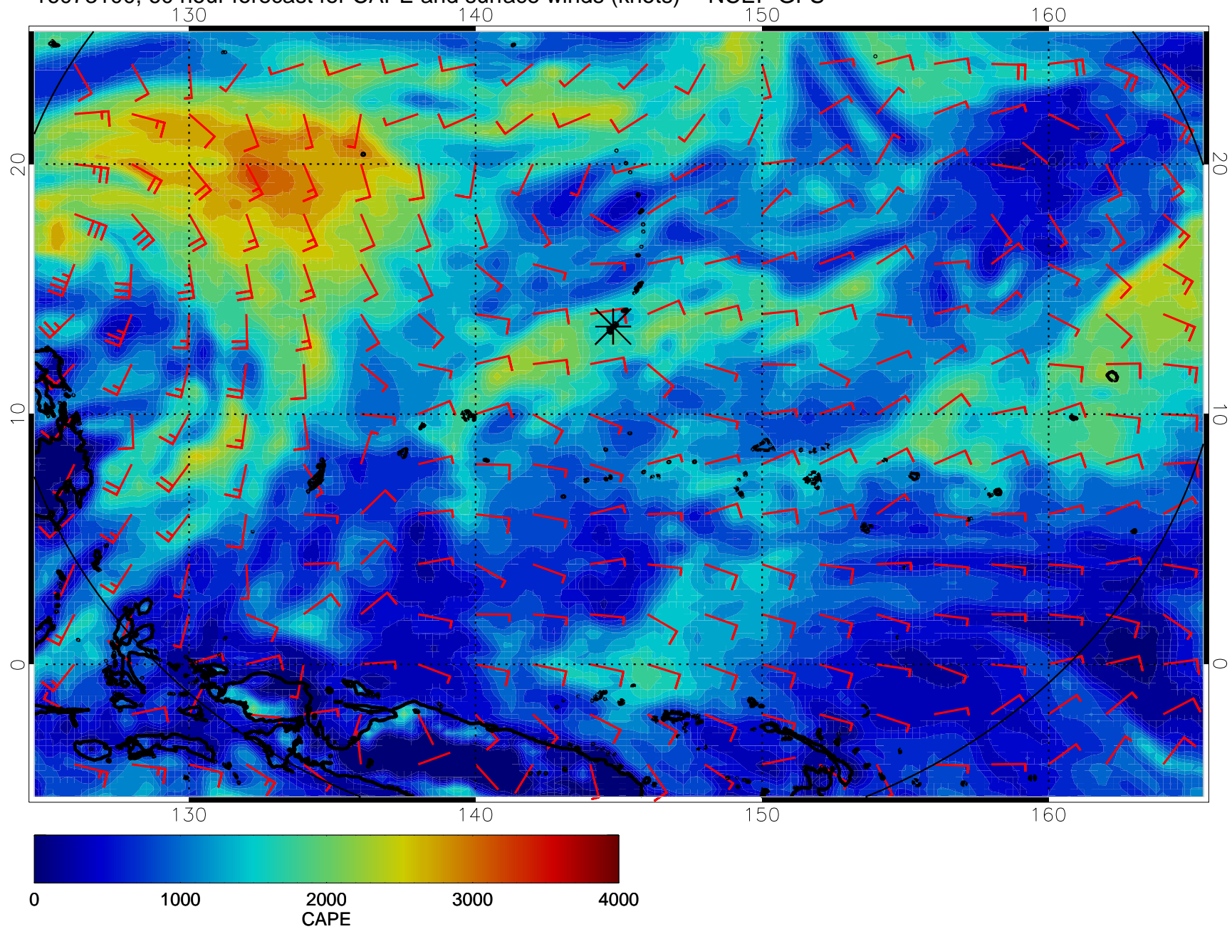
16073100, 60 hour forecast for CAPE and surface winds (knots) -- NCEP GFS
