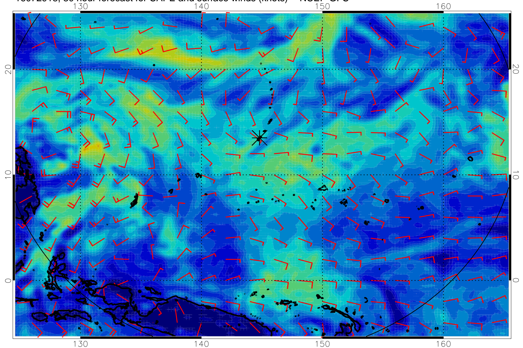
16072918, 30 hour forecast for CAPE and surface winds (knots) -- NCEP GFS
