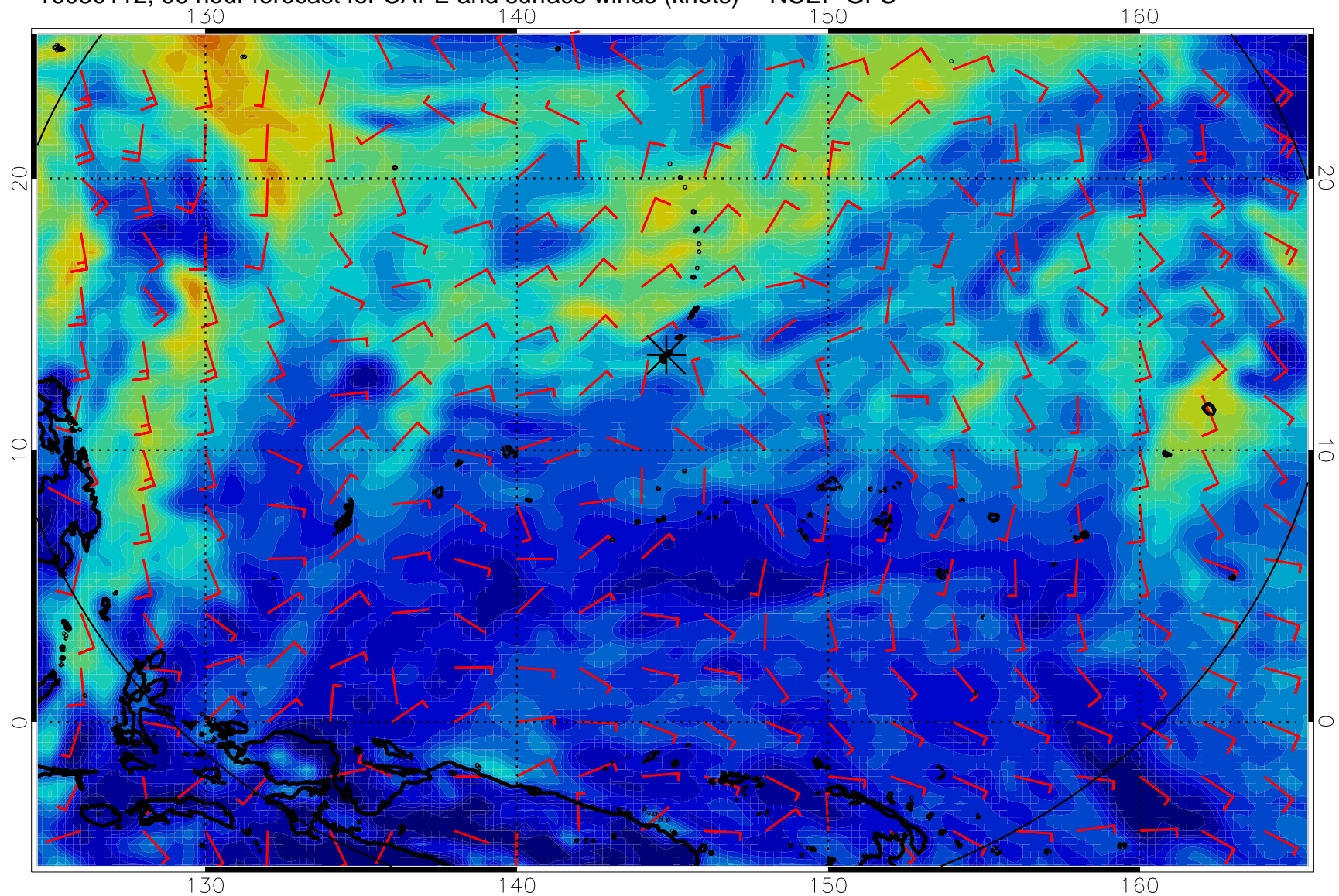
16080112, 96 hour forecast for CAPE and surface winds (knots) -- NCEP GFS
