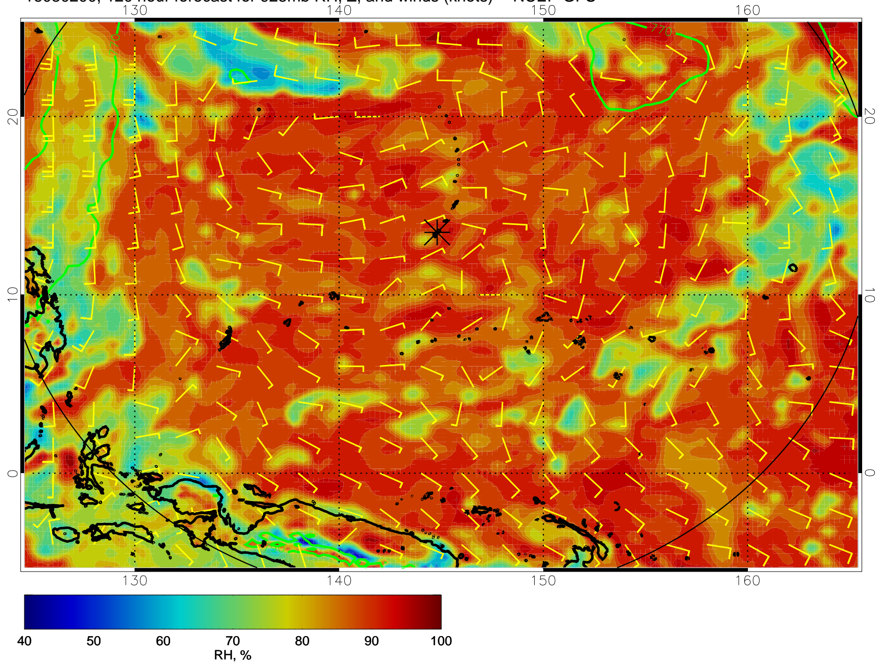
16080200, 120 hour forecast for 925mb RH, Z, and winds (knots) -- NCEP GFS
