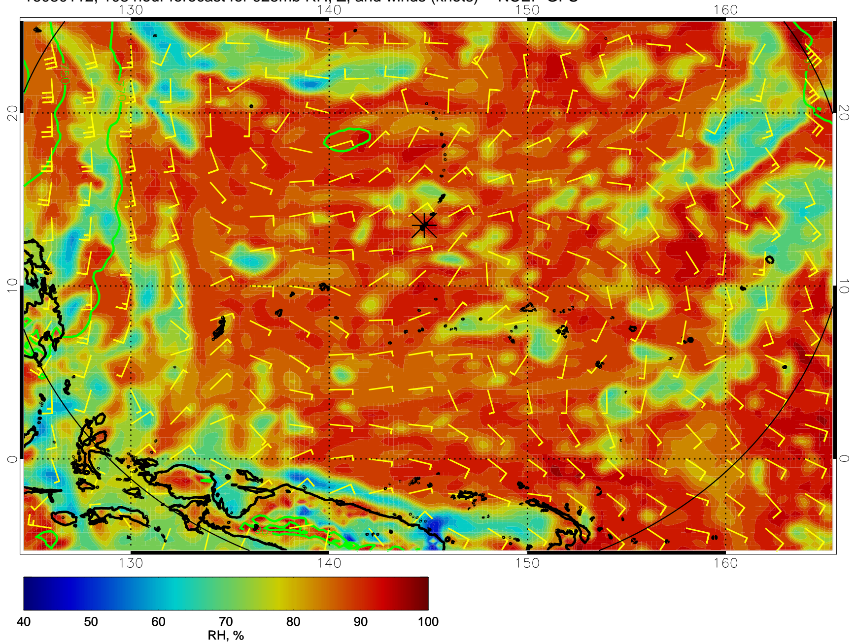
16080112, 108 hour forecast for 925mb RH, Z, and winds (knots) -- NCEP GFS
