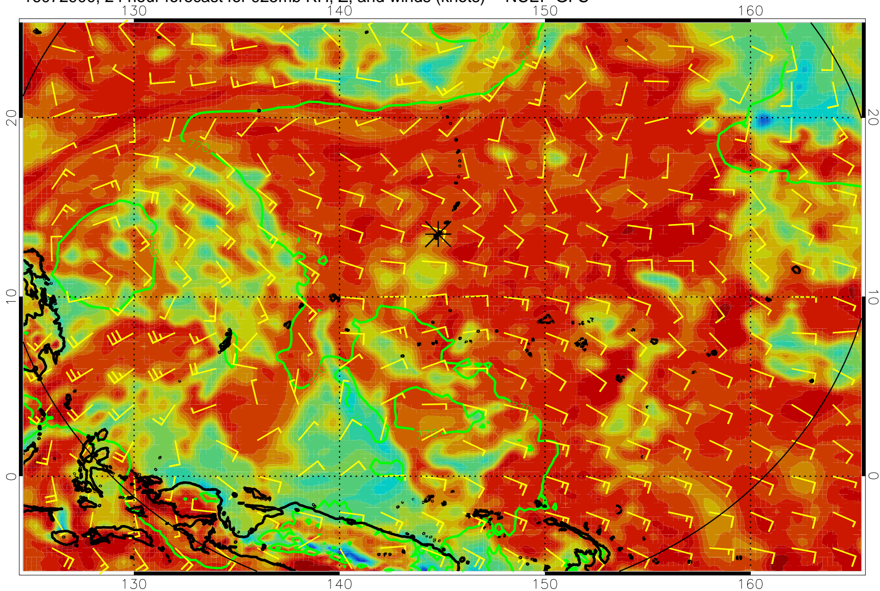
16072900, 24 hour forecast for 925mb RH, Z, and winds (knots) -- NCEP GFS
