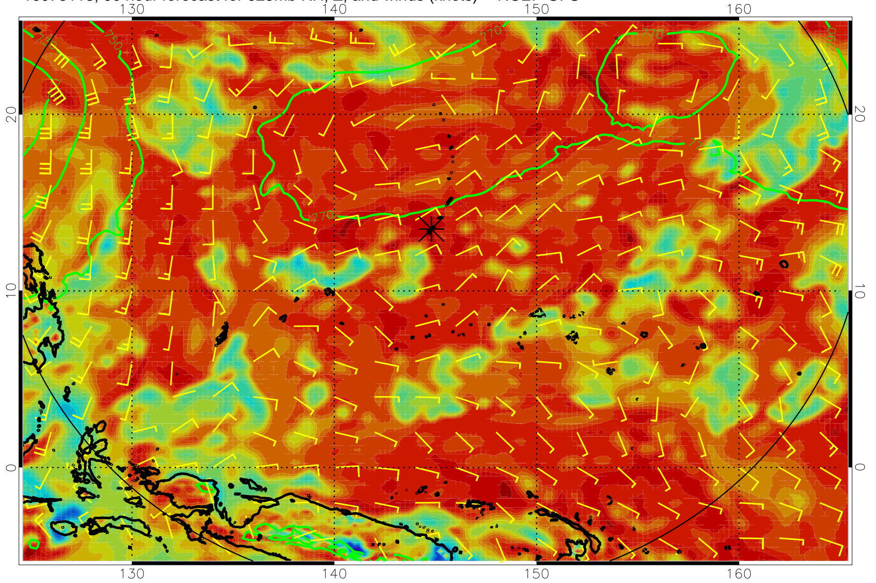
16073118, 90 hour forecast for 925mb RH, Z, and winds (knots) -- NCEP GFS
