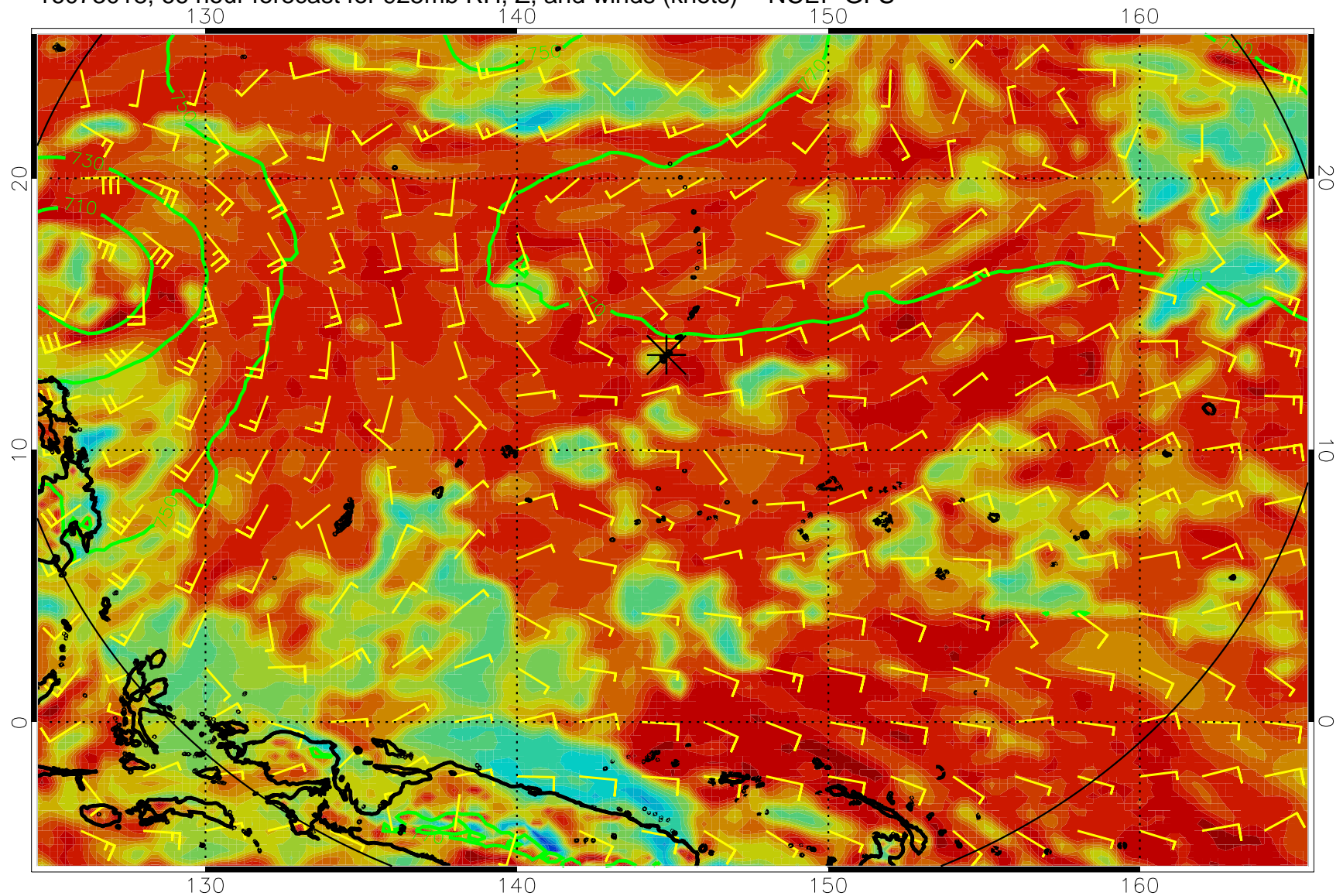
16073018, 66 hour forecast for 925mb RH, Z, and winds (knots) -- NCEP GFS
