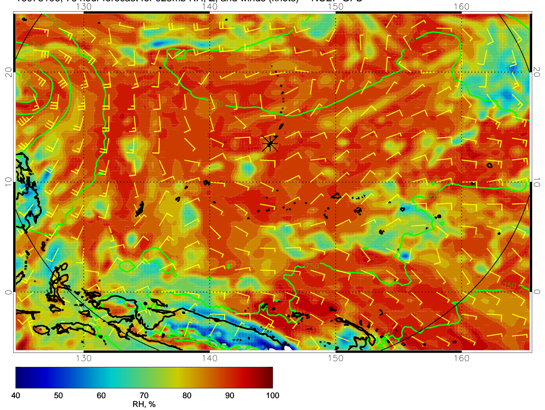
16073106, 78 hour forecast for 925mb RH, Z, and winds (knots) -- NCEP GFS
