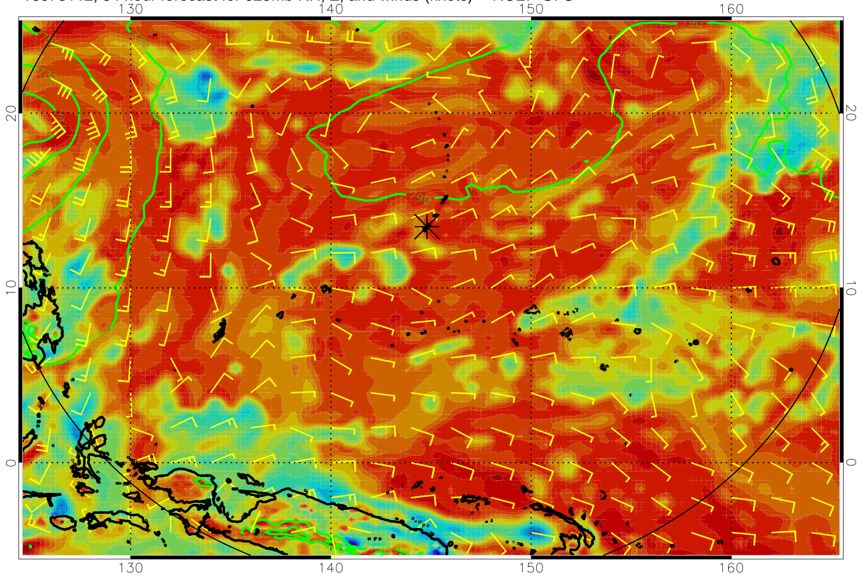
16073112, 84 hour forecast for 925mb RH, Z, and winds (knots) -- NCEP GFS
