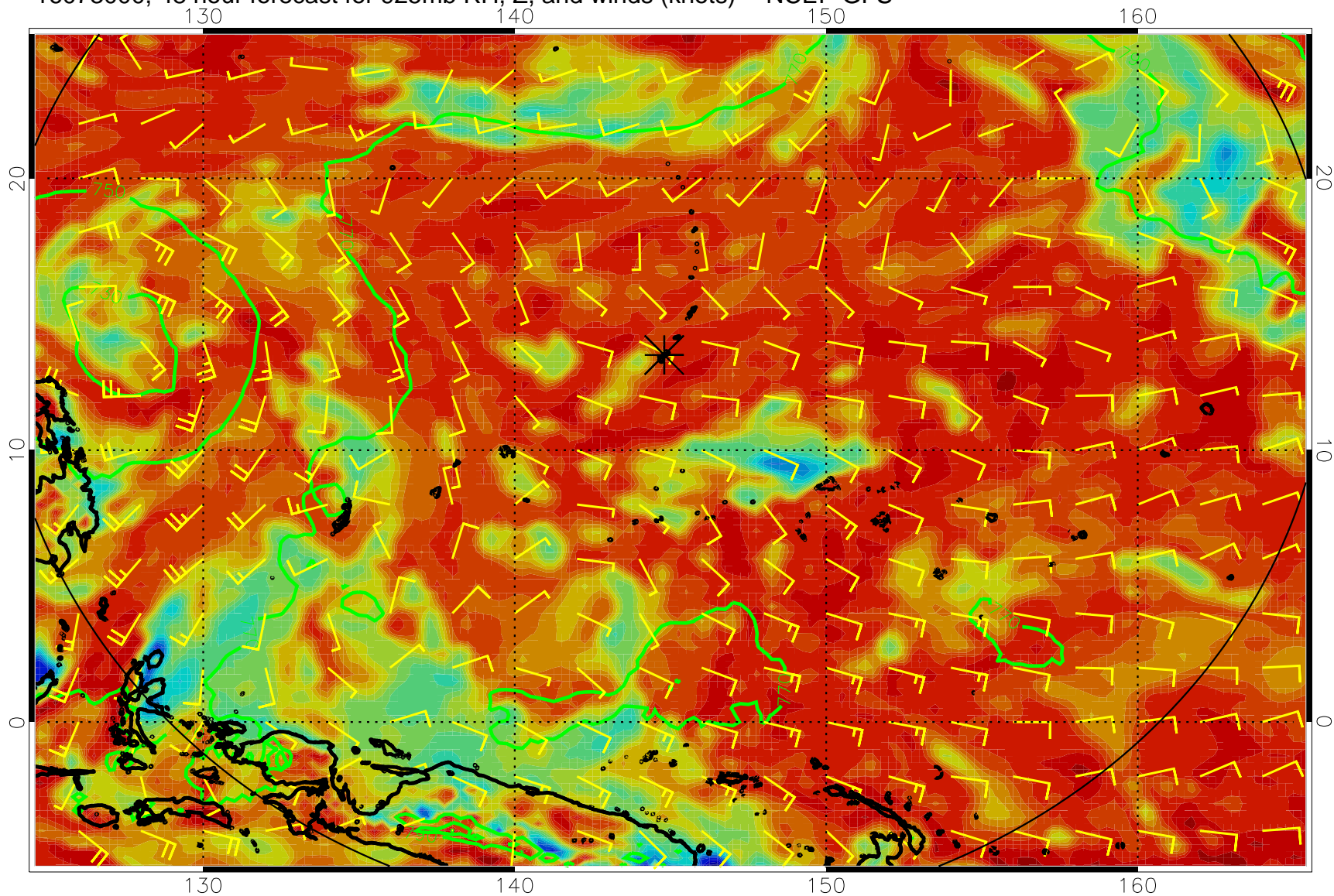
16073000, 48 hour forecast for 925mb RH, Z, and winds (knots) -- NCEP GFS
