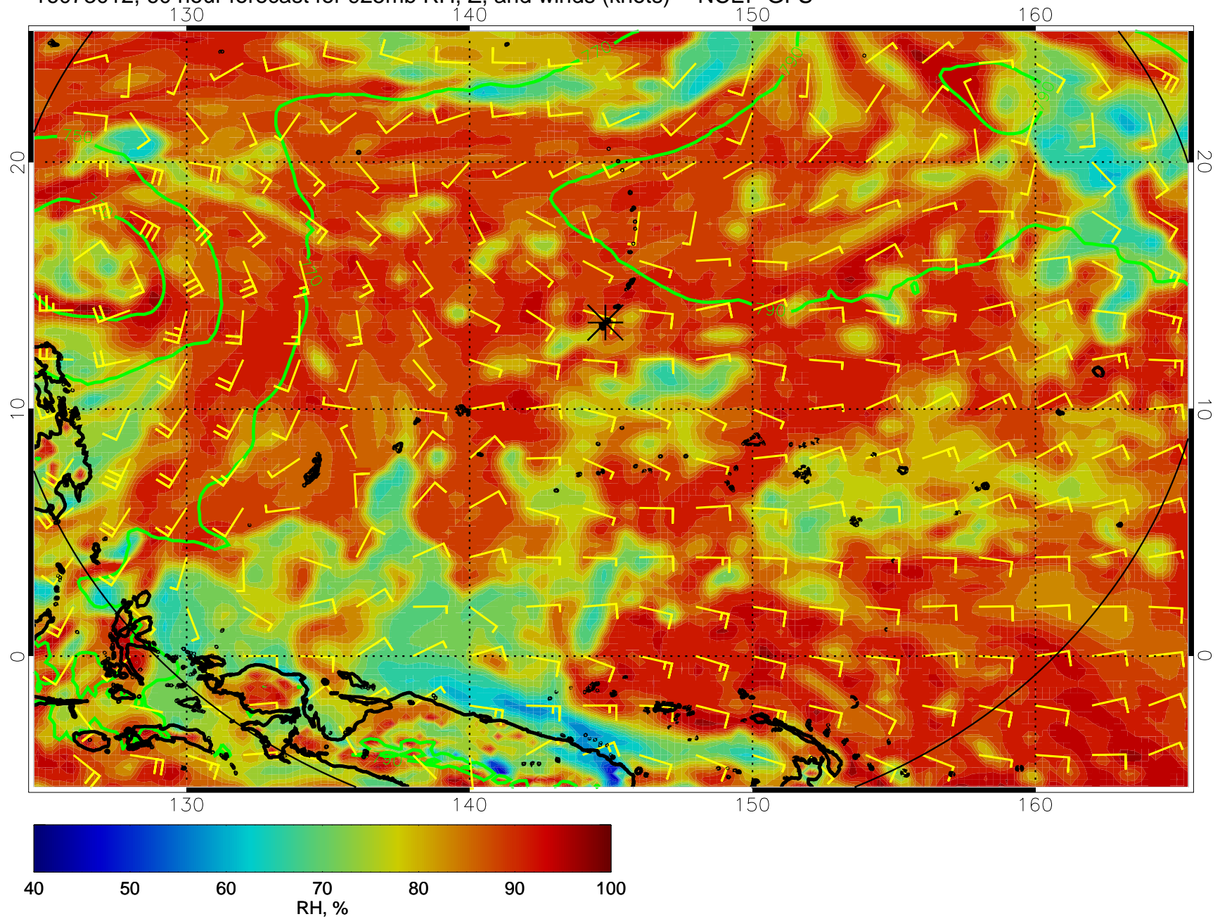
16073012, 60 hour forecast for 925mb RH, Z, and winds (knots) -- NCEP GFS
