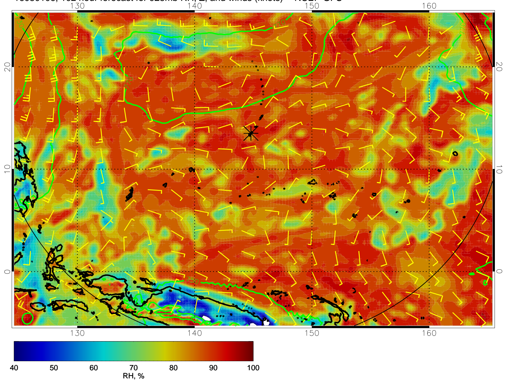
16080106, 102 hour forecast for 925mb RH, Z, and winds (knots) -- NCEP GFS
