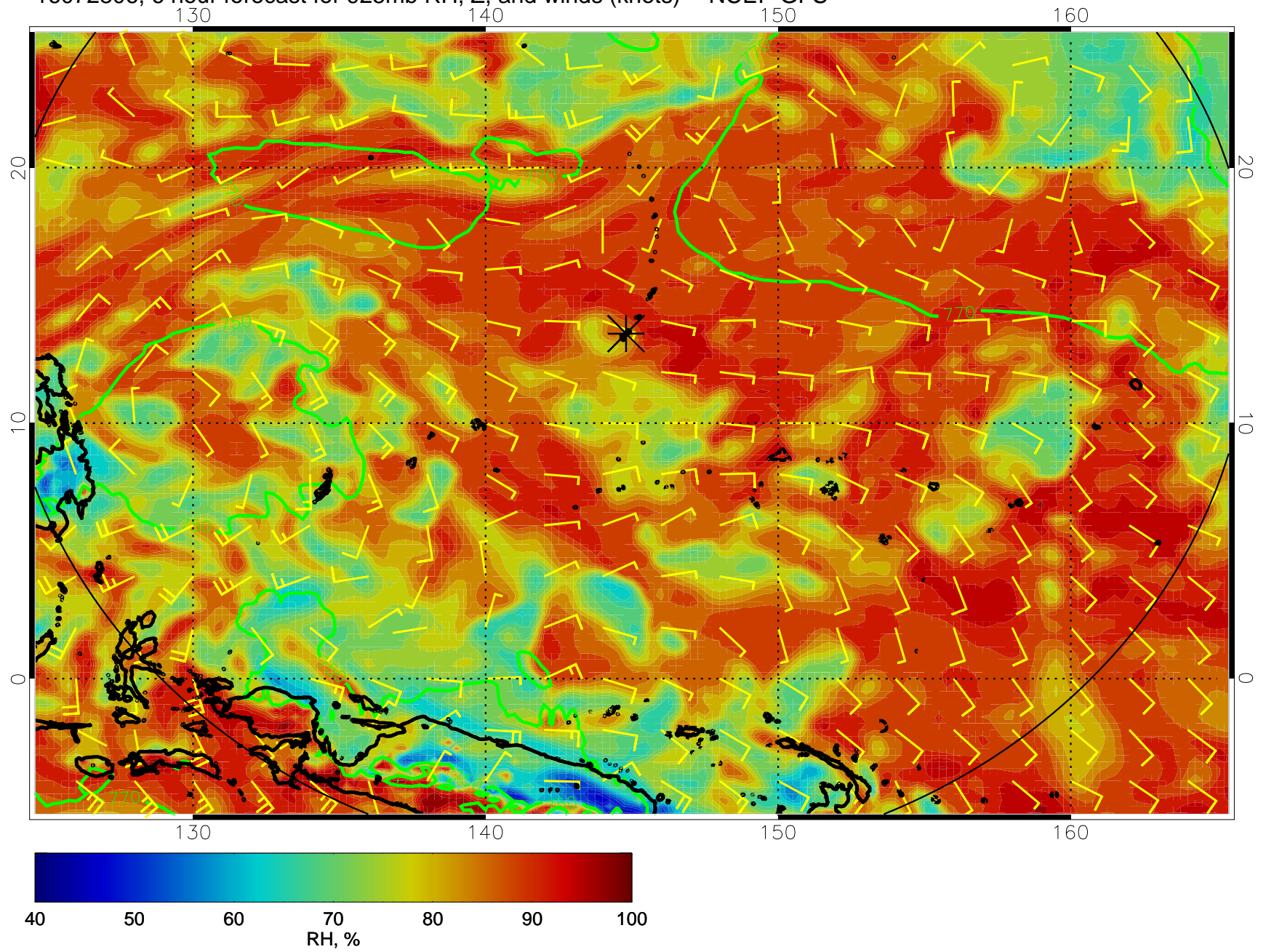
16072806, 6 hour forecast for 925mb RH, Z, and winds (knots) -- NCEP GFS
