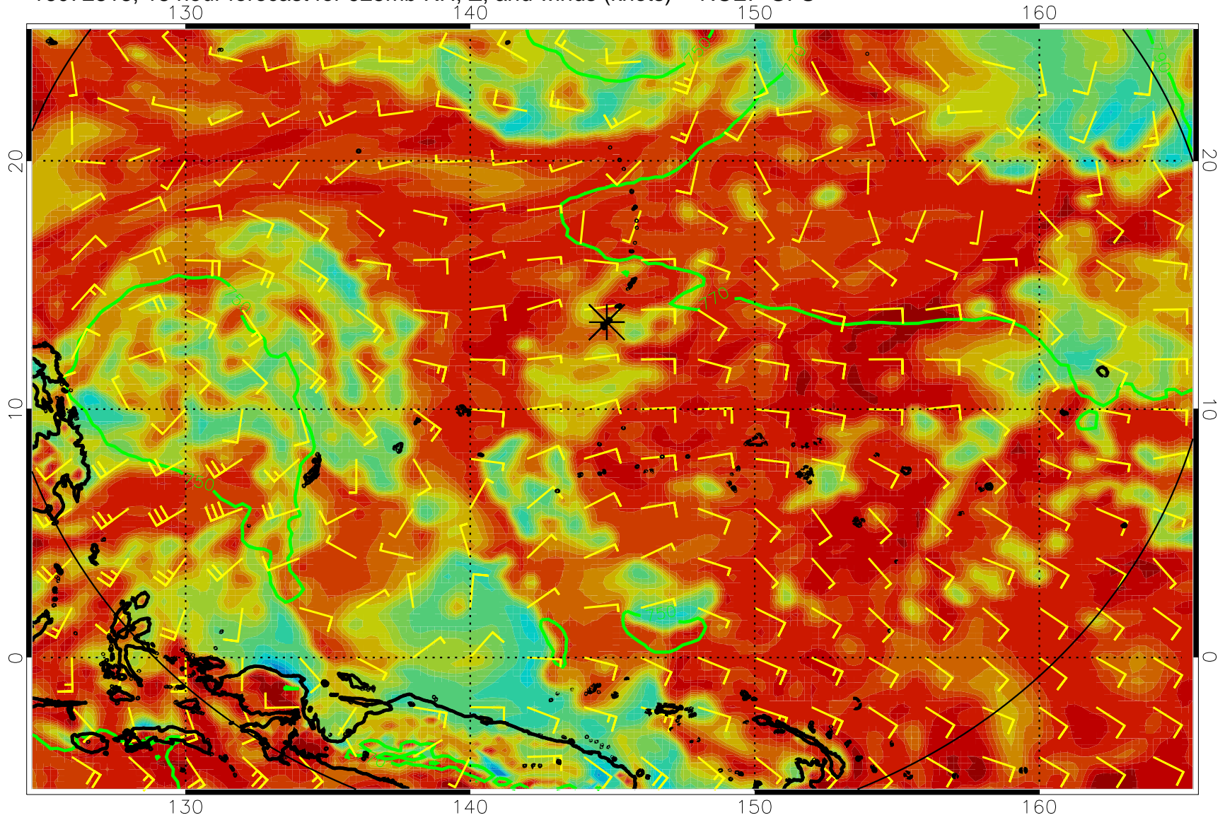
16072818, 18 hour forecast for 925mb RH, Z, and winds (knots) -- NCEP GFS
