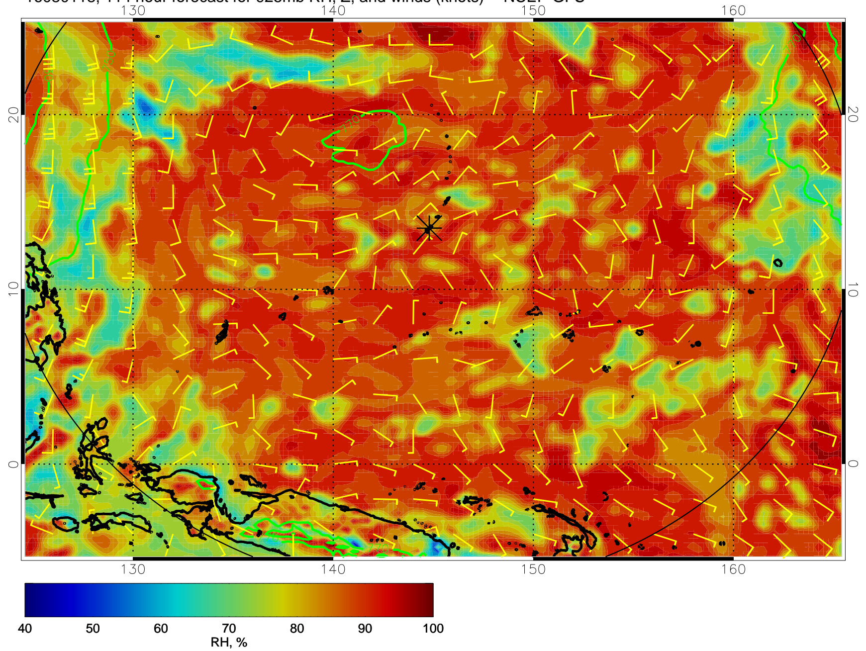
16080118, 114 hour forecast for 925mb RH, Z, and winds (knots) -- NCEP GFS
