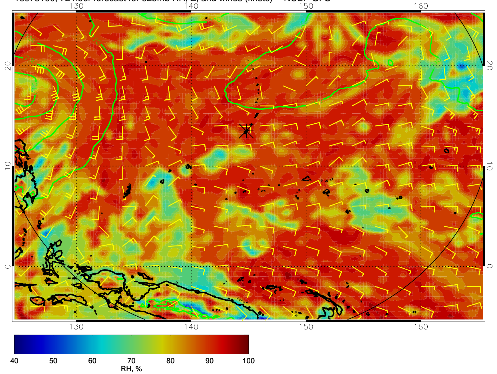
16073100, 72 hour forecast for 925mb RH, Z, and winds (knots) -- NCEP GFS
