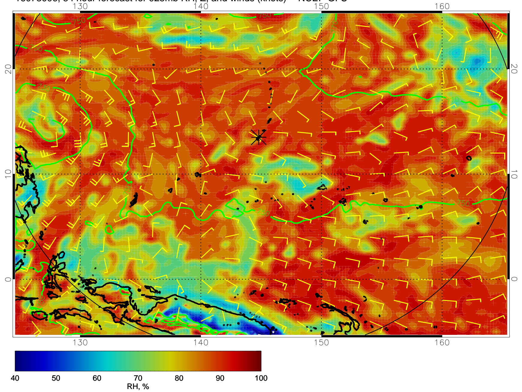
16073006, 54 hour forecast for 925mb RH, Z, and winds (knots) -- NCEP GFS
