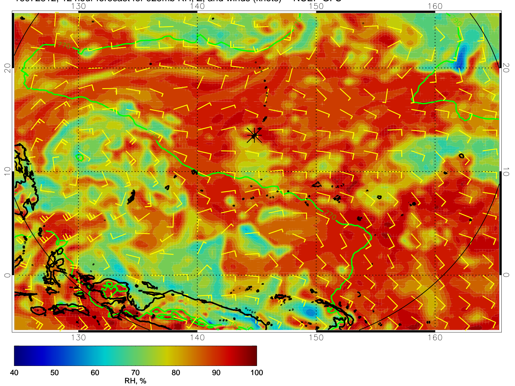
16072812, 12 hour forecast for 925mb RH, Z, and winds (knots) -- NCEP GFS
