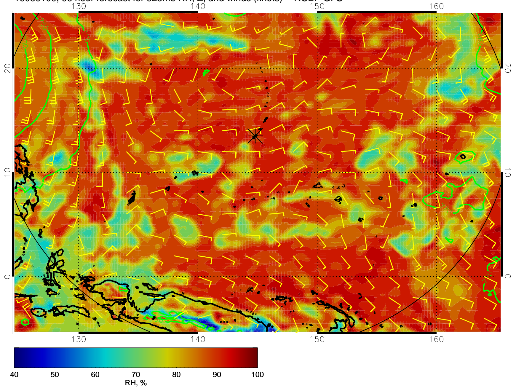
16080100, 96 hour forecast for 925mb RH, Z, and winds (knots) -- NCEP GFS
