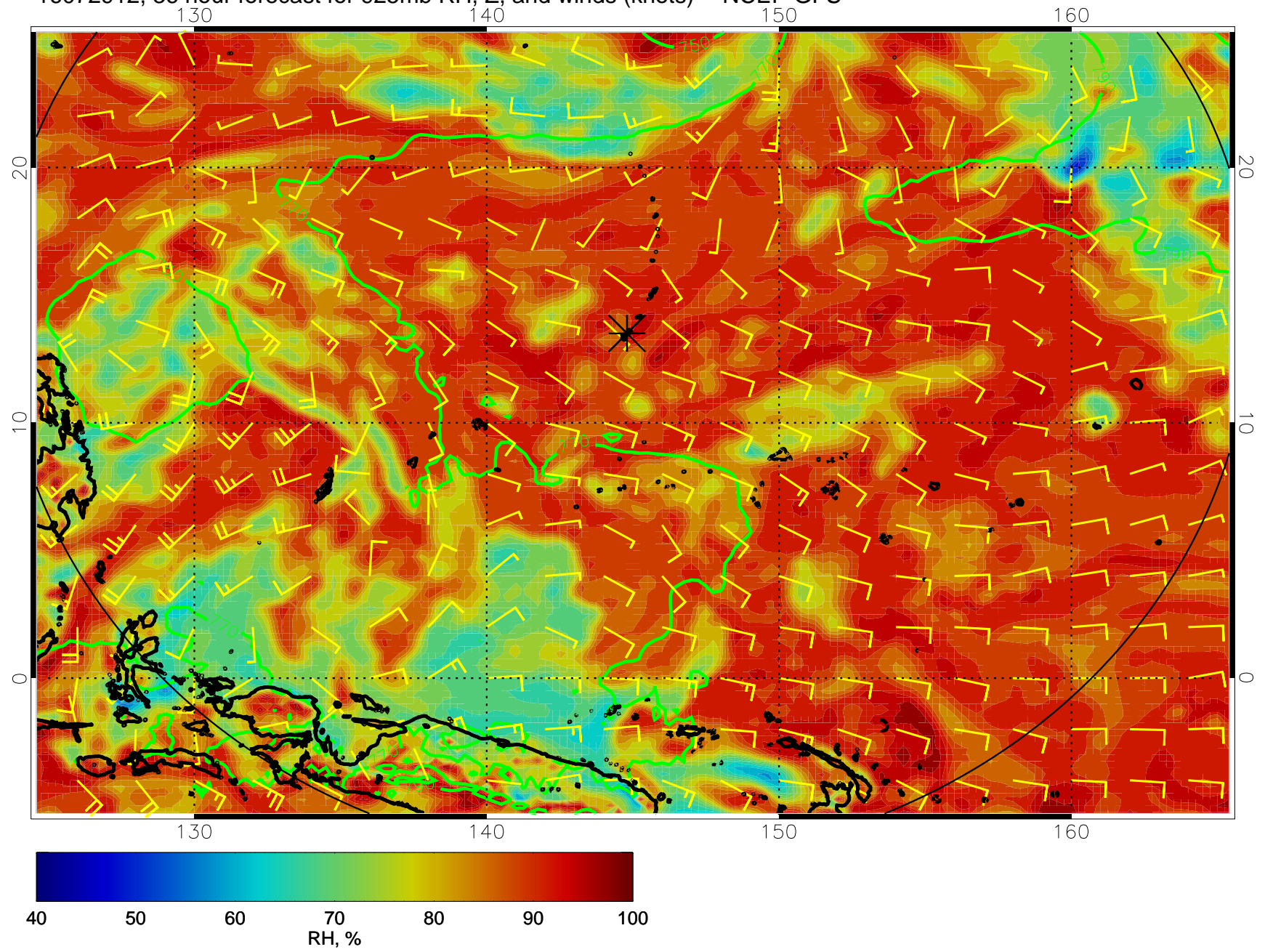
16072912, 36 hour forecast for 925mb RH, Z, and winds (knots) -- NCEP GFS
