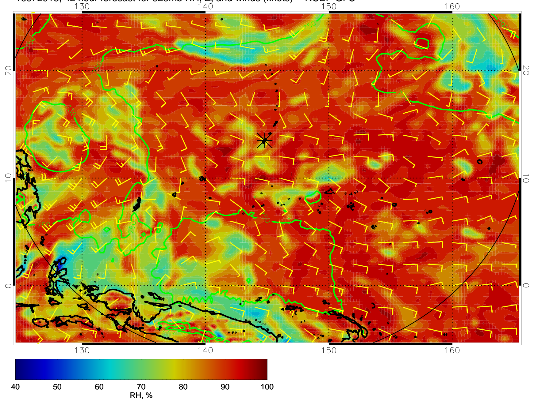
16072918, 42 hour forecast for 925mb RH, Z, and winds (knots) -- NCEP GFS
