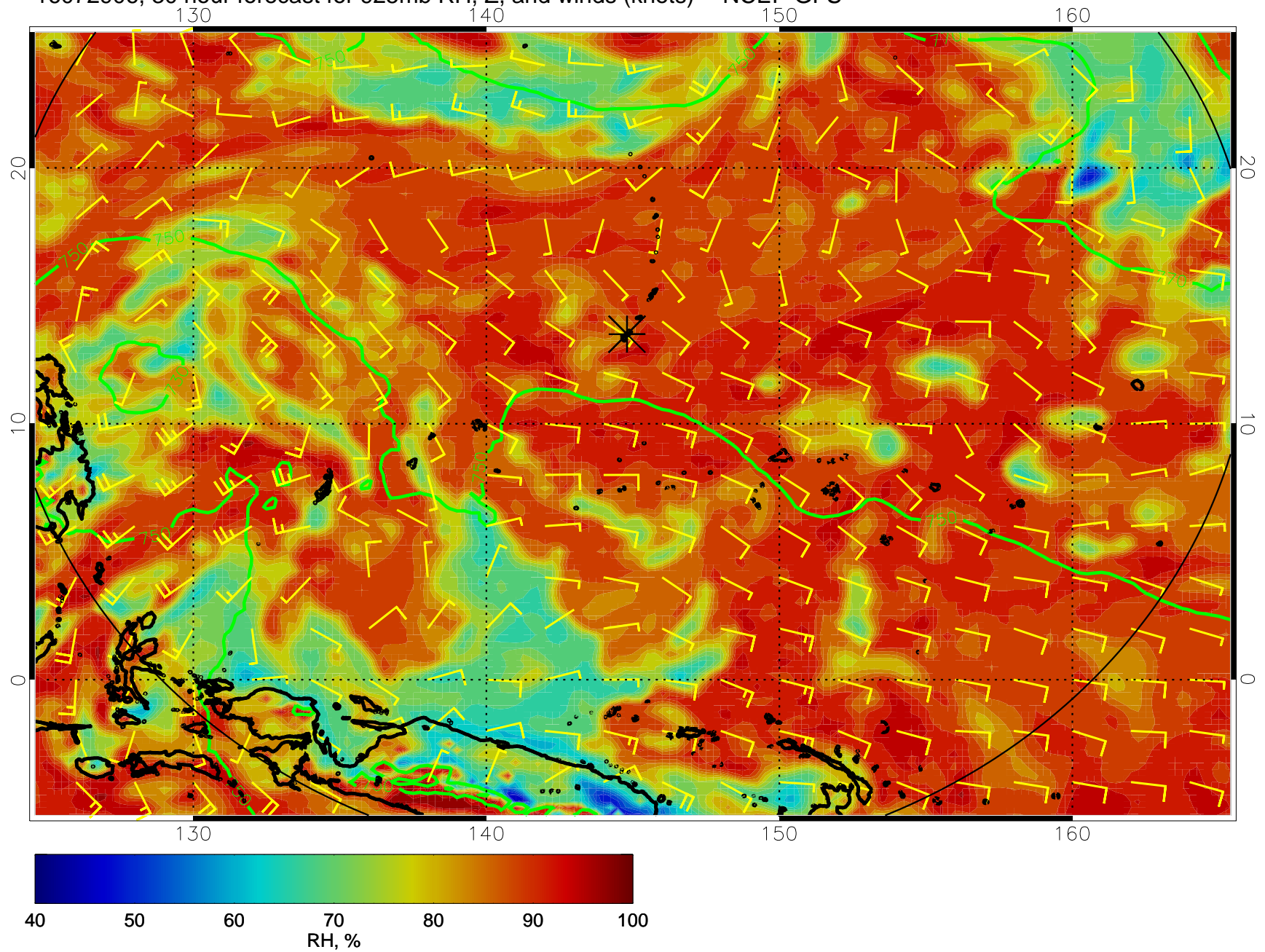
16072906, 30 hour forecast for 925mb RH, Z, and winds (knots) -- NCEP GFS
