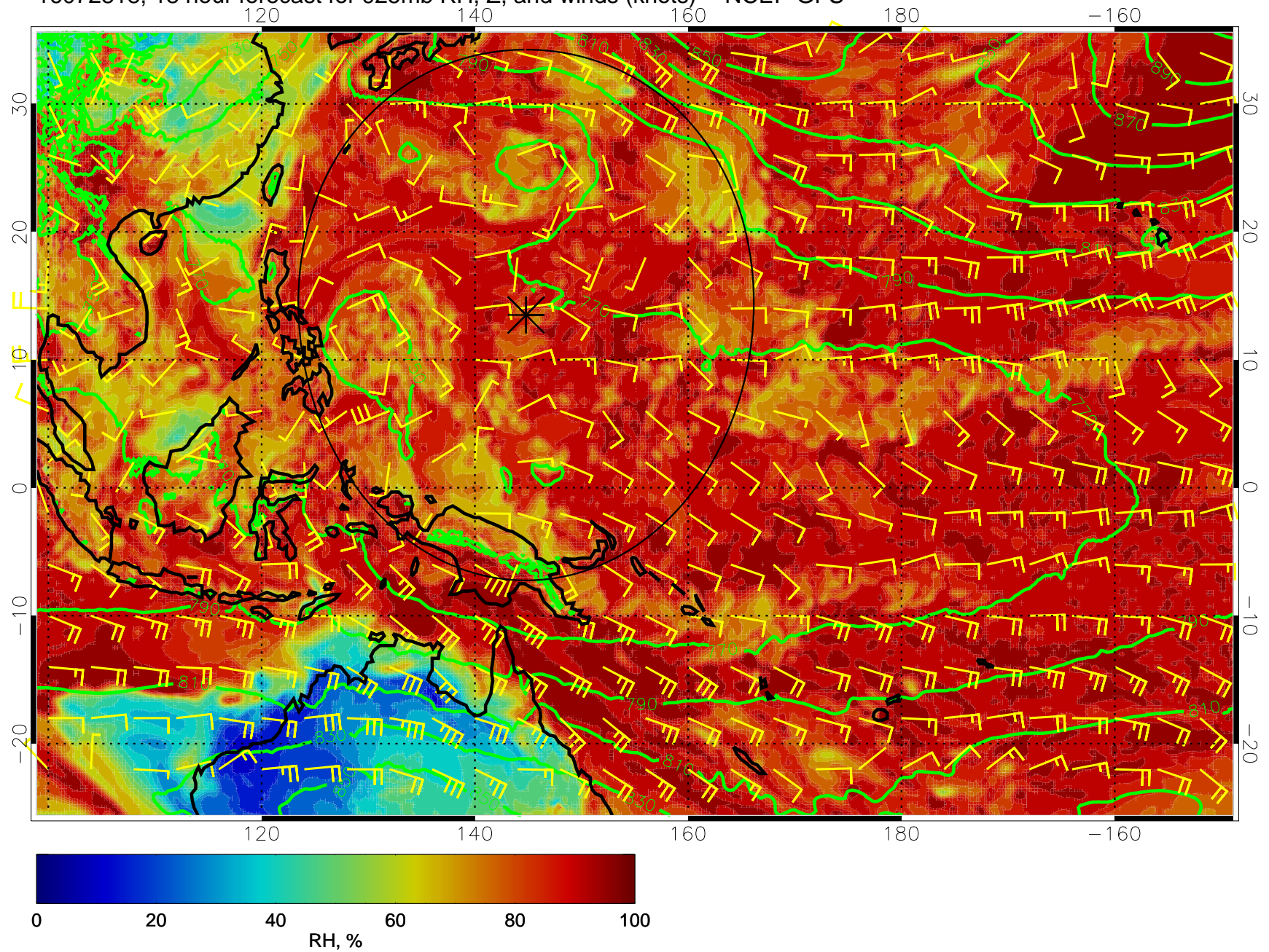
16072818, 18 hour forecast for 925mb RH, Z, and winds (knots) -- NCEP GFS
