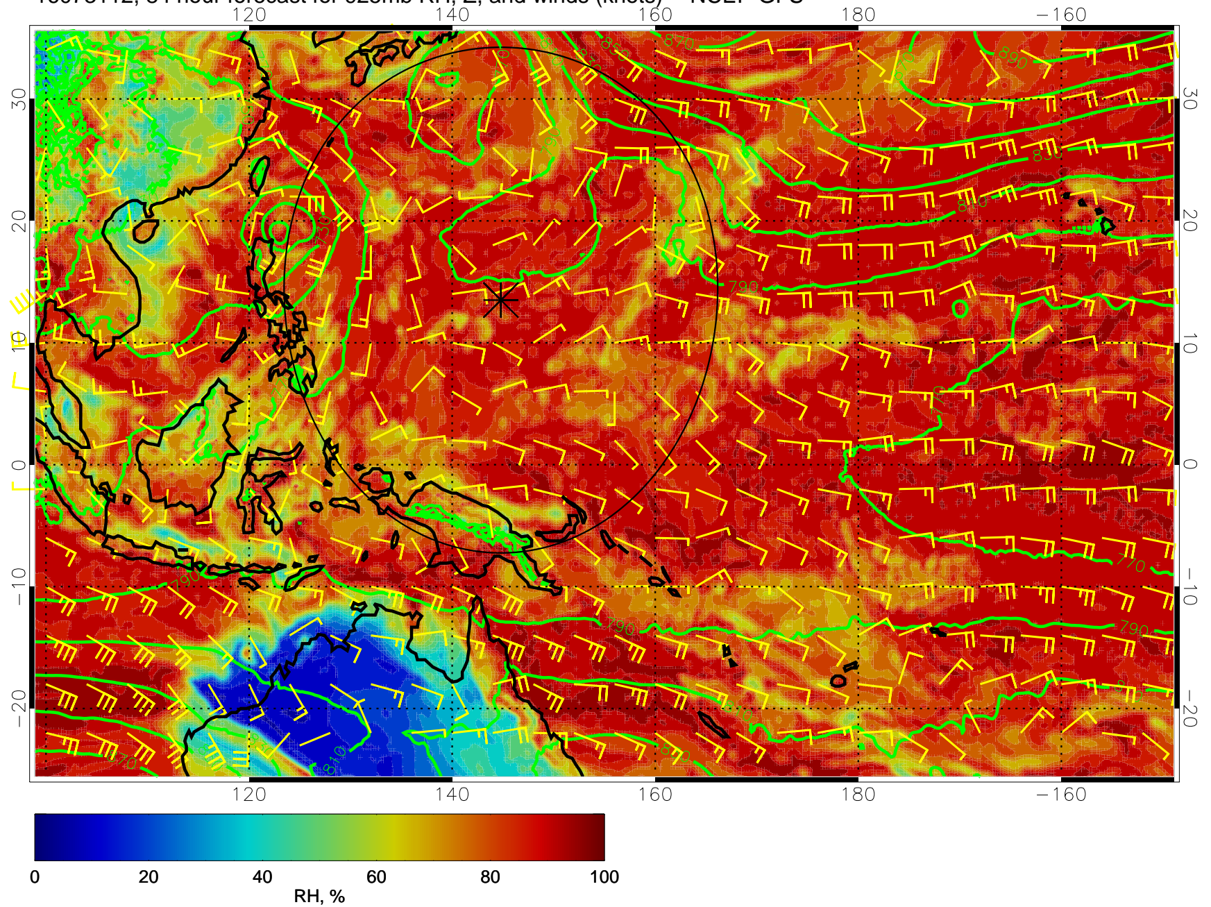
16073112, 84 hour forecast for 925mb RH, Z, and winds (knots) -- NCEP GFS
