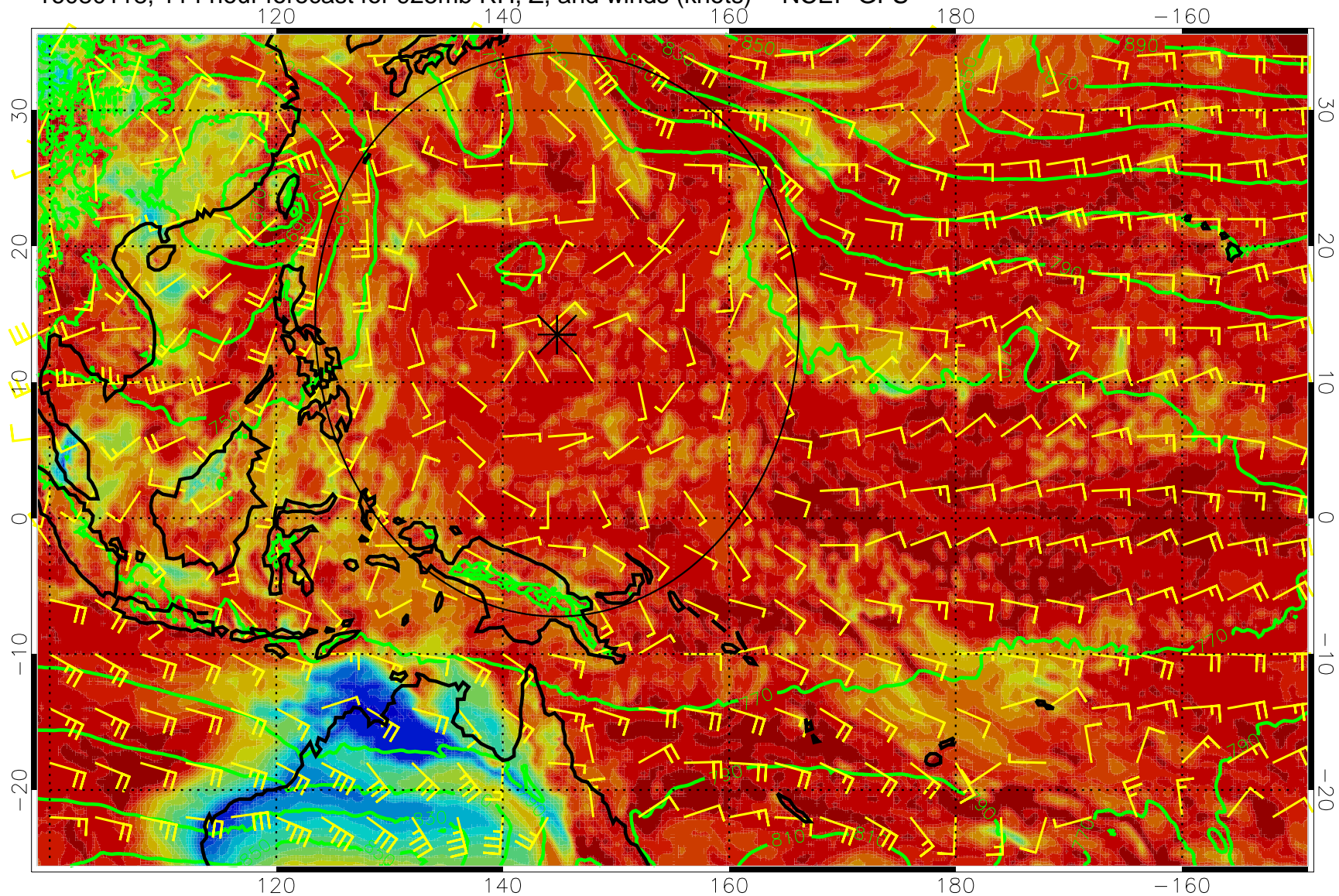
16080118, 114 hour forecast for 925mb RH, Z, and winds (knots) -- NCEP GFS
