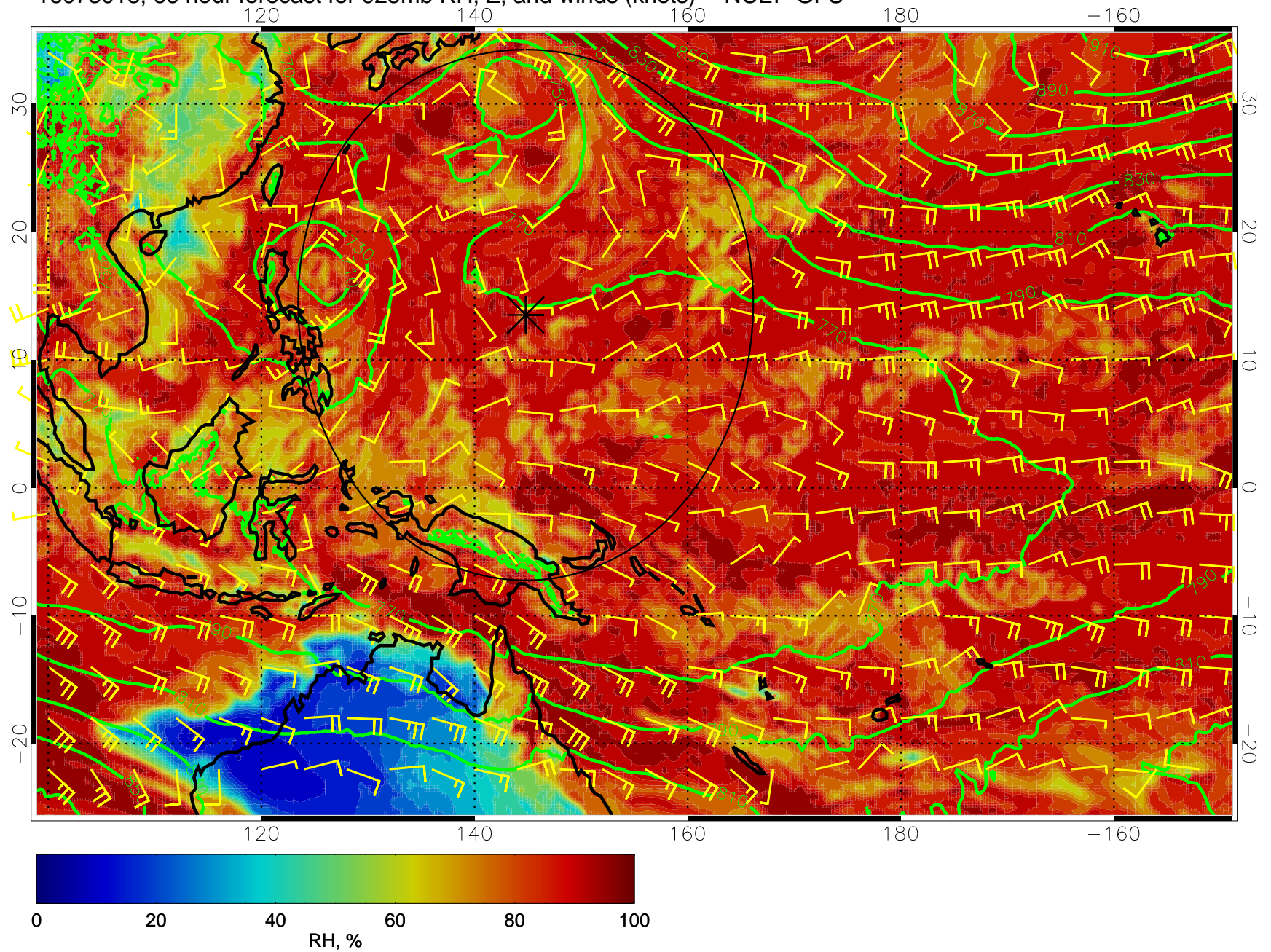
16073018, 66 hour forecast for 925mb RH, Z, and winds (knots) -- NCEP GFS
