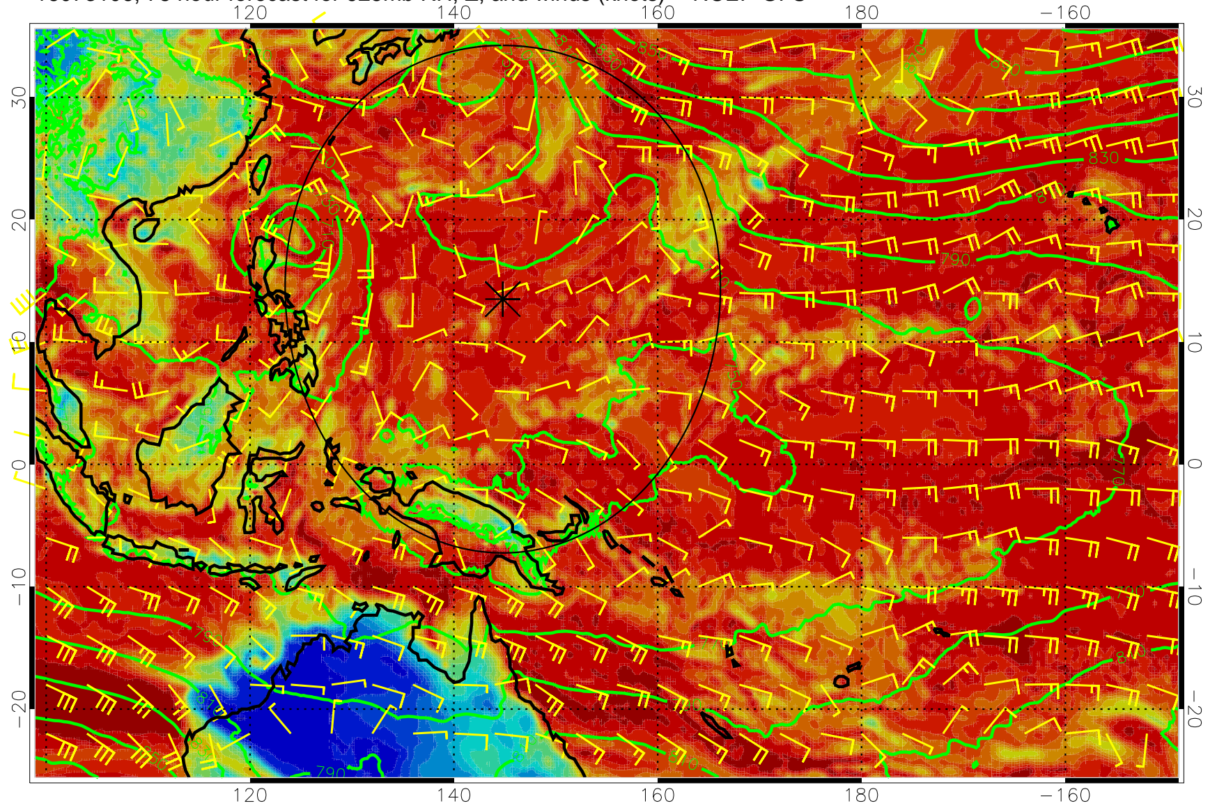
16073106, 78 hour forecast for 925mb RH, Z, and winds (knots) -- NCEP GFS
