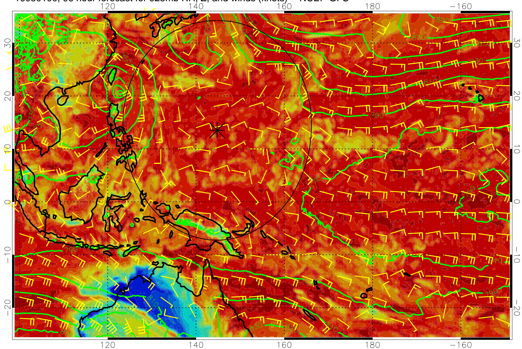
16080100, 96 hour forecast for 925mb RH, Z, and winds (knots) -- NCEP GFS
