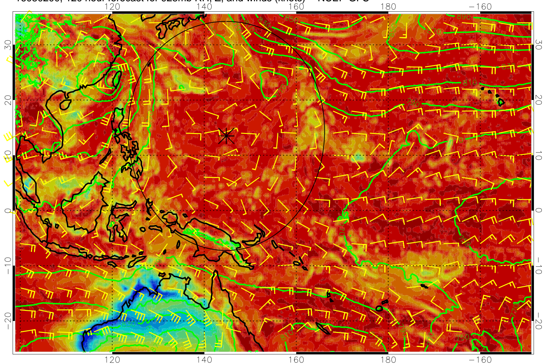
16080200, 120 hour forecast for 925mb RH, Z, and winds (knots) -- NCEP GFS
