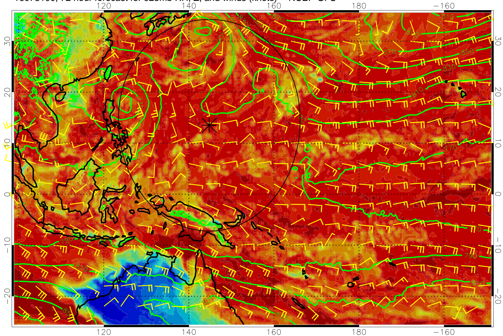
16073100, 72 hour forecast for 925mb RH, Z, and winds (knots) -- NCEP GFS
