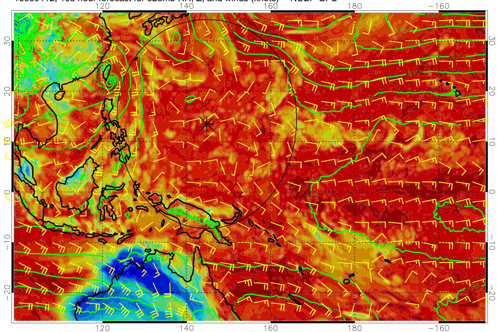
16080112, 108 hour forecast for 925mb RH, Z, and winds (knots) -- NCEP GFS
