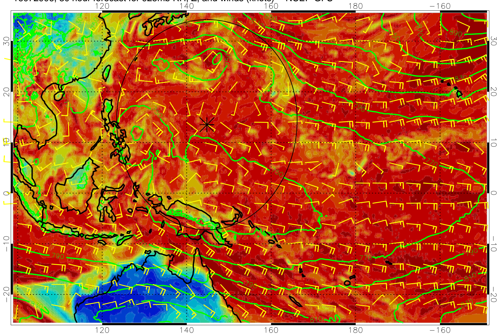
16072906, 30 hour forecast for 925mb RH, Z, and winds (knots) -- NCEP GFS
