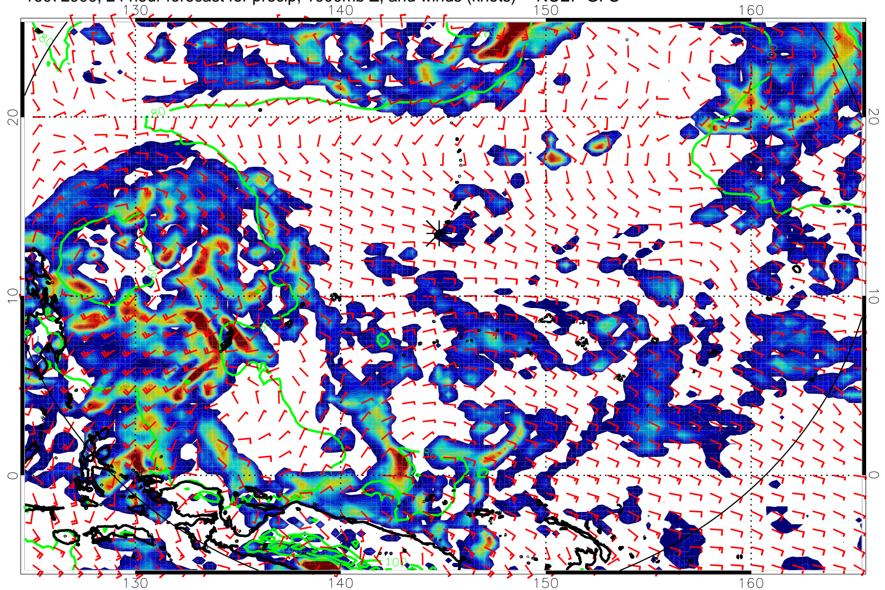
16072900, 24 hour forecast for precip, 1000mb Z, and winds (knots) -- NCEP GFS
