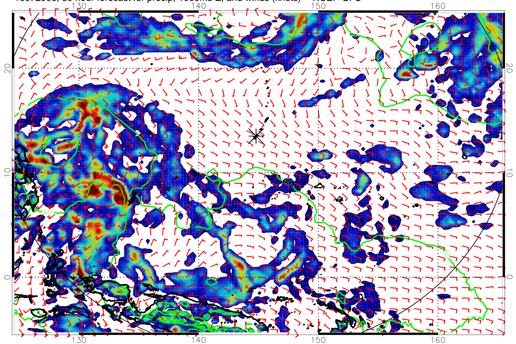
16072906, 30 hour forecast for precip, 1000mb Z, and winds (knots) -- NCEP GFS
