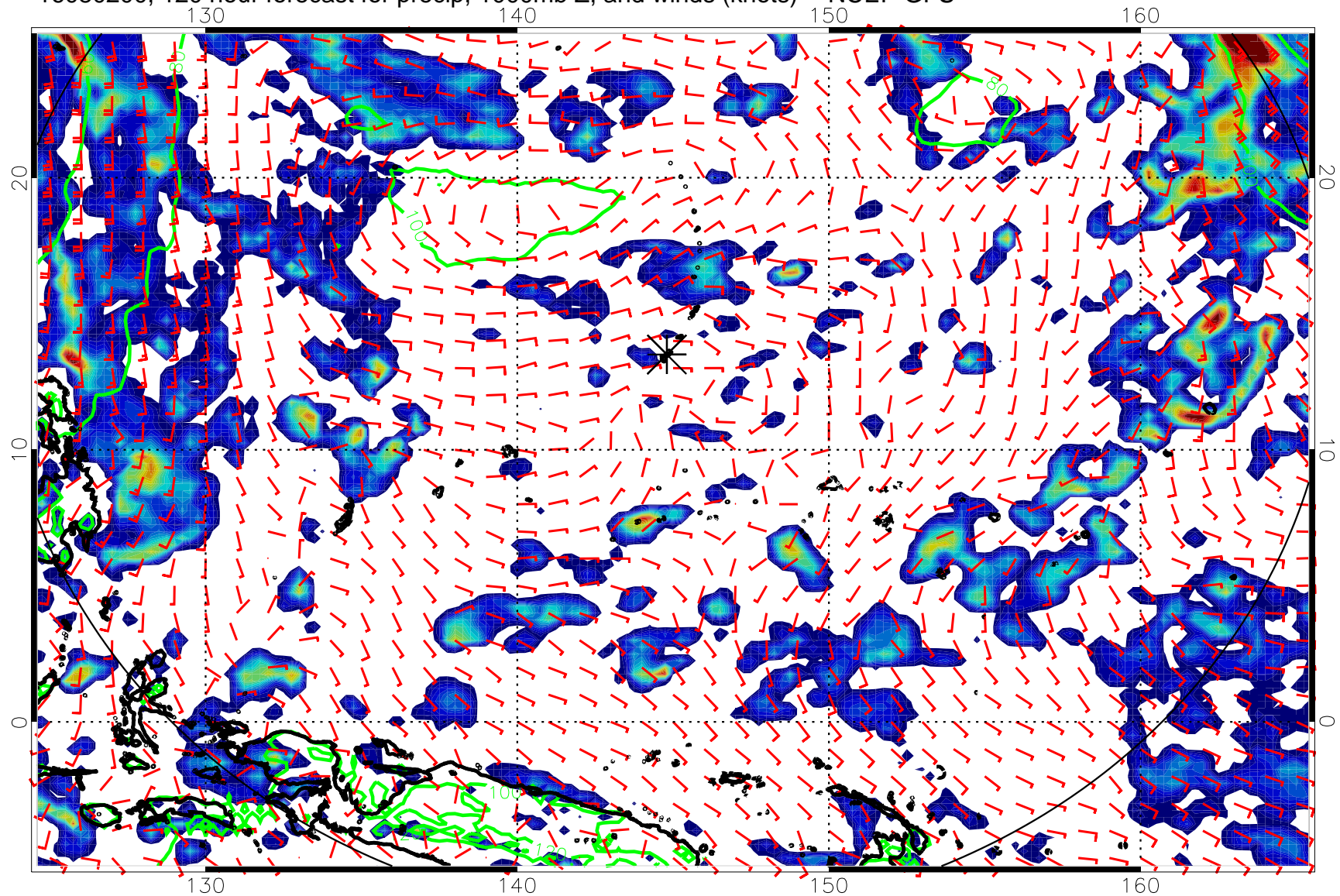
16080200, 120 hour forecast for precip, 1000mb Z, and winds (knots) -- NCEP GFS
