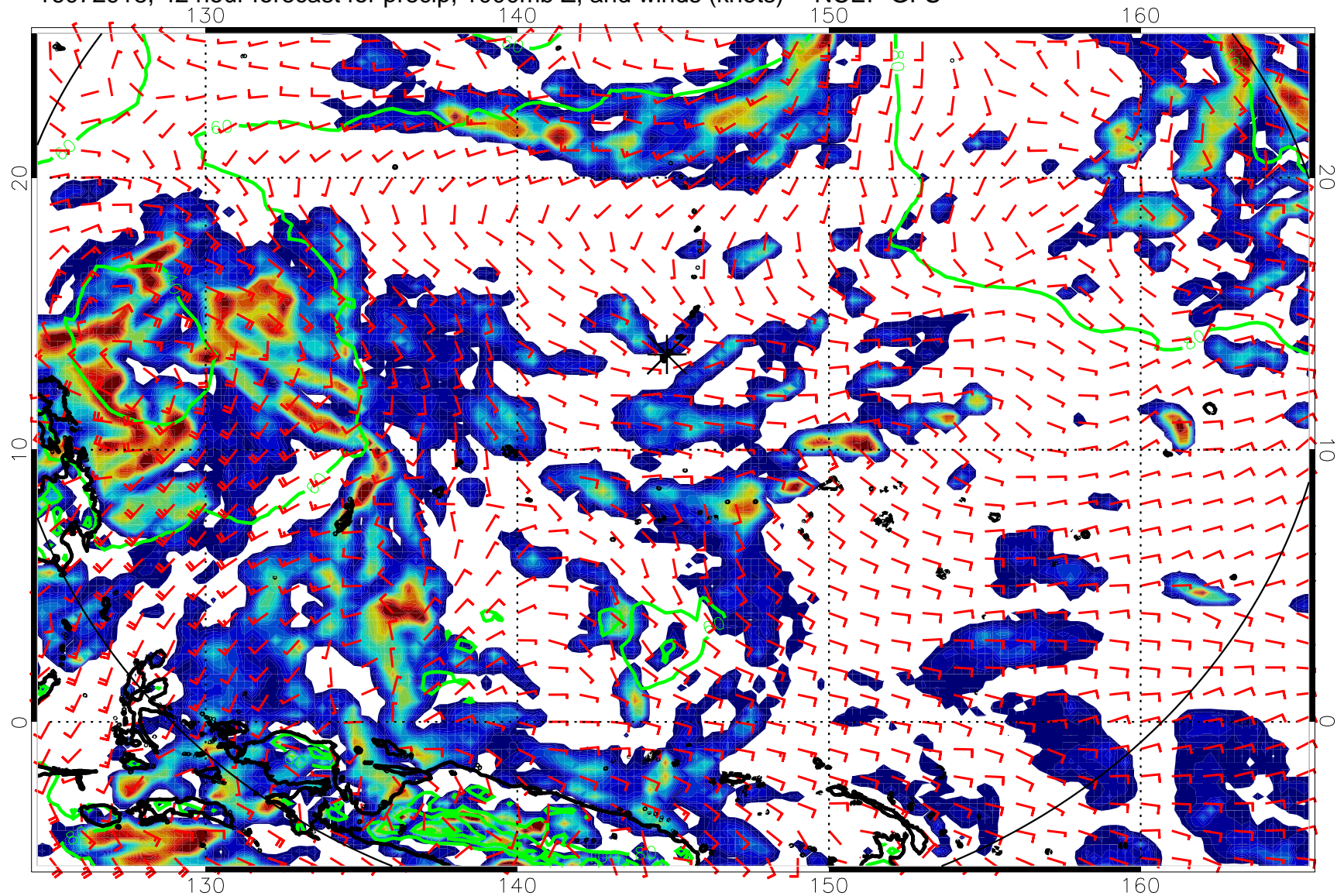
16072918, 42 hour forecast for precip, 1000mb Z, and winds (knots) -- NCEP GFS
