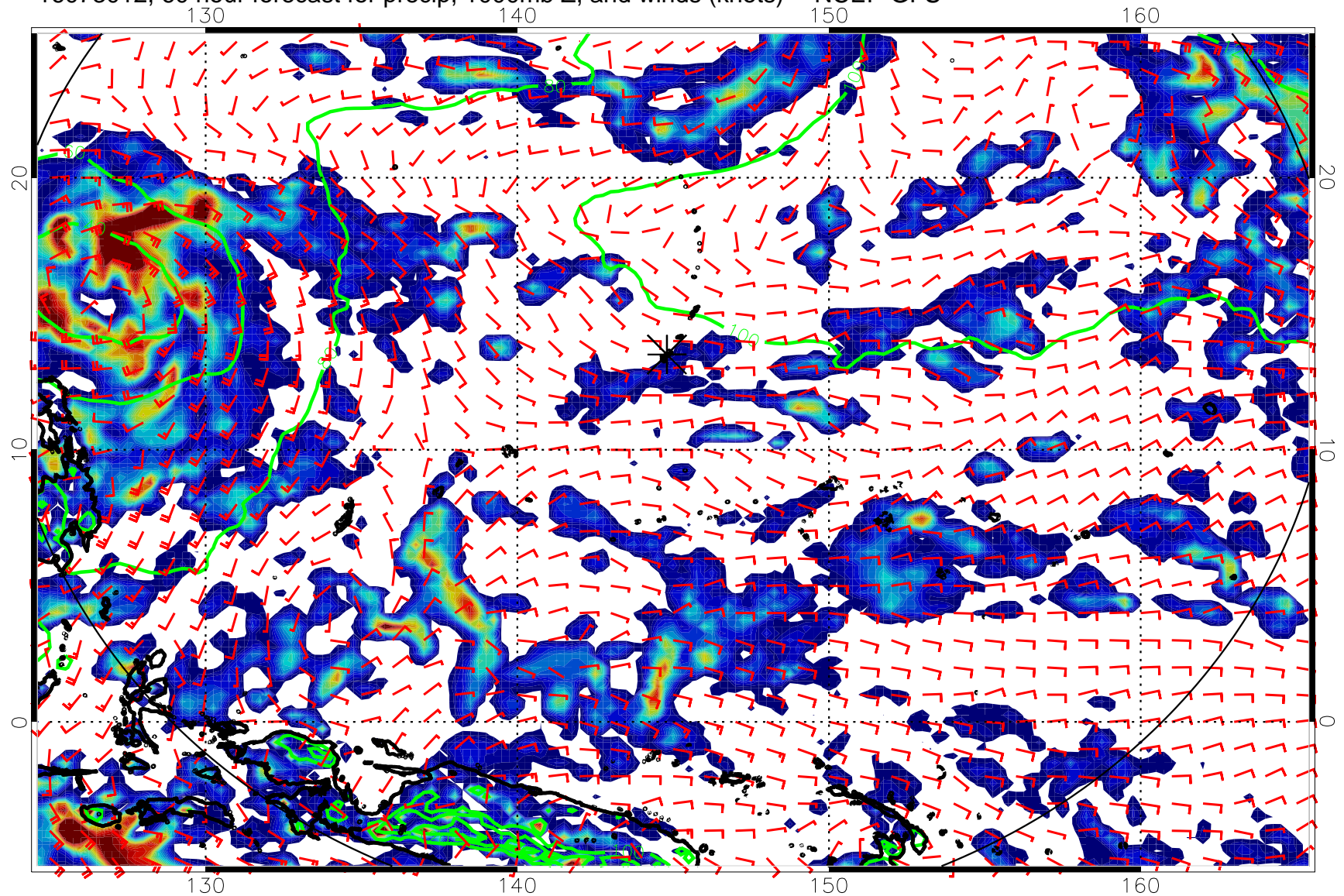
16073012, 60 hour forecast for precip, 1000mb Z, and winds (knots) -- NCEP GFS
