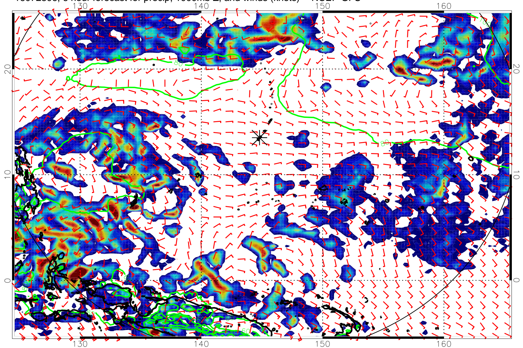
16072806, 6 hour forecast for precip, 1000mb Z, and winds (knots) -- NCEP GFS
