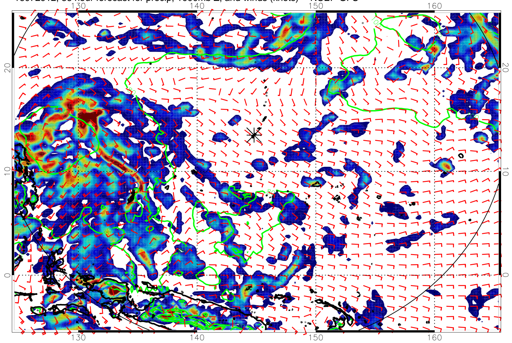
16072912, 36 hour forecast for precip, 1000mb Z, and winds (knots) -- NCEP GFS
