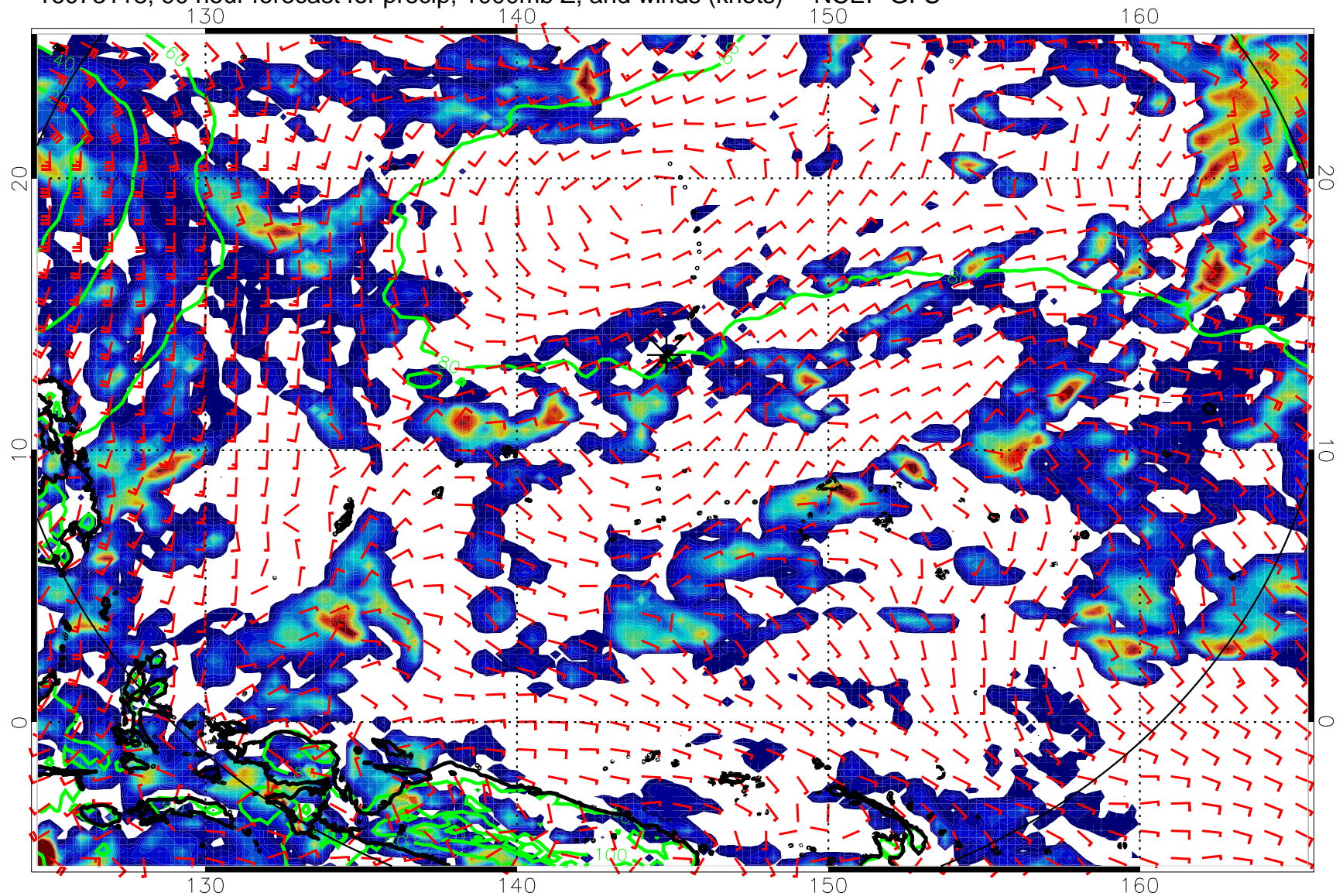
16073118, 90 hour forecast for precip, 1000mb Z, and winds (knots) -- NCEP GFS
