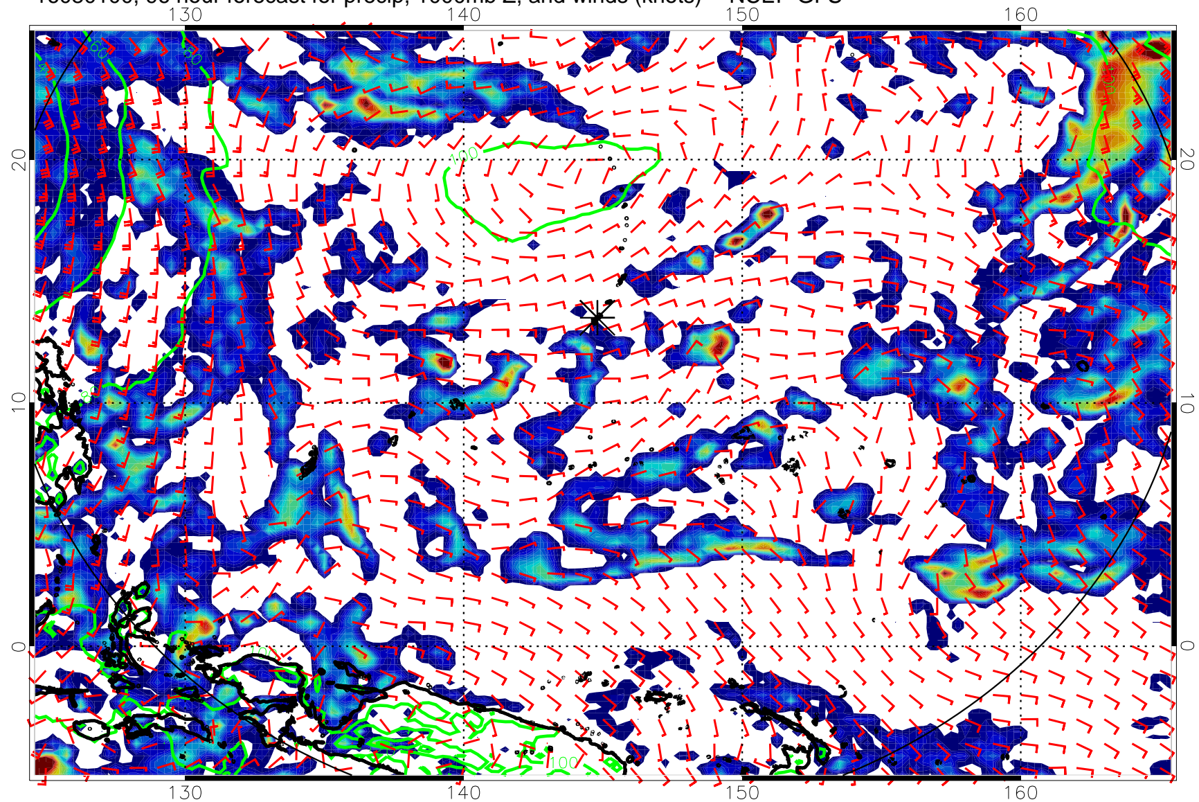
16080100, 96 hour forecast for precip, 1000mb Z, and winds (knots) -- NCEP GFS
