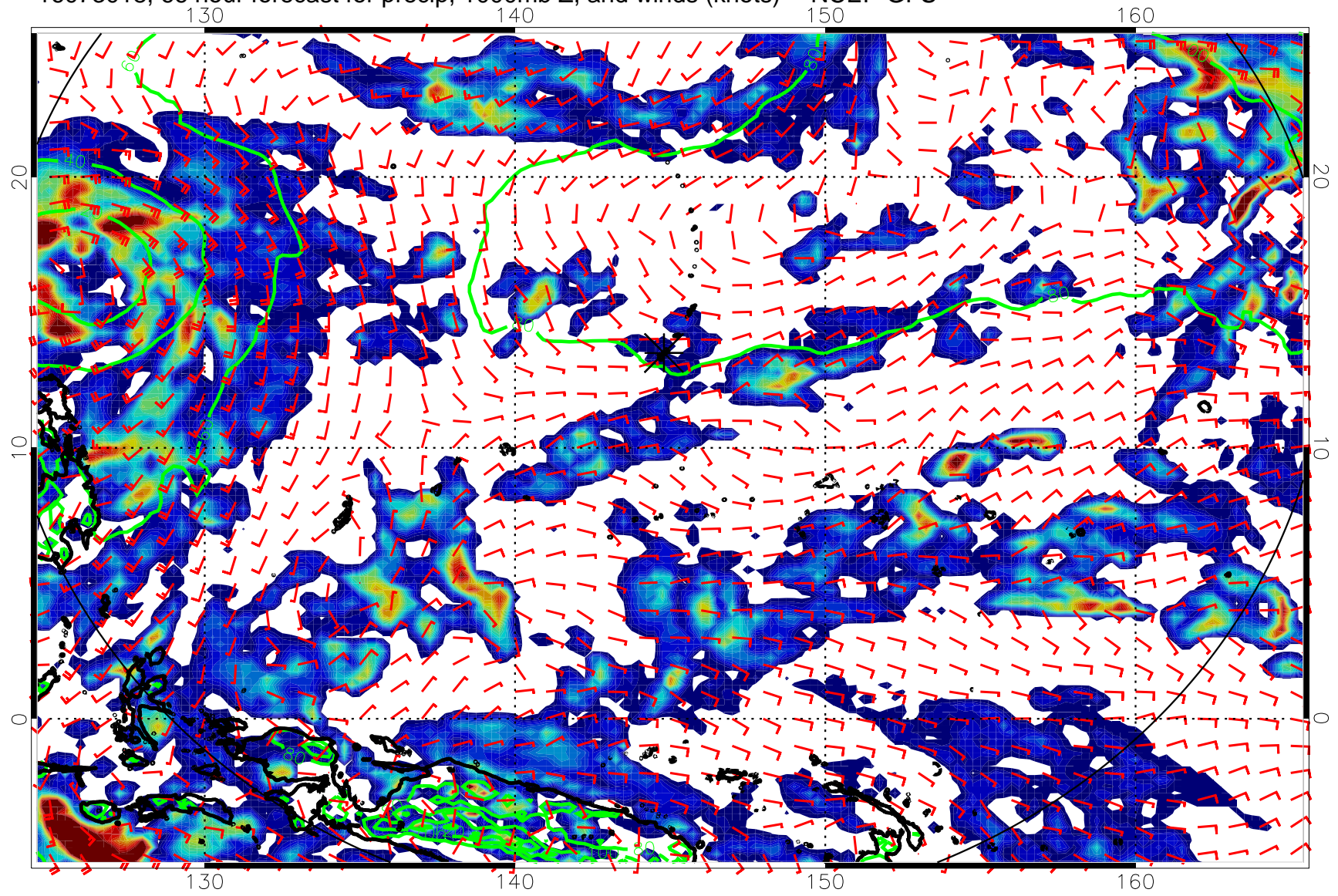
16073018, 66 hour forecast for precip, 1000mb Z, and winds (knots) -- NCEP GFS
