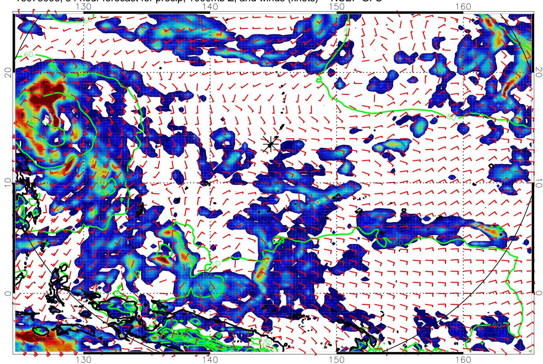
16073006, 54 hour forecast for precip, 1000mb Z, and winds (knots) -- NCEP GFS
