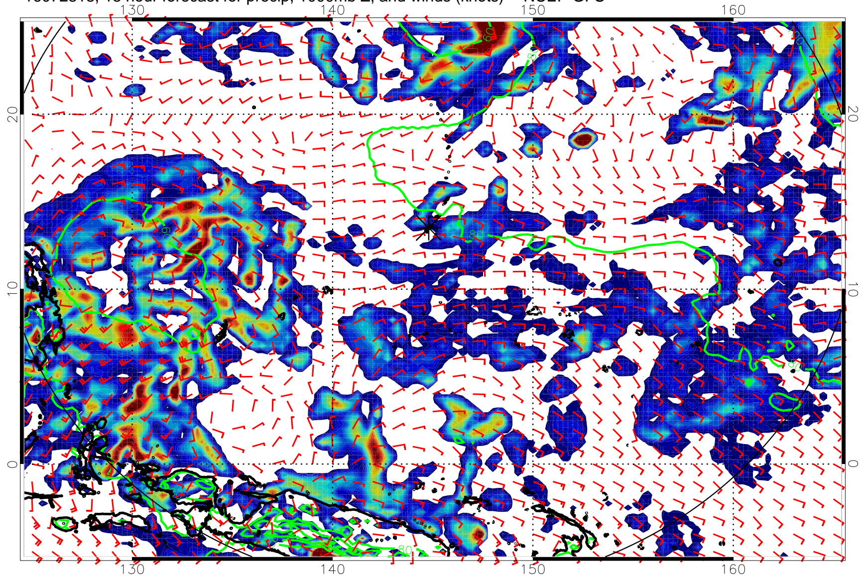
16072818, 18 hour forecast for precip, 1000mb Z, and winds (knots) -- NCEP GFS
