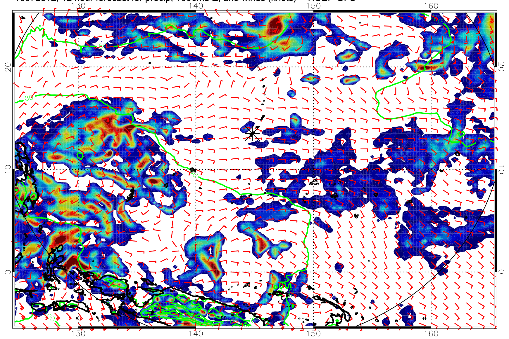
16072812, 12 hour forecast for precip, 1000mb Z, and winds (knots) -- NCEP GFS
