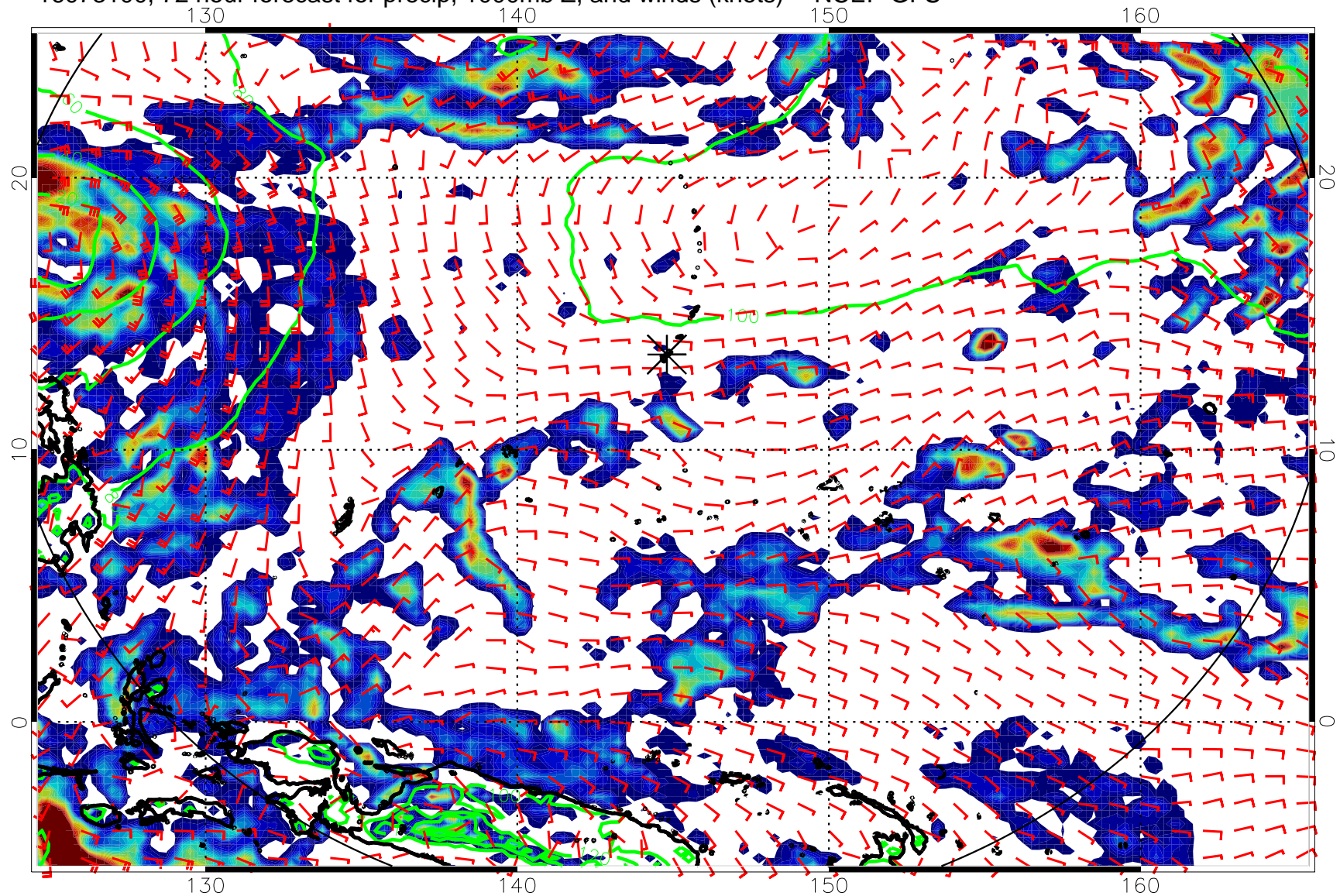
16073100, 72 hour forecast for precip, 1000mb Z, and winds (knots) -- NCEP GFS
