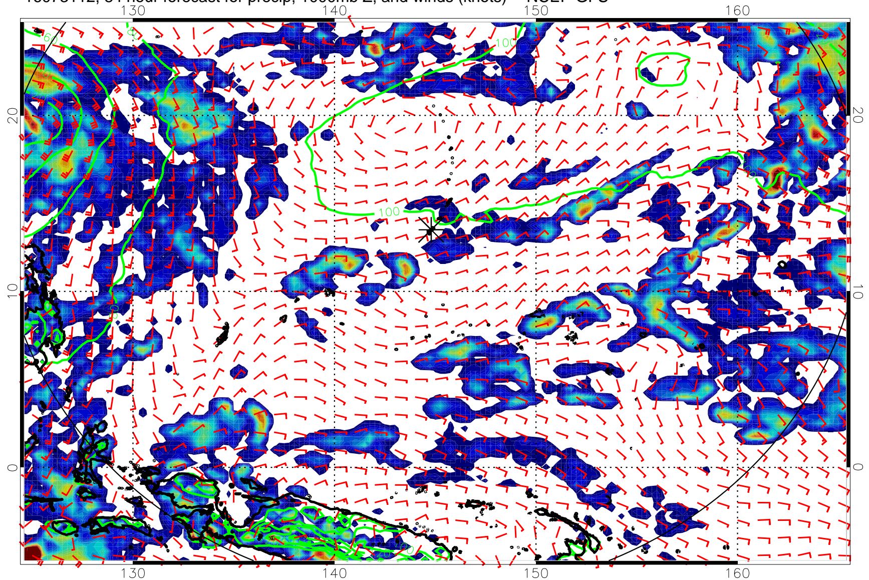
16073112, 84 hour forecast for precip, 1000mb Z, and winds (knots) -- NCEP GFS
