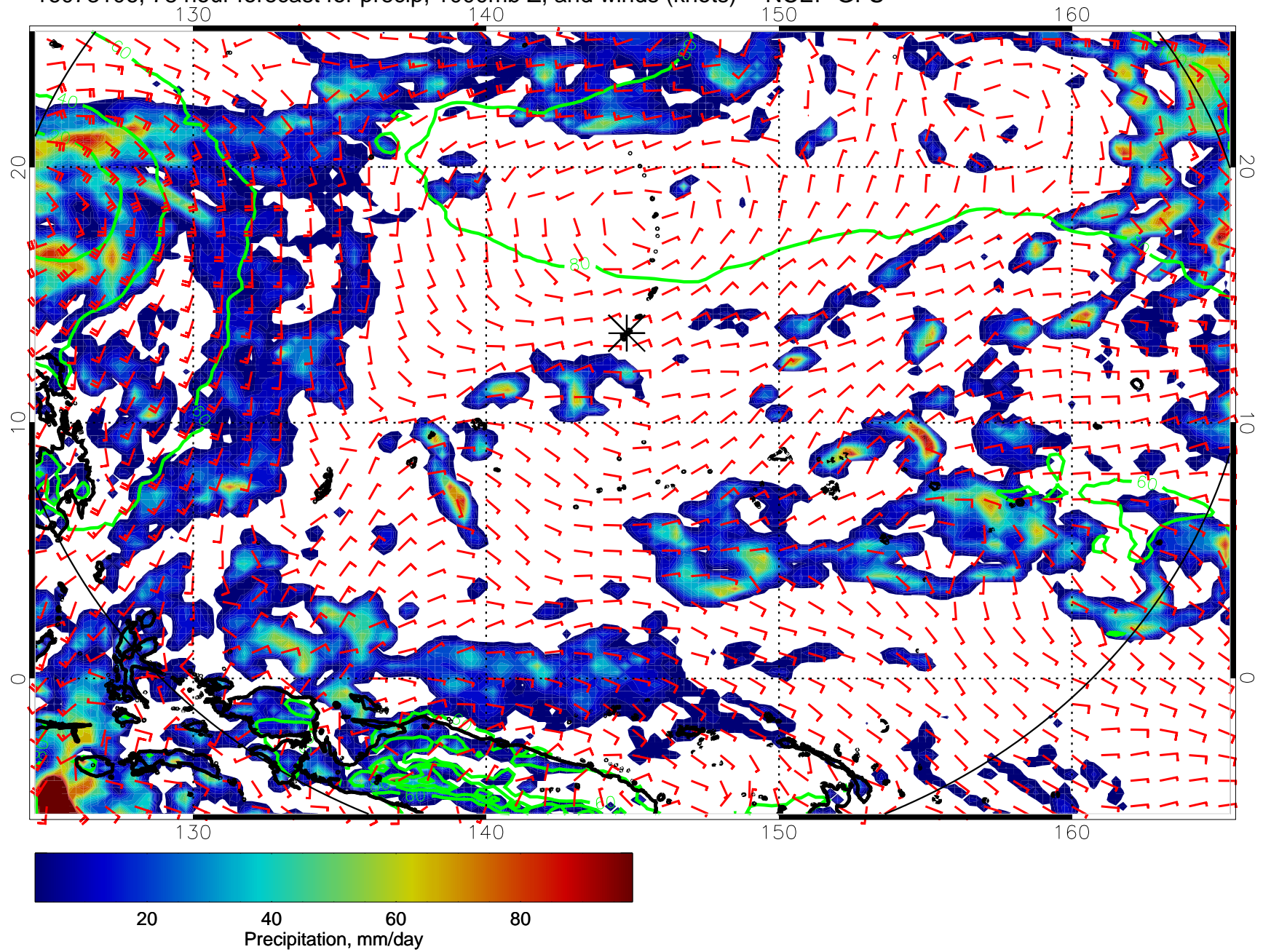
16073106, 78 hour forecast for precip, 1000mb Z, and winds (knots) -- NCEP GFS
