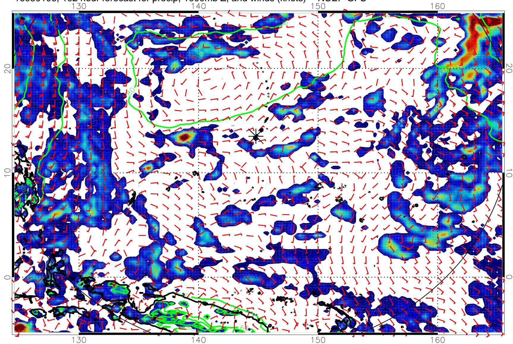
16080106, 102 hour forecast for precip, 1000mb Z, and winds (knots) -- NCEP GFS
