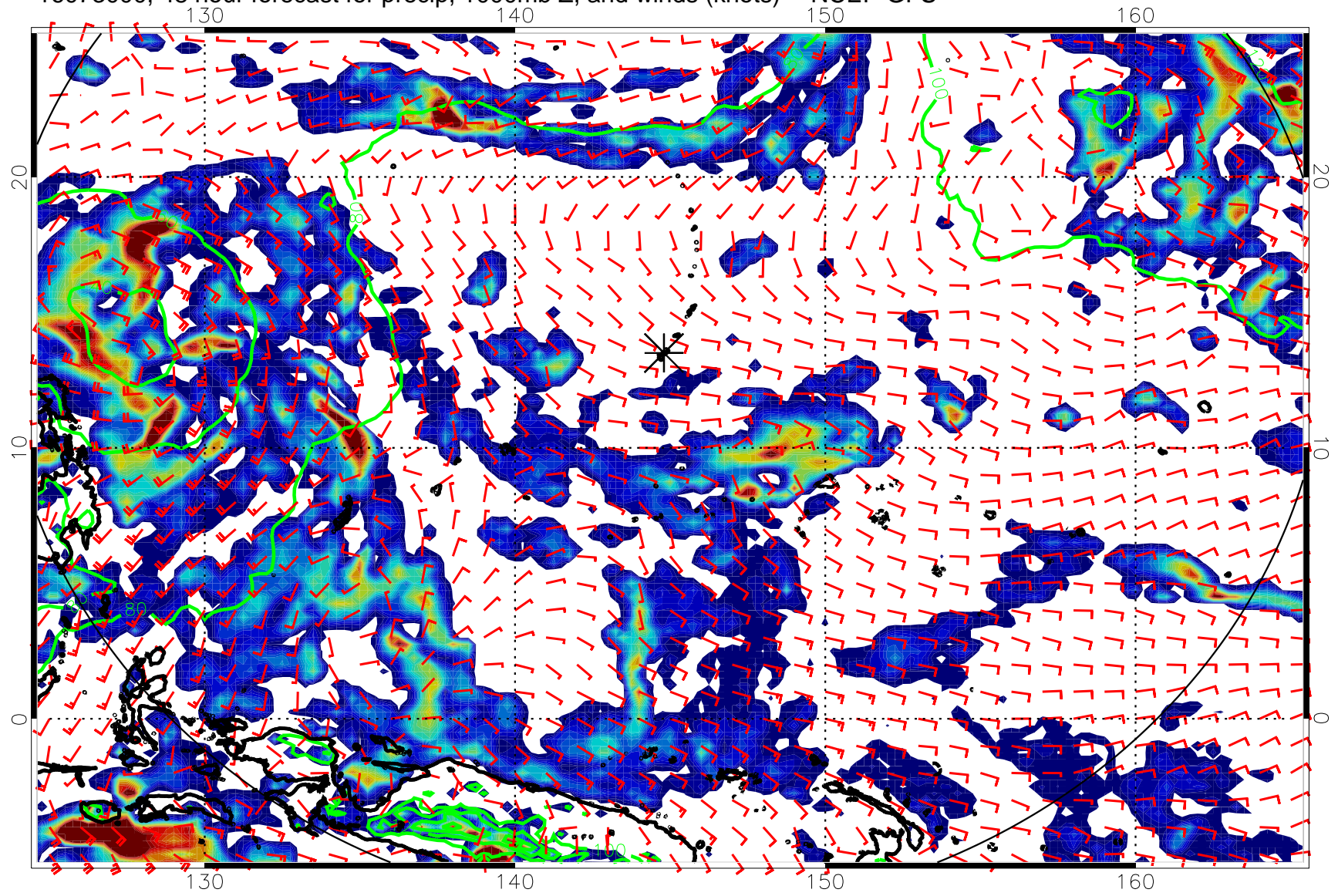
16073000, 48 hour forecast for precip, 1000mb Z, and winds (knots) -- NCEP GFS
