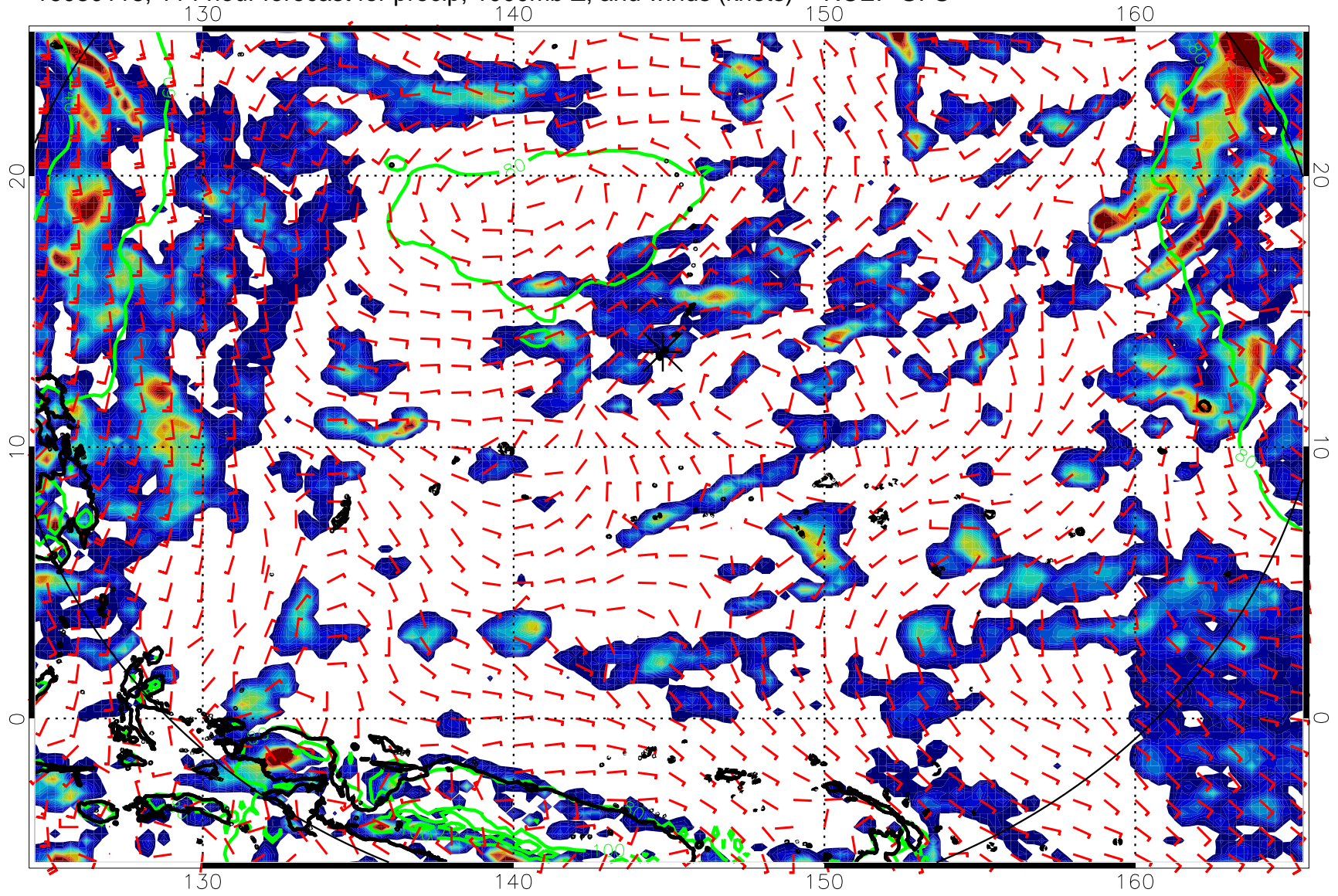
16080118, 114 hour forecast for precip, 1000mb Z, and winds (knots) -- NCEP GFS
