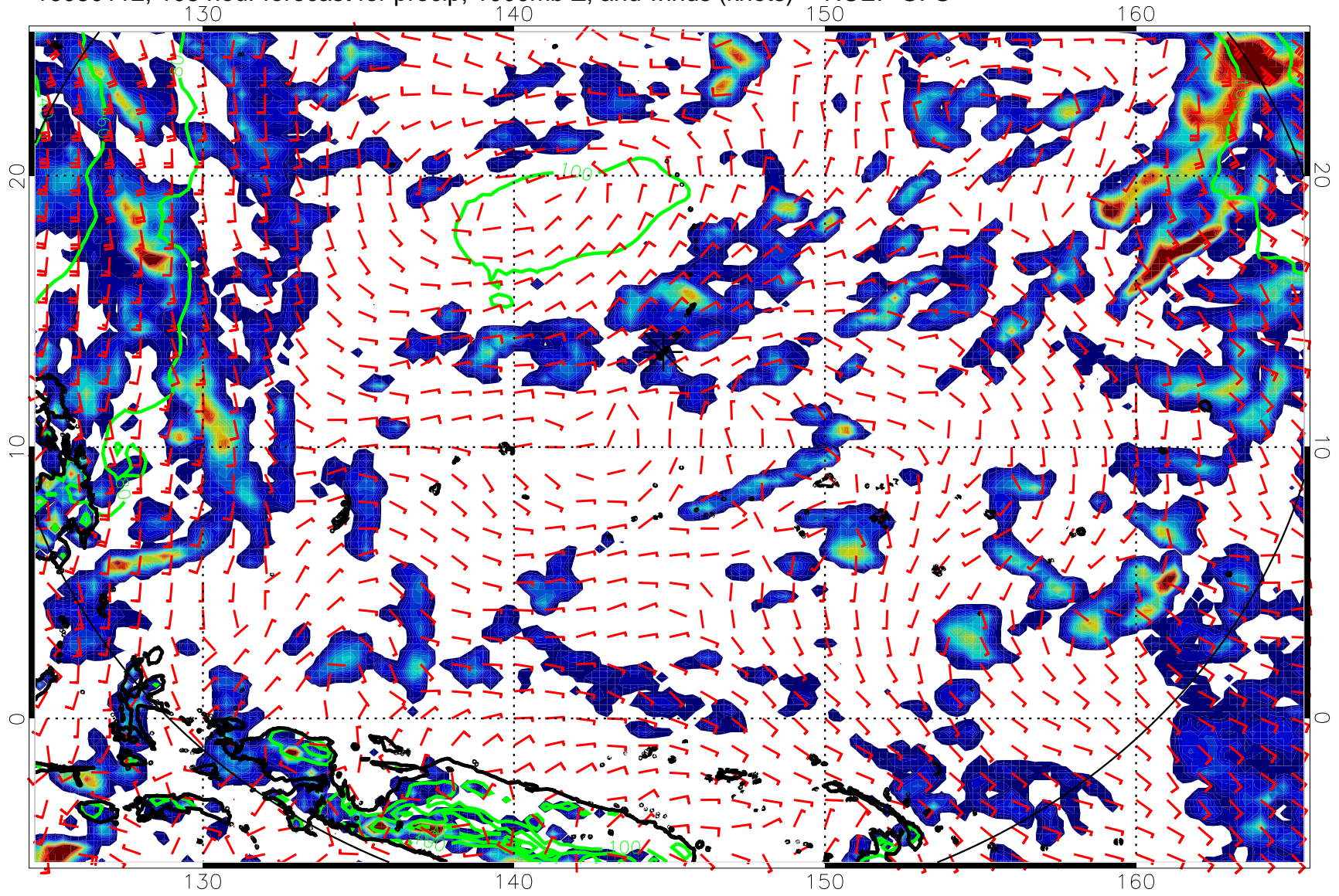
16080112, 108 hour forecast for precip, 1000mb Z, and winds (knots) -- NCEP GFS
