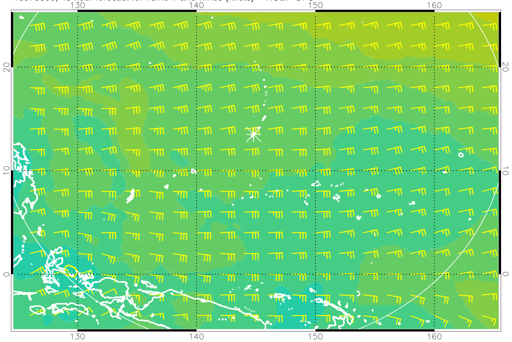
16073000, 48 hour forecast for 70mb T and winds (knots) -- NCEP GFS
