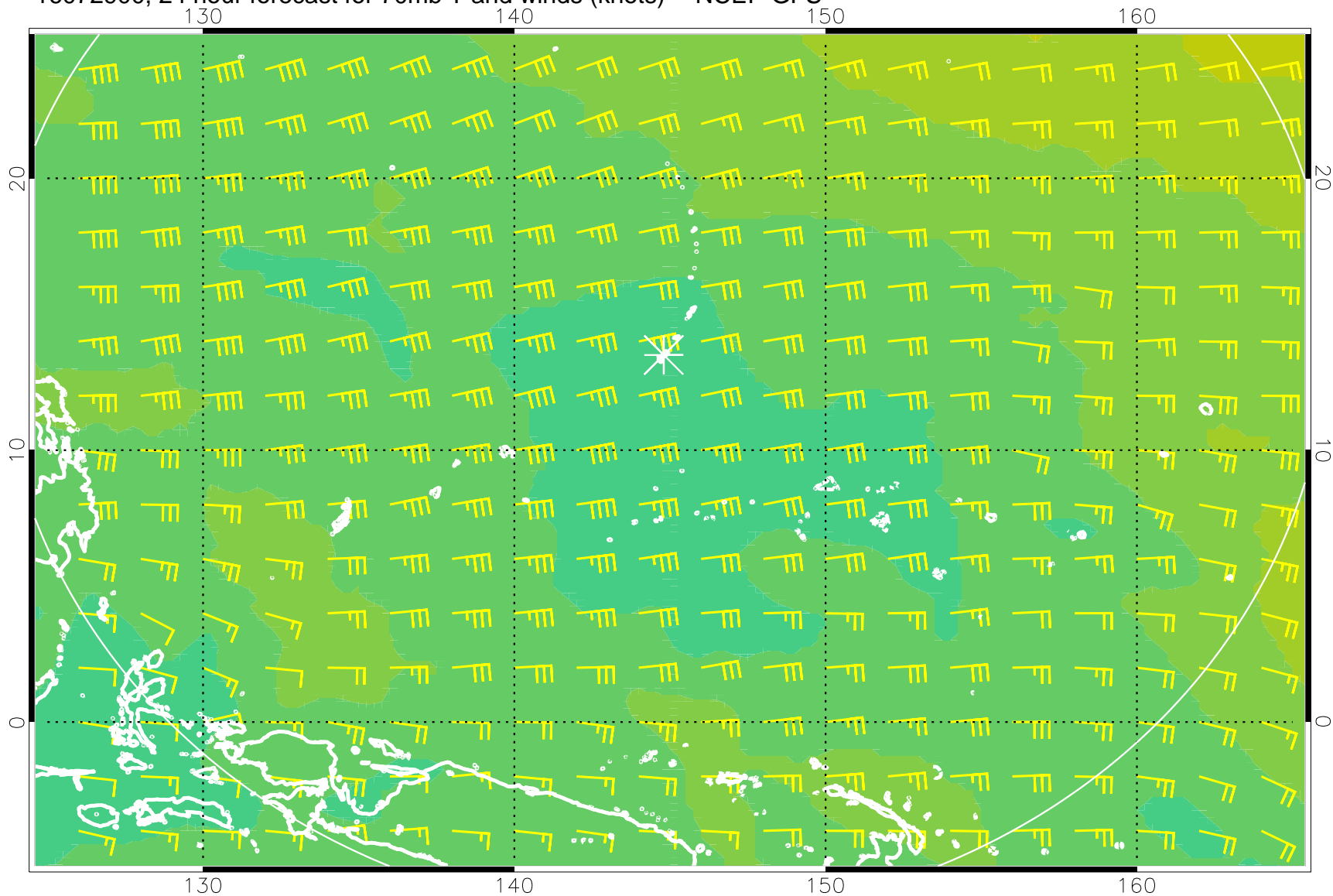
16072900, 24 hour forecast for 70mb T and winds (knots) -- NCEP GFS
