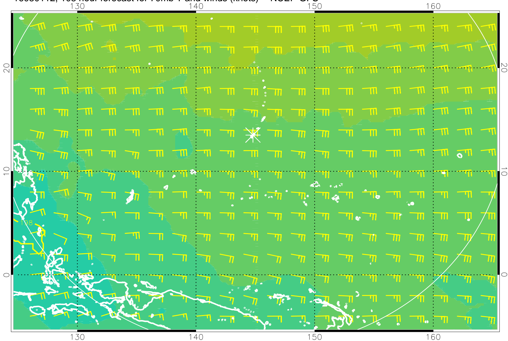
16080112, 108 hour forecast for 70mb T and winds (knots) -- NCEP GFS
