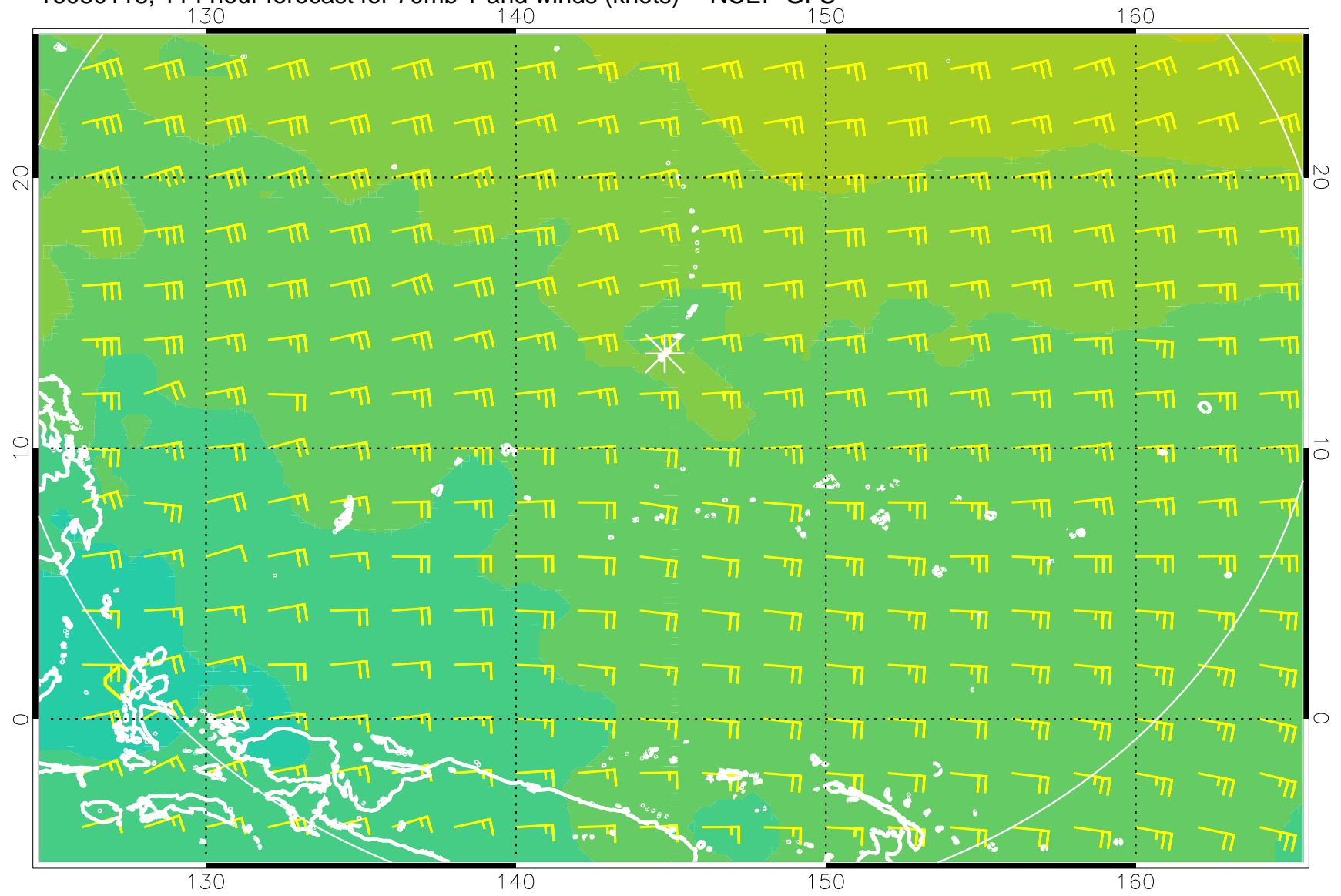
16080118, 114 hour forecast for 70mb T and winds (knots) -- NCEP GFS
