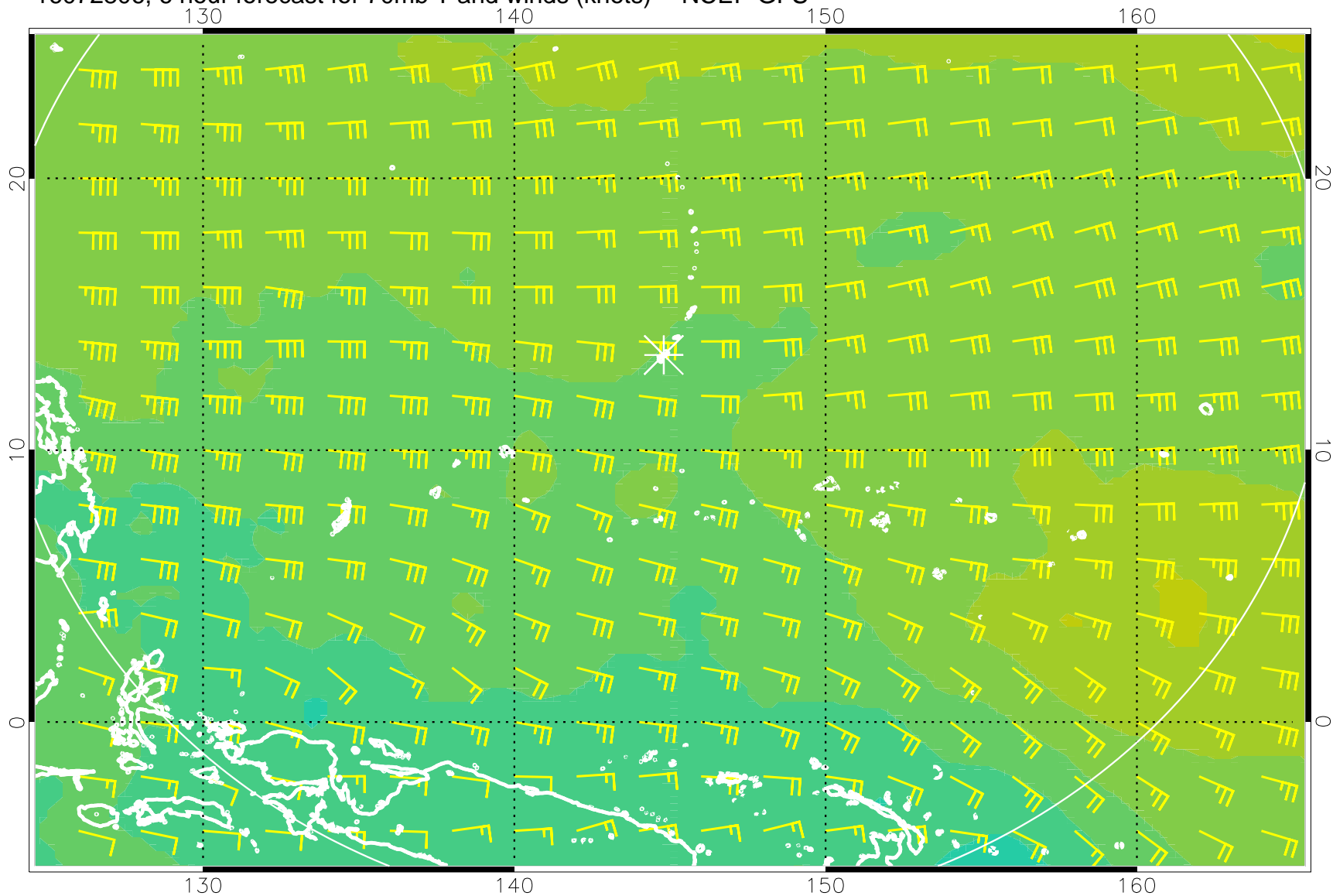
16072806, 6 hour forecast for 70mb T and winds (knots) -- NCEP GFS
