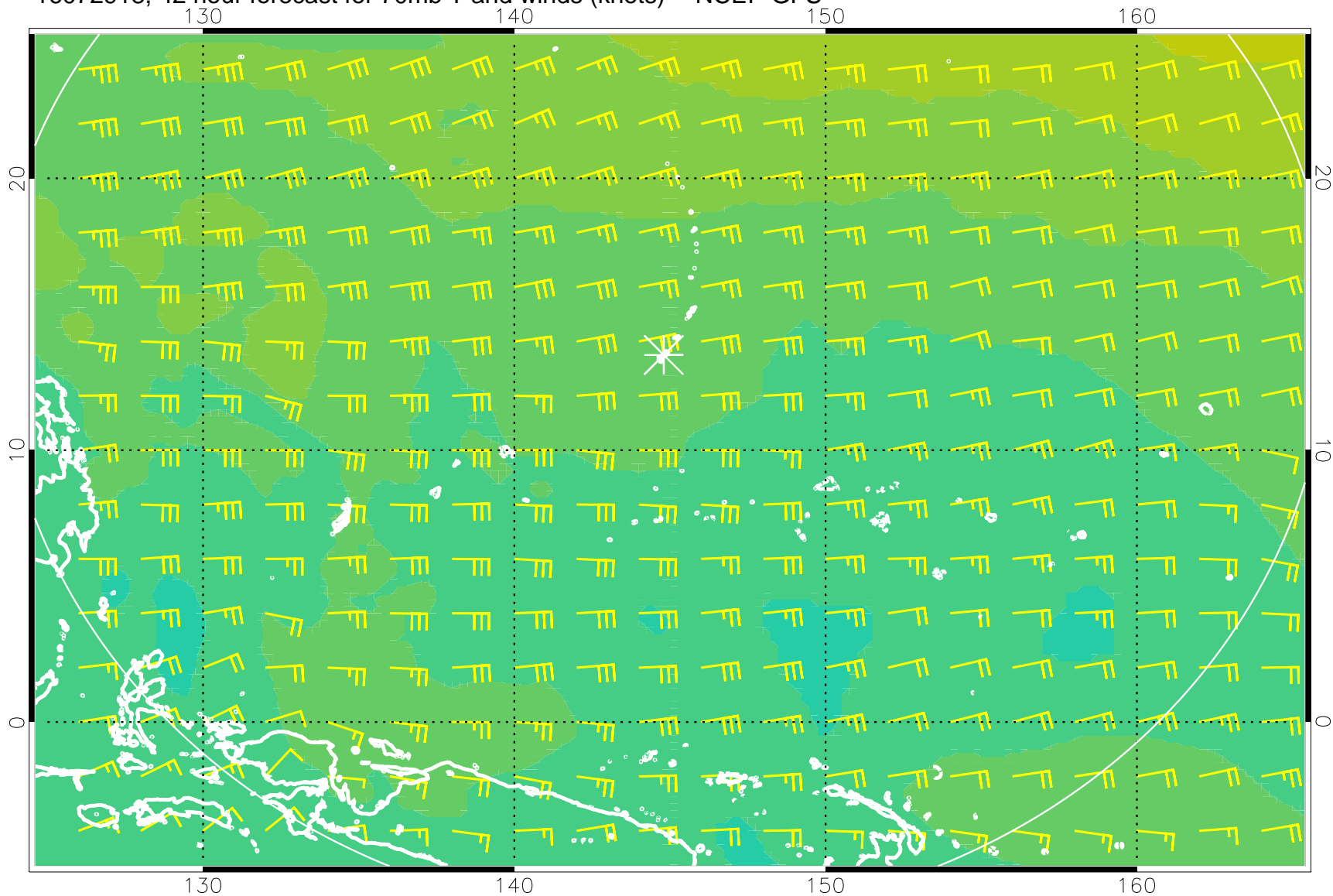
16072918, 42 hour forecast for 70mb T and winds (knots) -- NCEP GFS
