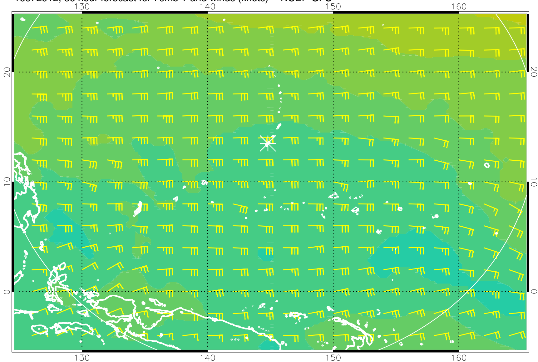
16072912, 36 hour forecast for 70mb T and winds (knots) -- NCEP GFS
