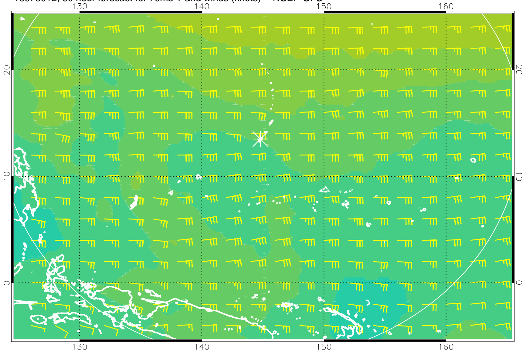
16073012, 60 hour forecast for 70mb T and winds (knots) -- NCEP GFS
