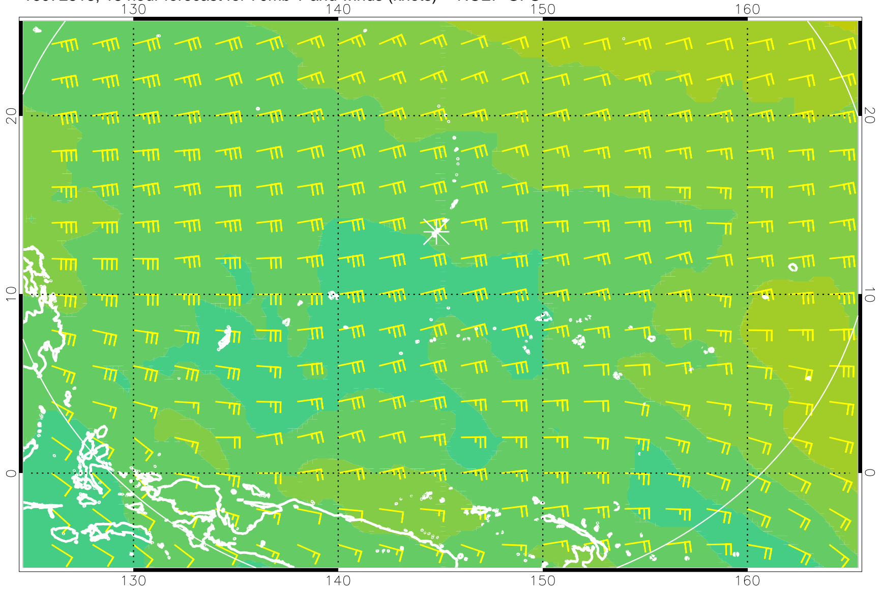
16072818, 18 hour forecast for 70mb T and winds (knots) -- NCEP GFS
