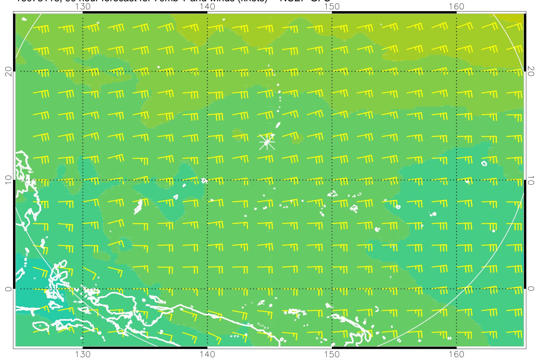
16073118, 90 hour forecast for 70mb T and winds (knots) -- NCEP GFS
