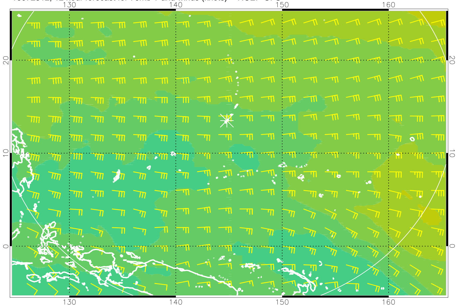
16072812, 12 hour forecast for 70mb T and winds (knots) -- NCEP GFS
