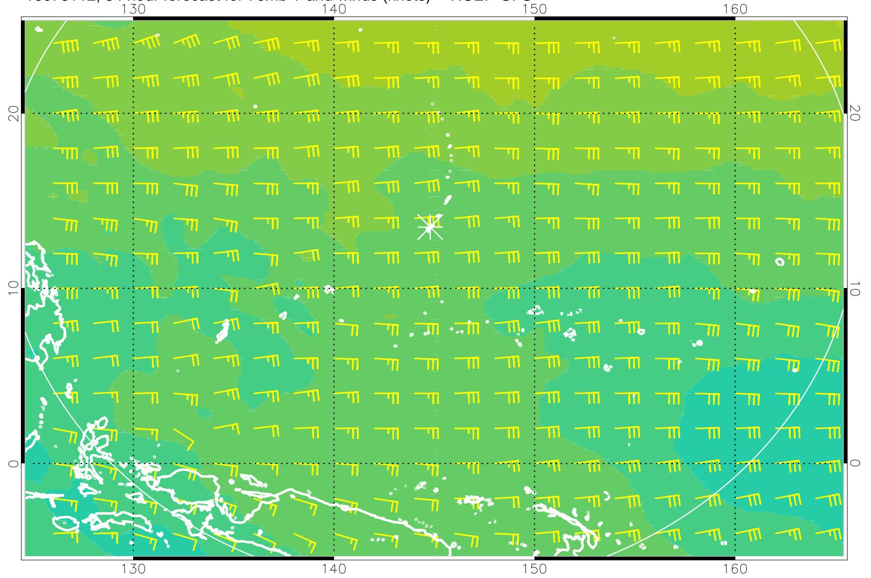
16073112, 84 hour forecast for 70mb T and winds (knots) -- NCEP GFS
