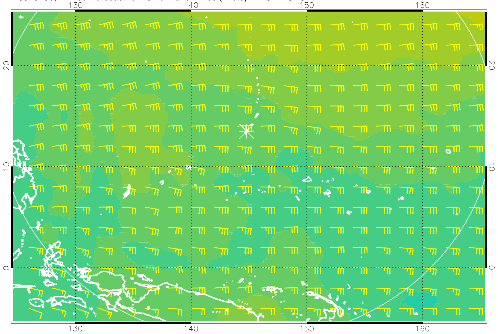
16073100, 72 hour forecast for 70mb T and winds (knots) -- NCEP GFS
