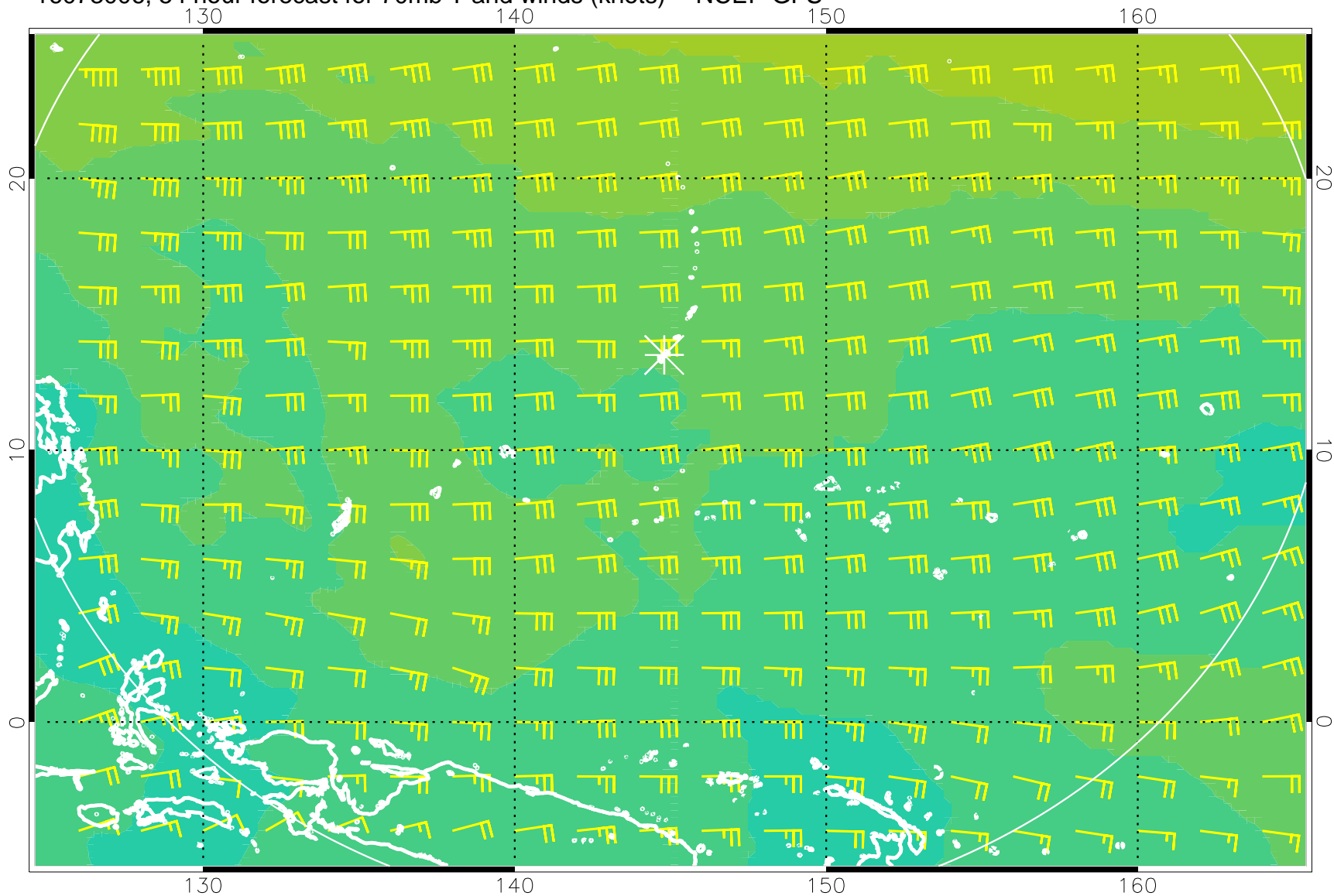
16073006, 54 hour forecast for 70mb T and winds (knots) -- NCEP GFS
