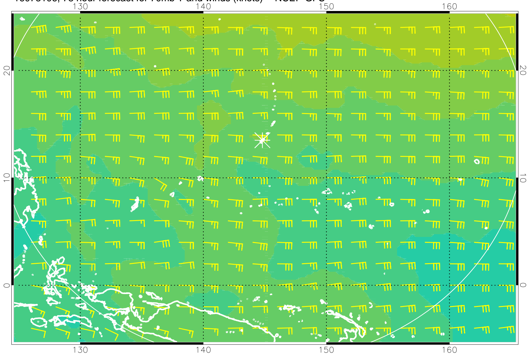
16073106, 78 hour forecast for 70mb T and winds (knots) -- NCEP GFS
