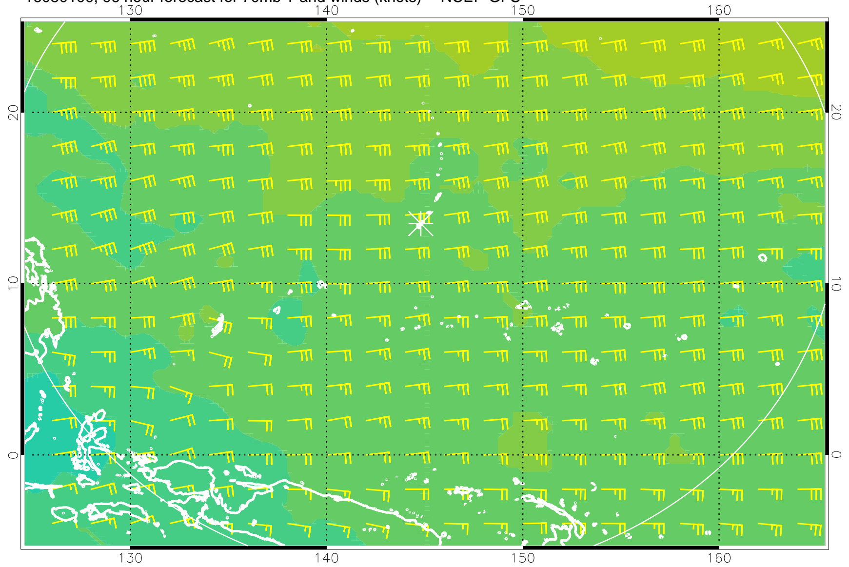
16080100, 96 hour forecast for 70mb T and winds (knots) -- NCEP GFS
