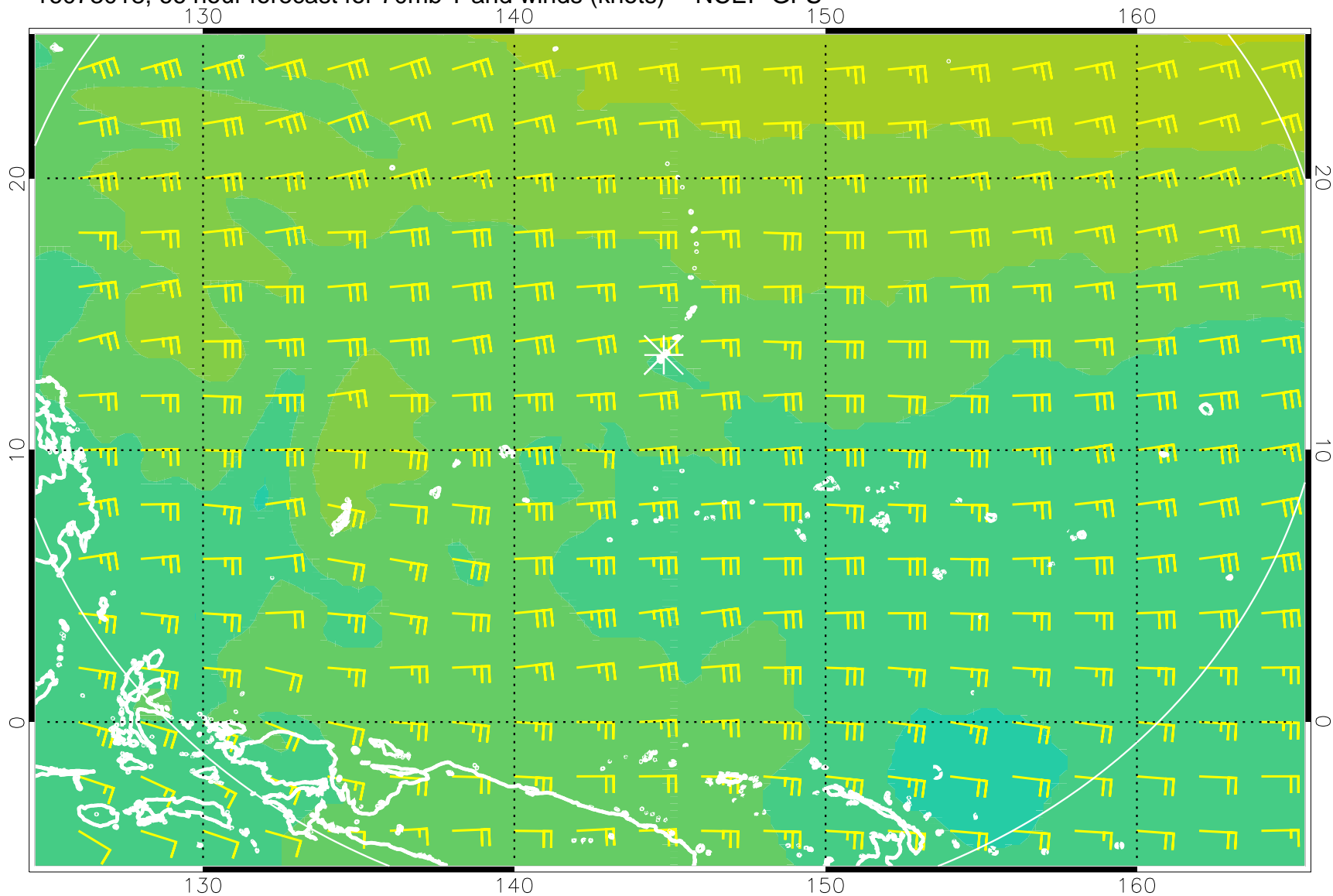
16073018, 66 hour forecast for 70mb T and winds (knots) -- NCEP GFS
