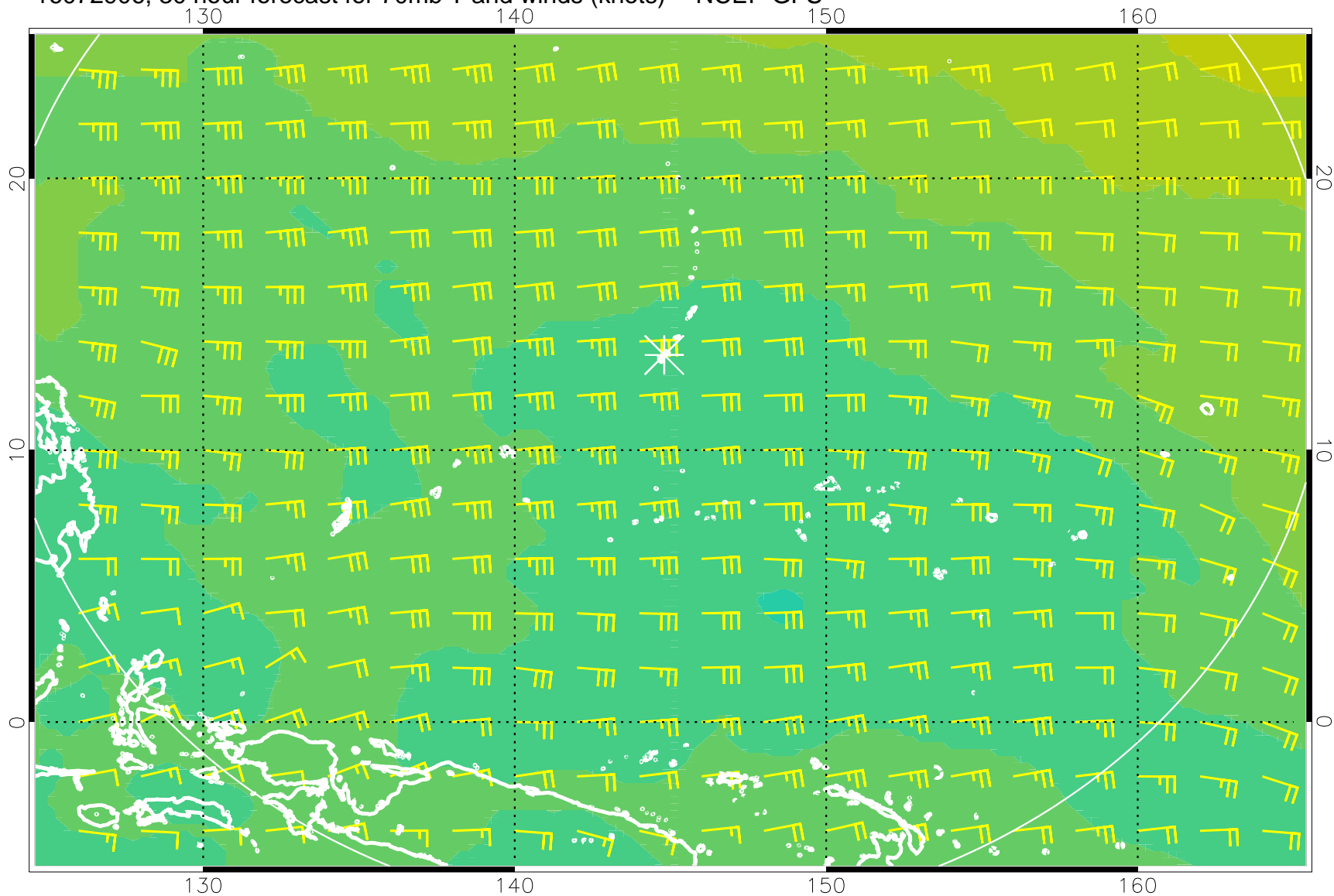
16072906, 30 hour forecast for 70mb T and winds (knots) -- NCEP GFS
