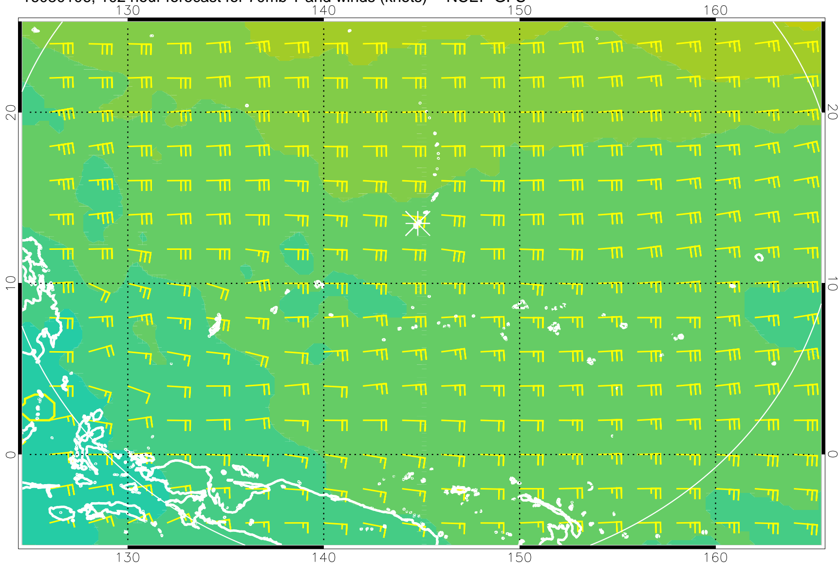
16080106, 102 hour forecast for 70mb T and winds (knots) -- NCEP GFS
