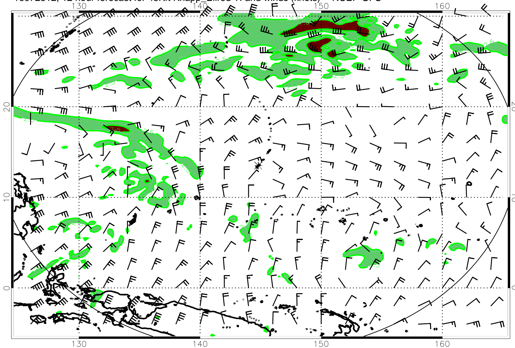
16072812, 12 hour forecast for 45Kft Knapp_Ellrod TI and winds (knots) -- NCEP GFS
