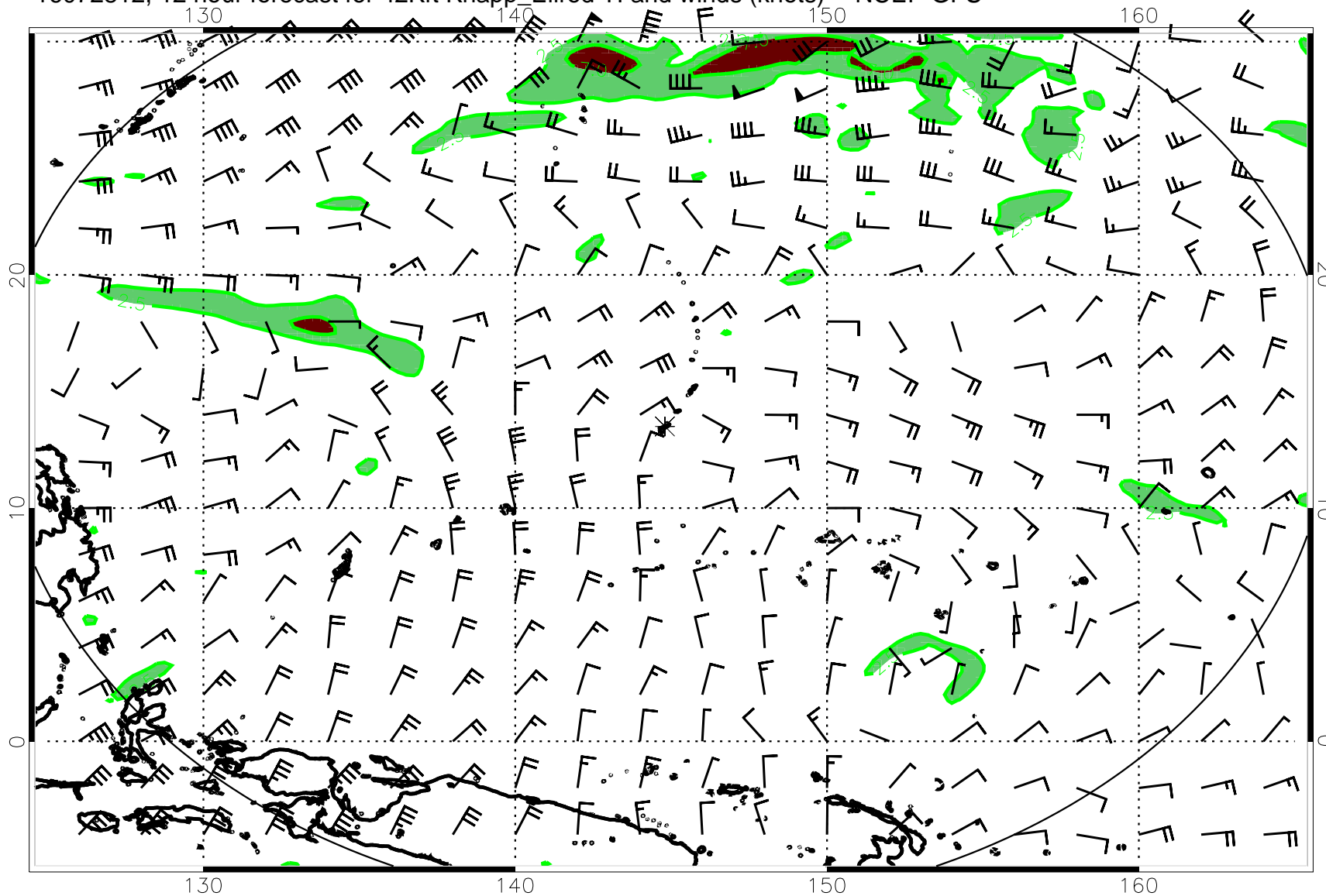
16072812, 12 hour forecast for 42Kft Knapp_Ellrod TI and winds (knots) -- NCEP GFS
