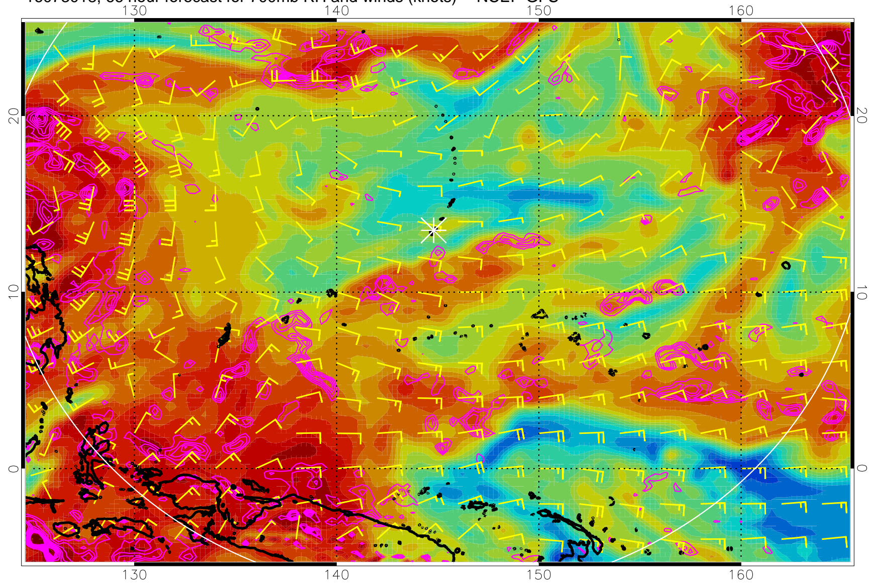
16073018, 66 hour forecast for 700mb RH and winds (knots) -- NCEP GFS
