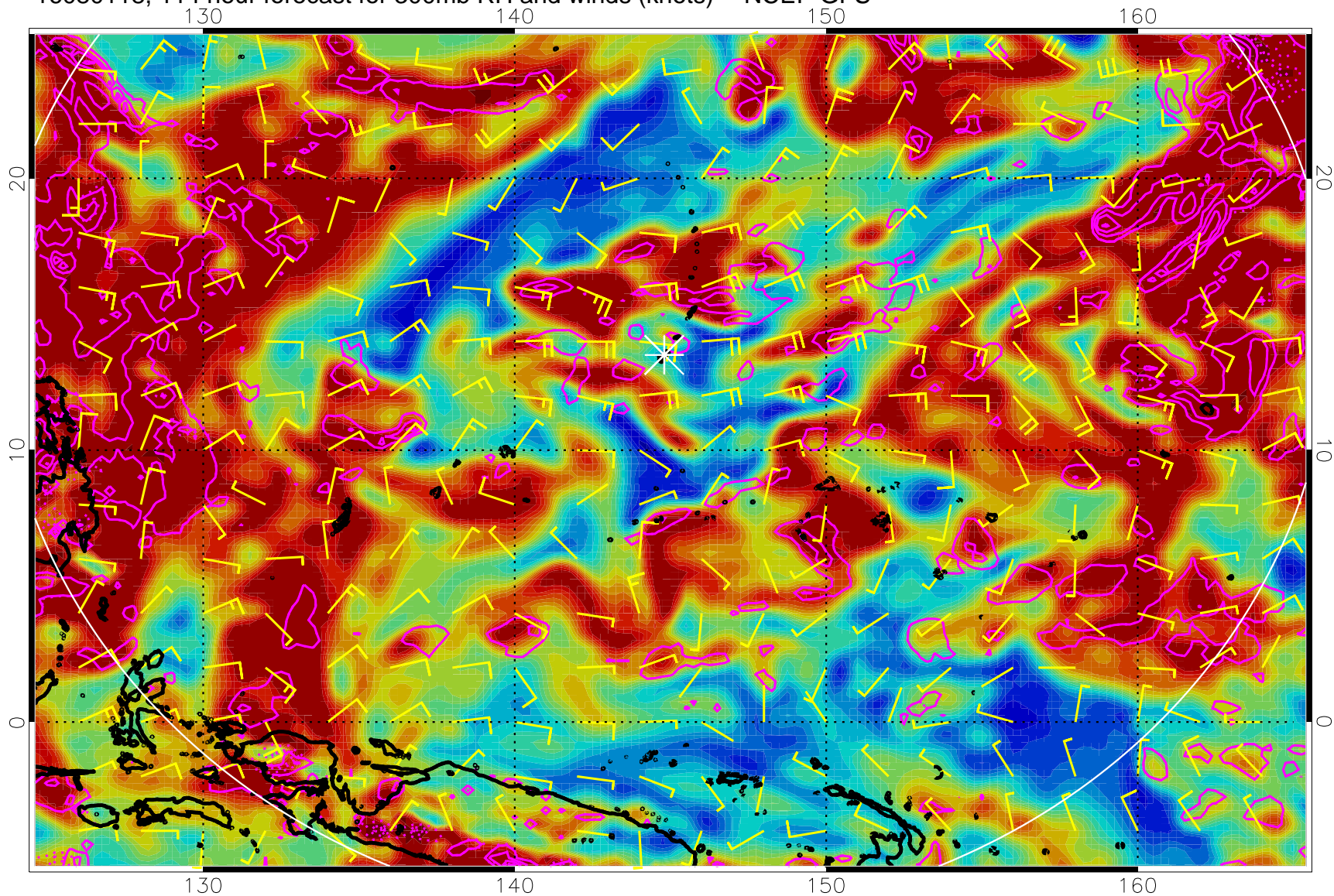
16080118, 114 hour forecast for 300mb RH and winds (knots) -- NCEP GFS
