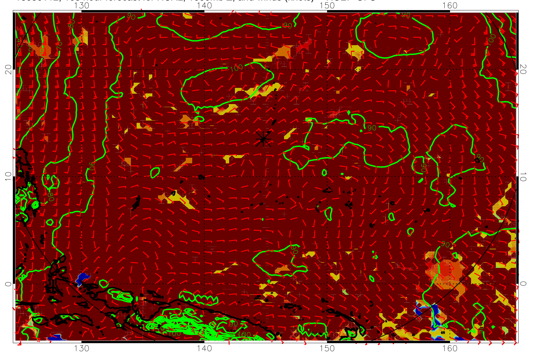
16080112, 108 hour forecast for HCAL, 1000mb Z, and winds (knots) -- NCEP GFS
