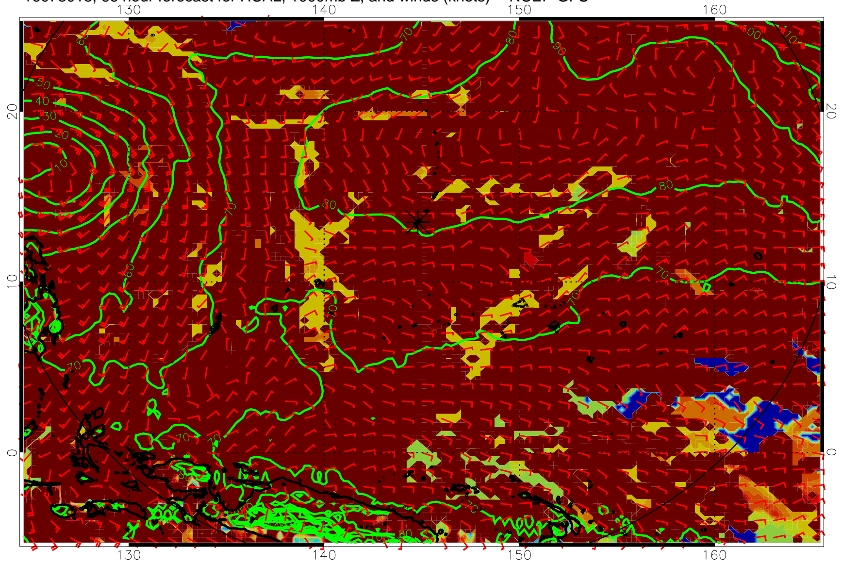
16073018, 66 hour forecast for HCAL, 1000mb Z, and winds (knots) -- NCEP GFS
