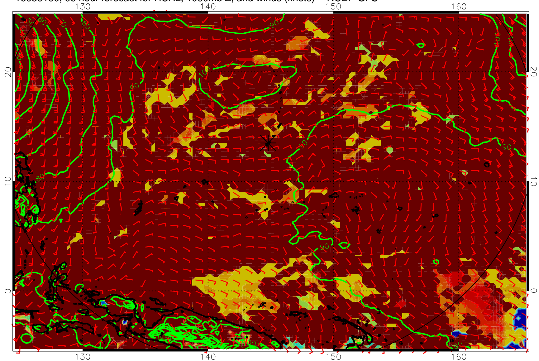
16080100, 96 hour forecast for HCAL, 1000mb Z, and winds (knots) -- NCEP GFS
