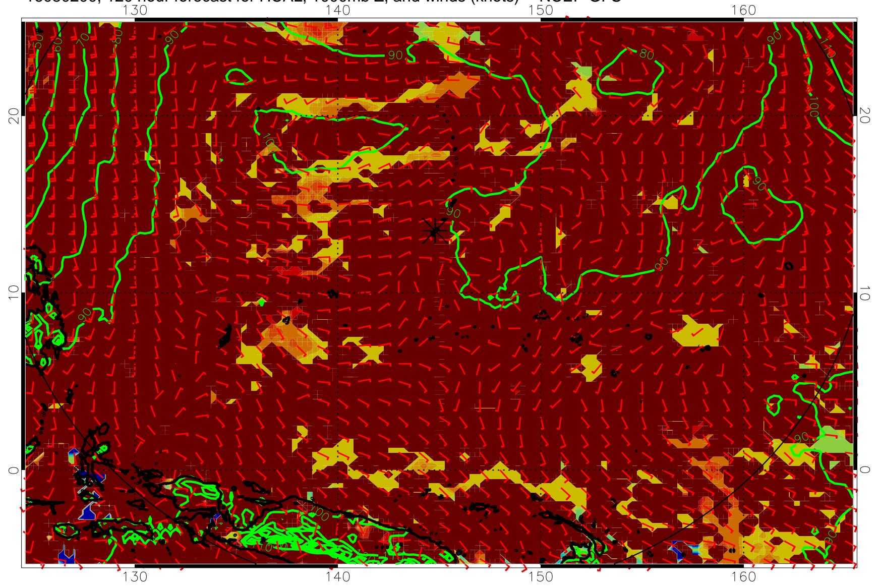
16080200, 120 hour forecast for HCAL, 1000mb Z, and winds (knots) -- NCEP GFS
