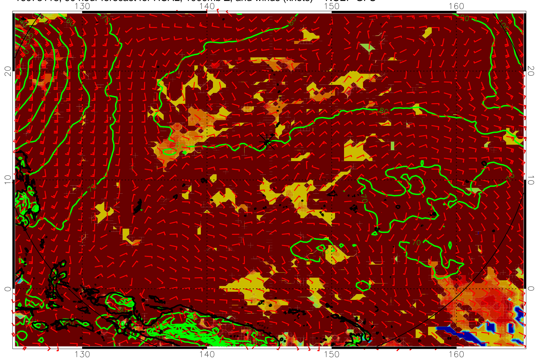
16073118, 90 hour forecast for HCAL, 1000mb Z, and winds (knots) -- NCEP GFS
