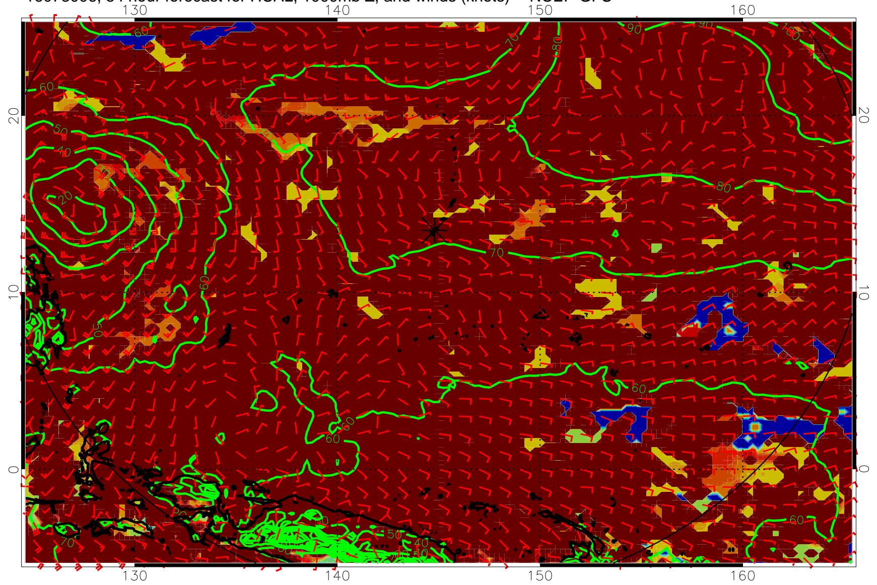
16073006, 54 hour forecast for HCAL, 1000mb Z, and winds (knots) -- NCEP GFS
