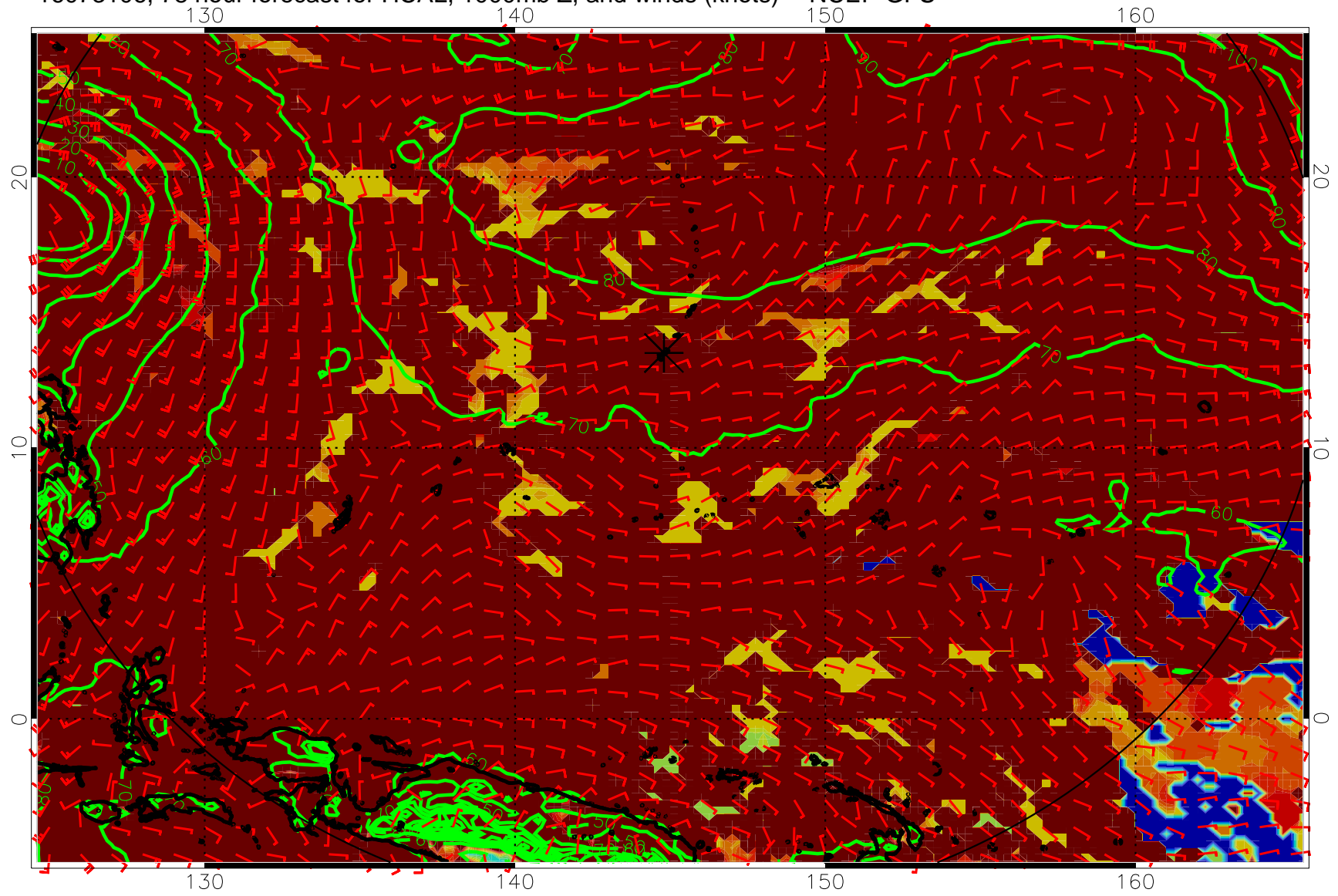
16073106, 78 hour forecast for HCAL, 1000mb Z, and winds (knots) -- NCEP GFS
