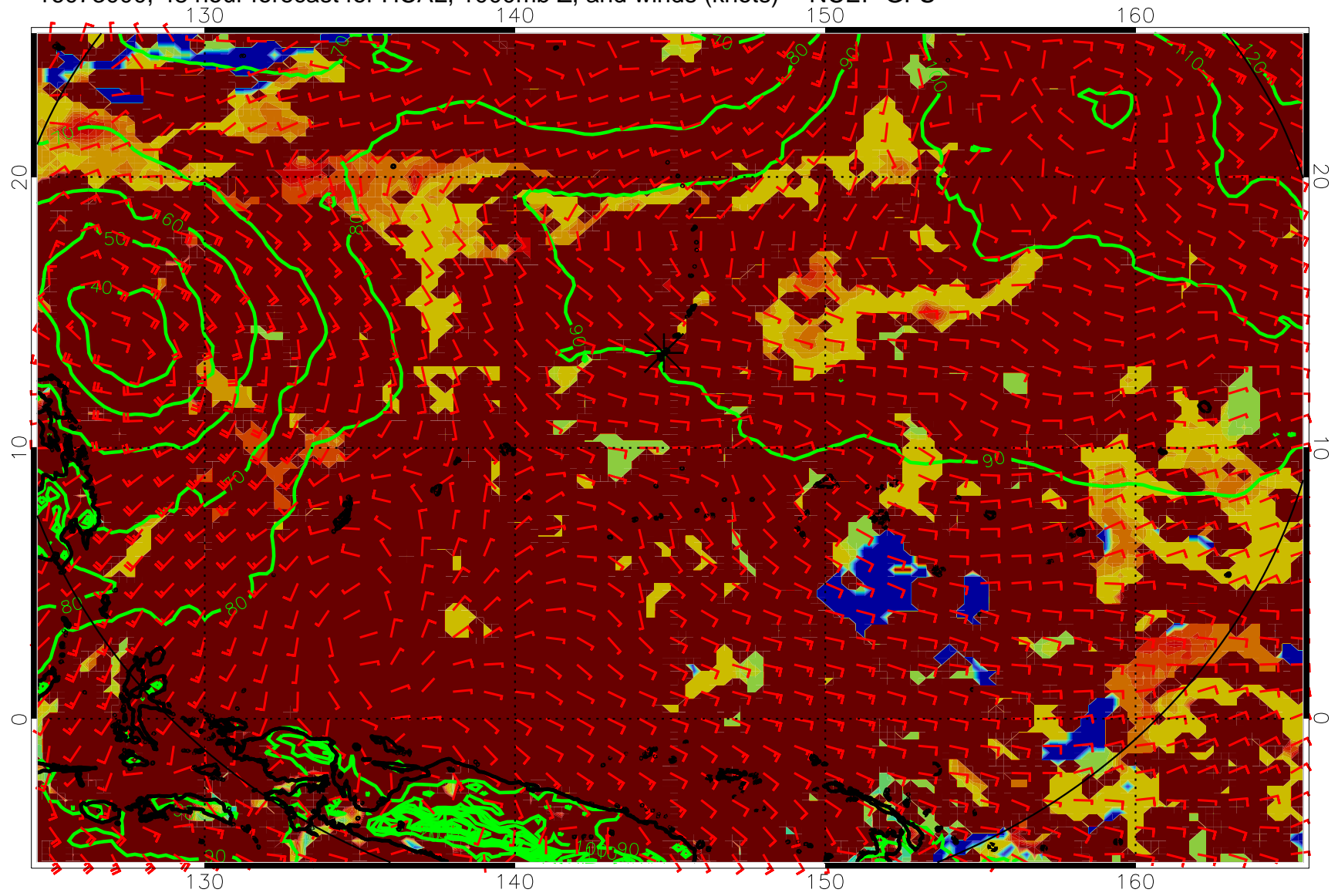
16073000, 48 hour forecast for HCAL, 1000mb Z, and winds (knots) -- NCEP GFS
