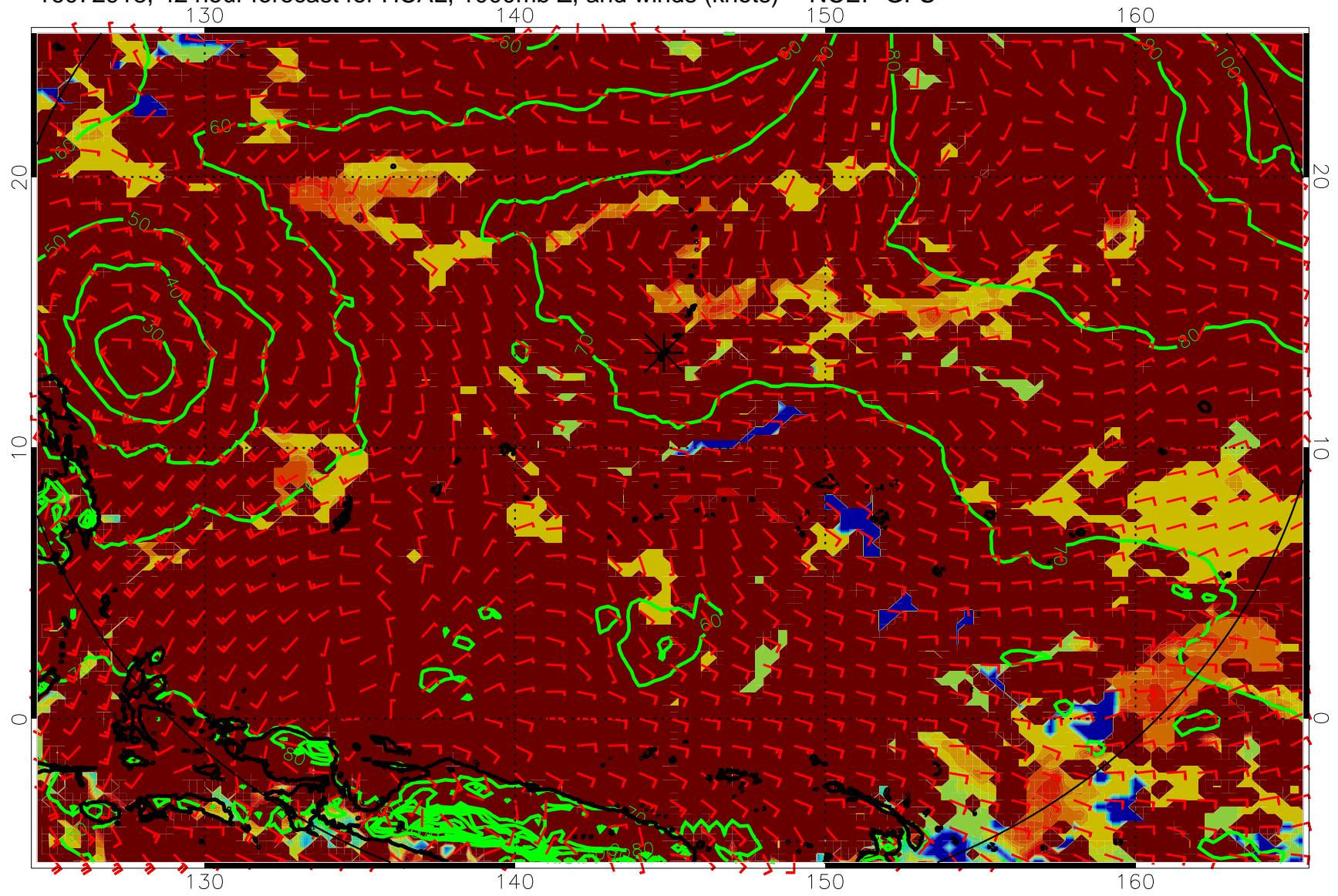
16072918, 42 hour forecast for HCAL, 1000mb Z, and winds (knots) -- NCEP GFS
