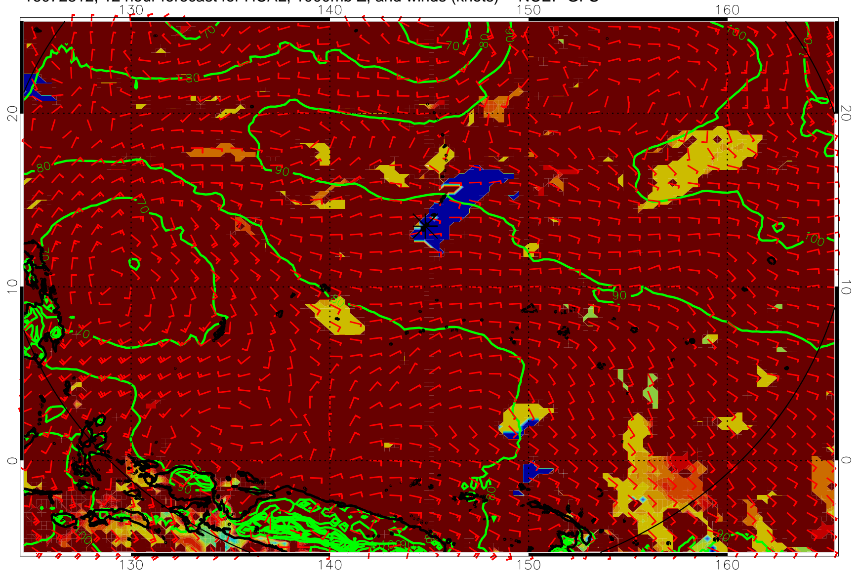
16072812, 12 hour forecast for HCAL, 1000mb Z, and winds (knots) -- NCEP GFS
