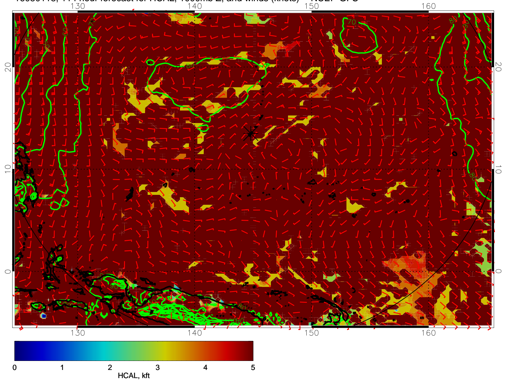
16080118, 114 hour forecast for HCAL, 1000mb Z, and winds (knots) -- NCEP GFS
