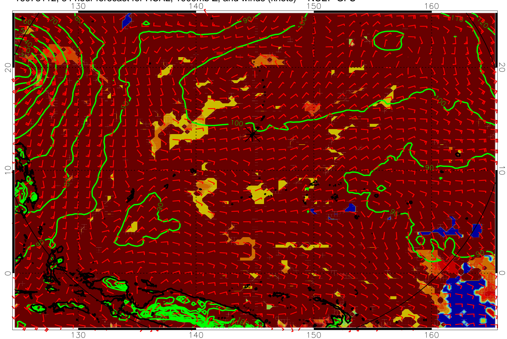
16073112, 84 hour forecast for HCAL, 1000mb Z, and winds (knots) -- NCEP GFS
