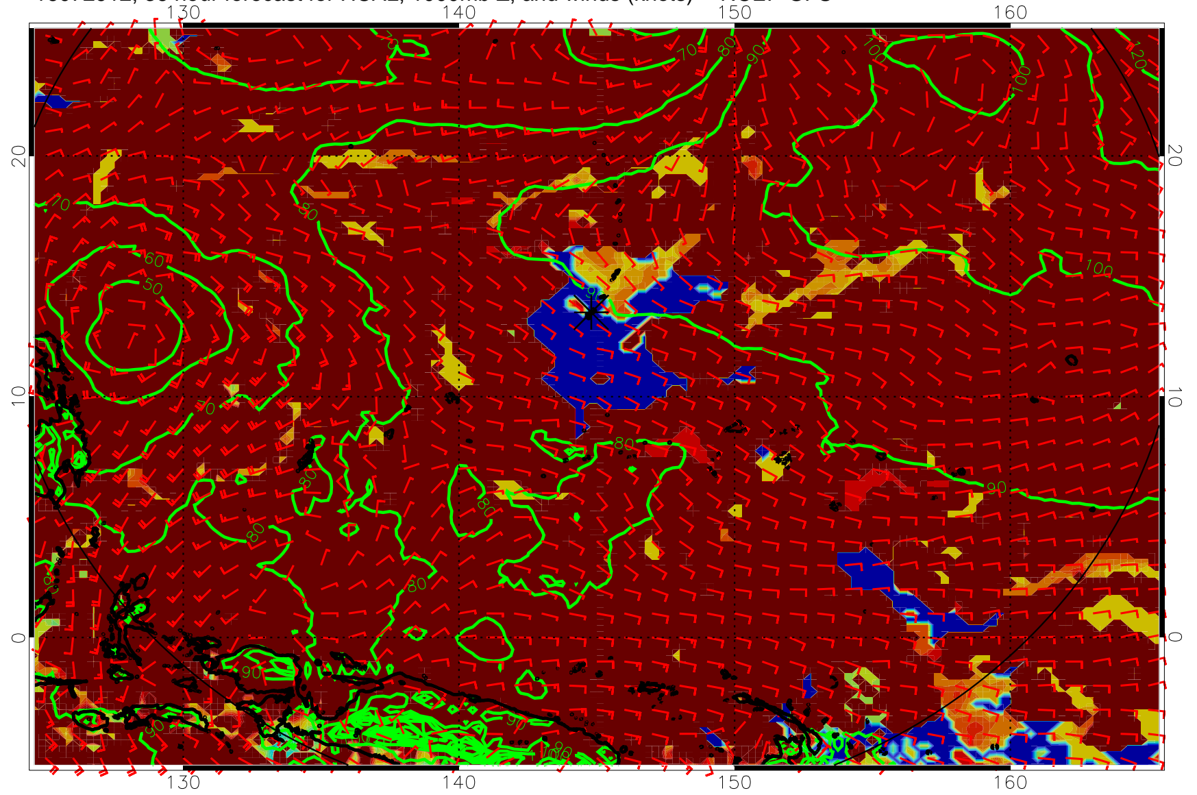
16072912, 36 hour forecast for HCAL, 1000mb Z, and winds (knots) -- NCEP GFS
