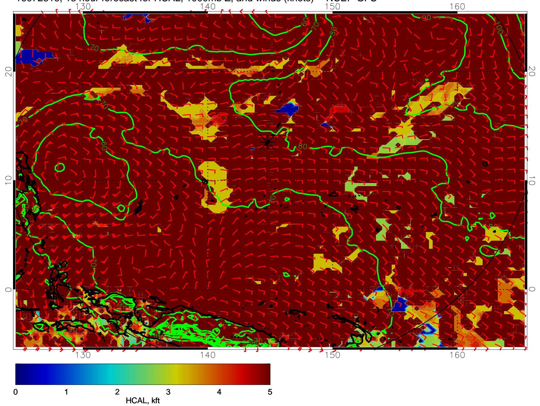
16072818, 18 hour forecast for HCAL, 1000mb Z, and winds (knots) -- NCEP GFS
