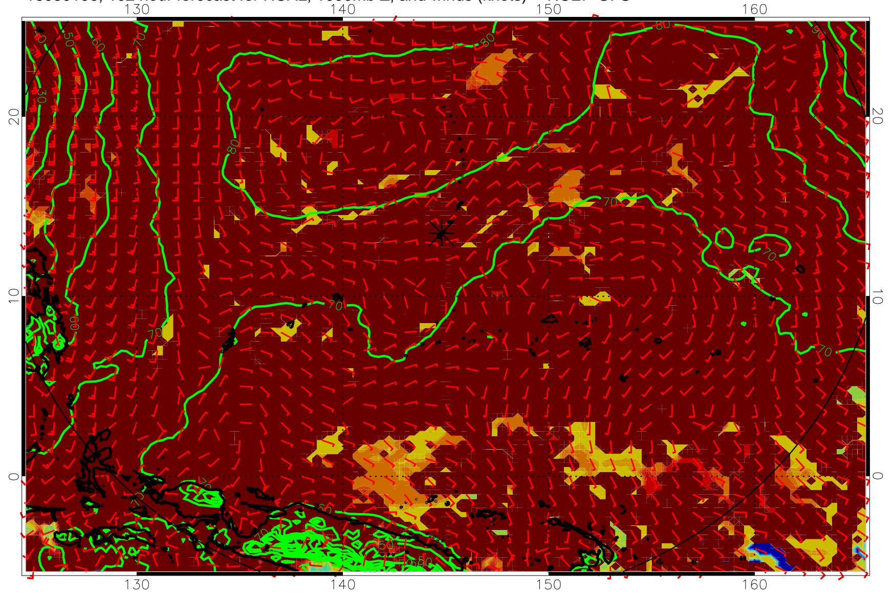
16080106, 102 hour forecast for HCAL, 1000mb Z, and winds (knots) -- NCEP GFS
