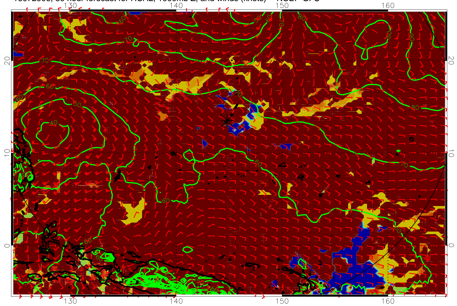
16072906, 30 hour forecast for HCAL, 1000mb Z, and winds (knots) -- NCEP GFS
