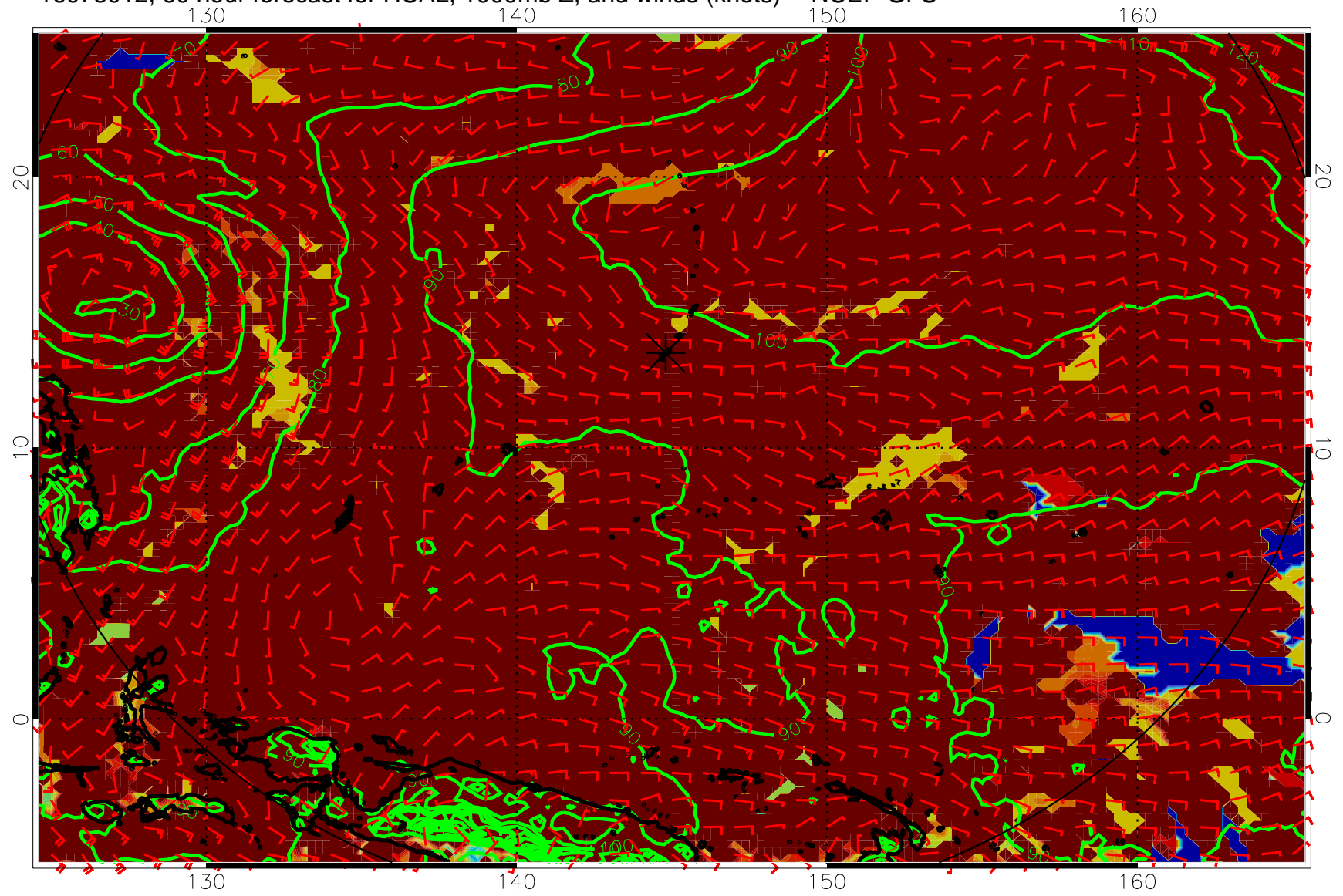
16073012, 60 hour forecast for HCAL, 1000mb Z, and winds (knots) -- NCEP GFS
