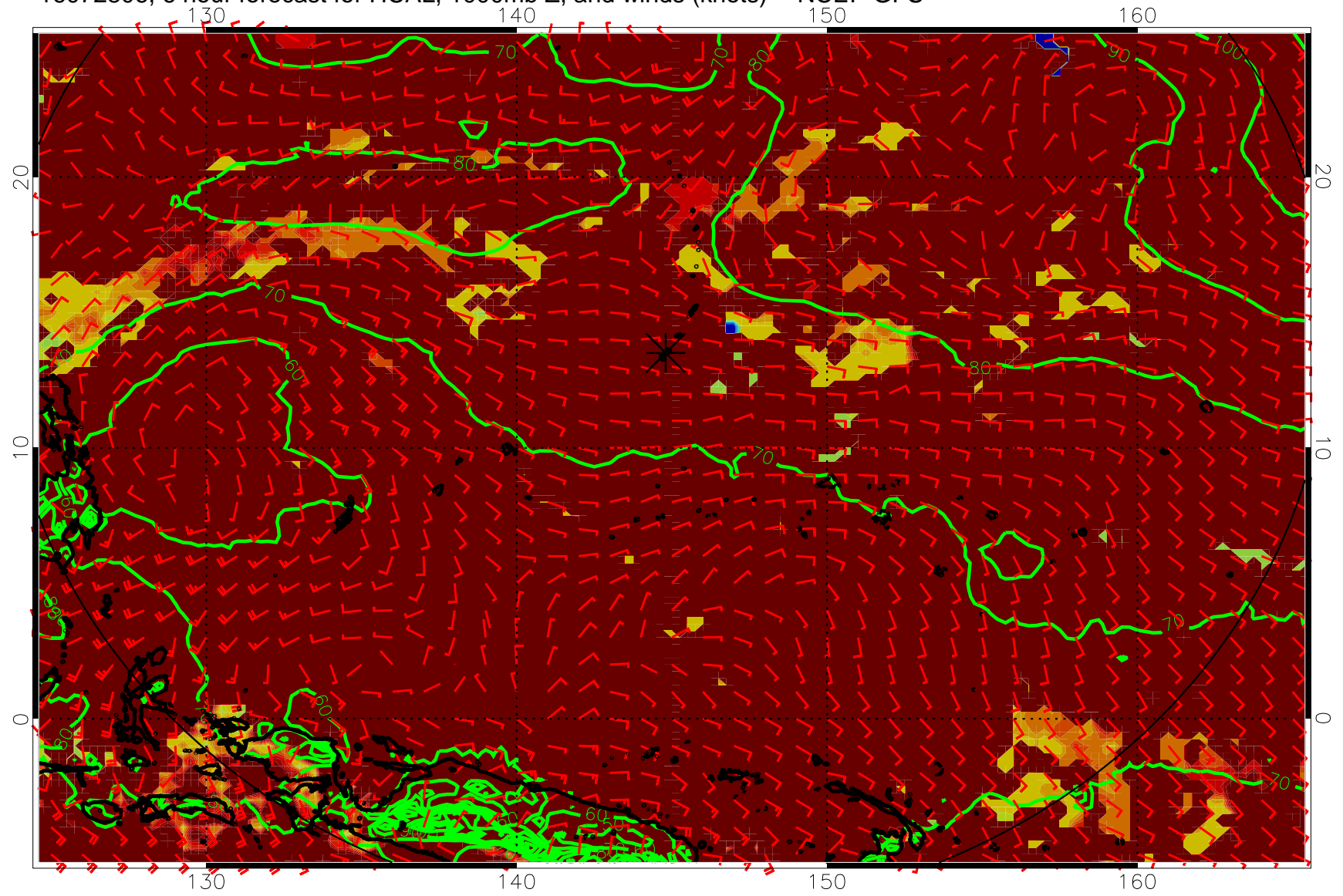
16072806, 6 hour forecast for HCAL, 1000mb Z, and winds (knots) -- NCEP GFS
