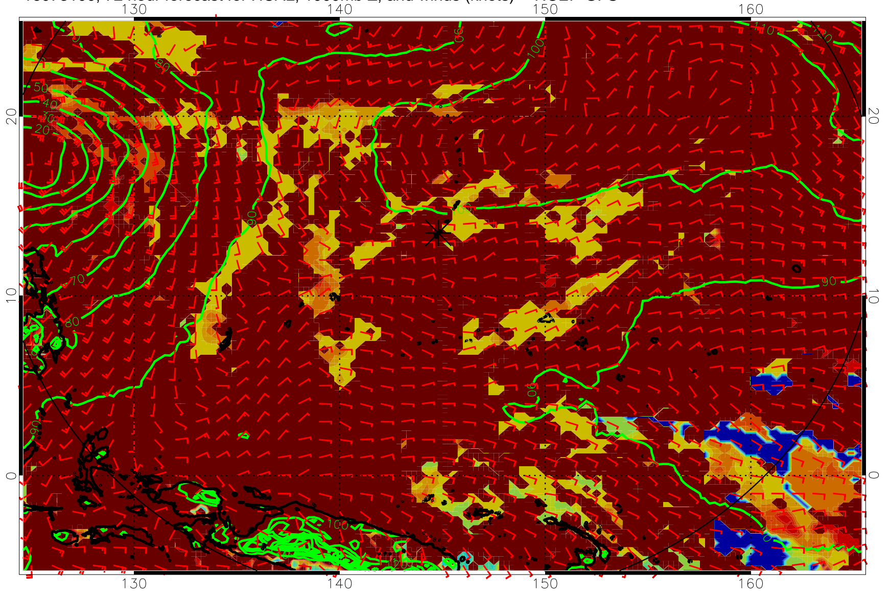
16073100, 72 hour forecast for HCAL, 1000mb Z, and winds (knots) -- NCEP GFS
