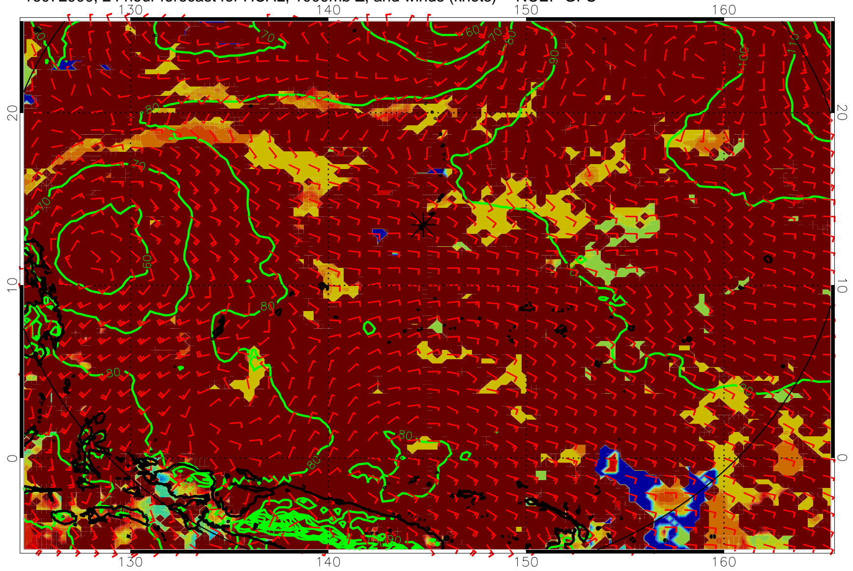
16072900, 24 hour forecast for HCAL, 1000mb Z, and winds (knots) -- NCEP GFS
