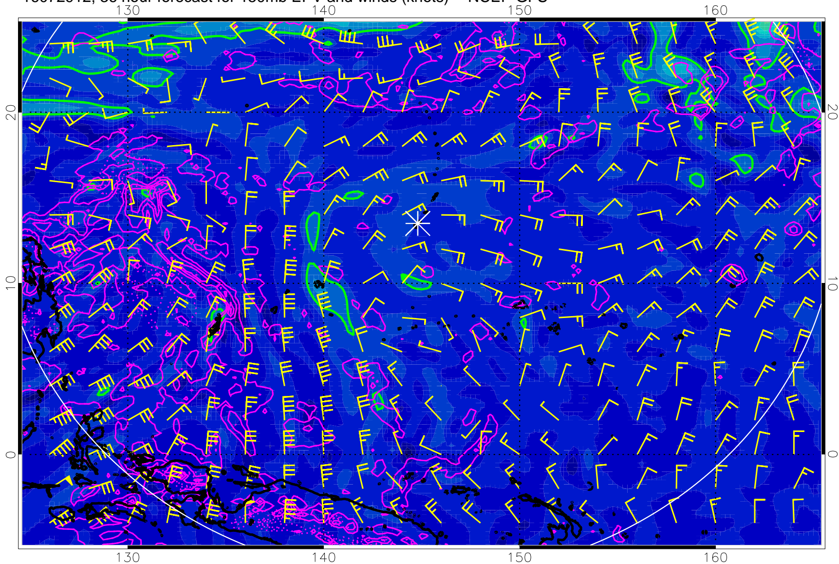
16072912, 36 hour forecast for 150mb EPV and winds (knots) -- NCEP GFS
