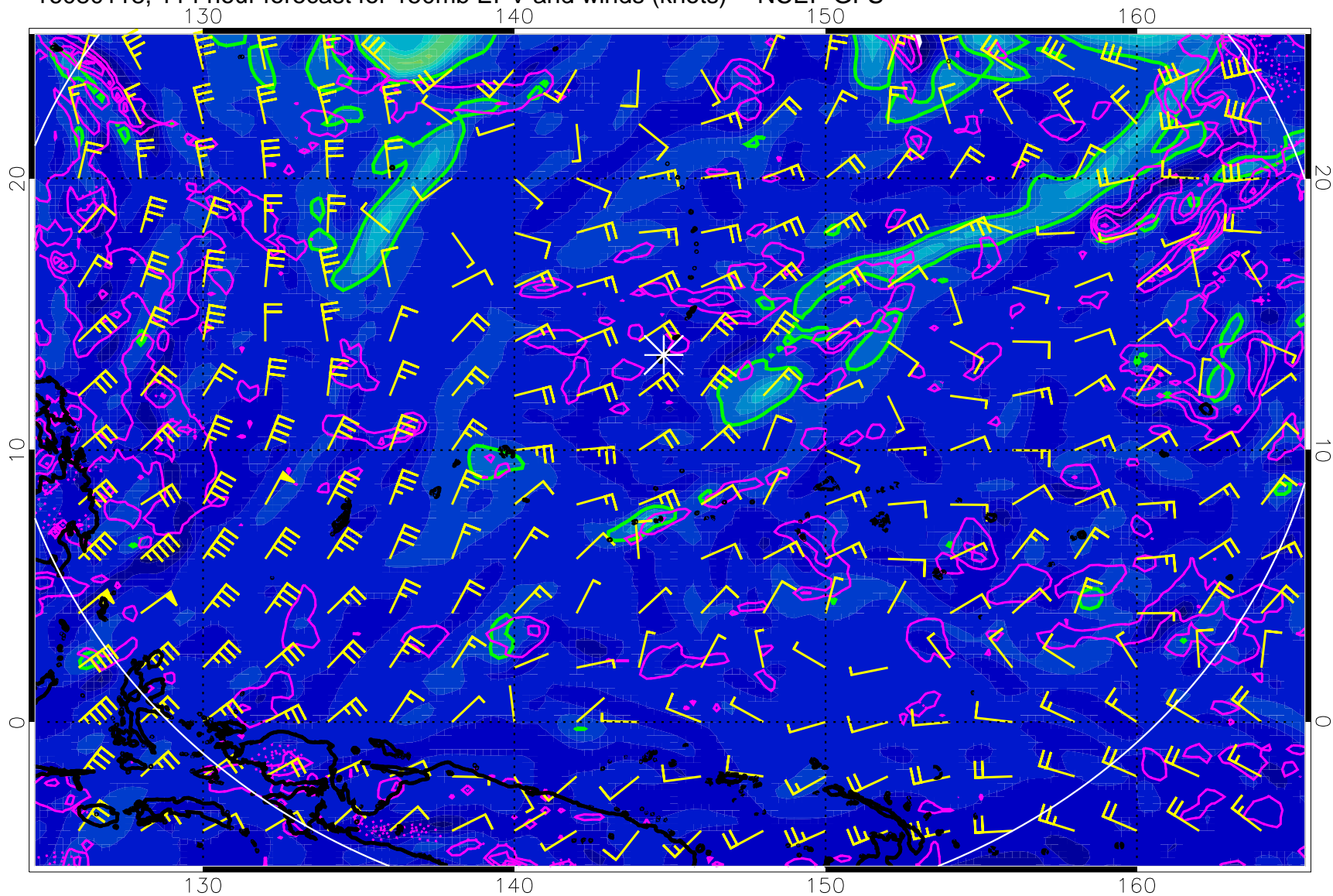
16080118, 114 hour forecast for 150mb EPV and winds (knots) -- NCEP GFS
