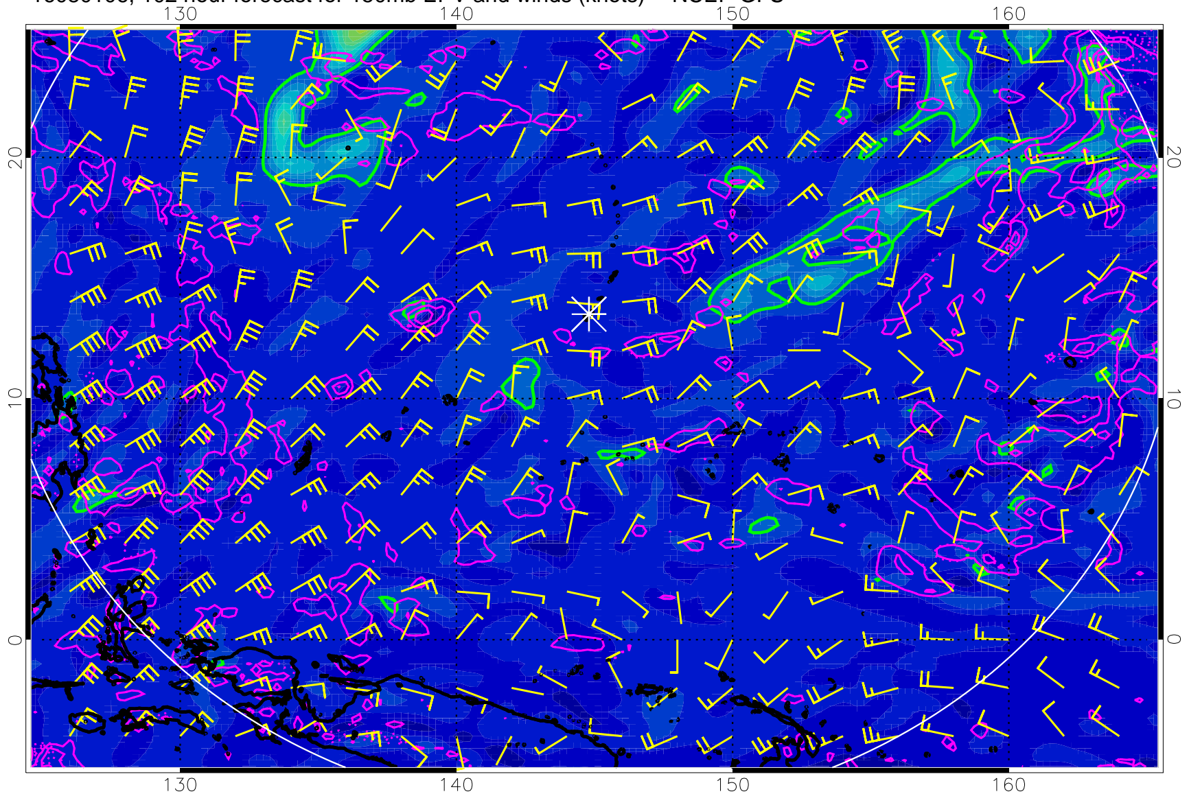
16080106, 102 hour forecast for 150mb EPV and winds (knots) -- NCEP GFS
