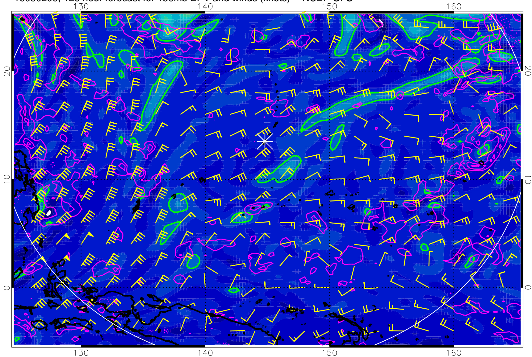
16080200, 120 hour forecast for 150mb EPV and winds (knots) -- NCEP GFS
