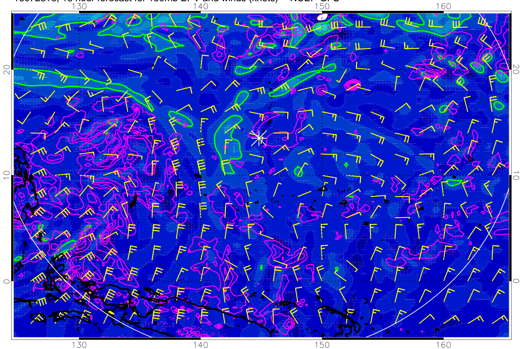
16072818, 18 hour forecast for 150mb EPV and winds (knots) -- NCEP GFS
