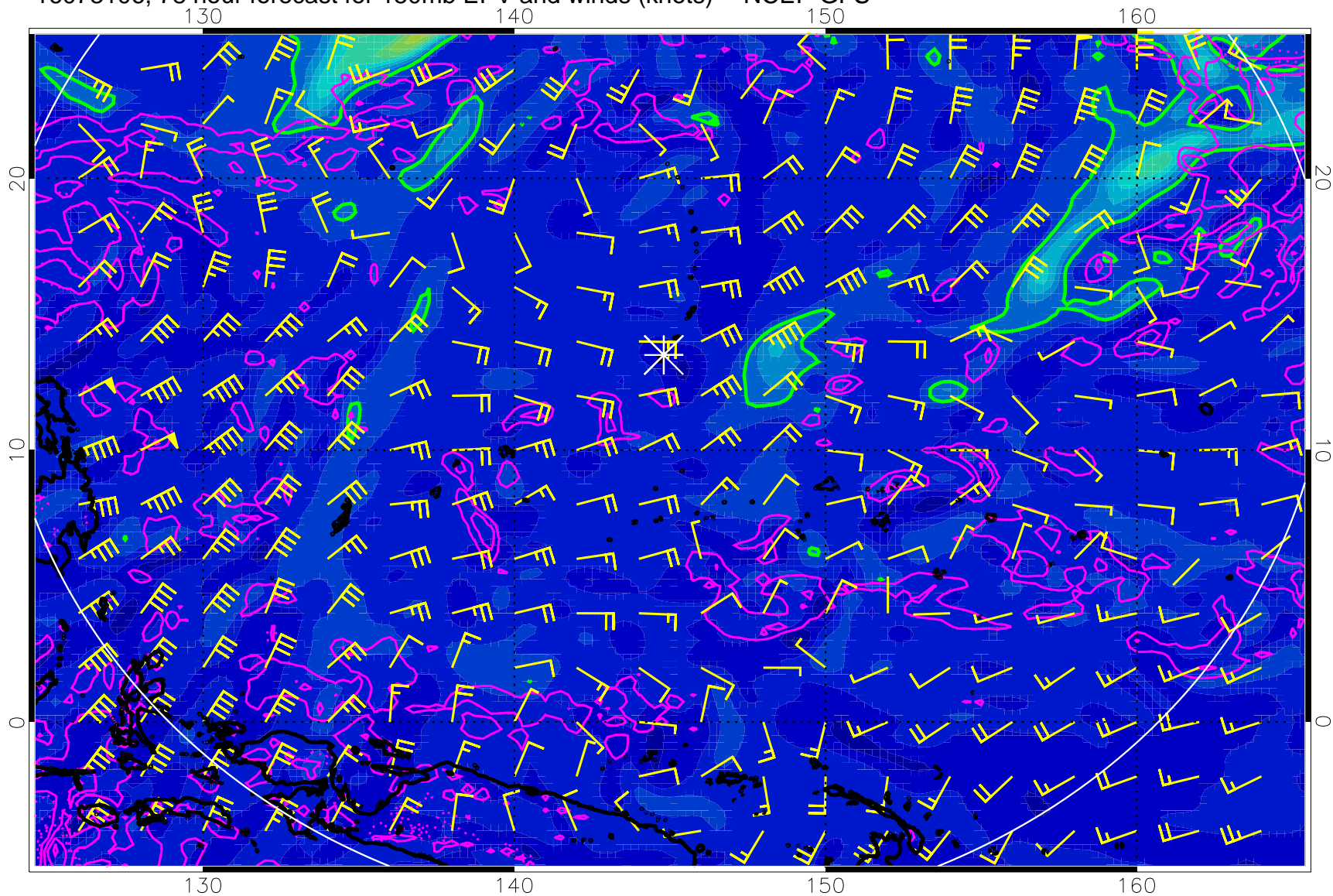
16073106, 78 hour forecast for 150mb EPV and winds (knots) -- NCEP GFS
