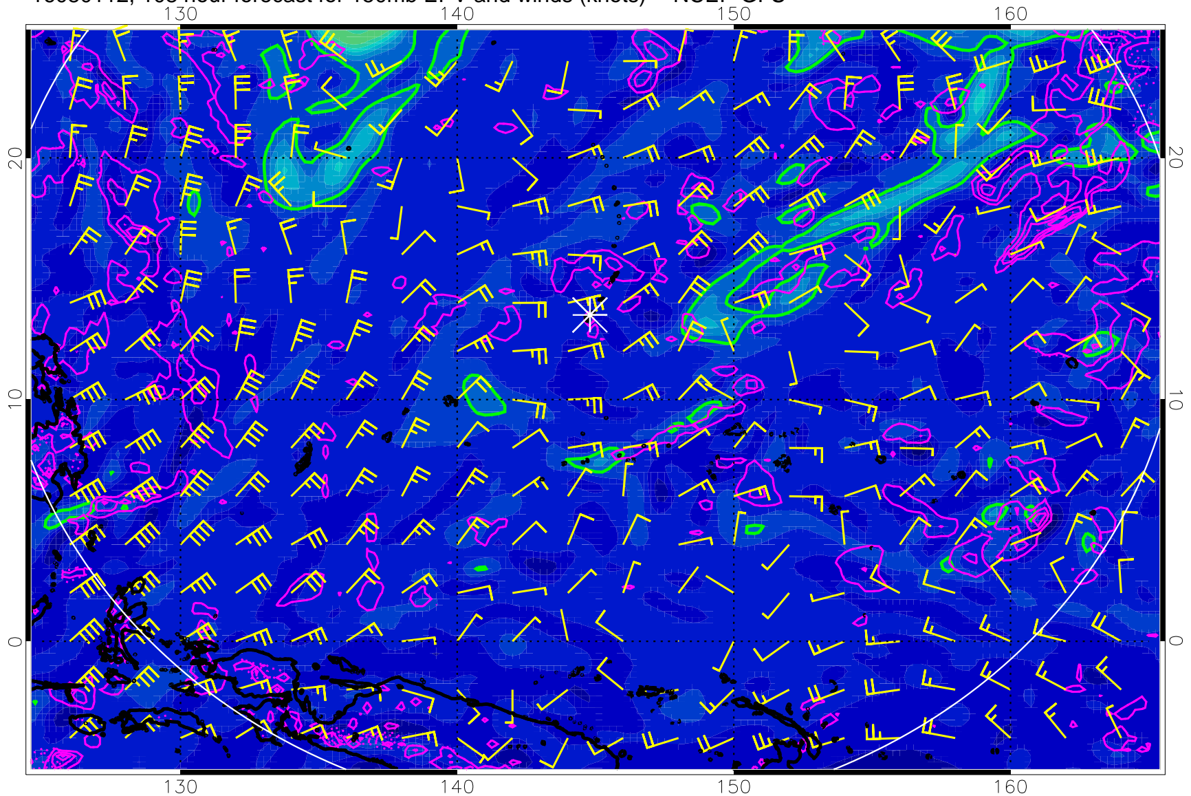
16080112, 108 hour forecast for 150mb EPV and winds (knots) -- NCEP GFS
