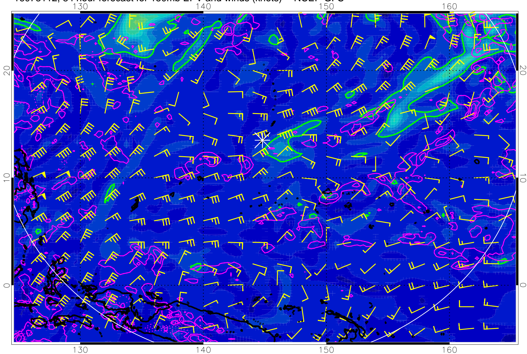
16073112, 84 hour forecast for 150mb EPV and winds (knots) -- NCEP GFS
