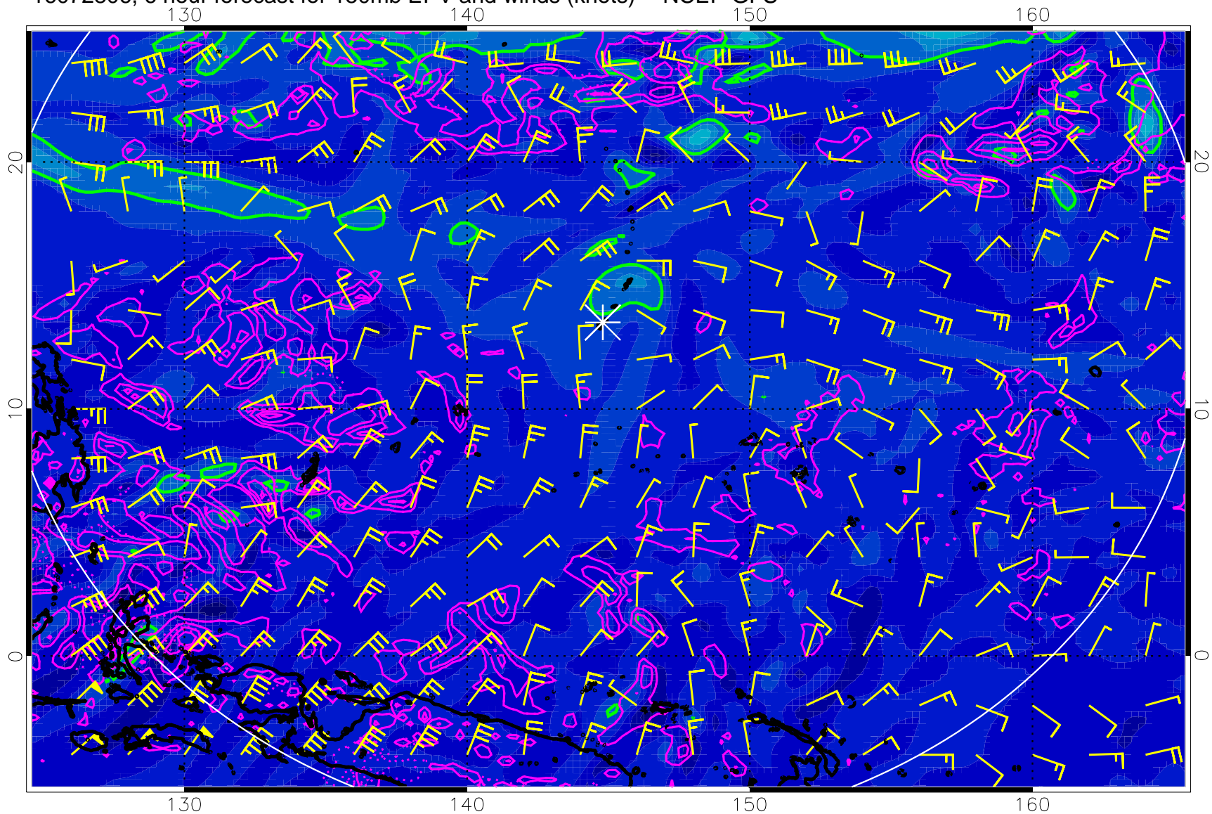
16072806, 6 hour forecast for 150mb EPV and winds (knots) -- NCEP GFS
