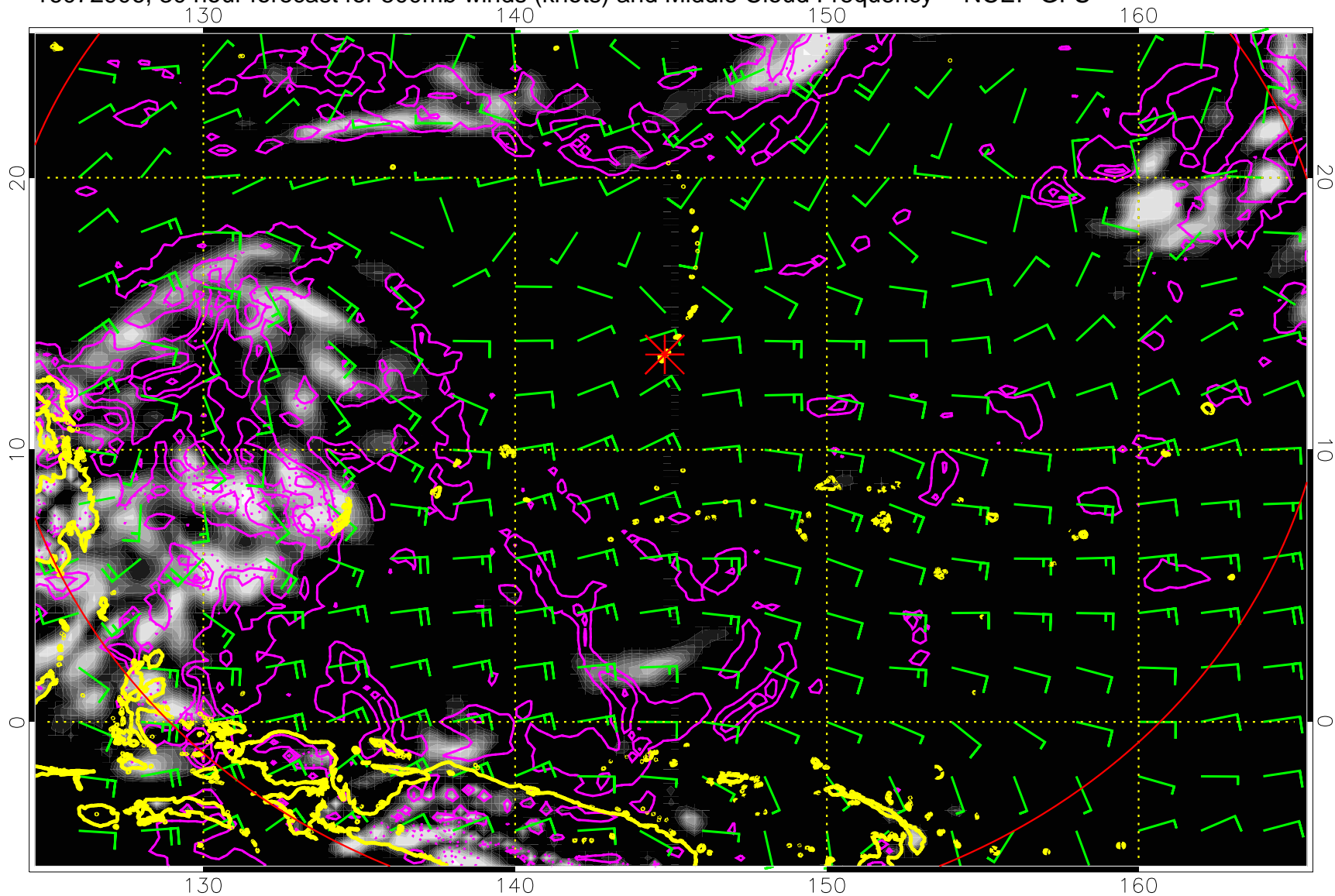
16072906, 30 hour forecast for 500mb winds (knots) and Middle Cloud Frequency -- NCEP GFS
