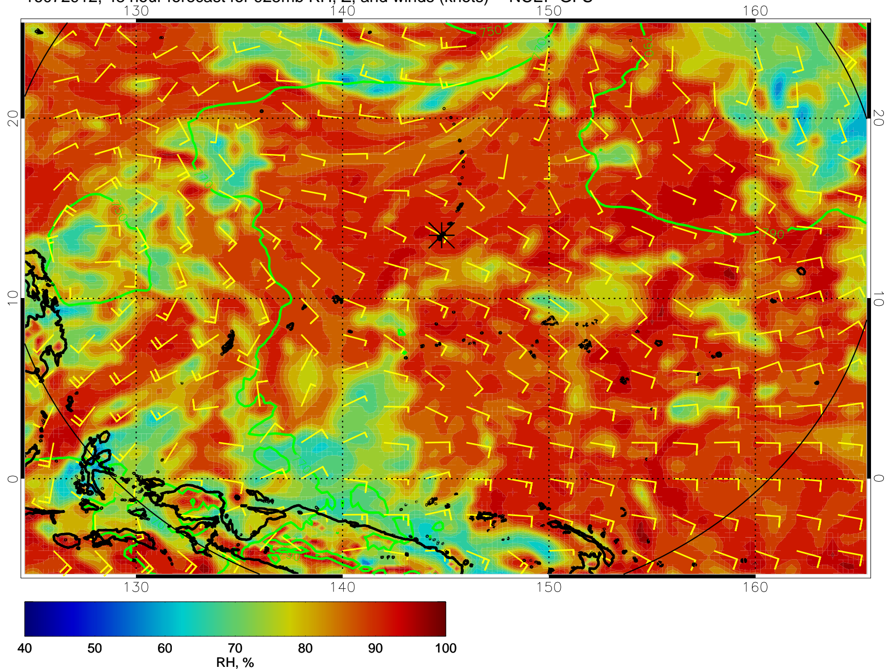
16072912, 48 hour forecast for 925mb RH, Z, and winds (knots) -- NCEP GFS
