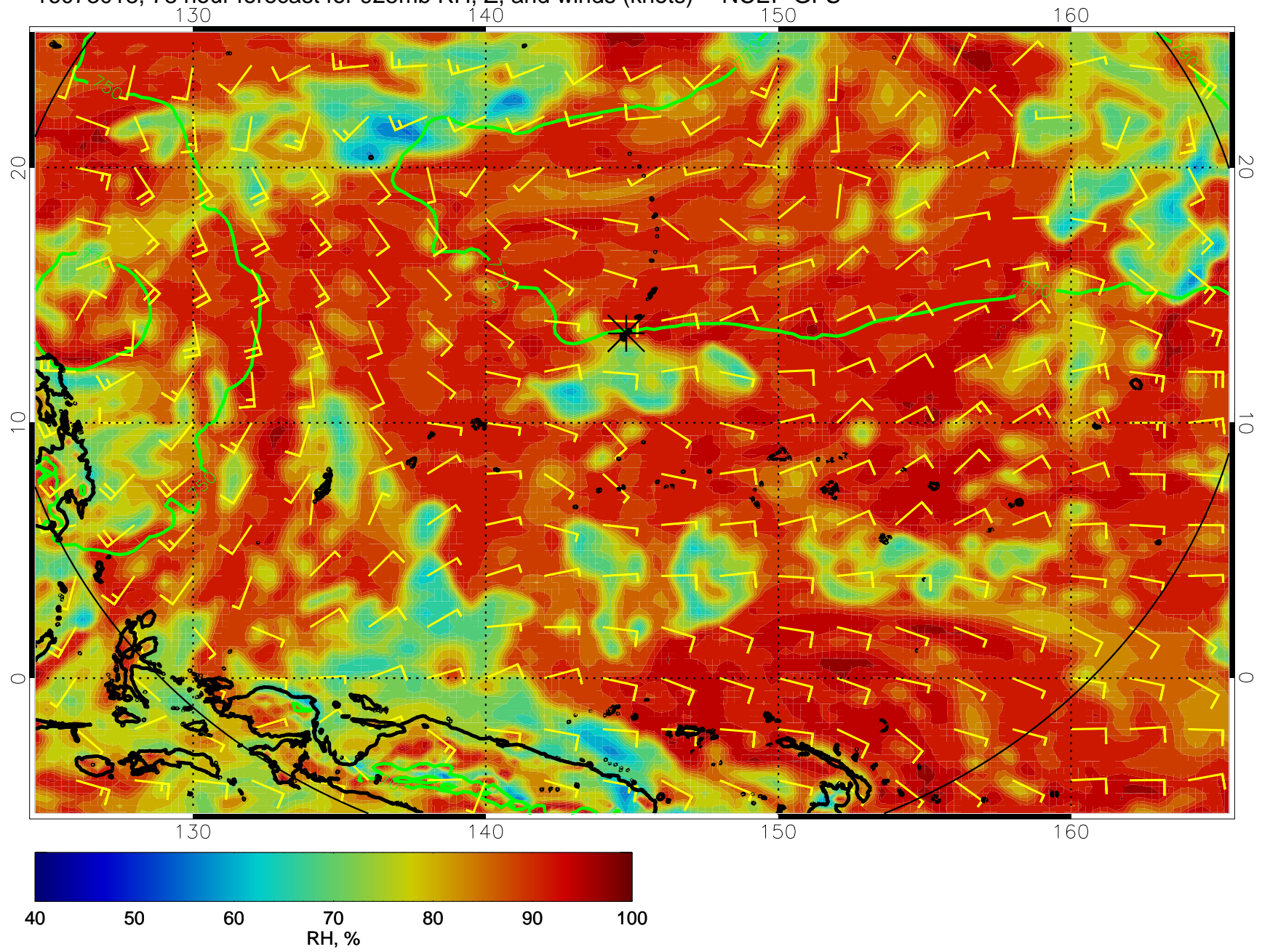
16073018, 78 hour forecast for 925mb RH, Z, and winds (knots) -- NCEP GFS
