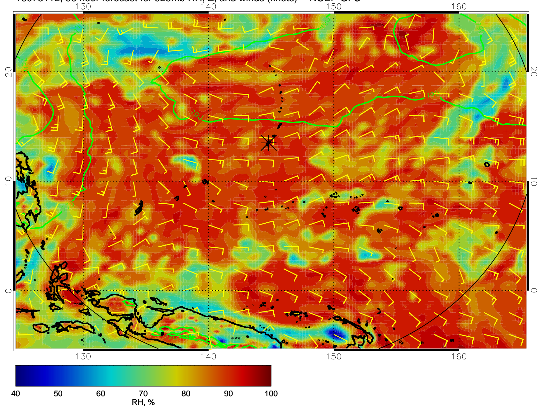
16073112, 96 hour forecast for 925mb RH, Z, and winds (knots) -- NCEP GFS
