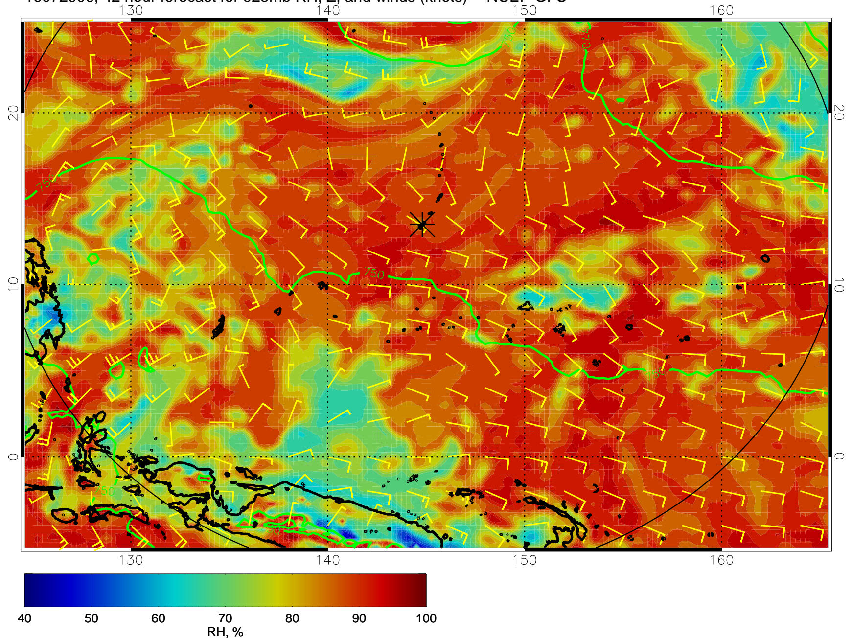
16072906, 42 hour forecast for 925mb RH, Z, and winds (knots) -- NCEP GFS
