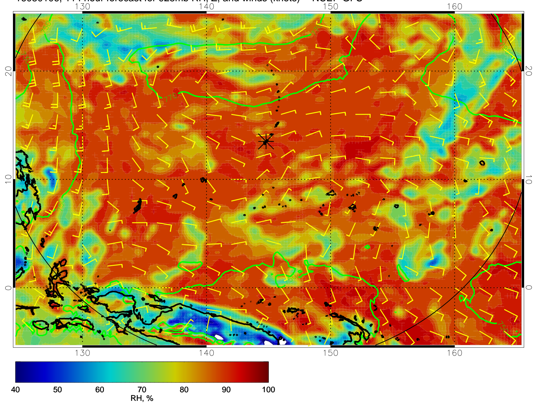
16080106, 114 hour forecast for 925mb RH, Z, and winds (knots) -- NCEP GFS
