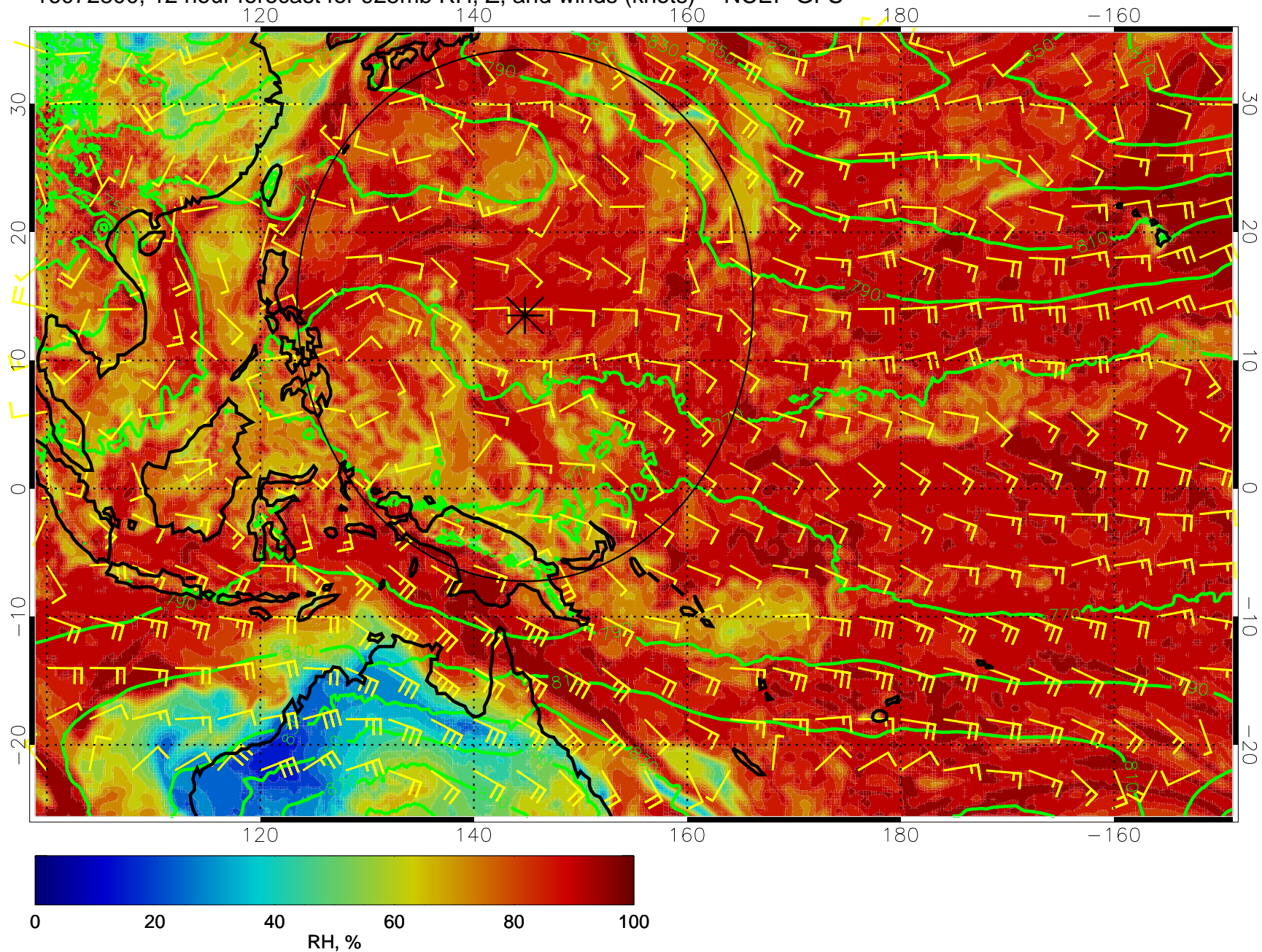
16072800, 12 hour forecast for 925mb RH, Z, and winds (knots) -- NCEP GFS
