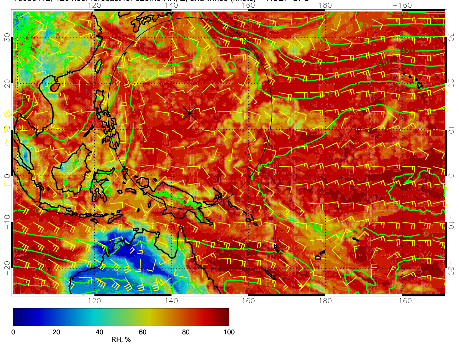
16080112, 120 hour forecast for 925mb RH, Z, and winds (knots) -- NCEP GFS
