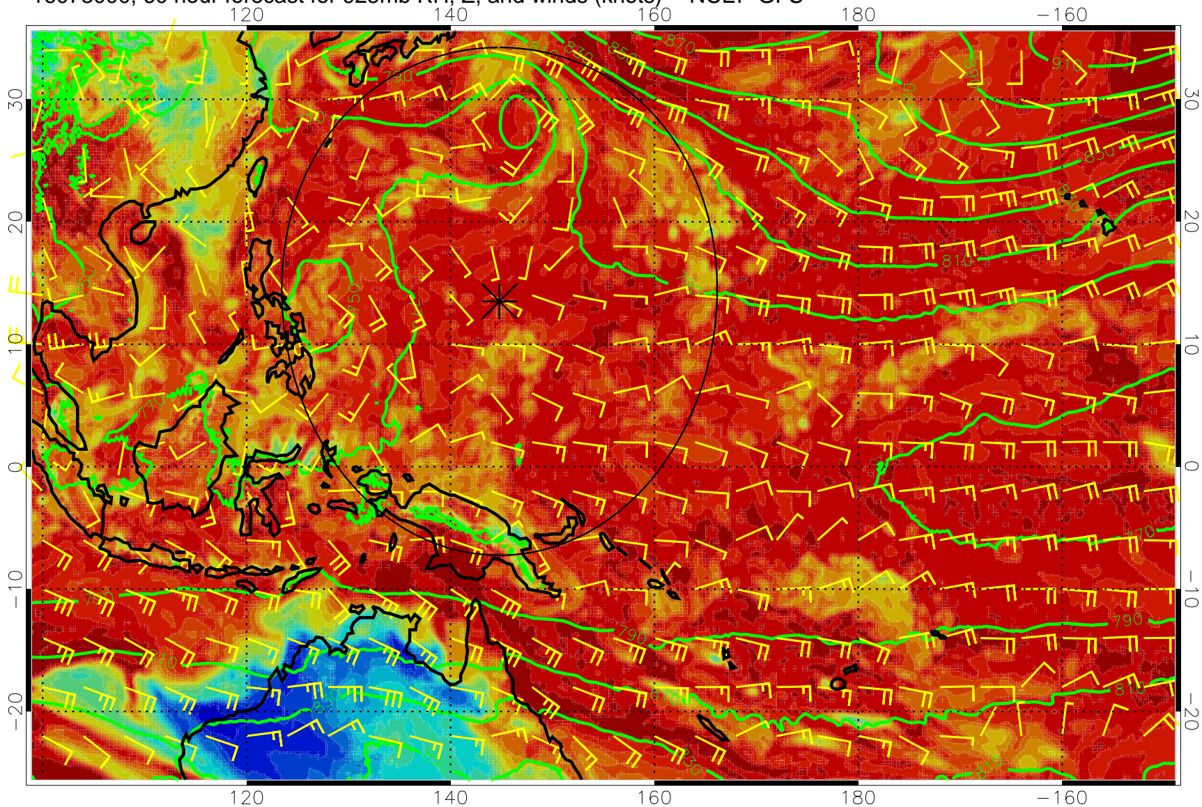
16073000, 60 hour forecast for 925mb RH, Z, and winds (knots) -- NCEP GFS
