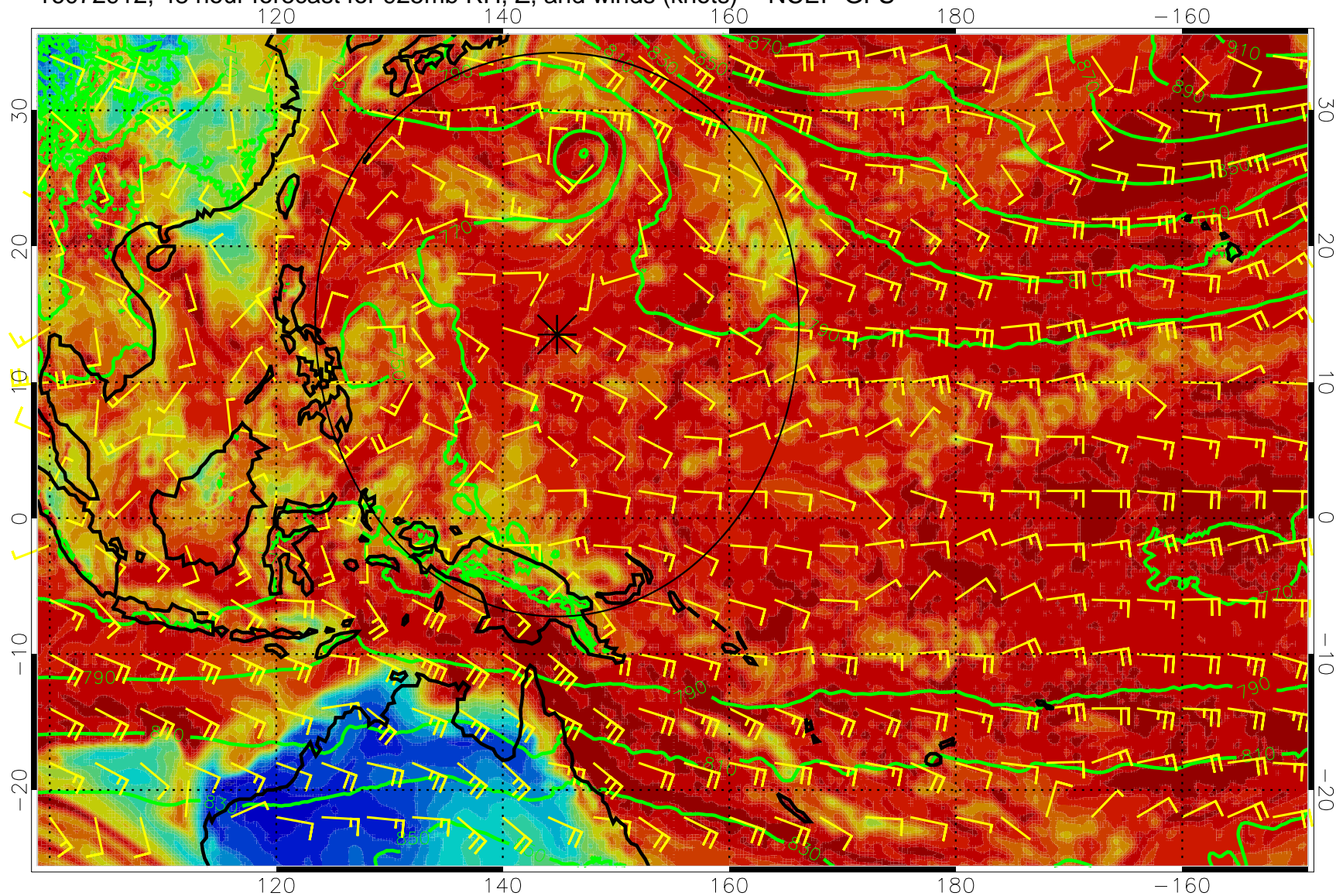
16072912, 48 hour forecast for 925mb RH, Z, and winds (knots) -- NCEP GFS
