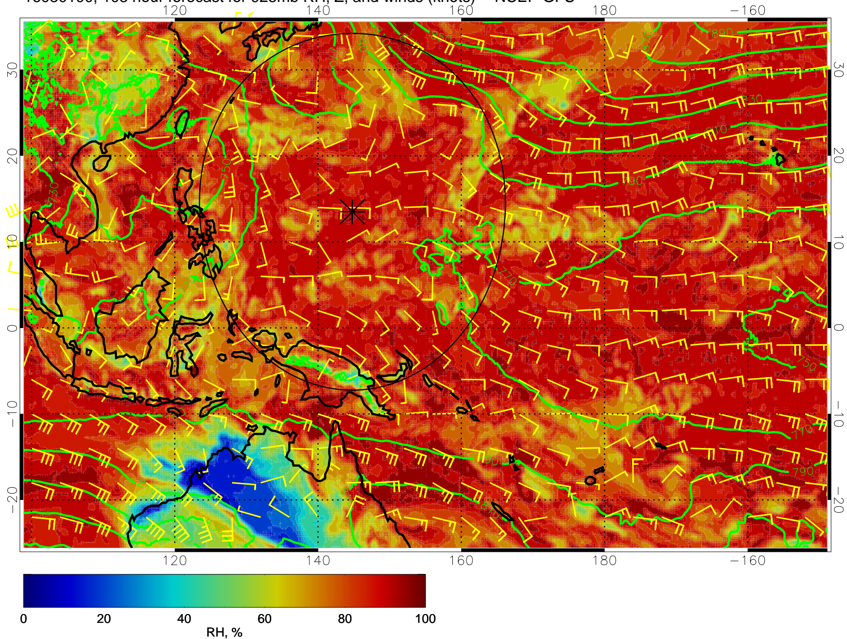
16080100, 108 hour forecast for 925mb RH, Z, and winds (knots) -- NCEP GFS
