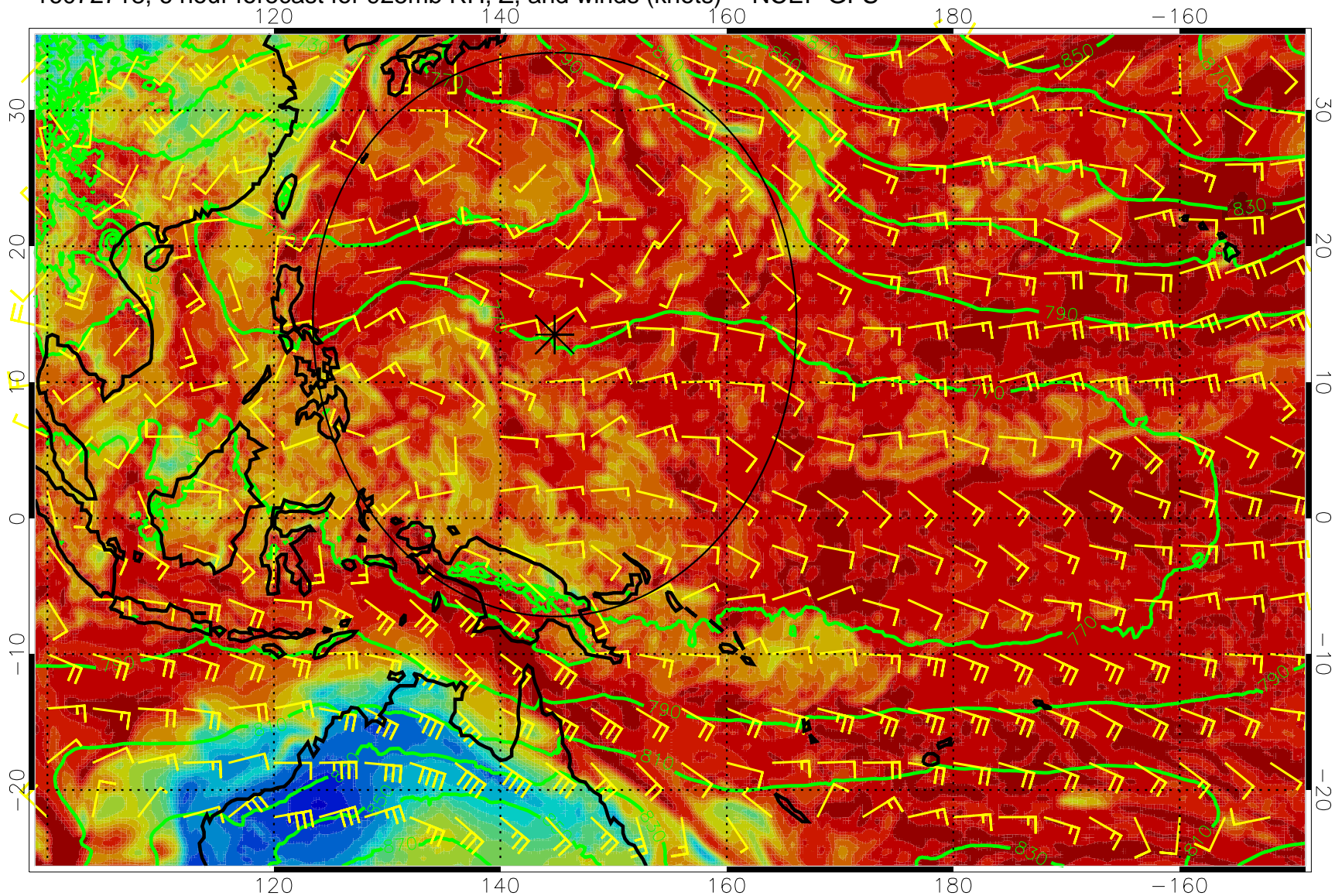
16072718, 6 hour forecast for 925mb RH, Z, and winds (knots) -- NCEP GFS
