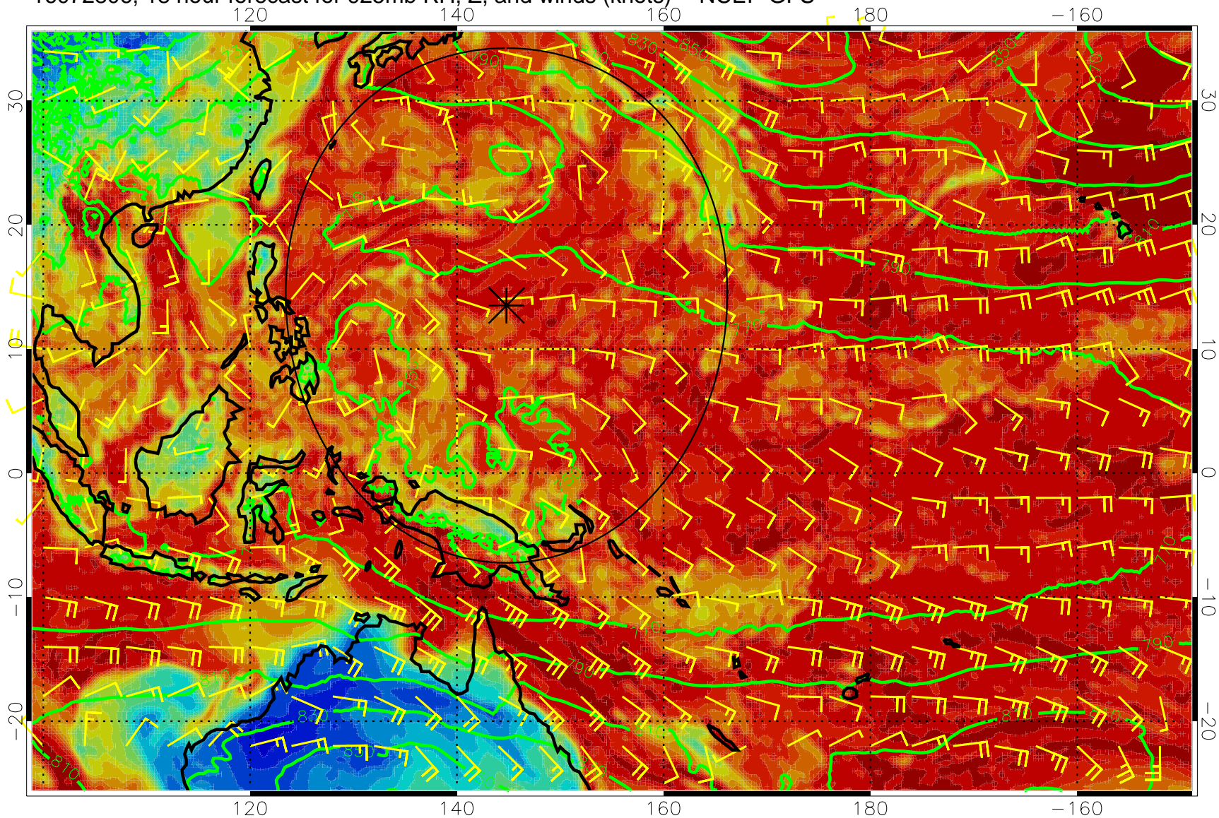
16072806, 18 hour forecast for 925mb RH, Z, and winds (knots) -- NCEP GFS
