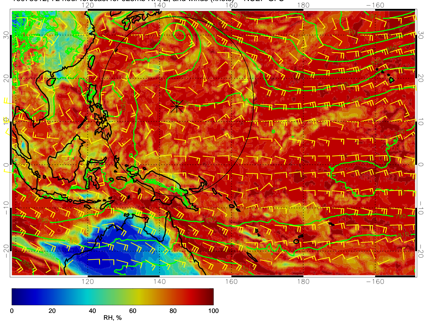
16073012, 72 hour forecast for 925mb RH, Z, and winds (knots) -- NCEP GFS
