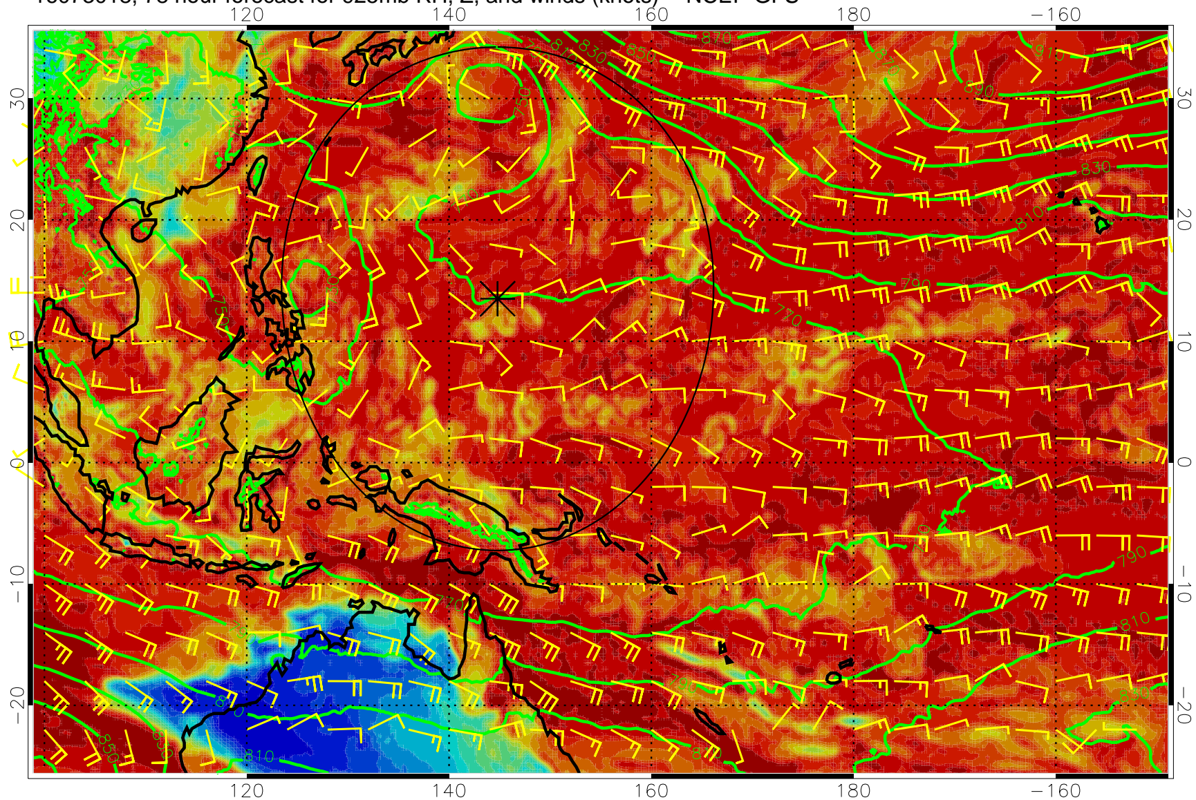
16073018, 78 hour forecast for 925mb RH, Z, and winds (knots) -- NCEP GFS
