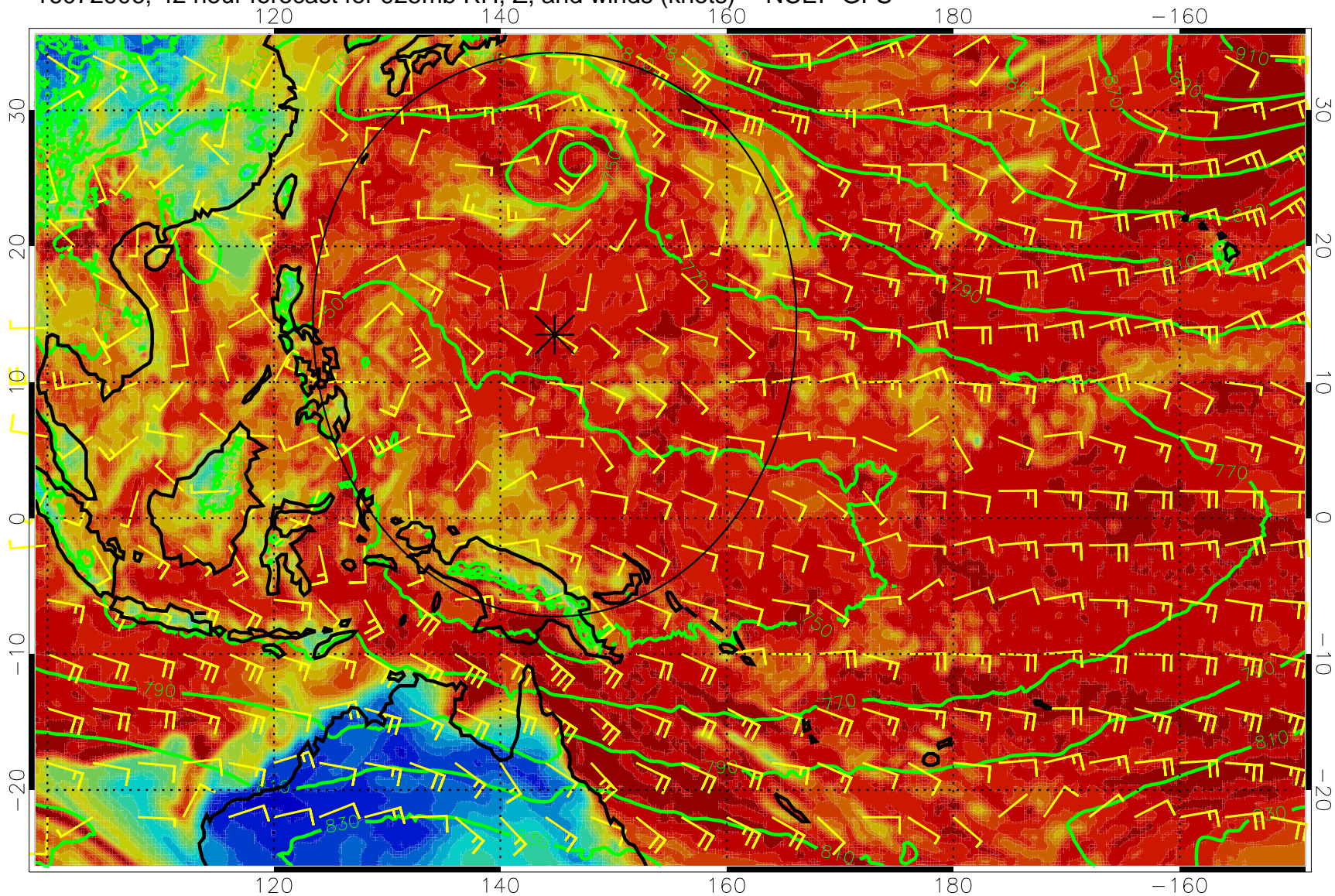
16072906, 42 hour forecast for 925mb RH, Z, and winds (knots) -- NCEP GFS
