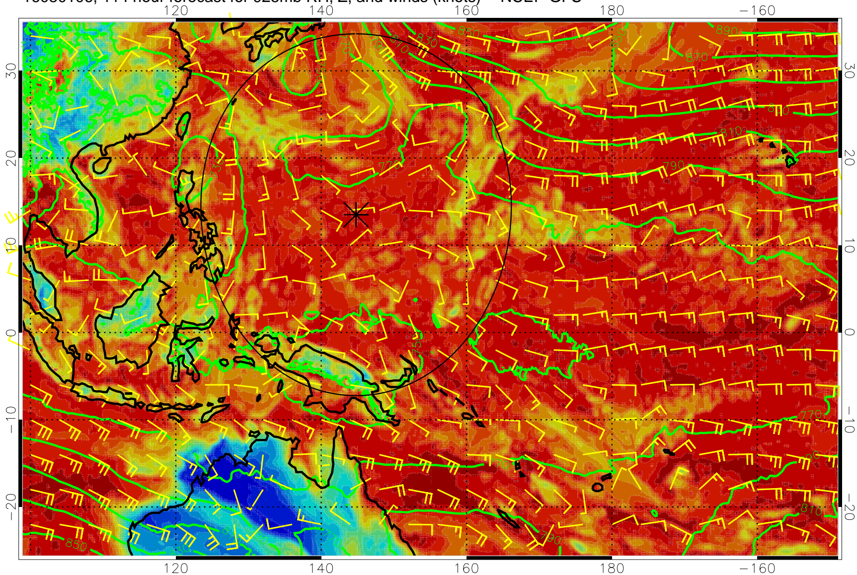
16080106, 114 hour forecast for 925mb RH, Z, and winds (knots) -- NCEP GFS
