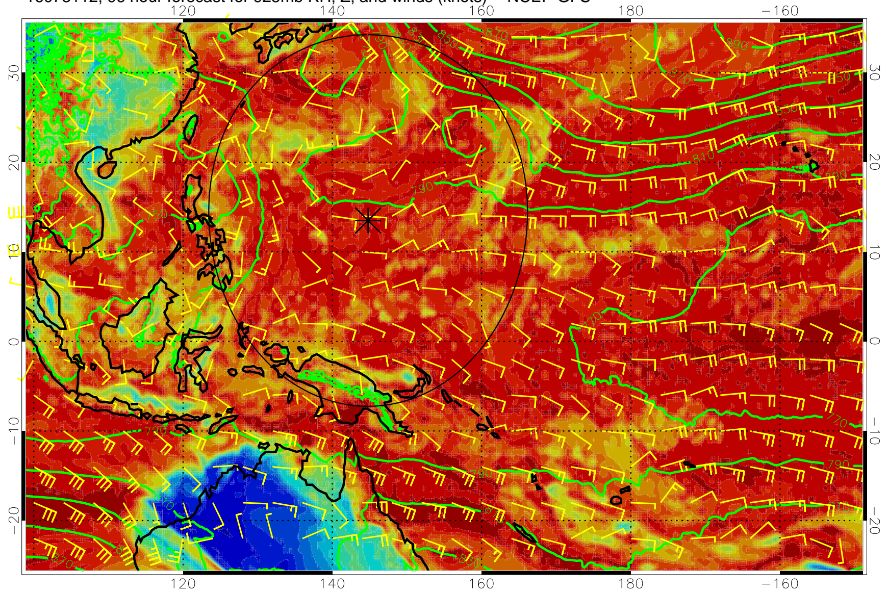
16073112, 96 hour forecast for 925mb RH, Z, and winds (knots) -- NCEP GFS
