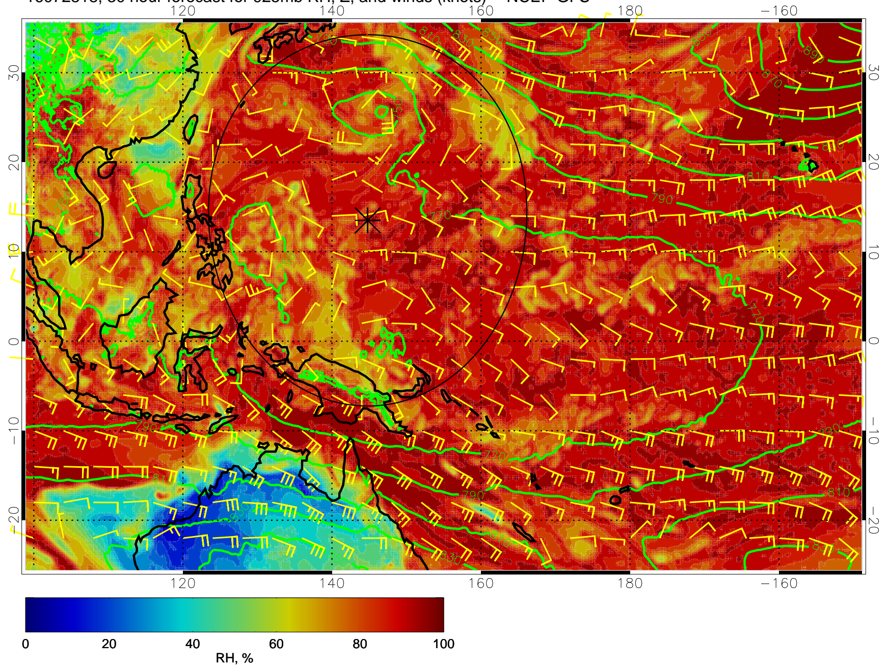
16072818, 30 hour forecast for 925mb RH, Z, and winds (knots) -- NCEP GFS
