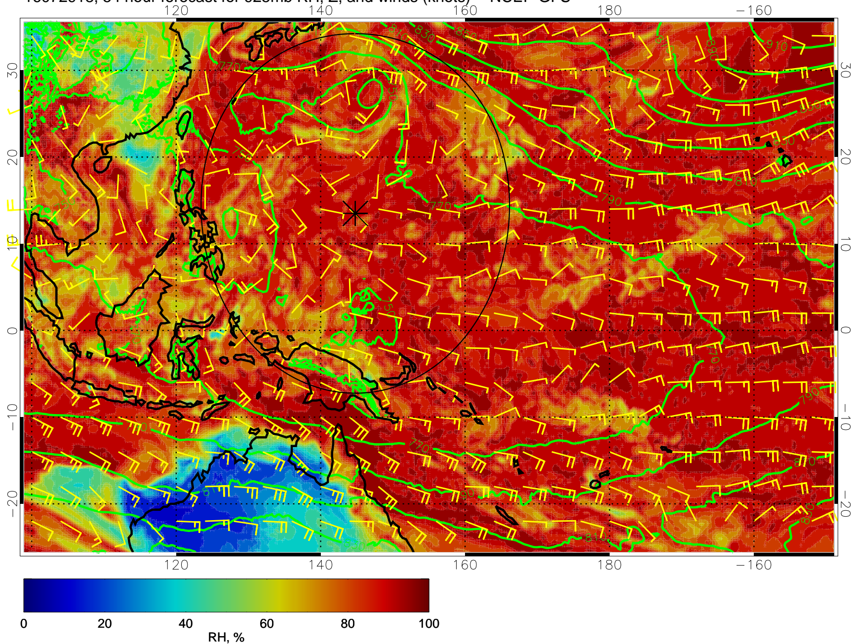
16072918, 54 hour forecast for 925mb RH, Z, and winds (knots) -- NCEP GFS
