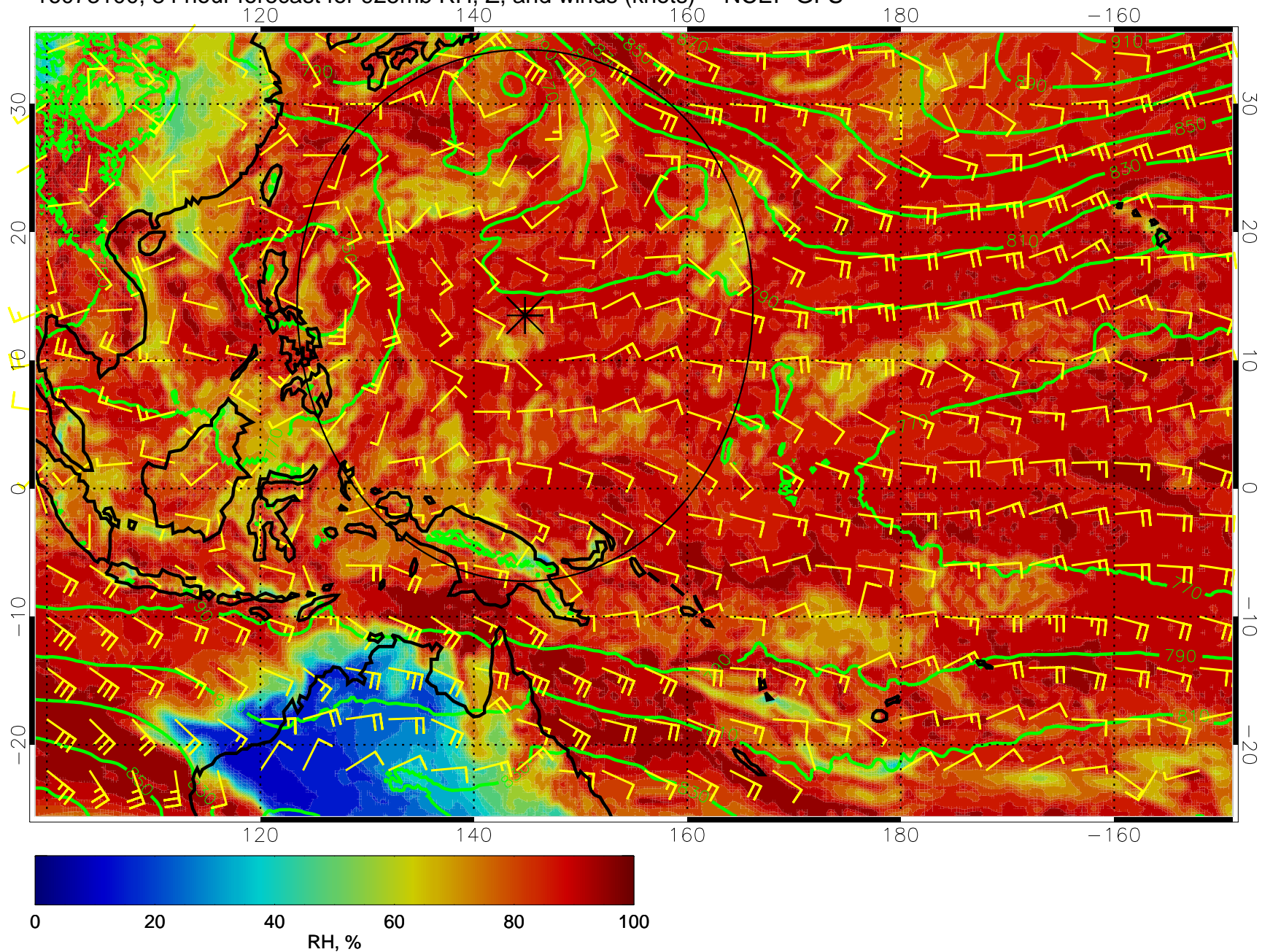
16073100, 84 hour forecast for 925mb RH, Z, and winds (knots) -- NCEP GFS
