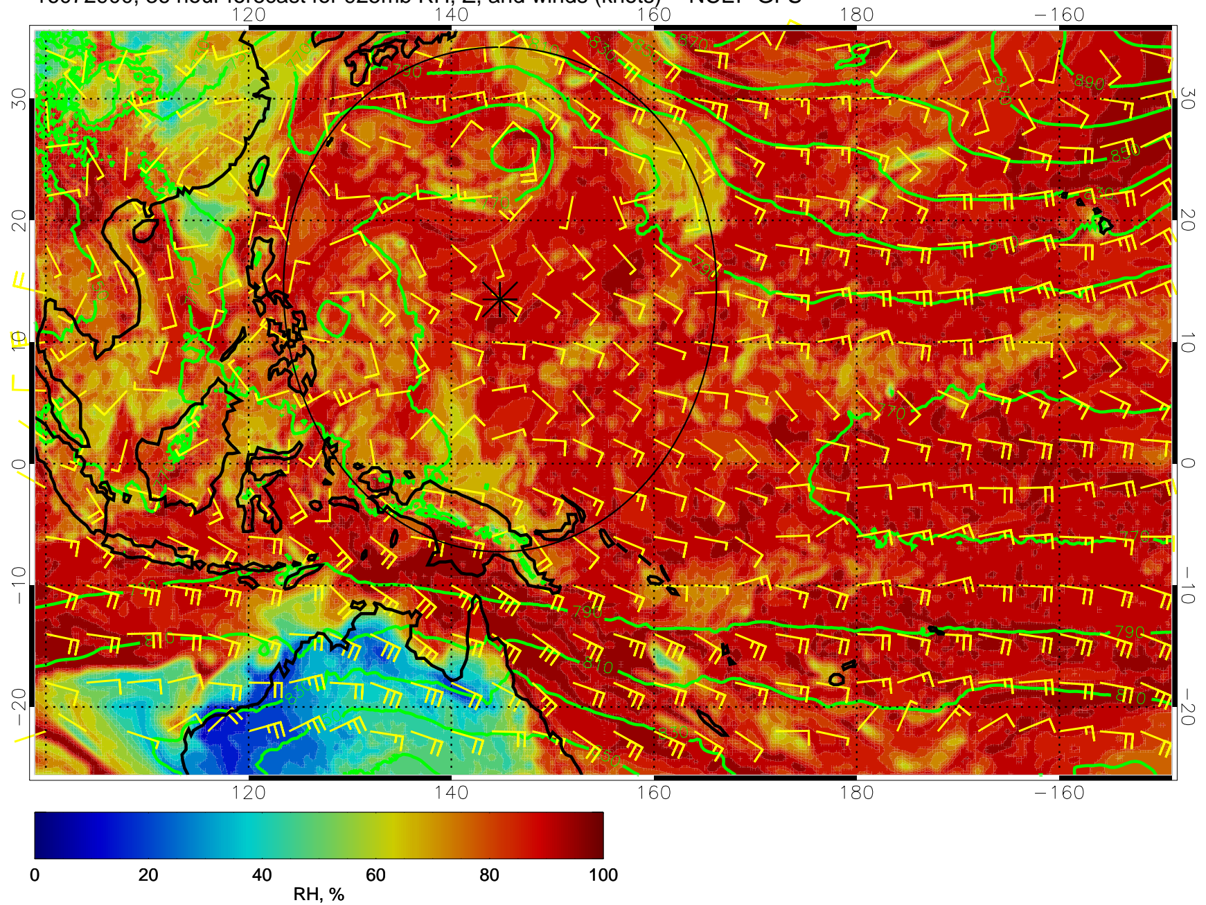
16072900, 36 hour forecast for 925mb RH, Z, and winds (knots) -- NCEP GFS
