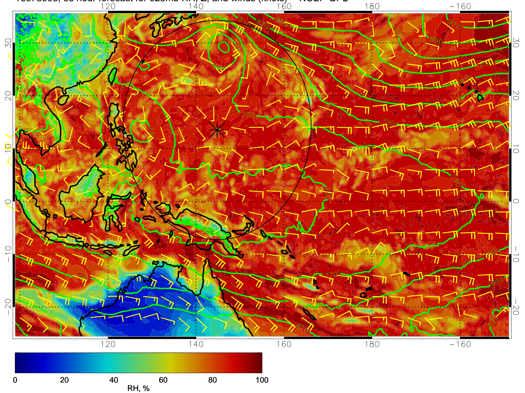
16073006, 66 hour forecast for 925mb RH, Z, and winds (knots) -- NCEP GFS
