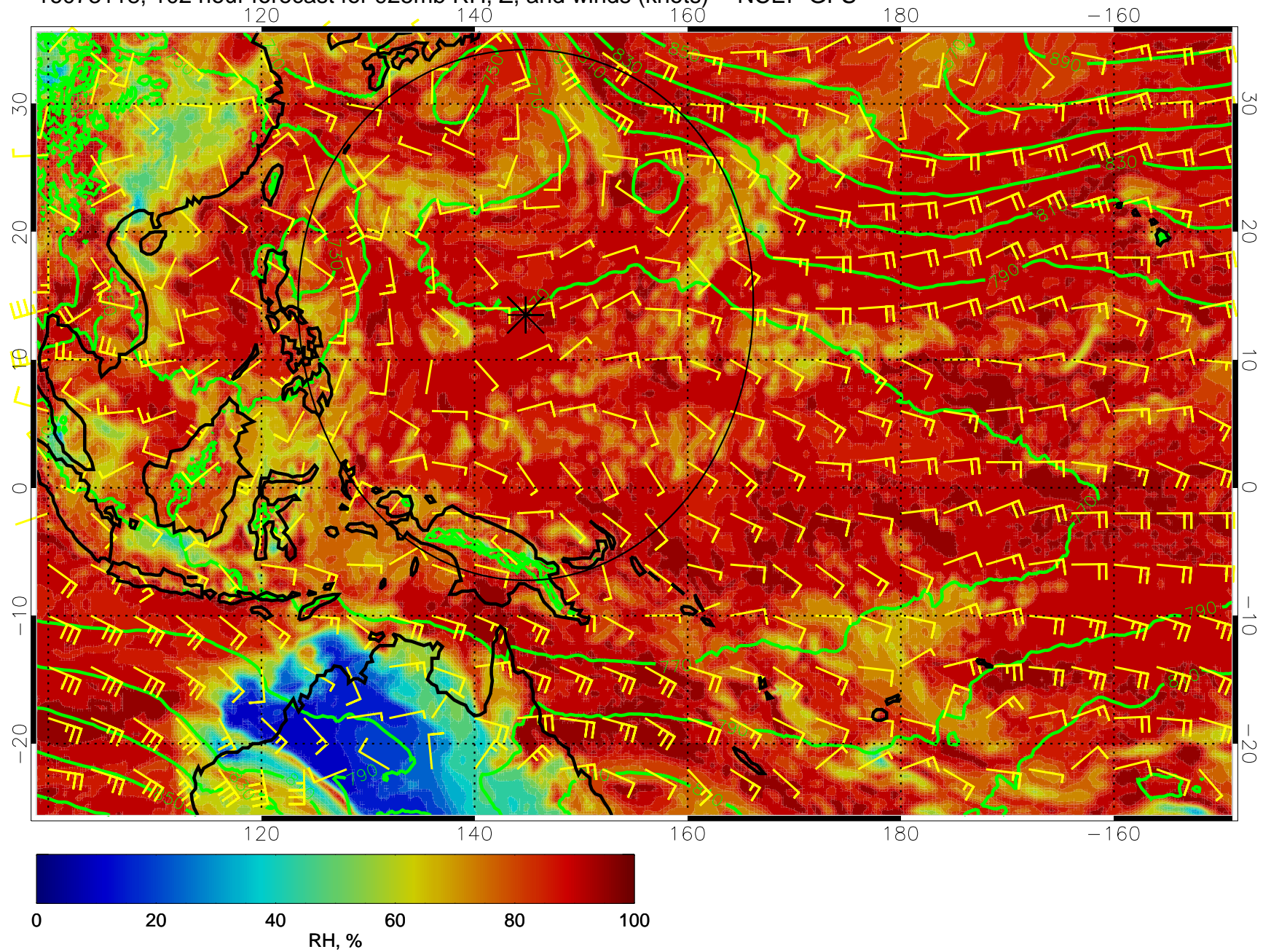
16073118, 102 hour forecast for 925mb RH, Z, and winds (knots) -- NCEP GFS
