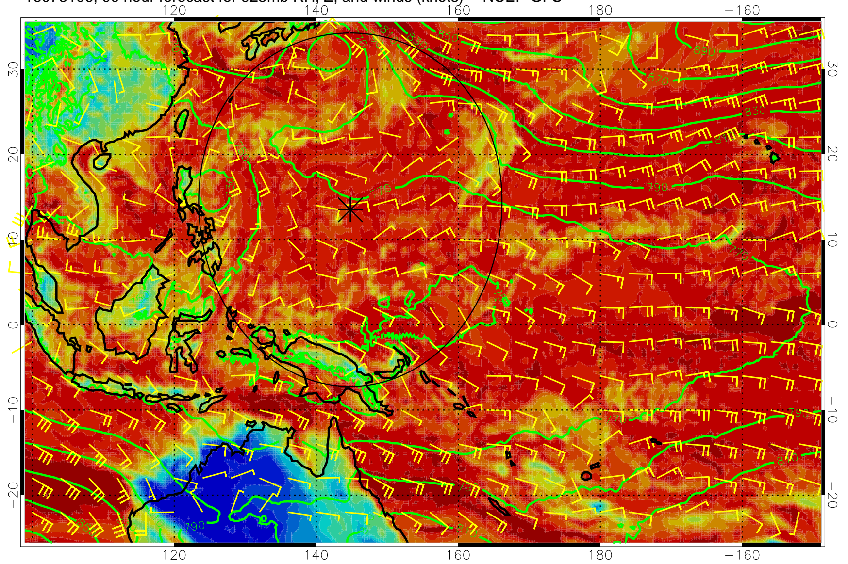
16073106, 90 hour forecast for 925mb RH, Z, and winds (knots) -- NCEP GFS
