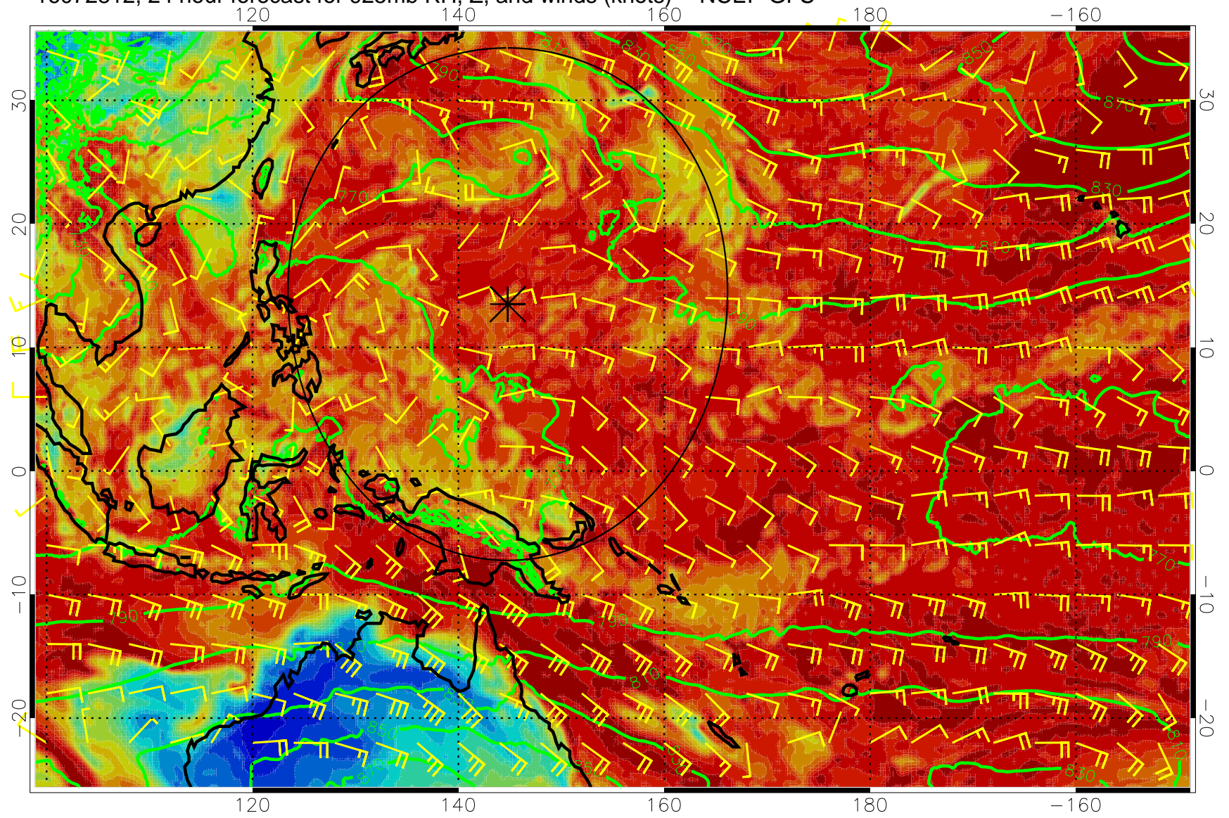
16072812, 24 hour forecast for 925mb RH, Z, and winds (knots) -- NCEP GFS
