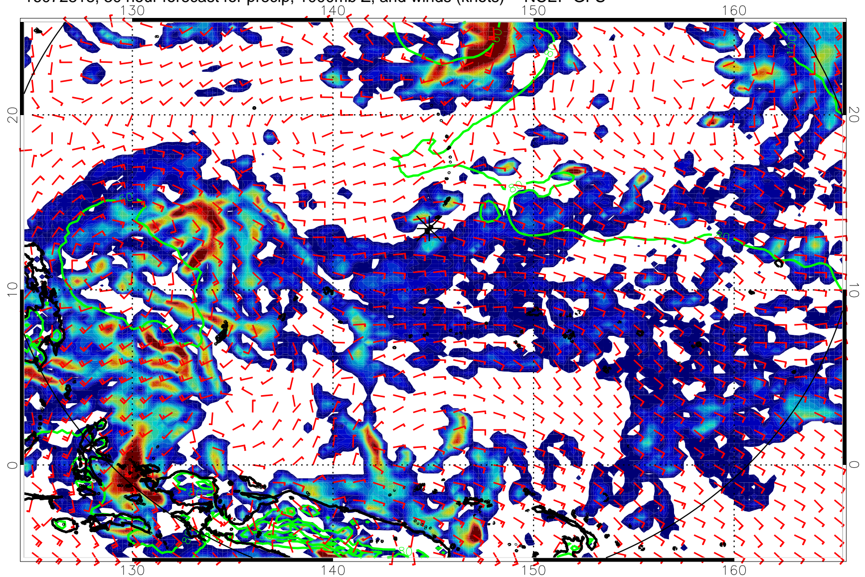
16072818, 30 hour forecast for precip, 1000mb Z, and winds (knots) -- NCEP GFS
