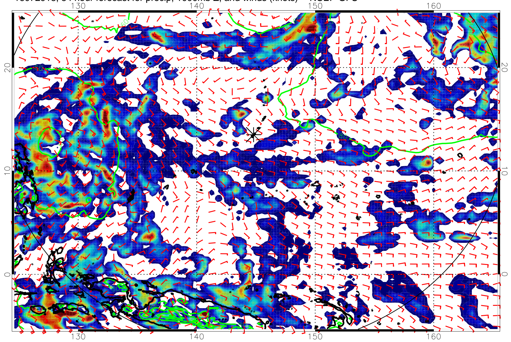
16072918, 54 hour forecast for precip, 1000mb Z, and winds (knots) -- NCEP GFS
