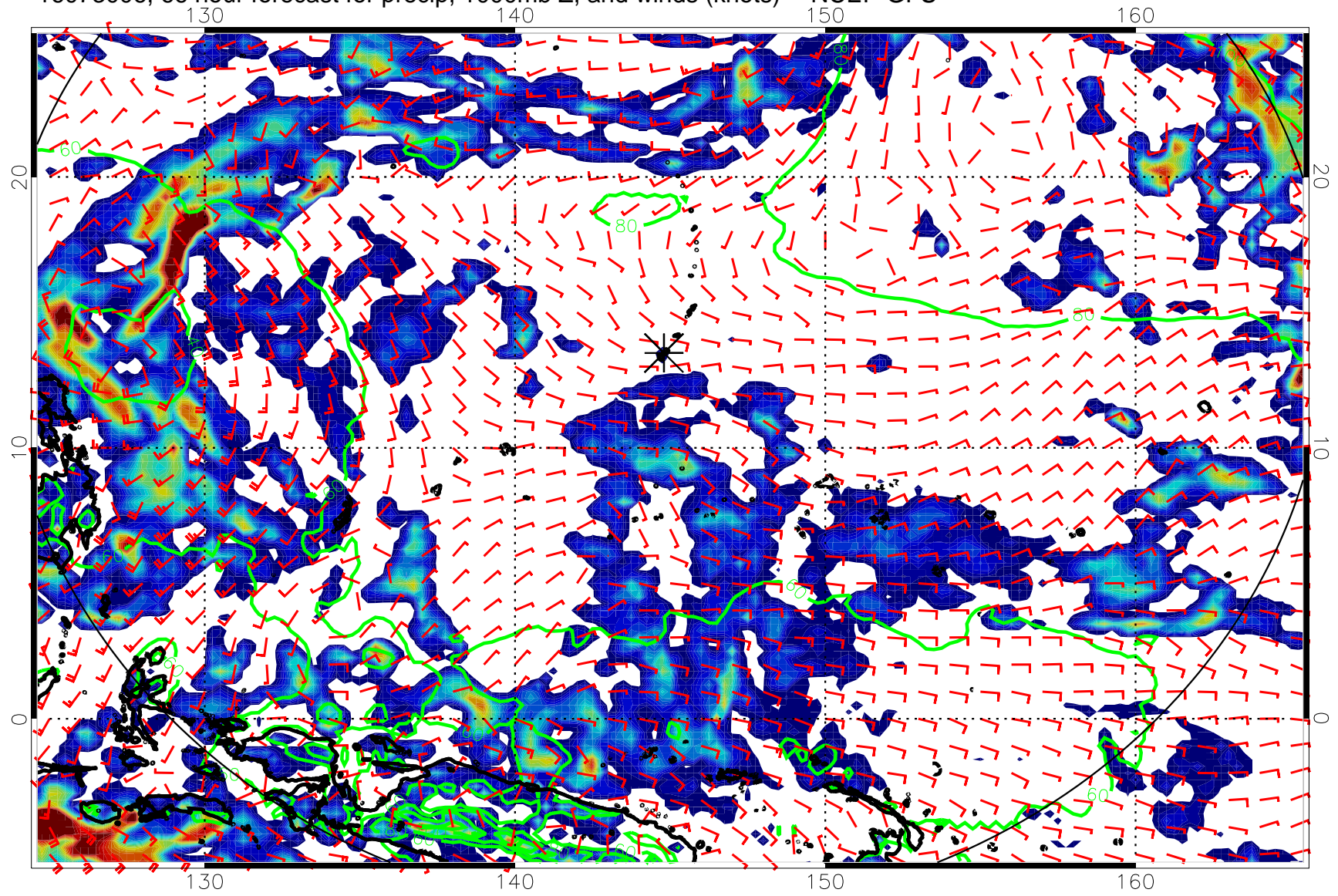
16073006, 66 hour forecast for precip, 1000mb Z, and winds (knots) -- NCEP GFS
