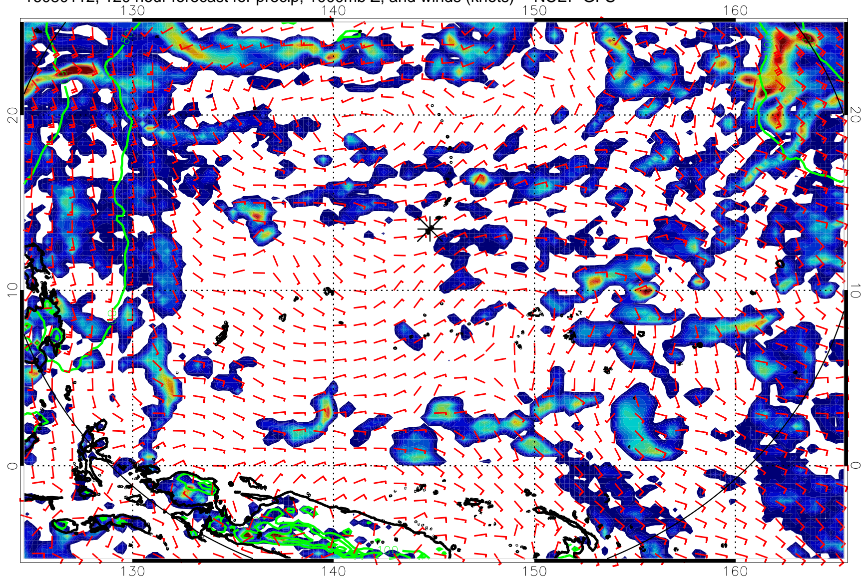
16080112, 120 hour forecast for precip, 1000mb Z, and winds (knots) -- NCEP GFS
