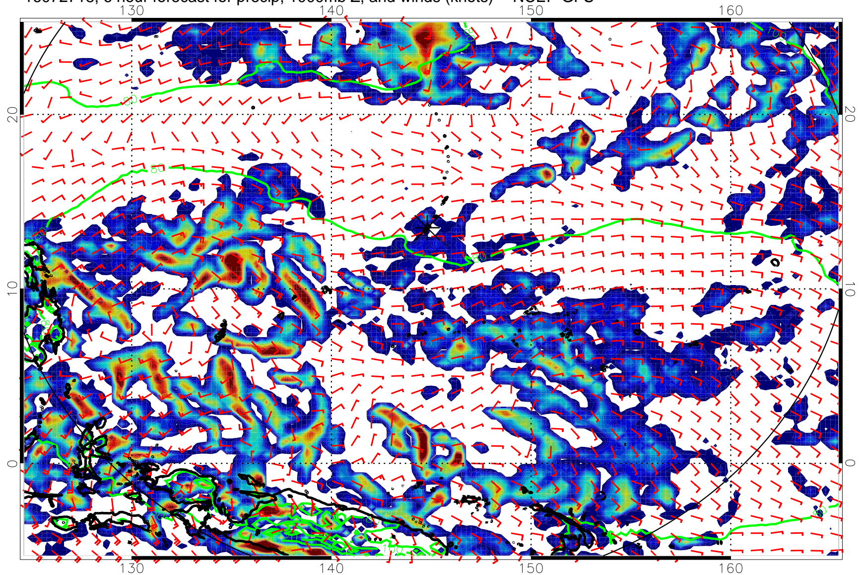
16072718, 6 hour forecast for precip, 1000mb Z, and winds (knots) -- NCEP GFS
