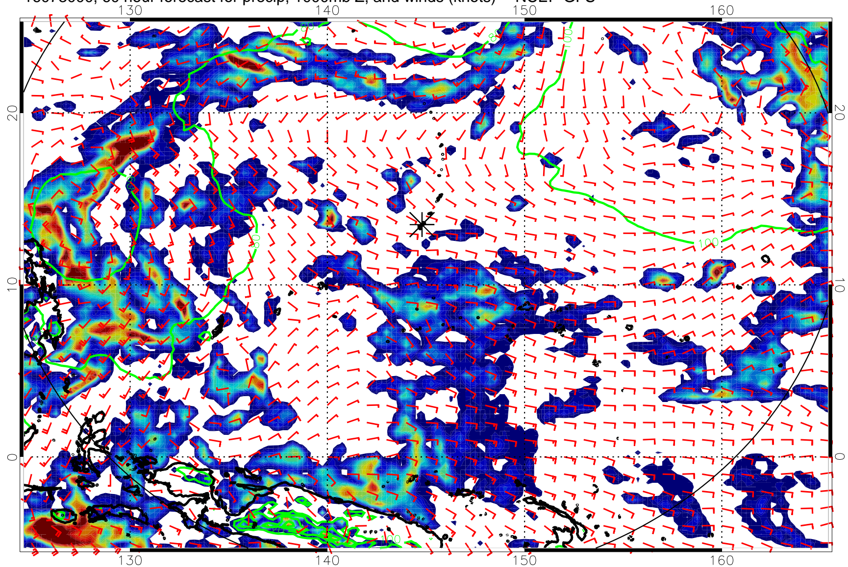
16073000, 60 hour forecast for precip, 1000mb Z, and winds (knots) -- NCEP GFS
