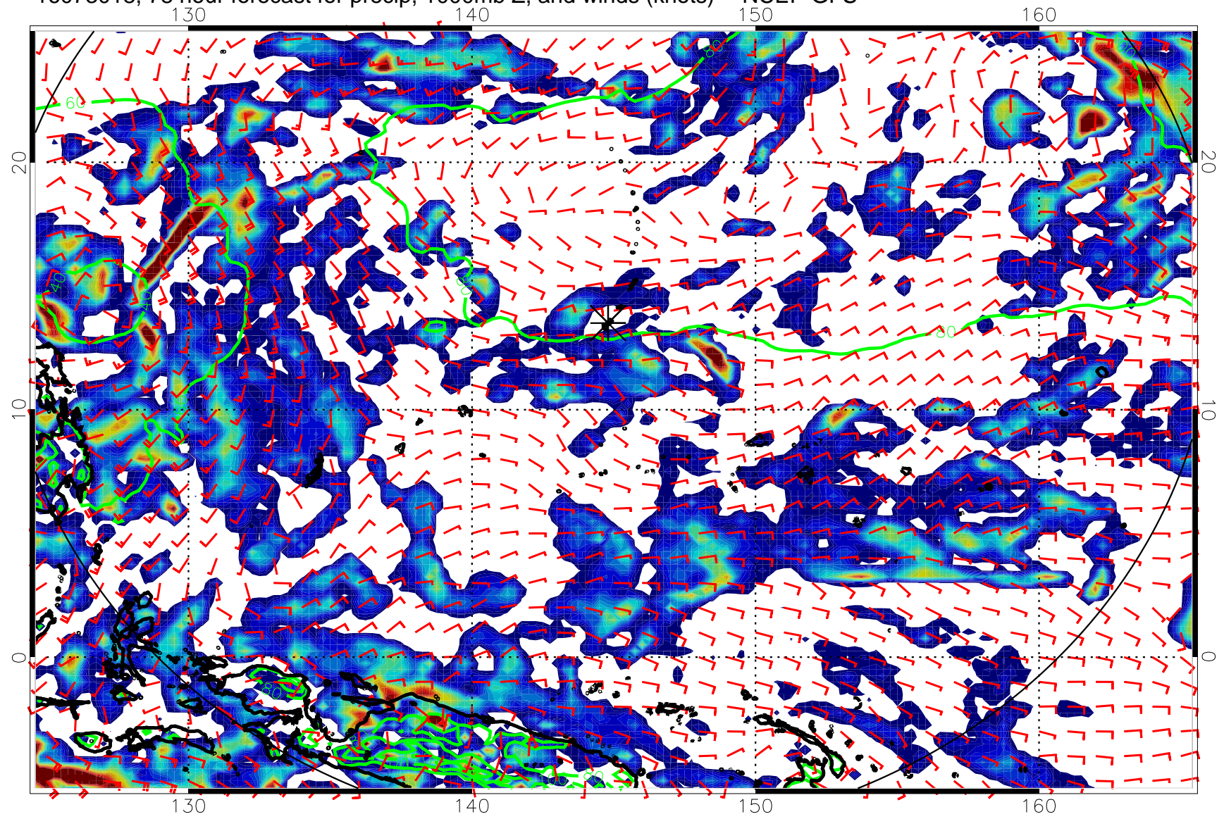
16073018, 78 hour forecast for precip, 1000mb Z, and winds (knots) -- NCEP GFS
