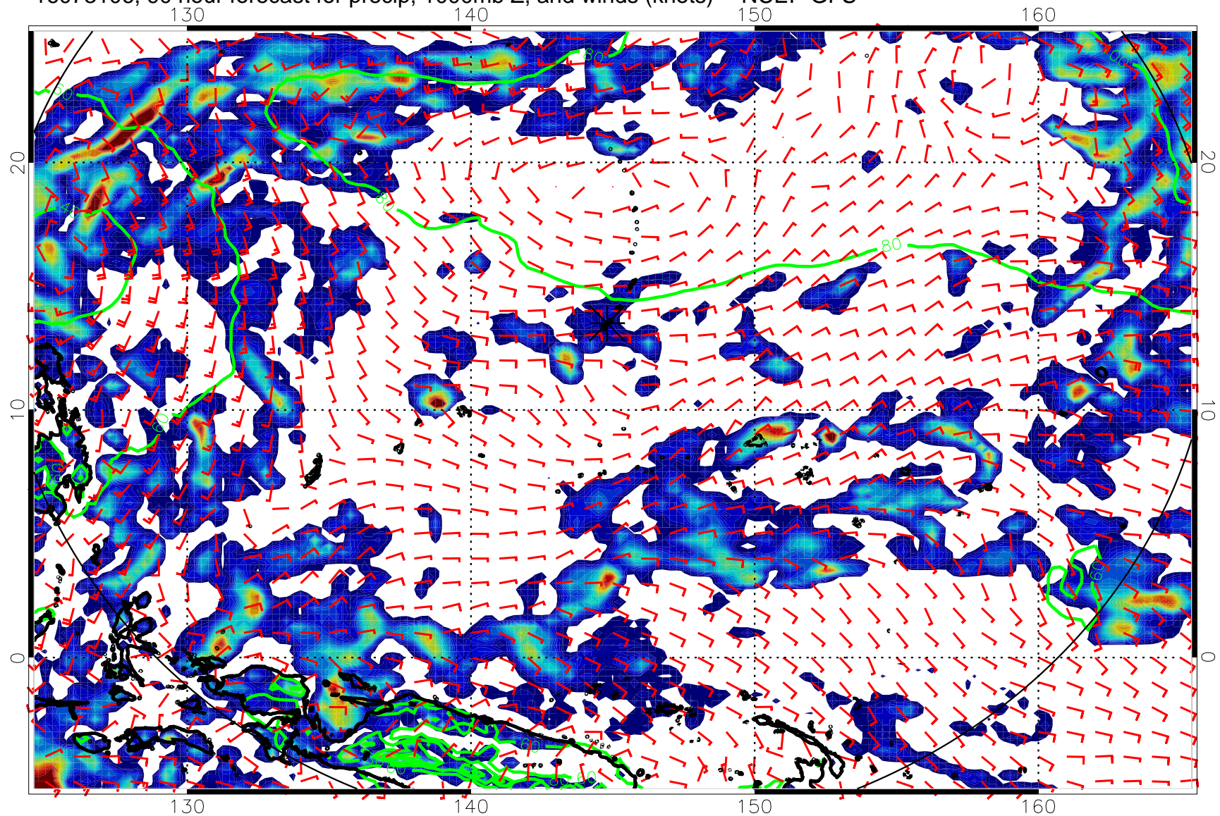
16073106, 90 hour forecast for precip, 1000mb Z, and winds (knots) -- NCEP GFS
