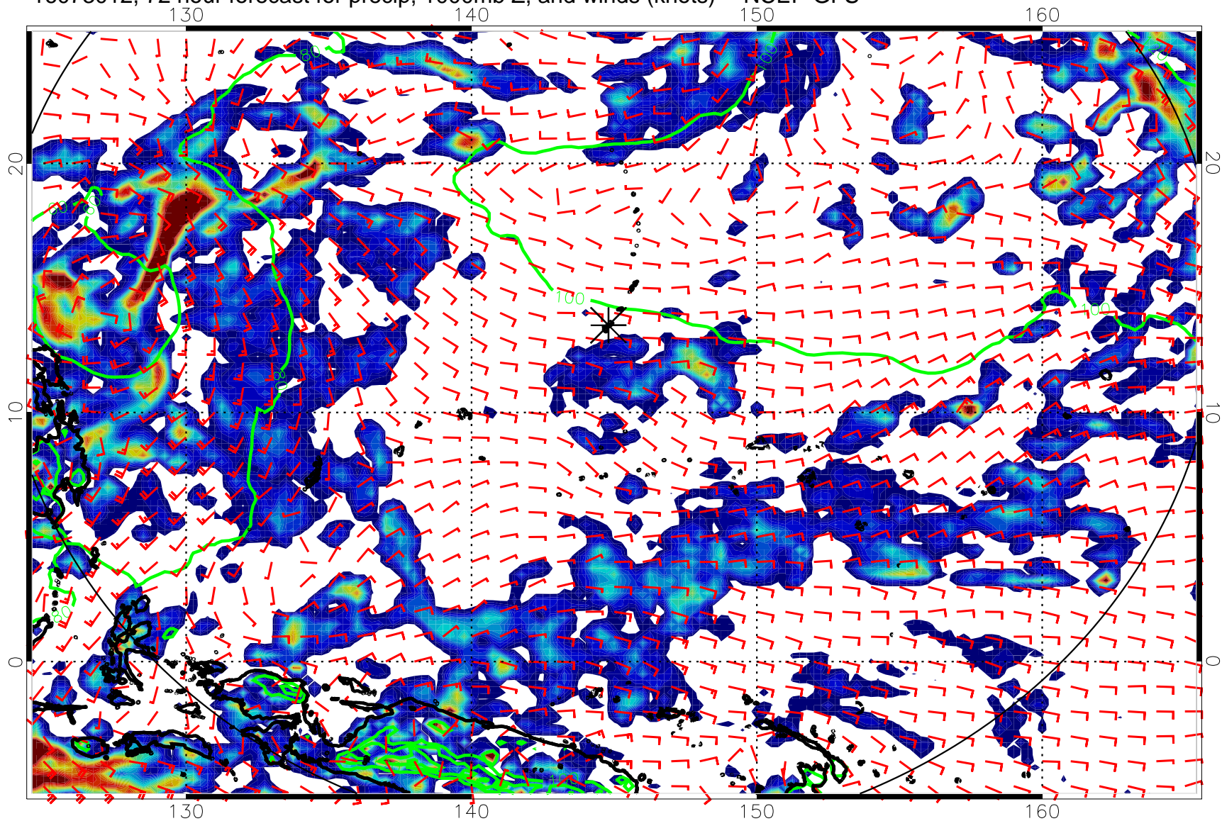
16073012, 72 hour forecast for precip, 1000mb Z, and winds (knots) -- NCEP GFS
