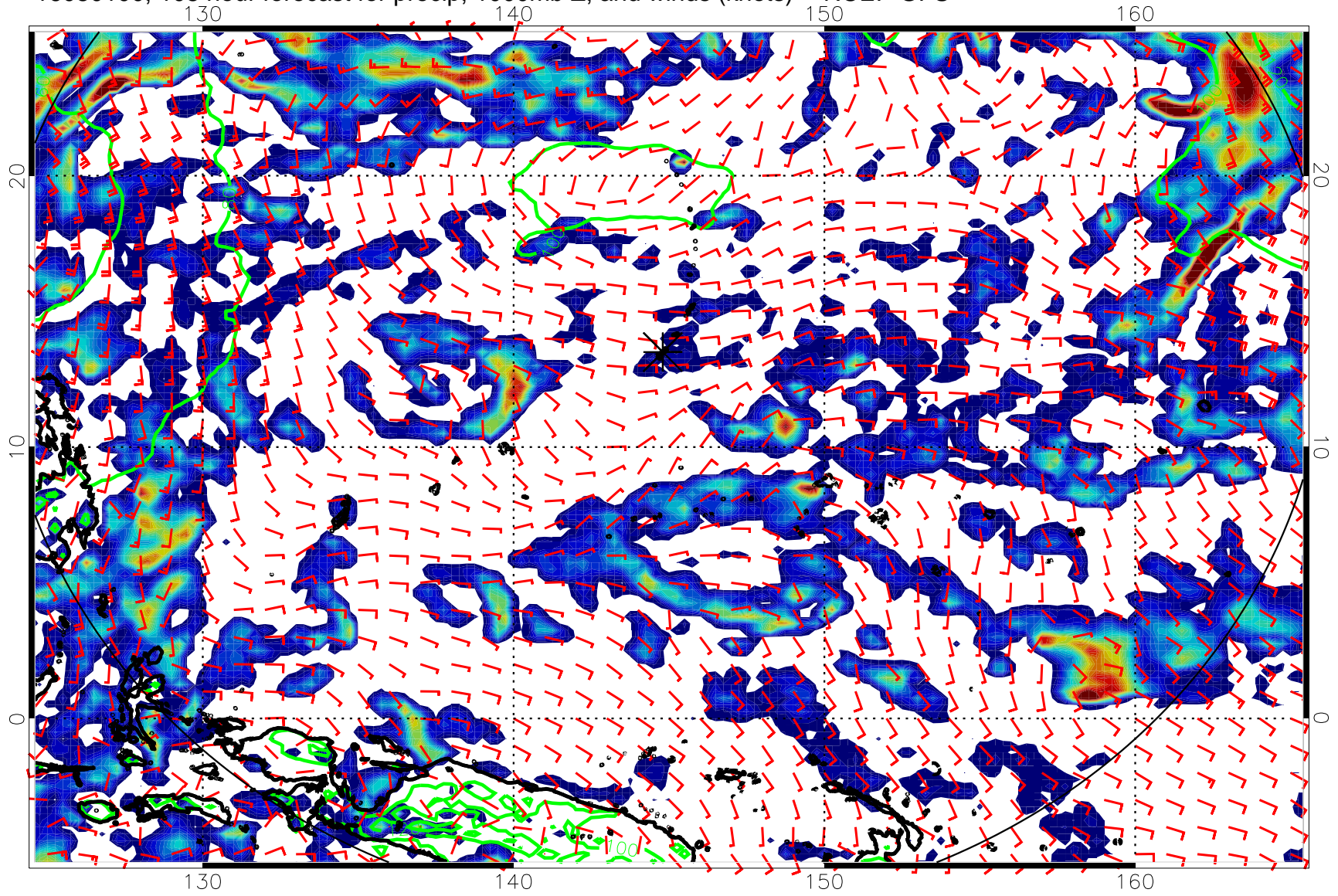
16080100, 108 hour forecast for precip, 1000mb Z, and winds (knots) -- NCEP GFS
