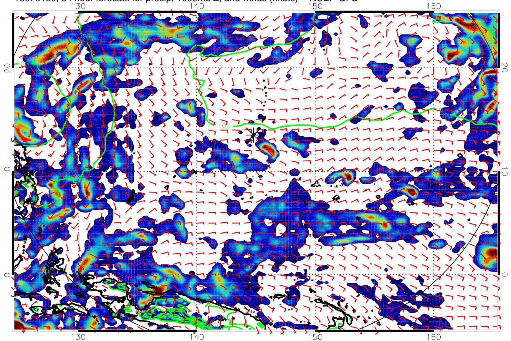
16073100, 84 hour forecast for precip, 1000mb Z, and winds (knots) -- NCEP GFS
