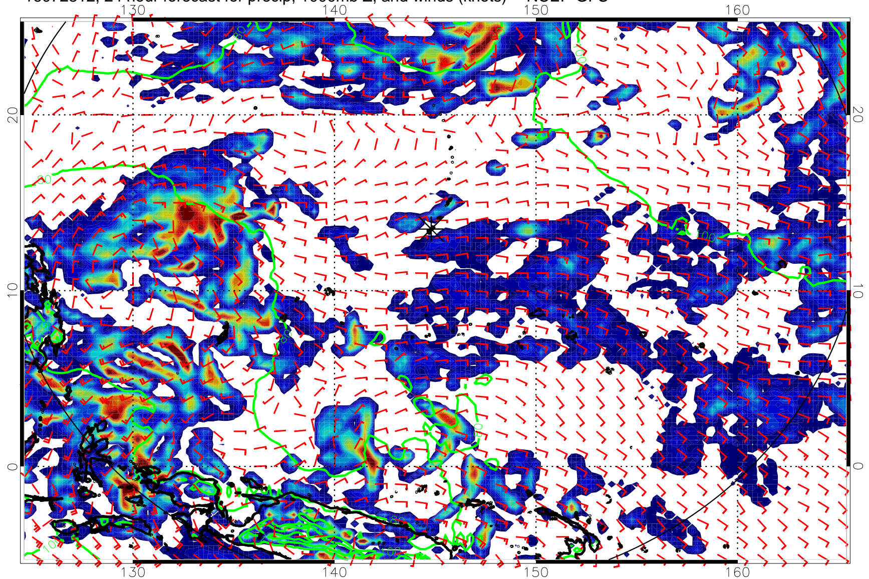
16072812, 24 hour forecast for precip, 1000mb Z, and winds (knots) -- NCEP GFS
