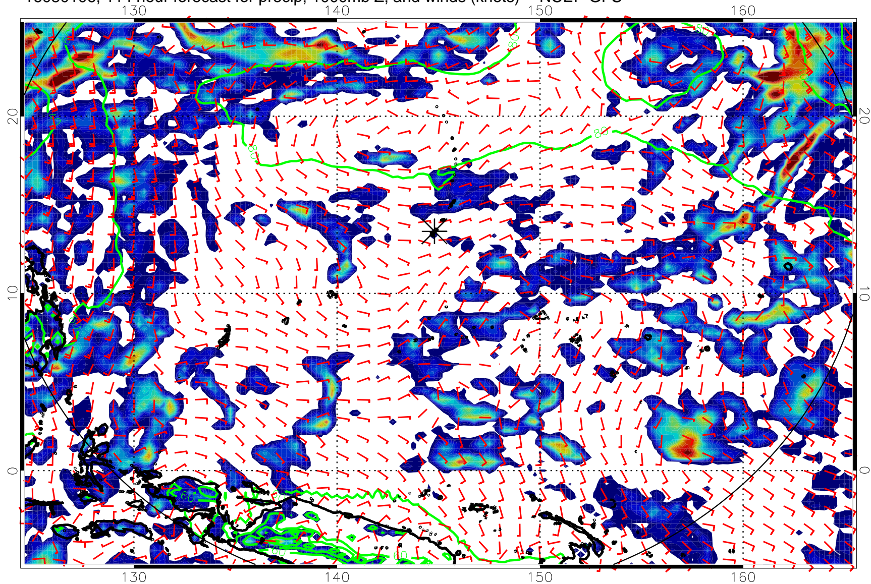
16080106, 114 hour forecast for precip, 1000mb Z, and winds (knots) -- NCEP GFS
