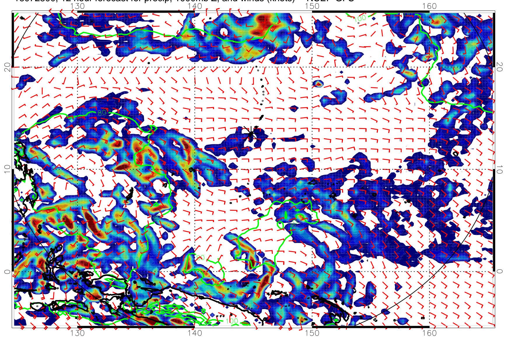
16072800, 12 hour forecast for precip, 1000mb Z, and winds (knots) -- NCEP GFS
