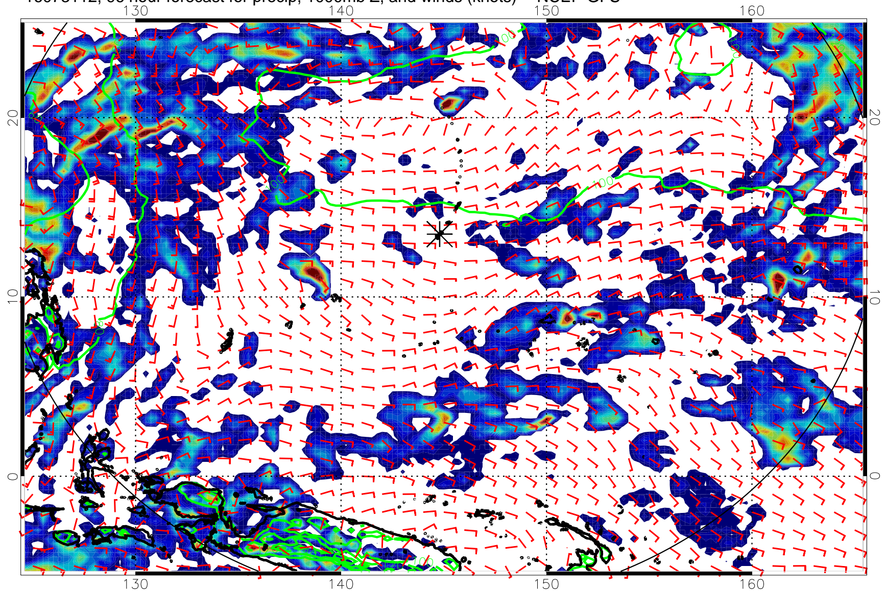
16073112, 96 hour forecast for precip, 1000mb Z, and winds (knots) -- NCEP GFS
