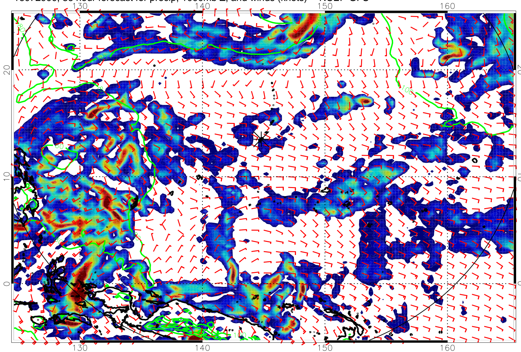
16072900, 36 hour forecast for precip, 1000mb Z, and winds (knots) -- NCEP GFS
