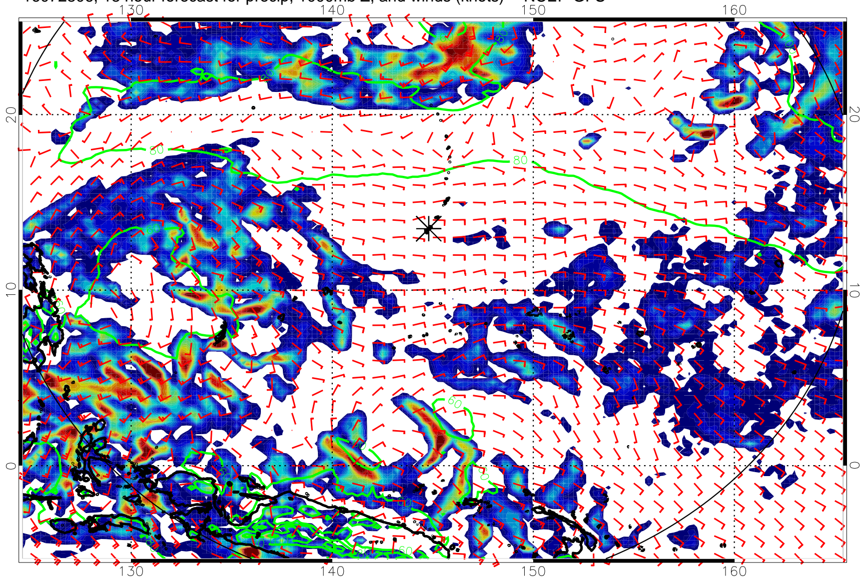
16072806, 18 hour forecast for precip, 1000mb Z, and winds (knots) -- NCEP GFS
