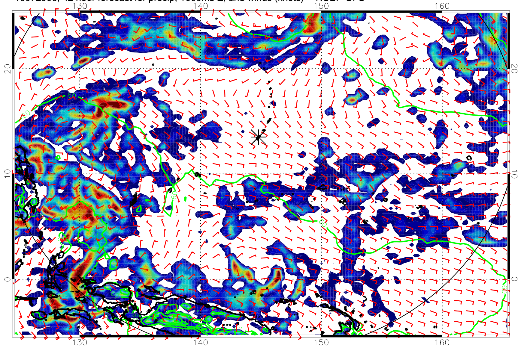
16072906, 42 hour forecast for precip, 1000mb Z, and winds (knots) -- NCEP GFS
