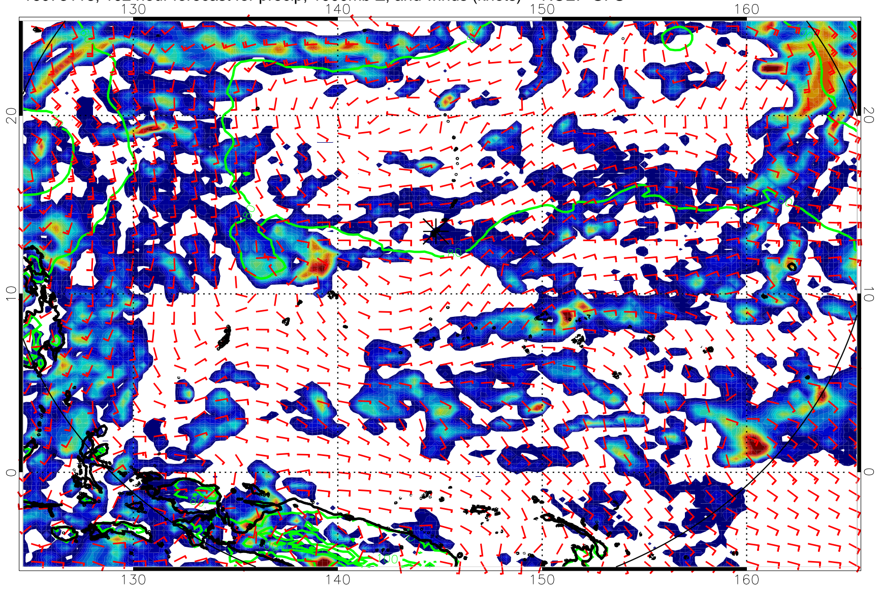
16073118, 102 hour forecast for precip, 1000mb Z, and winds (knots) -- NCEP GFS
