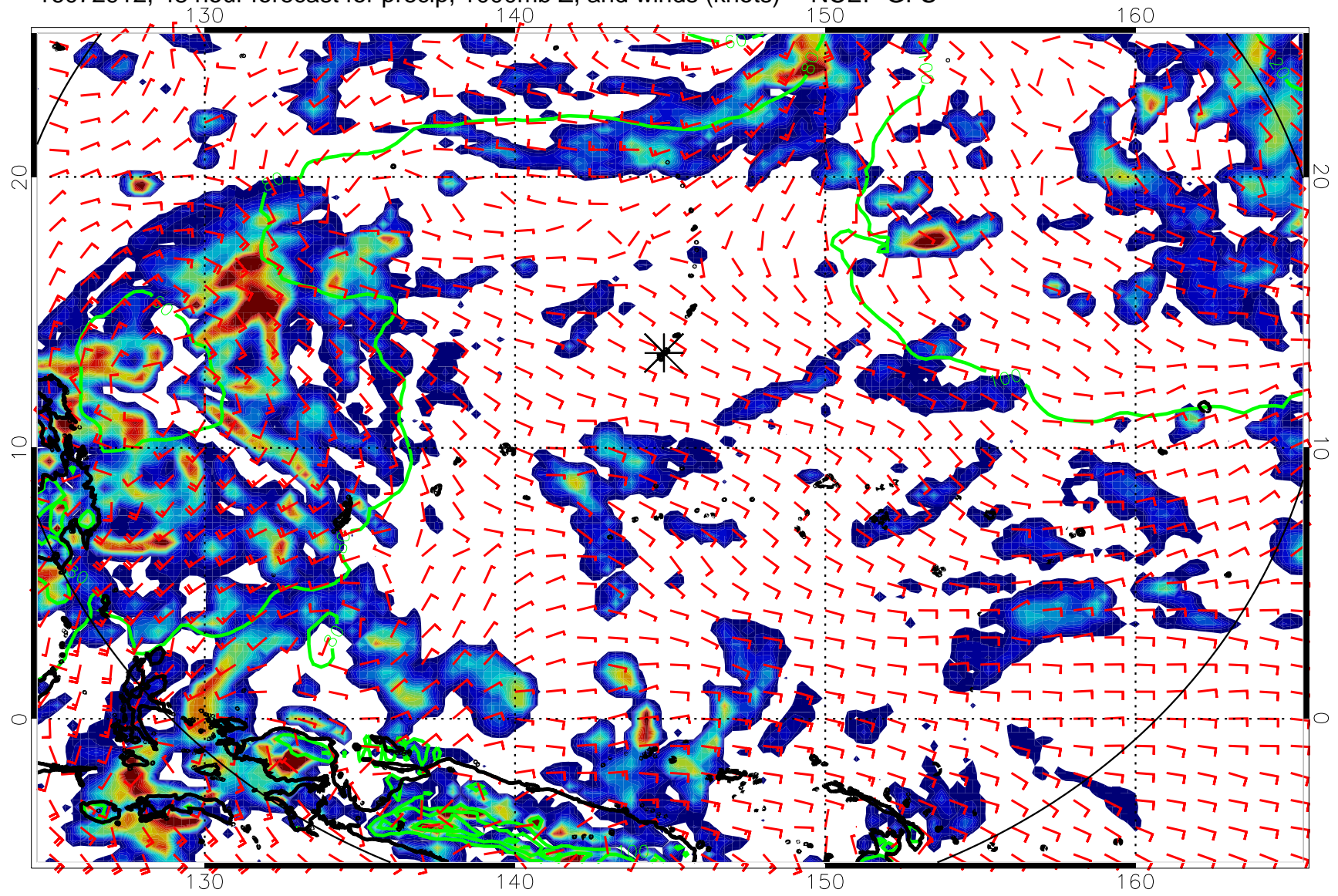
16072912, 48 hour forecast for precip, 1000mb Z, and winds (knots) -- NCEP GFS
