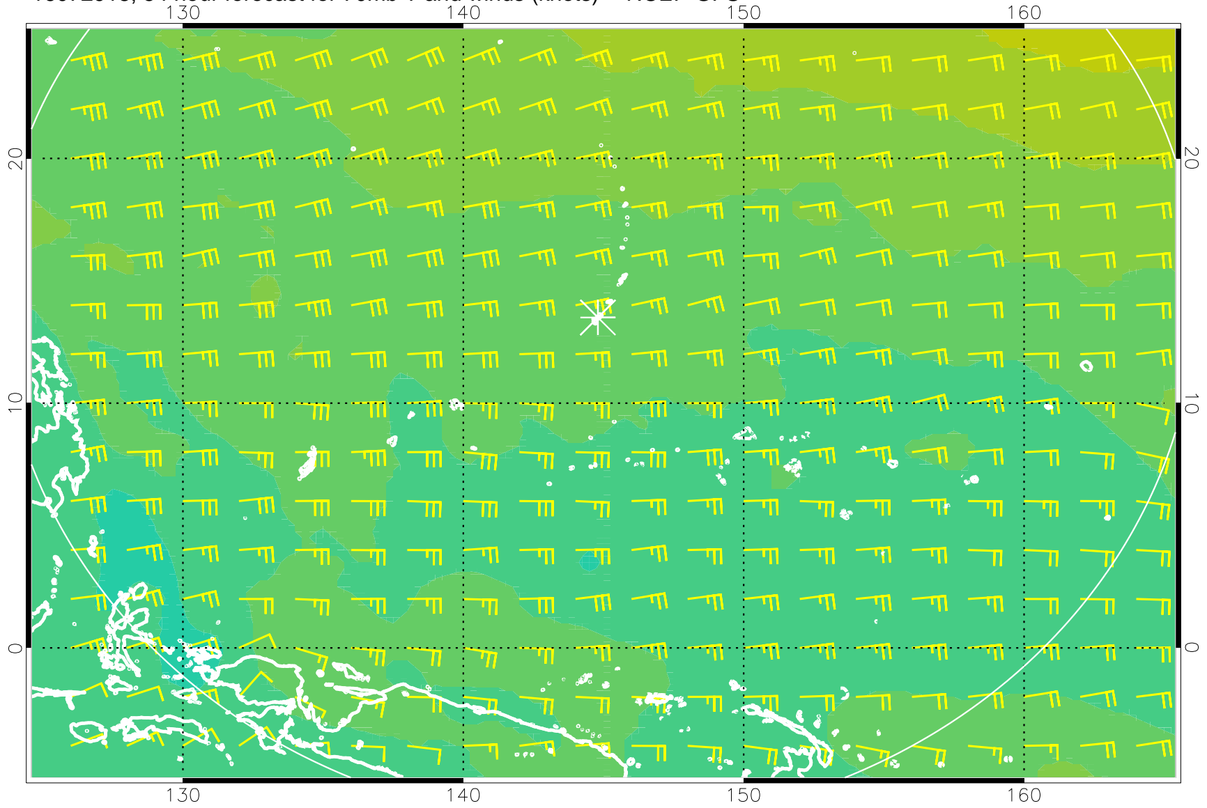
16072918, 54 hour forecast for 70mb T and winds (knots) -- NCEP GFS
