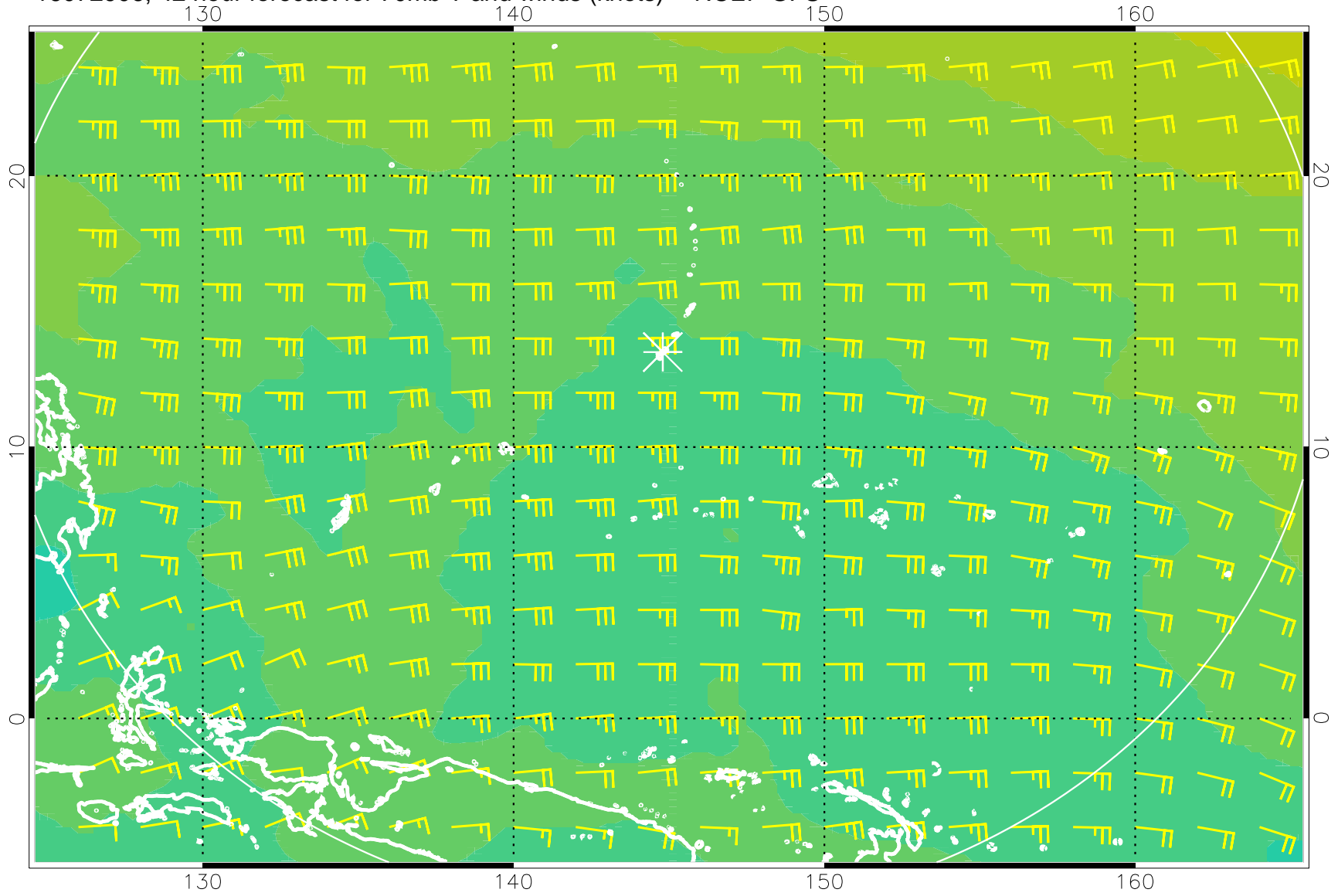
16072906, 42 hour forecast for 70mb T and winds (knots) -- NCEP GFS
