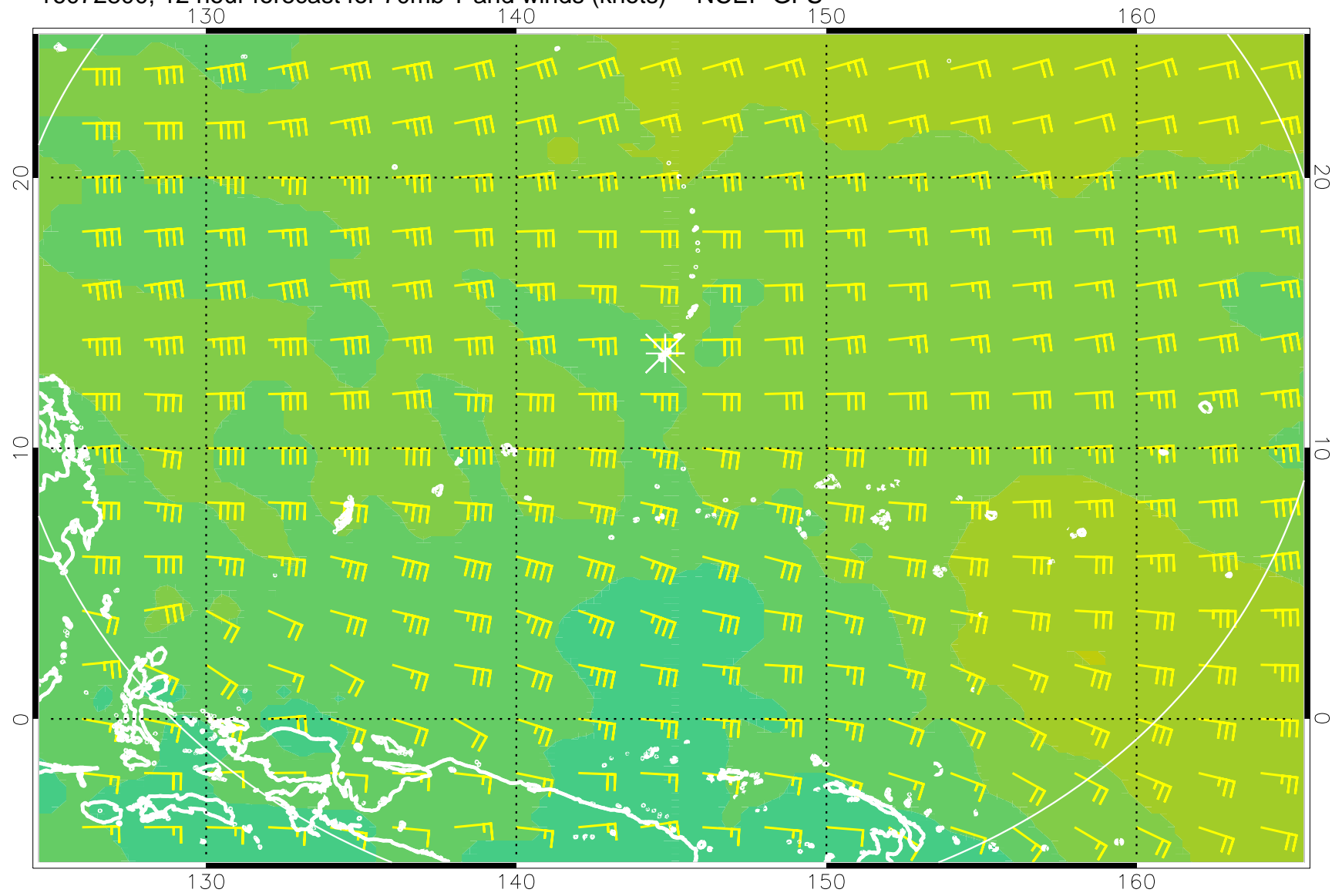
16072800, 12 hour forecast for 70mb T and winds (knots) -- NCEP GFS
