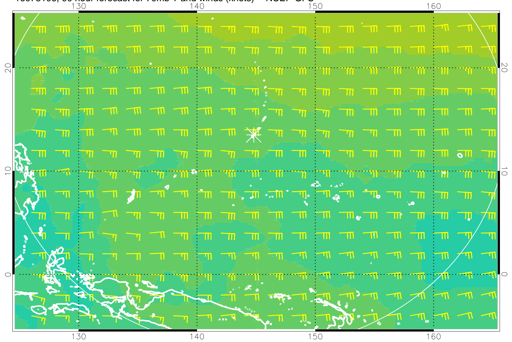
16073106, 90 hour forecast for 70mb T and winds (knots) -- NCEP GFS
