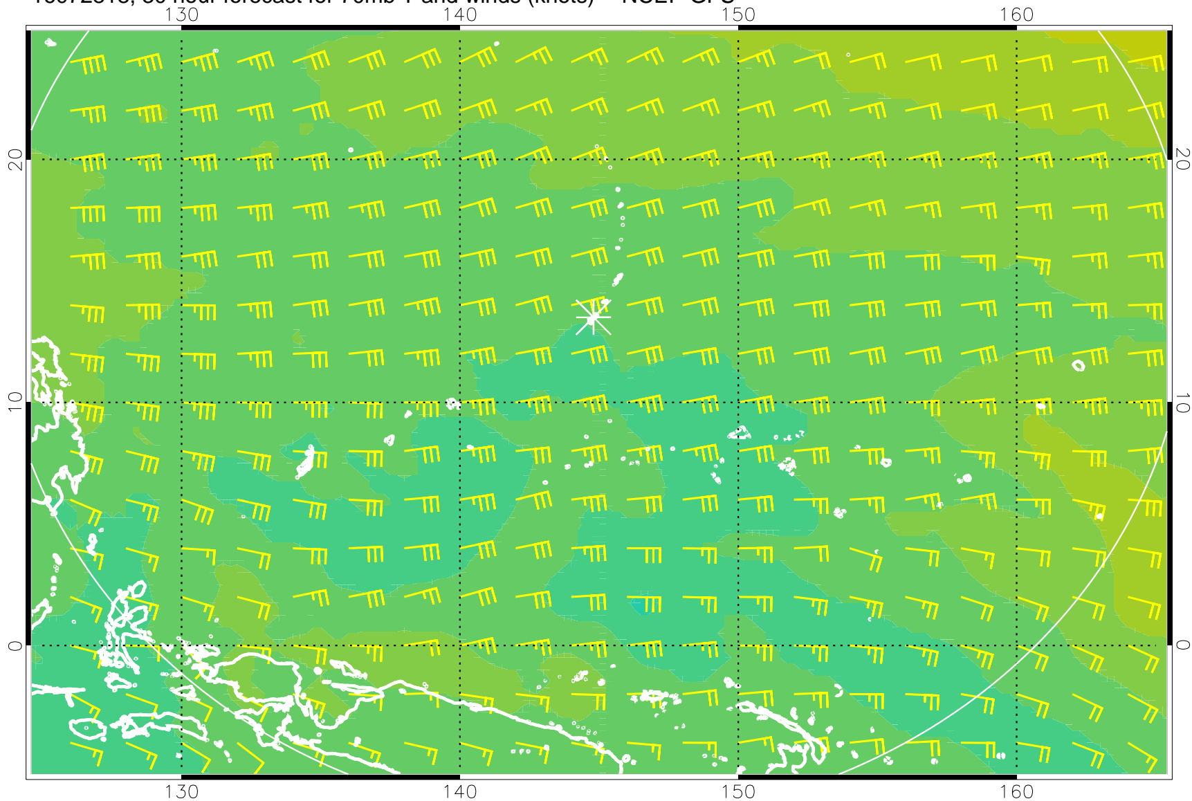
16072818, 30 hour forecast for 70mb T and winds (knots) -- NCEP GFS
