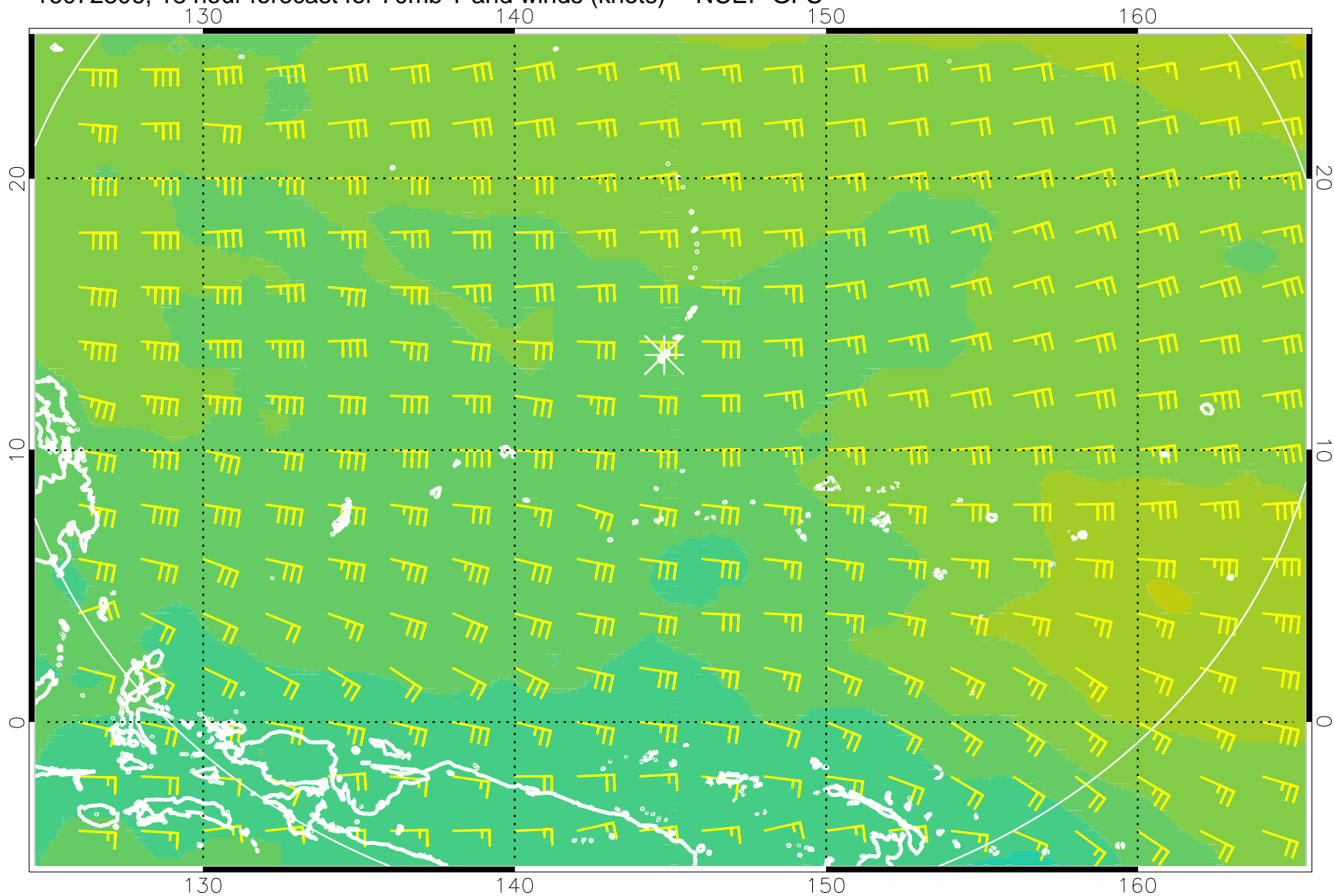
16072806, 18 hour forecast for 70mb T and winds (knots) -- NCEP GFS
