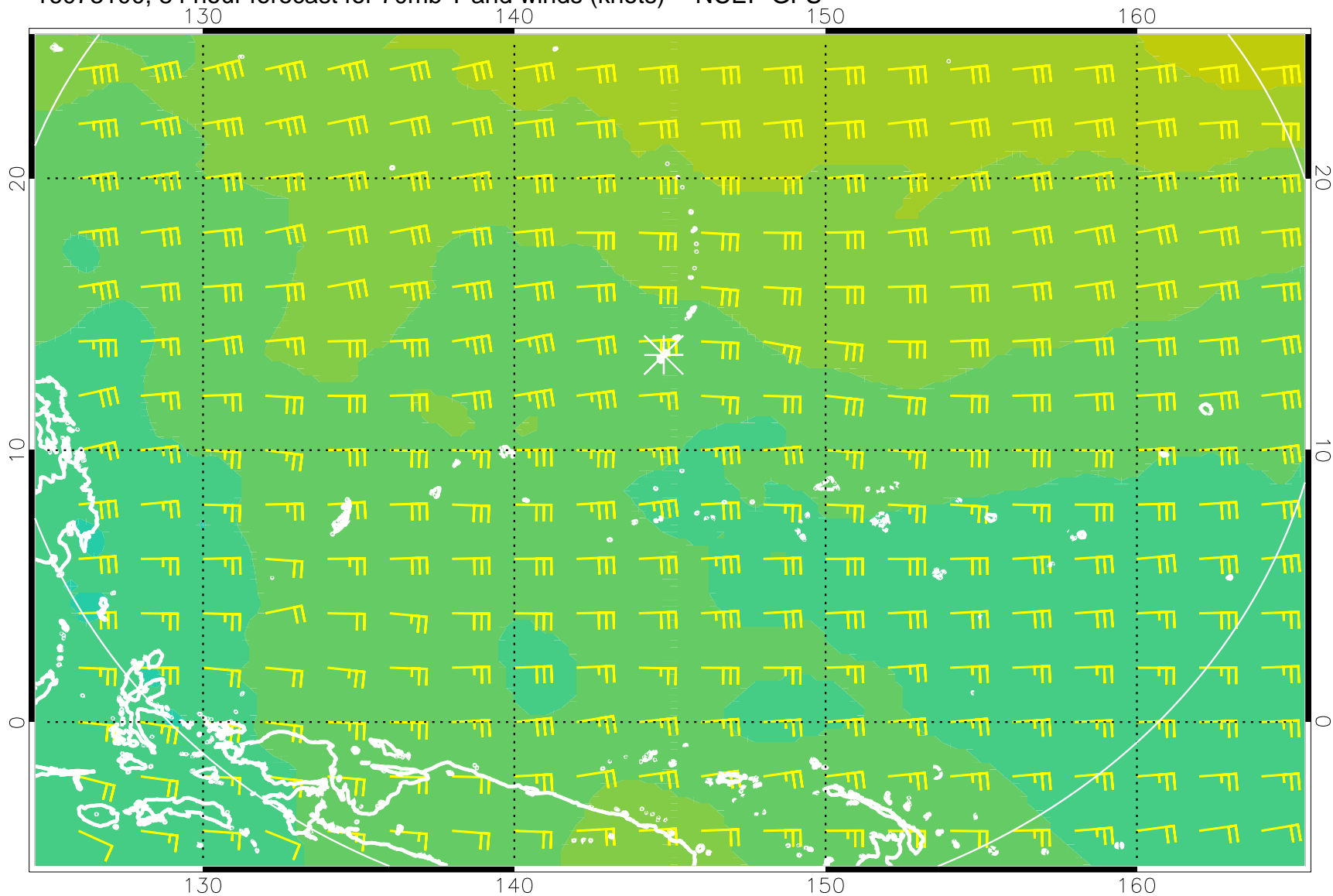
16073100, 84 hour forecast for 70mb T and winds (knots) -- NCEP GFS
