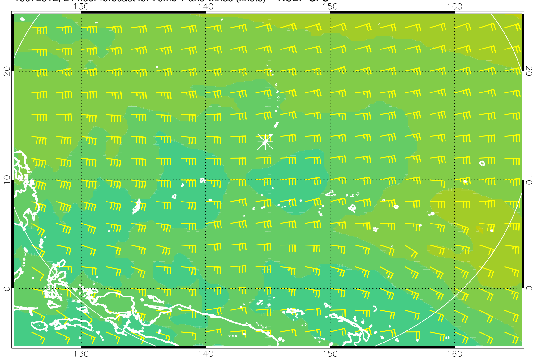
16072812, 24 hour forecast for 70mb T and winds (knots) -- NCEP GFS
