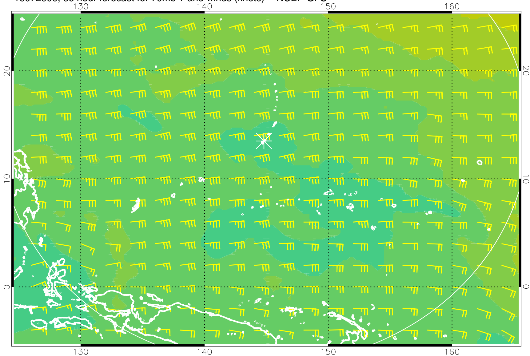
16072900, 36 hour forecast for 70mb T and winds (knots) -- NCEP GFS
