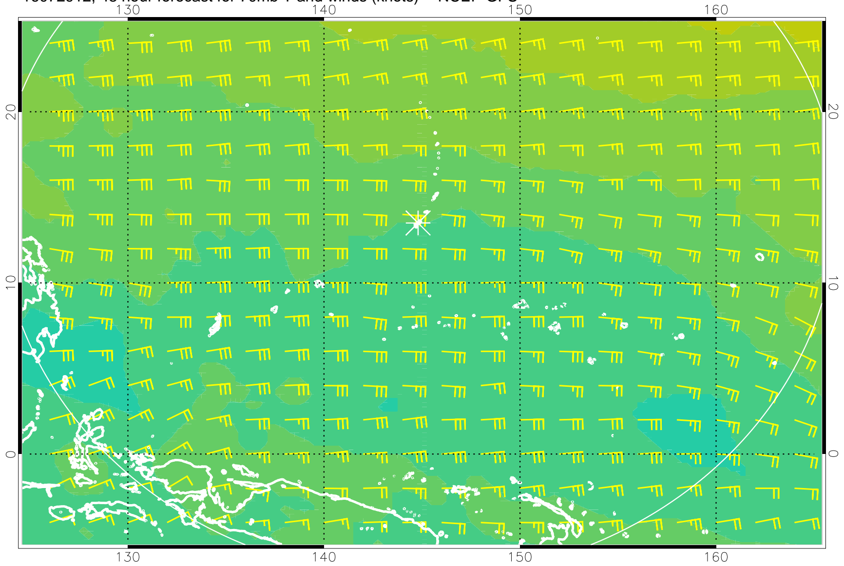
16072912, 48 hour forecast for 70mb T and winds (knots) -- NCEP GFS
