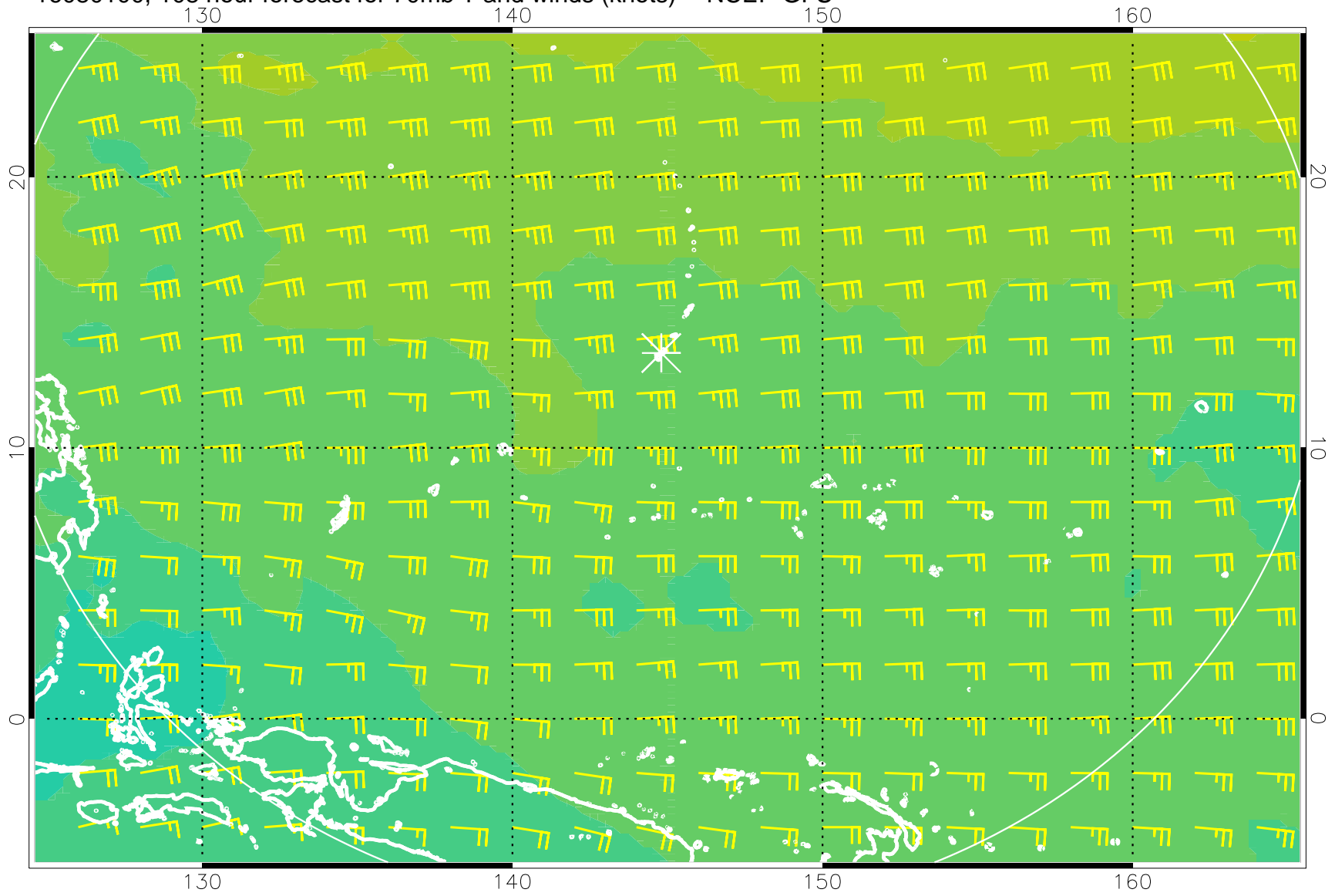
16080100, 108 hour forecast for 70mb T and winds (knots) -- NCEP GFS
