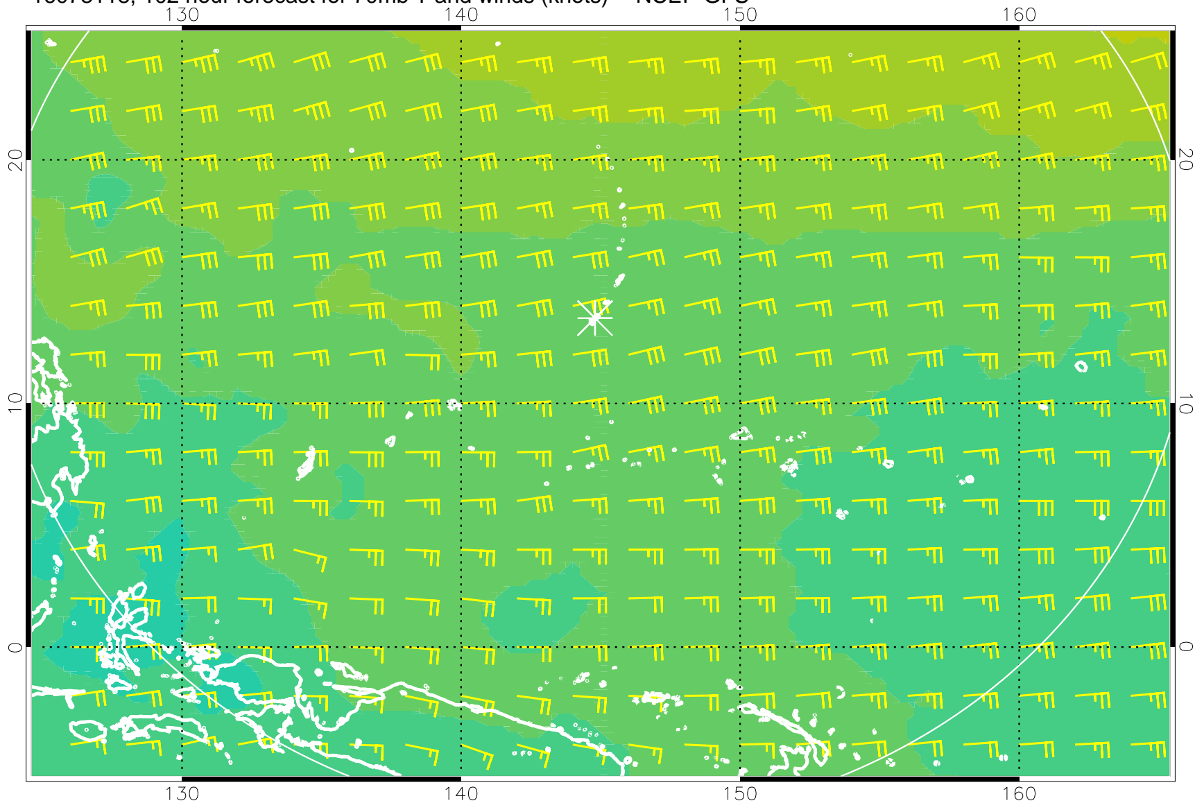
16073118, 102 hour forecast for 70mb T and winds (knots) -- NCEP GFS
