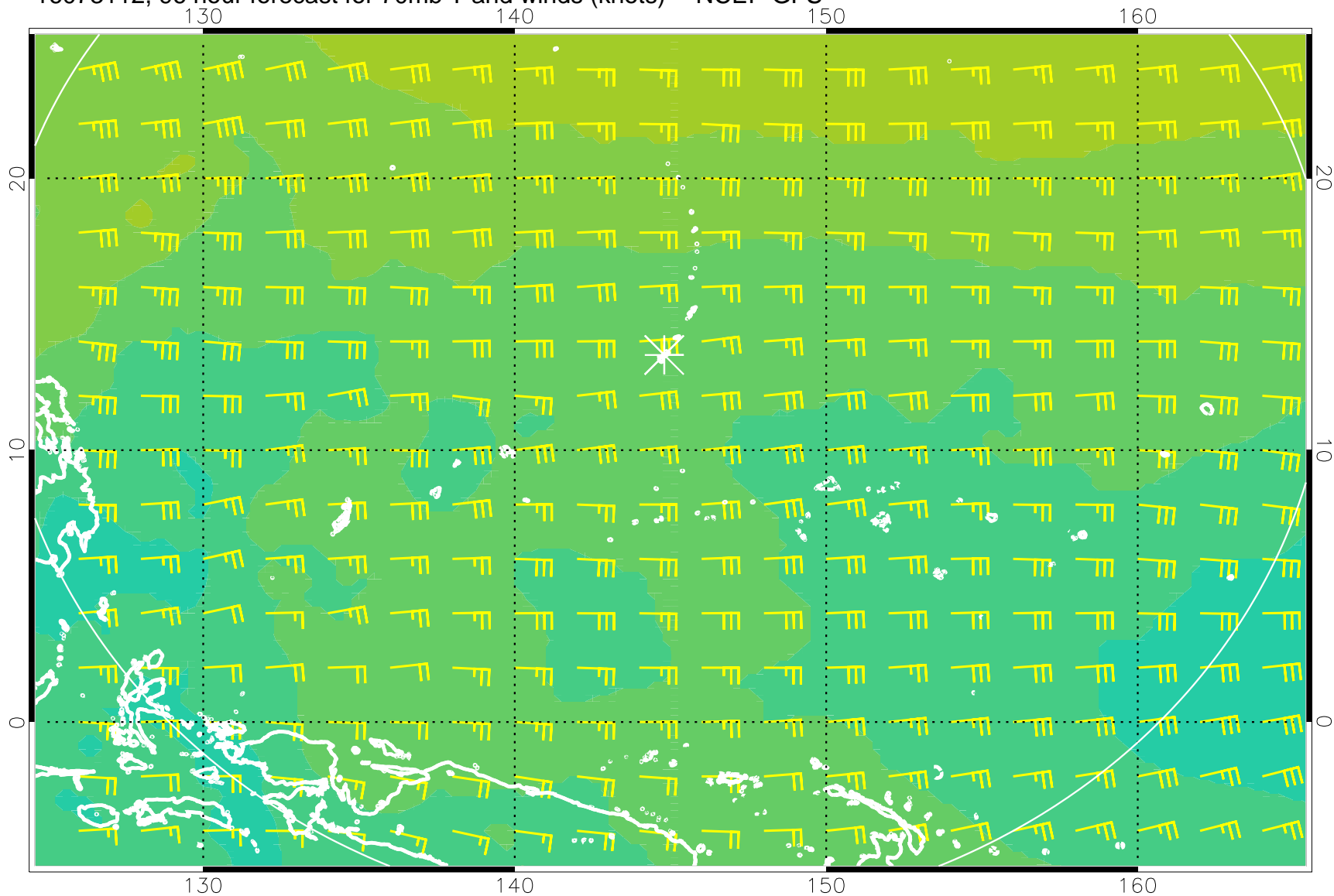
16073112, 96 hour forecast for 70mb T and winds (knots) -- NCEP GFS
