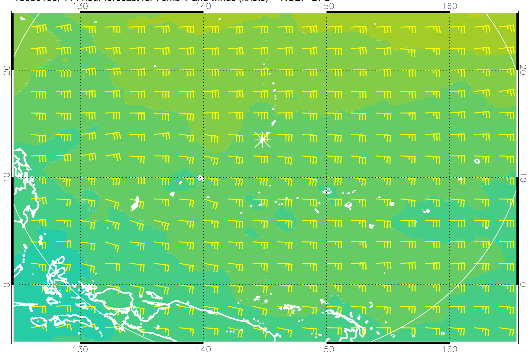
16080106, 114 hour forecast for 70mb T and winds (knots) -- NCEP GFS
