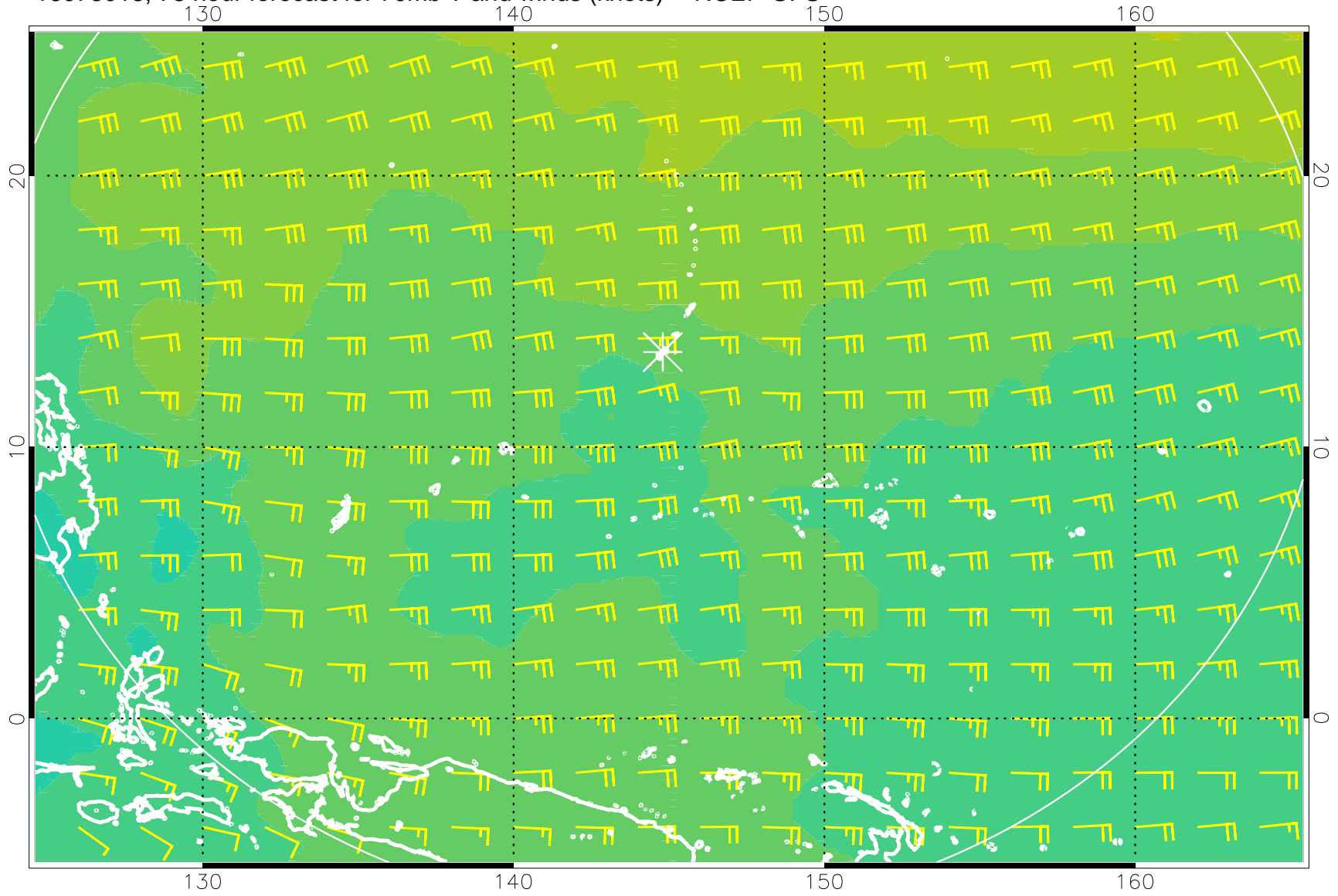
16073018, 78 hour forecast for 70mb T and winds (knots) -- NCEP GFS
