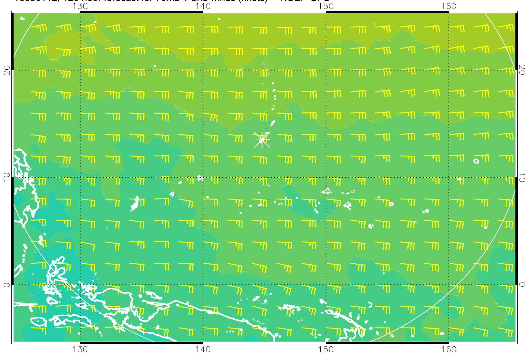
16080112, 120 hour forecast for 70mb T and winds (knots) -- NCEP GFS
