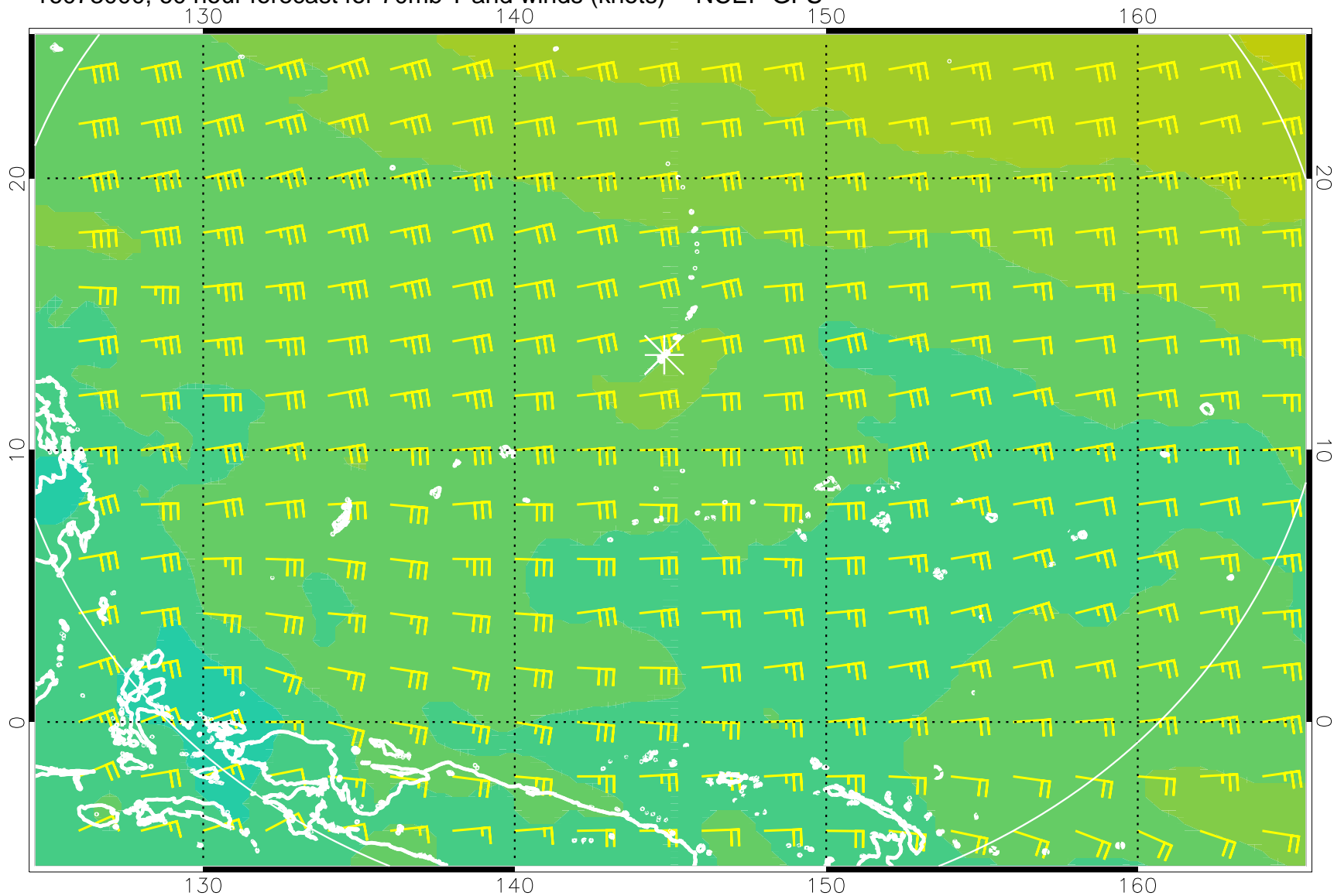
16073000, 60 hour forecast for 70mb T and winds (knots) -- NCEP GFS
