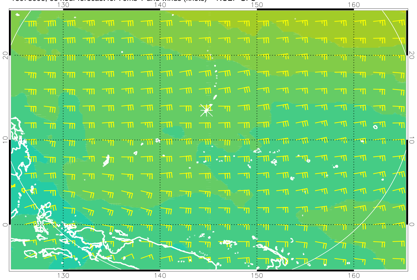
16073006, 66 hour forecast for 70mb T and winds (knots) -- NCEP GFS
