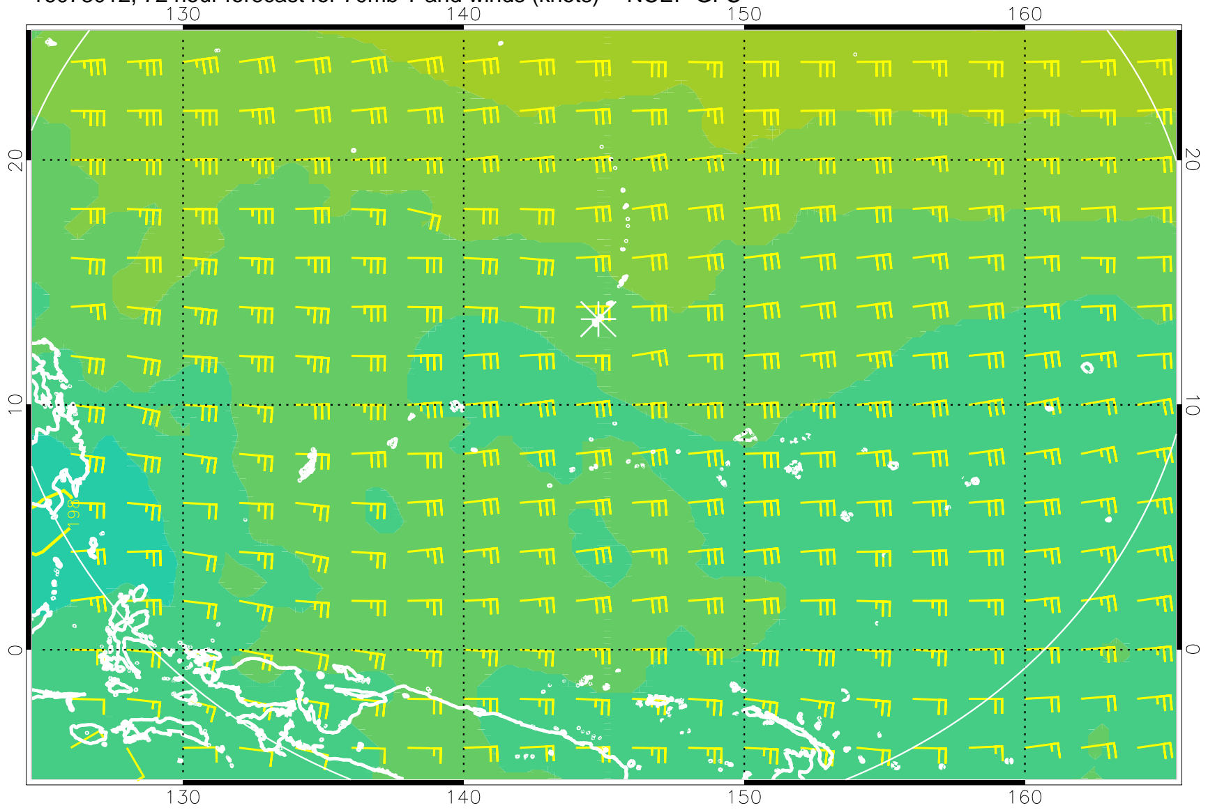
16073012, 72 hour forecast for 70mb T and winds (knots) -- NCEP GFS
