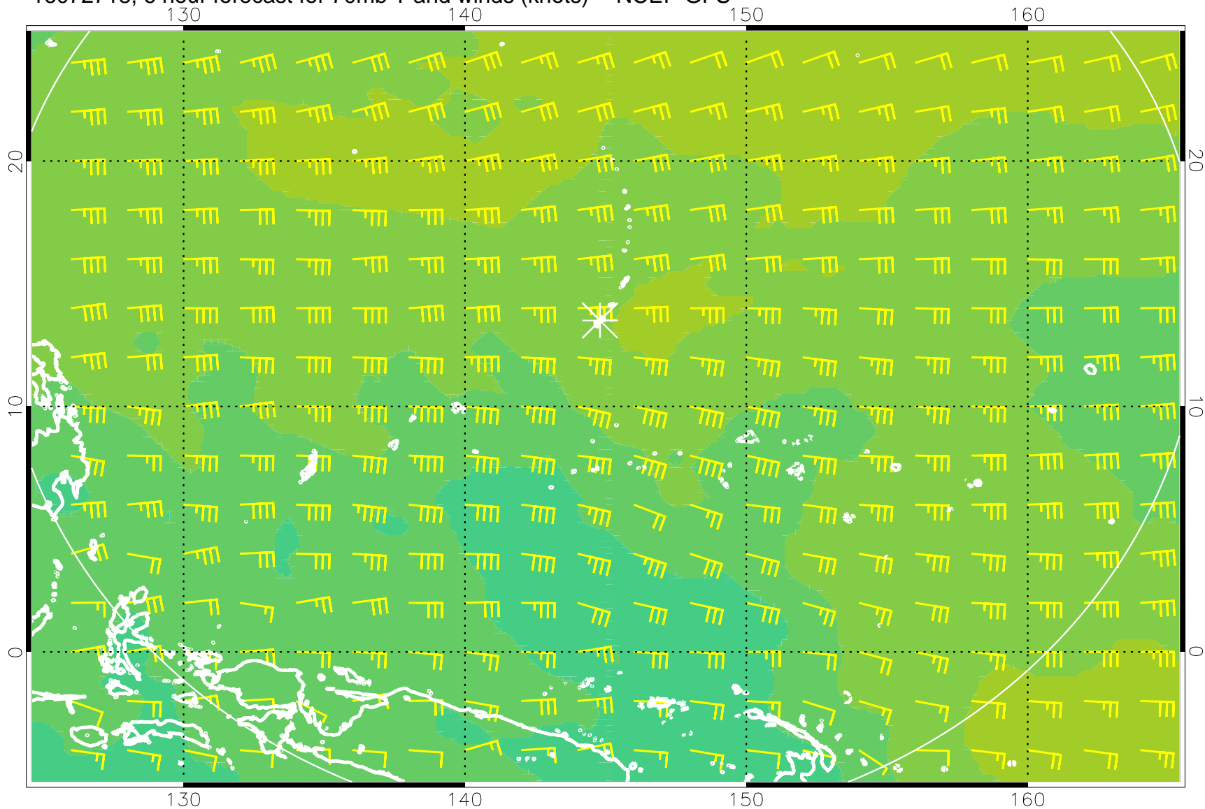
16072718, 6 hour forecast for 70mb T and winds (knots) -- NCEP GFS
