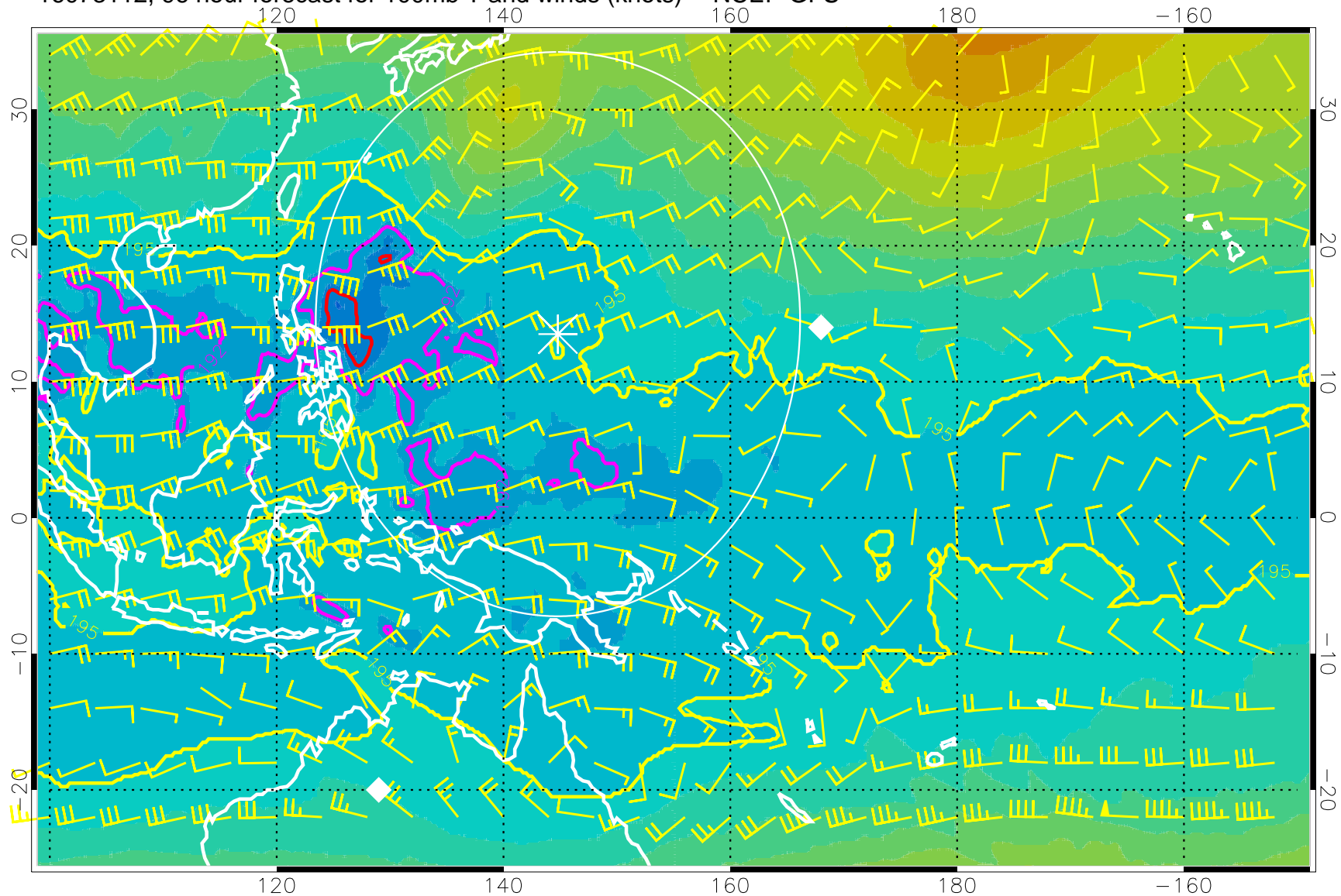
16073112, 96 hour forecast for 100mb T and winds (knots) -- NCEP GFS
