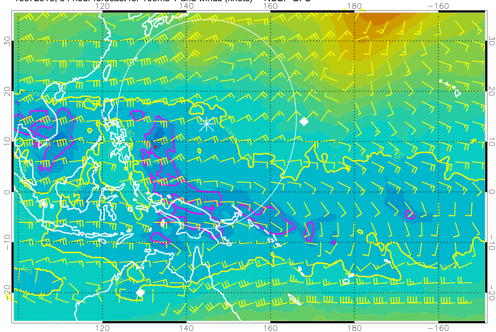
16072918, 54 hour forecast for 100mb T and winds (knots) -- NCEP GFS
