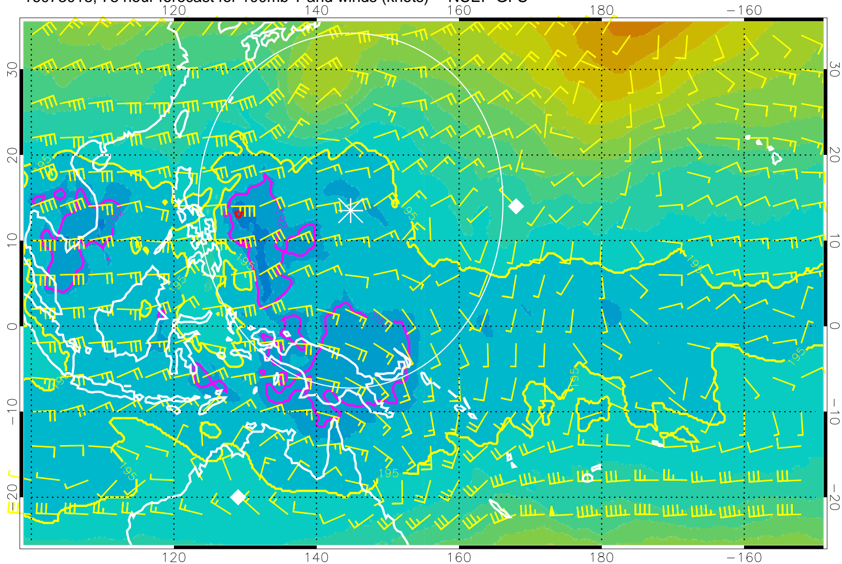
16073018, 78 hour forecast for 100mb T and winds (knots) -- NCEP GFS
