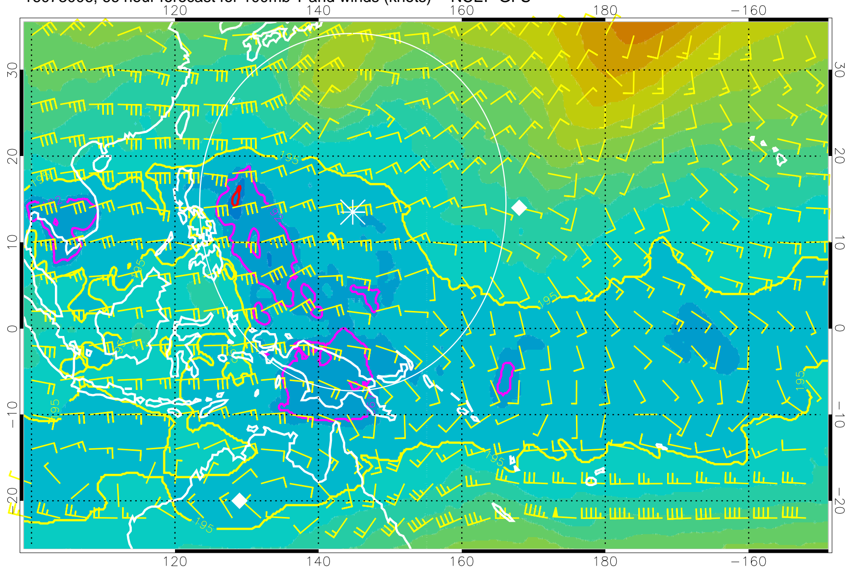
16073006, 66 hour forecast for 100mb T and winds (knots) -- NCEP GFS
