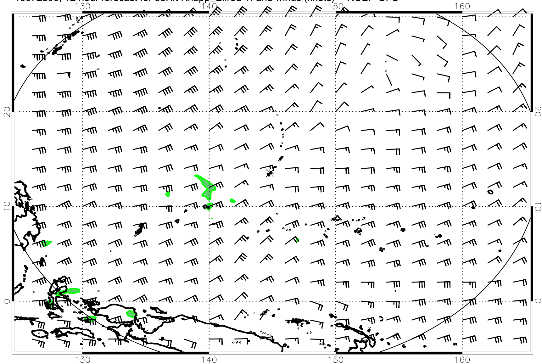
16072800, 12 hour forecast for 53Kft Knapp_Ellrod TI and winds (knots) -- NCEP GFS
