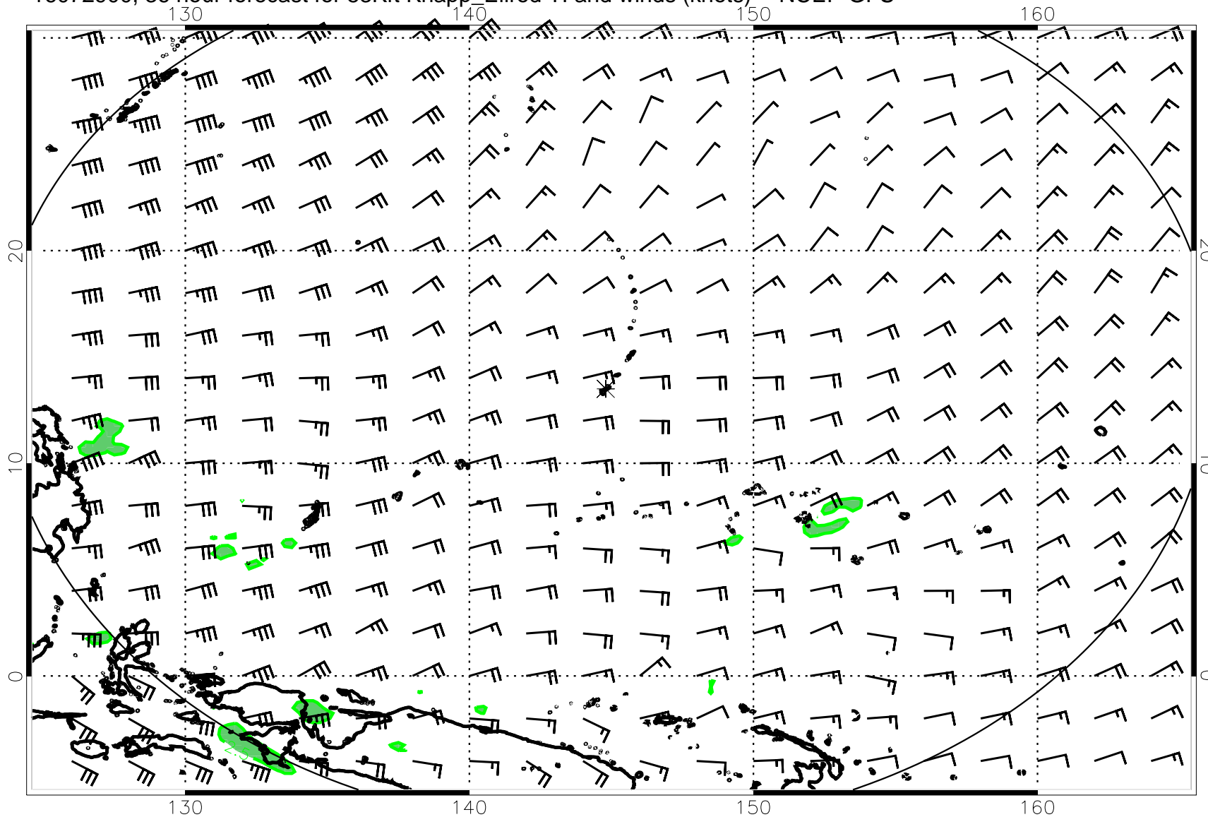
16072900, 36 hour forecast for 53Kft Knapp_Ellrod TI and winds (knots) -- NCEP GFS
