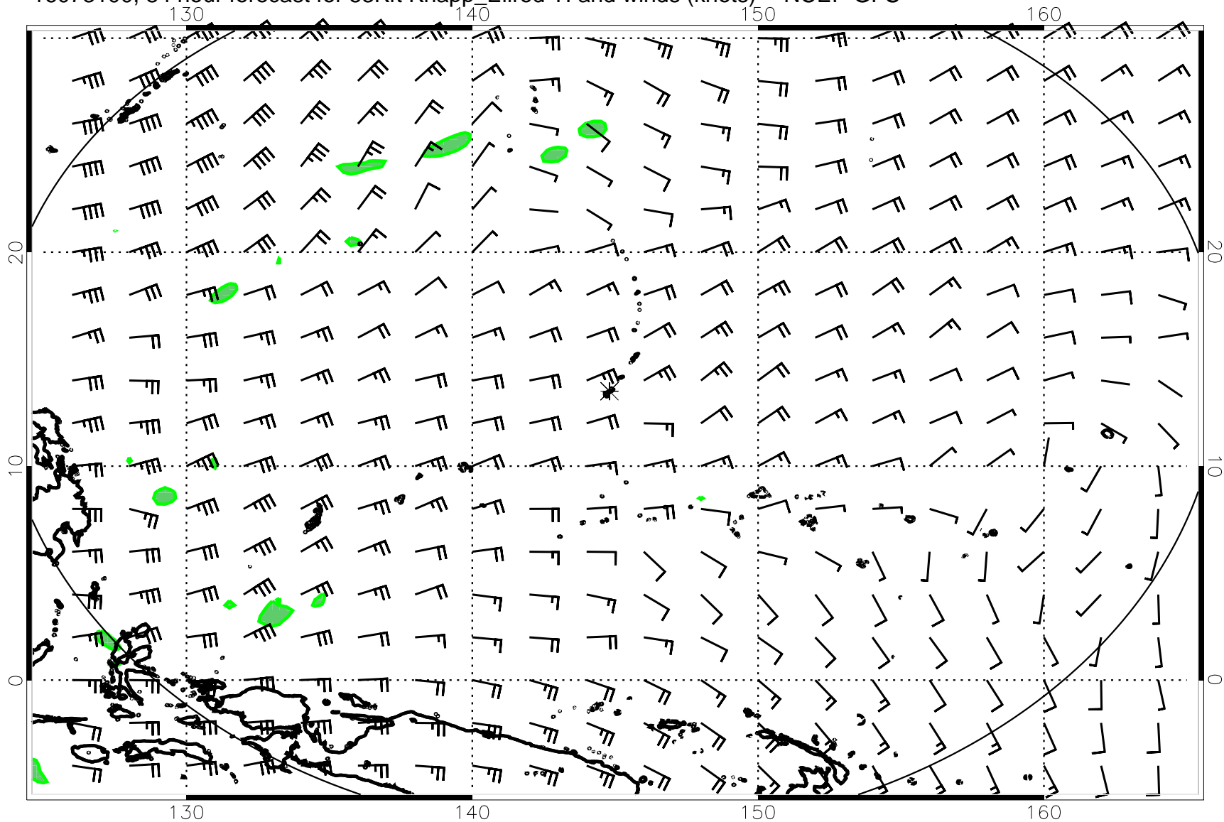
16073100, 84 hour forecast for 53Kft Knapp_Ellrod TI and winds (knots) -- NCEP GFS
