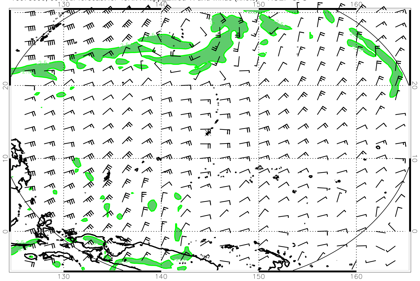
16073000, 60 hour forecast for 49Kft Knapp_Ellrod TI and winds (knots) -- NCEP GFS
