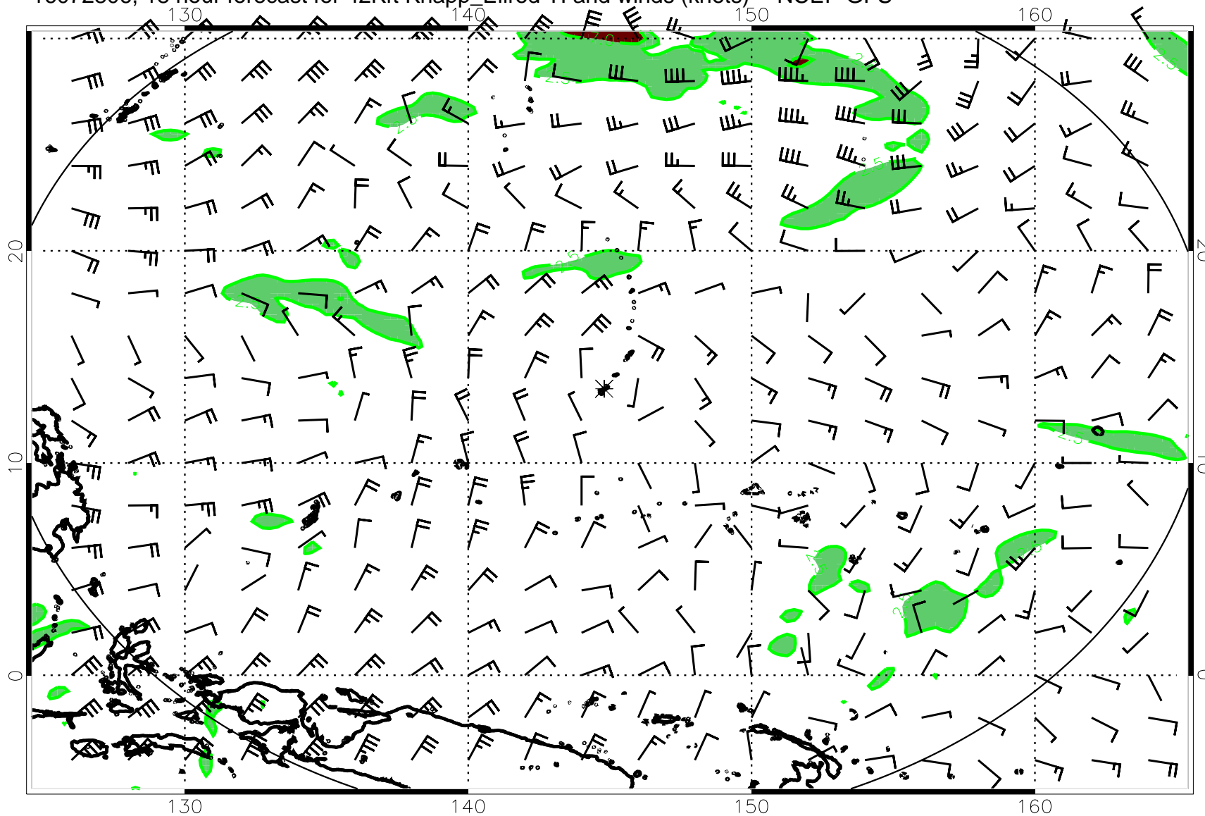
16072806, 18 hour forecast for 42Kft Knapp_Ellrod TI and winds (knots) -- NCEP GFS
