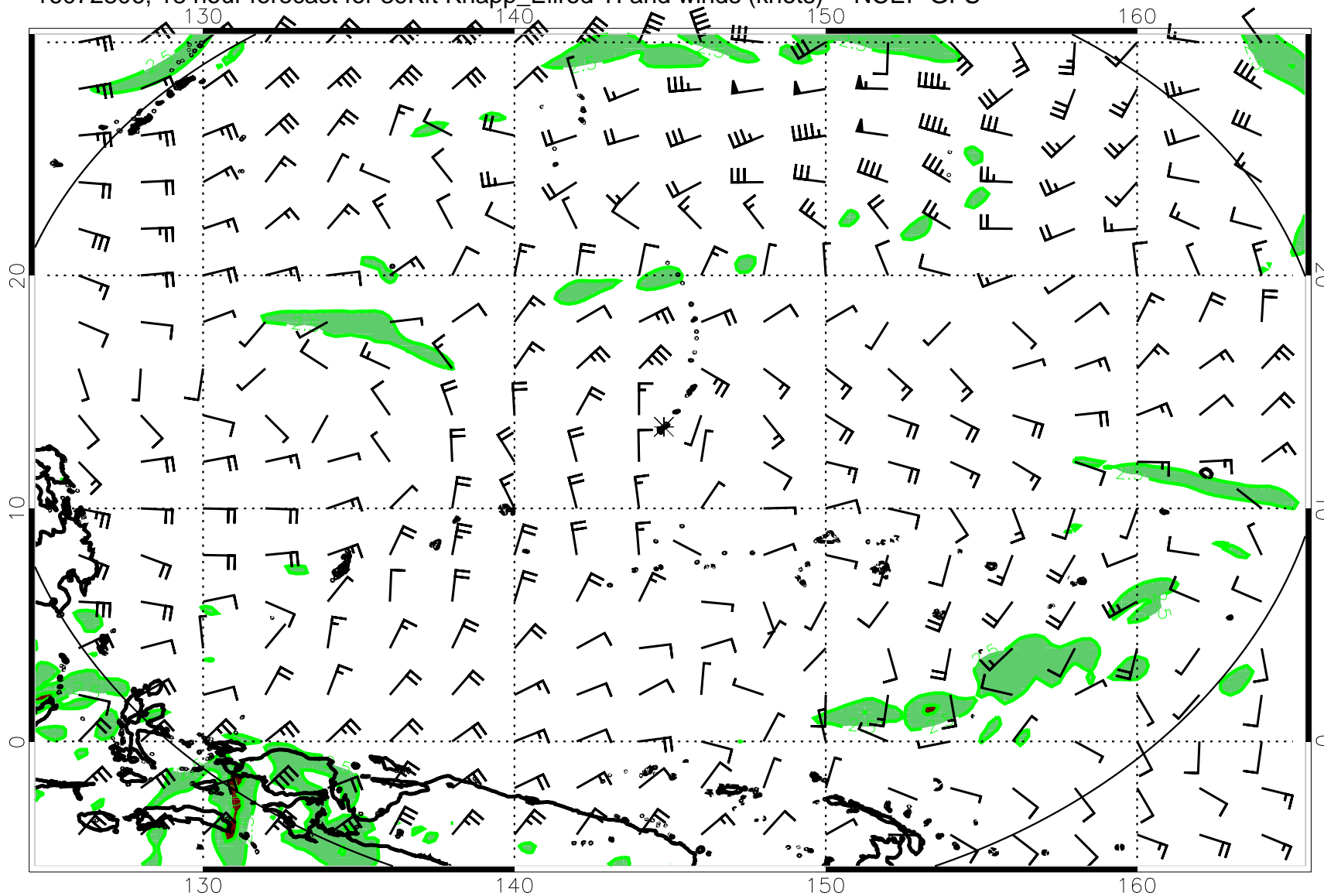
16072806, 18 hour forecast for 39Kft Knapp_Ellrod TI and winds (knots) -- NCEP GFS
