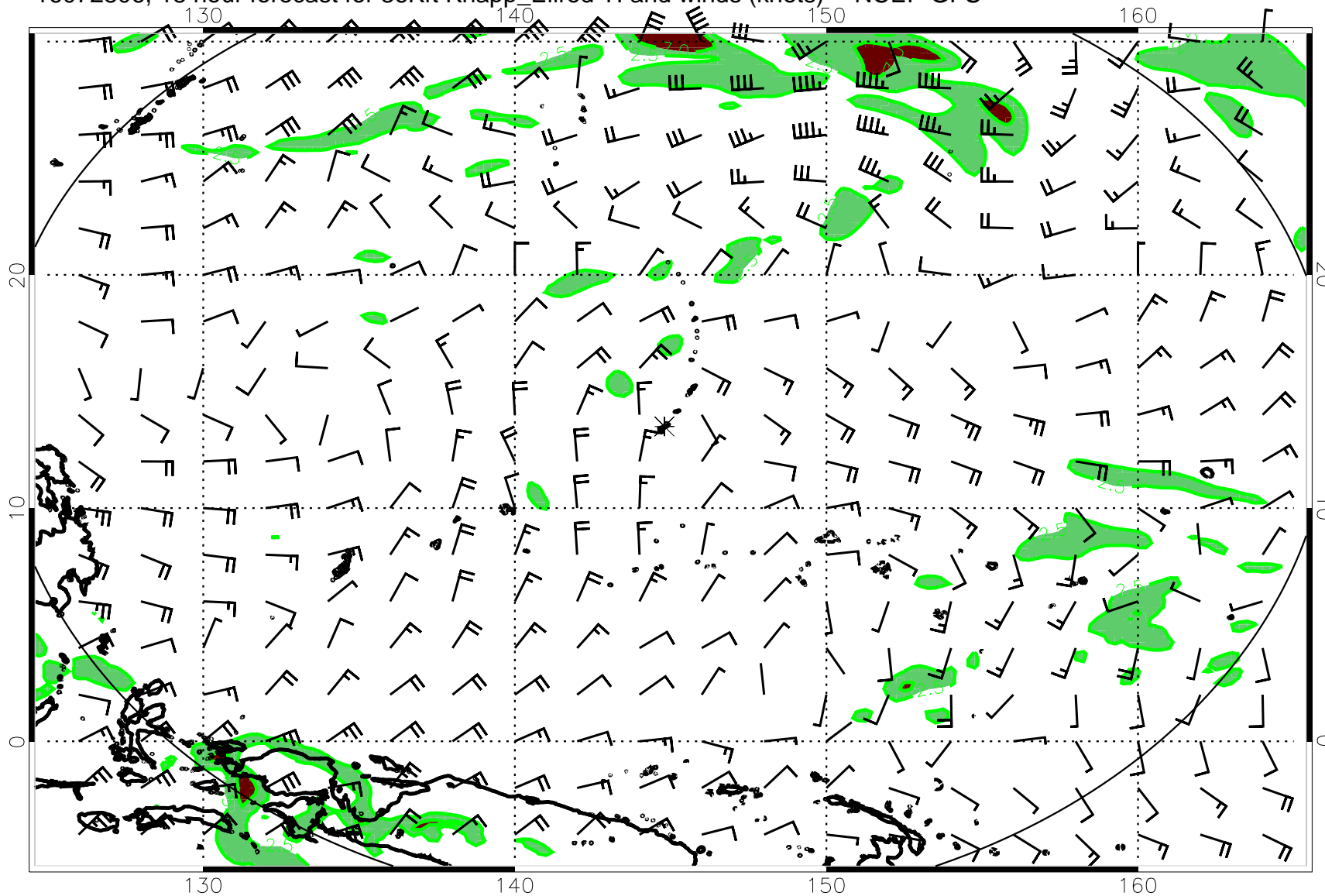
16072806, 18 hour forecast for 36Kft Knapp_Ellrod TI and winds (knots) -- NCEP GFS
