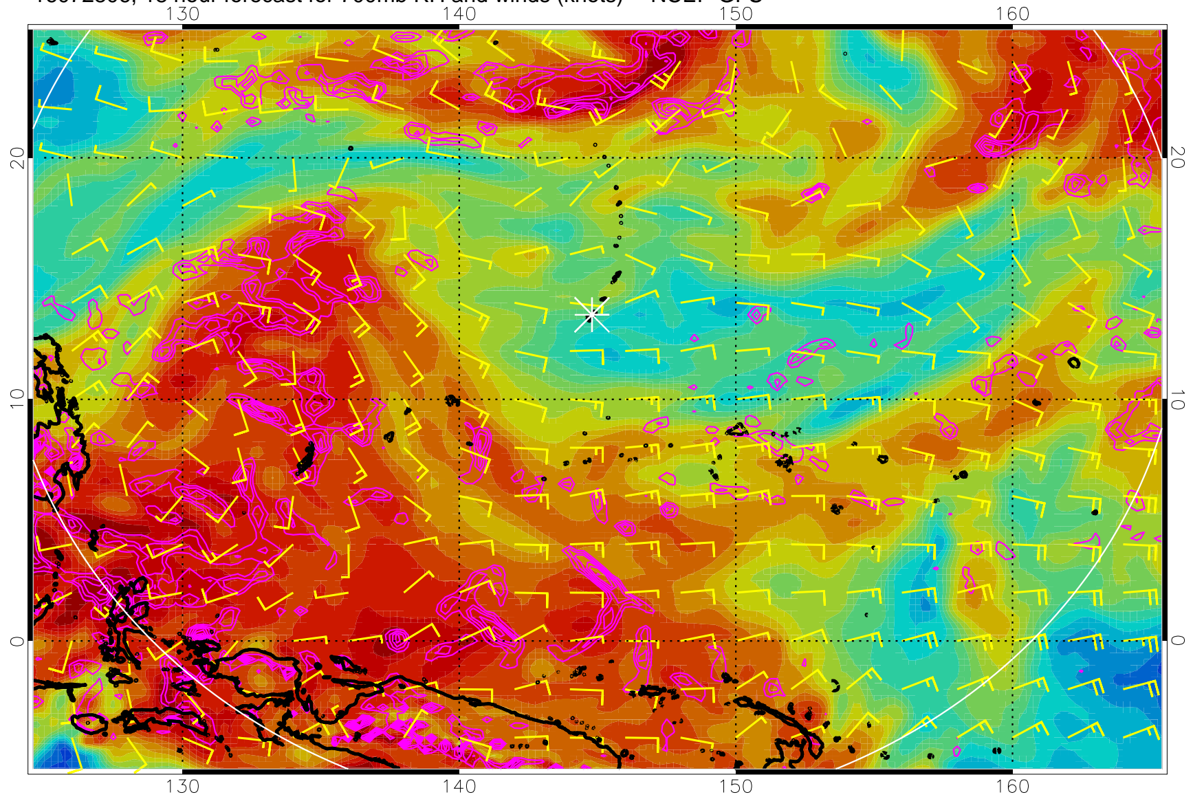
16072806, 18 hour forecast for 700mb RH and winds (knots) -- NCEP GFS
