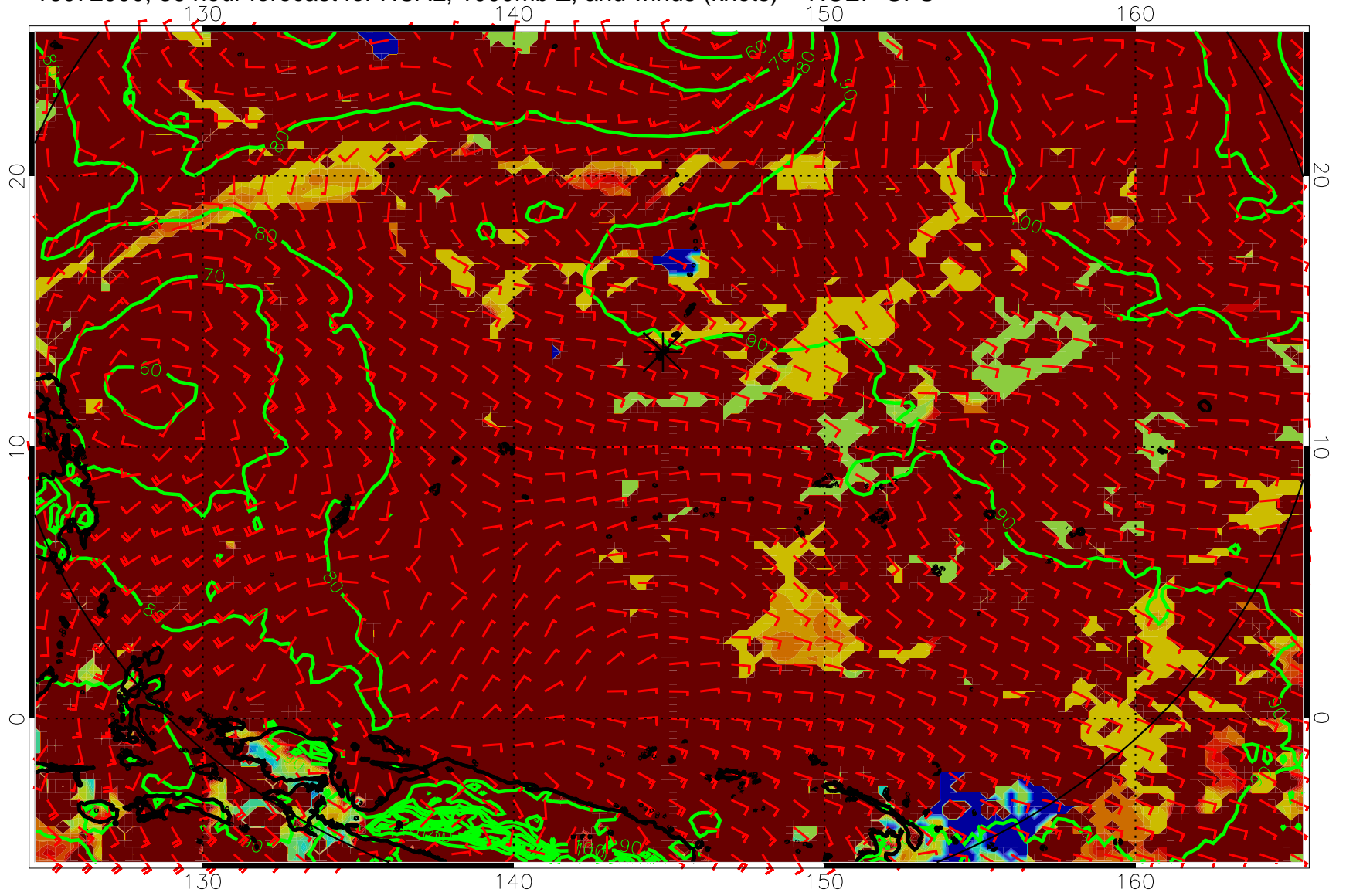
16072900, 36 hour forecast for HCAL, 1000mb Z, and winds (knots) -- NCEP GFS
