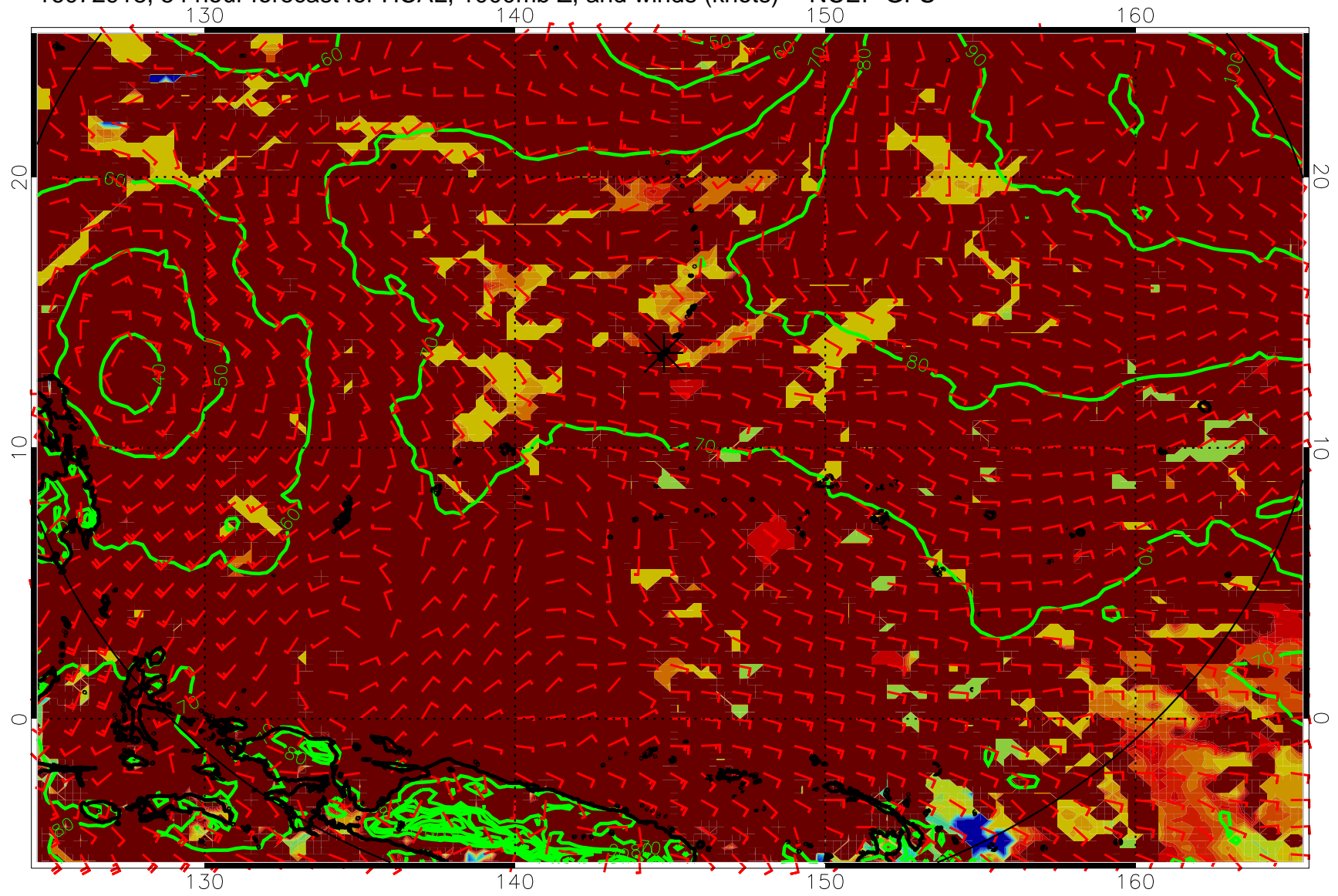
16072918, 54 hour forecast for HCAL, 1000mb Z, and winds (knots) -- NCEP GFS
