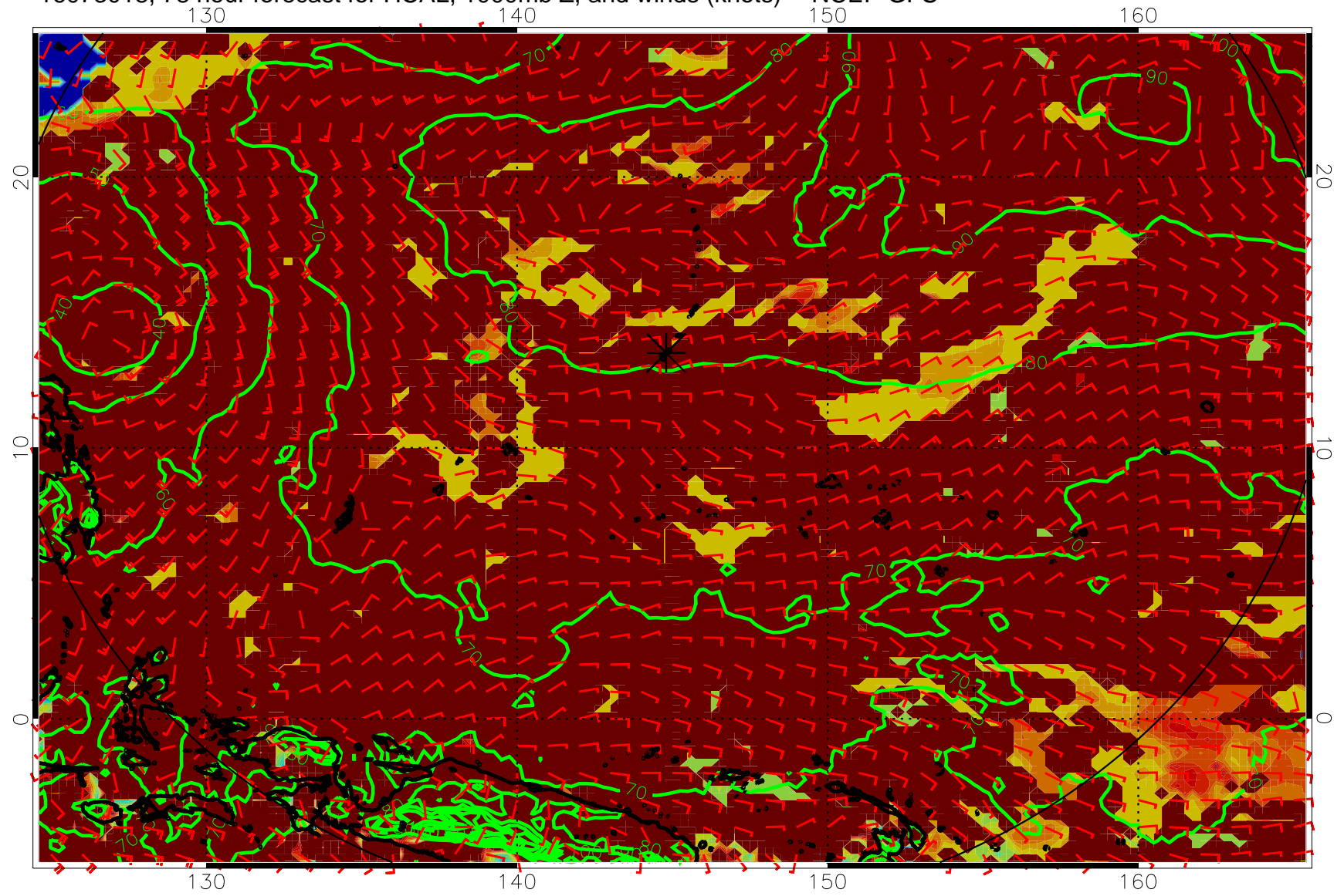
16073018, 78 hour forecast for HCAL, 1000mb Z, and winds (knots) -- NCEP GFS
