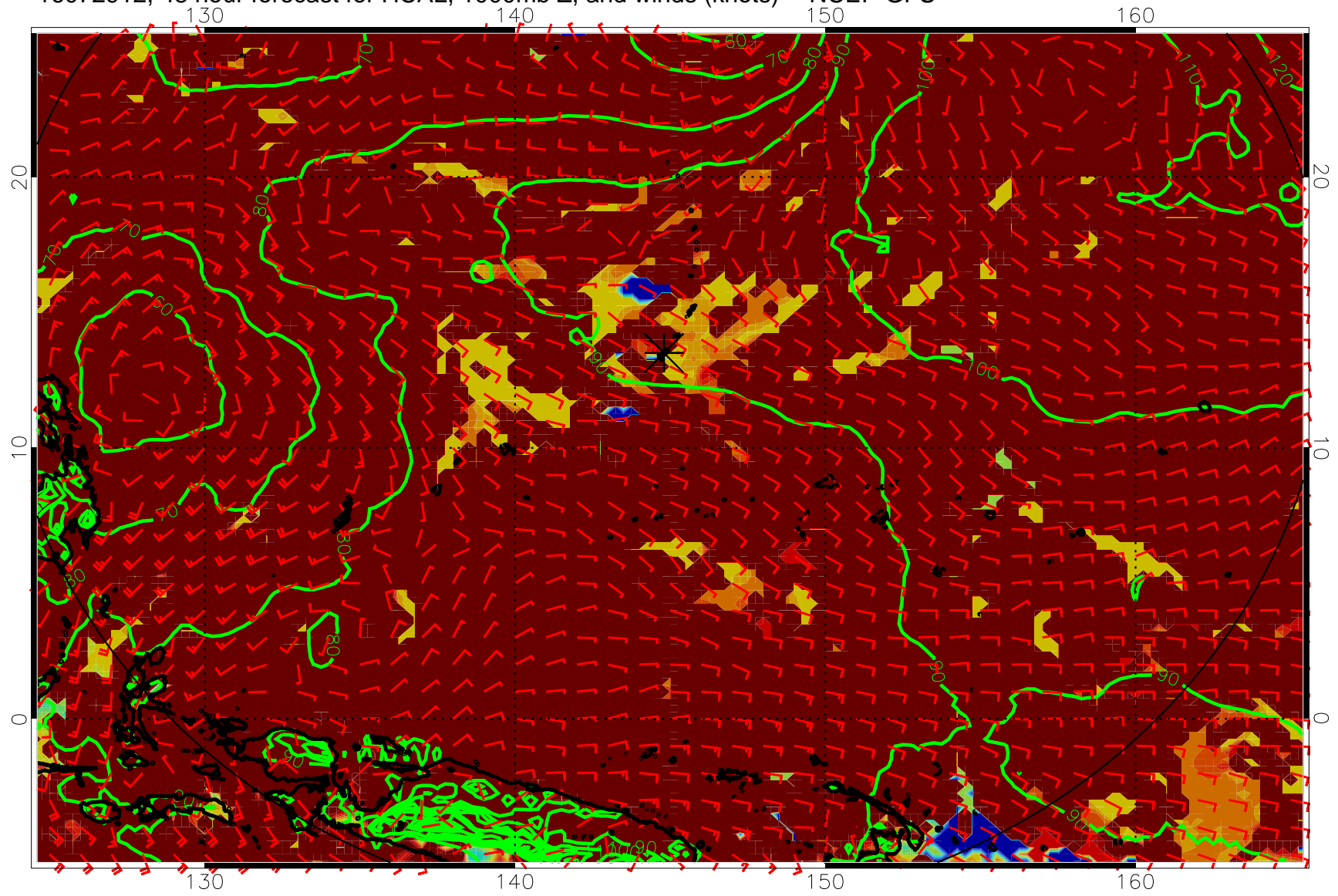
16072912, 48 hour forecast for HCAL, 1000mb Z, and winds (knots) -- NCEP GFS
