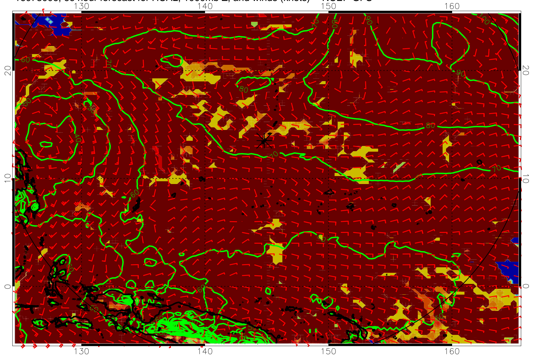
16073006, 66 hour forecast for HCAL, 1000mb Z, and winds (knots) -- NCEP GFS
