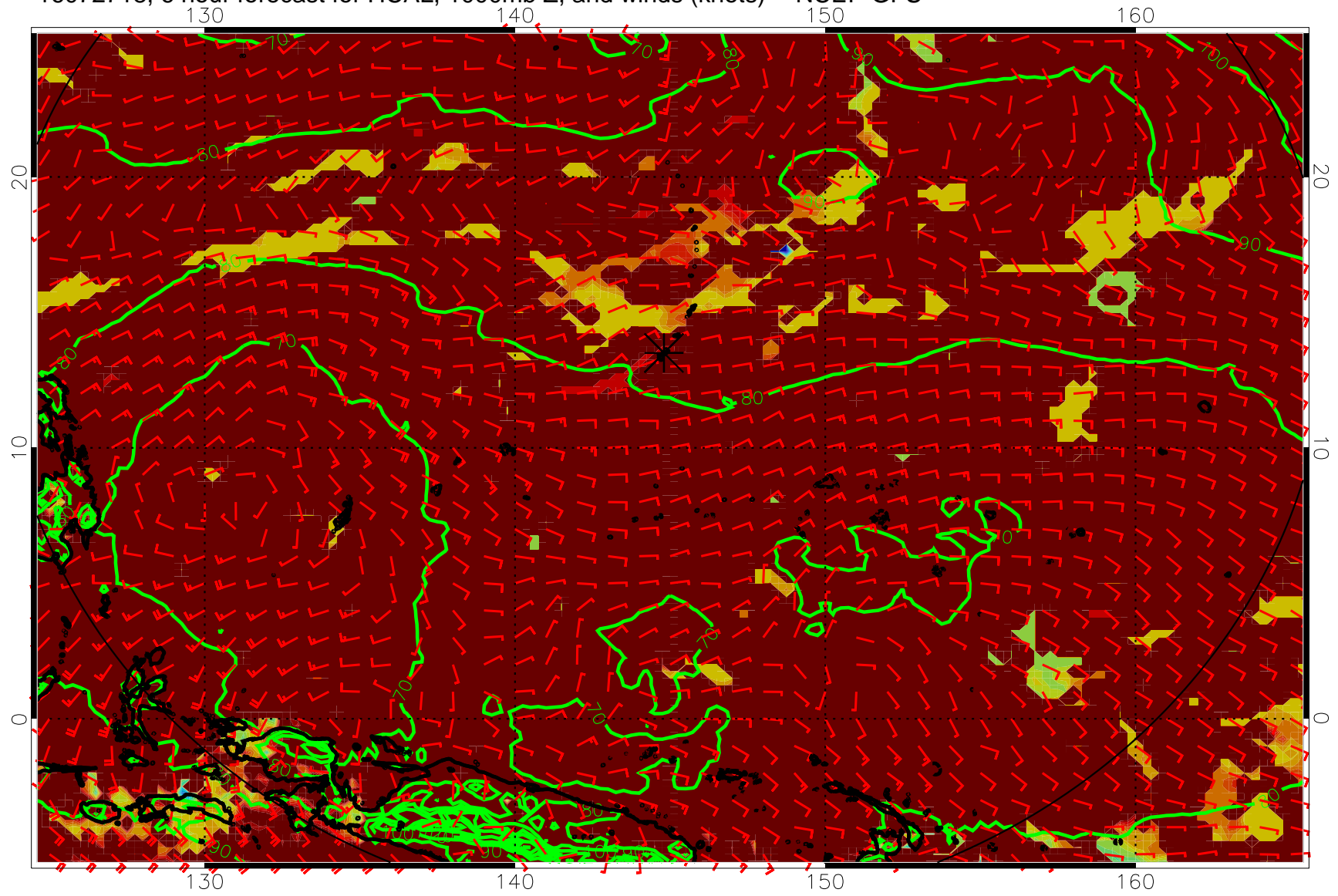
16072718, 6 hour forecast for HCAL, 1000mb Z, and winds (knots) -- NCEP GFS
