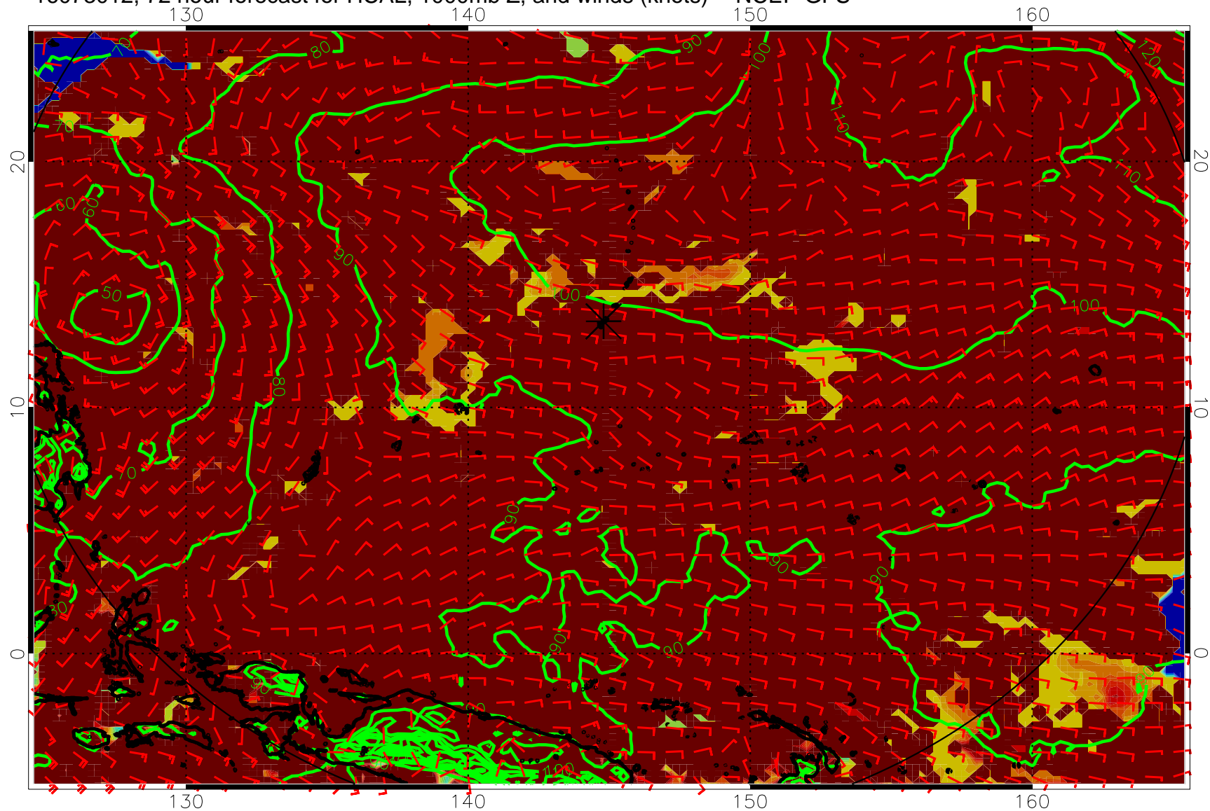
16073012, 72 hour forecast for HCAL, 1000mb Z, and winds (knots) -- NCEP GFS
