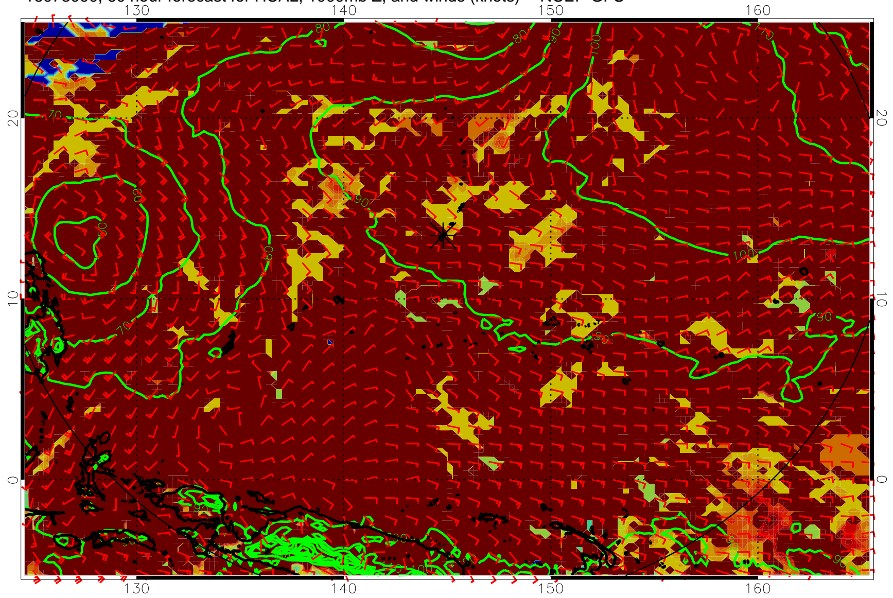
16073000, 60 hour forecast for HCAL, 1000mb Z, and winds (knots) -- NCEP GFS
