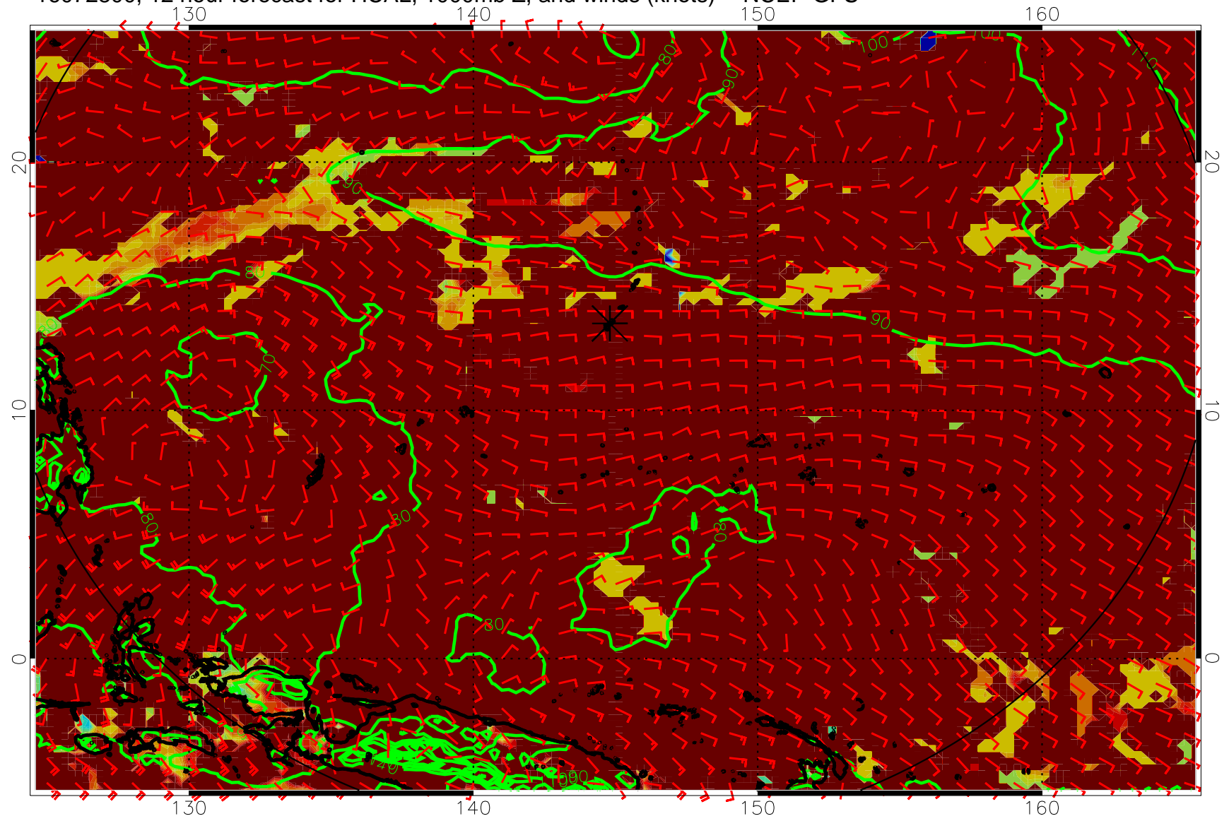
16072800, 12 hour forecast for HCAL, 1000mb Z, and winds (knots) -- NCEP GFS
