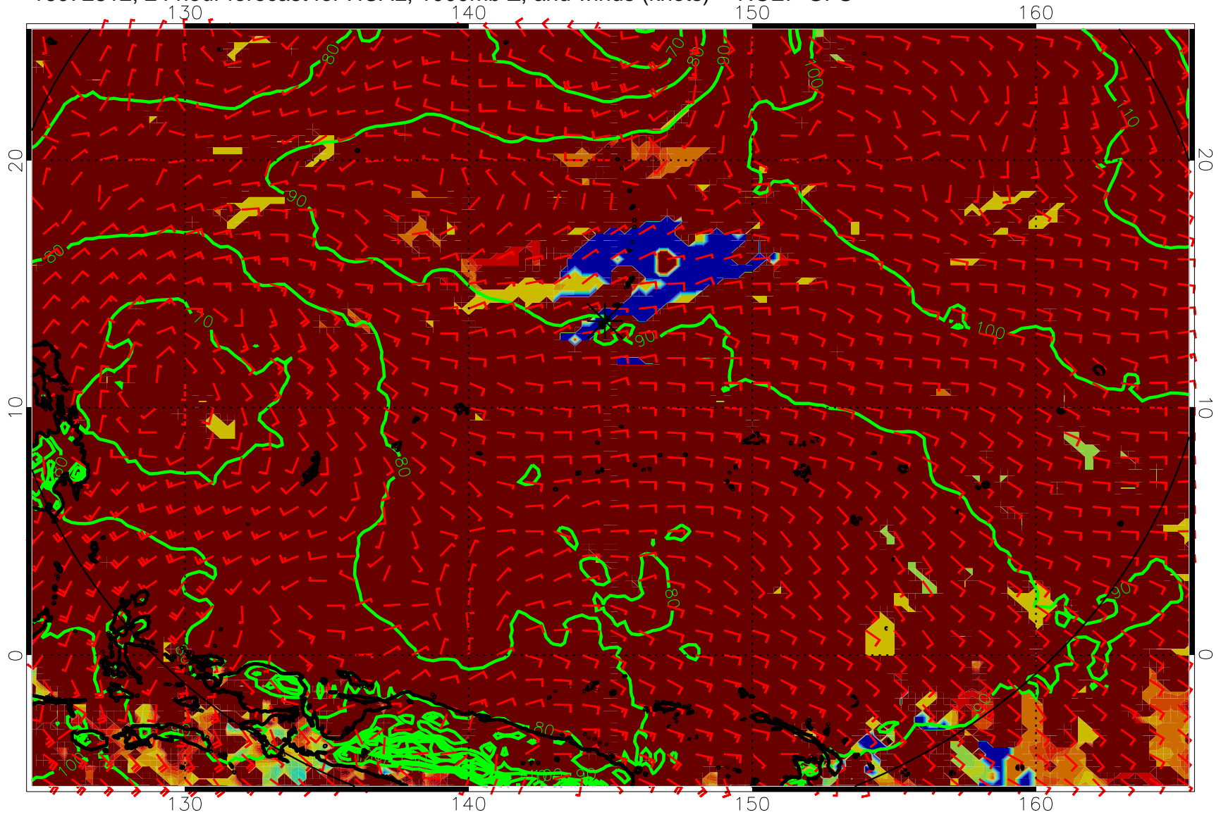
16072812, 24 hour forecast for HCAL, 1000mb Z, and winds (knots) -- NCEP GFS
