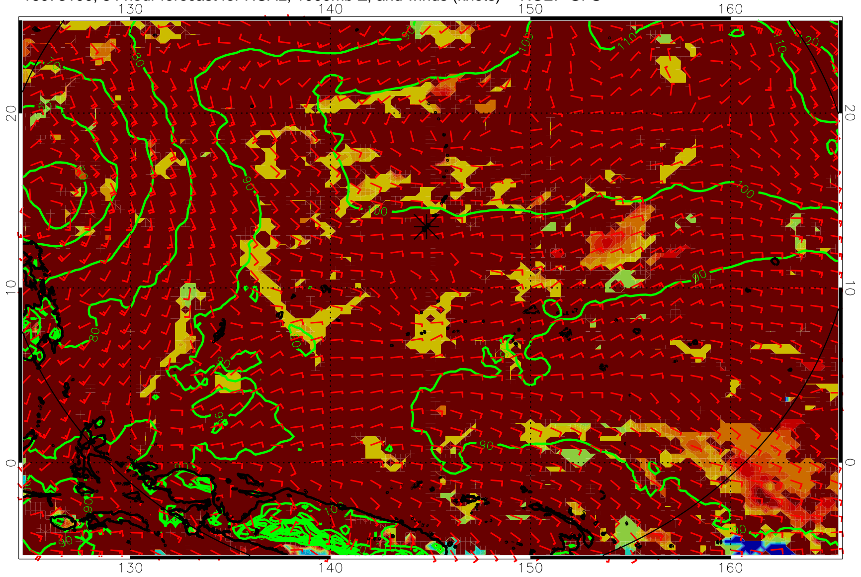
16073100, 84 hour forecast for HCAL, 1000mb Z, and winds (knots) -- NCEP GFS
