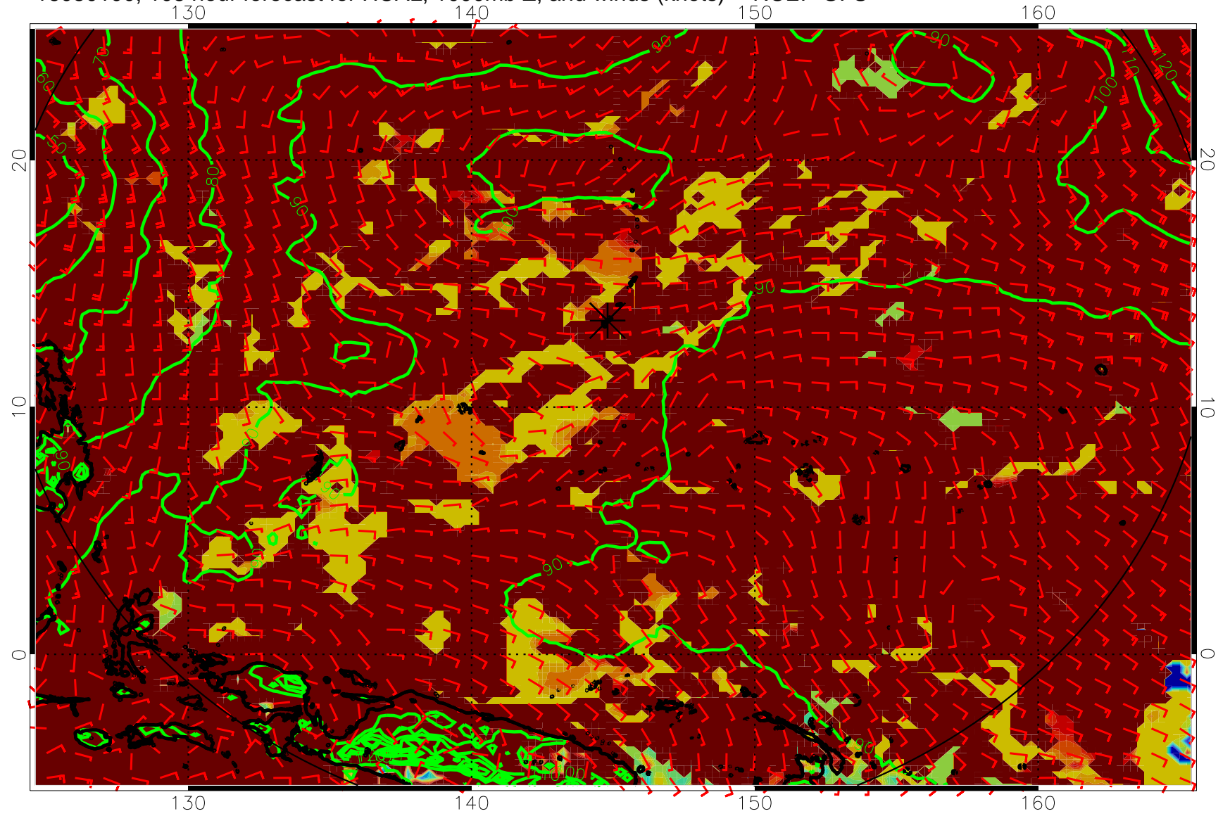
16080100, 108 hour forecast for HCAL, 1000mb Z, and winds (knots) -- NCEP GFS
