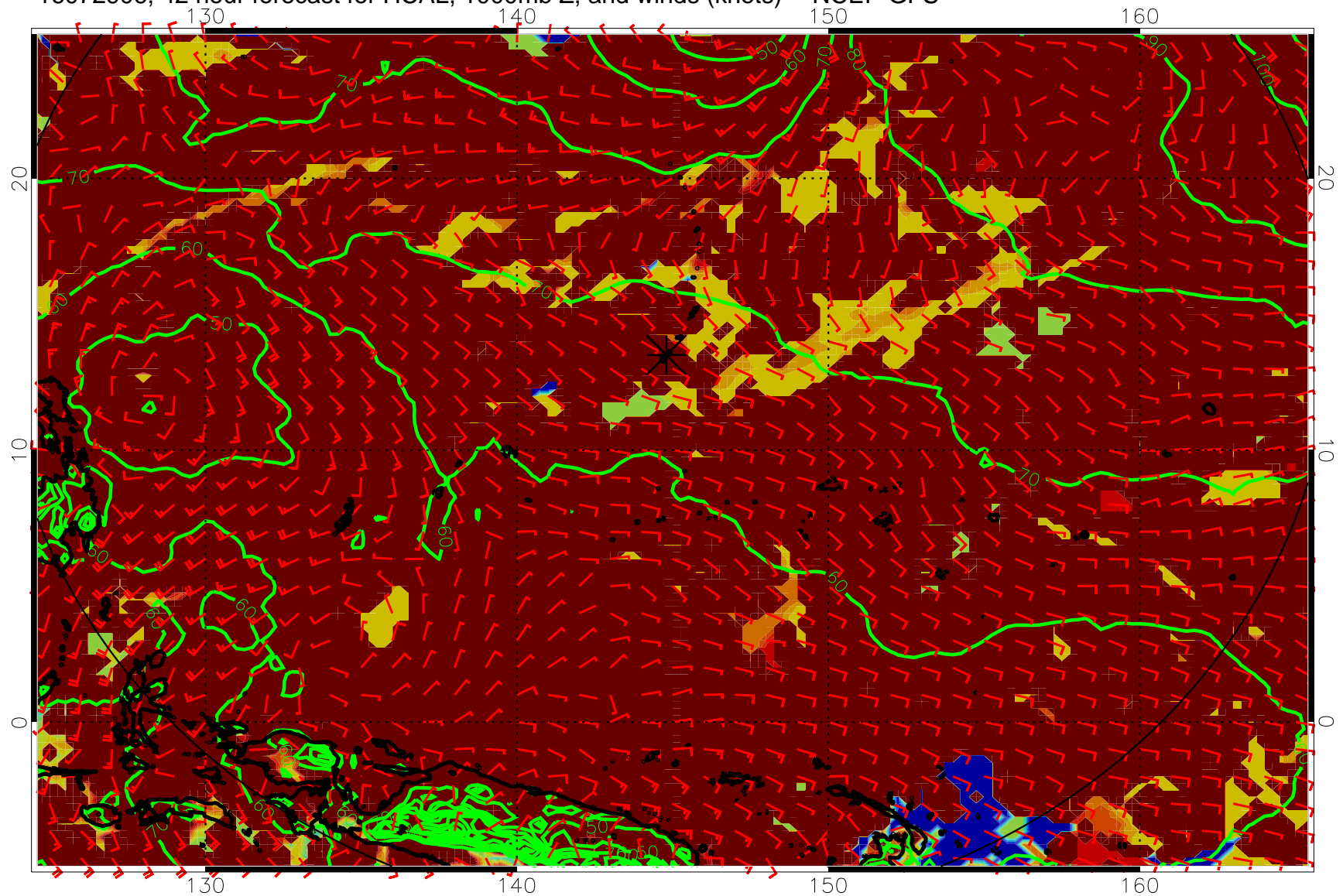
16072906, 42 hour forecast for HCAL, 1000mb Z, and winds (knots) -- NCEP GFS
