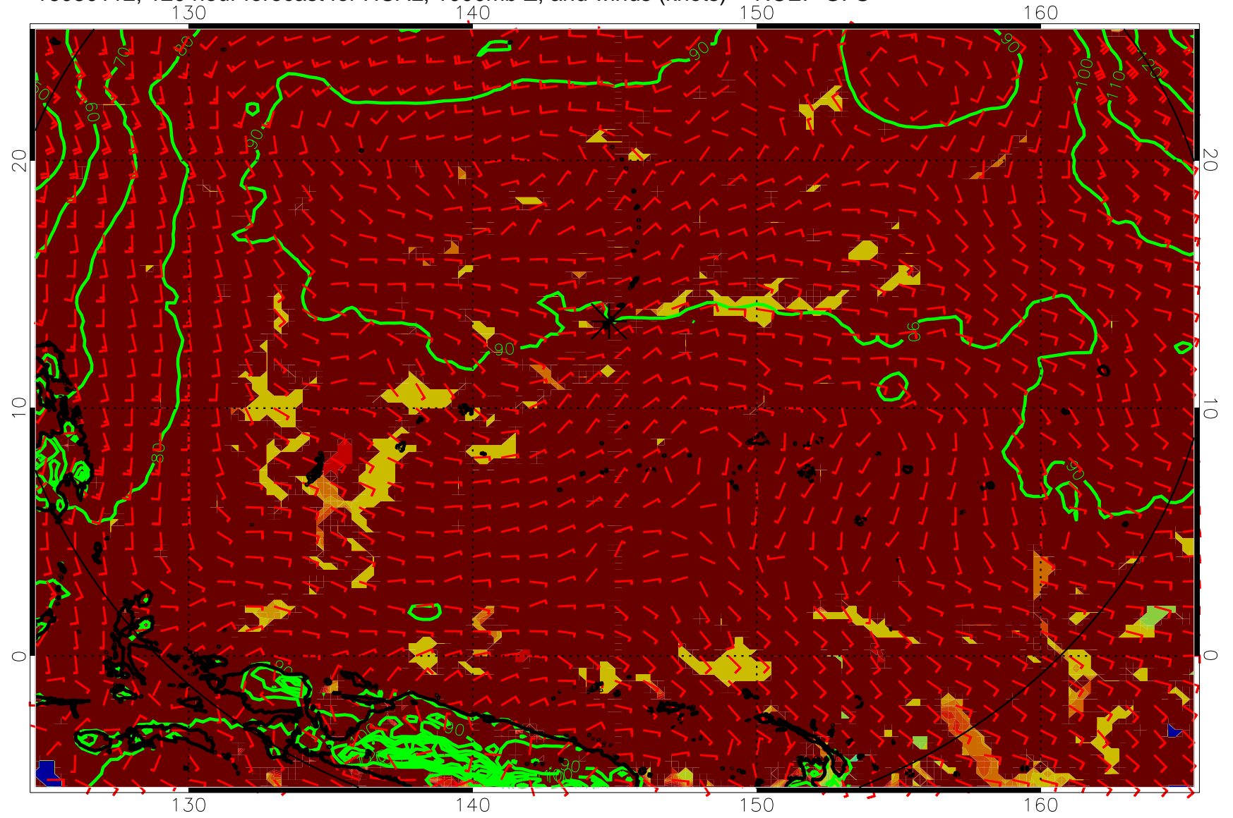
16080112, 120 hour forecast for HCAL, 1000mb Z, and winds (knots) -- NCEP GFS
