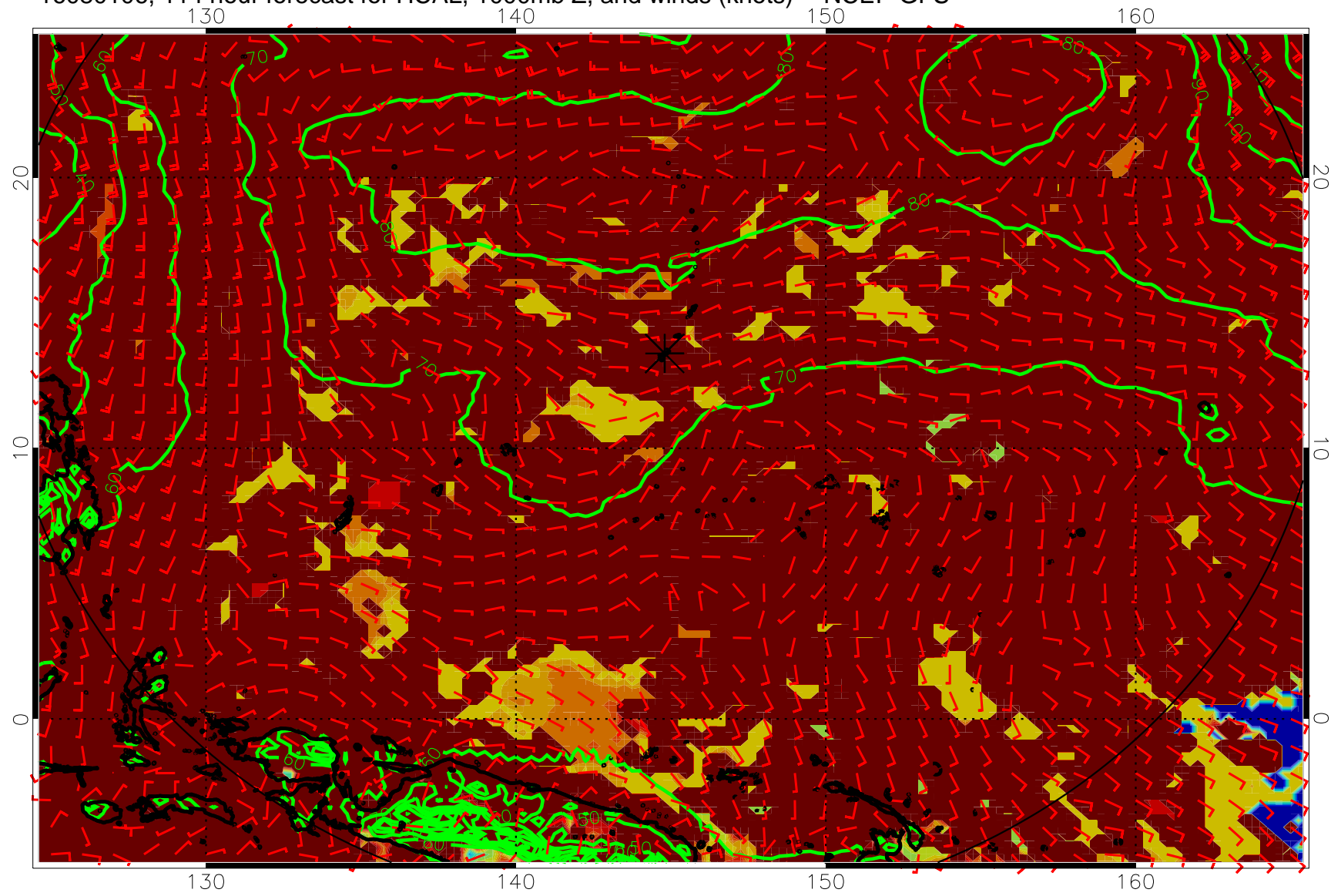
16080106, 114 hour forecast for HCAL, 1000mb Z, and winds (knots) -- NCEP GFS
