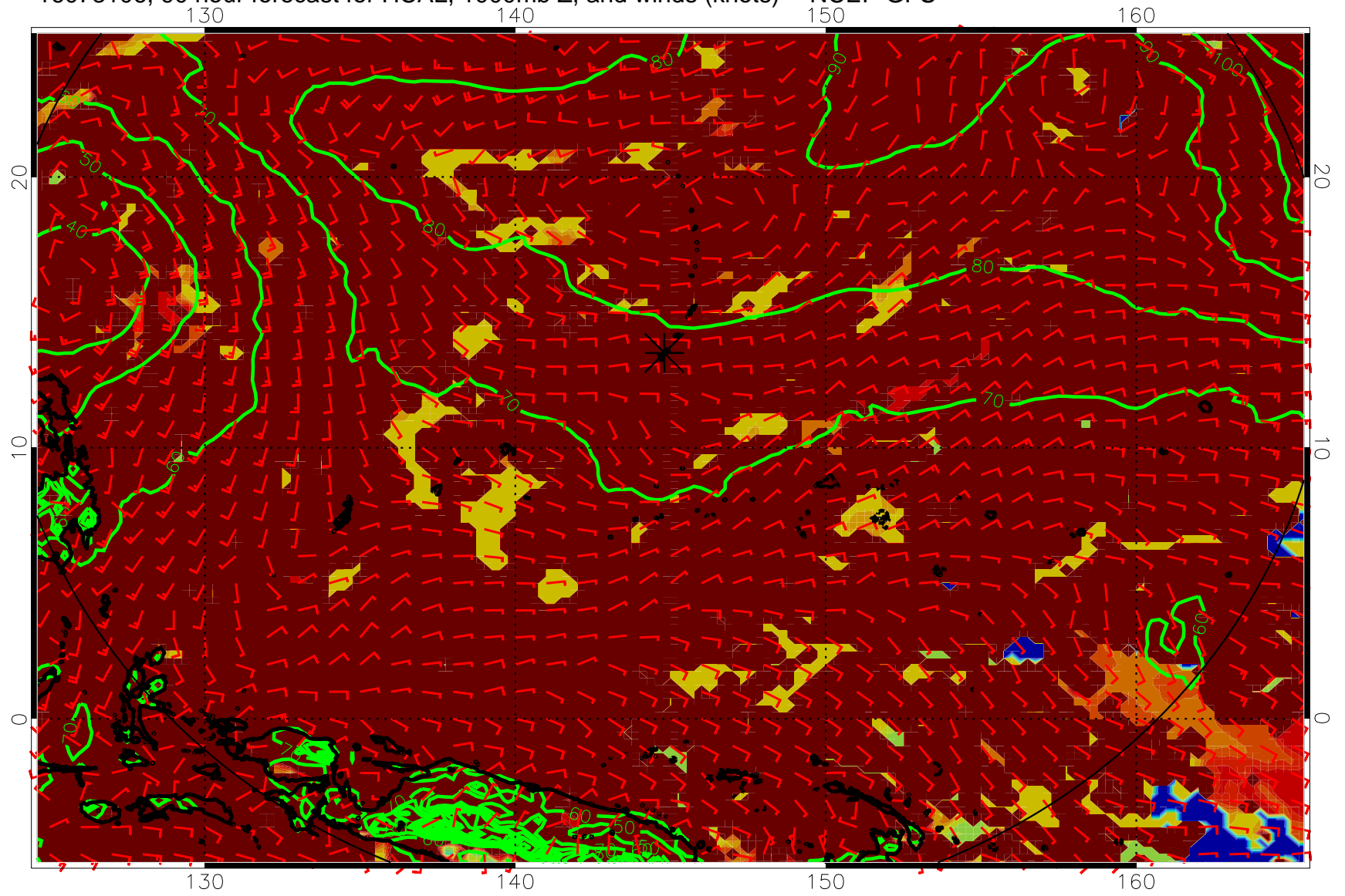
16073106, 90 hour forecast for HCAL, 1000mb Z, and winds (knots) -- NCEP GFS
