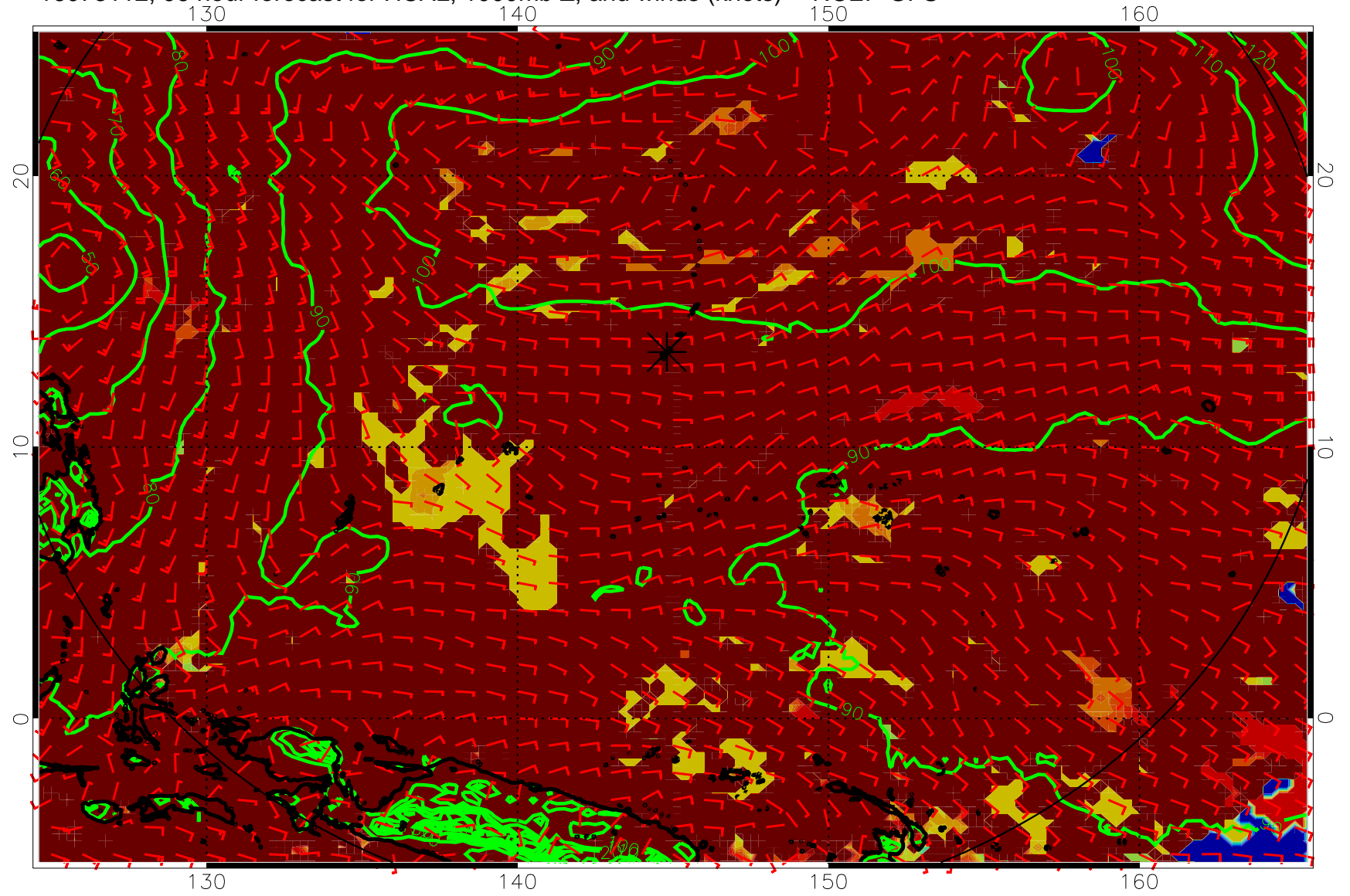
16073112, 96 hour forecast for HCAL, 1000mb Z, and winds (knots) -- NCEP GFS
