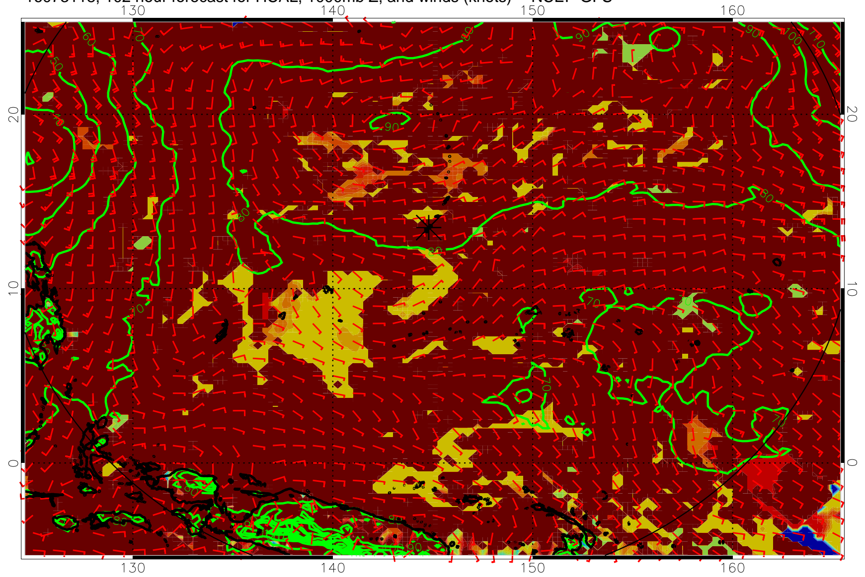
16073118, 102 hour forecast for HCAL, 1000mb Z, and winds (knots) -- NCEP GFS
