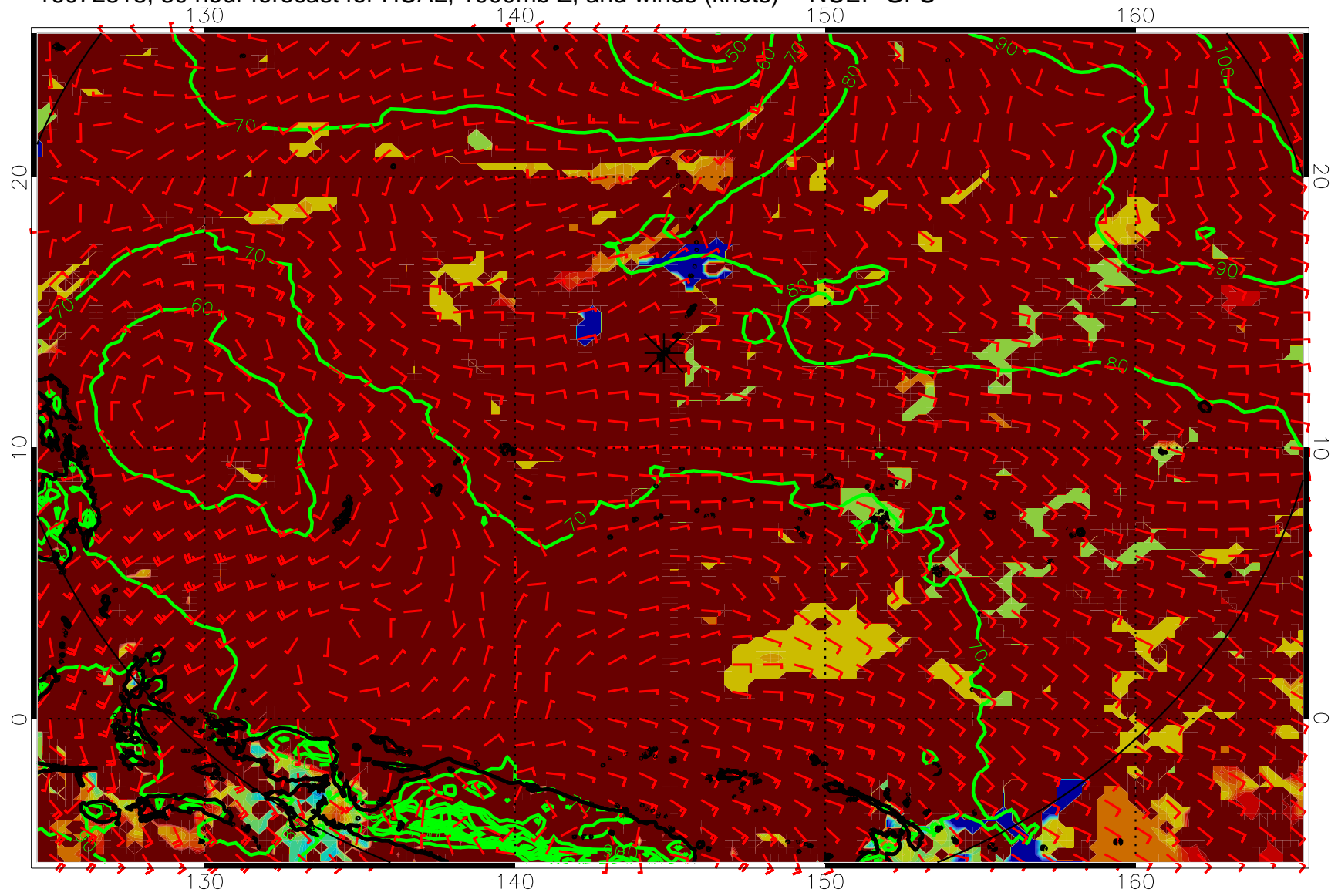
16072818, 30 hour forecast for HCAL, 1000mb Z, and winds (knots) -- NCEP GFS
