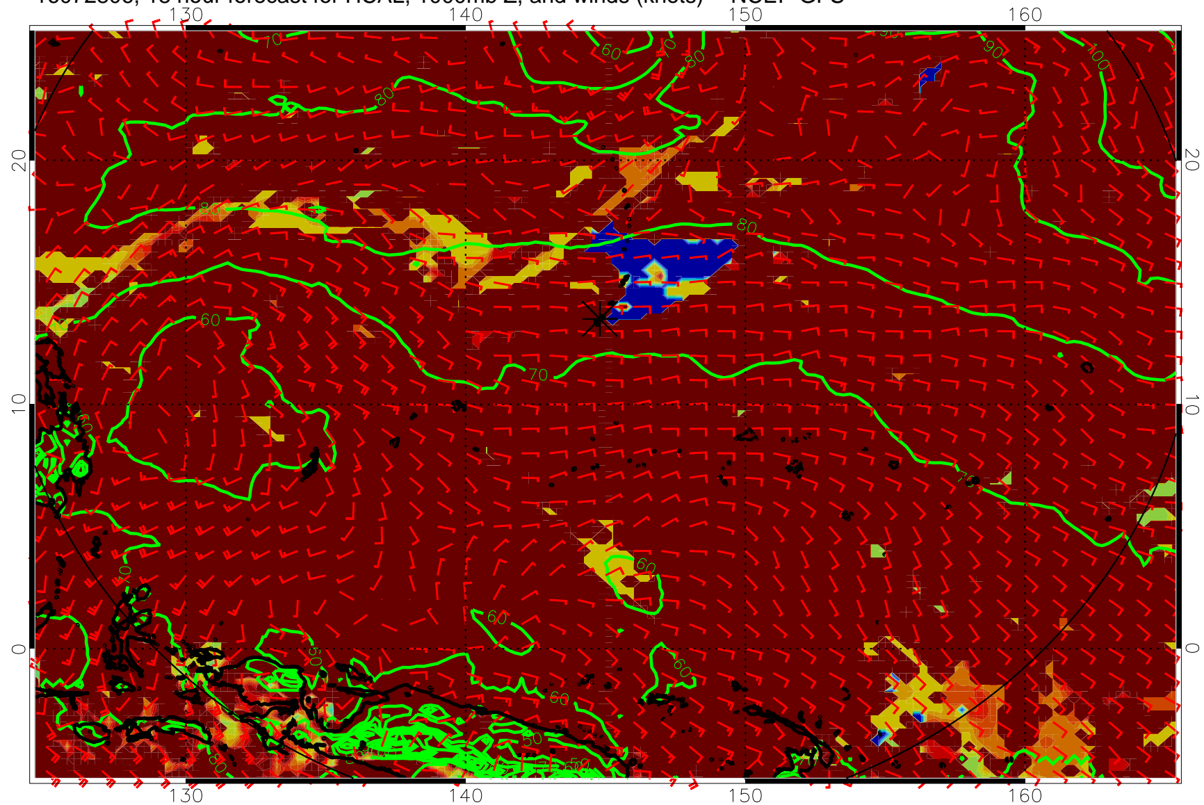
16072806, 18 hour forecast for HCAL, 1000mb Z, and winds (knots) -- NCEP GFS
