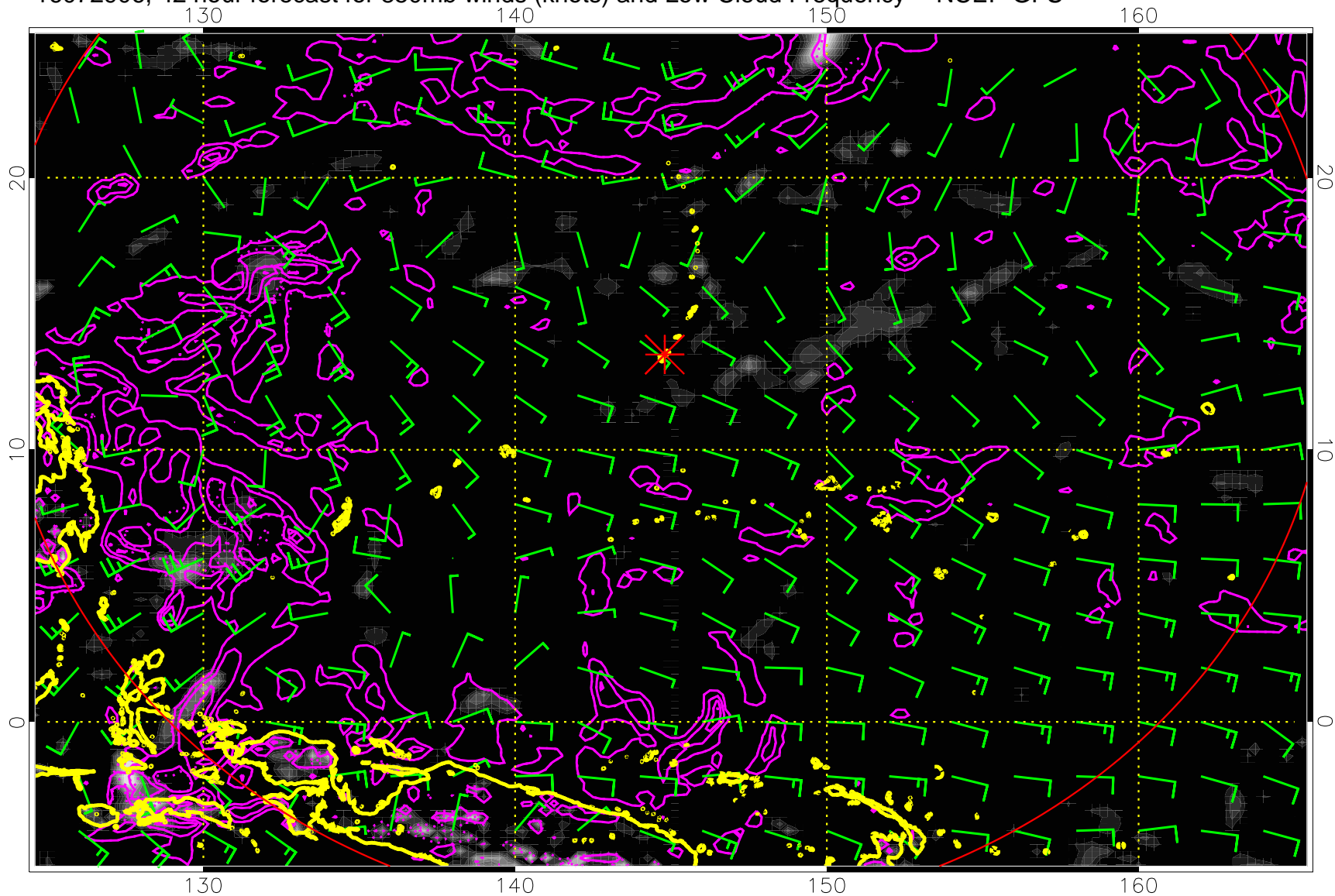
16072906, 42 hour forecast for 850mb winds (knots) and Low Cloud Frequency -- NCEP GFS
